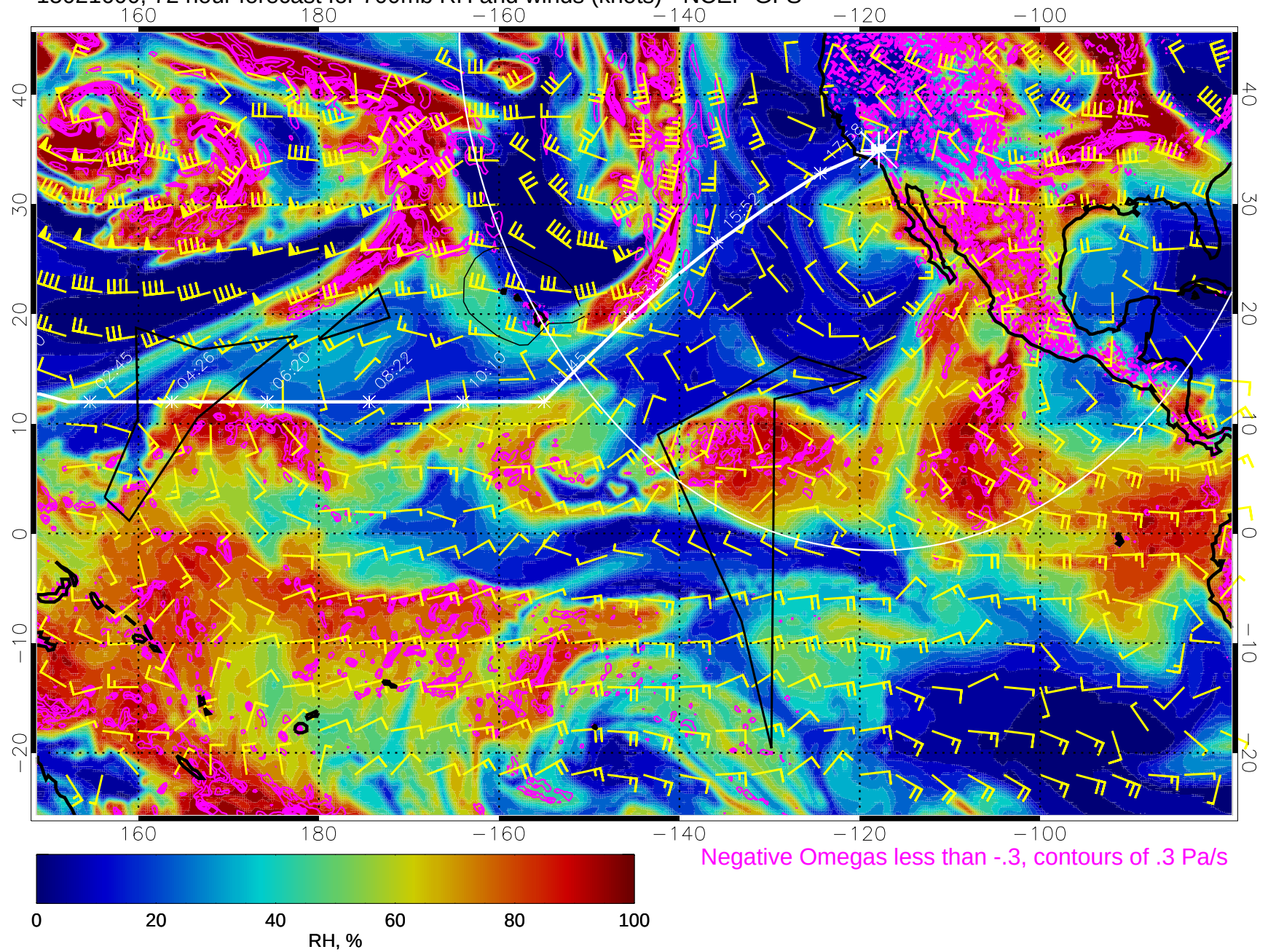
15021600, 72 hour forecast for 700mb RH and winds (knots) - NCEP GFS
