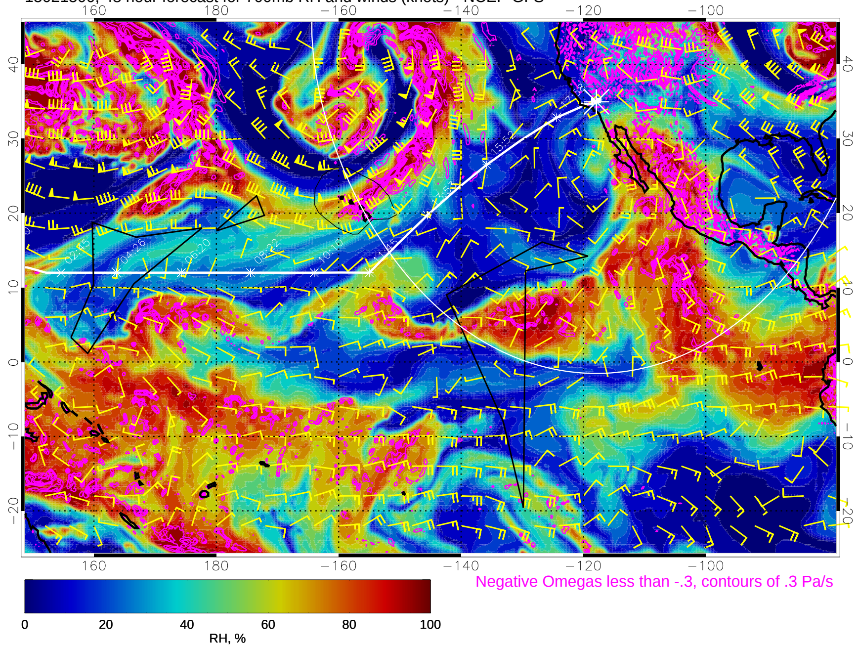
15021500, 48 hour forecast for 700mb RH and winds (knots) - NCEP GFS
