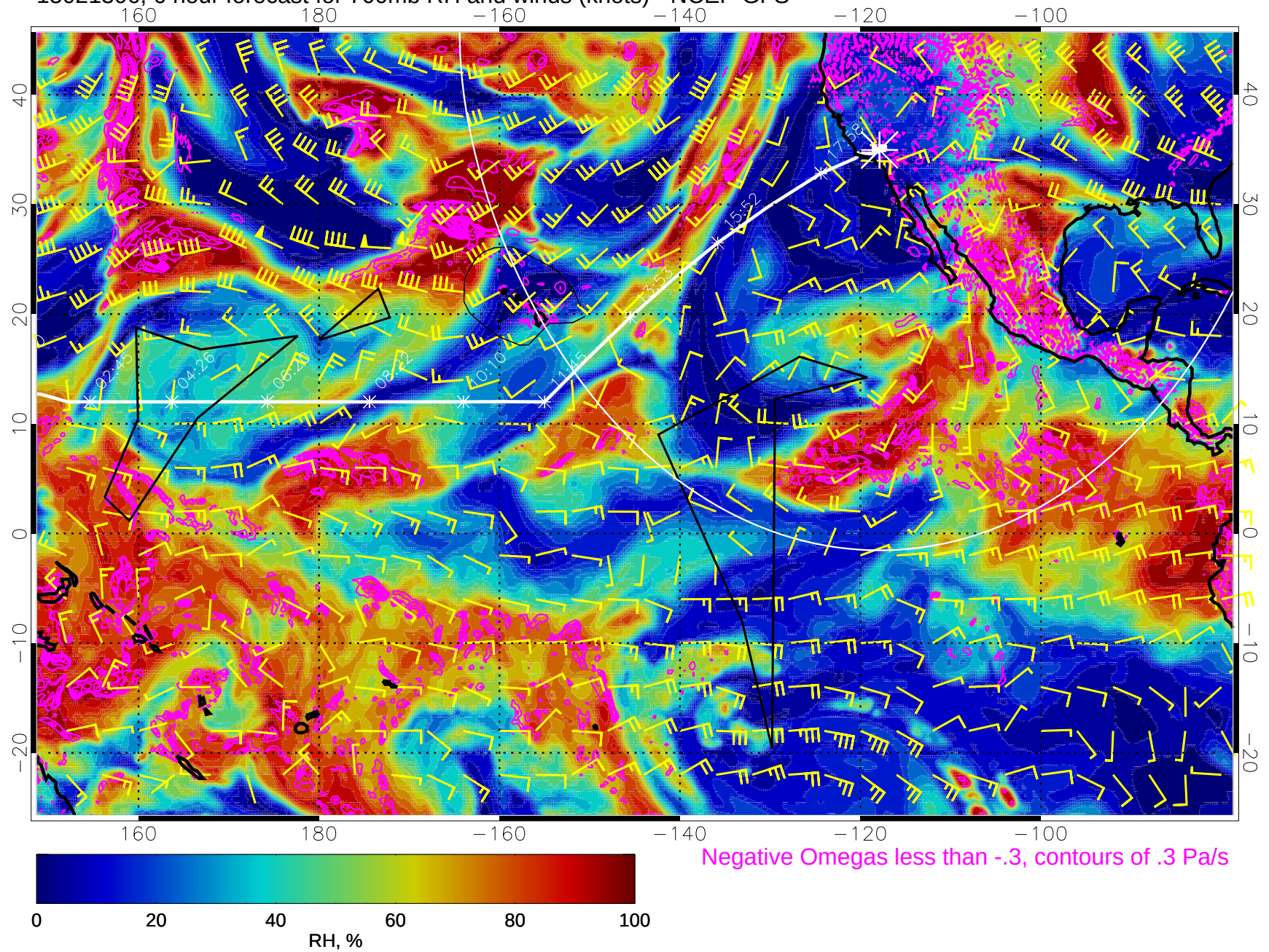
15021306, 6 hour forecast for 700mb RH and winds (knots) - NCEP GFS
