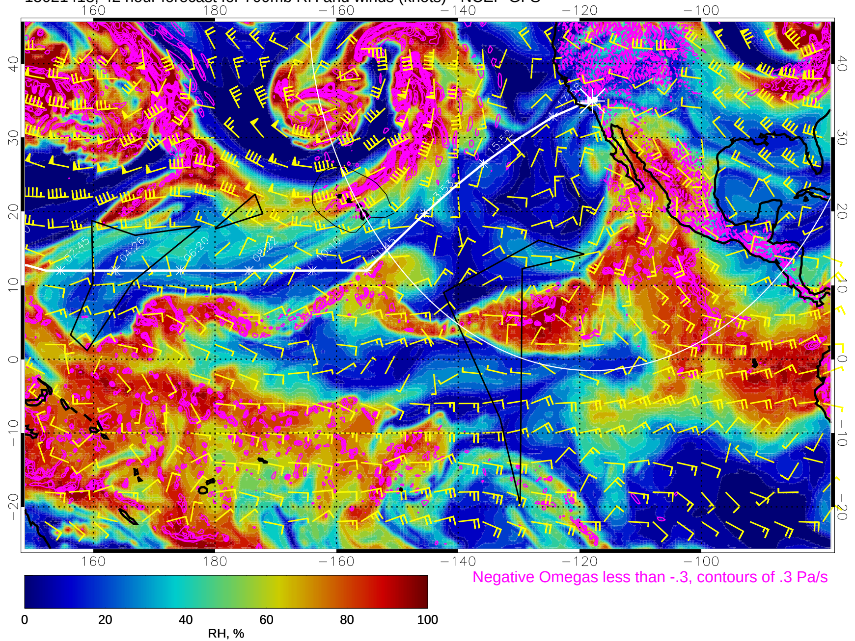
15021418, 42 hour forecast for 700mb RH and winds (knots) - NCEP GFS
