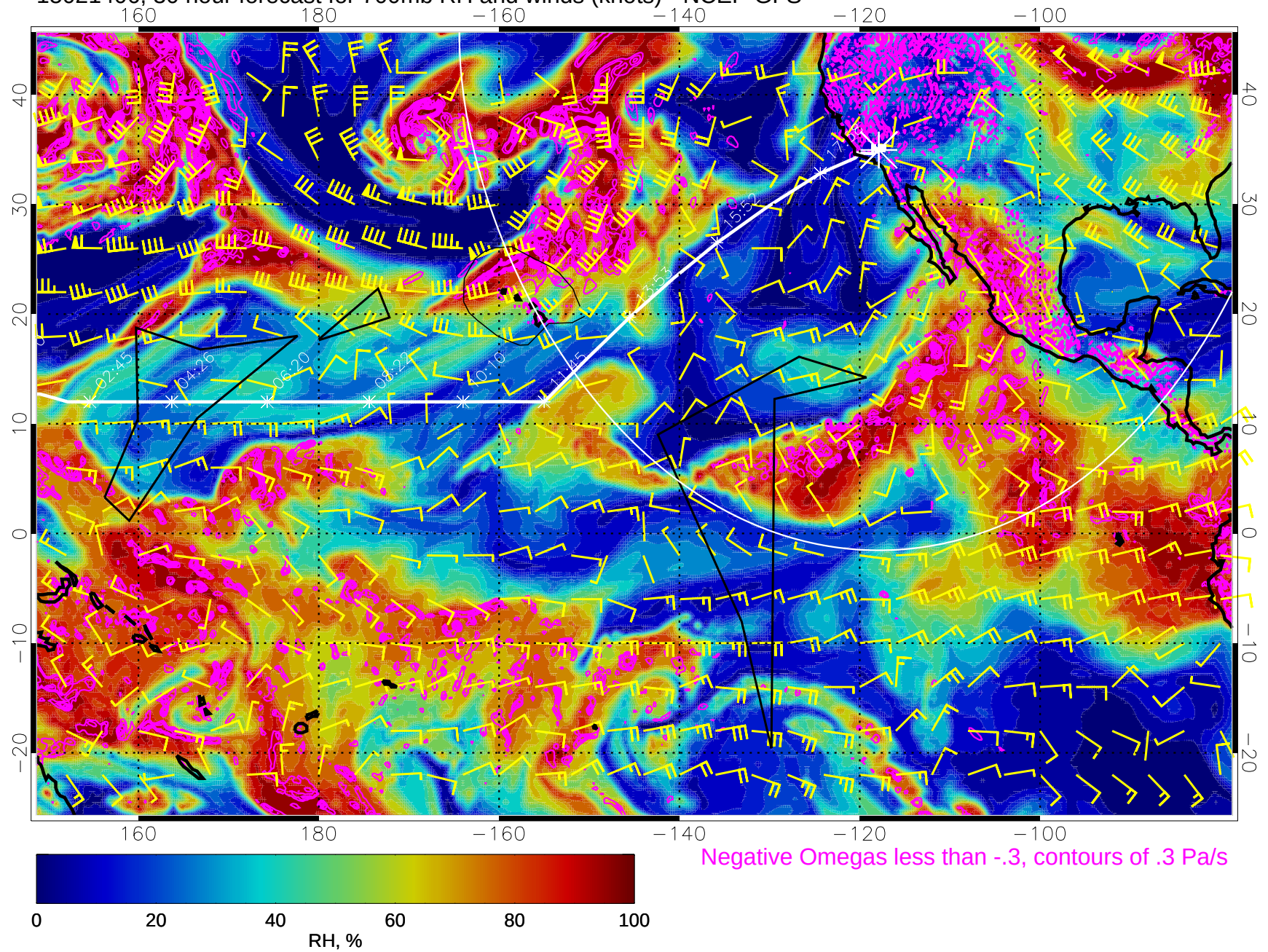
15021406, 30 hour forecast for 700mb RH and winds (knots) - NCEP GFS
