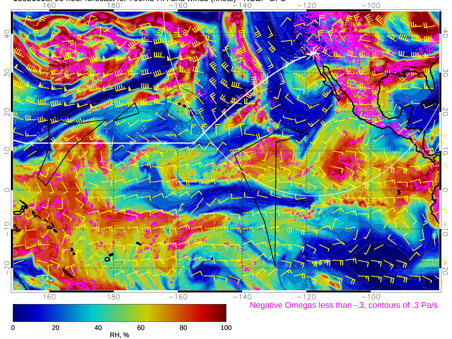
15021618, 90 hour forecast for 700mb RH and winds (knots) - NCEP GFS
