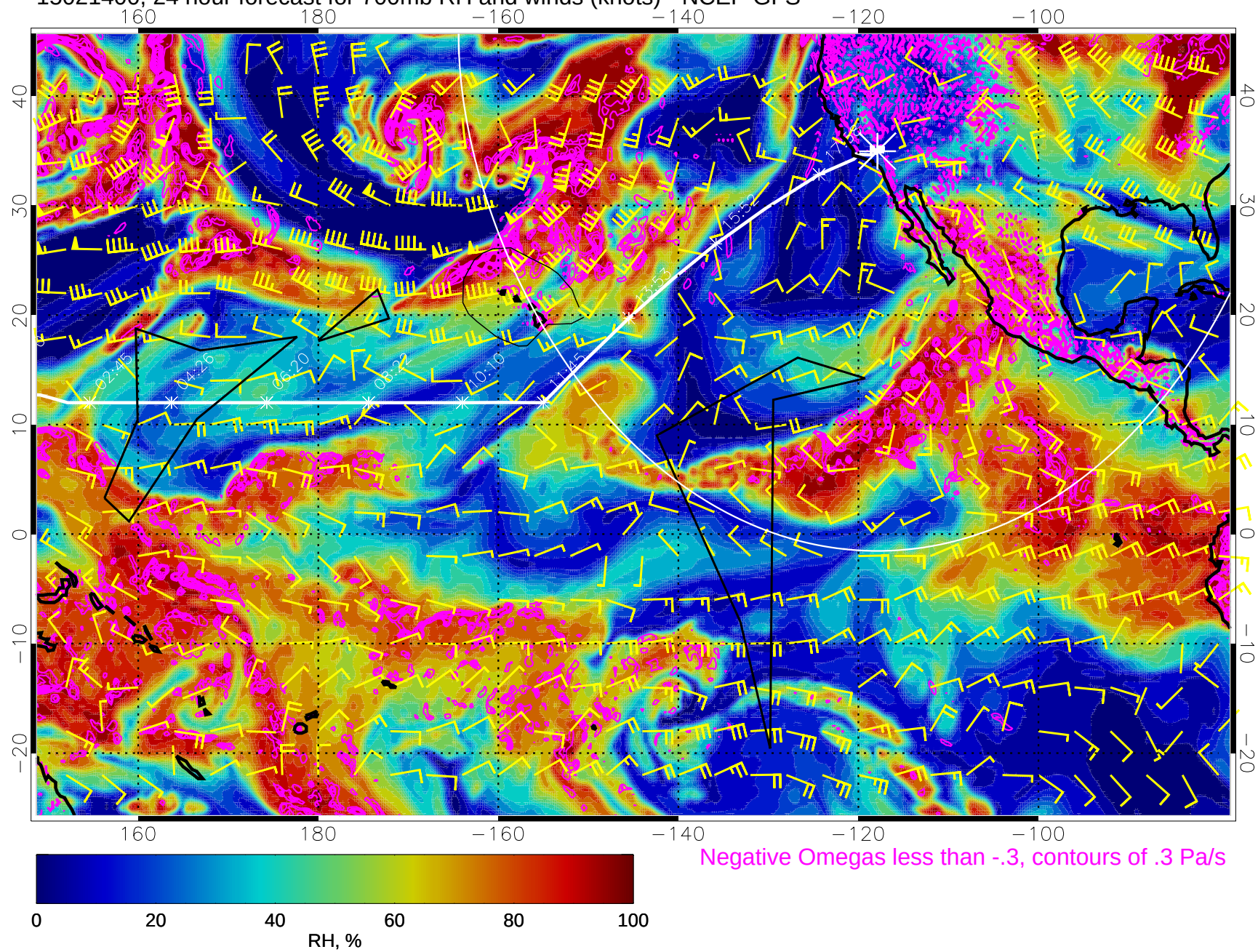
15021400, 24 hour forecast for 700mb RH and winds (knots) - NCEP GFS
