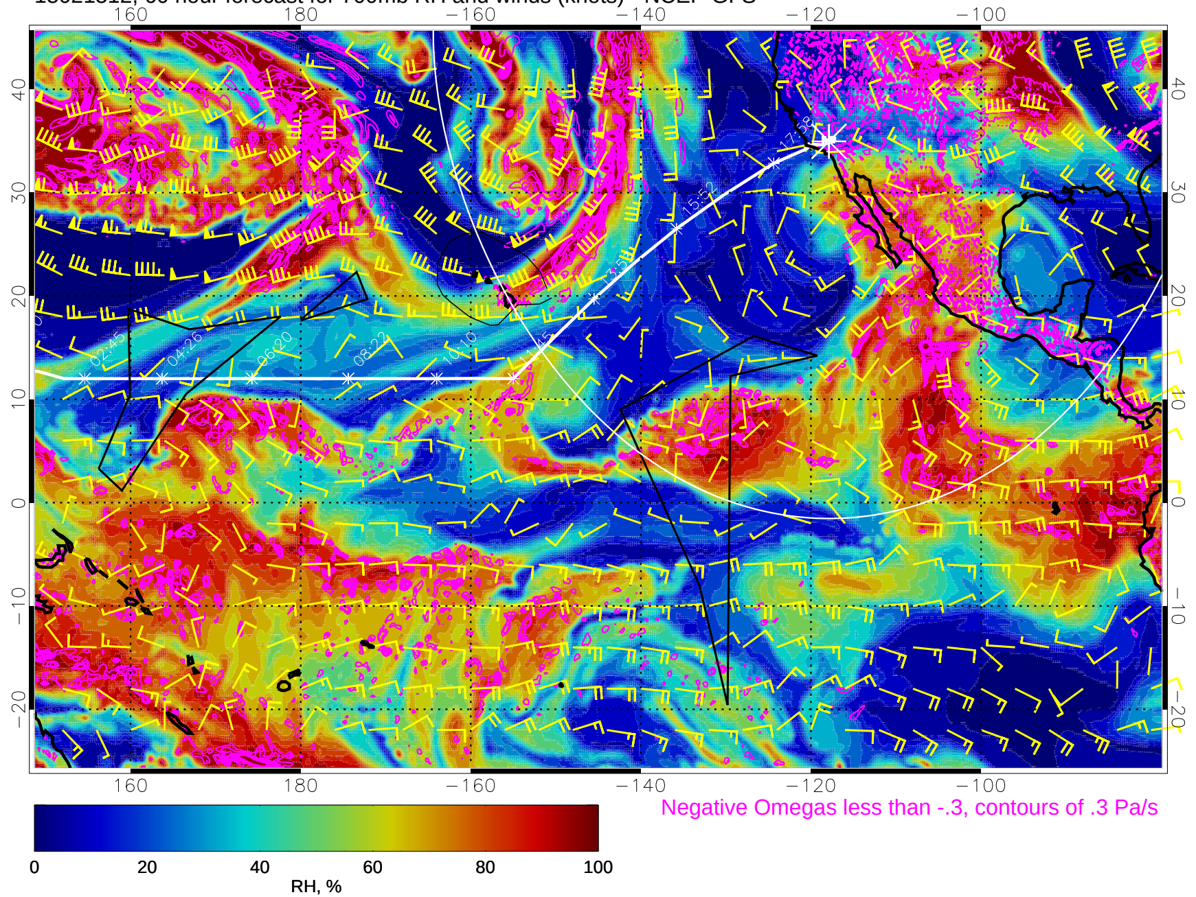
15021512, 60 hour forecast for 700mb RH and winds (knots) - NCEP GFS
