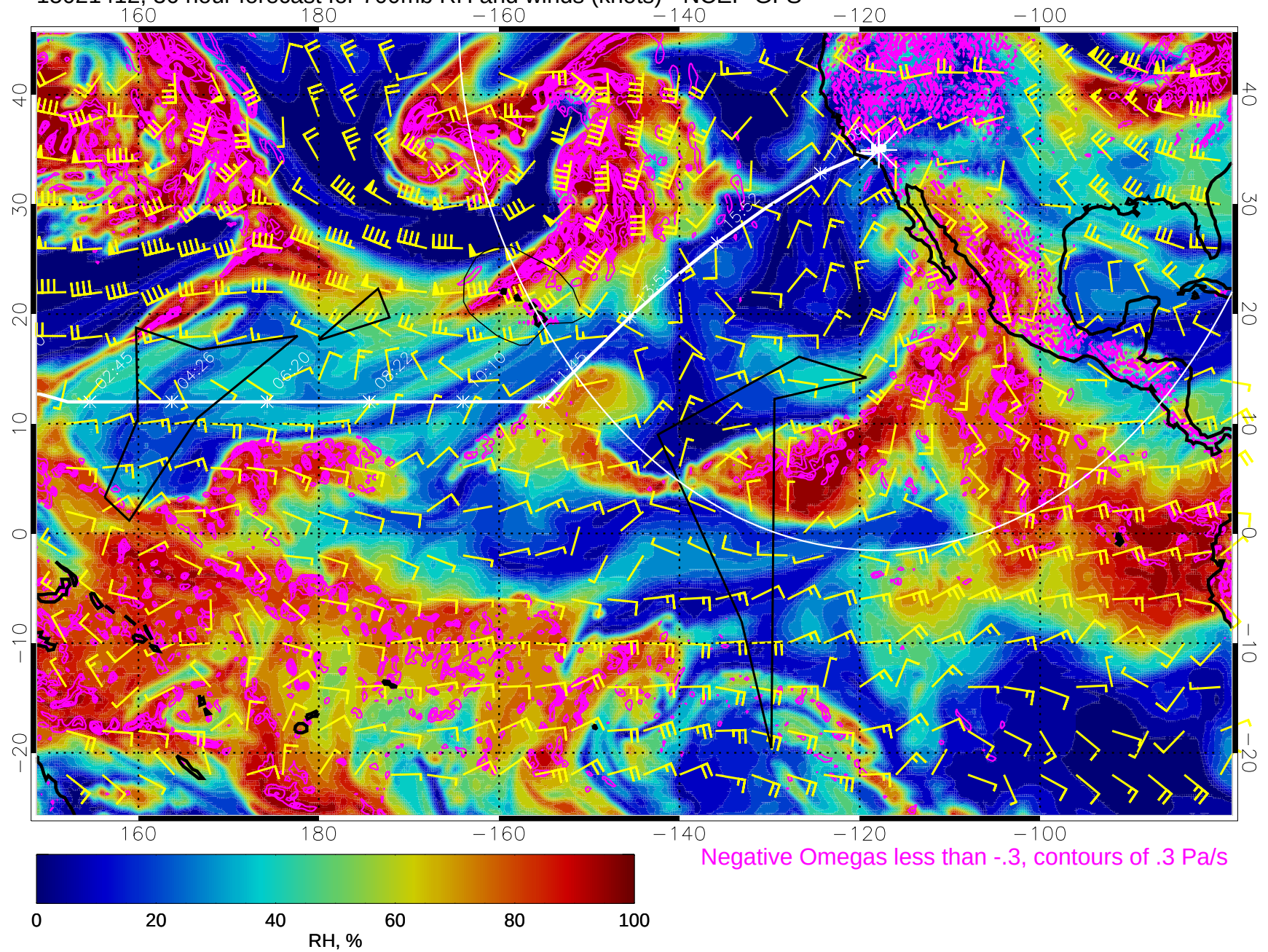
15021412, 36 hour forecast for 700mb RH and winds (knots) - NCEP GFS
