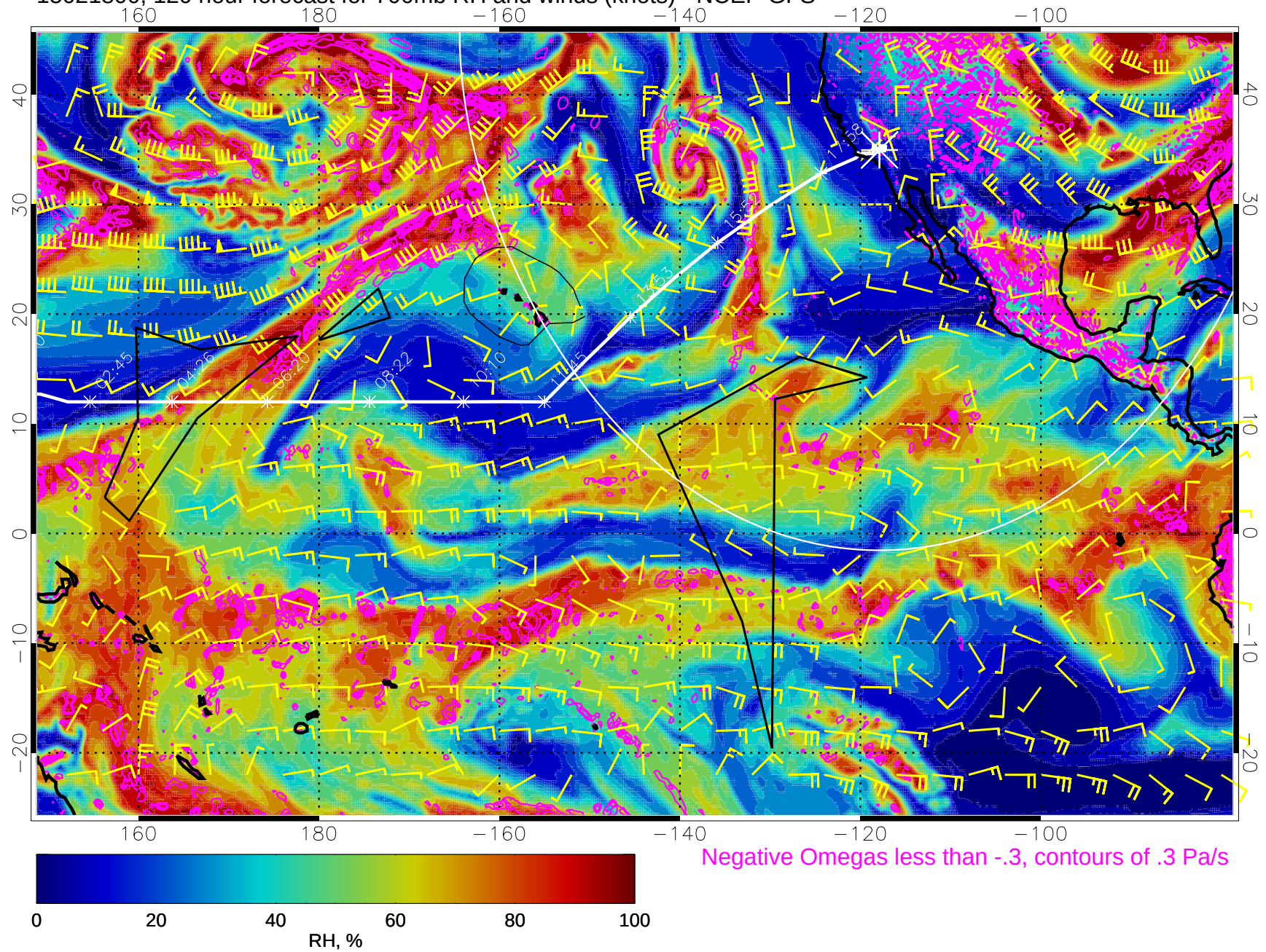
15021800, 120 hour forecast for 700mb RH and winds (knots) - NCEP GFS
