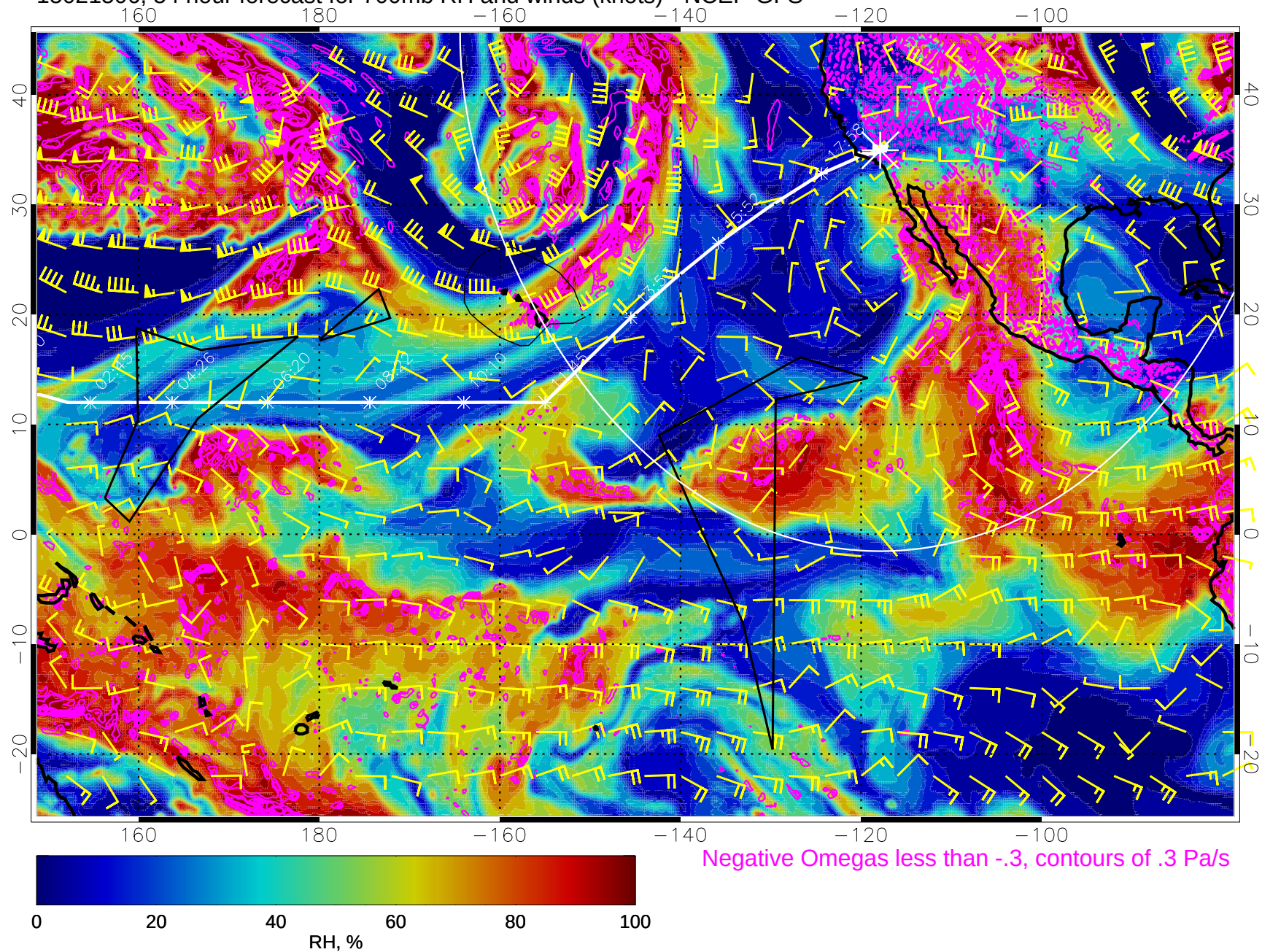
15021506, 54 hour forecast for 700mb RH and winds (knots) - NCEP GFS
