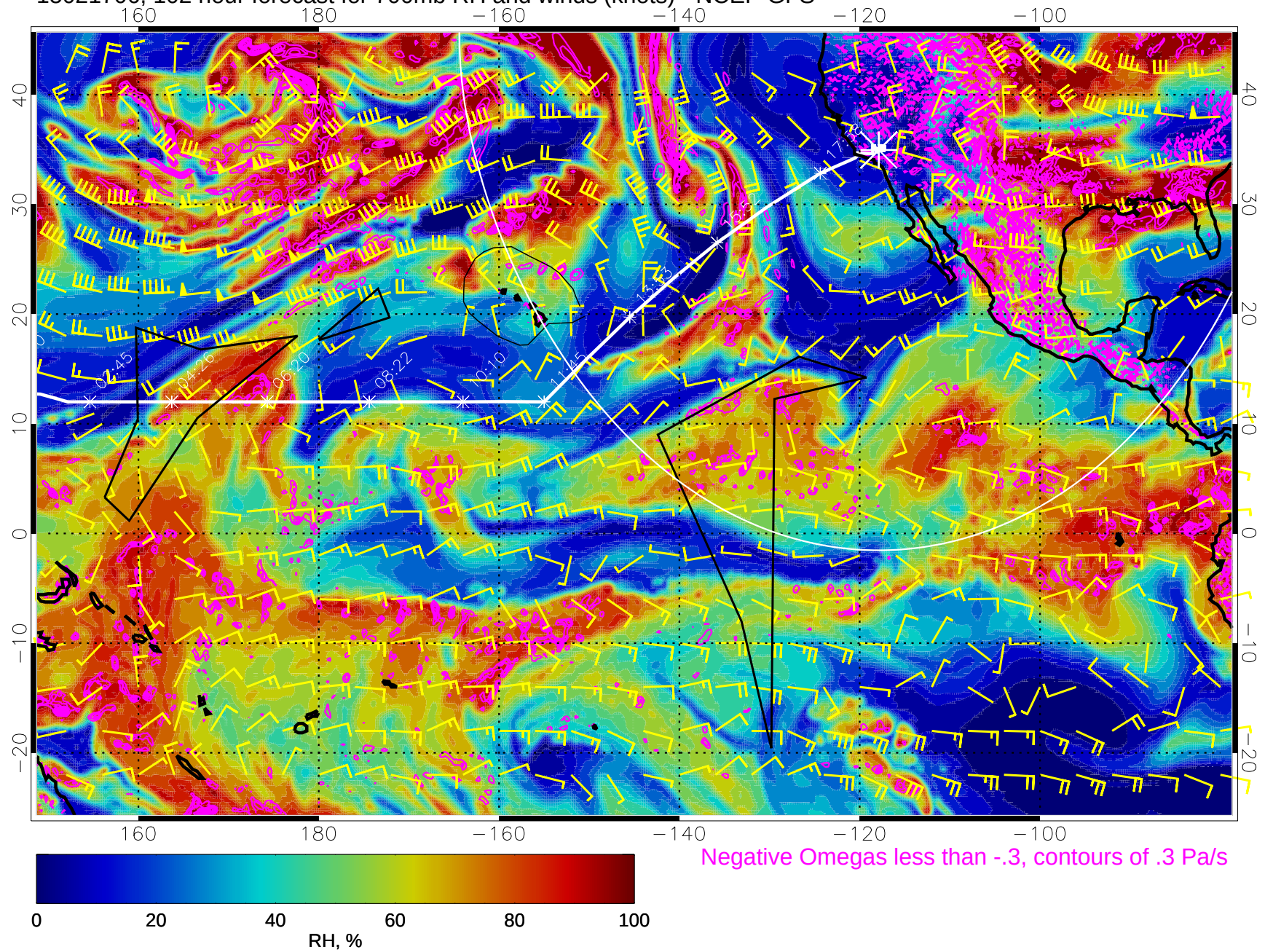
15021706, 102 hour forecast for 700mb RH and winds (knots) - NCEP GFS
