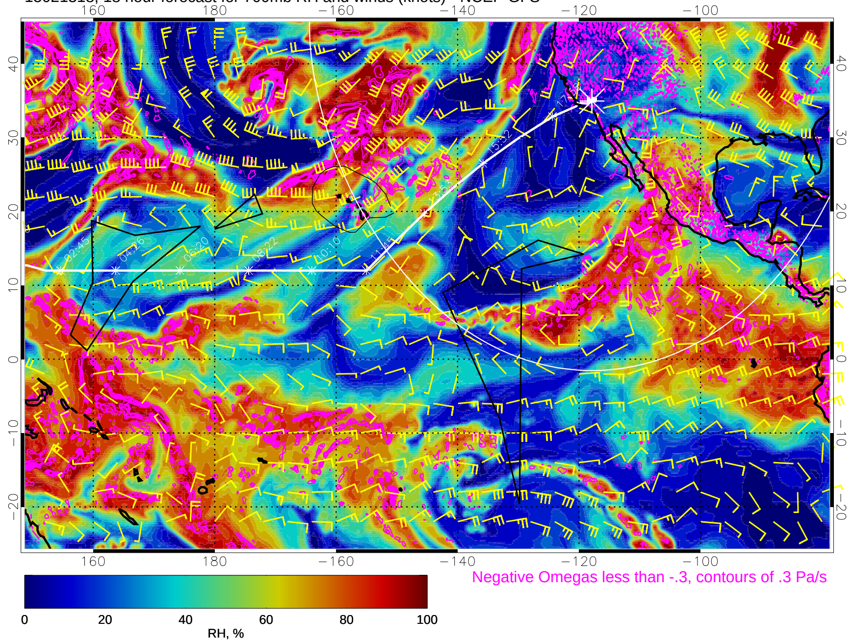
15021318, 18 hour forecast for 700mb RH and winds (knots) - NCEP GFS
