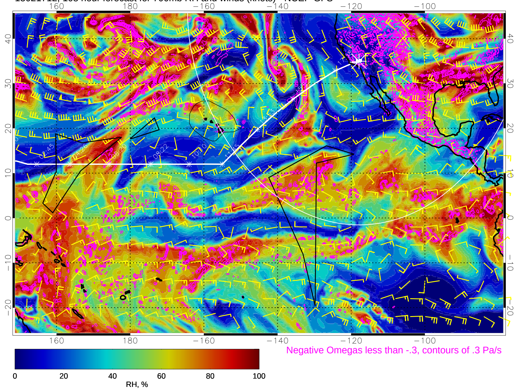
15021712, 108 hour forecast for 700mb RH and winds (knots) - NCEP GFS
