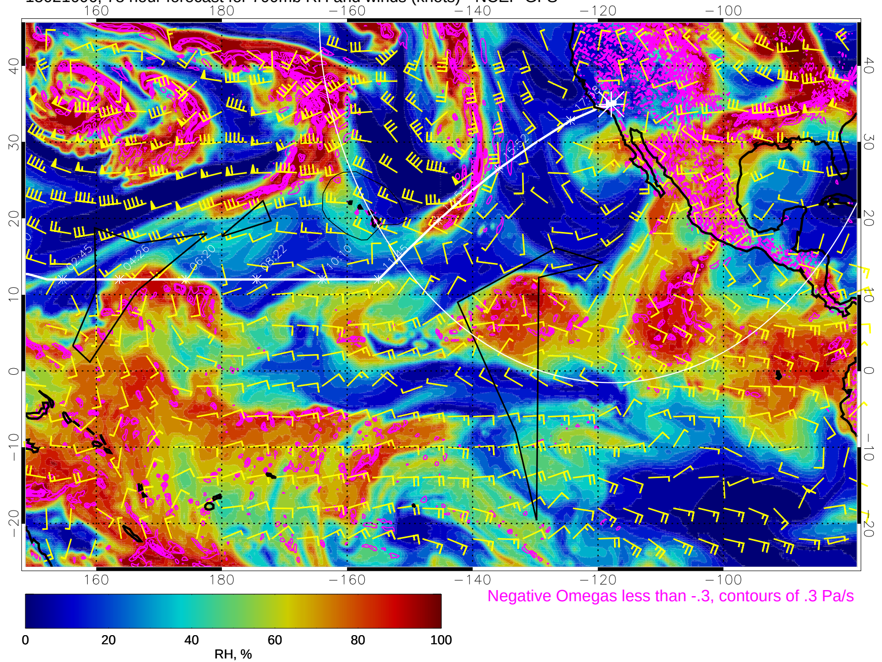
15021606, 78 hour forecast for 700mb RH and winds (knots) - NCEP GFS
