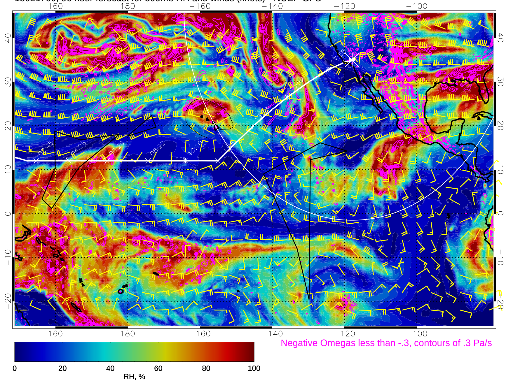
15021700, 96 hour forecast for 500mb RH and winds (knots) - NCEP GFS
