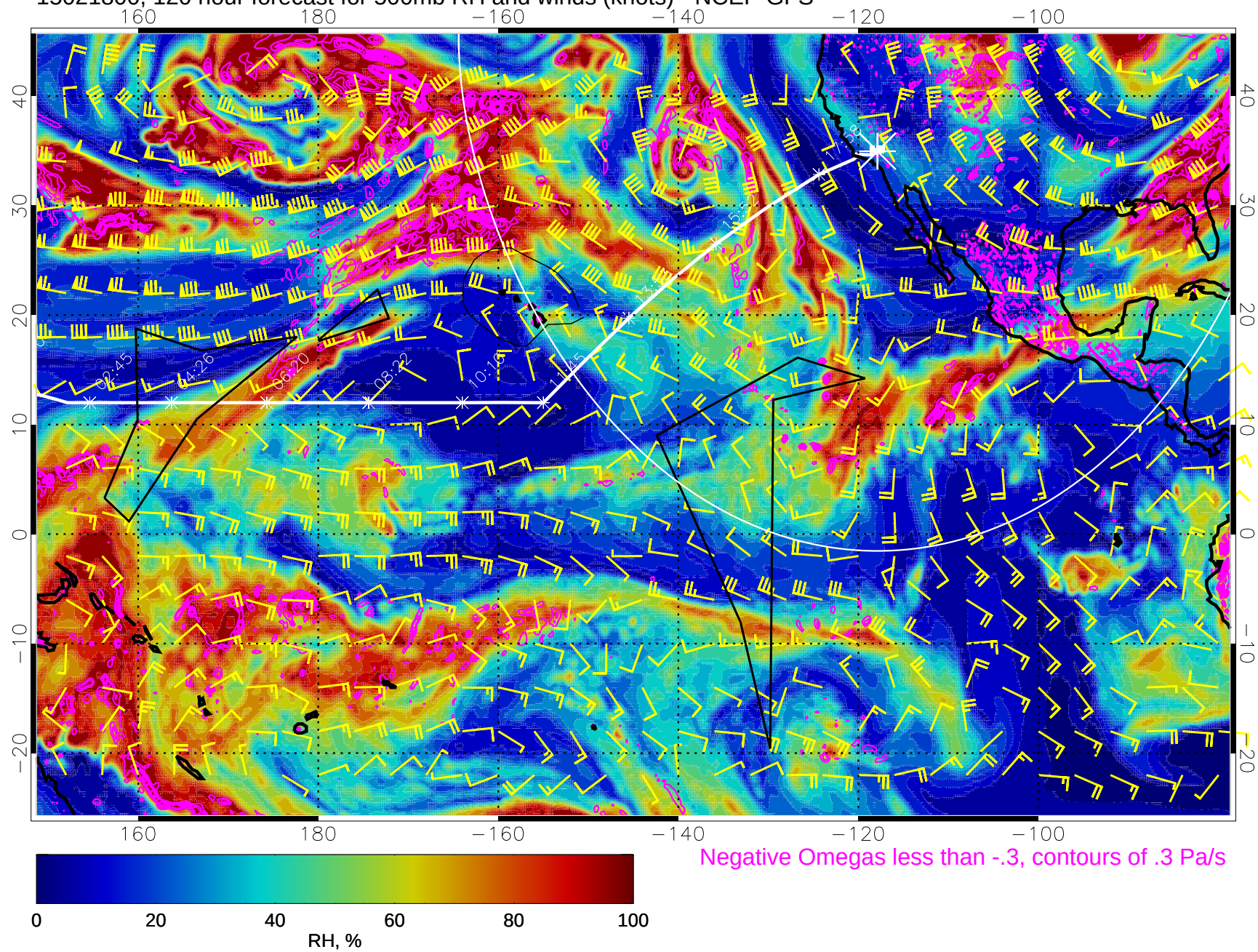
15021800, 120 hour forecast for 500mb RH and winds (knots) - NCEP GFS
