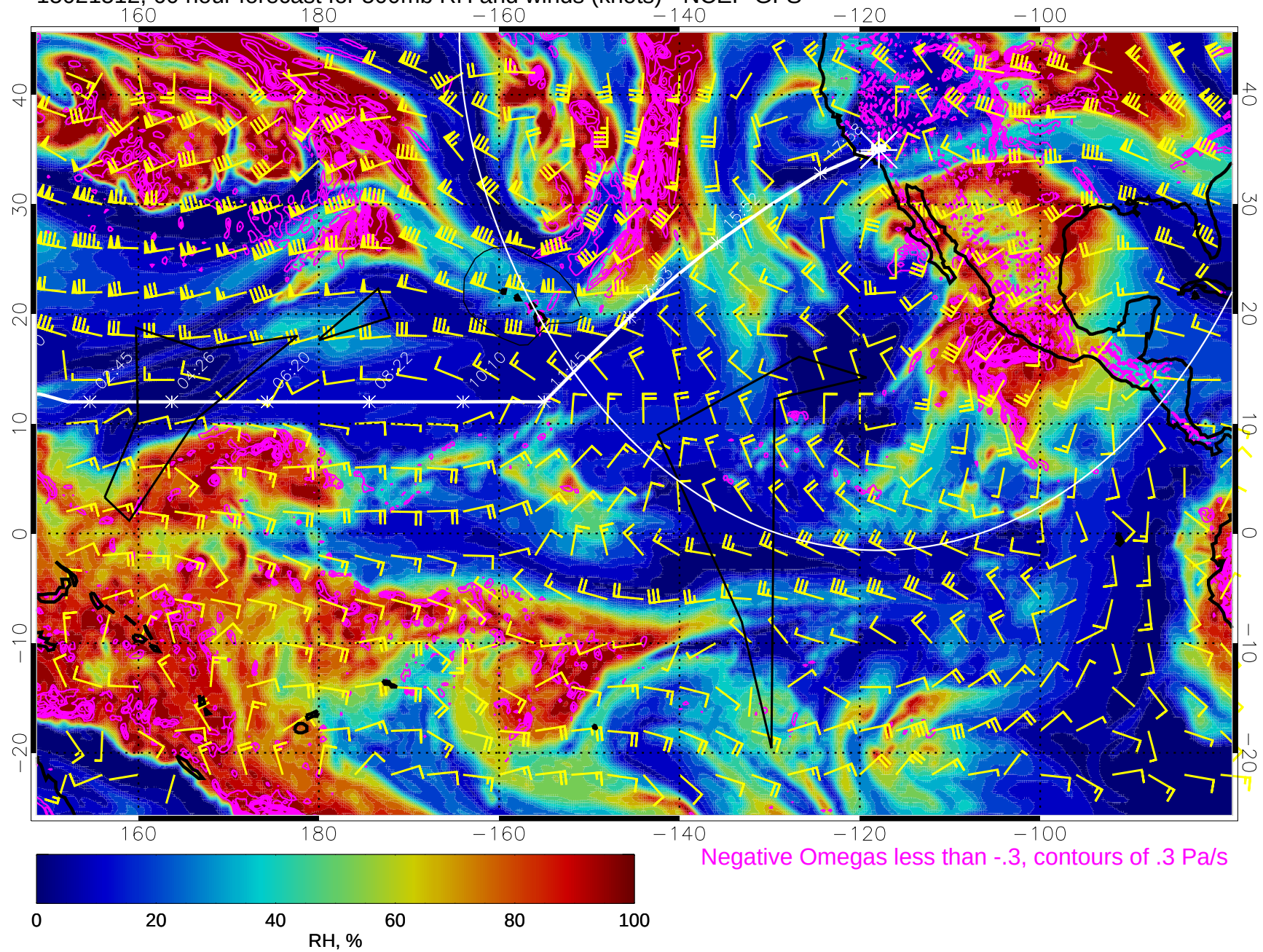
15021512, 60 hour forecast for 500mb RH and winds (knots) - NCEP GFS
