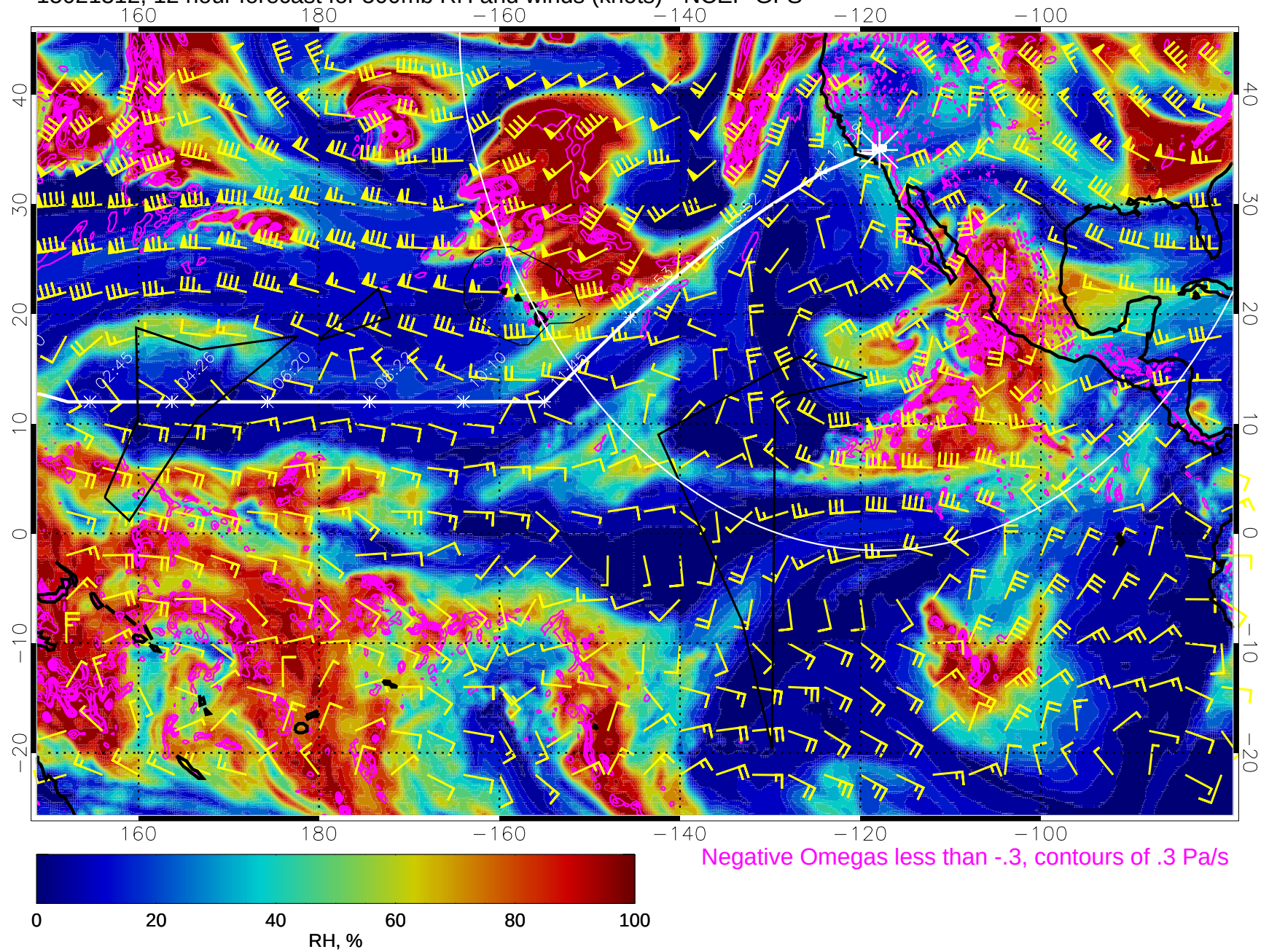
15021312, 12 hour forecast for 500mb RH and winds (knots) - NCEP GFS
