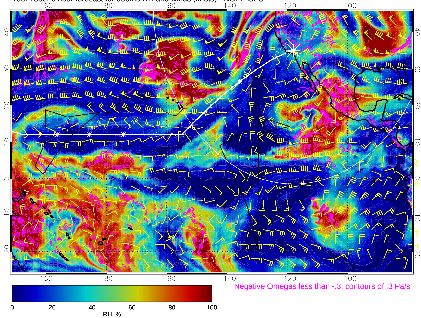
15021306, 6 hour forecast for 500mb RH and winds (knots) - NCEP GFS
