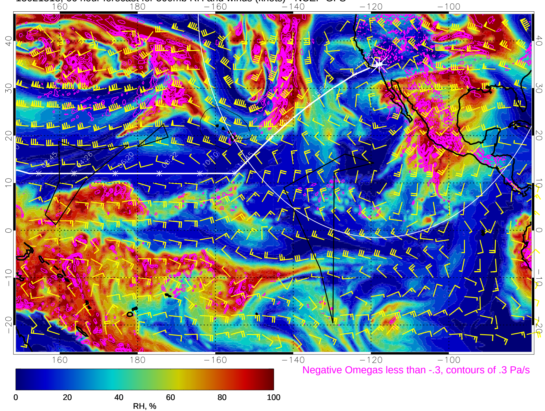
15021518, 66 hour forecast for 500mb RH and winds (knots) - NCEP GFS
