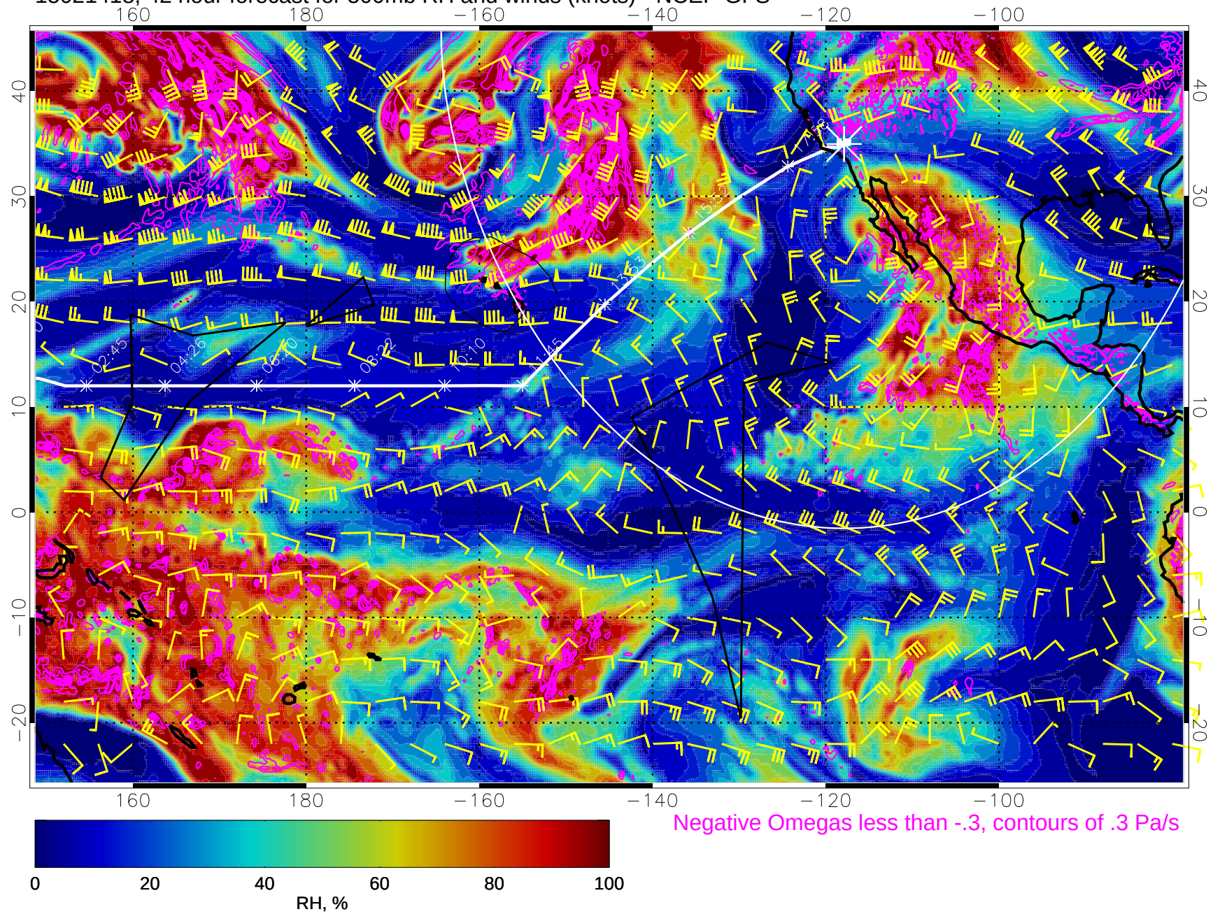
15021418, 42 hour forecast for 500mb RH and winds (knots) - NCEP GFS
