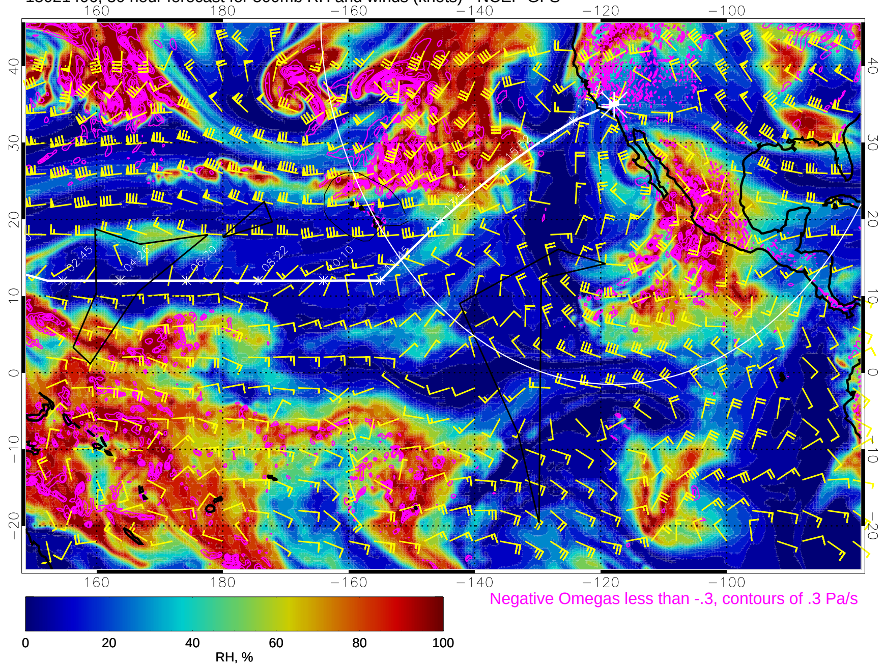
15021406, 30 hour forecast for 500mb RH and winds (knots) - NCEP GFS
