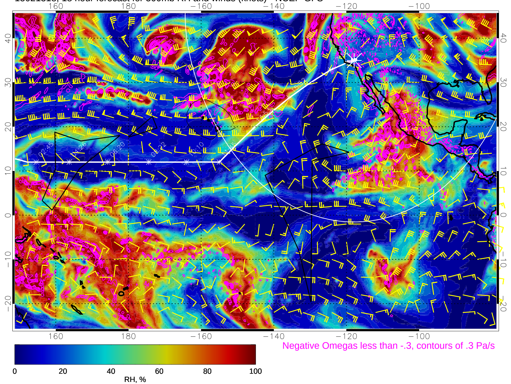
15021318, 18 hour forecast for 500mb RH and winds (knots) - NCEP GFS
