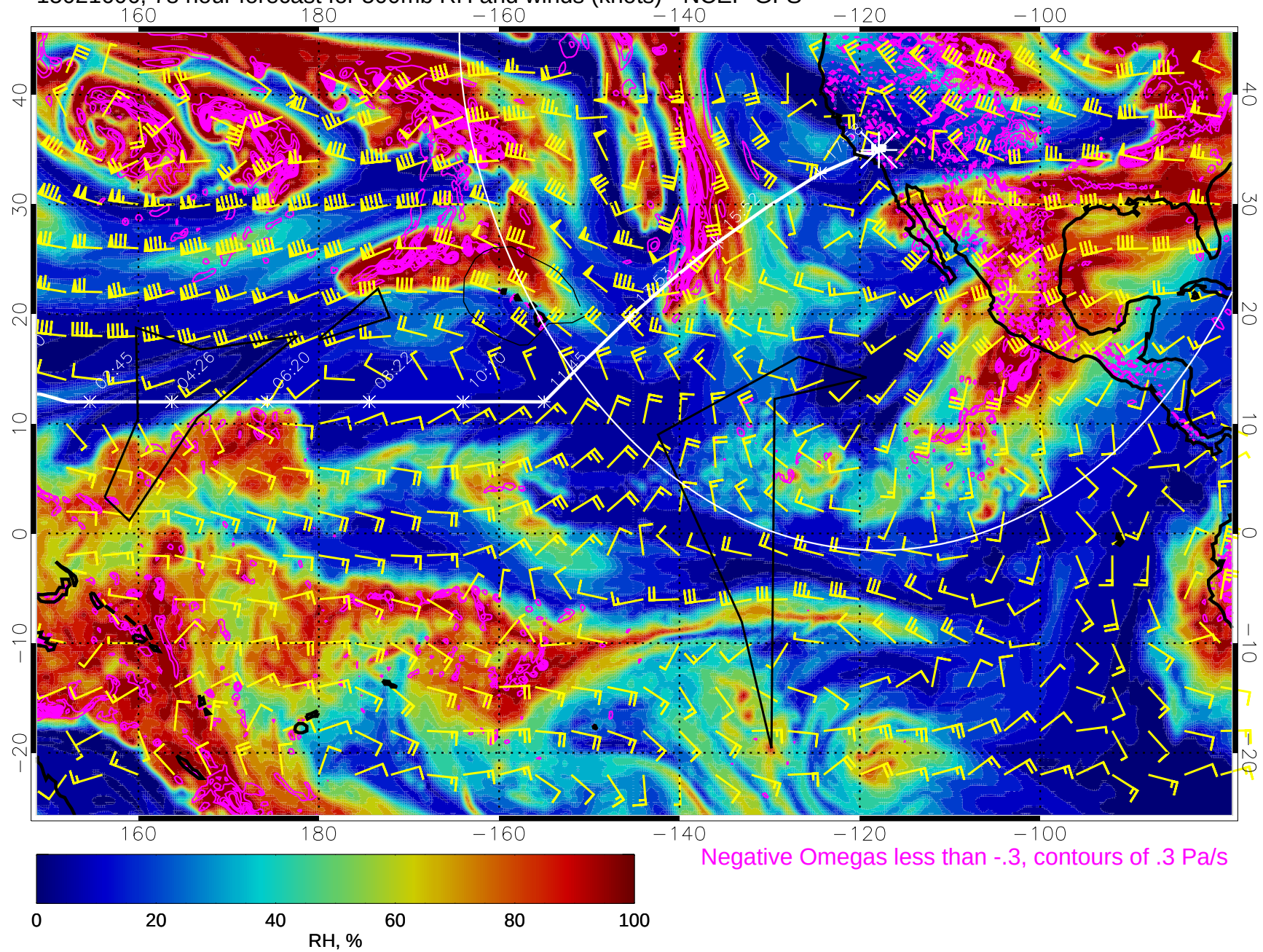
15021606, 78 hour forecast for 500mb RH and winds (knots) - NCEP GFS
