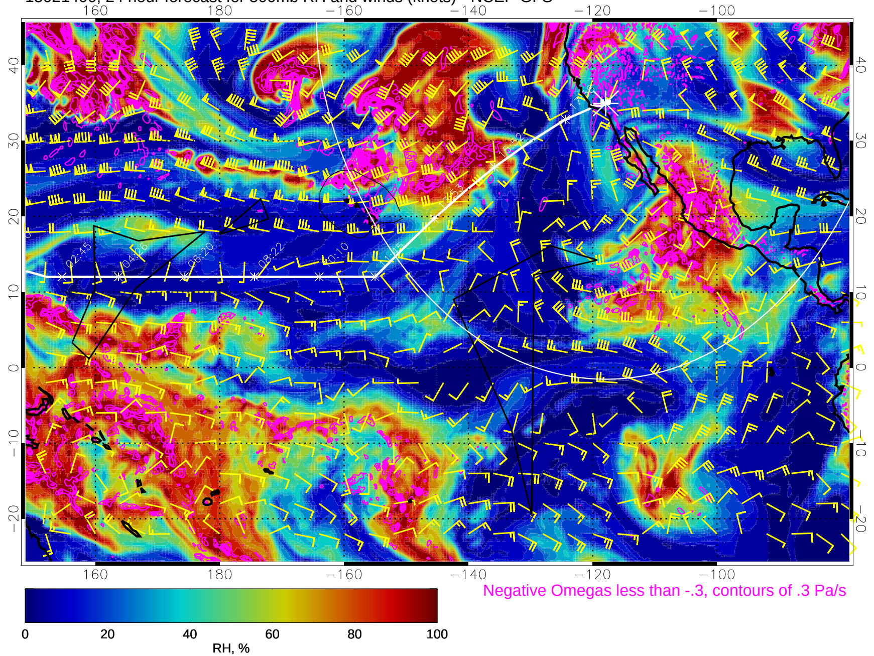
15021400, 24 hour forecast for 500mb RH and winds (knots) - NCEP GFS
