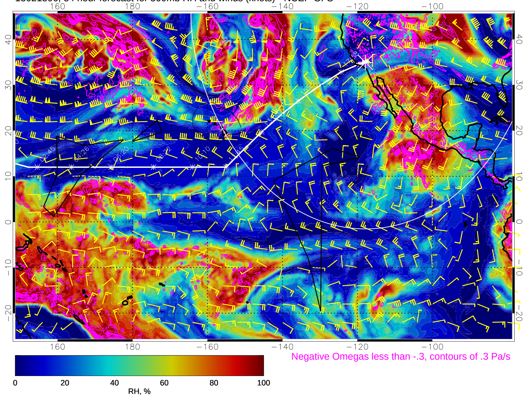
15021506, 54 hour forecast for 500mb RH and winds (knots) - NCEP GFS
