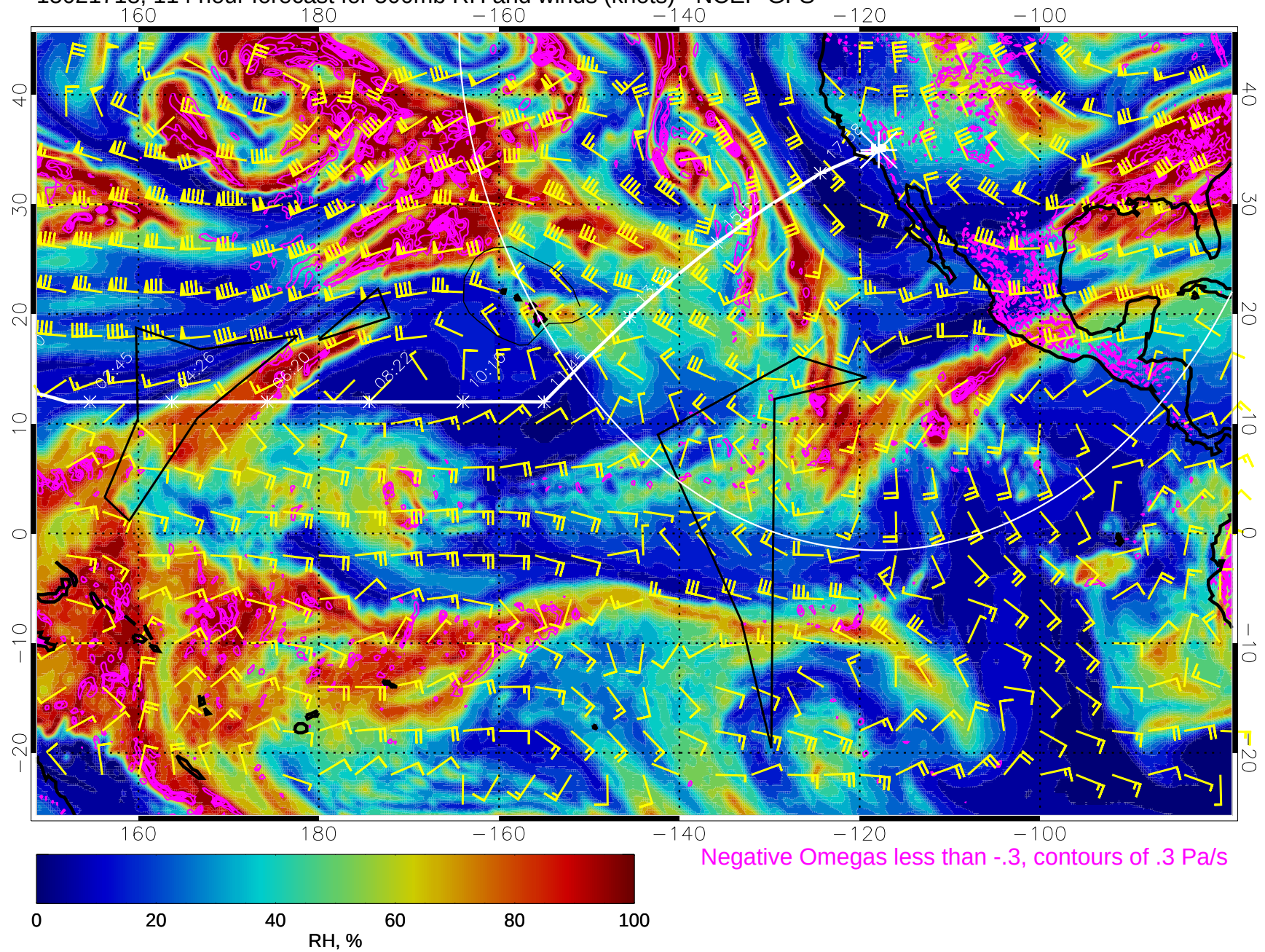
15021718, 114 hour forecast for 500mb RH and winds (knots) - NCEP GFS
