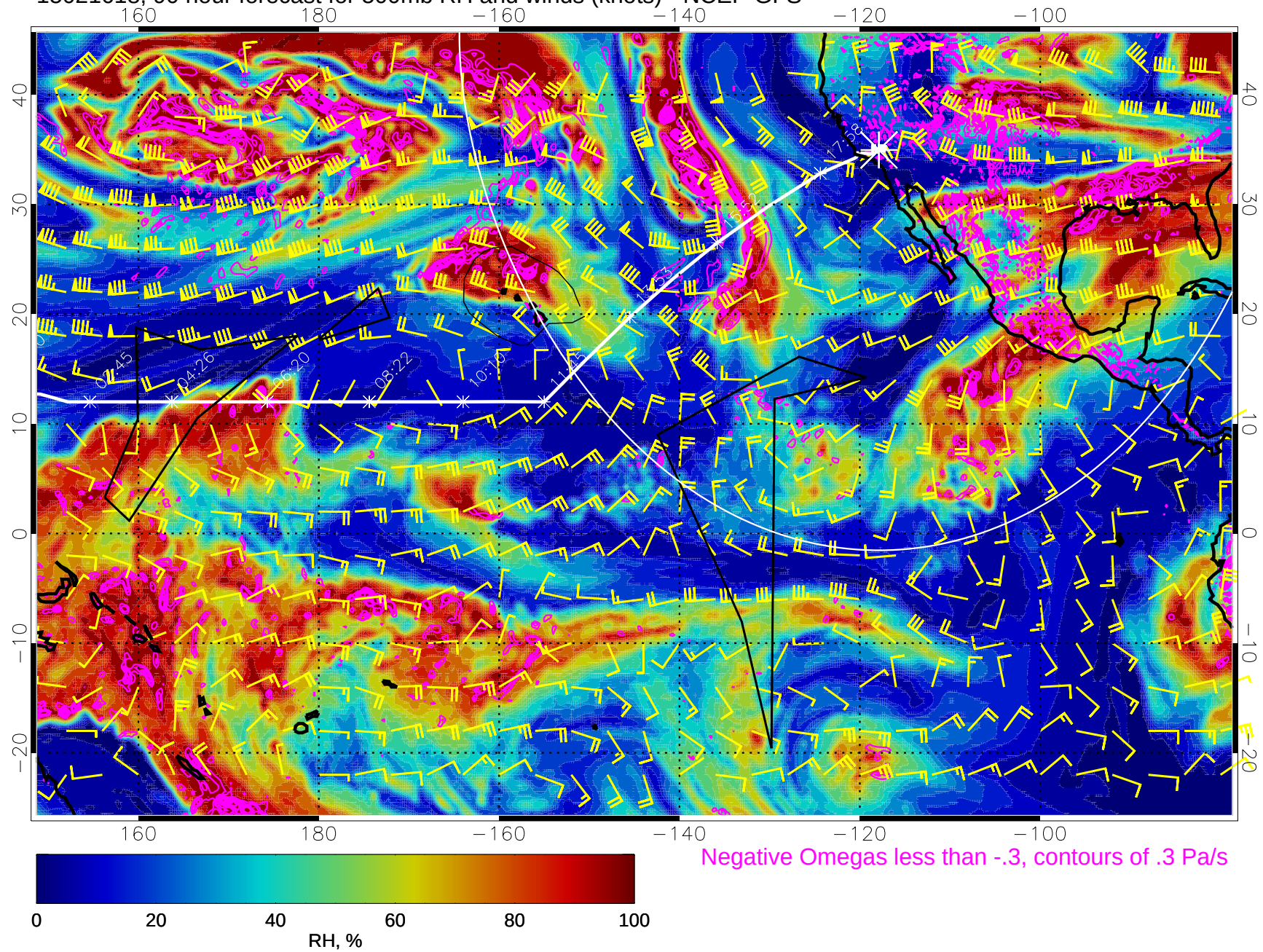
15021618, 90 hour forecast for 500mb RH and winds (knots) - NCEP GFS
