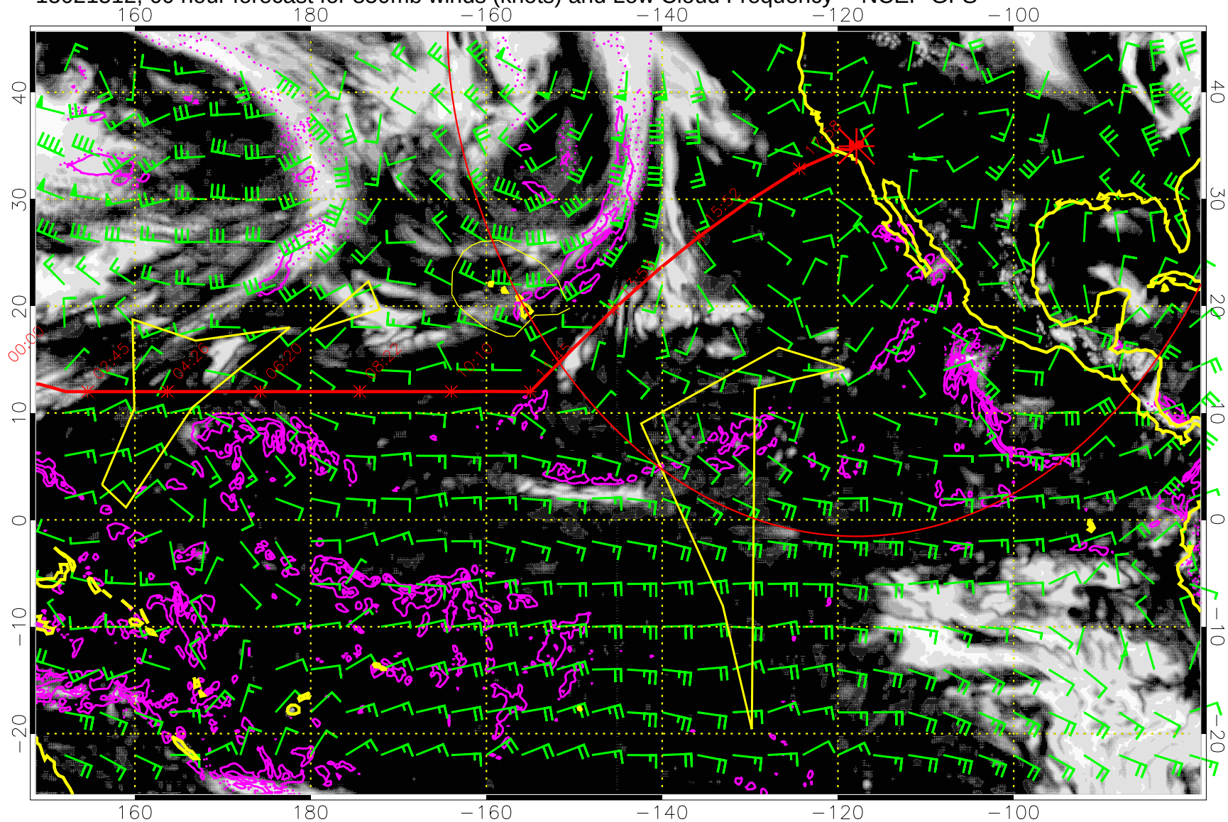
15021512, 60 hour forecast for 850mb winds (knots) and Low Cloud Frequency -- NCEP GFS
