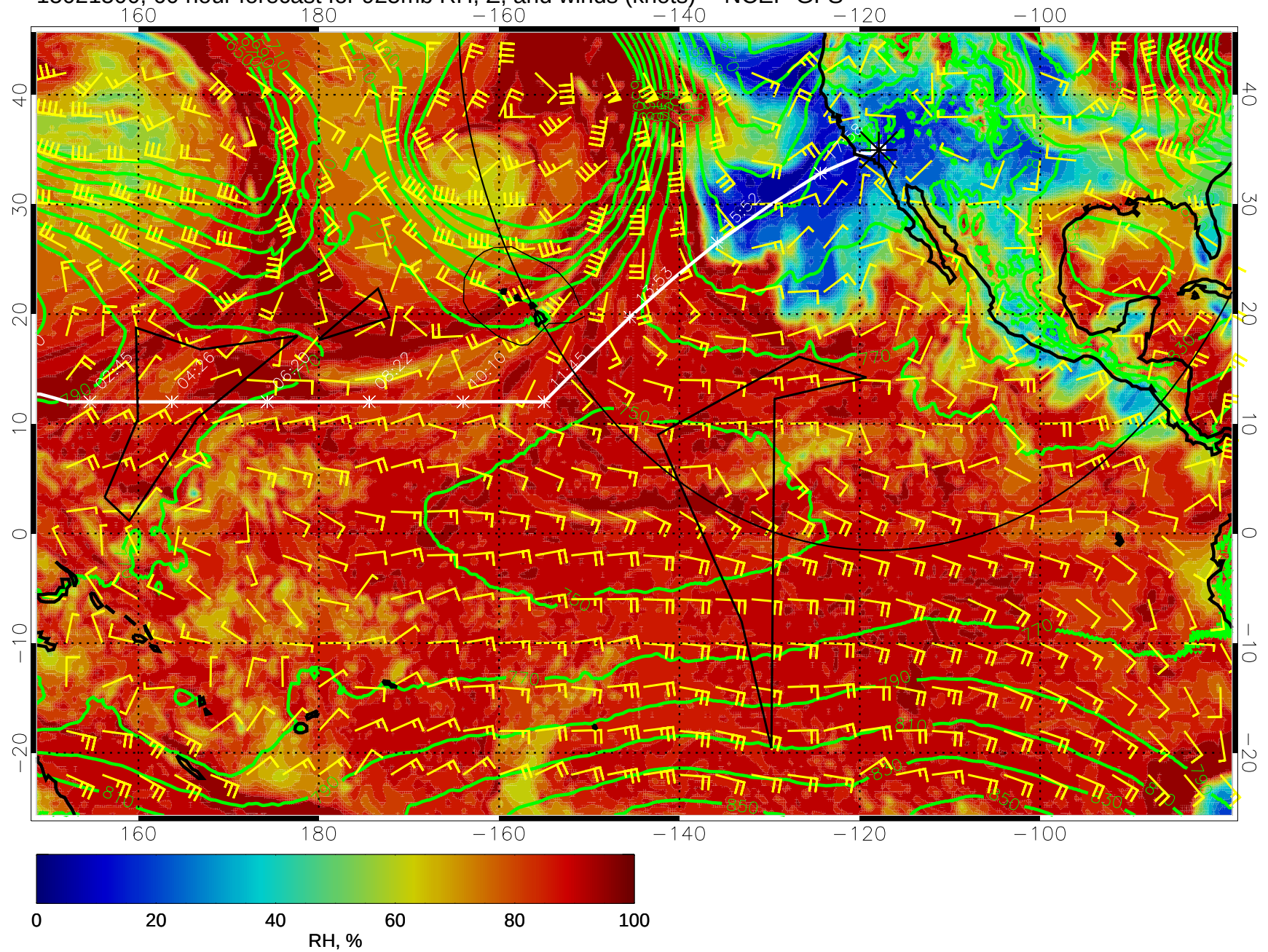
15021500, 60 hour forecast for 925mb RH, Z, and winds (knots) -- NCEP GFS
