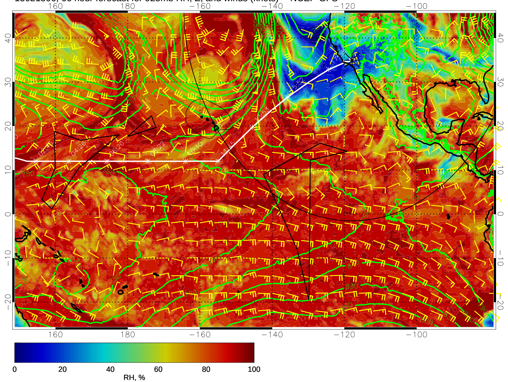
15021506, 66 hour forecast for 925mb RH, Z, and winds (knots) -- NCEP GFS
