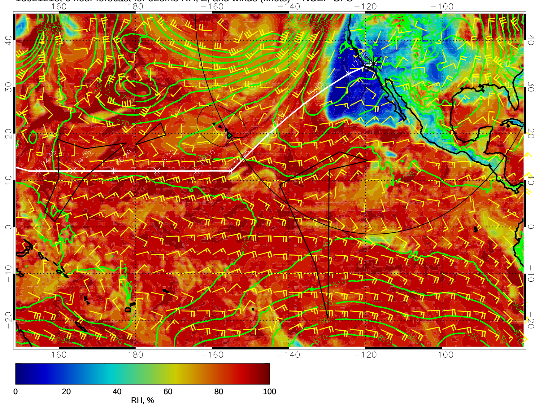
15021218, 6 hour forecast for 925mb RH, Z, and winds (knots) -- NCEP GFS
