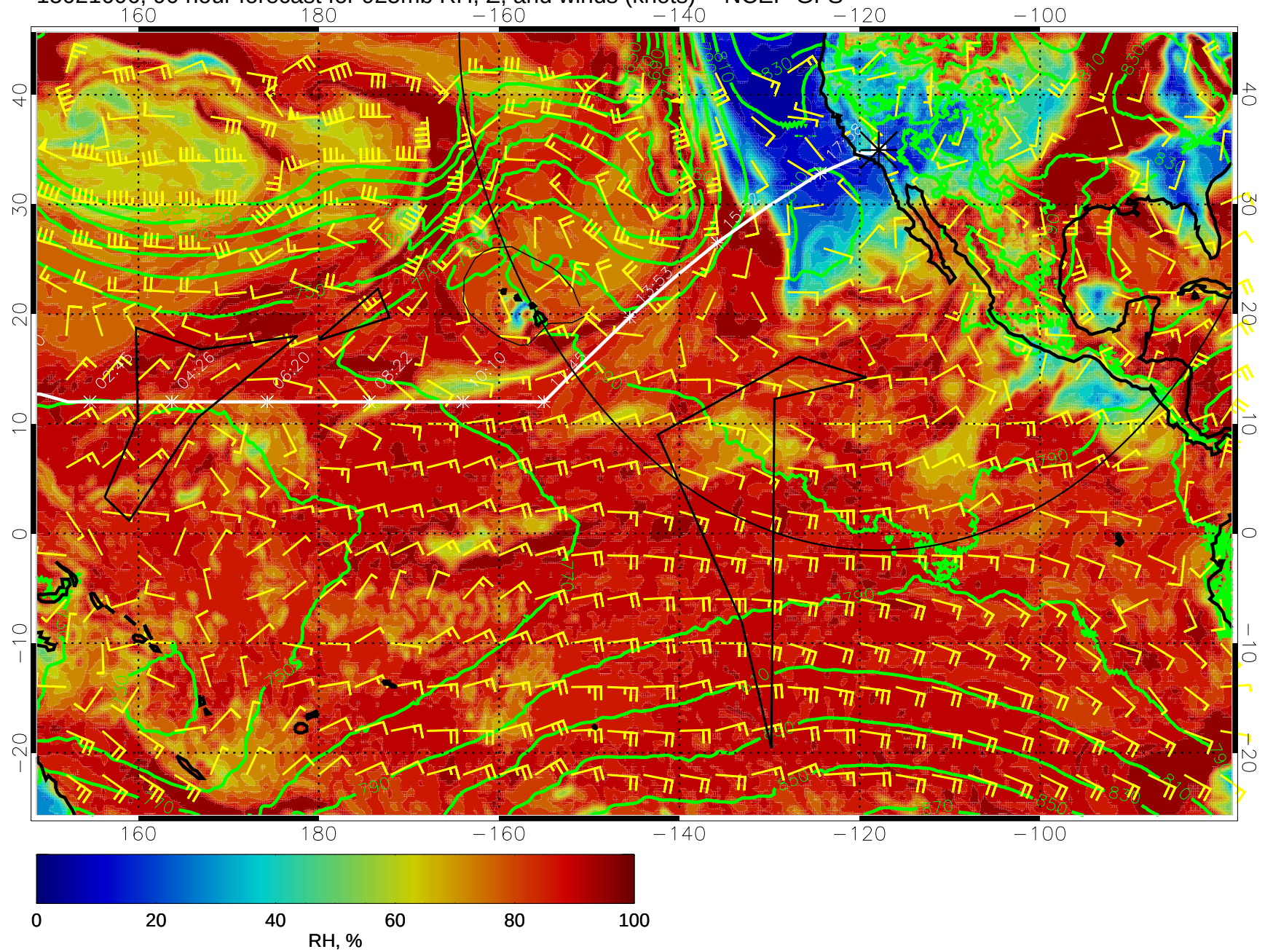
15021606, 90 hour forecast for 925mb RH, Z, and winds (knots) -- NCEP GFS
