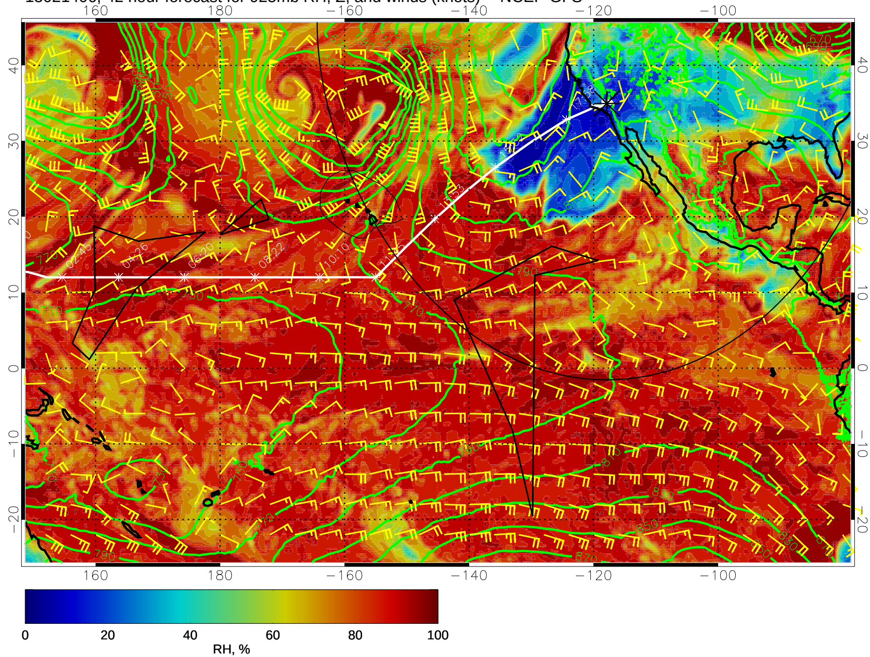
15021406, 42 hour forecast for 925mb RH, Z, and winds (knots) -- NCEP GFS
