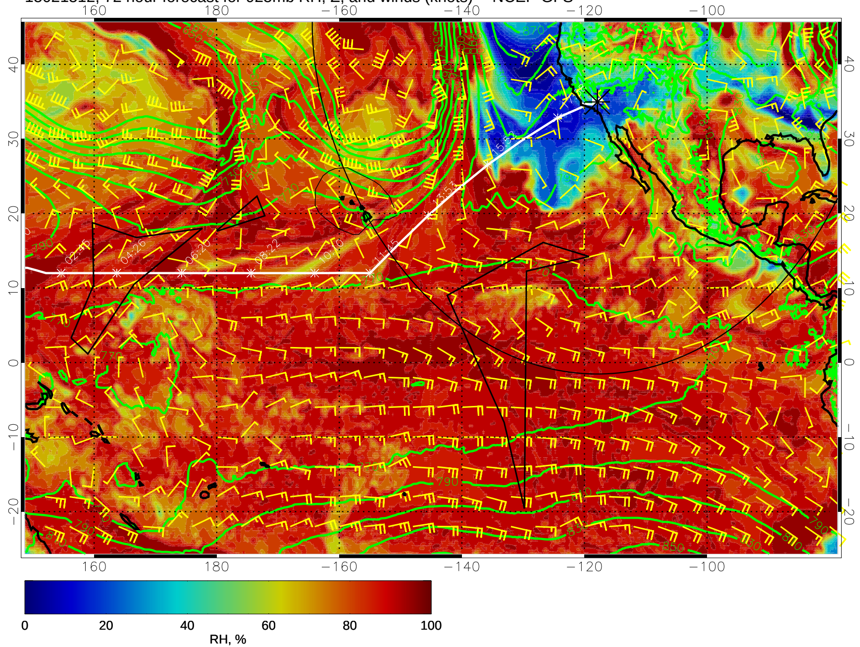
15021512, 72 hour forecast for 925mb RH, Z, and winds (knots) -- NCEP GFS
