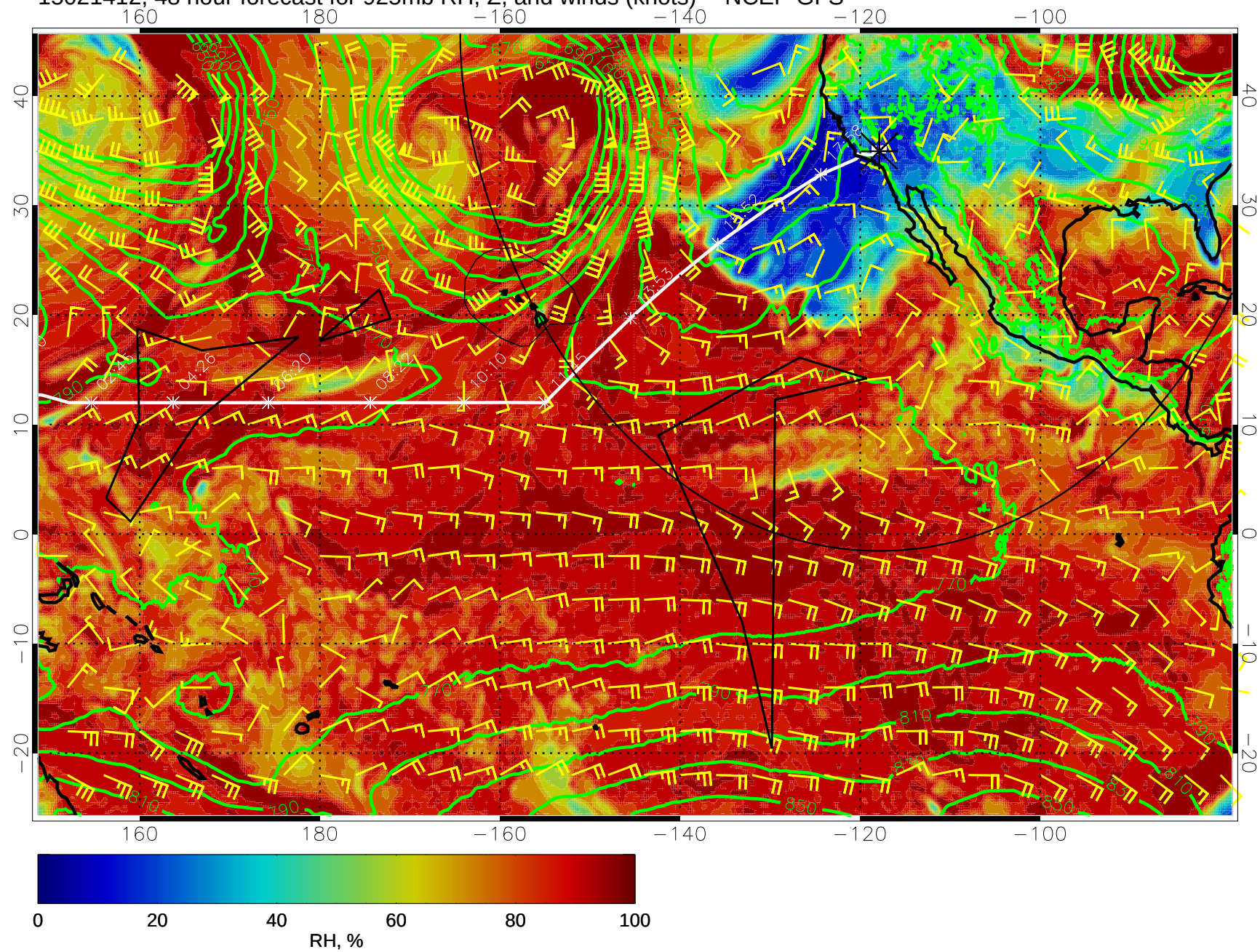
15021412, 48 hour forecast for 925mb RH, Z, and winds (knots) -- NCEP GFS
