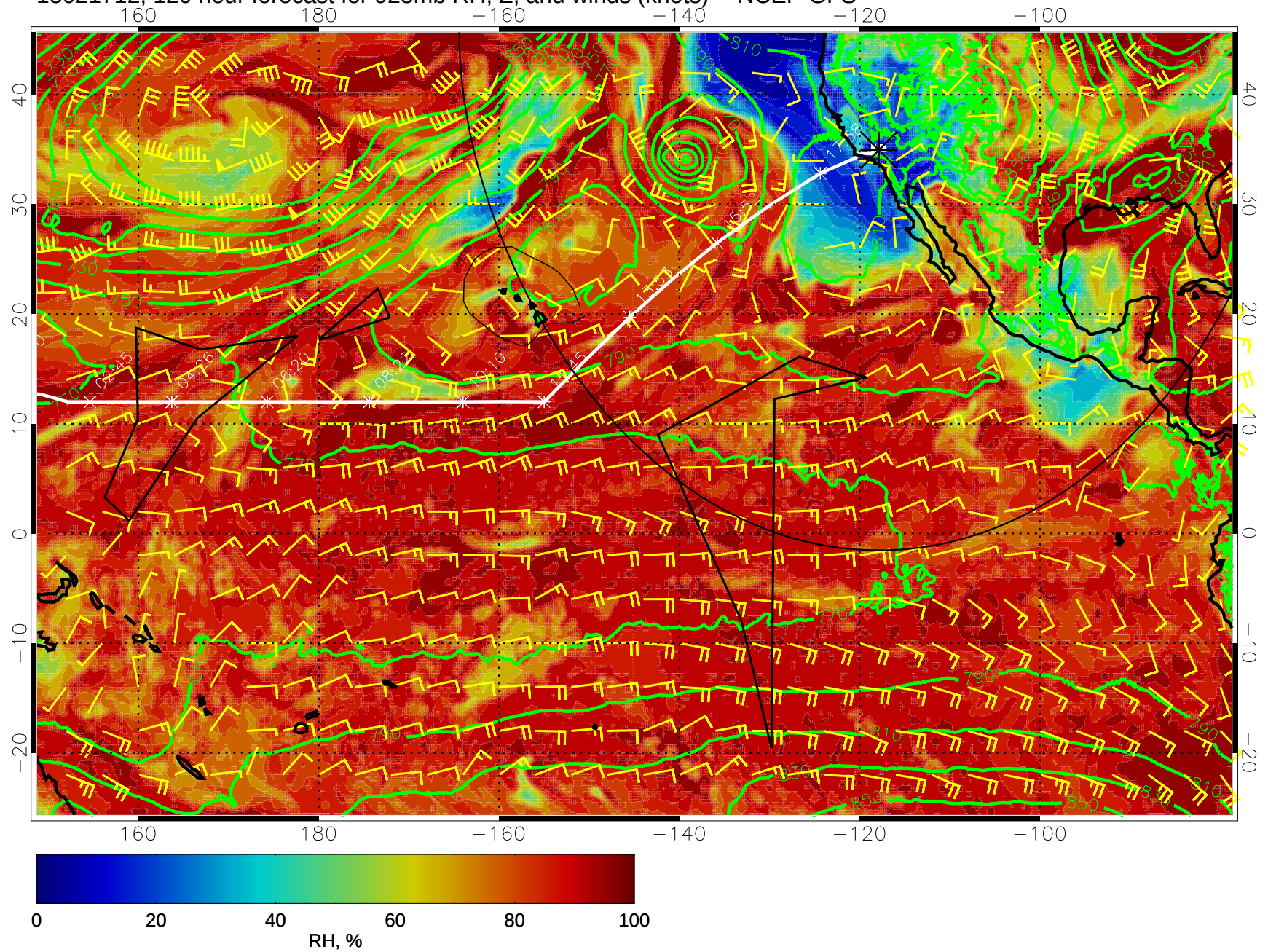
15021712, 120 hour forecast for 925mb RH, Z, and winds (knots) -- NCEP GFS
