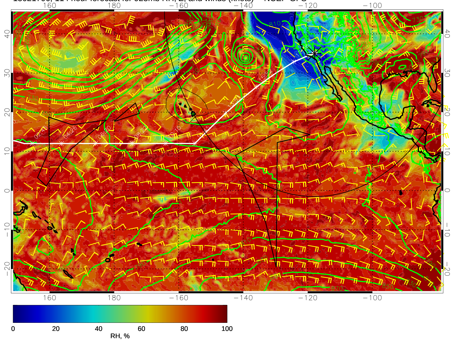
15021706, 114 hour forecast for 925mb RH, Z, and winds (knots) -- NCEP GFS
