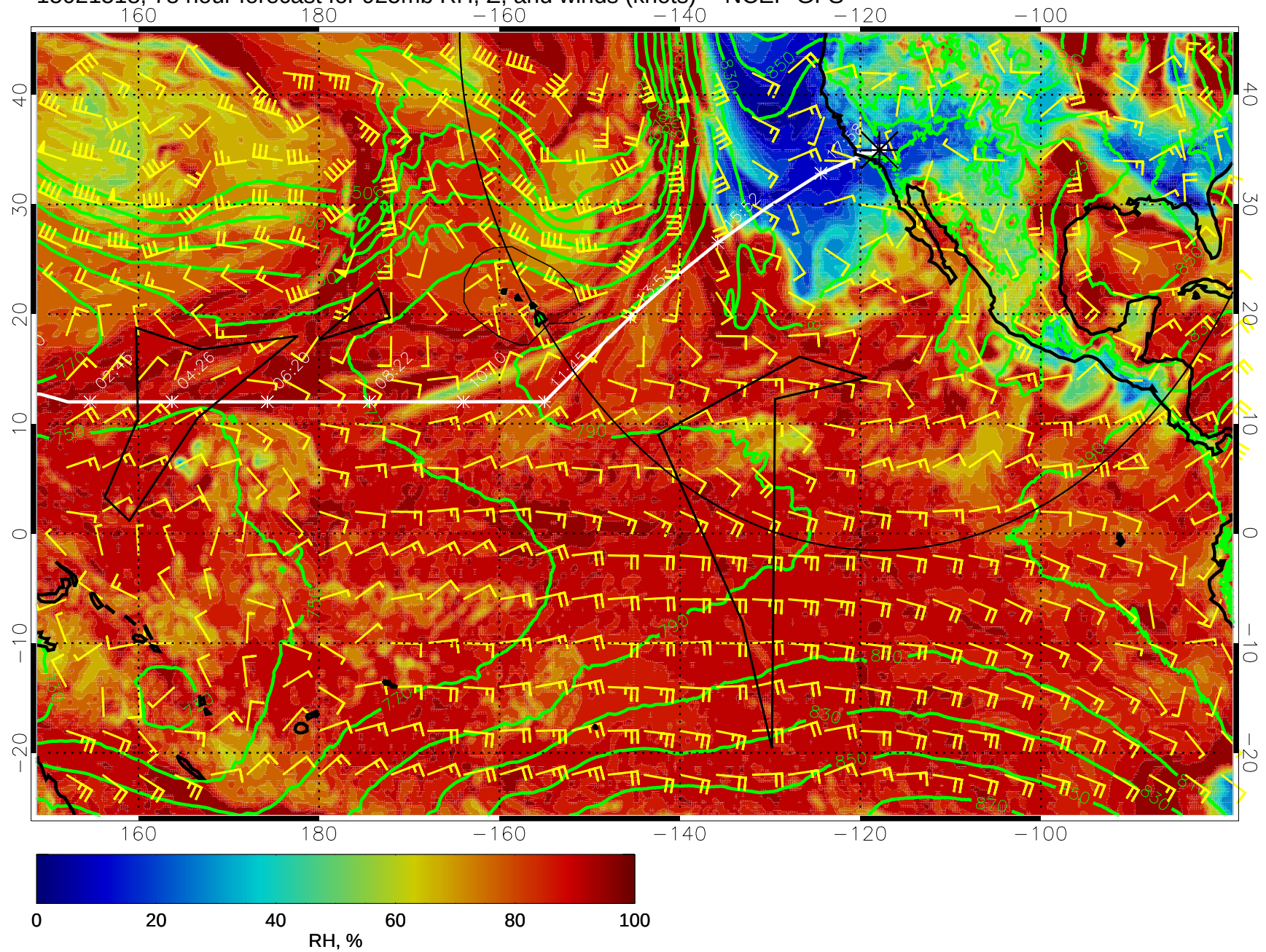
15021518, 78 hour forecast for 925mb RH, Z, and winds (knots) -- NCEP GFS
