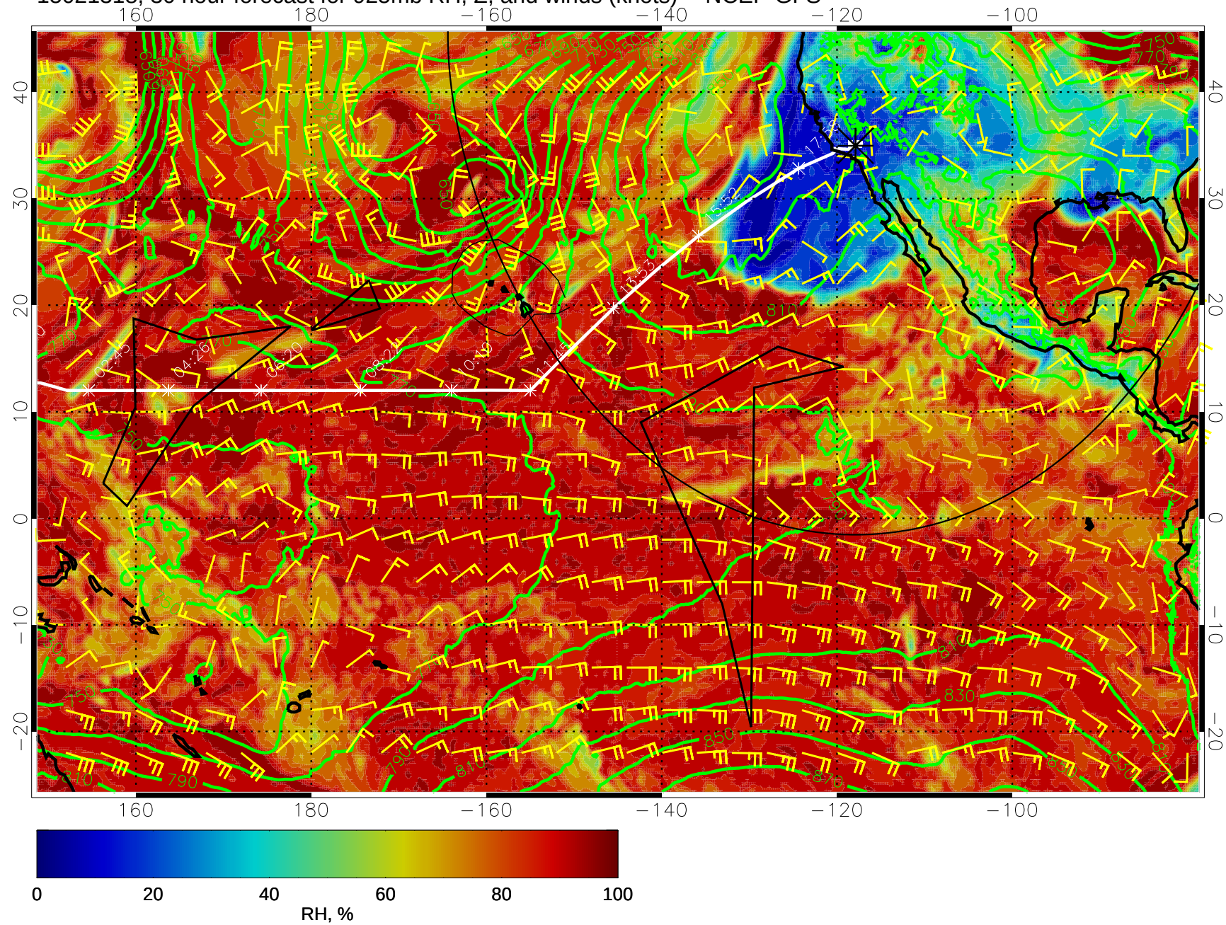
15021318, 30 hour forecast for 925mb RH, Z, and winds (knots) -- NCEP GFS
