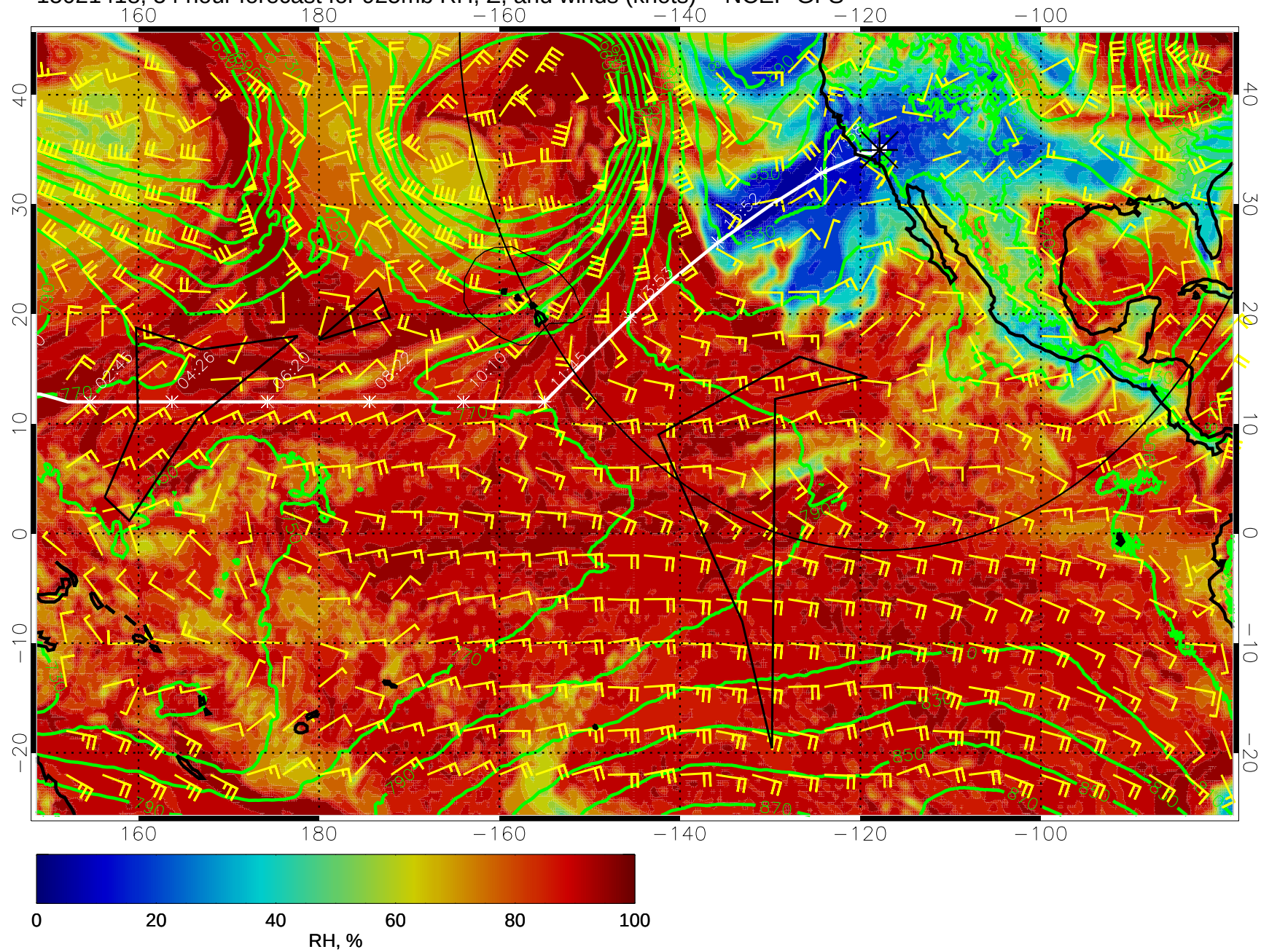
15021418, 54 hour forecast for 925mb RH, Z, and winds (knots) -- NCEP GFS
