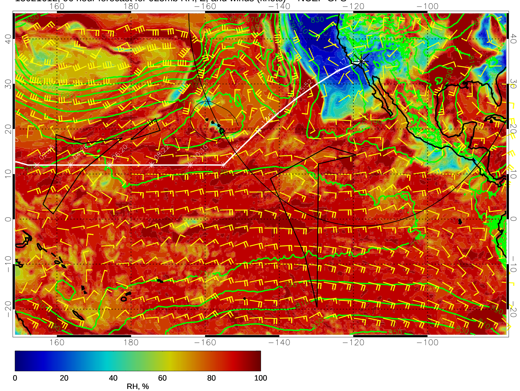
15021612, 96 hour forecast for 925mb RH, Z, and winds (knots) -- NCEP GFS
