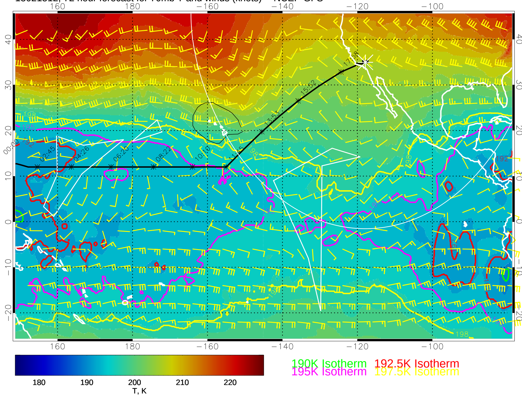
15021512, 72 hour forecast for 70mb T and winds (knots) -- NCEP GFS
