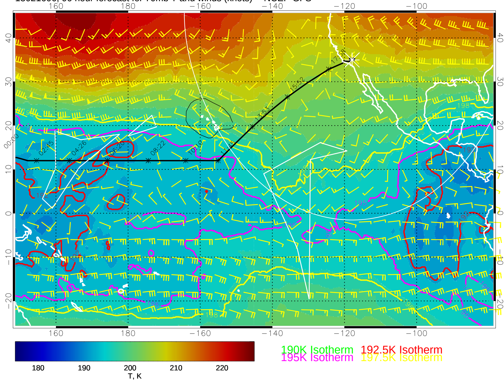
15021606, 90 hour forecast for 70mb T and winds (knots) -- NCEP GFS
