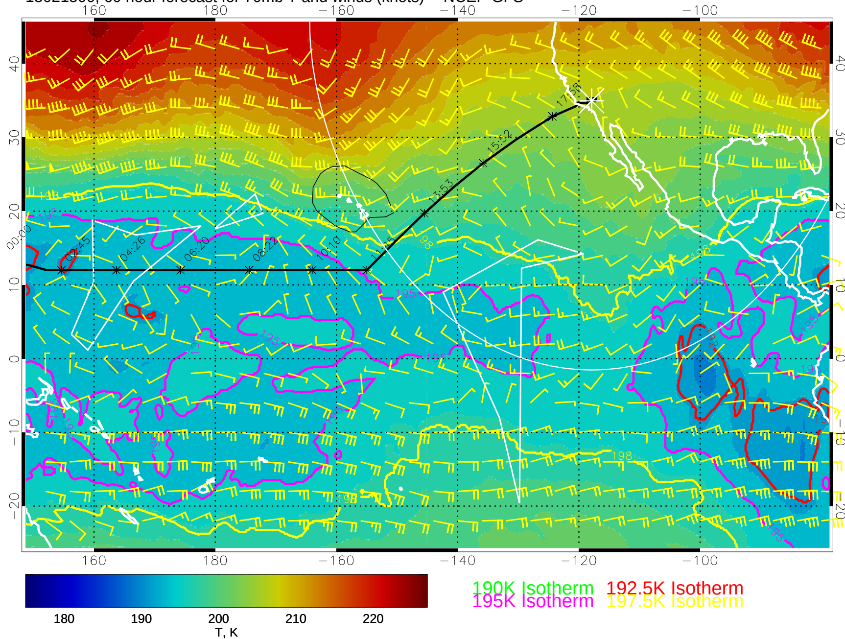
15021500, 60 hour forecast for 70mb T and winds (knots) -- NCEP GFS
