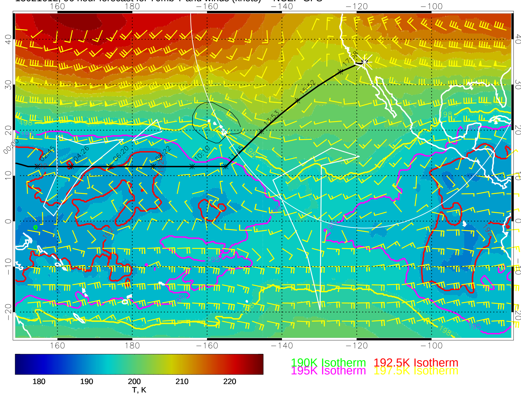
15021612, 96 hour forecast for 70mb T and winds (knots) -- NCEP GFS
