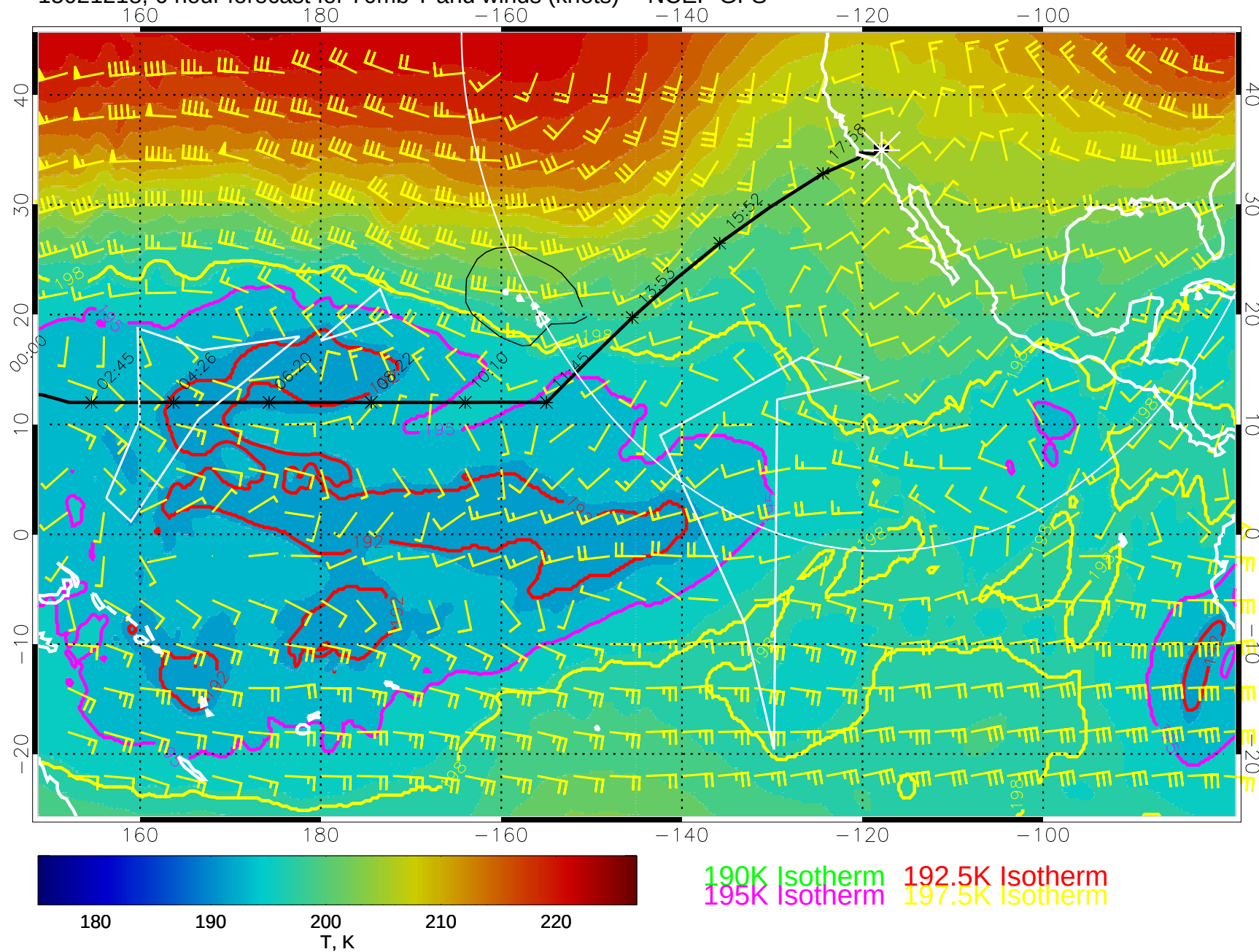
15021218, 6 hour forecast for 70mb T and winds (knots) -- NCEP GFS
