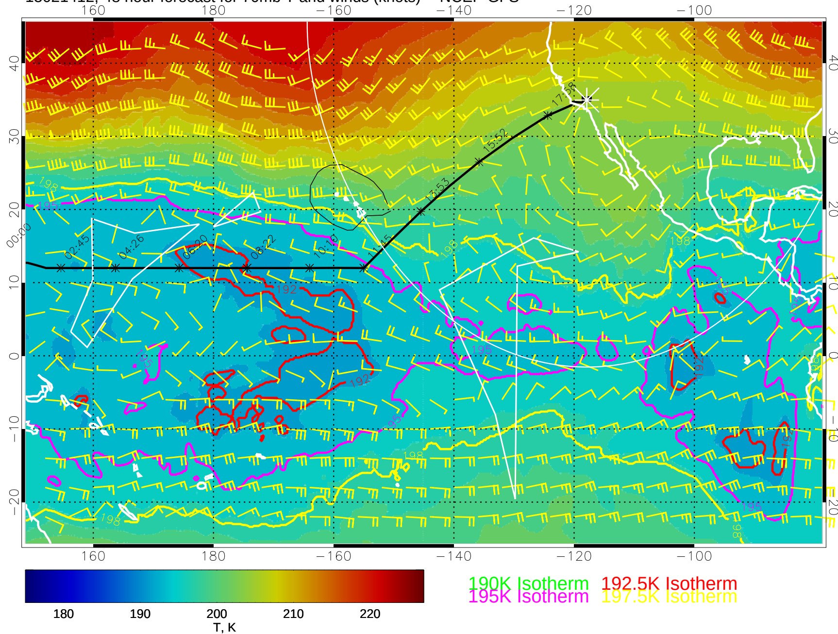
15021412, 48 hour forecast for 70mb T and winds (knots) -- NCEP GFS
