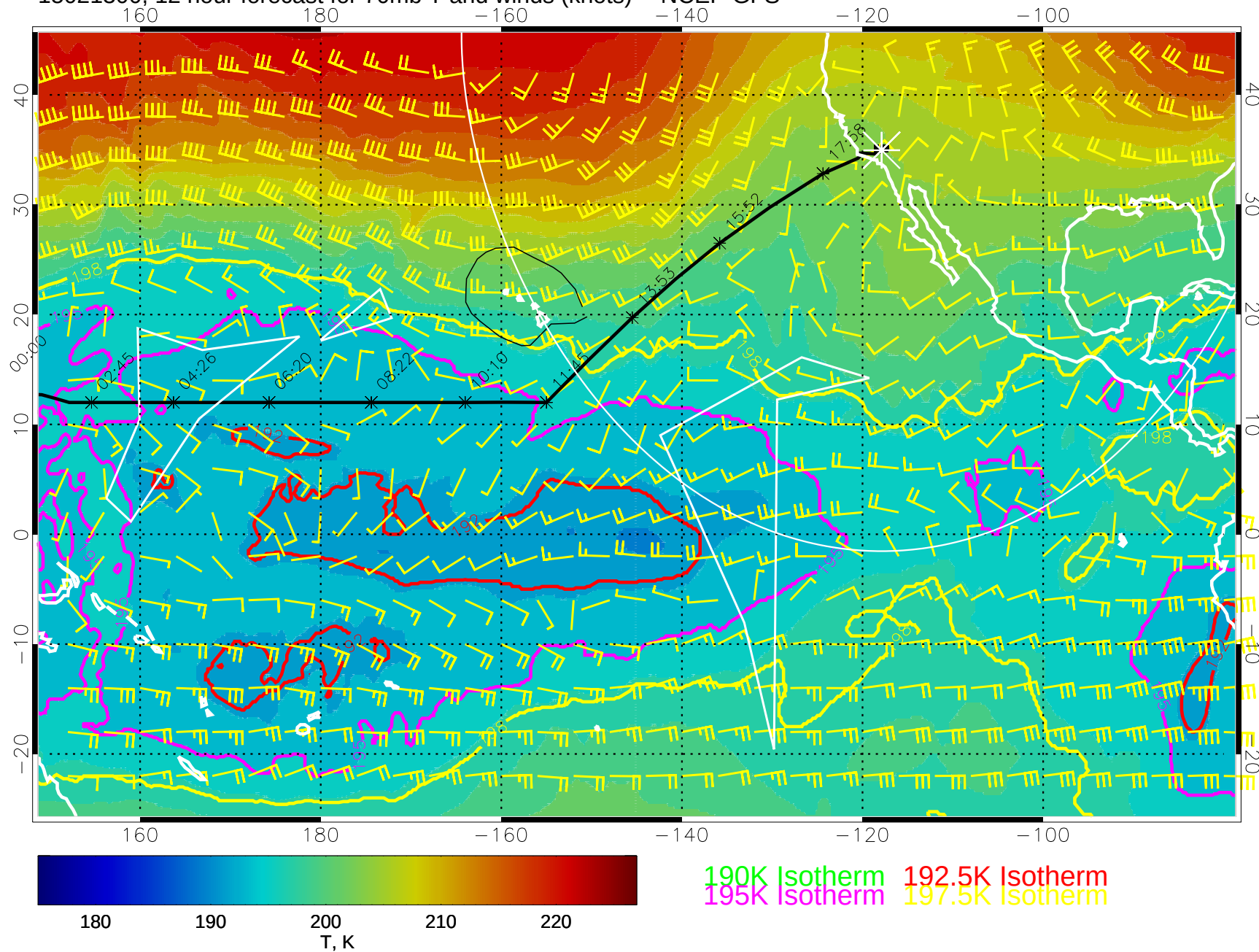
15021300, 12 hour forecast for 70mb T and winds (knots) -- NCEP GFS
