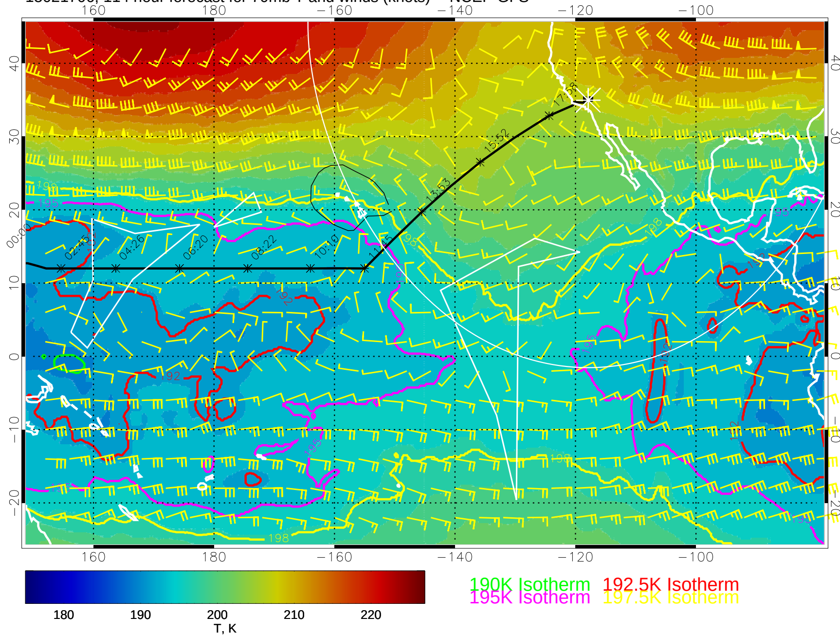
15021706, 114 hour forecast for 70mb T and winds (knots) -- NCEP GFS
