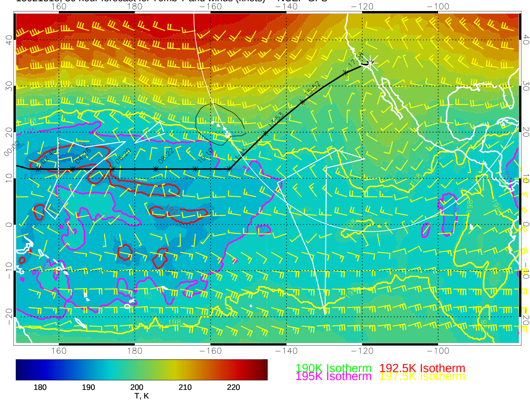
15021318, 30 hour forecast for 70mb T and winds (knots) -- NCEP GFS
