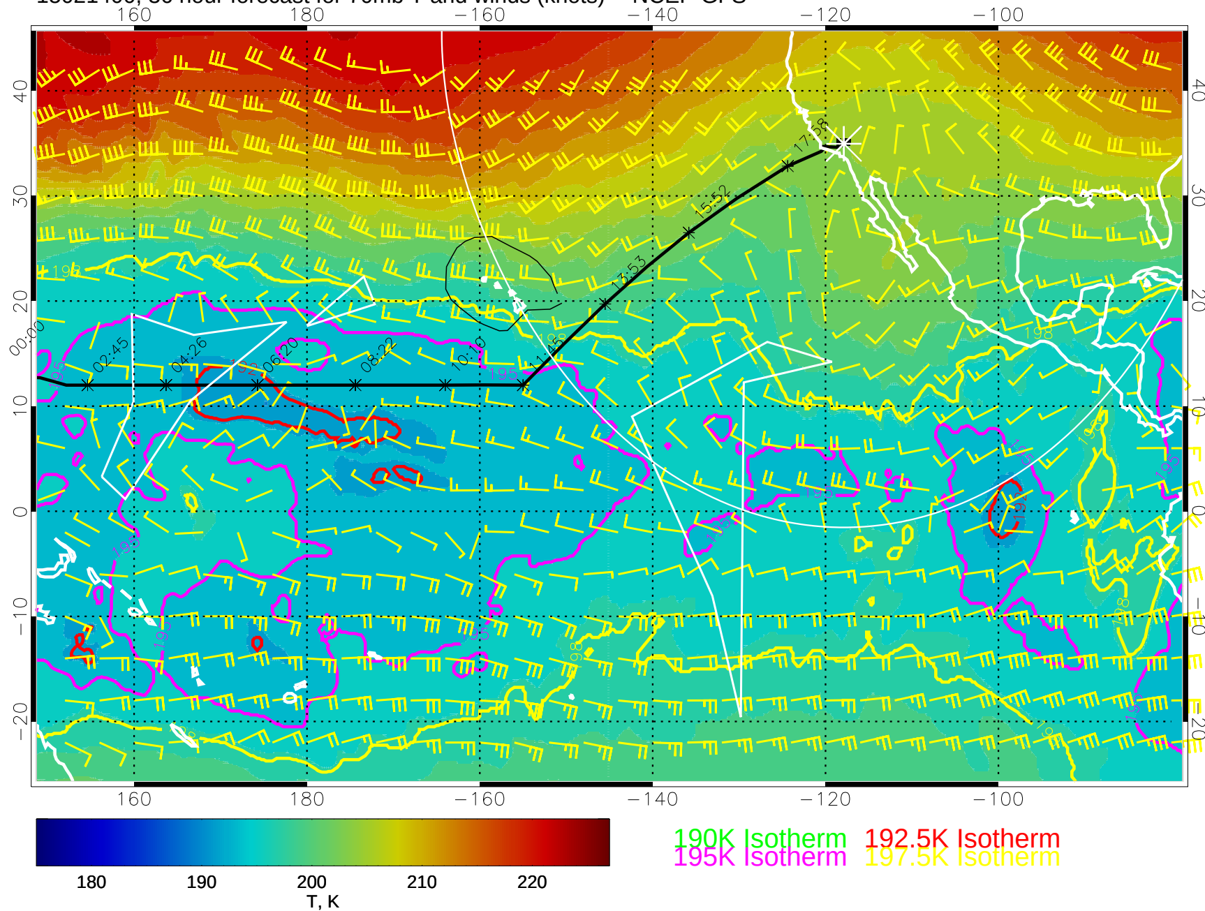
15021400, 36 hour forecast for 70mb T and winds (knots) -- NCEP GFS
