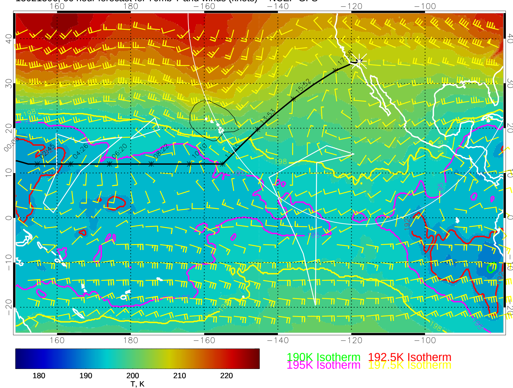
15021506, 66 hour forecast for 70mb T and winds (knots) -- NCEP GFS
