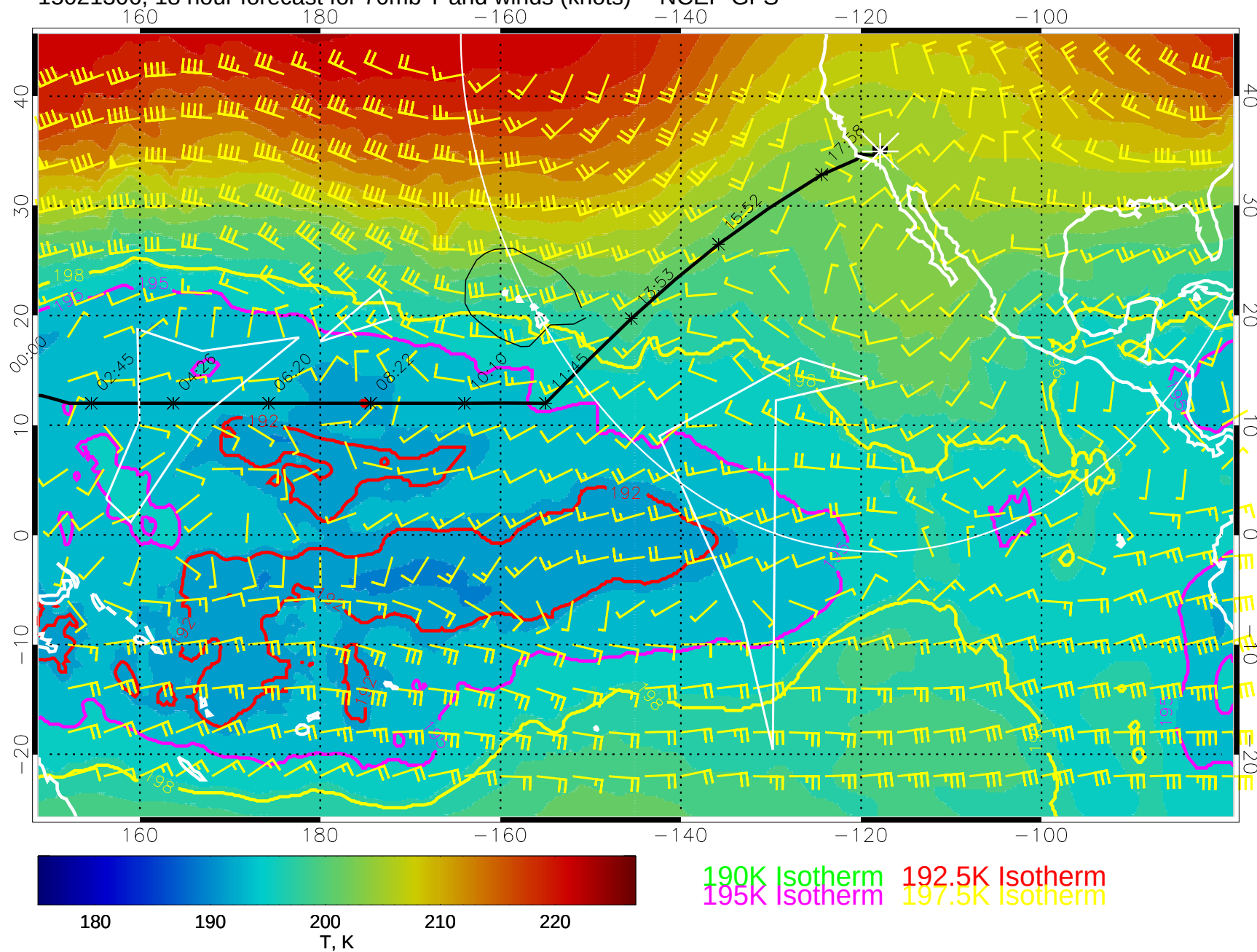
15021306, 18 hour forecast for 70mb T and winds (knots) -- NCEP GFS
