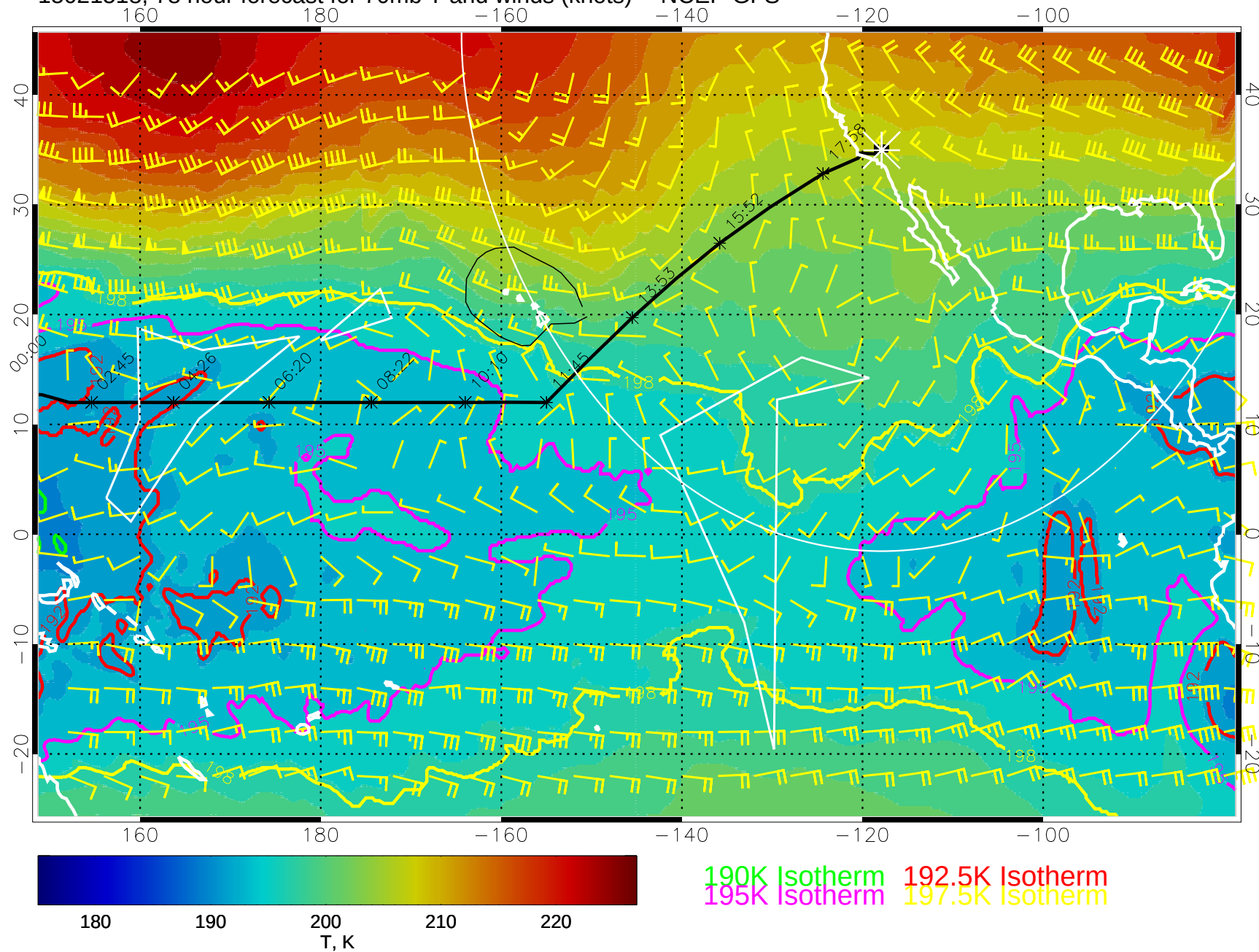
15021518, 78 hour forecast for 70mb T and winds (knots) -- NCEP GFS
