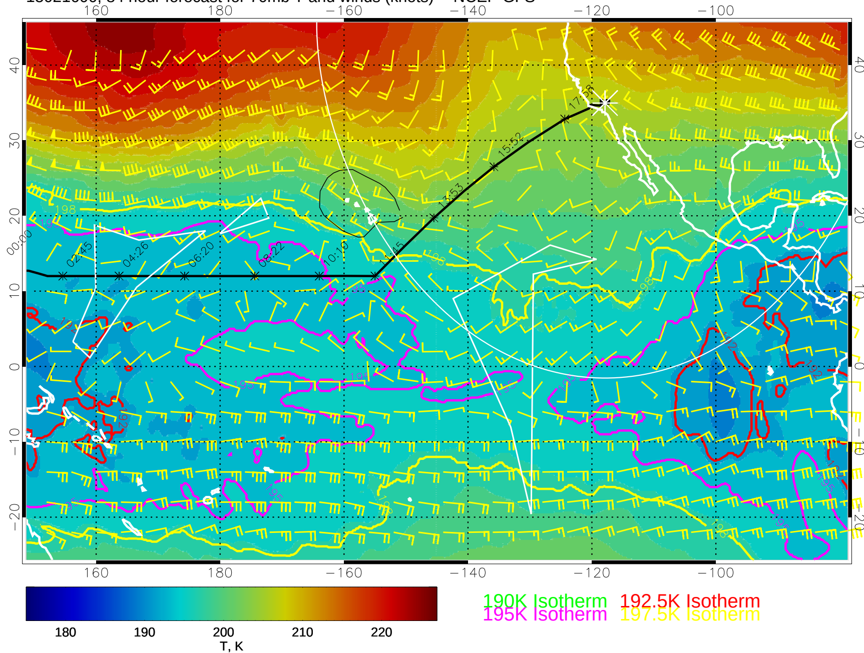
15021600, 84 hour forecast for 70mb T and winds (knots) -- NCEP GFS
