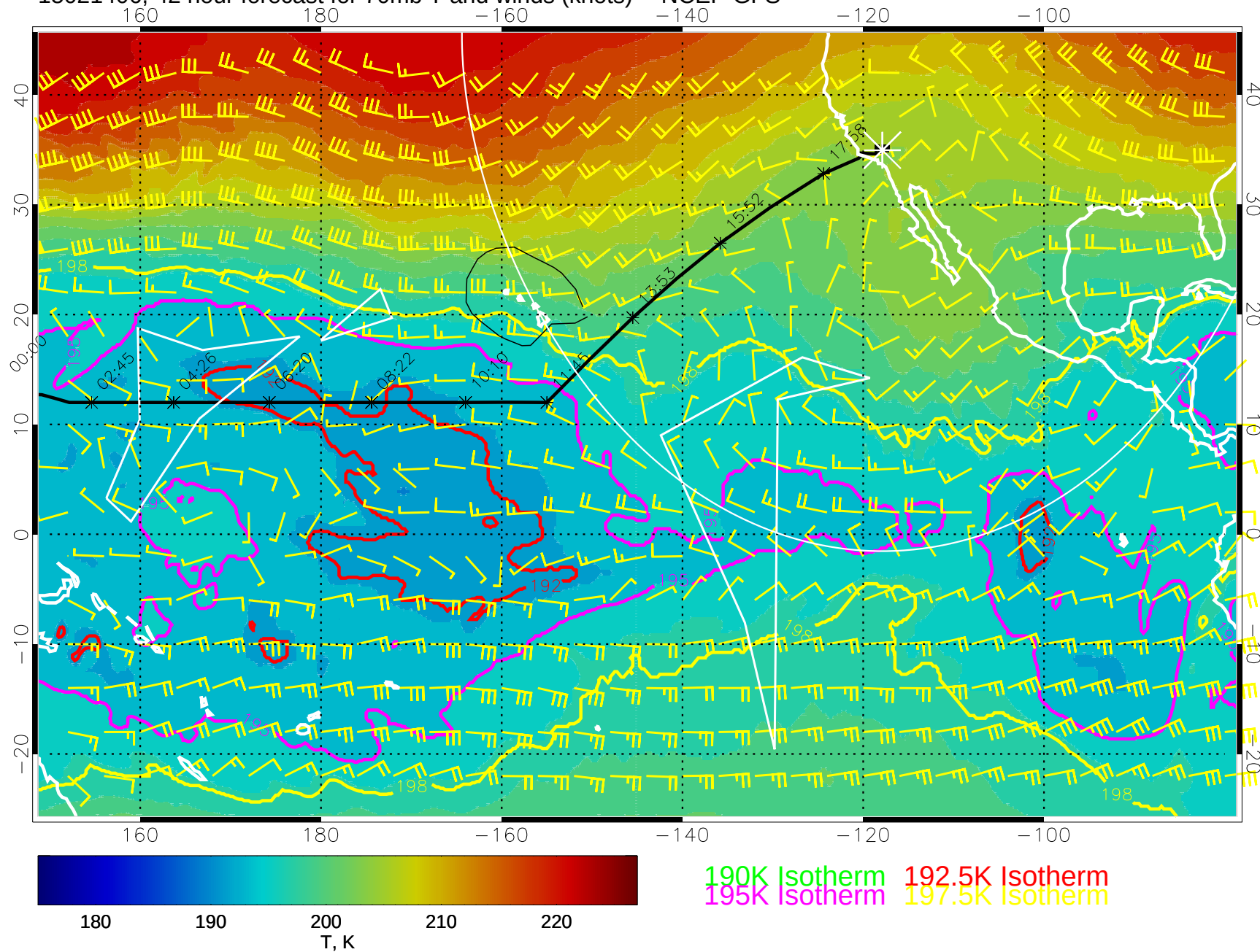
15021406, 42 hour forecast for 70mb T and winds (knots) -- NCEP GFS
