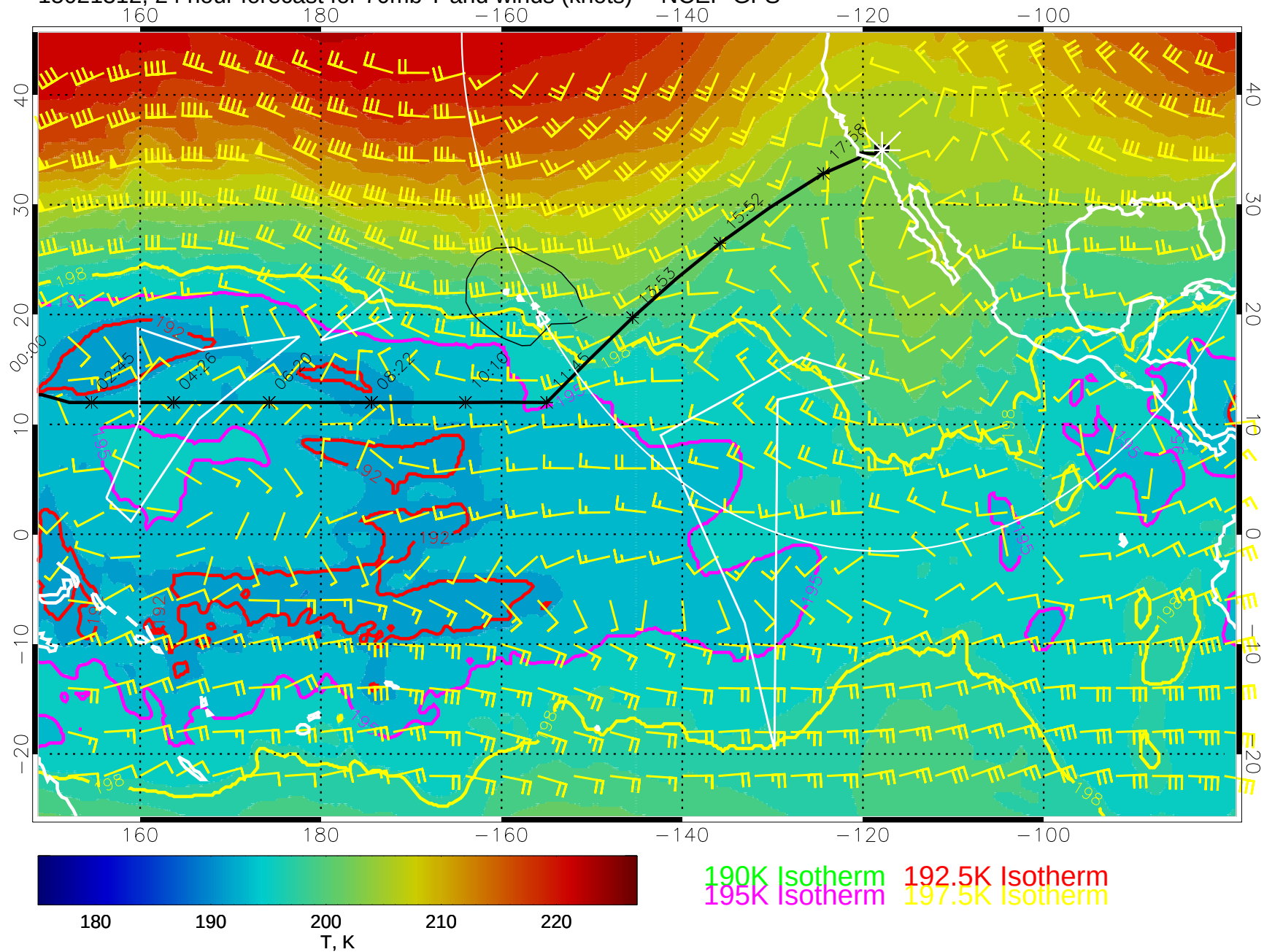
15021312, 24 hour forecast for 70mb T and winds (knots) -- NCEP GFS
