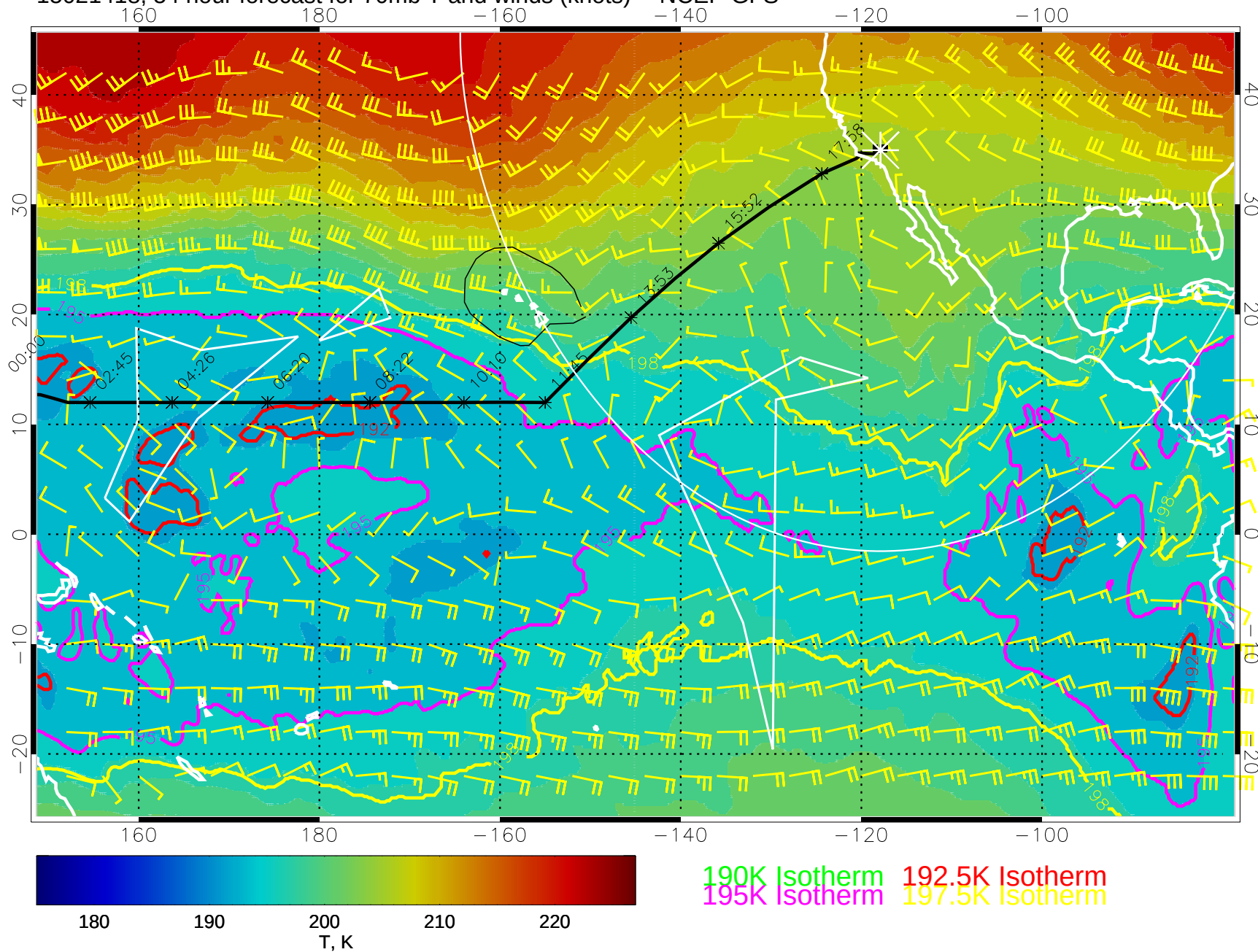
15021418, 54 hour forecast for 70mb T and winds (knots) -- NCEP GFS
