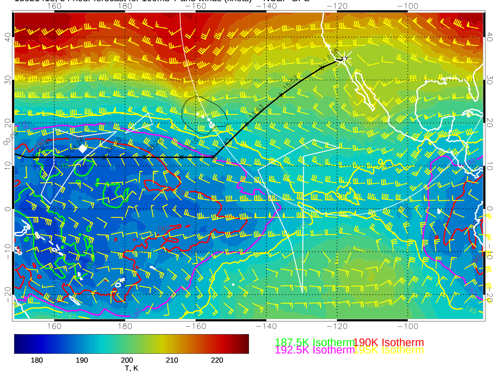
15021418, 54 hour forecast for 100mb T and winds (knots) -- NCEP GFS
