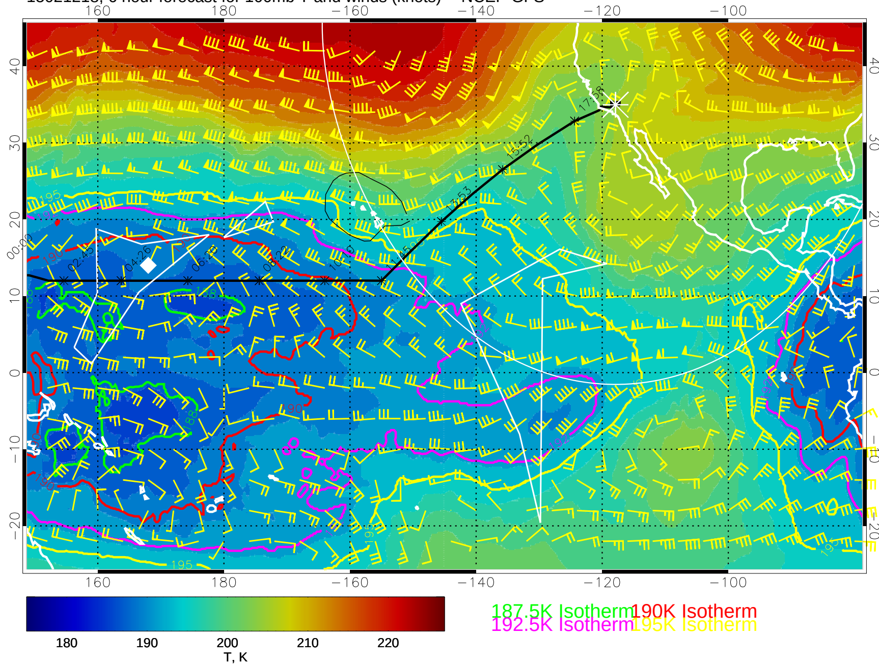
15021218, 6 hour forecast for 100mb T and winds (knots) -- NCEP GFS
