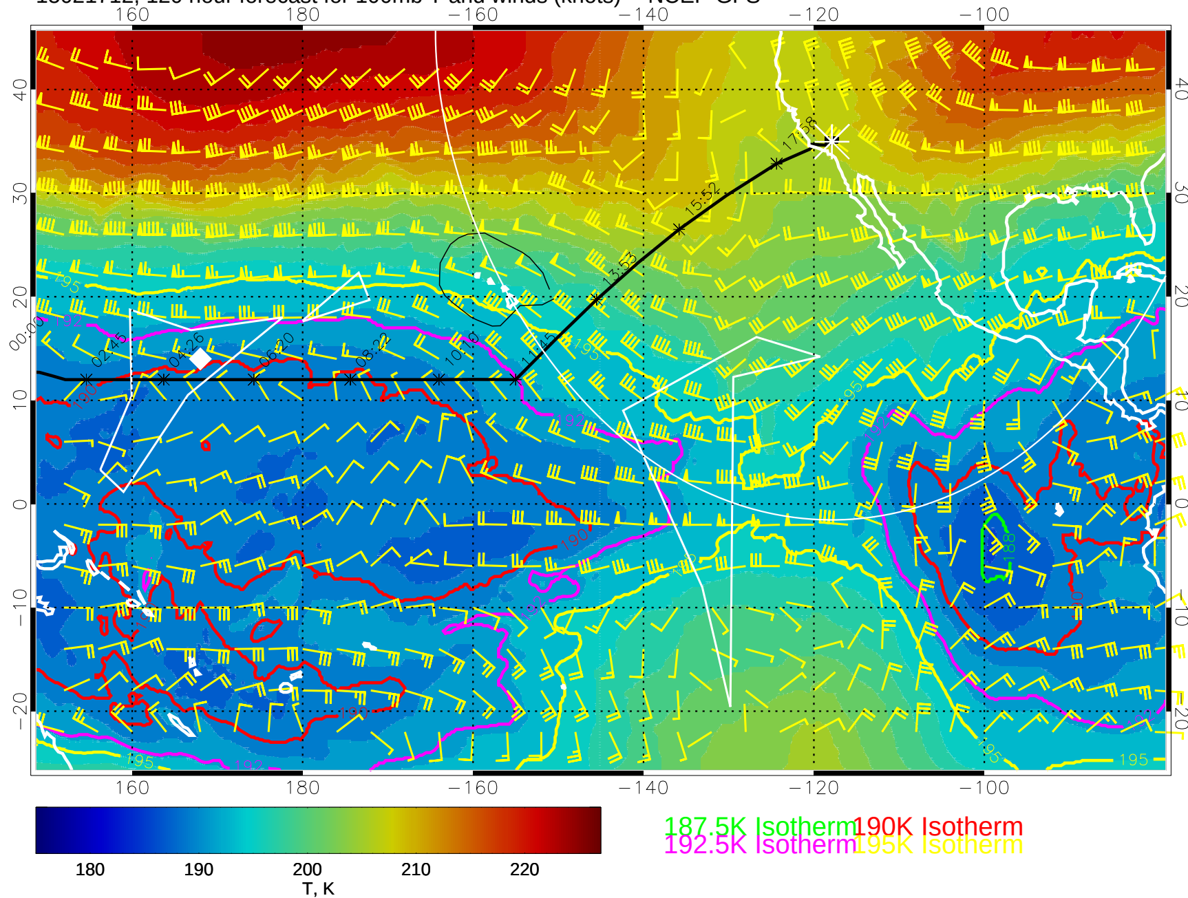
15021712, 120 hour forecast for 100mb T and winds (knots) -- NCEP GFS
