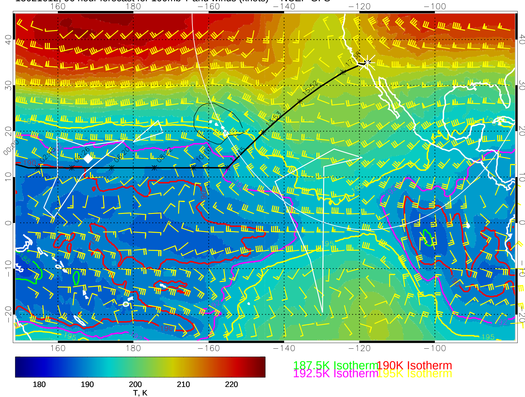
15021612, 96 hour forecast for 100mb T and winds (knots) -- NCEP GFS
