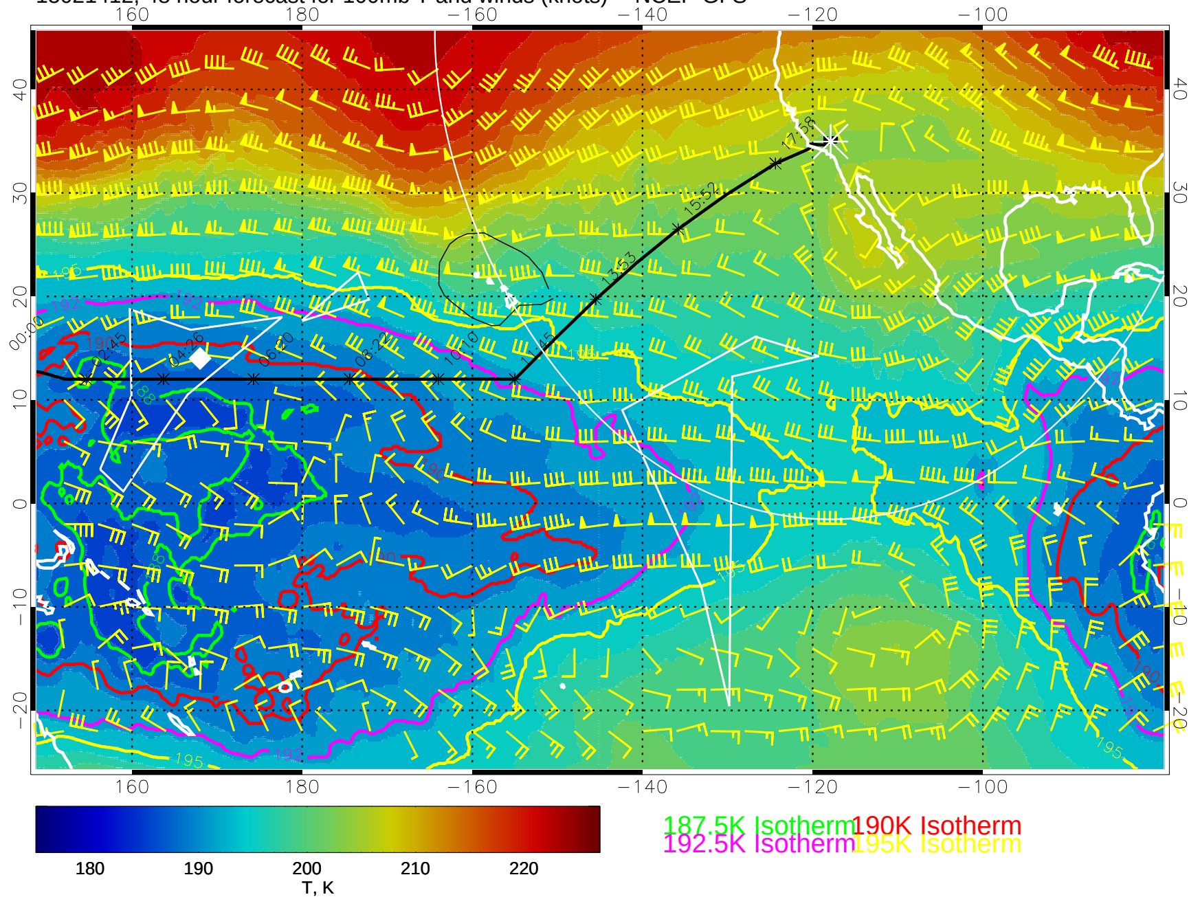
15021412, 48 hour forecast for 100mb T and winds (knots) -- NCEP GFS
