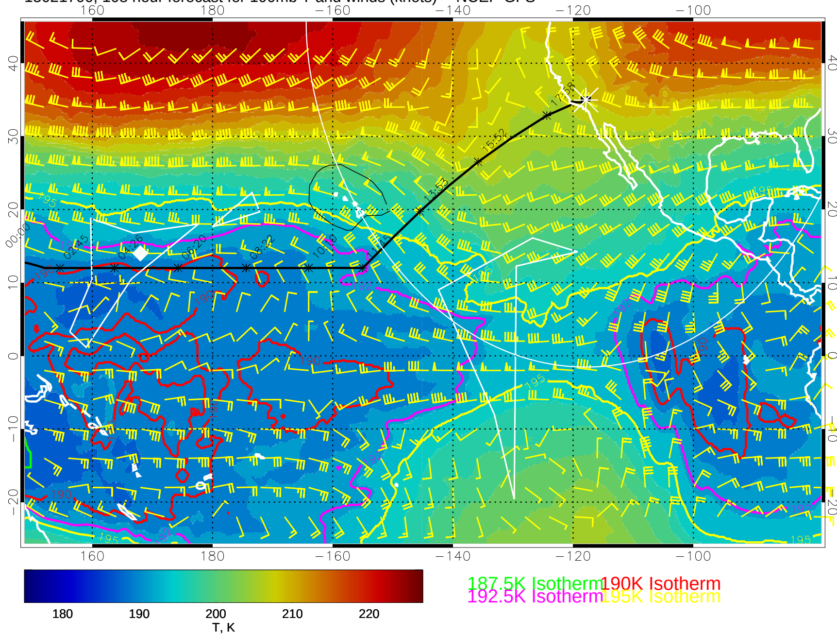
15021700, 108 hour forecast for 100mb T and winds (knots) -- NCEP GFS
