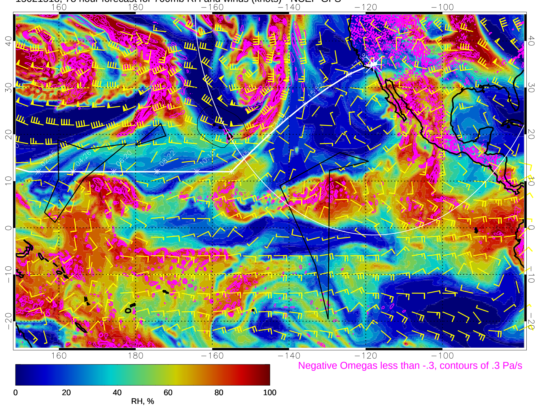
15021518, 78 hour forecast for 700mb RH and winds (knots) - NCEP GFS
