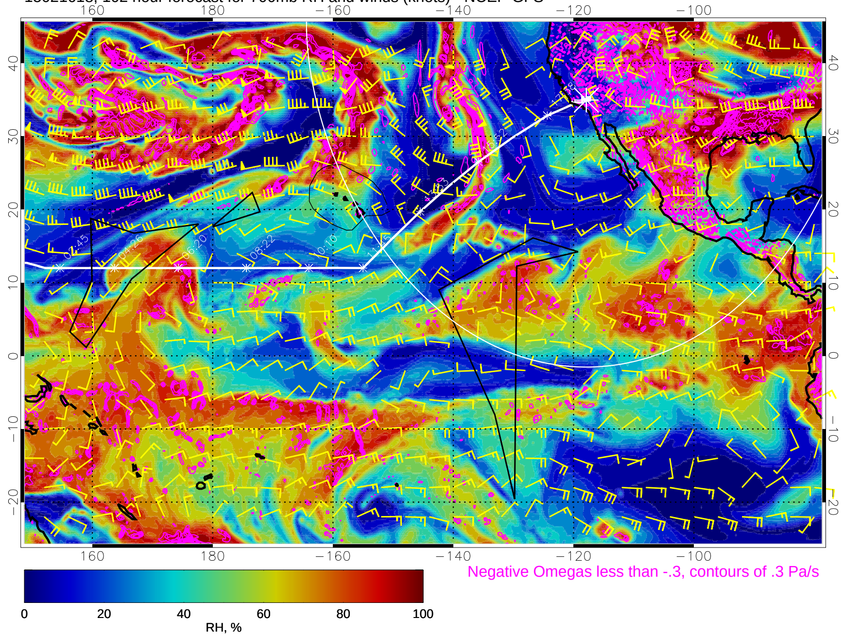
15021618, 102 hour forecast for 700mb RH and winds (knots) - NCEP GFS
