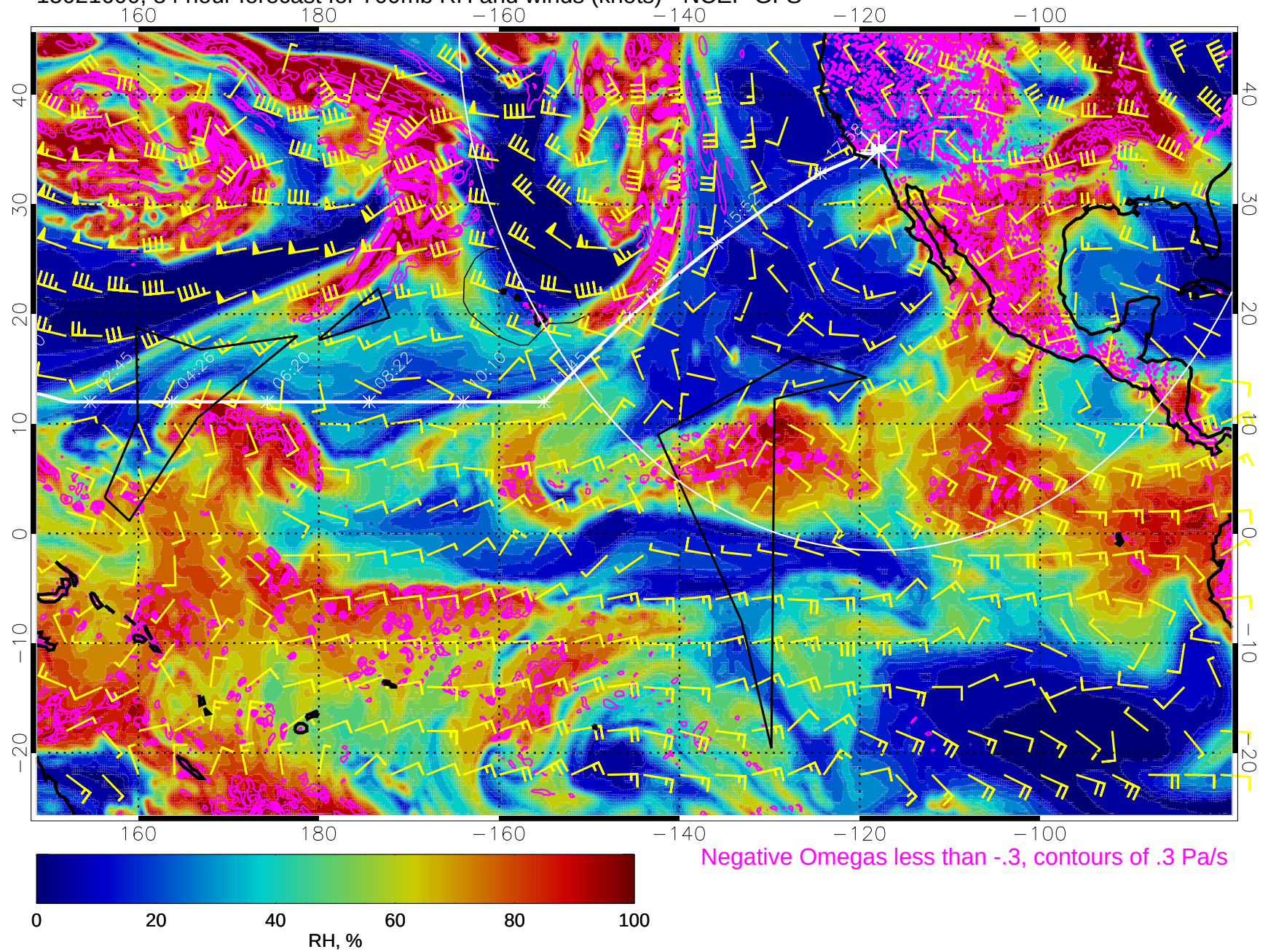
15021600, 84 hour forecast for 700mb RH and winds (knots) - NCEP GFS
