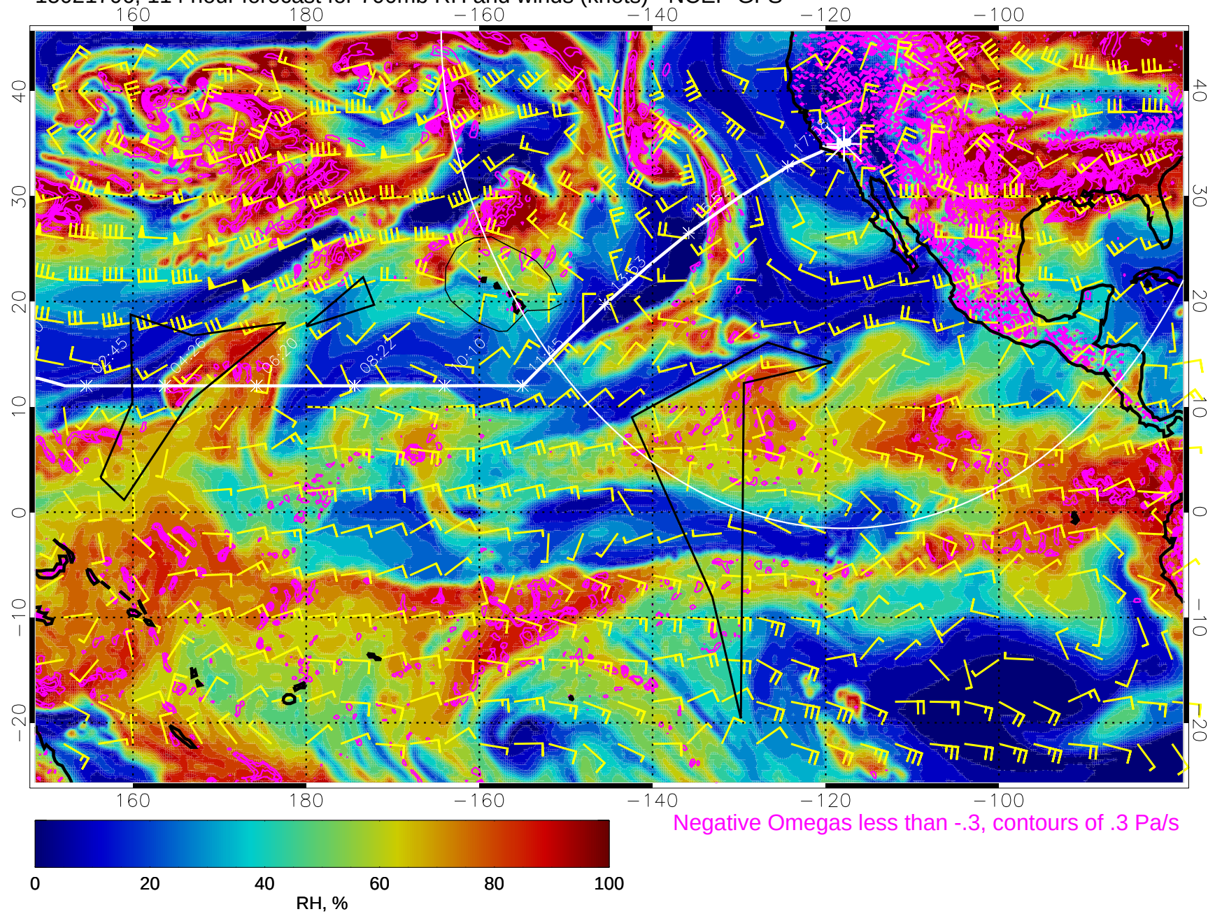
15021706, 114 hour forecast for 700mb RH and winds (knots) - NCEP GFS
