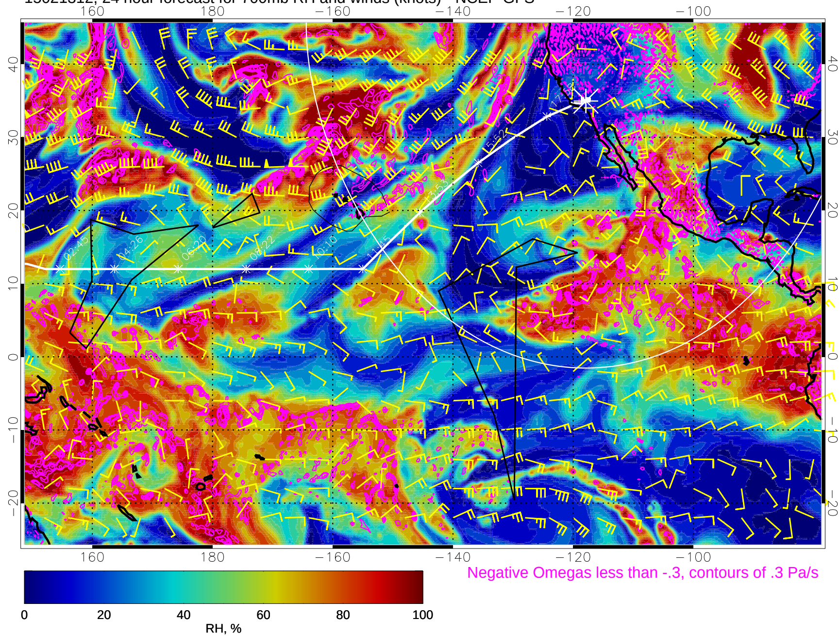
15021312, 24 hour forecast for 700mb RH and winds (knots) - NCEP GFS
