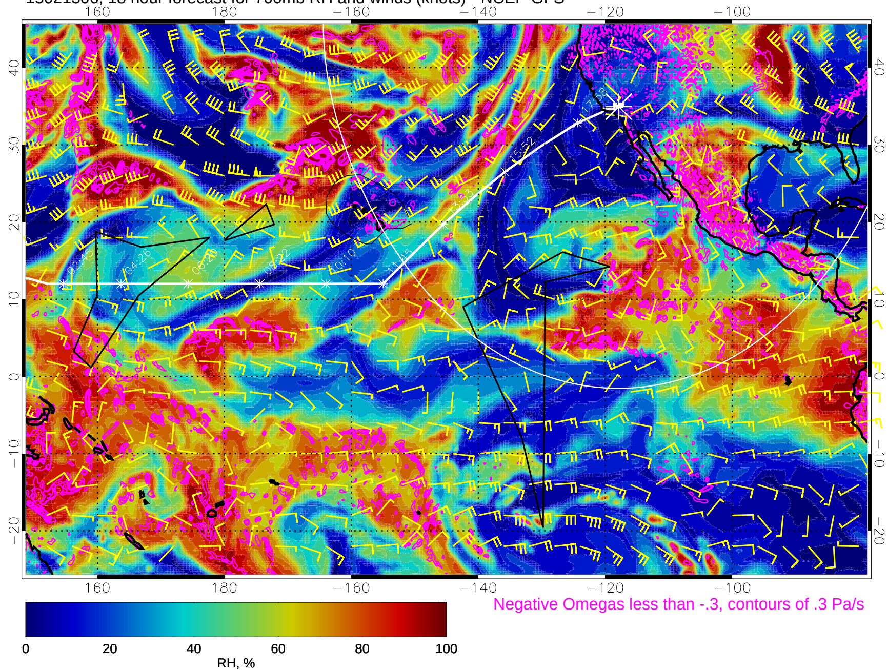
15021306, 18 hour forecast for 700mb RH and winds (knots) - NCEP GFS
