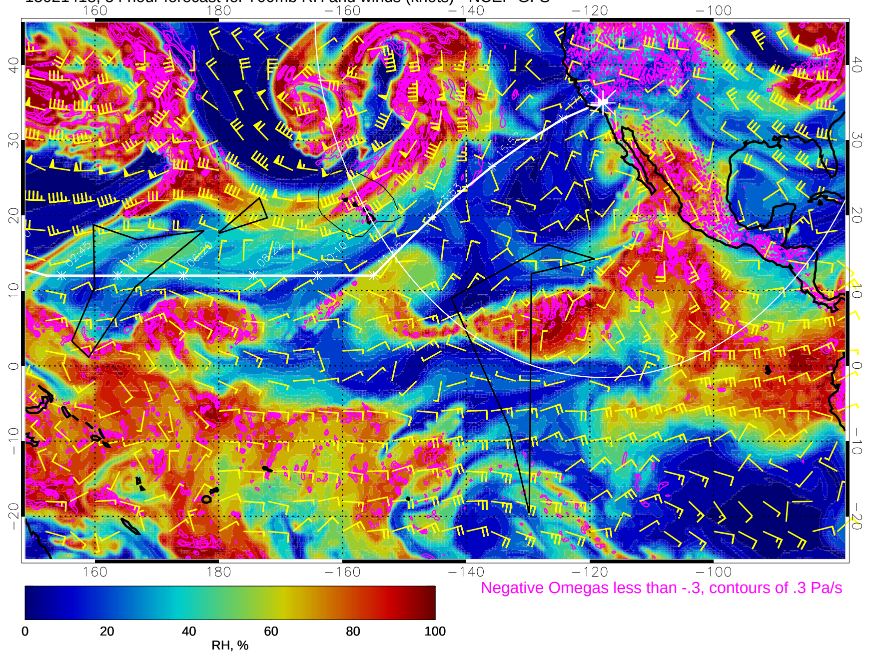
15021418, 54 hour forecast for 700mb RH and winds (knots) - NCEP GFS
