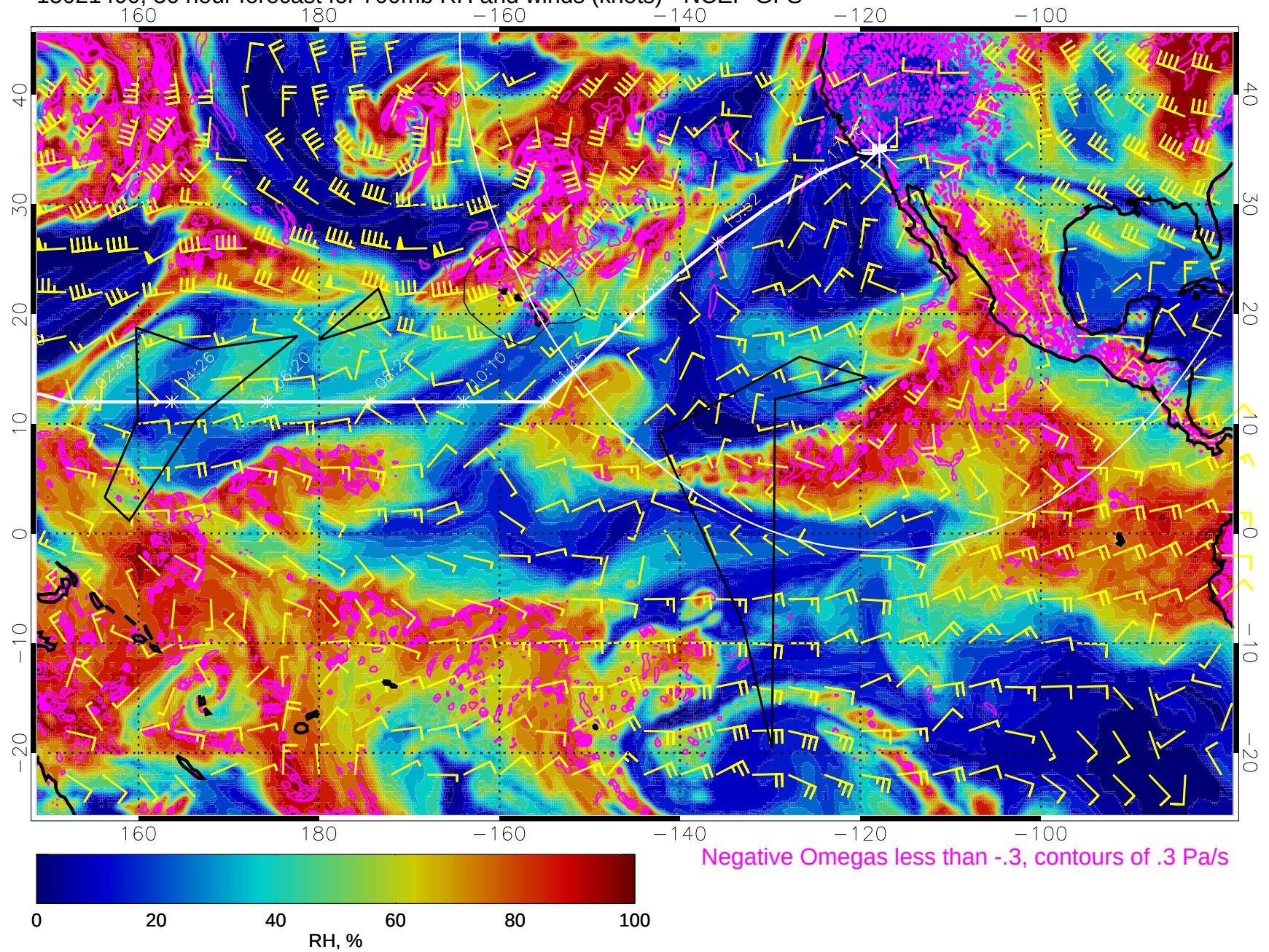
15021400, 36 hour forecast for 700mb RH and winds (knots) - NCEP GFS
