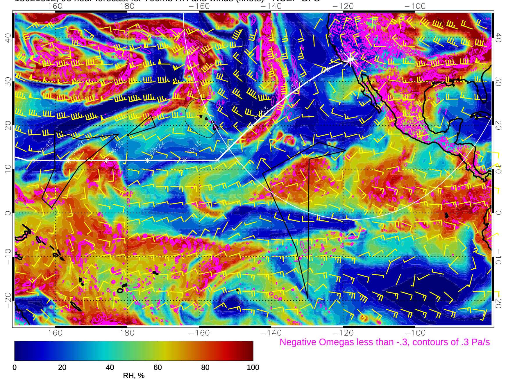
15021612, 96 hour forecast for 700mb RH and winds (knots) - NCEP GFS
