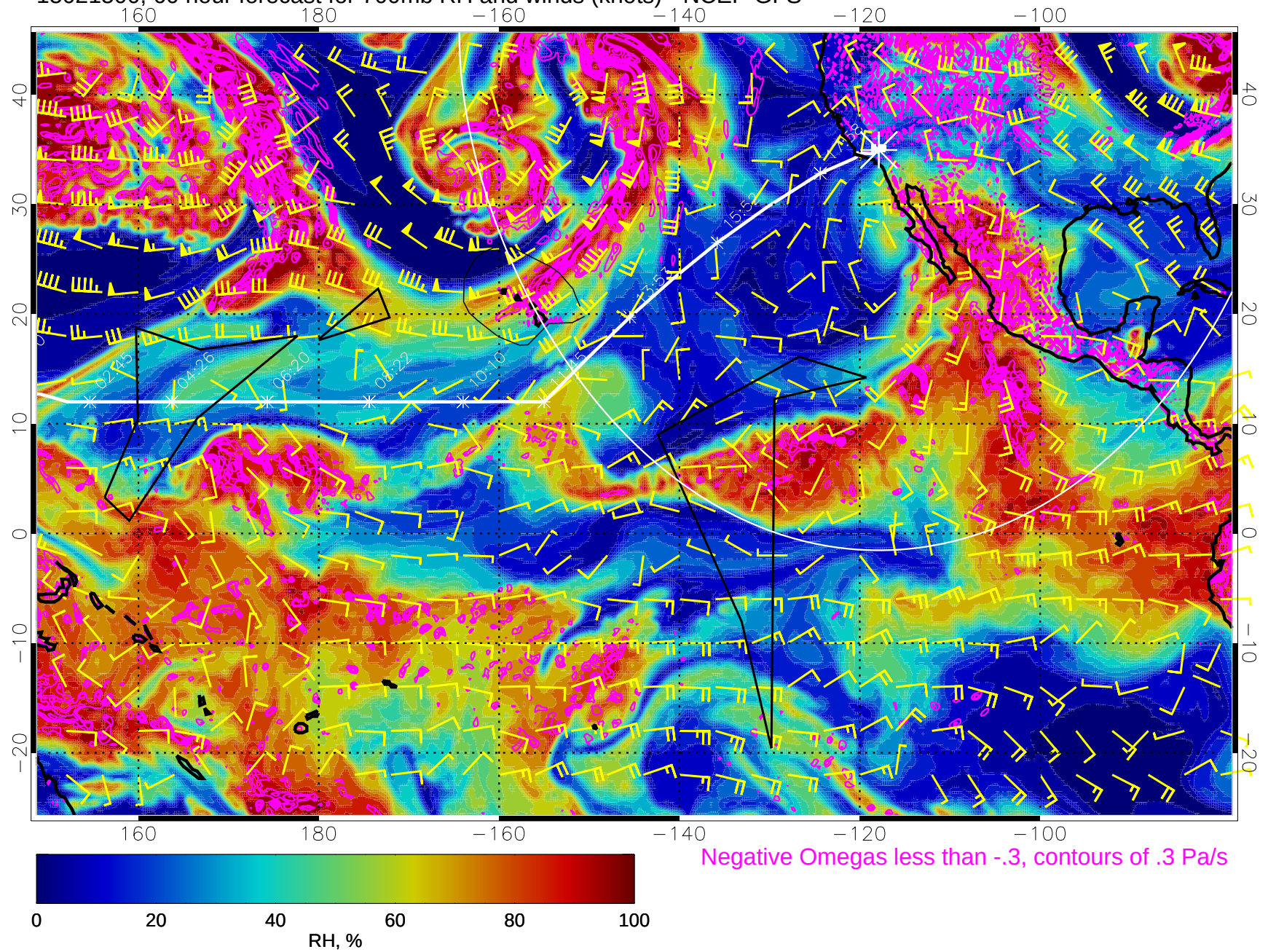
15021500, 60 hour forecast for 700mb RH and winds (knots) - NCEP GFS
