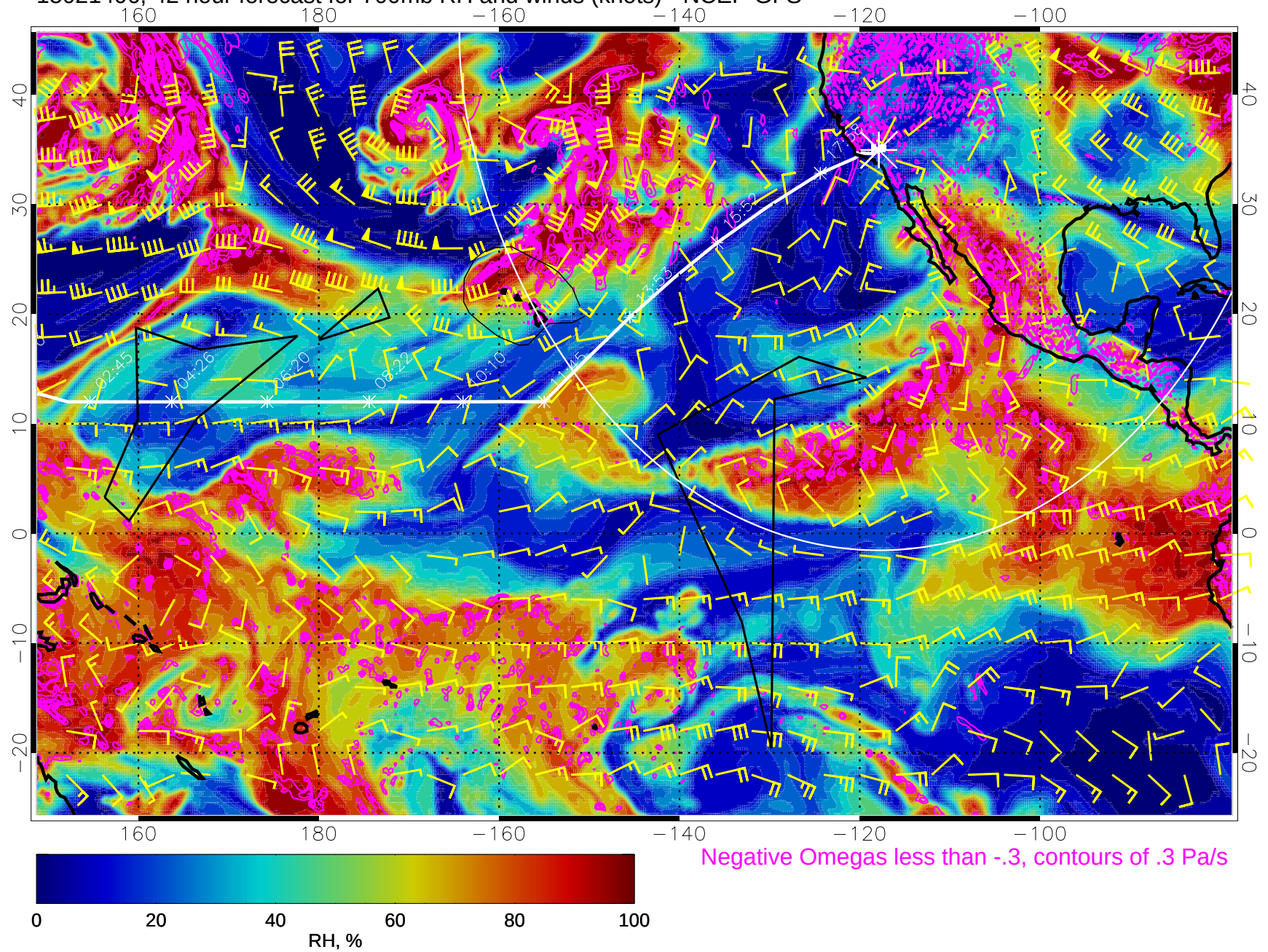
15021406, 42 hour forecast for 700mb RH and winds (knots) - NCEP GFS
