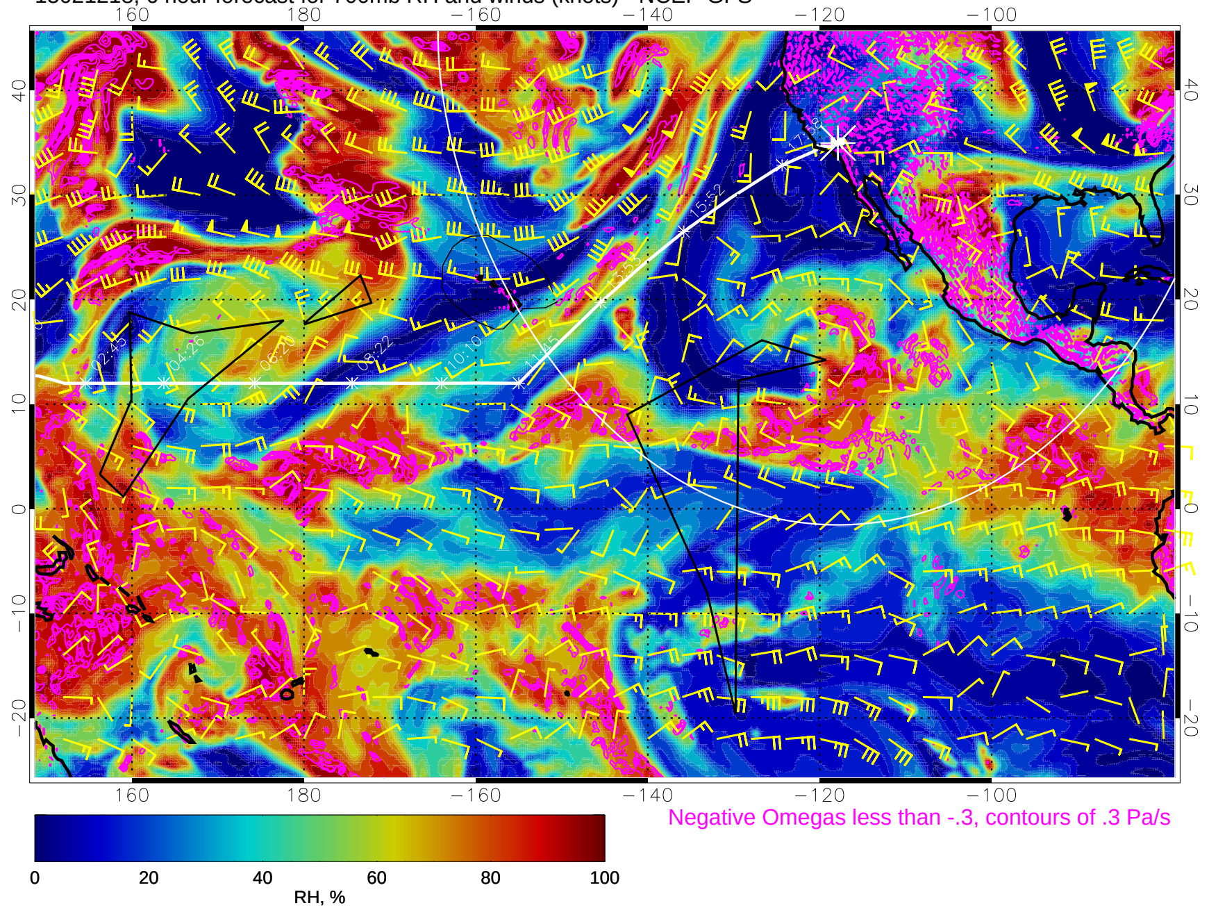
15021218, 6 hour forecast for 700mb RH and winds (knots) - NCEP GFS
