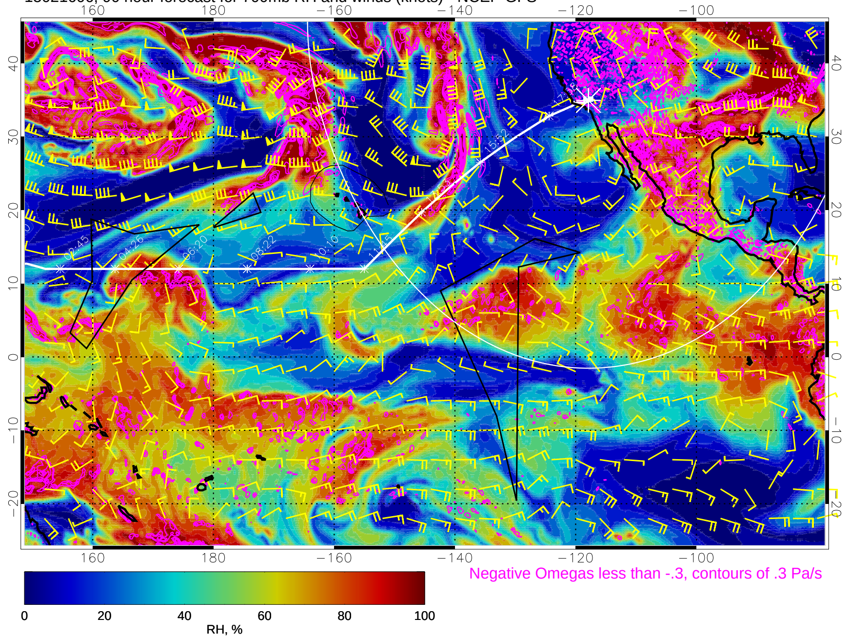
15021606, 90 hour forecast for 700mb RH and winds (knots) - NCEP GFS
