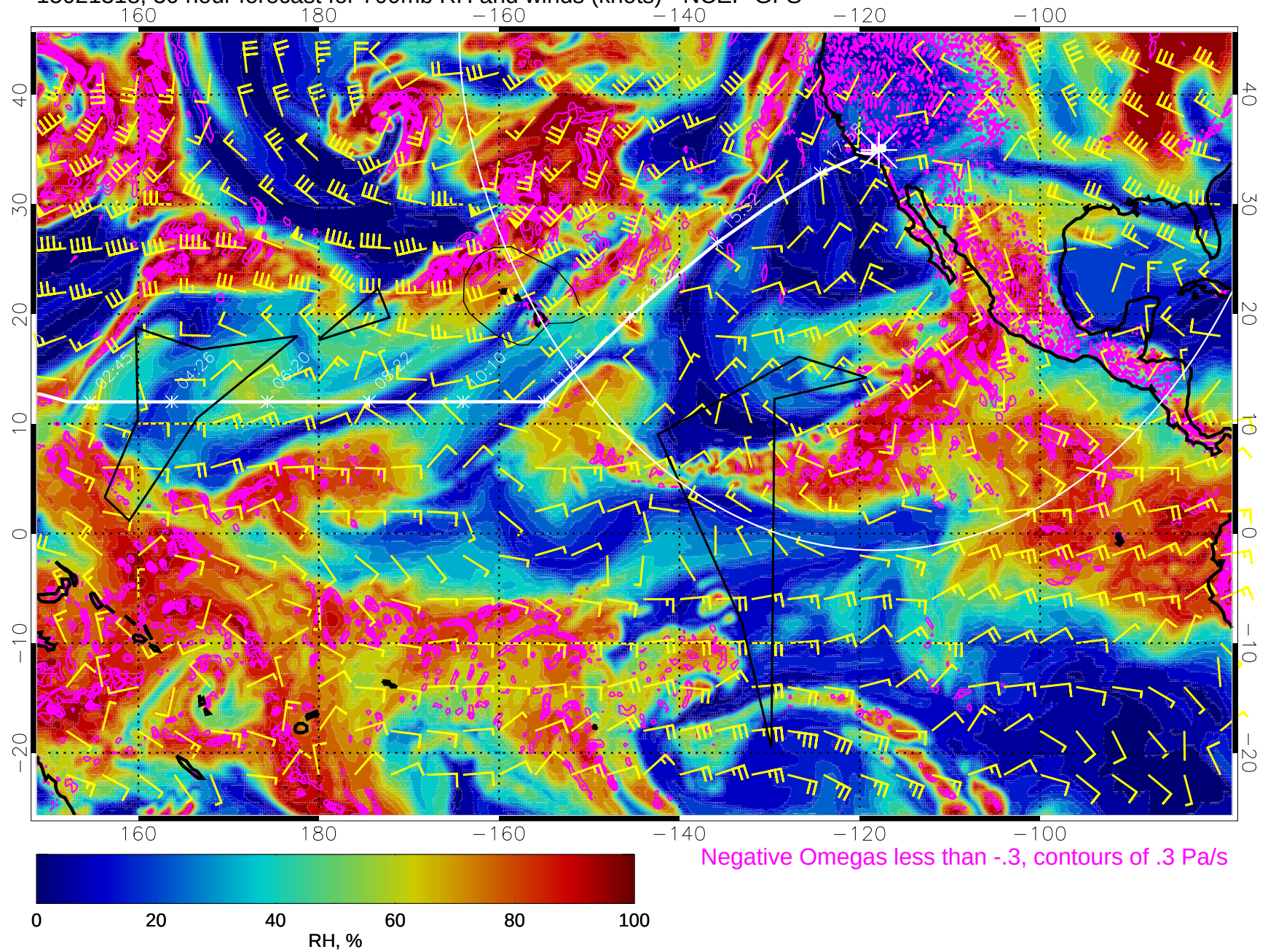
15021318, 30 hour forecast for 700mb RH and winds (knots) - NCEP GFS
