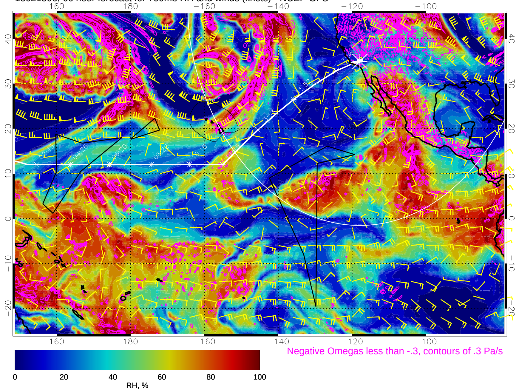
15021506, 66 hour forecast for 700mb RH and winds (knots) - NCEP GFS
