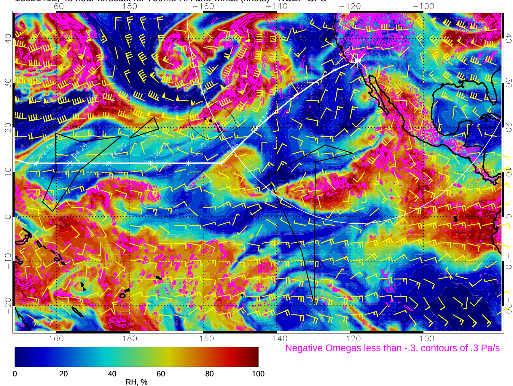
15021412, 48 hour forecast for 700mb RH and winds (knots) - NCEP GFS
