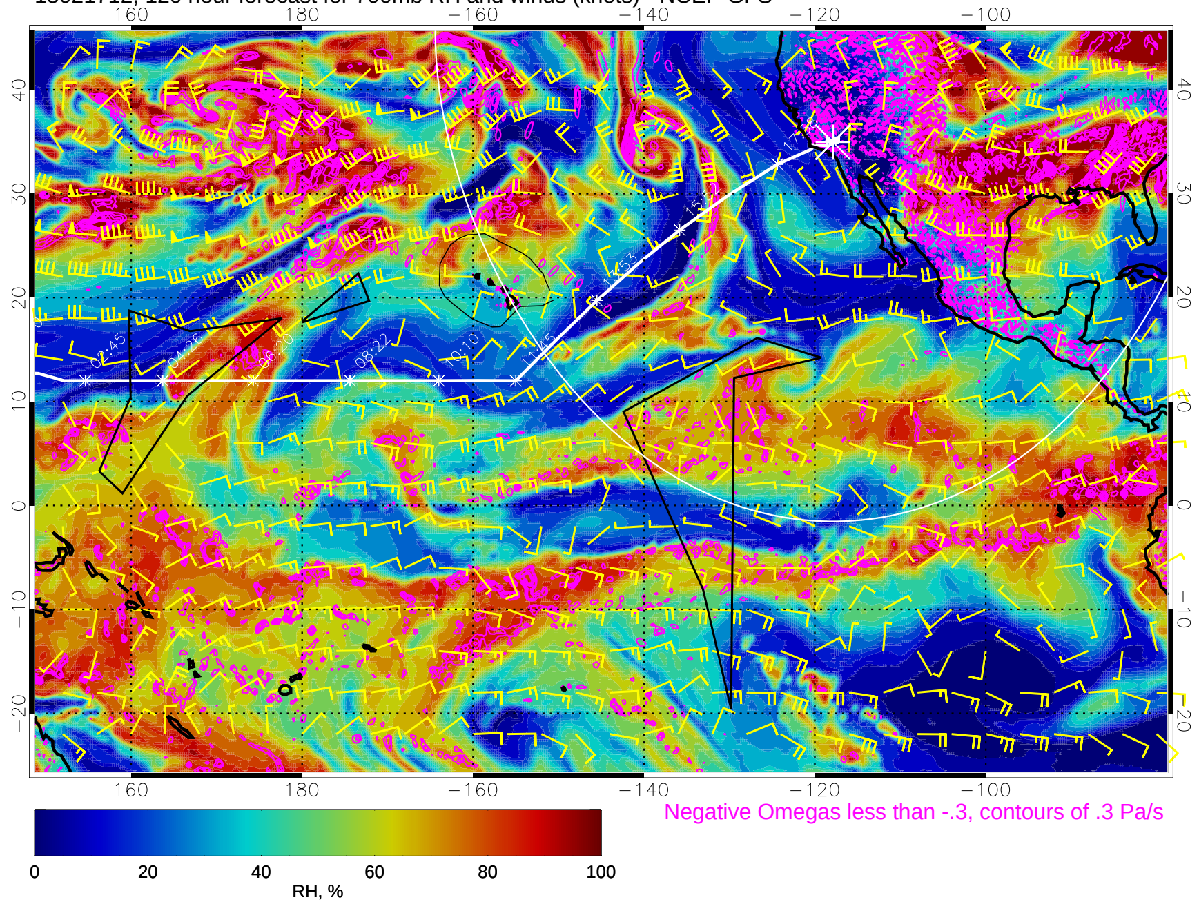
15021712, 120 hour forecast for 700mb RH and winds (knots) - NCEP GFS
