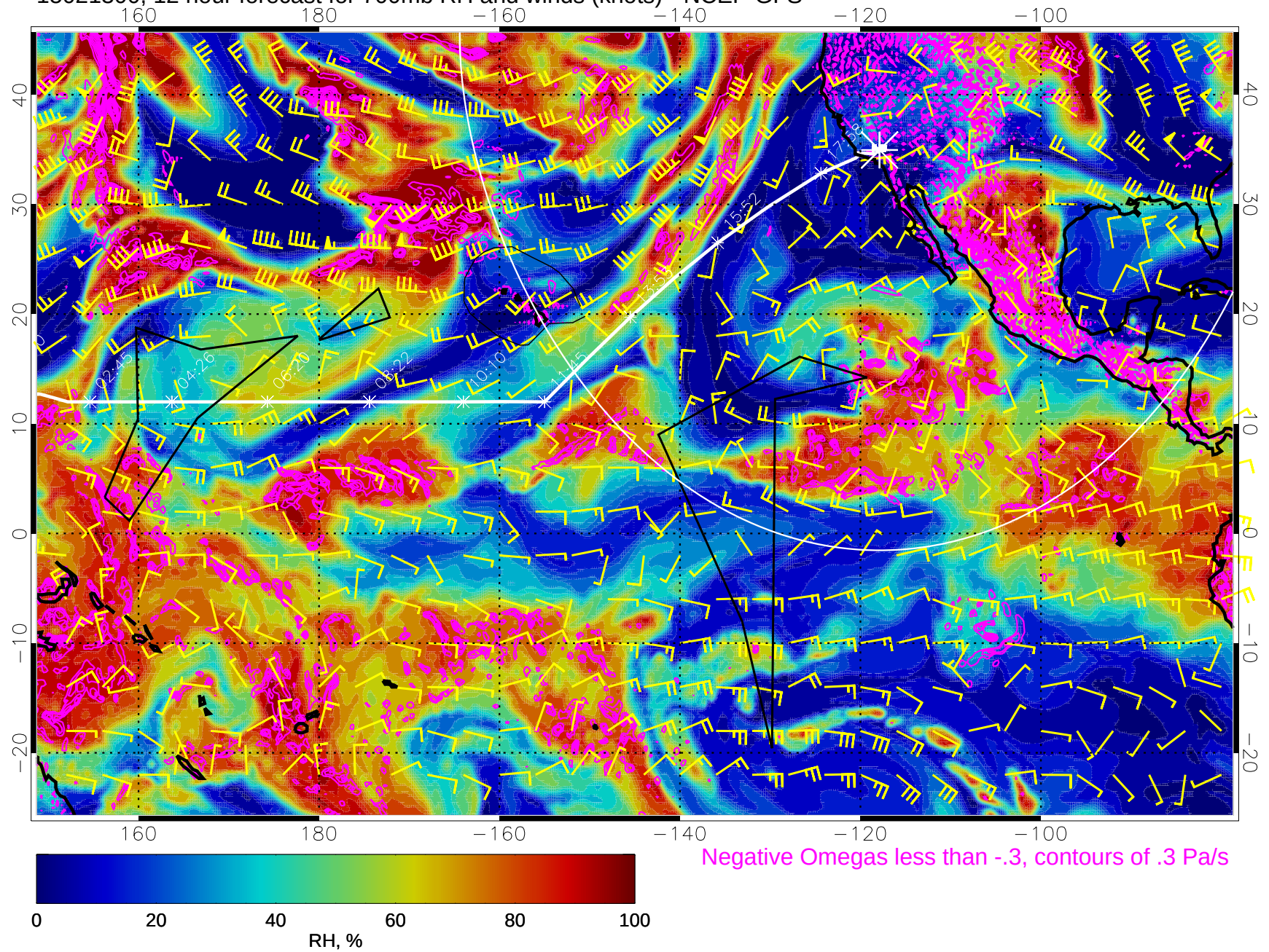
15021300, 12 hour forecast for 700mb RH and winds (knots) - NCEP GFS
