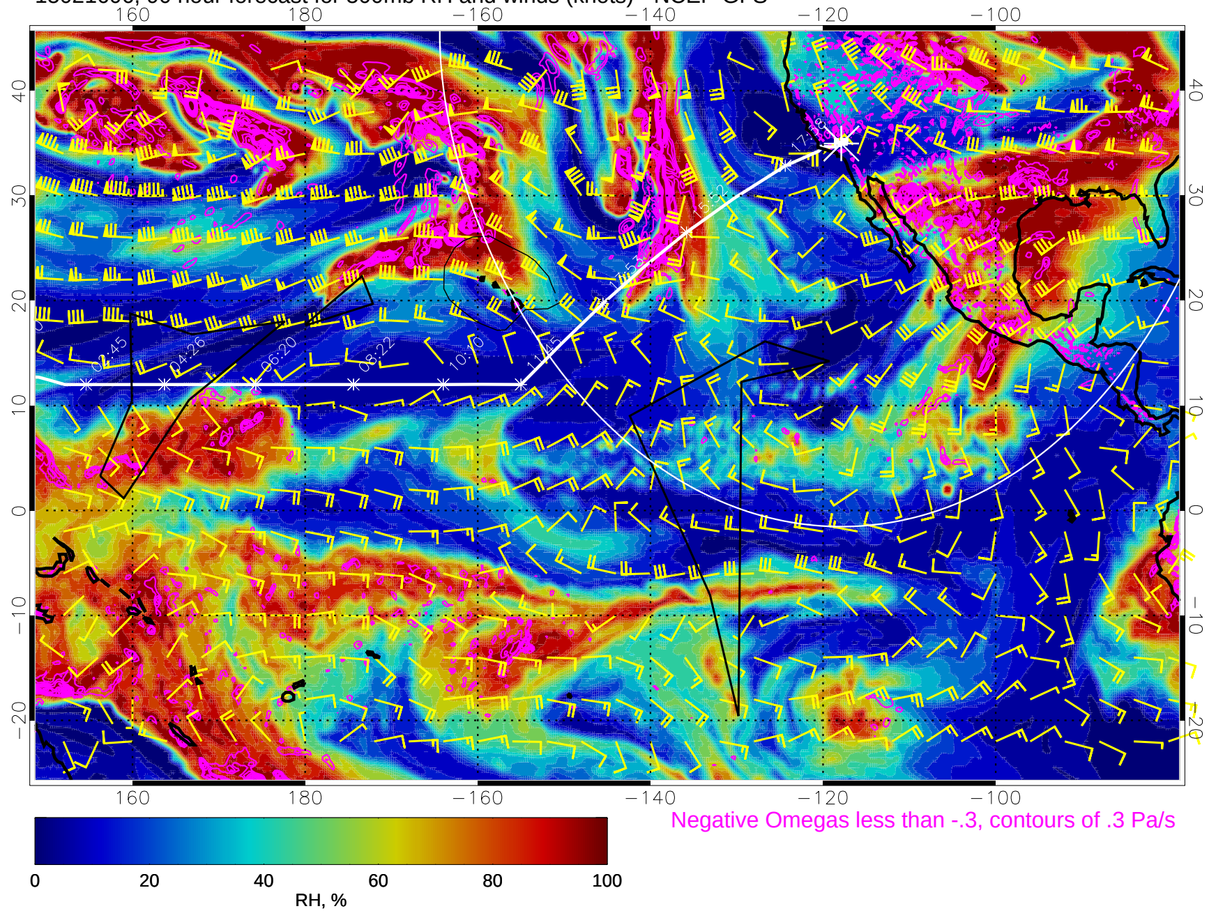
15021606, 90 hour forecast for 500mb RH and winds (knots) - NCEP GFS
