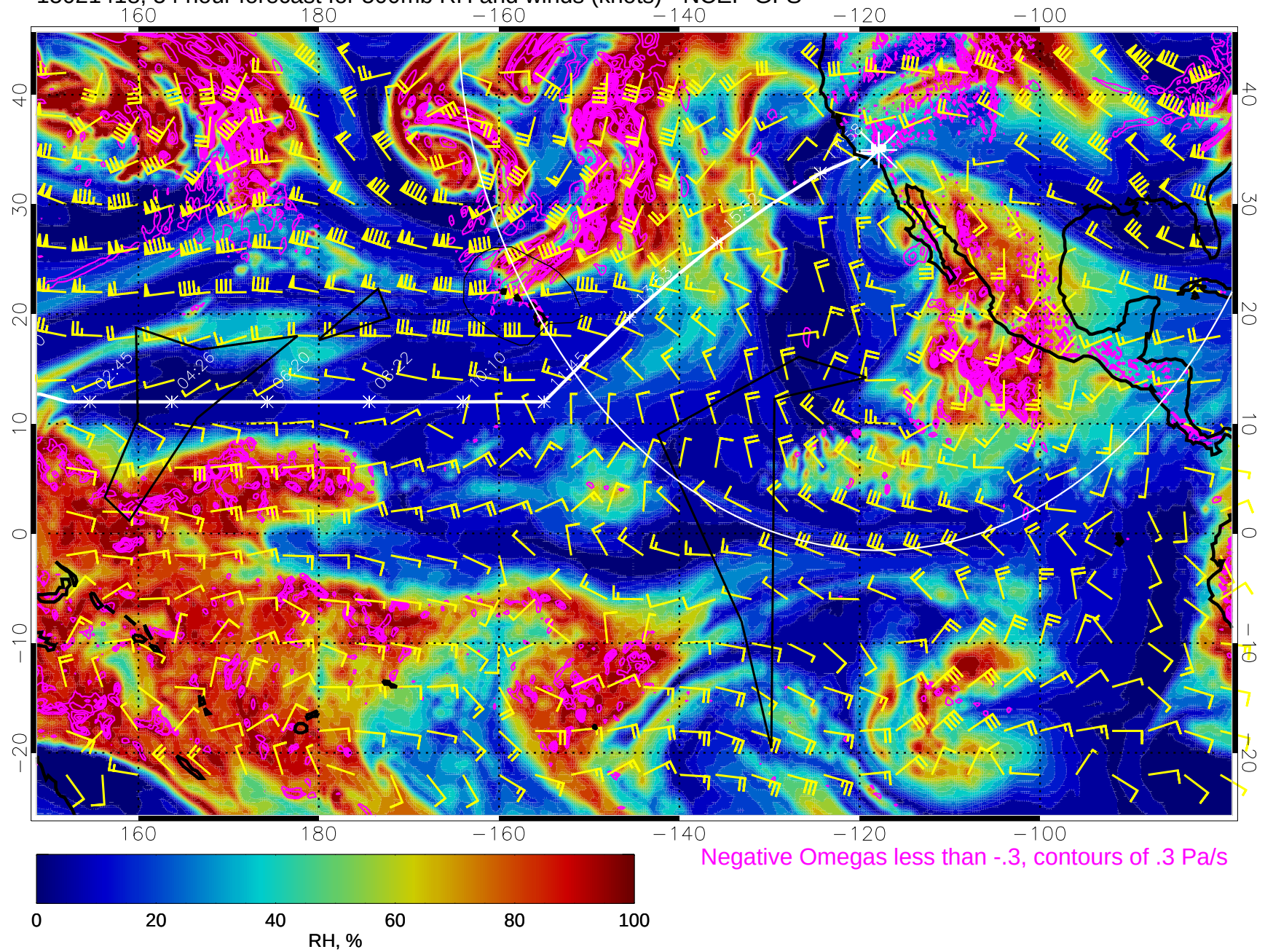
15021418, 54 hour forecast for 500mb RH and winds (knots) - NCEP GFS
