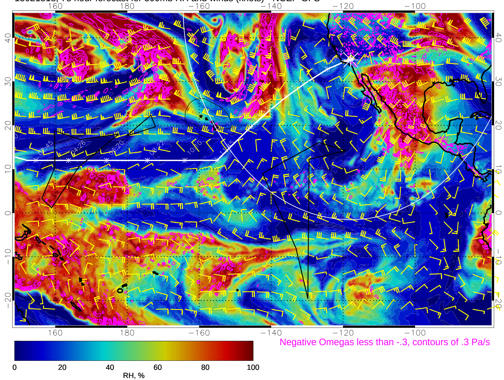
15021518, 78 hour forecast for 500mb RH and winds (knots) - NCEP GFS
