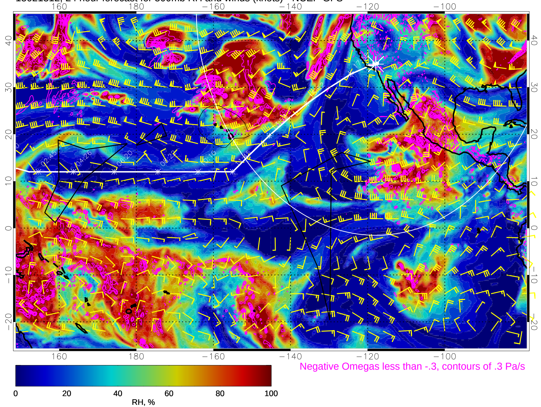
15021312, 24 hour forecast for 500mb RH and winds (knots) - NCEP GFS
