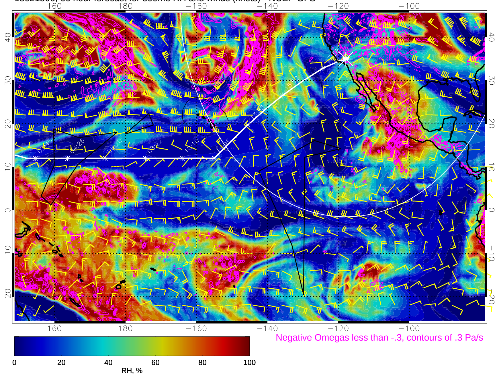
15021506, 66 hour forecast for 500mb RH and winds (knots) - NCEP GFS
