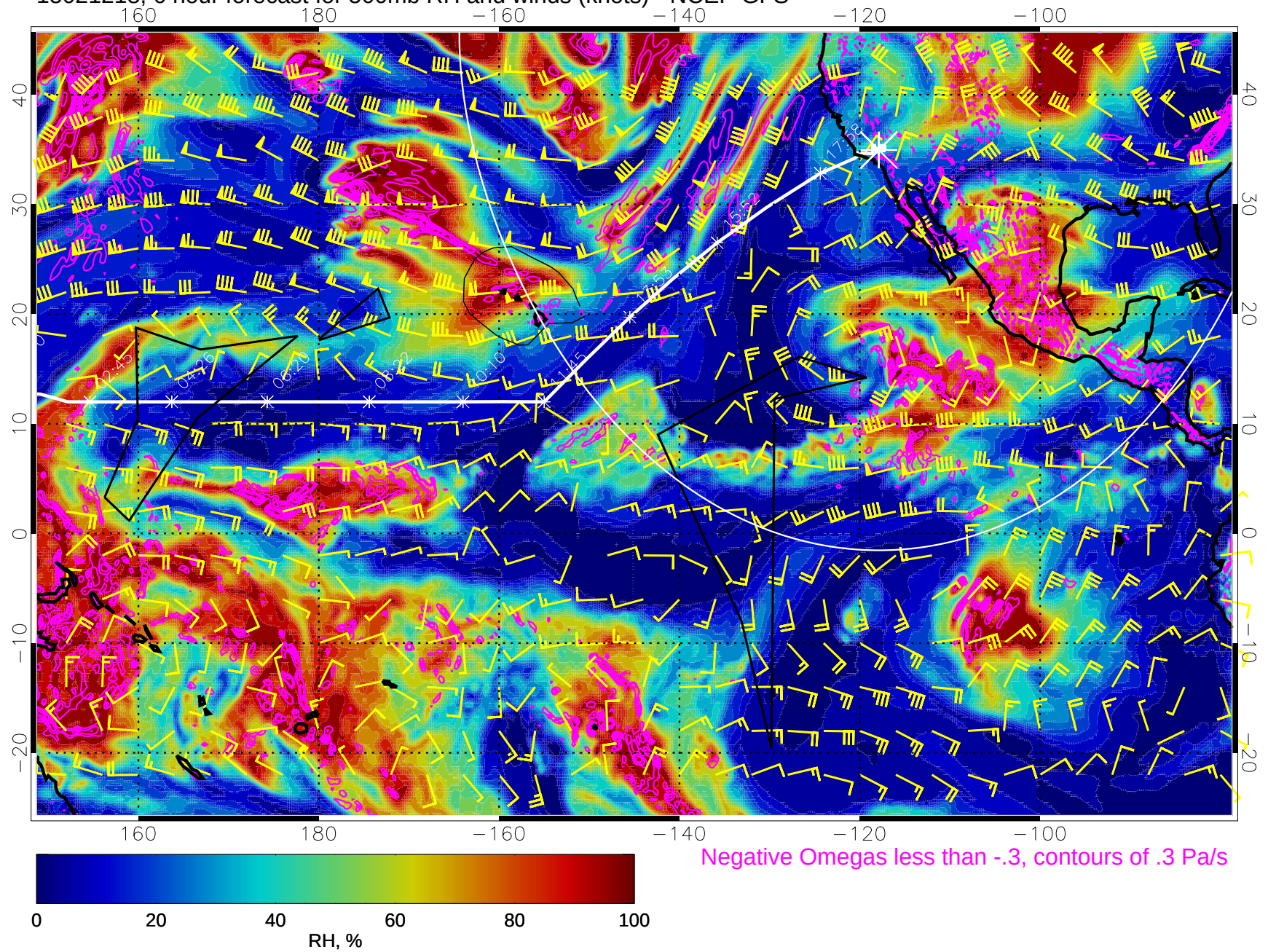
15021218, 6 hour forecast for 500mb RH and winds (knots) - NCEP GFS
