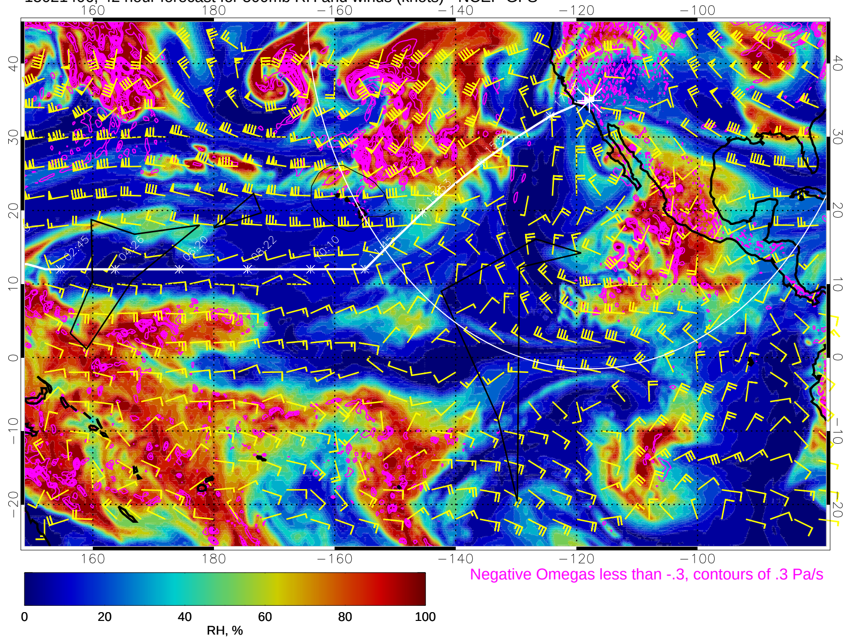
15021406, 42 hour forecast for 500mb RH and winds (knots) - NCEP GFS
