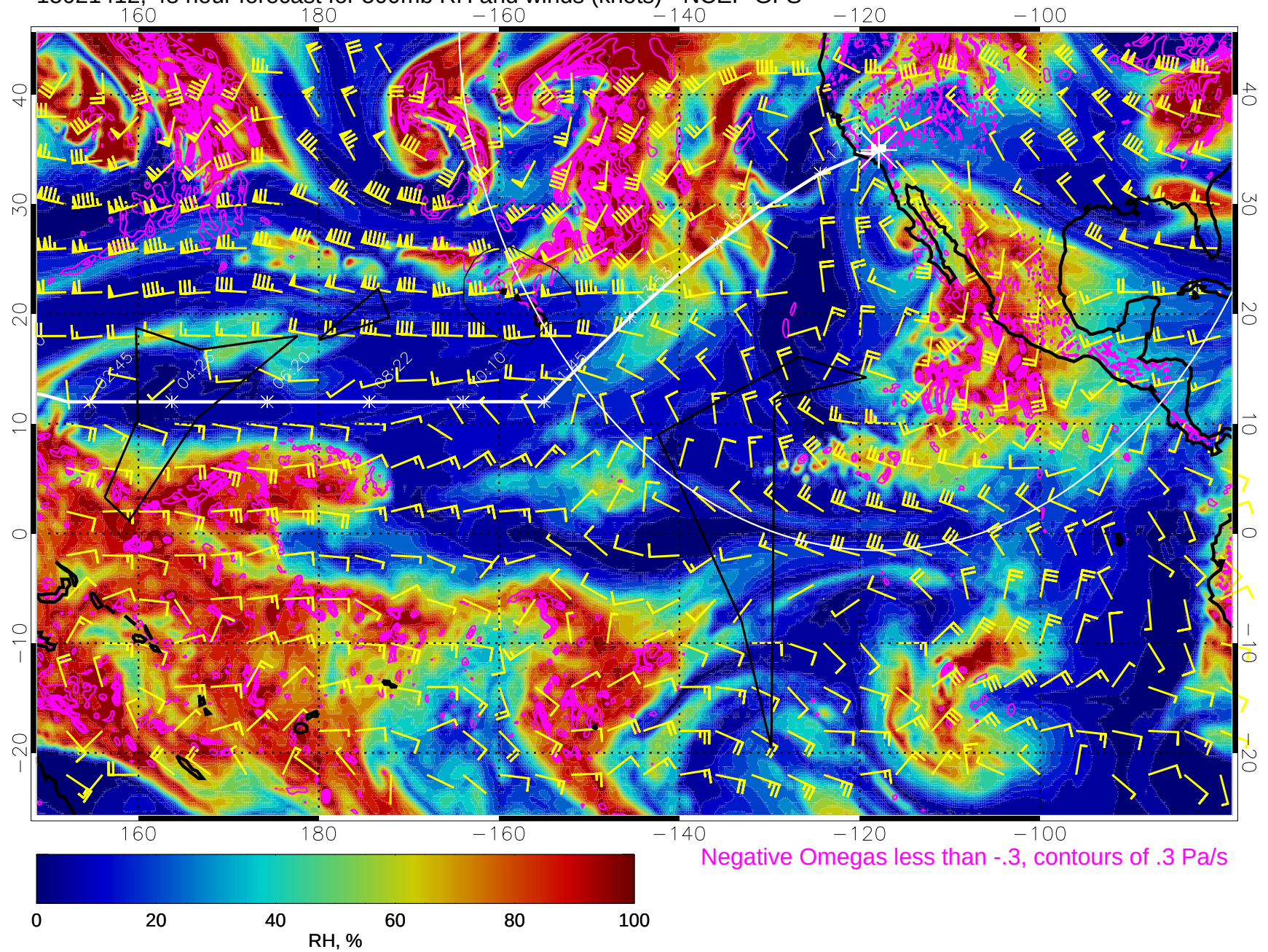
15021412, 48 hour forecast for 500mb RH and winds (knots) - NCEP GFS
