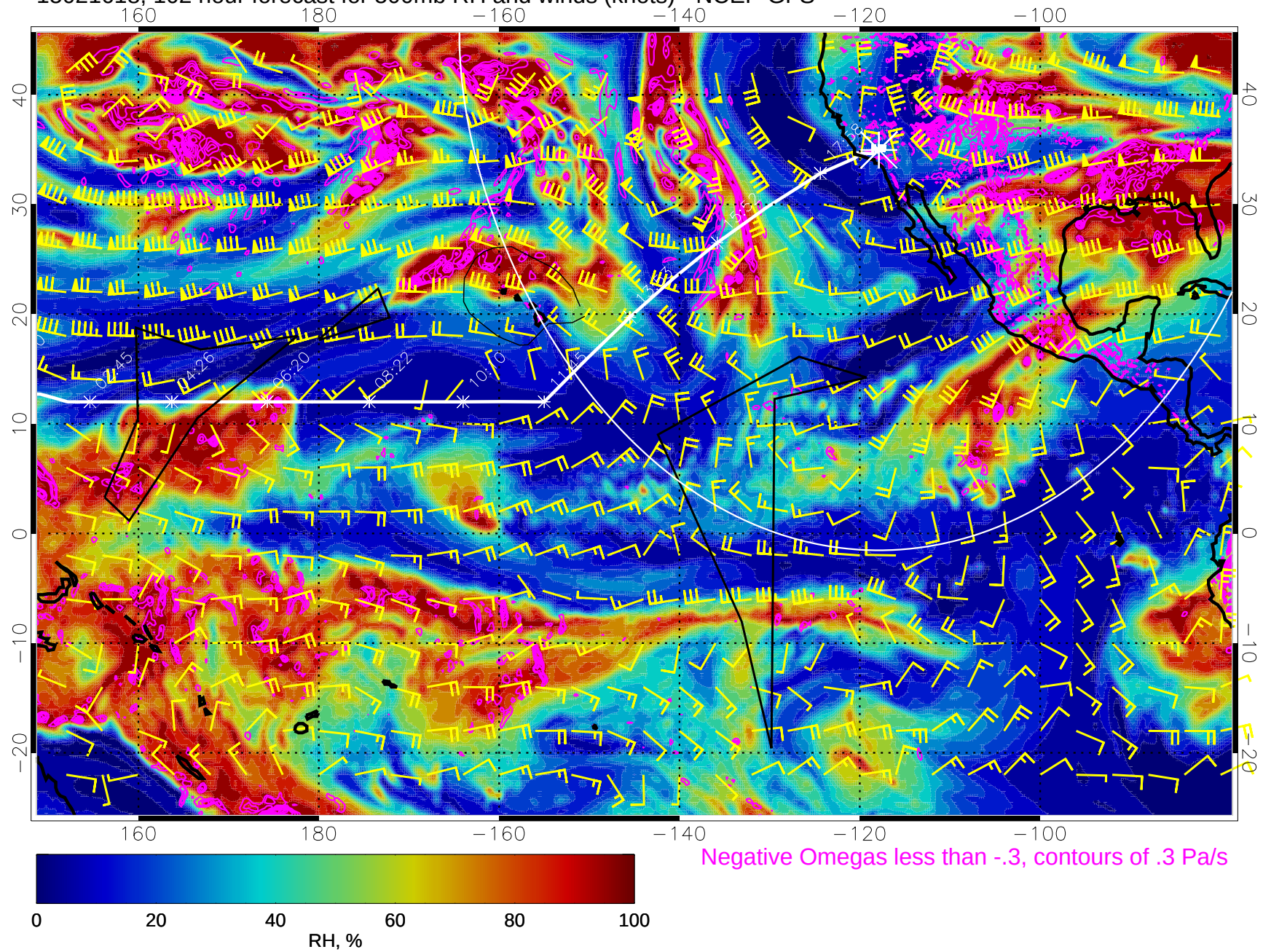
15021618, 102 hour forecast for 500mb RH and winds (knots) - NCEP GFS
