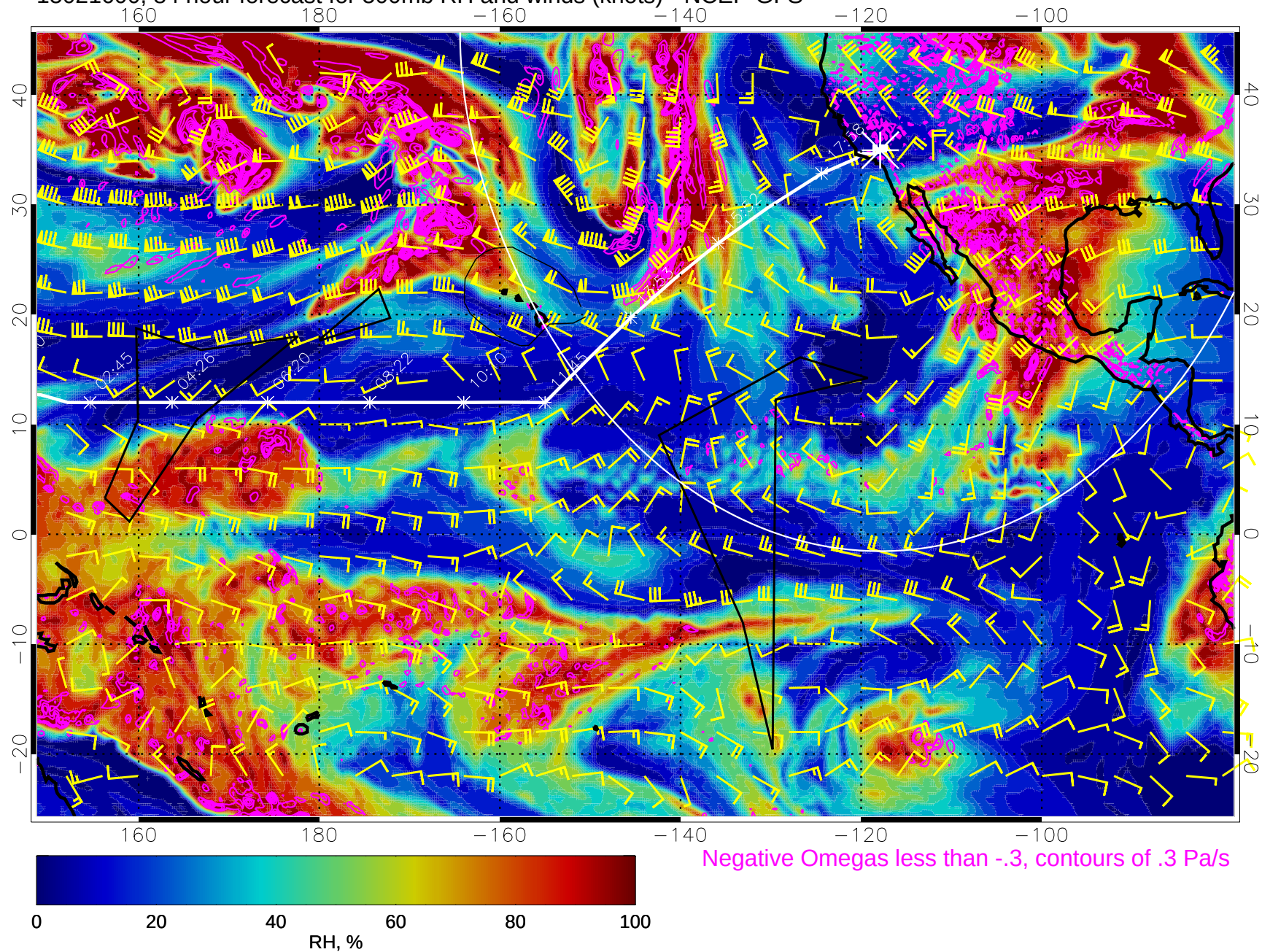
15021600, 84 hour forecast for 500mb RH and winds (knots) - NCEP GFS
