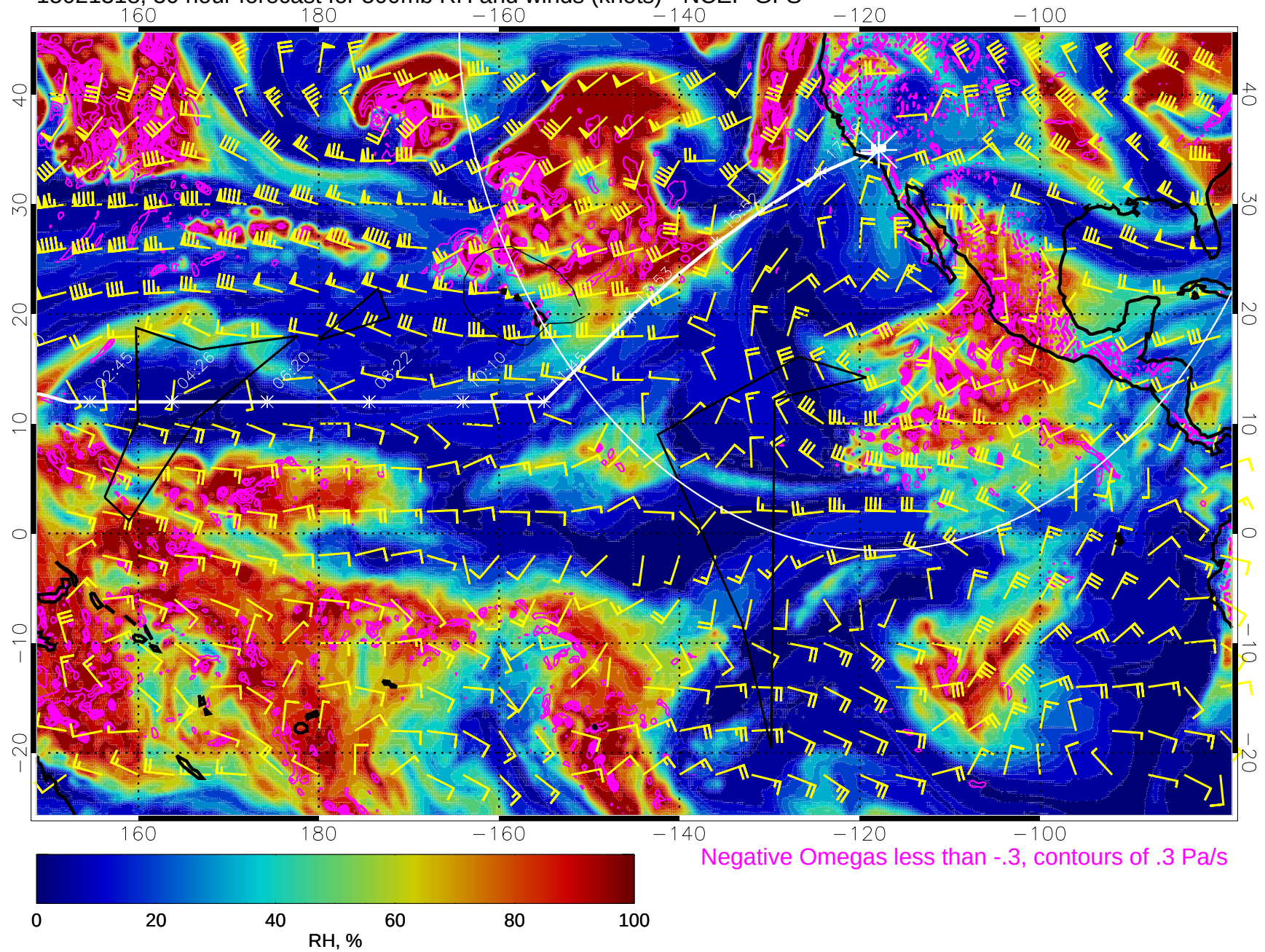
15021318, 30 hour forecast for 500mb RH and winds (knots) - NCEP GFS
