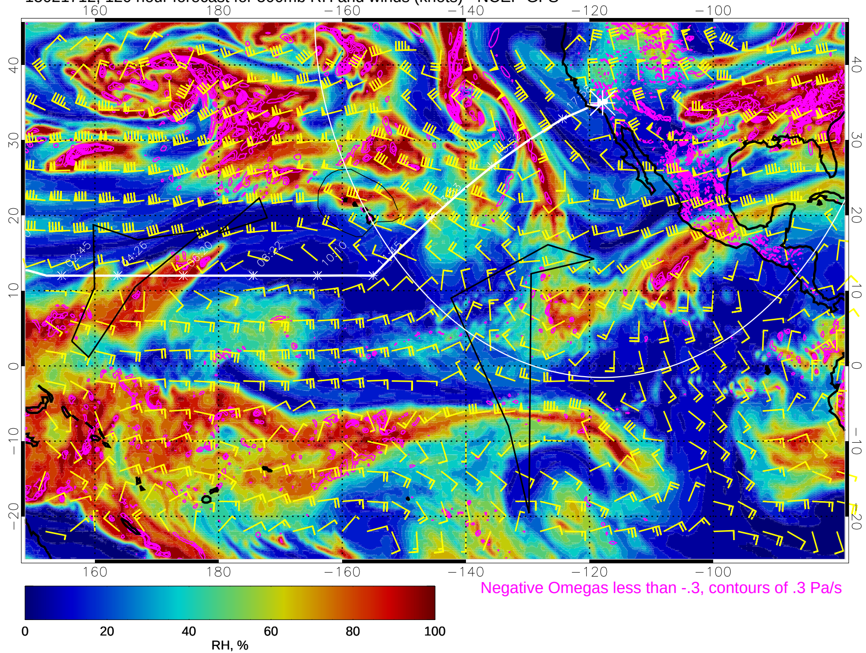
15021712, 120 hour forecast for 500mb RH and winds (knots) - NCEP GFS
