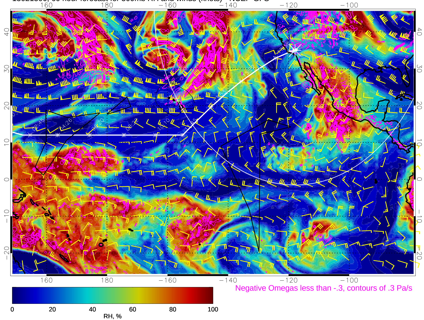
15021500, 60 hour forecast for 500mb RH and winds (knots) - NCEP GFS
