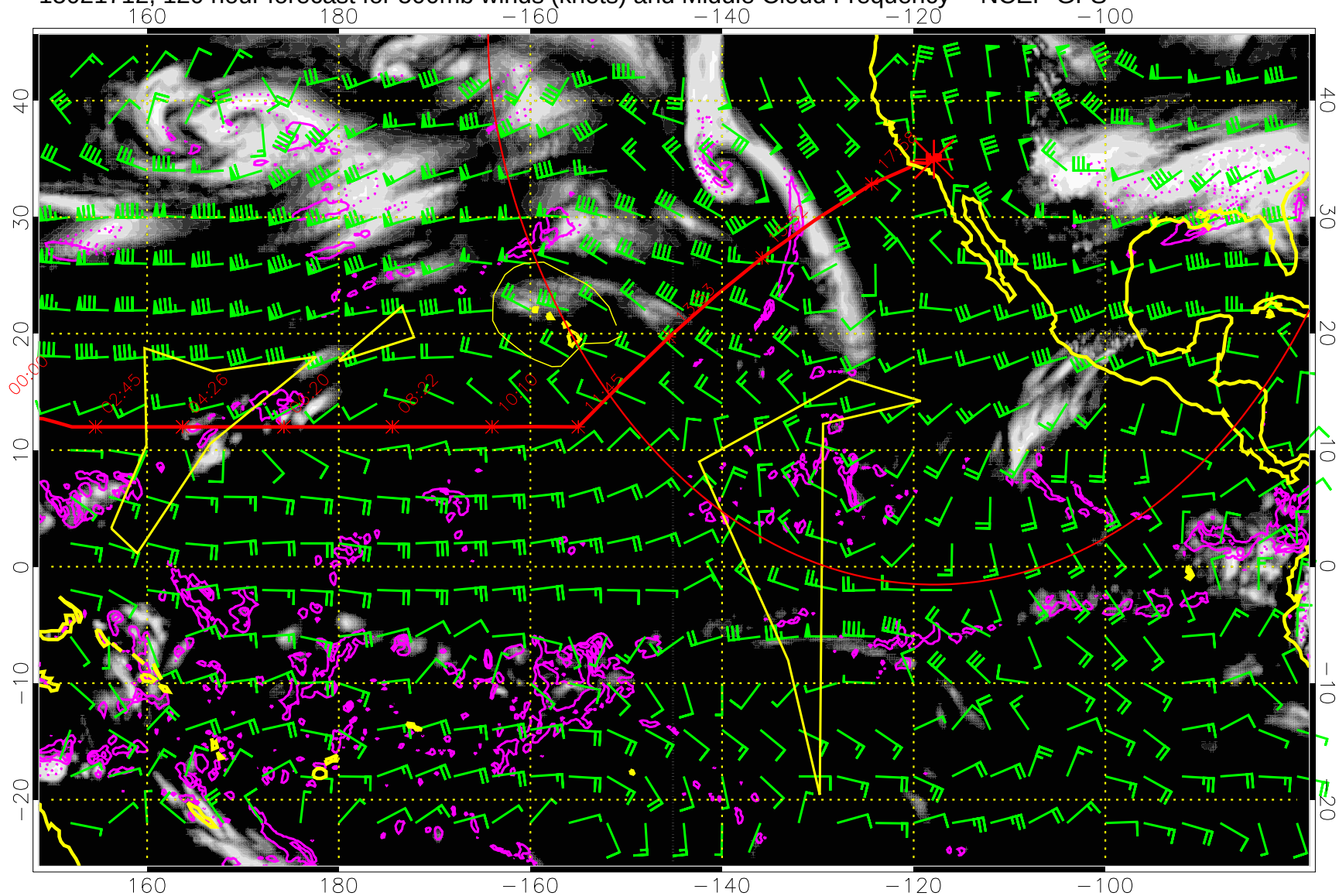
15021712, 120 hour forecast for 500mb winds (knots) and Middle Cloud Frequency -- NCEP GFS
