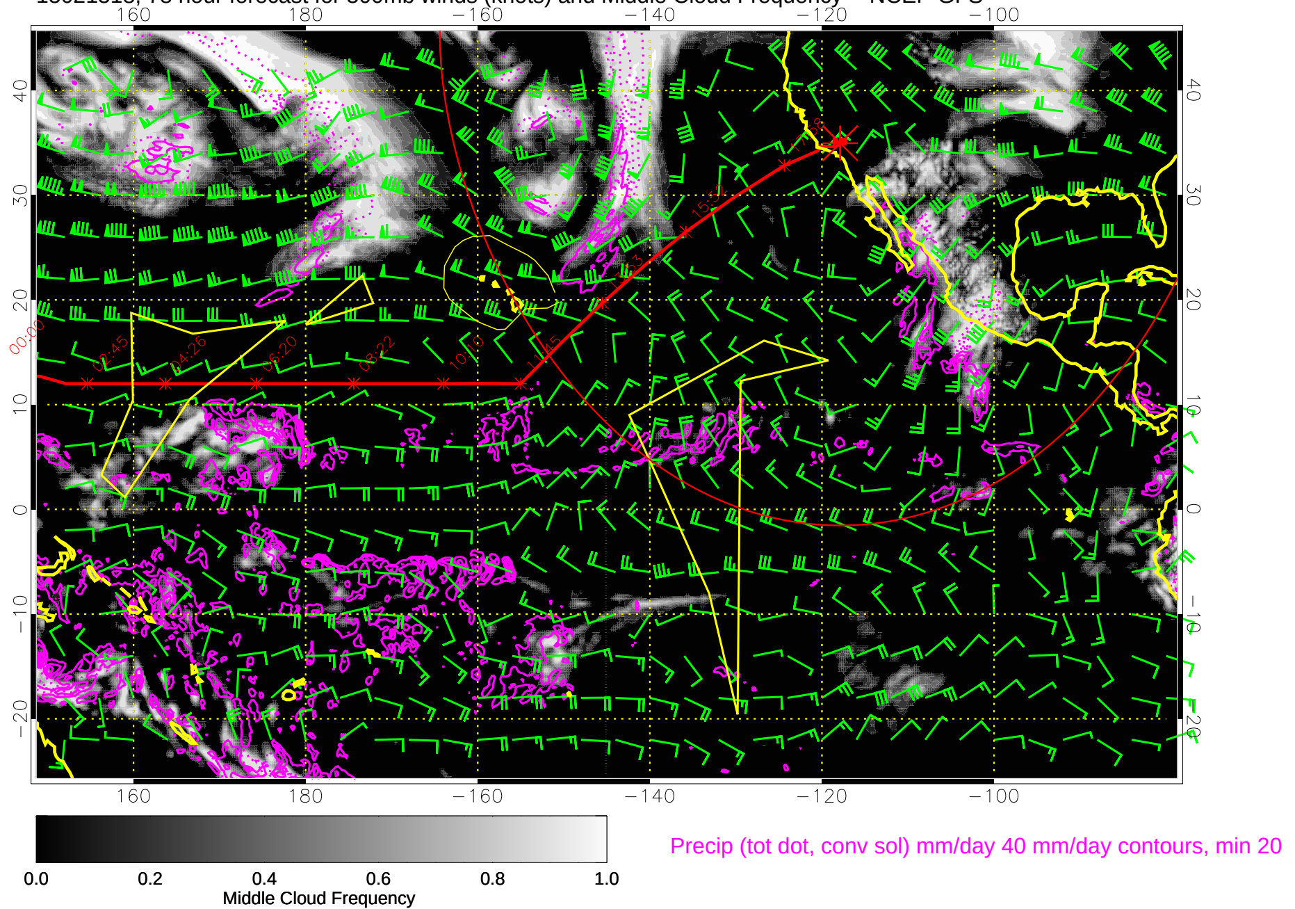
15021518, 78 hour forecast for 500mb winds (knots) and Middle Cloud Frequency -- NCEP GFS
