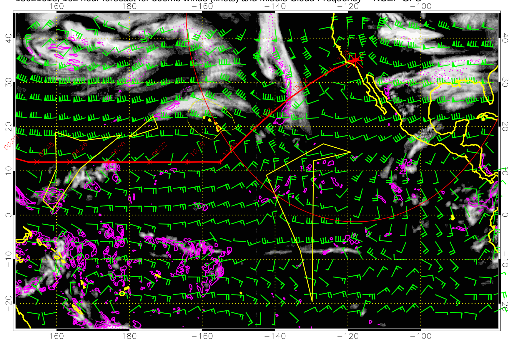
15021618, 102 hour forecast for 500mb winds (knots) and Middle Cloud Frequency -- NCEP GFS
