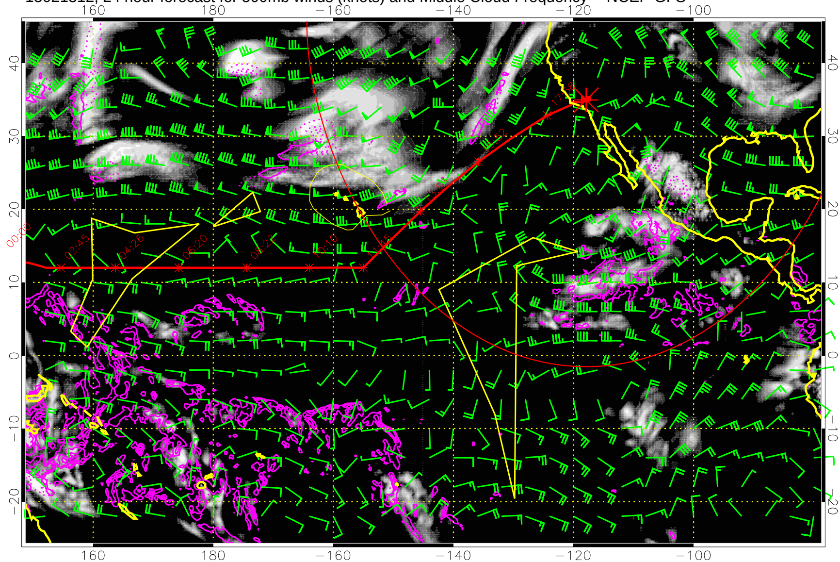
15021312, 24 hour forecast for 500mb winds (knots) and Middle Cloud Frequency -- NCEP GFS
