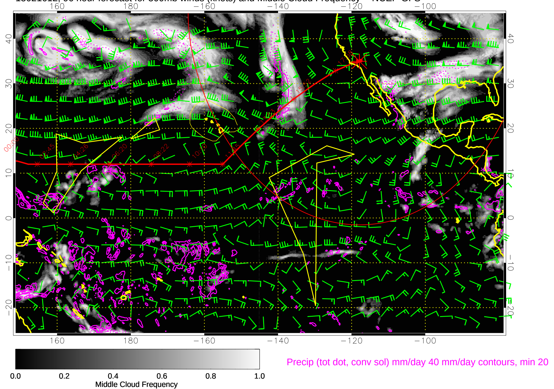
15021612, 96 hour forecast for 500mb winds (knots) and Middle Cloud Frequency -- NCEP GFS
