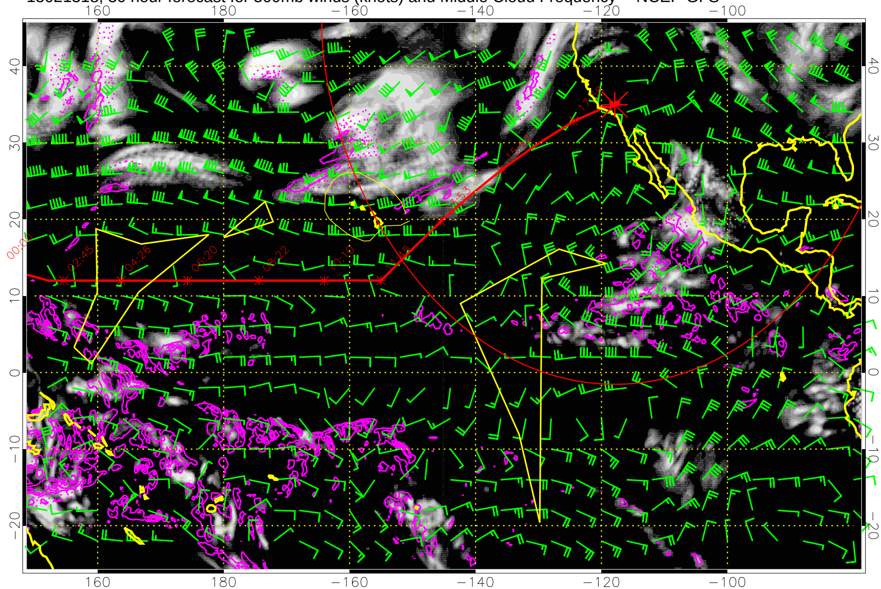
15021318, 30 hour forecast for 500mb winds (knots) and Middle Cloud Frequency -- NCEP GFS
