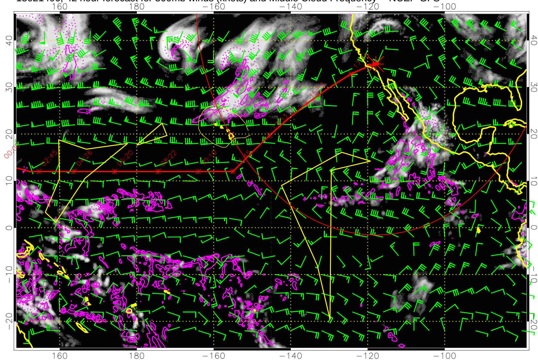
15021406, 42 hour forecast for 500mb winds (knots) and Middle Cloud Frequency -- NCEP GFS
