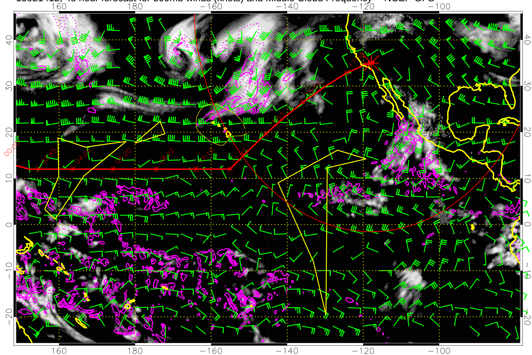
15021412, 48 hour forecast for 500mb winds (knots) and Middle Cloud Frequency -- NCEP GFS
