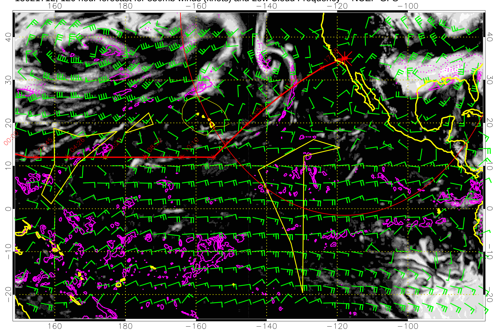
15021712, 120 hour forecast for 850mb winds (knots) and Low Cloud Frequency -- NCEP GFS
