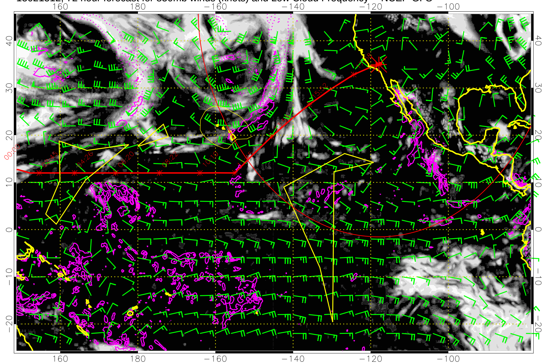
15021512, 72 hour forecast for 850mb winds (knots) and Low Cloud Frequency -- NCEP GFS
