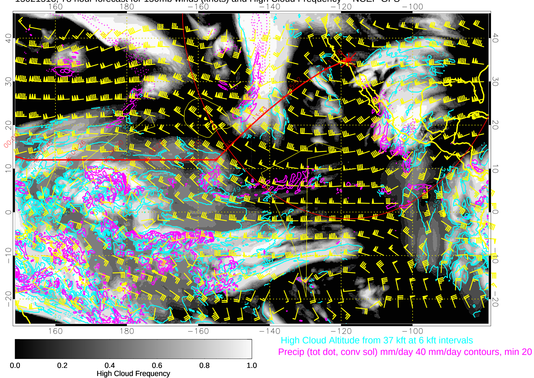
15021518, 78 hour forecast for 150mb winds (knots) and High Cloud Frequency -- NCEP GFS
