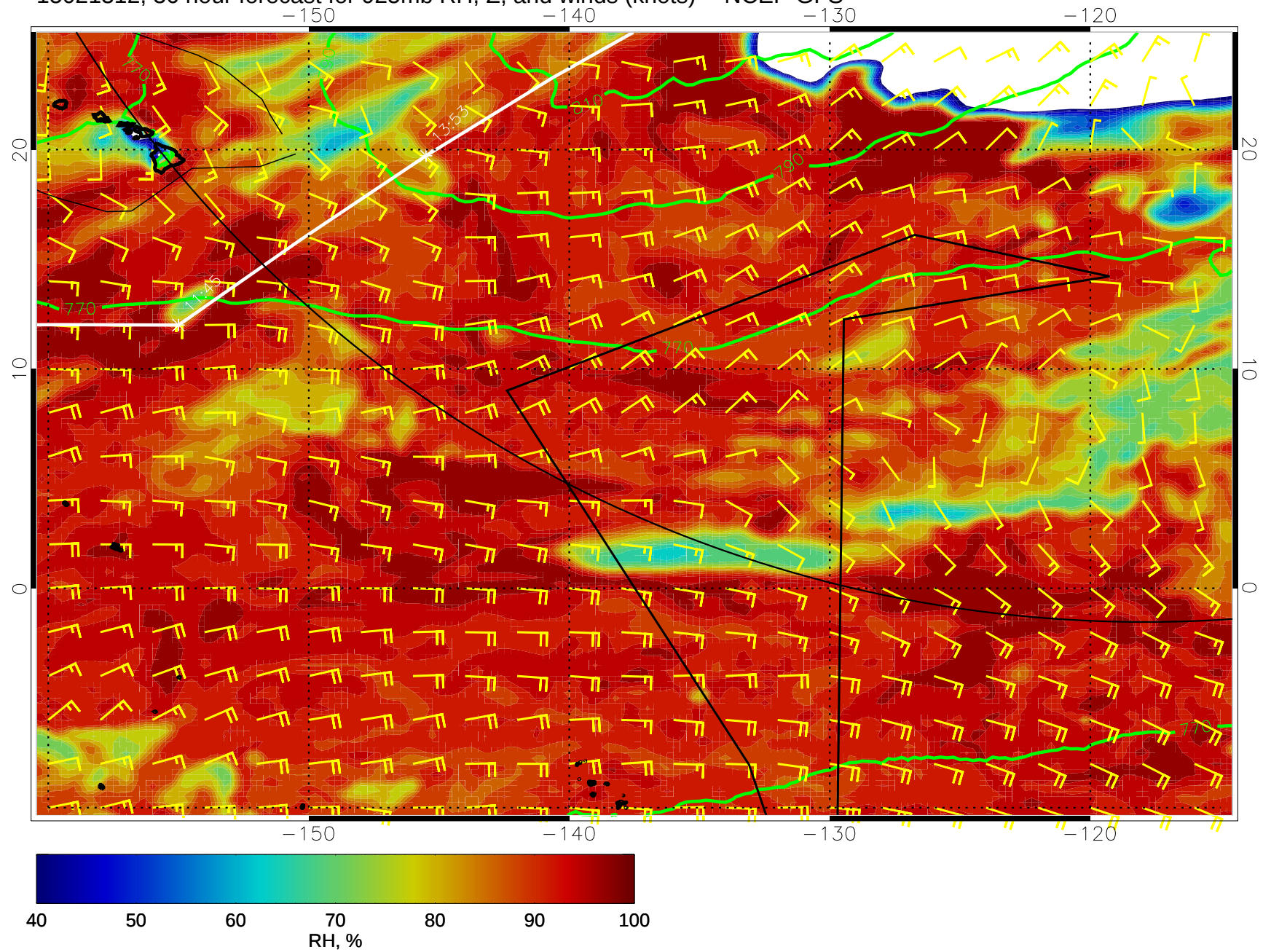
15021312, 36 hour forecast for 925mb RH, Z, and winds (knots) -- NCEP GFS
