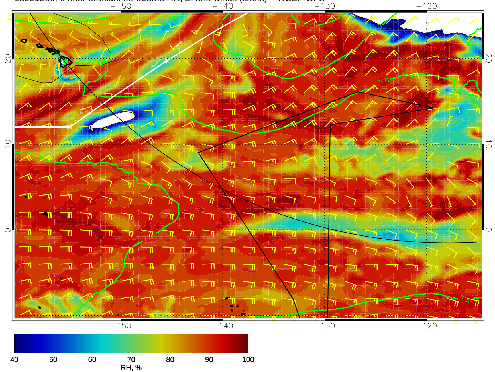
15021206, 6 hour forecast for 925mb RH, Z, and winds (knots) -- NCEP GFS
