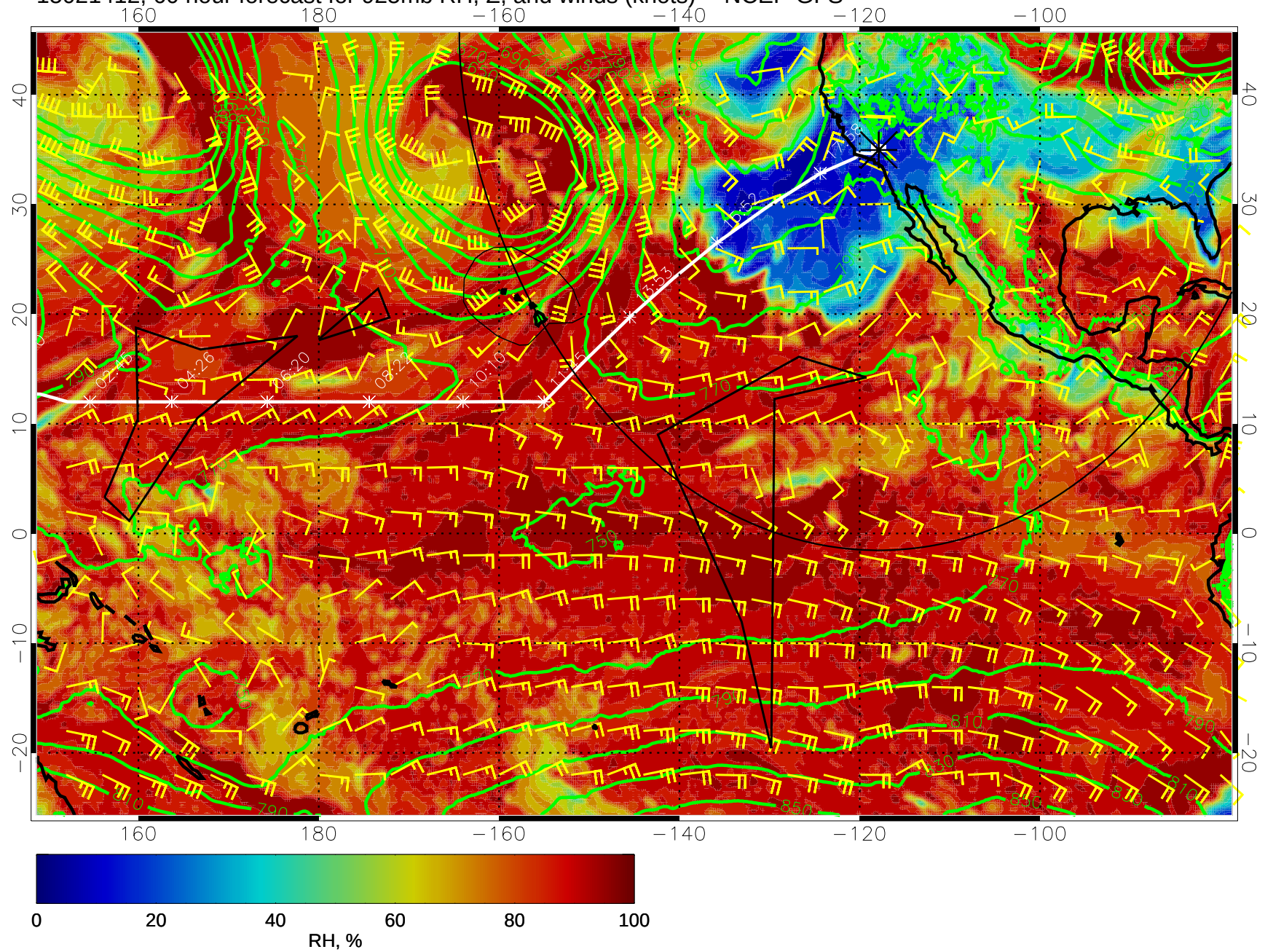
15021412, 60 hour forecast for 925mb RH, Z, and winds (knots) -- NCEP GFS
