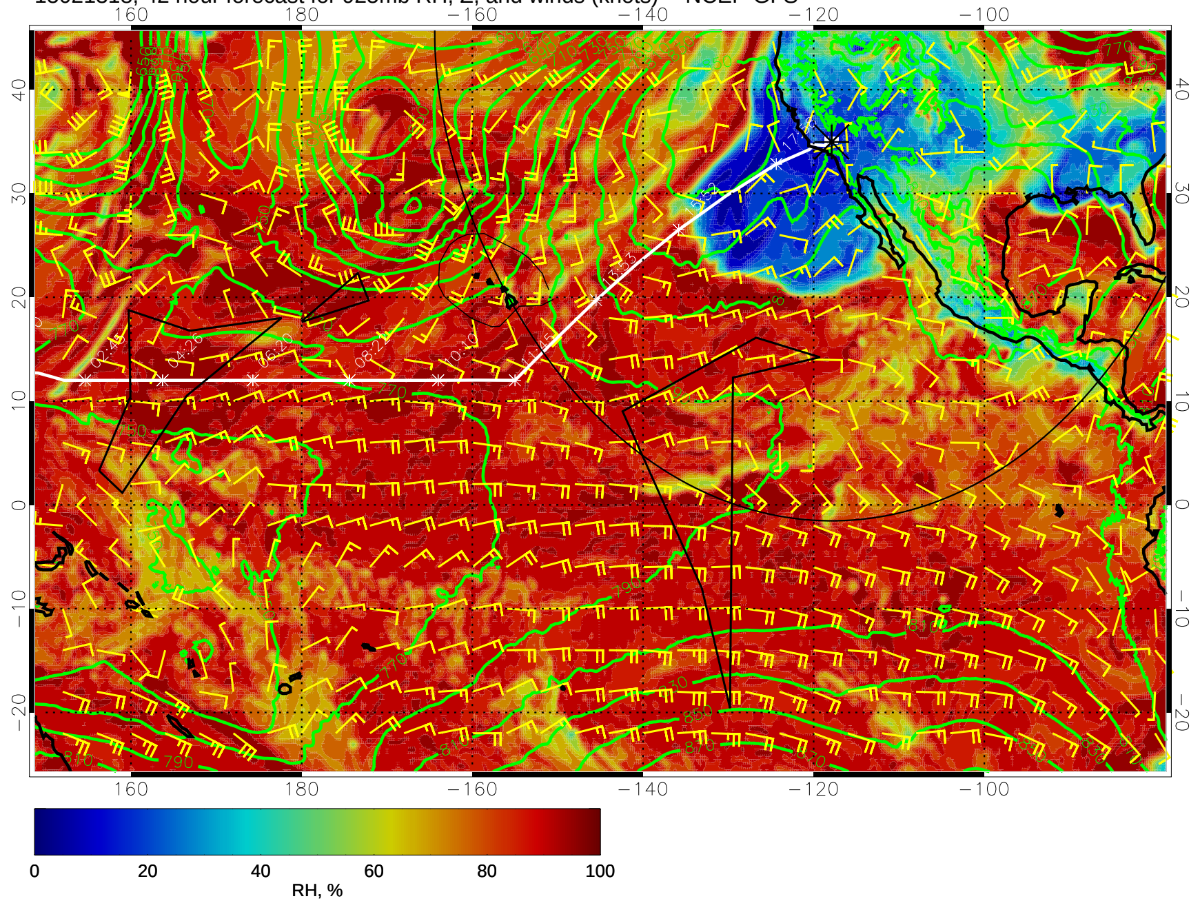
15021318, 42 hour forecast for 925mb RH, Z, and winds (knots) -- NCEP GFS
