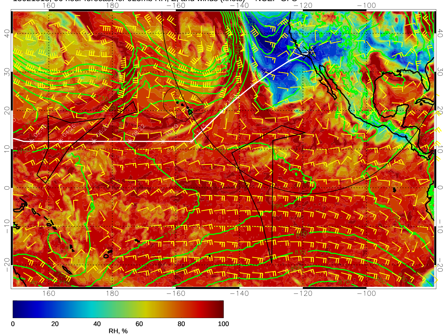
15021518, 90 hour forecast for 925mb RH, Z, and winds (knots) -- NCEP GFS
