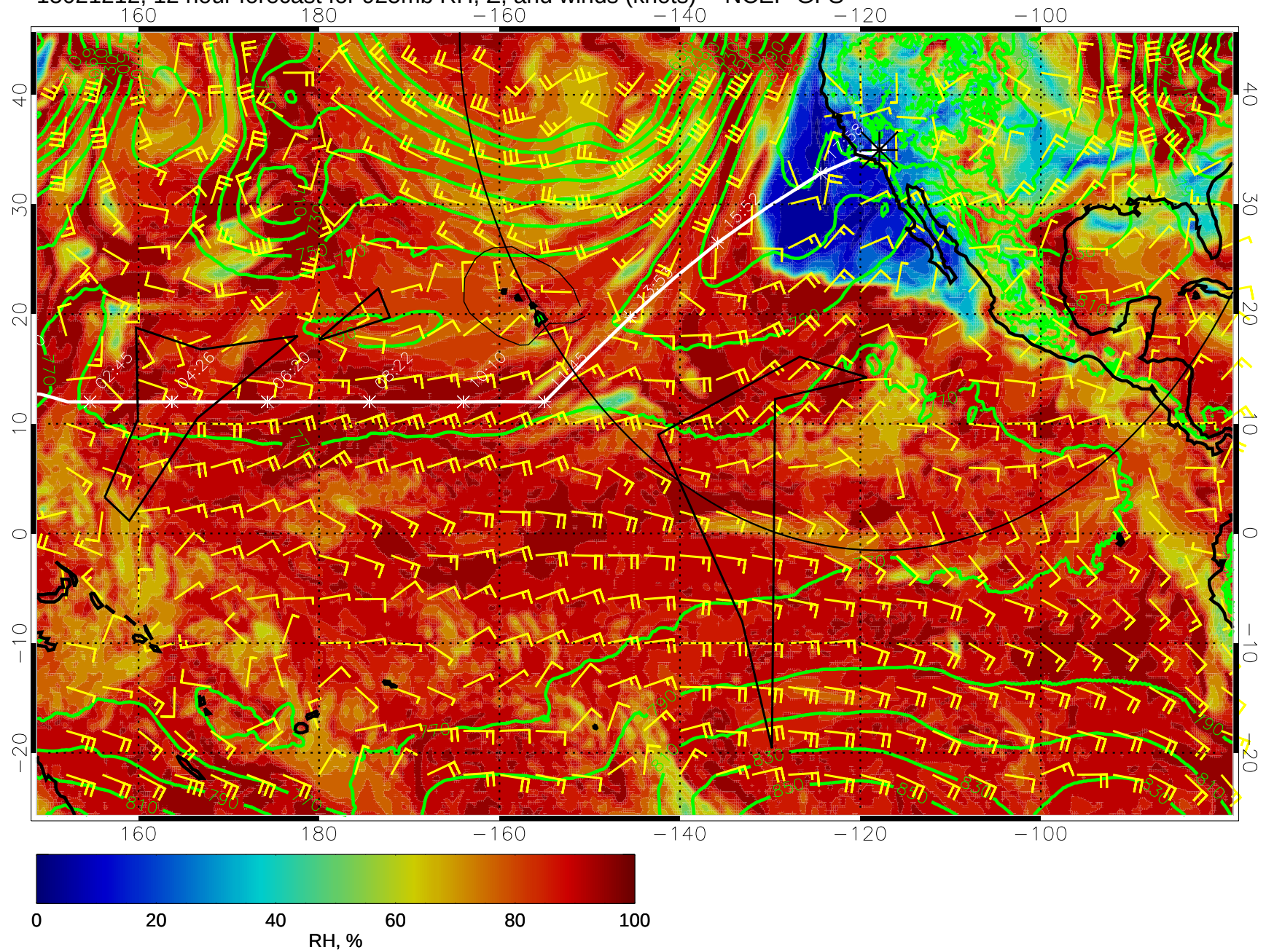
15021212, 12 hour forecast for 925mb RH, Z, and winds (knots) -- NCEP GFS
