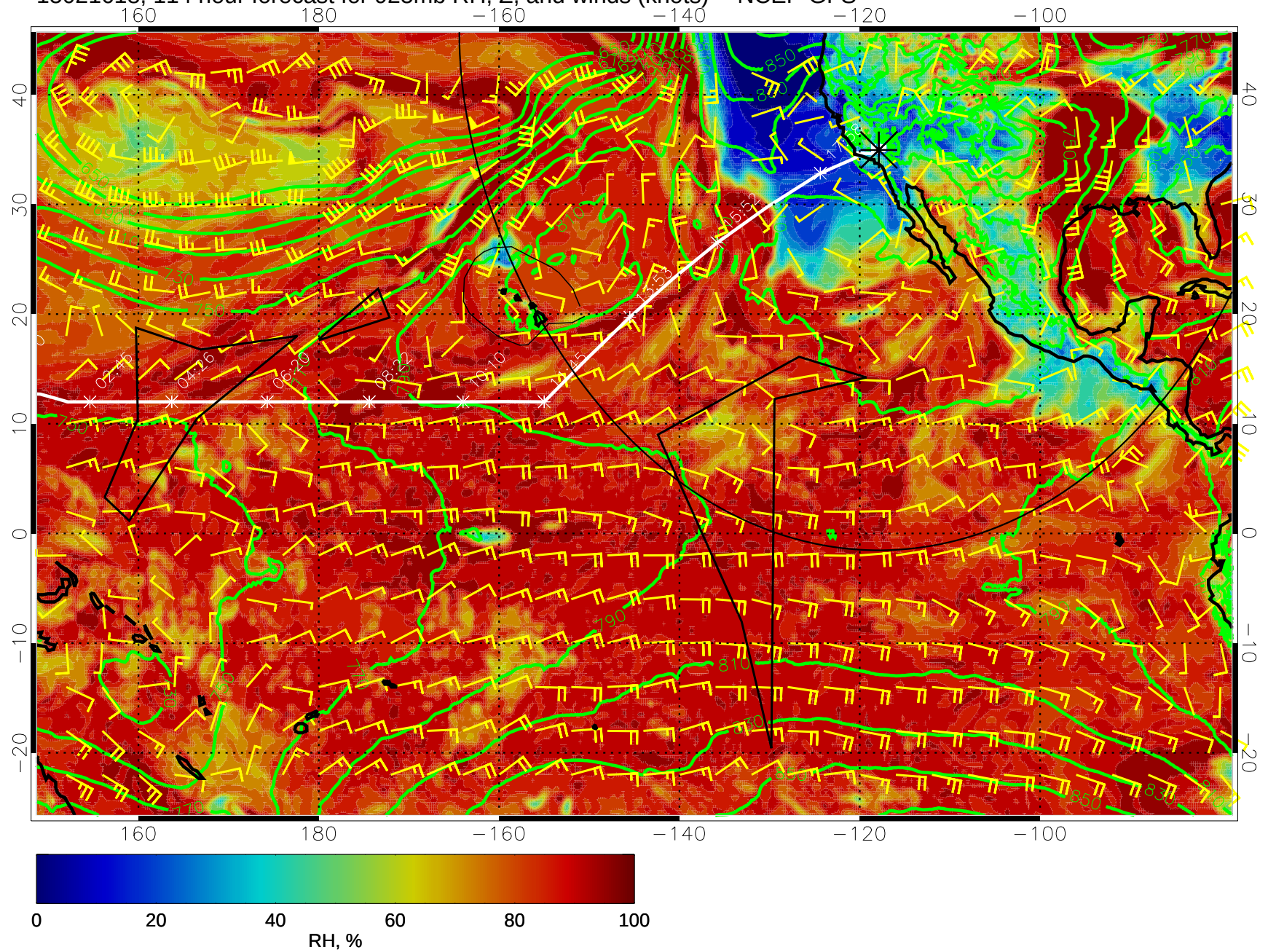
15021618, 114 hour forecast for 925mb RH, Z, and winds (knots) -- NCEP GFS
