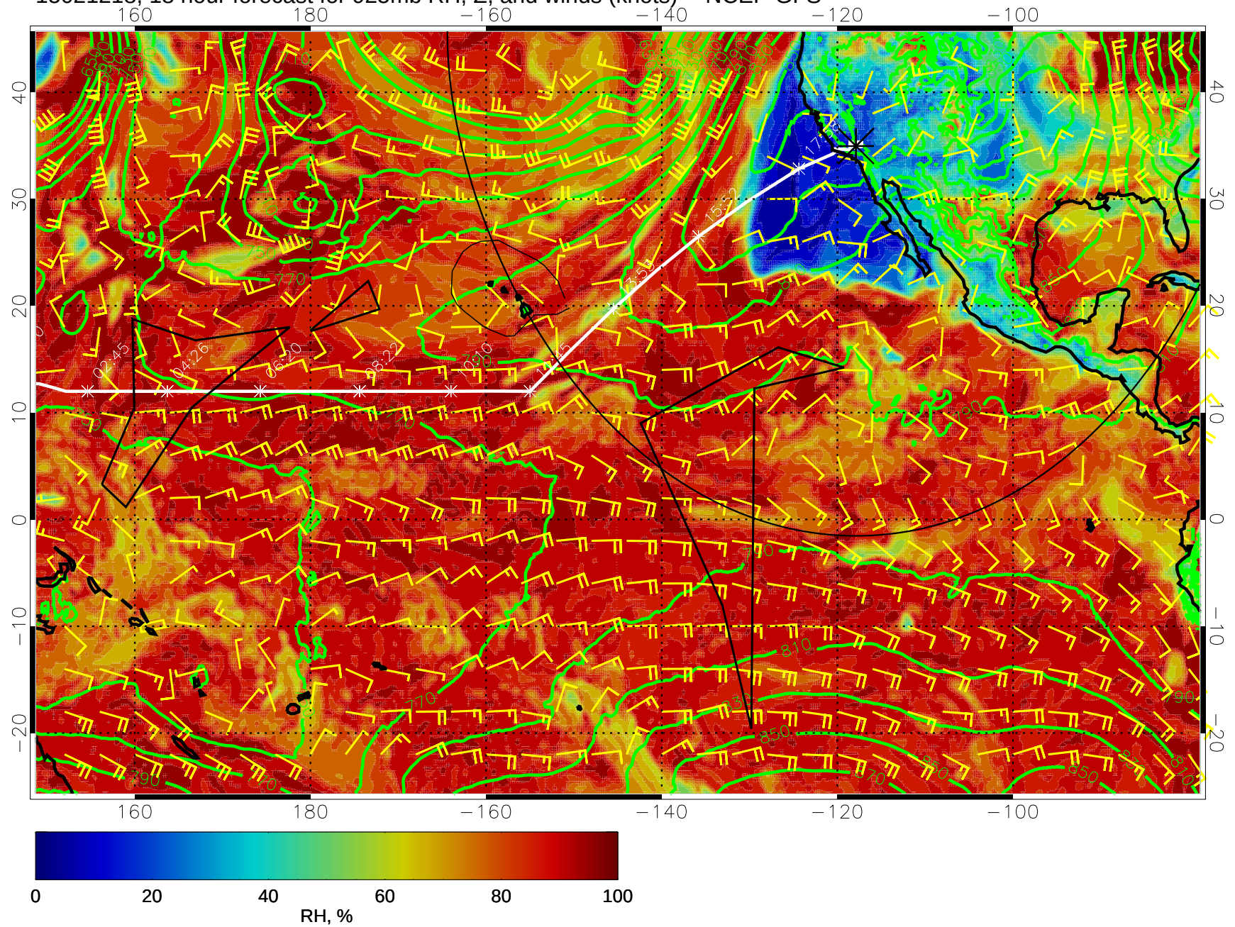
15021218, 18 hour forecast for 925mb RH, Z, and winds (knots) -- NCEP GFS
