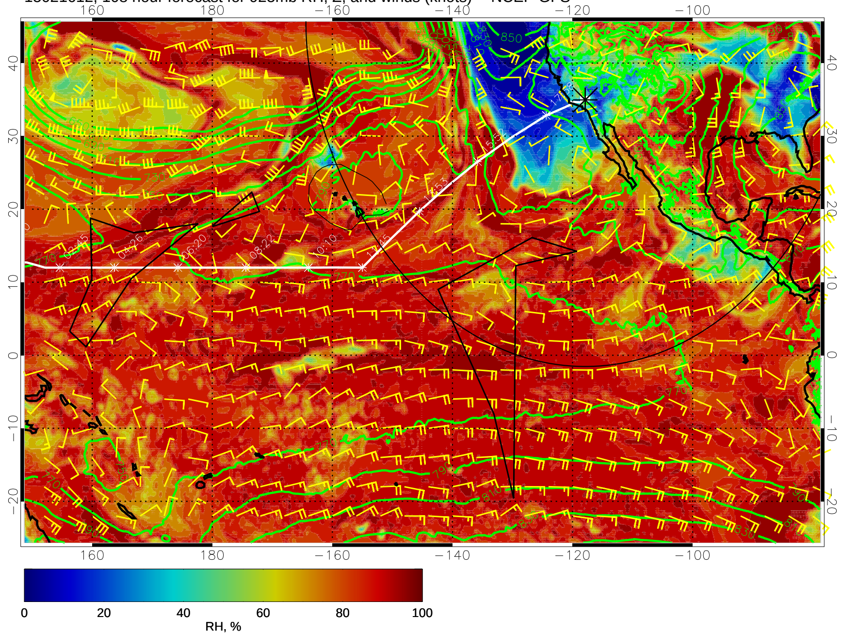
15021612, 108 hour forecast for 925mb RH, Z, and winds (knots) -- NCEP GFS
