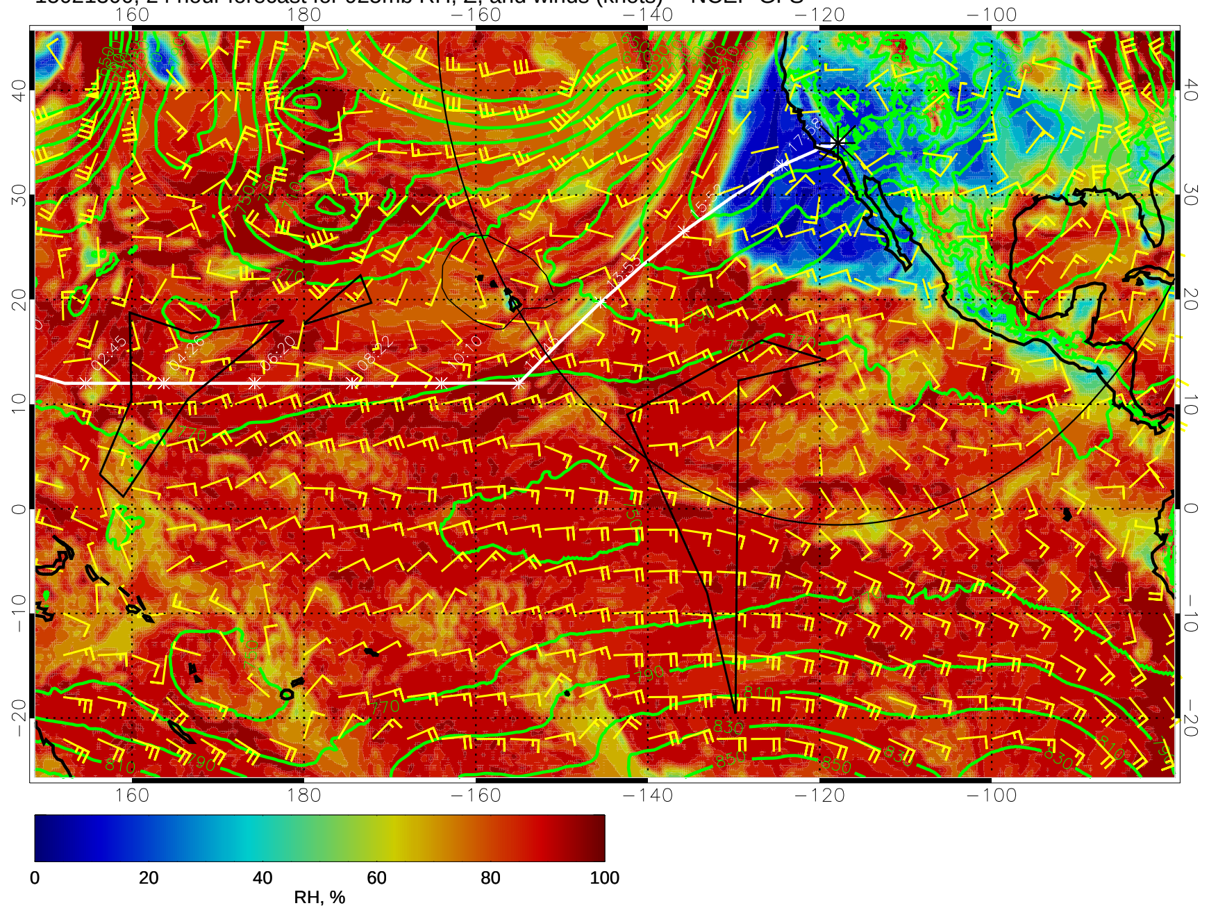
15021300, 24 hour forecast for 925mb RH, Z, and winds (knots) -- NCEP GFS
