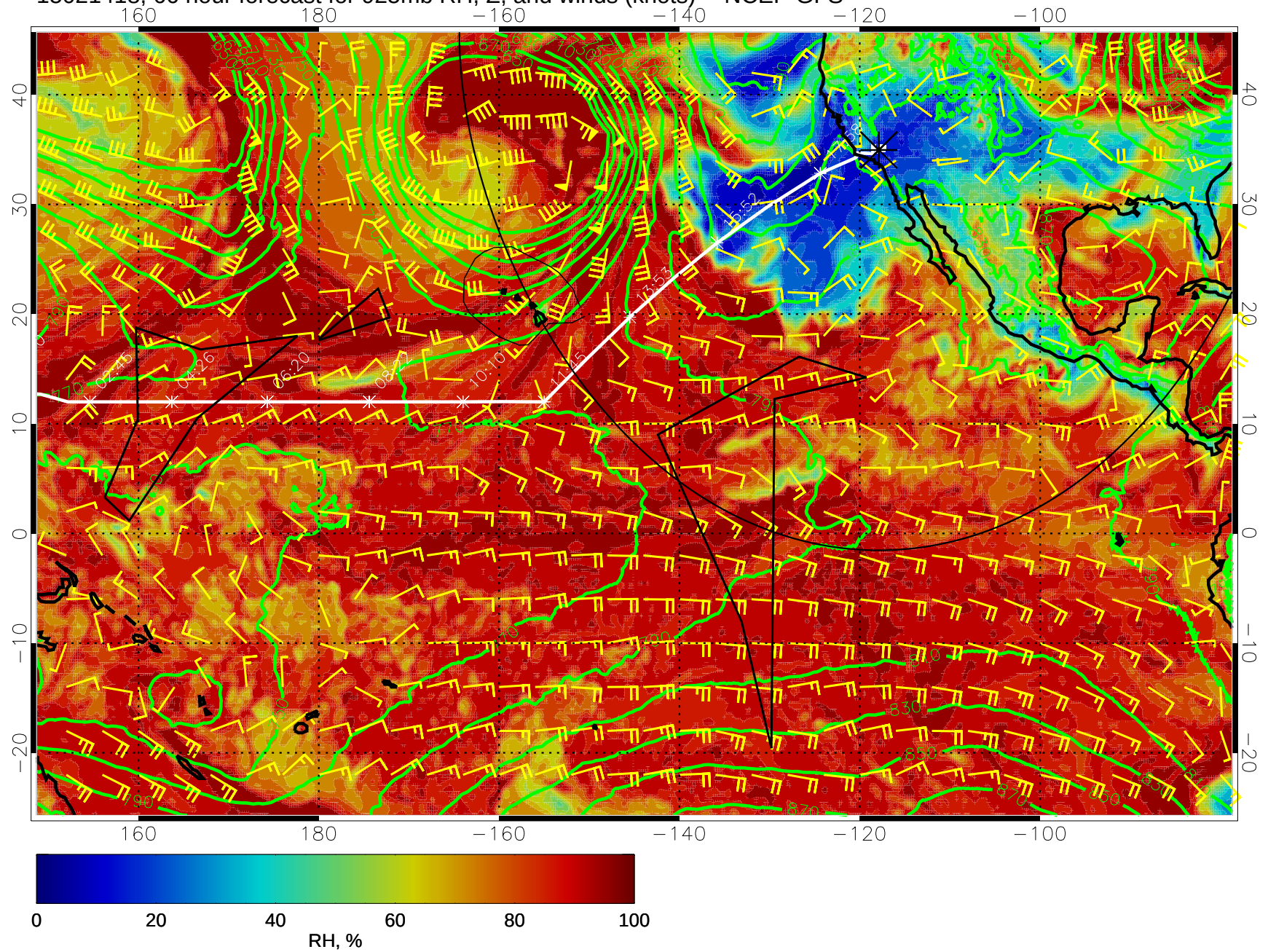
15021418, 66 hour forecast for 925mb RH, Z, and winds (knots) -- NCEP GFS
