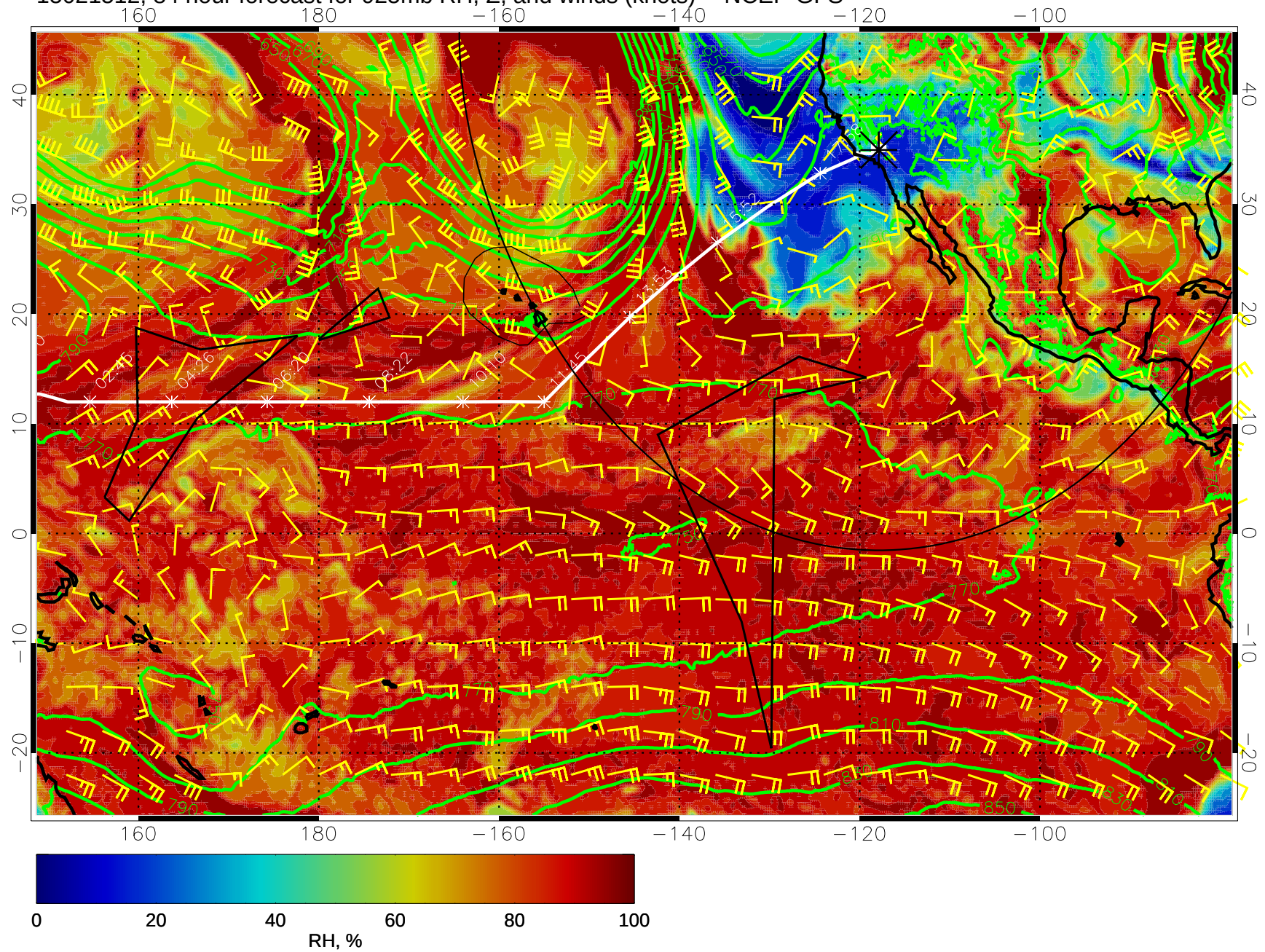
15021512, 84 hour forecast for 925mb RH, Z, and winds (knots) -- NCEP GFS
