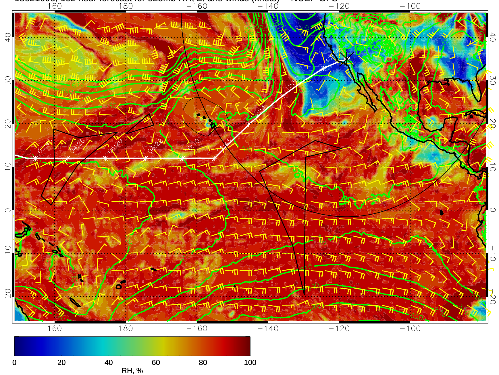
15021606, 102 hour forecast for 925mb RH, Z, and winds (knots) -- NCEP GFS
