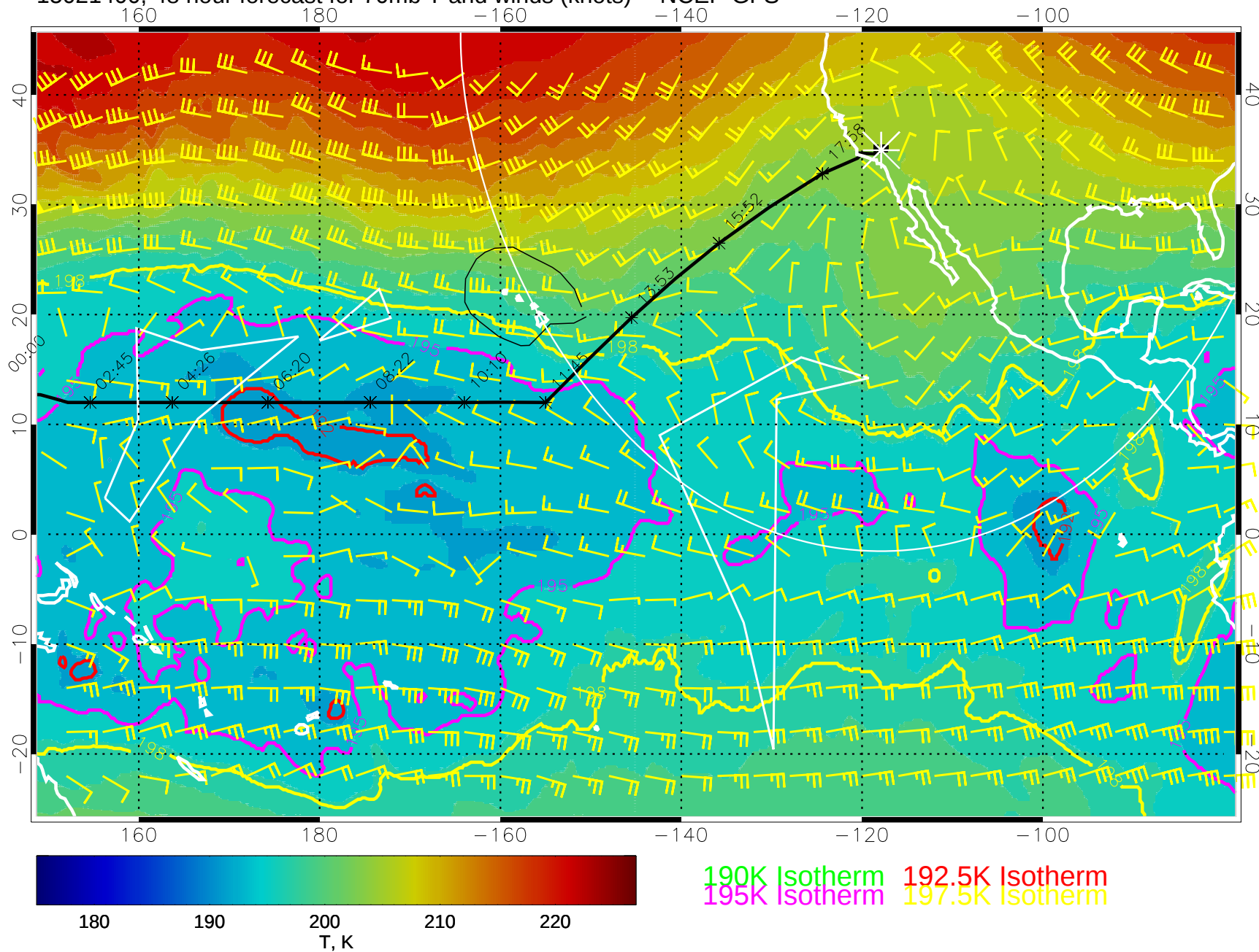
15021400, 48 hour forecast for 70mb T and winds (knots) -- NCEP GFS
