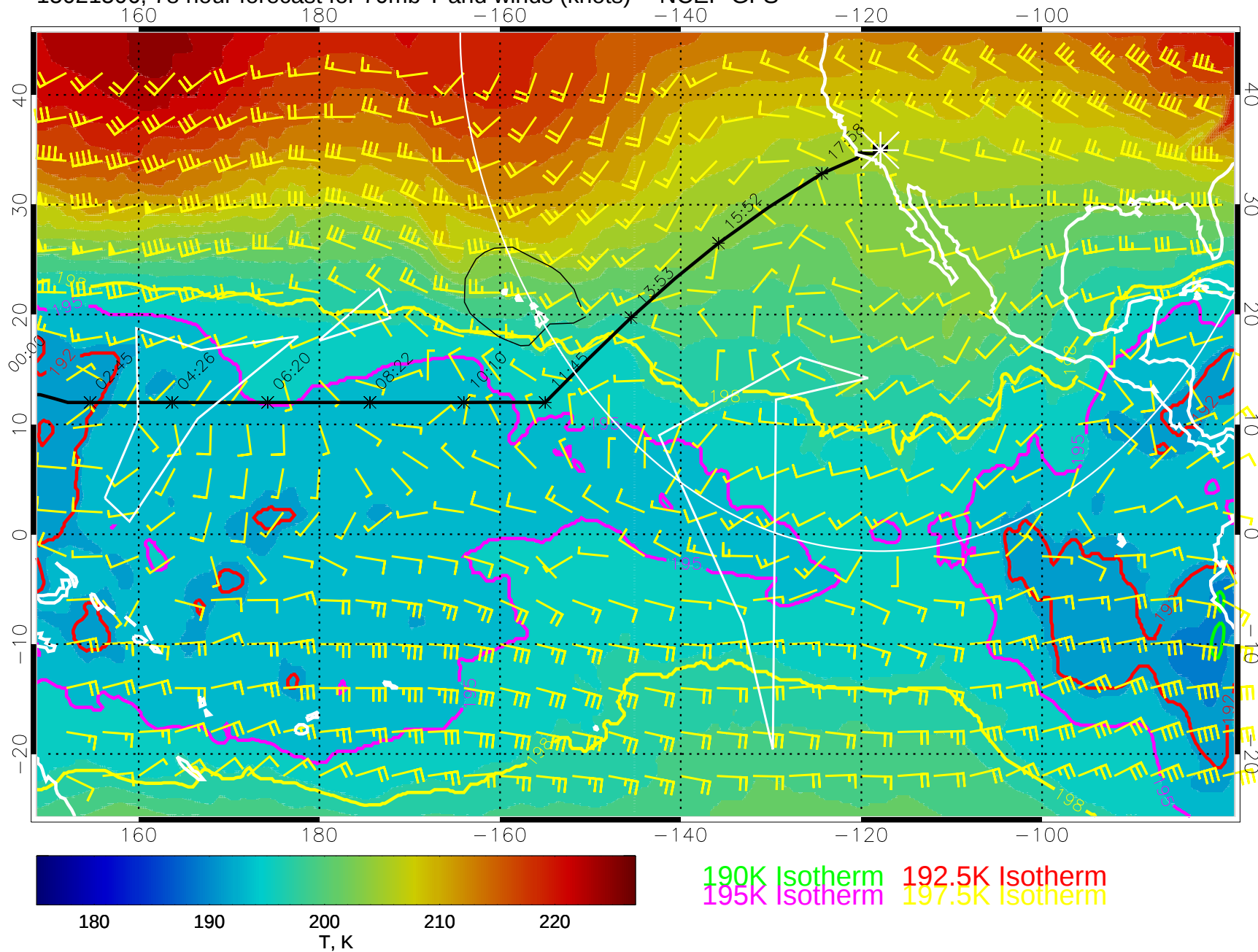
15021506, 78 hour forecast for 70mb T and winds (knots) -- NCEP GFS
