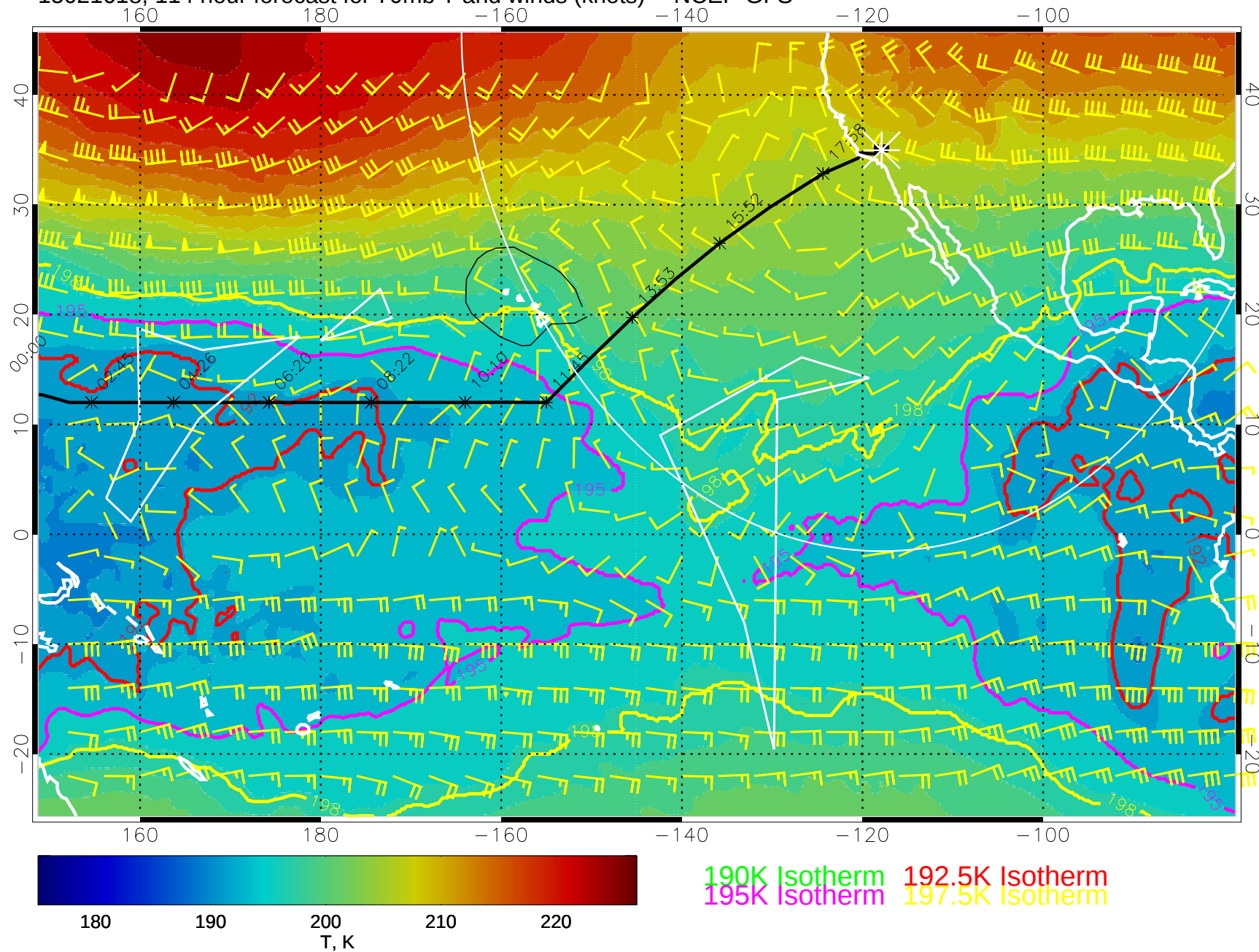
15021618, 114 hour forecast for 70mb T and winds (knots) -- NCEP GFS
