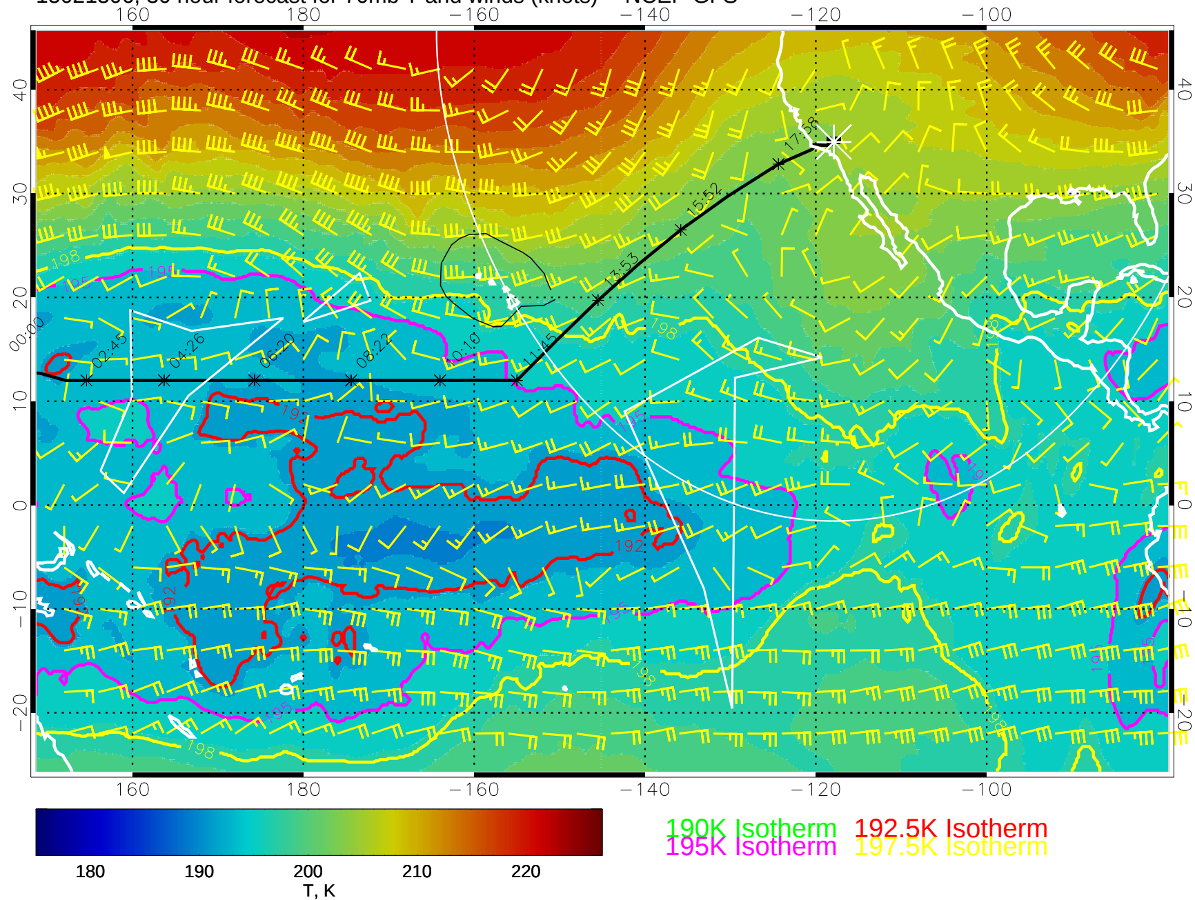
15021306, 30 hour forecast for 70mb T and winds (knots) -- NCEP GFS
