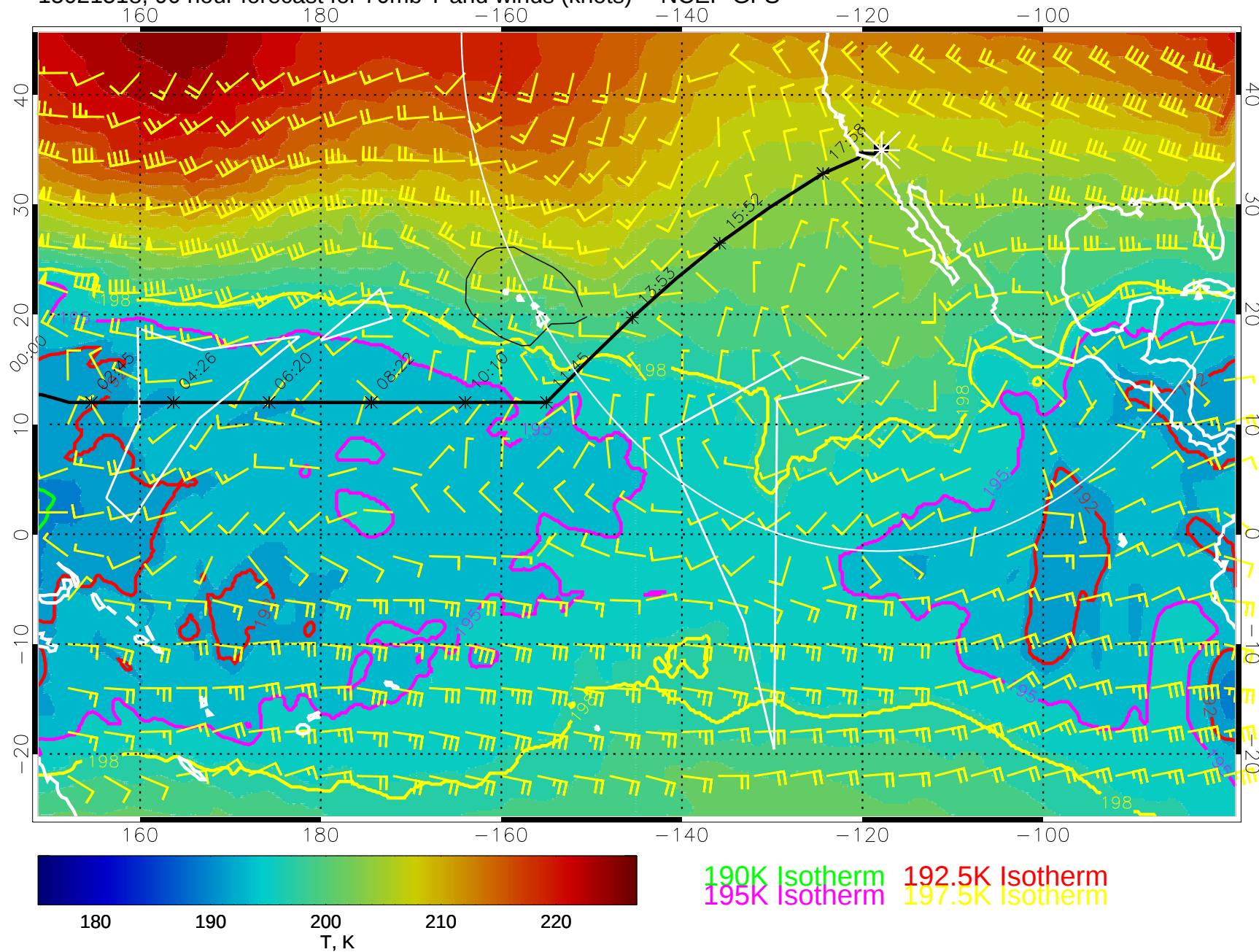
15021518, 90 hour forecast for 70mb T and winds (knots) -- NCEP GFS
