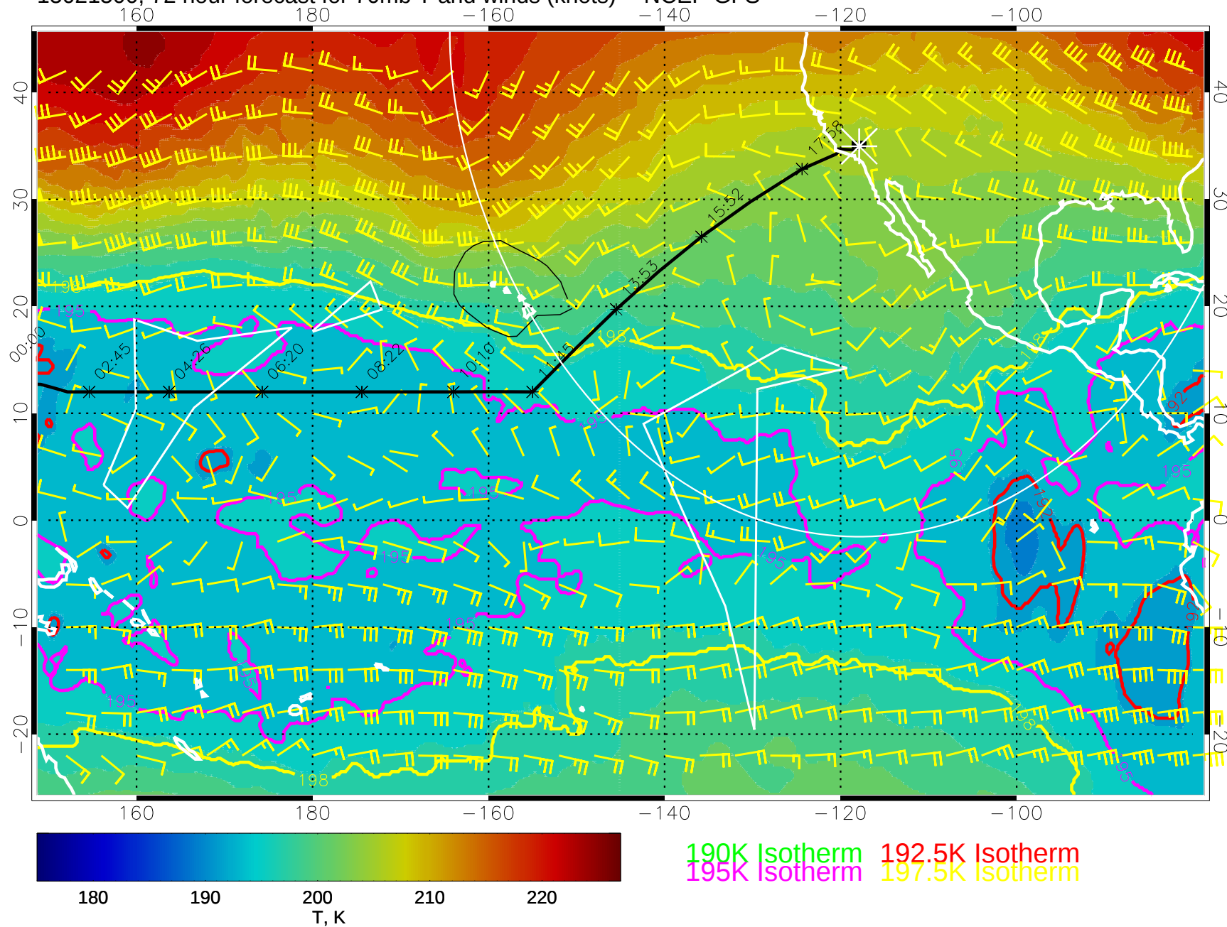
15021500, 72 hour forecast for 70mb T and winds (knots) -- NCEP GFS
