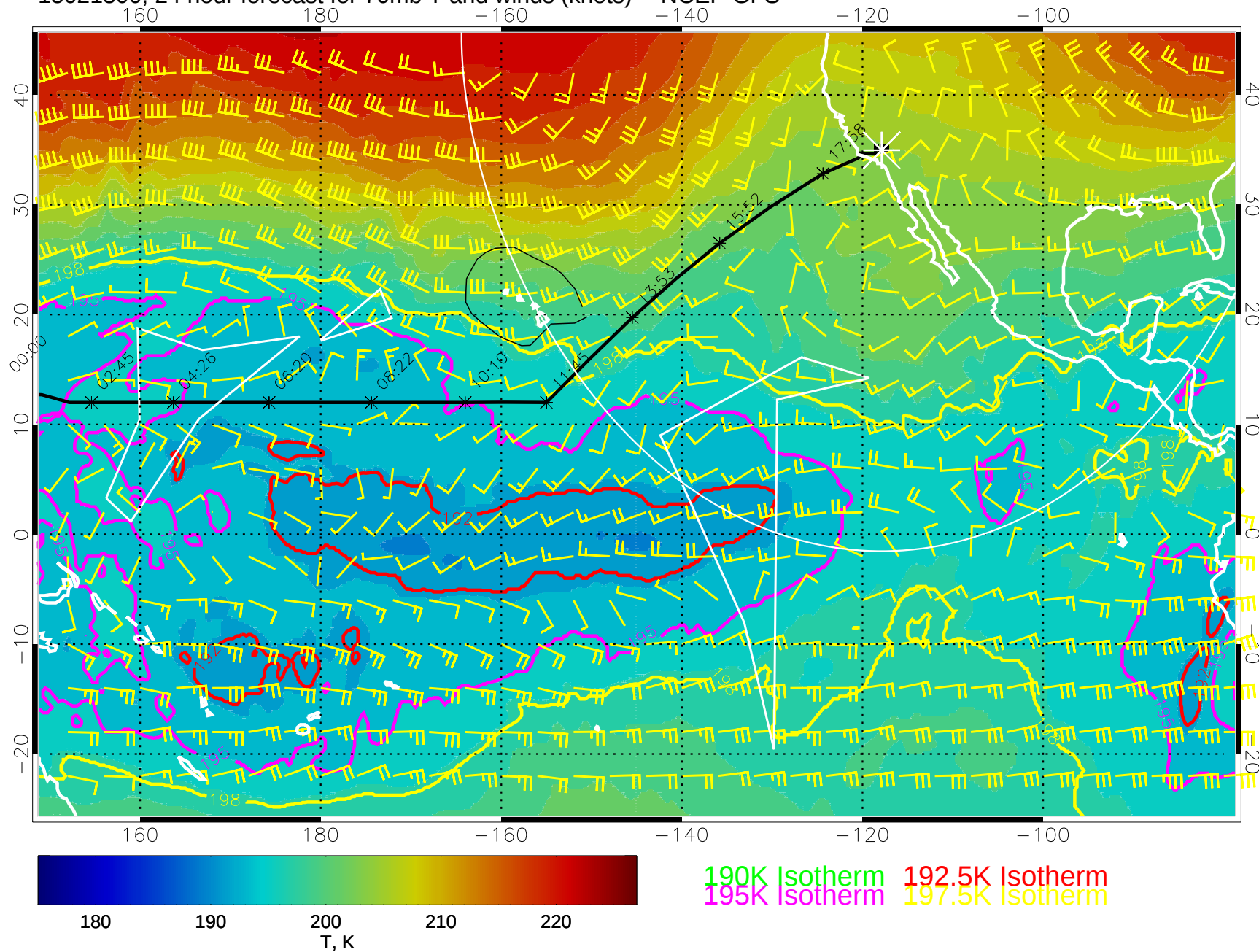
15021300, 24 hour forecast for 70mb T and winds (knots) -- NCEP GFS
