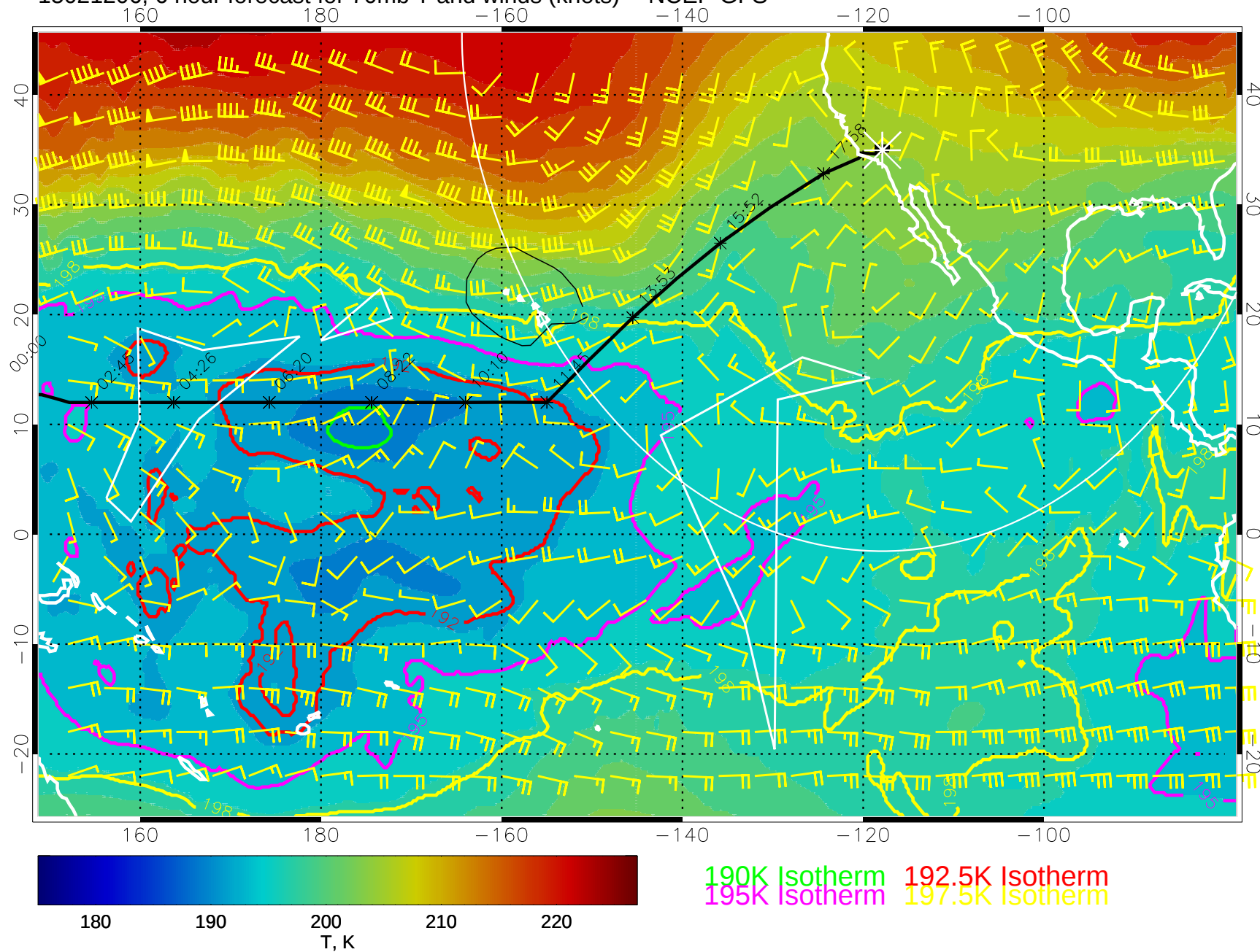
15021206, 6 hour forecast for 70mb T and winds (knots) -- NCEP GFS
