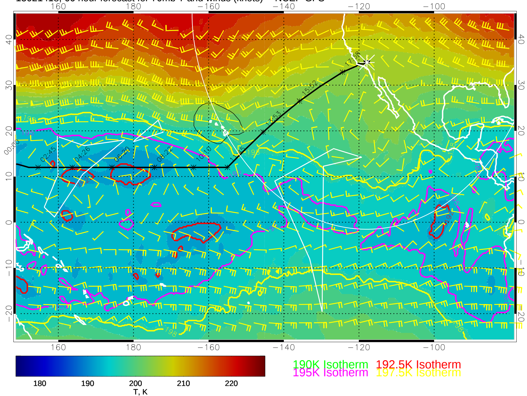
15021418, 66 hour forecast for 70mb T and winds (knots) -- NCEP GFS
