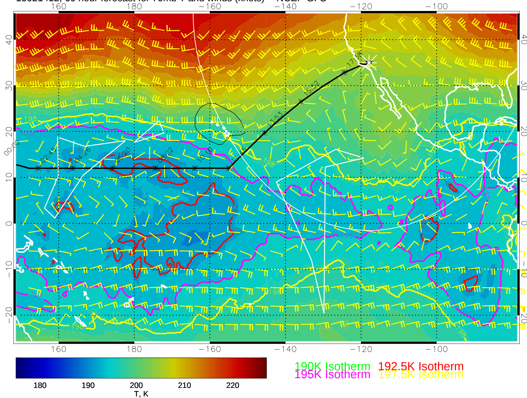
15021412, 60 hour forecast for 70mb T and winds (knots) -- NCEP GFS
