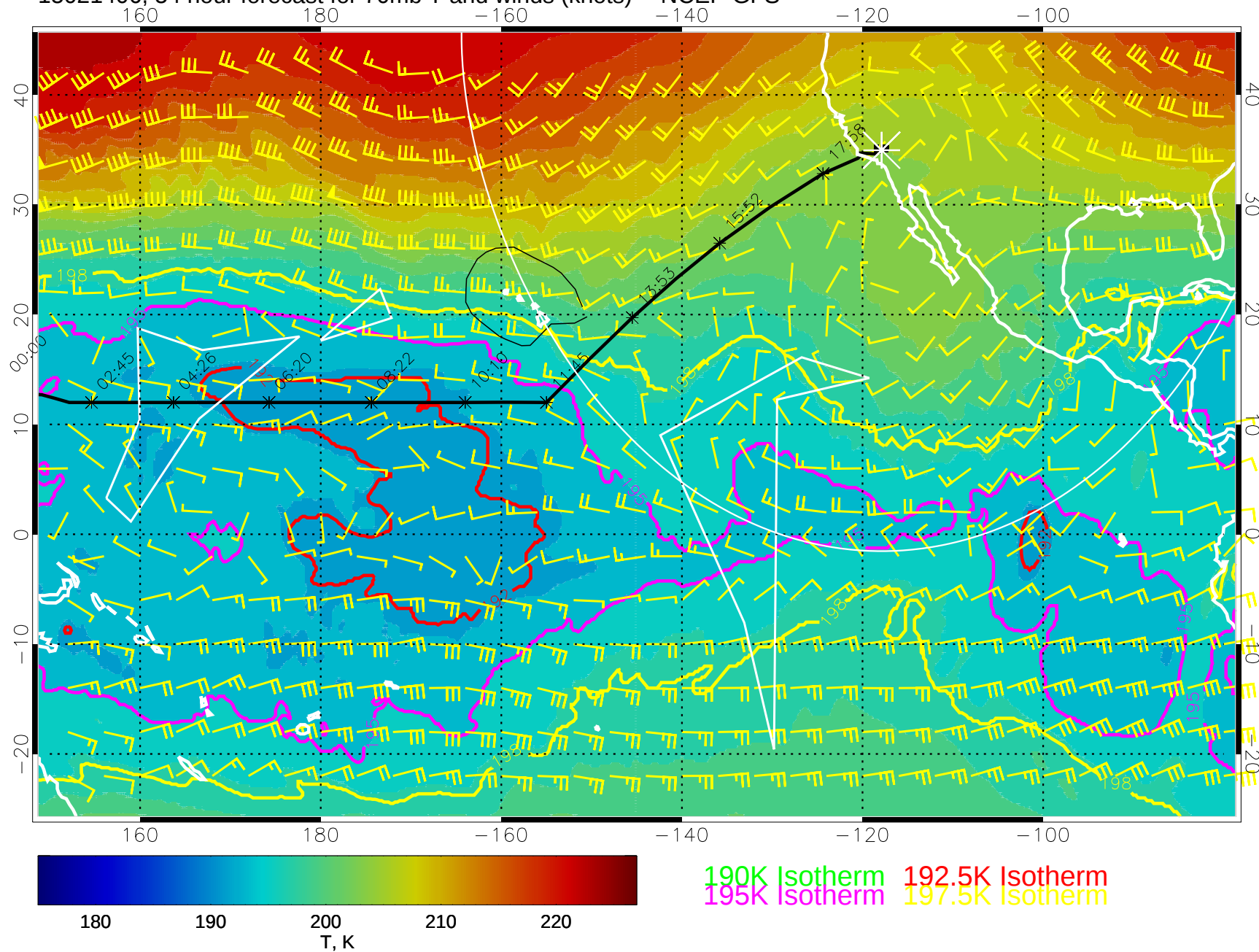
15021406, 54 hour forecast for 70mb T and winds (knots) -- NCEP GFS
