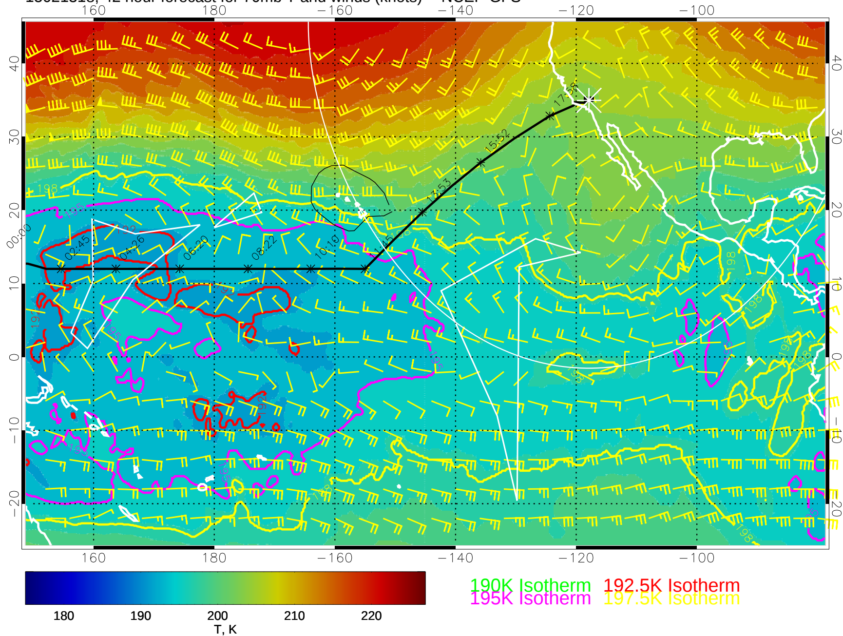
15021318, 42 hour forecast for 70mb T and winds (knots) -- NCEP GFS
