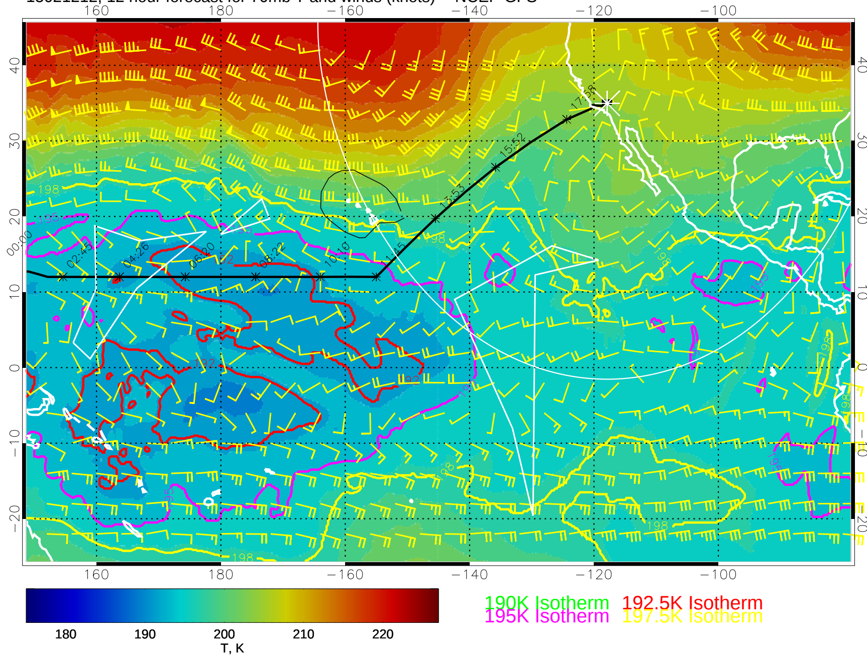
15021212, 12 hour forecast for 70mb T and winds (knots) -- NCEP GFS
