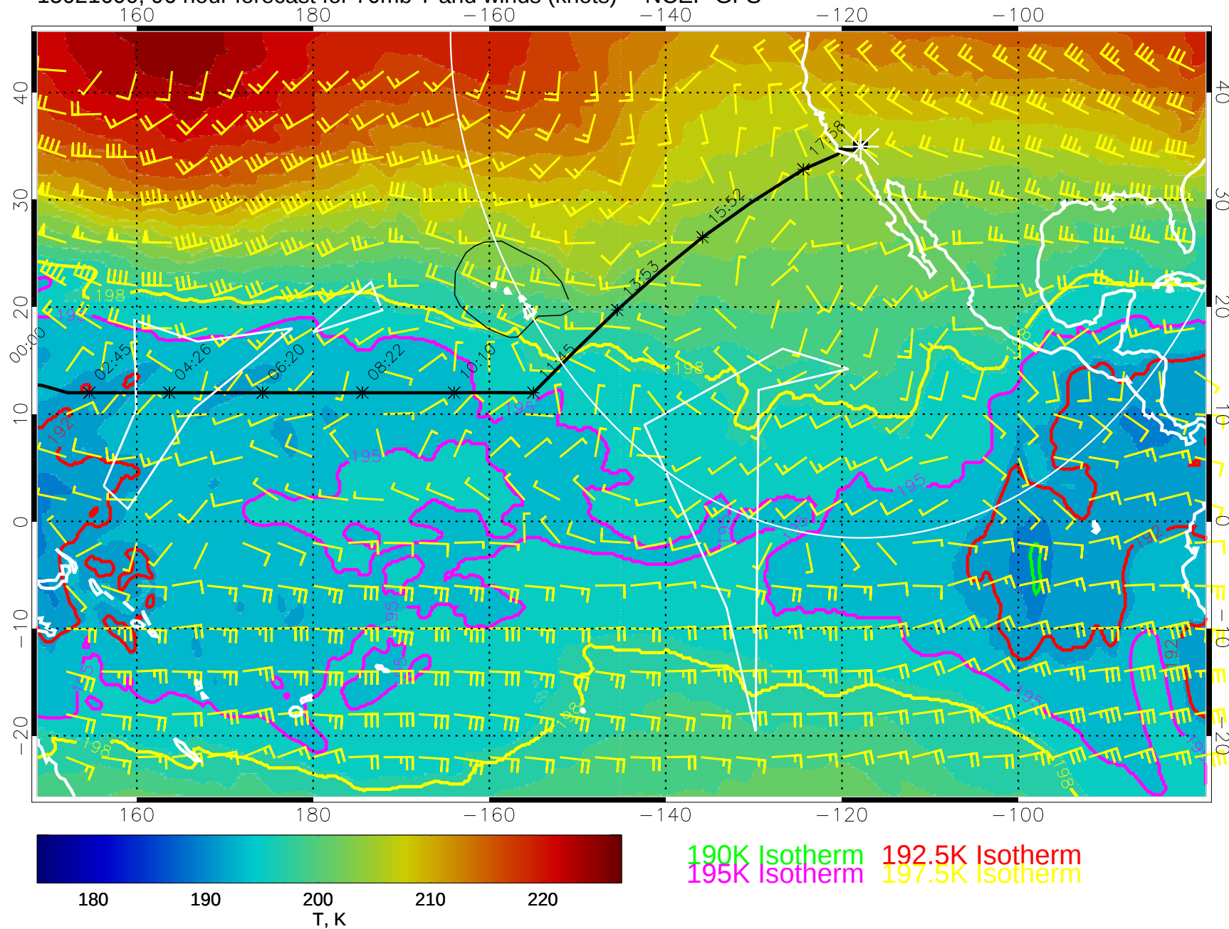
15021600, 96 hour forecast for 70mb T and winds (knots) -- NCEP GFS
