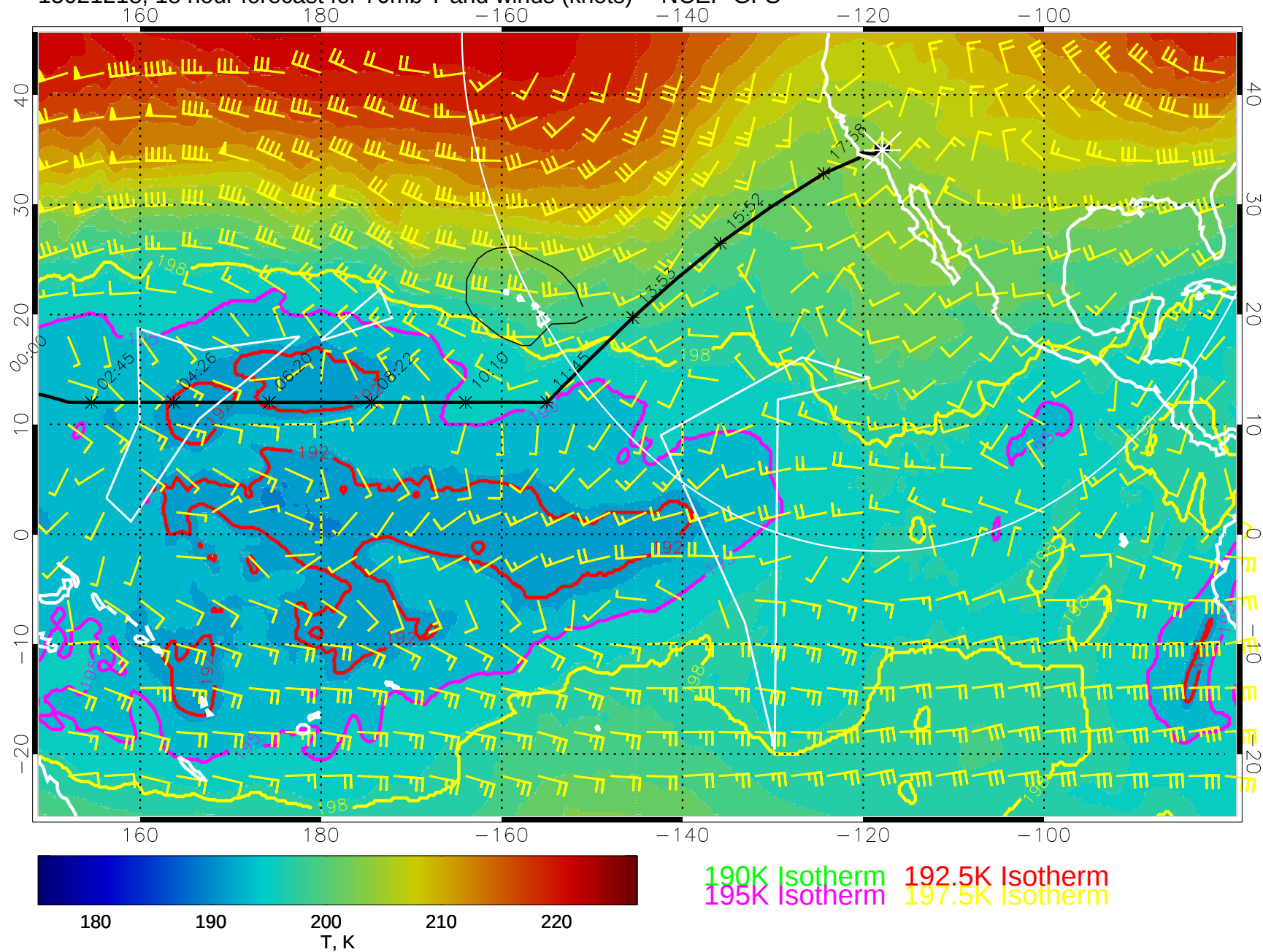
15021218, 18 hour forecast for 70mb T and winds (knots) -- NCEP GFS
