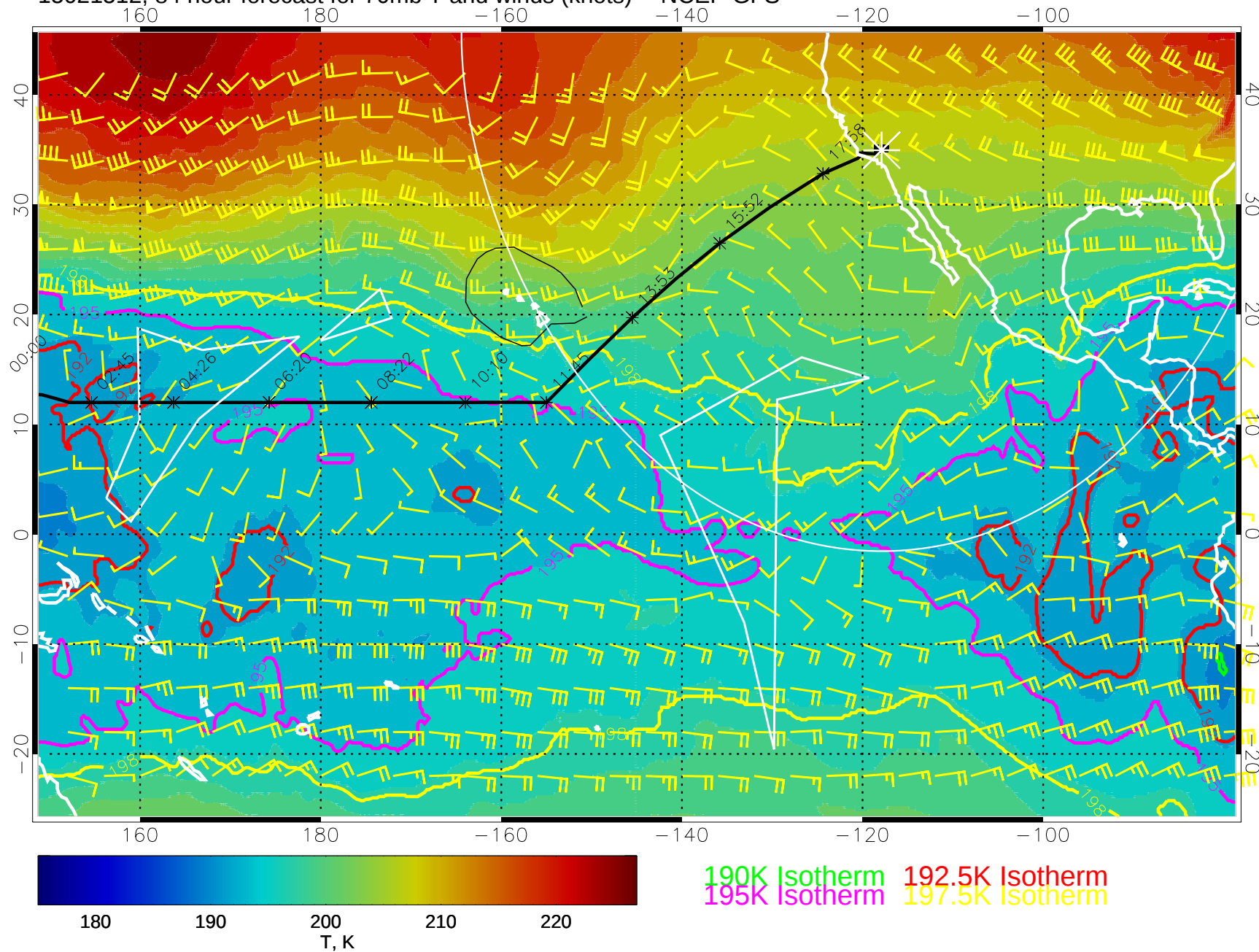
15021512, 84 hour forecast for 70mb T and winds (knots) -- NCEP GFS
