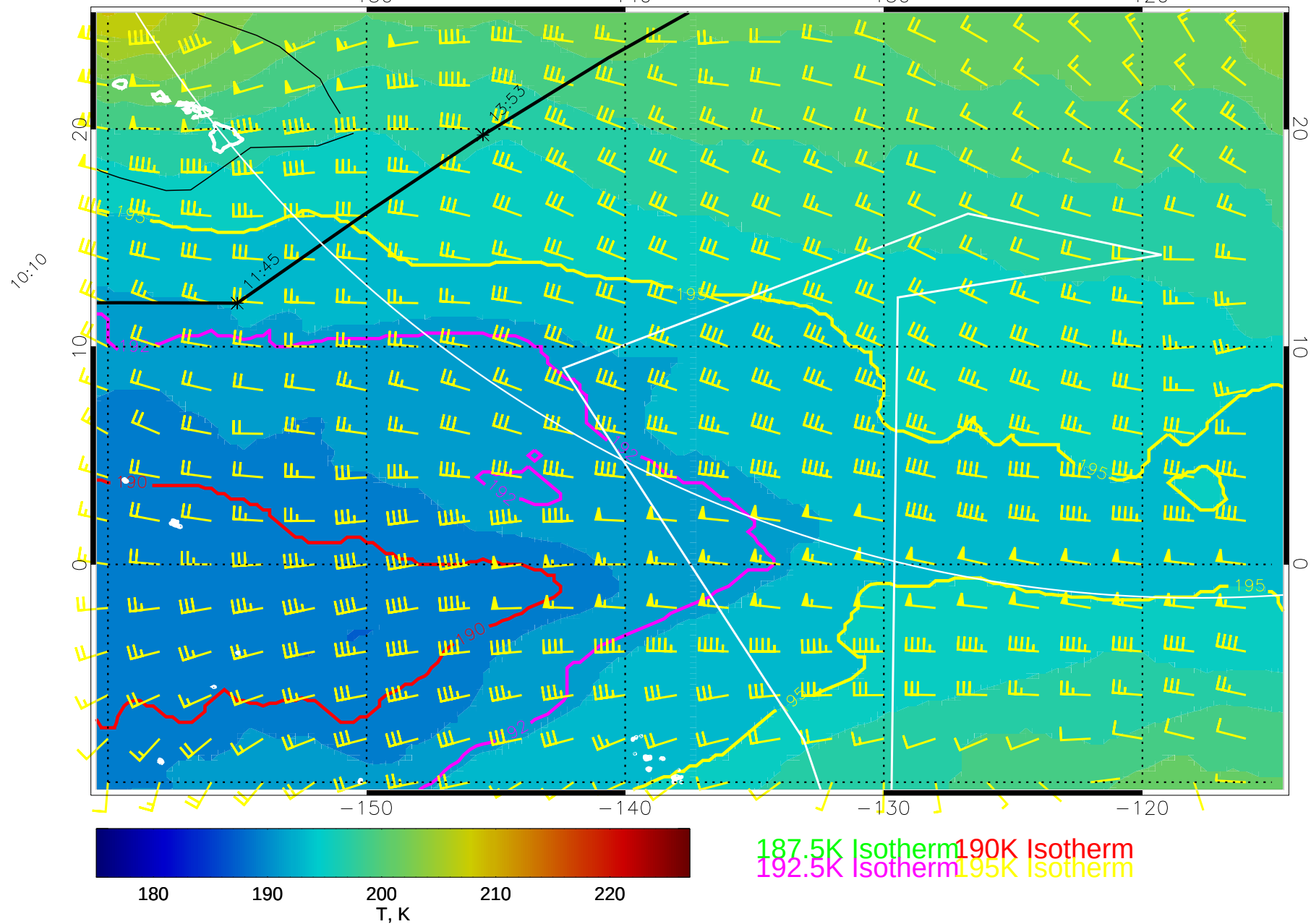
15021500, 72 hour forecast for 100mb T and winds (knots) -- NCEP GFS
