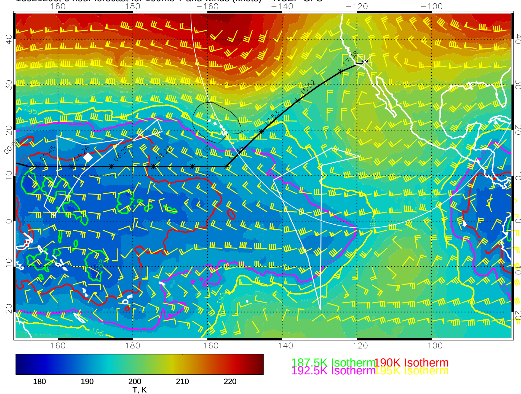
15021206, 6 hour forecast for 100mb T and winds (knots) -- NCEP GFS
