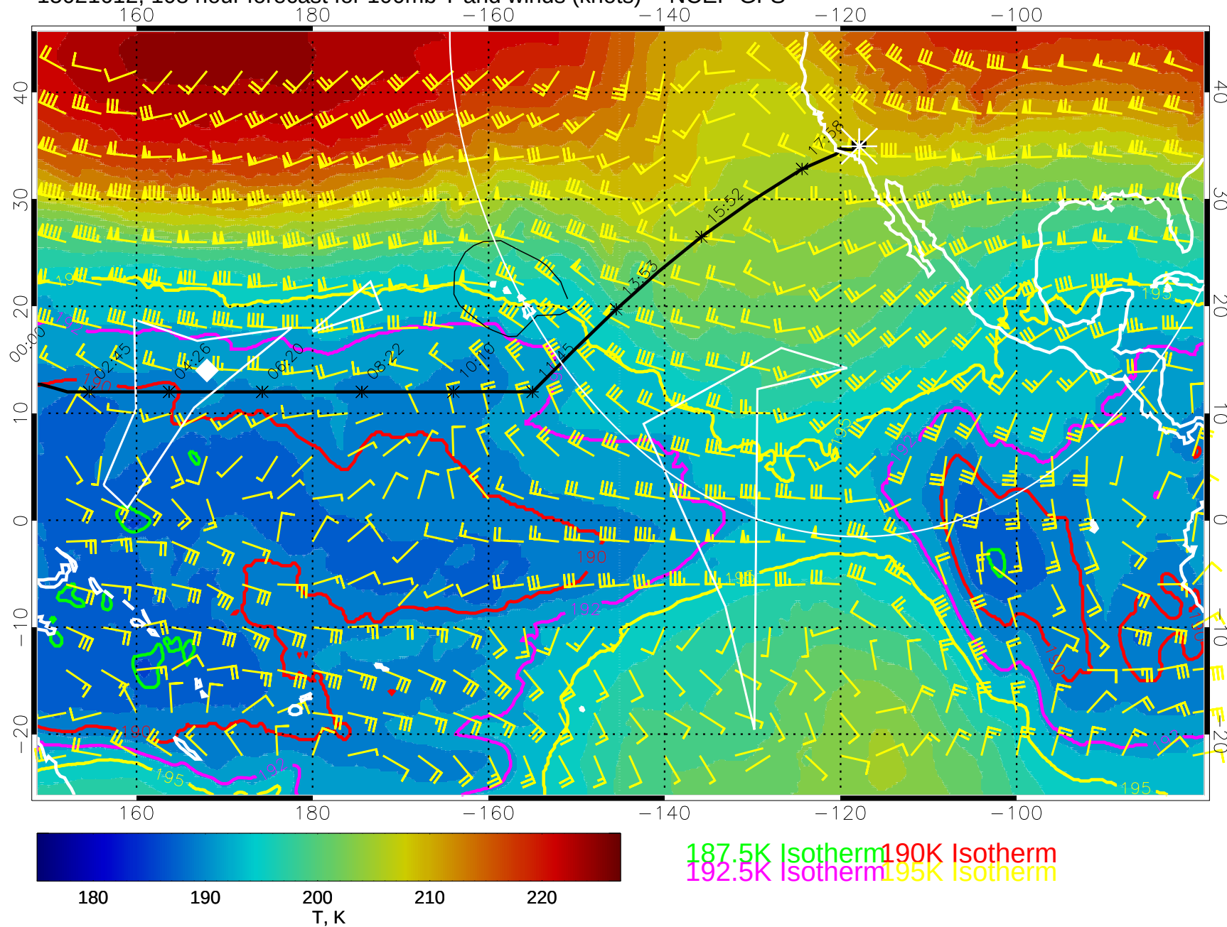
15021612, 108 hour forecast for 100mb T and winds (knots) -- NCEP GFS
