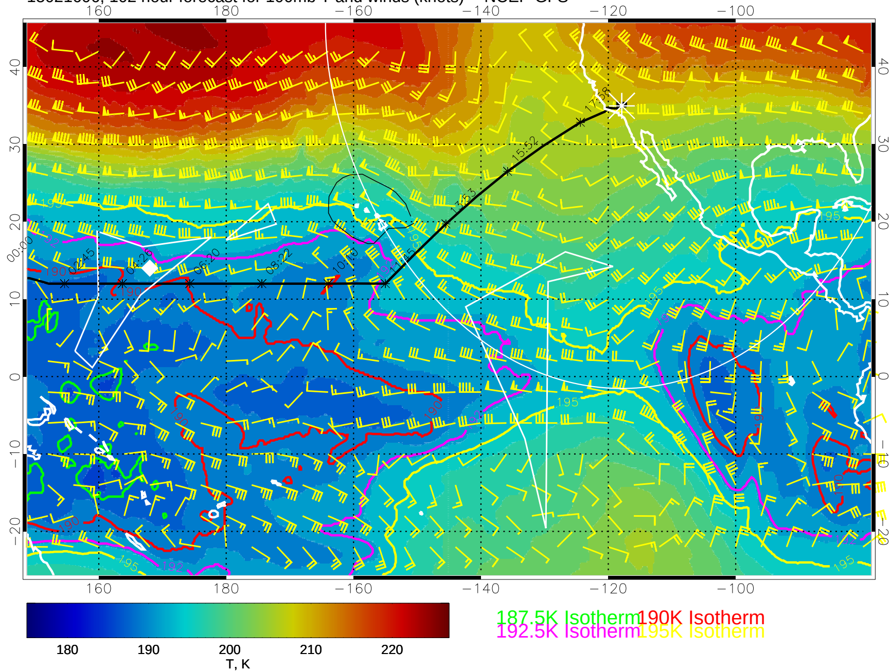
15021606, 102 hour forecast for 100mb T and winds (knots) -- NCEP GFS
