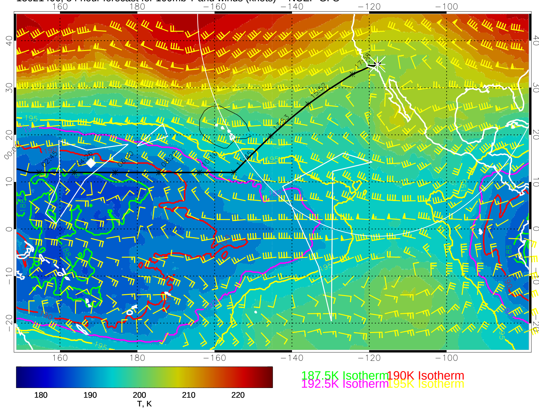
15021406, 54 hour forecast for 100mb T and winds (knots) -- NCEP GFS
