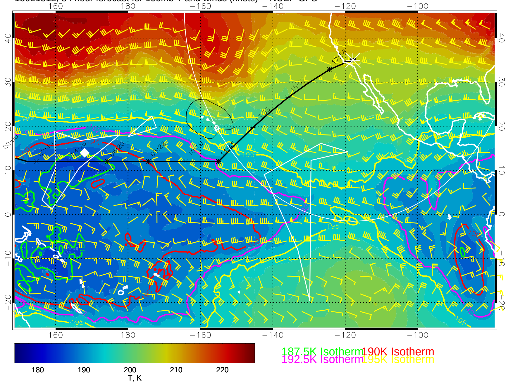
15021512, 84 hour forecast for 100mb T and winds (knots) -- NCEP GFS
