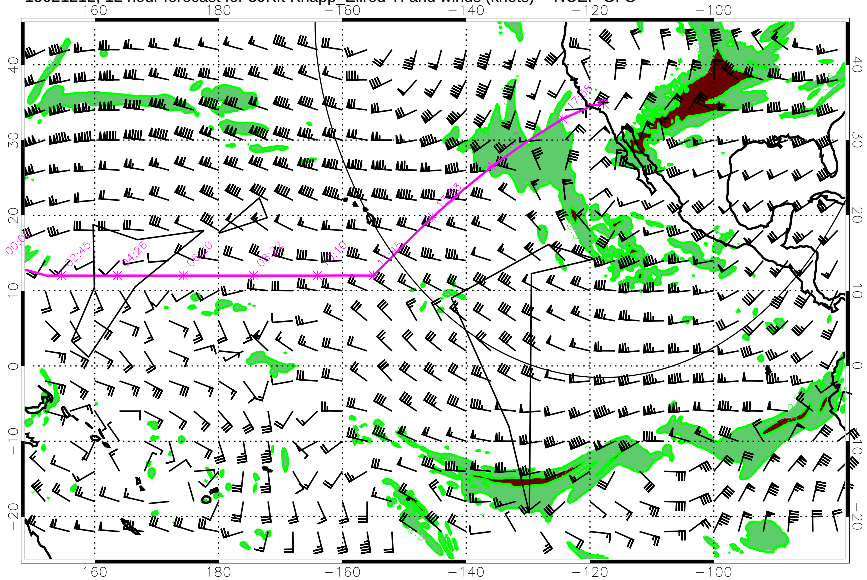
15021212, 12 hour forecast for 39Kft Knapp_Ellrod TI and winds (knots) -- NCEP GFS
