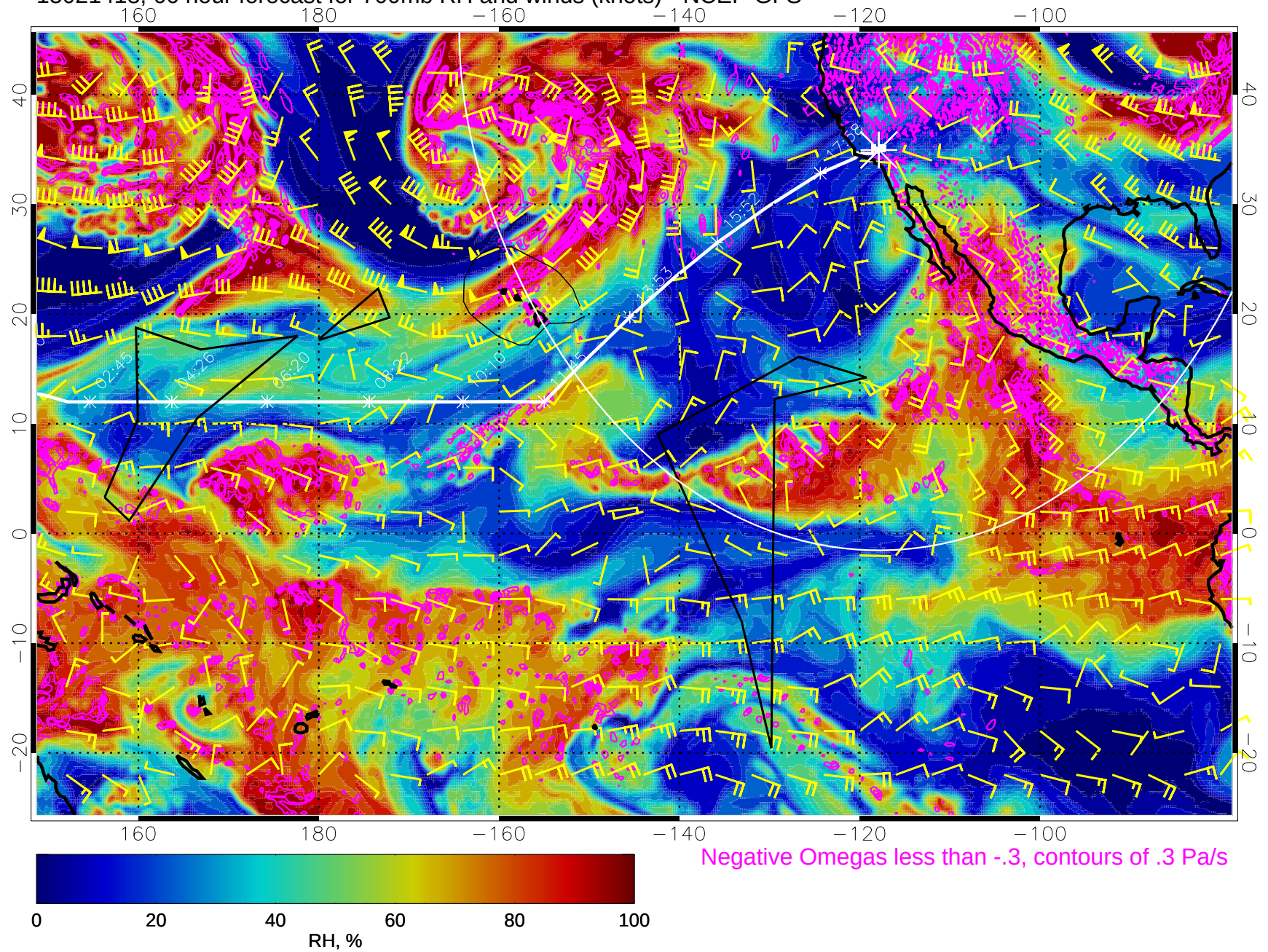
15021418, 66 hour forecast for 700mb RH and winds (knots) - NCEP GFS
