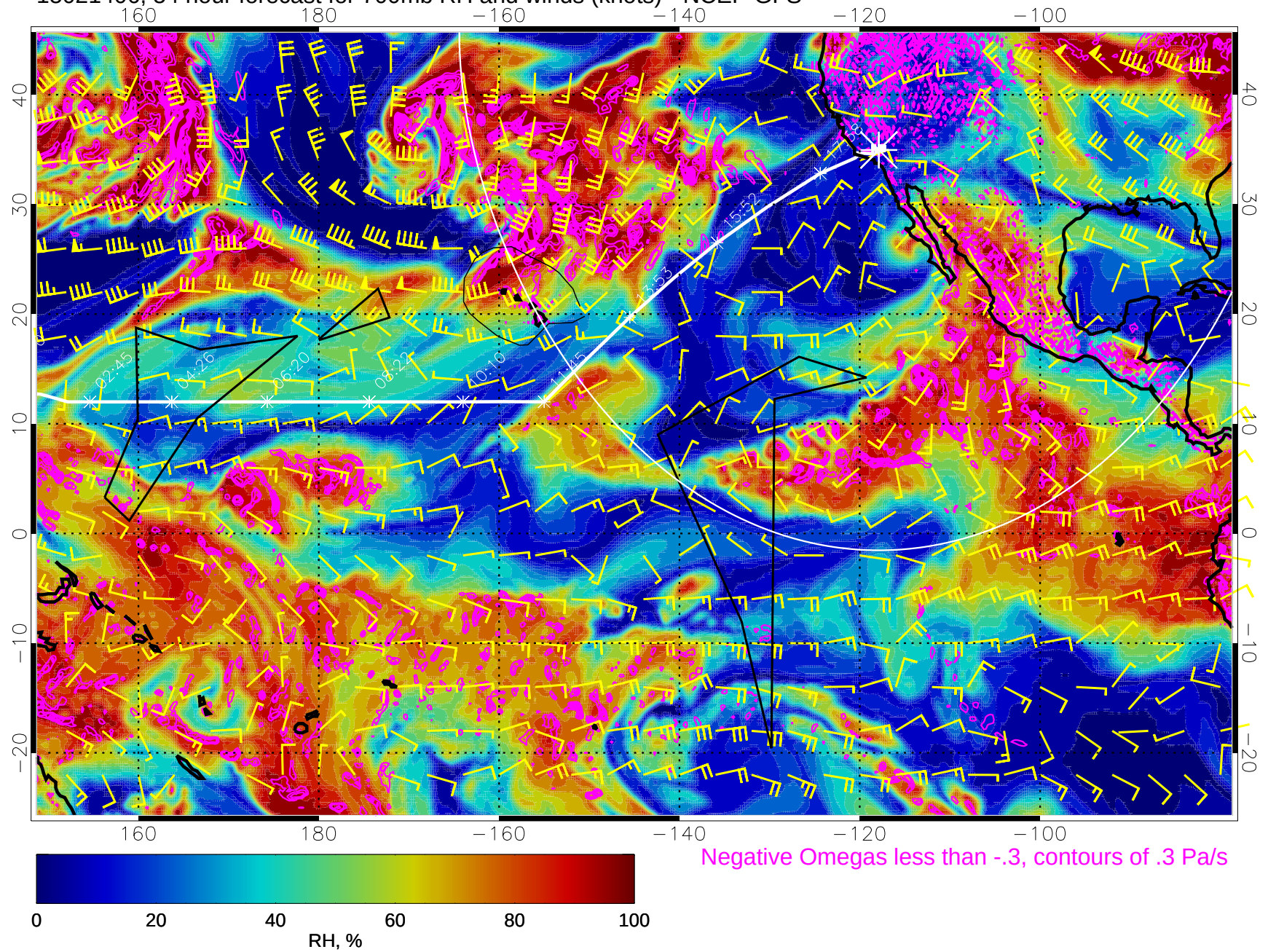
15021406, 54 hour forecast for 700mb RH and winds (knots) - NCEP GFS
