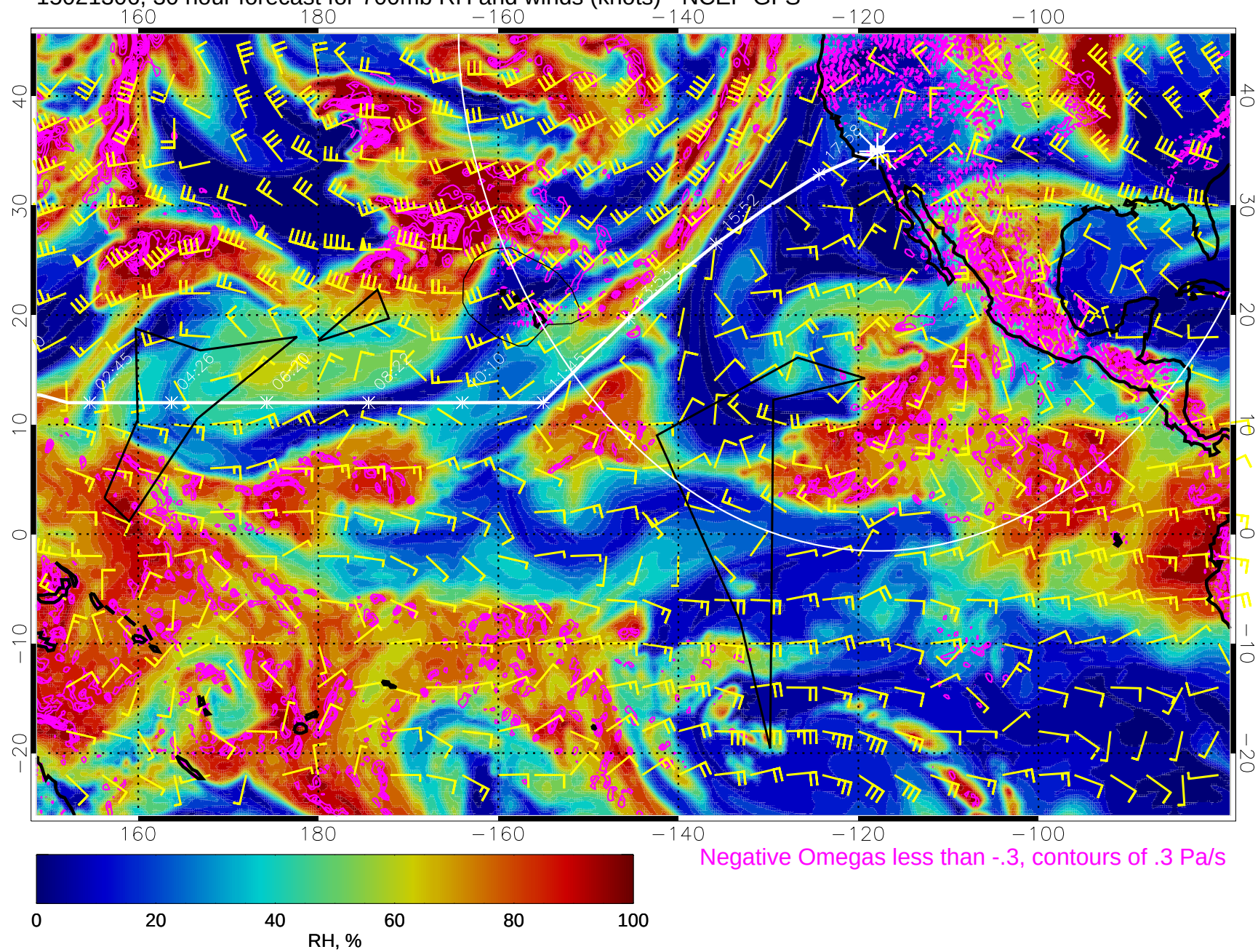
15021306, 30 hour forecast for 700mb RH and winds (knots) - NCEP GFS
