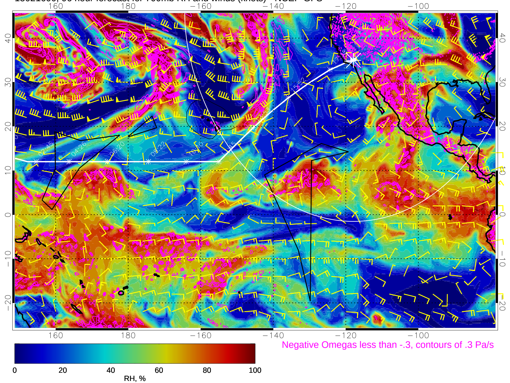
15021600, 96 hour forecast for 700mb RH and winds (knots) - NCEP GFS
