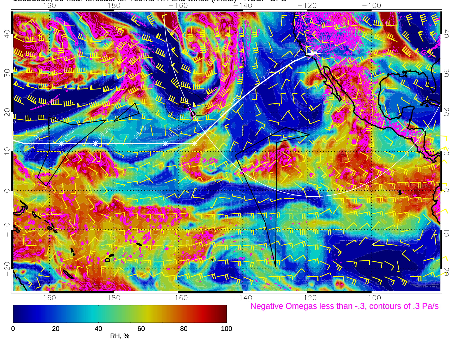
15021518, 90 hour forecast for 700mb RH and winds (knots) - NCEP GFS
