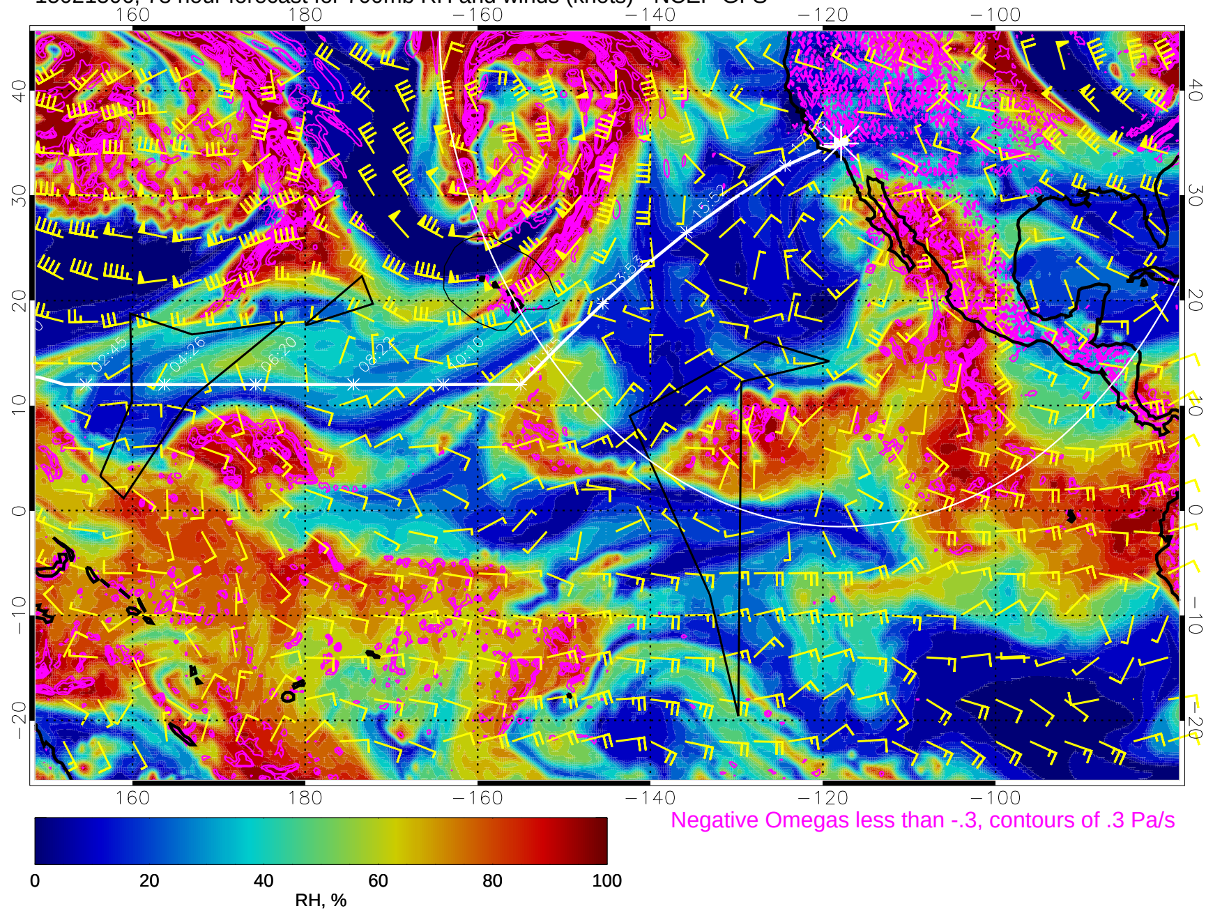
15021506, 78 hour forecast for 700mb RH and winds (knots) - NCEP GFS
