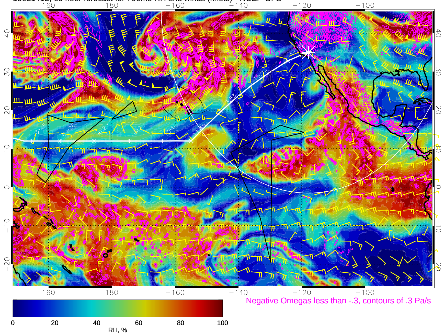
15021412, 60 hour forecast for 700mb RH and winds (knots) - NCEP GFS
