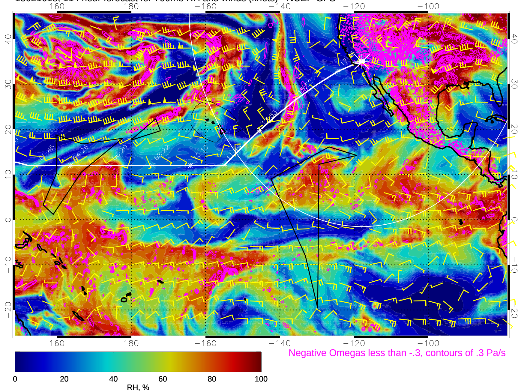
15021618, 114 hour forecast for 700mb RH and winds (knots) - NCEP GFS
