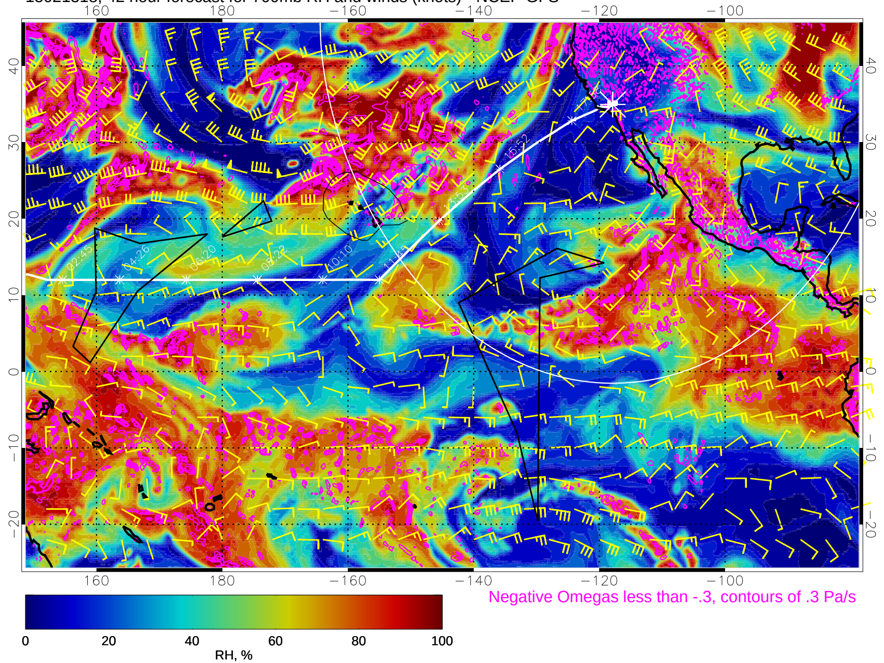
15021318, 42 hour forecast for 700mb RH and winds (knots) - NCEP GFS
