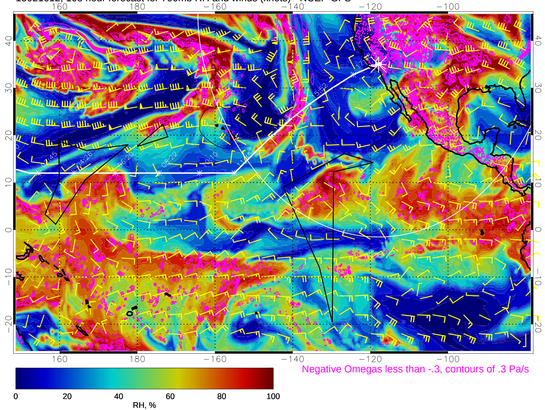
15021612, 108 hour forecast for 700mb RH and winds (knots) - NCEP GFS
