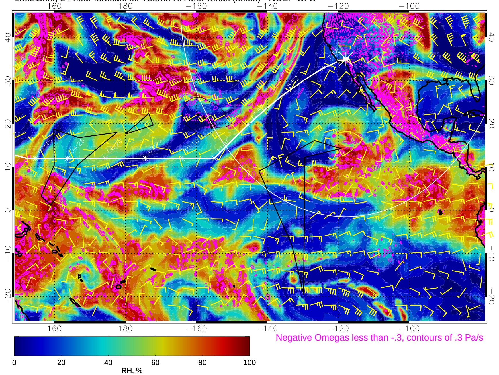
15021300, 24 hour forecast for 700mb RH and winds (knots) - NCEP GFS
