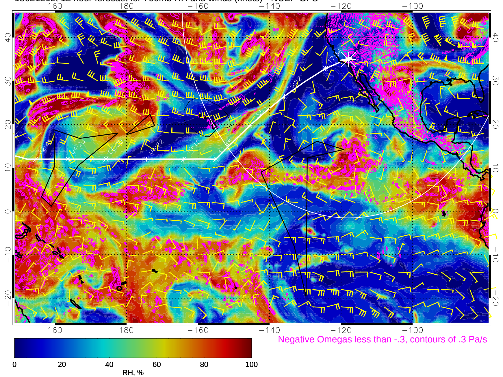
15021212, 12 hour forecast for 700mb RH and winds (knots) - NCEP GFS
