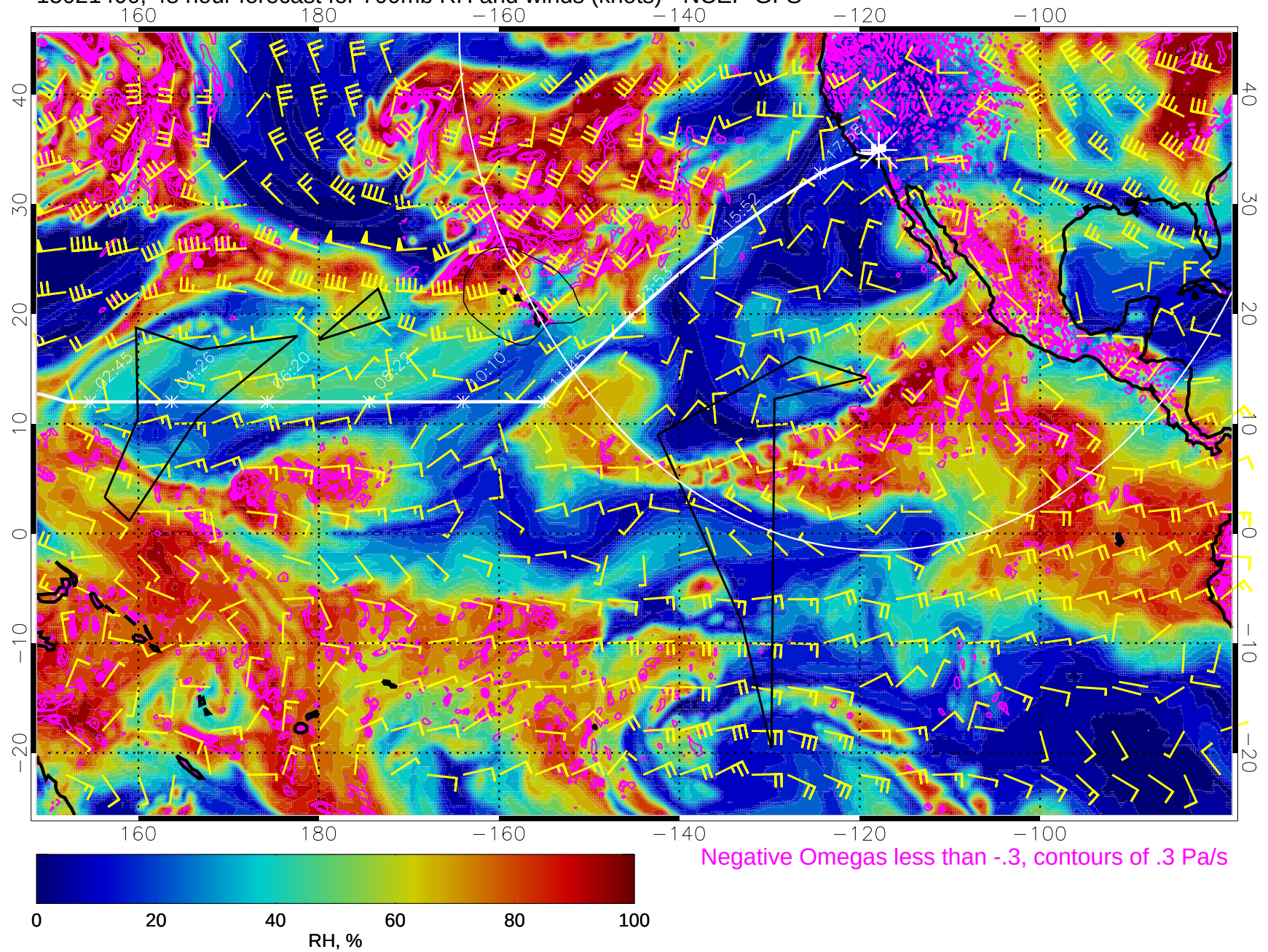
15021400, 48 hour forecast for 700mb RH and winds (knots) - NCEP GFS
