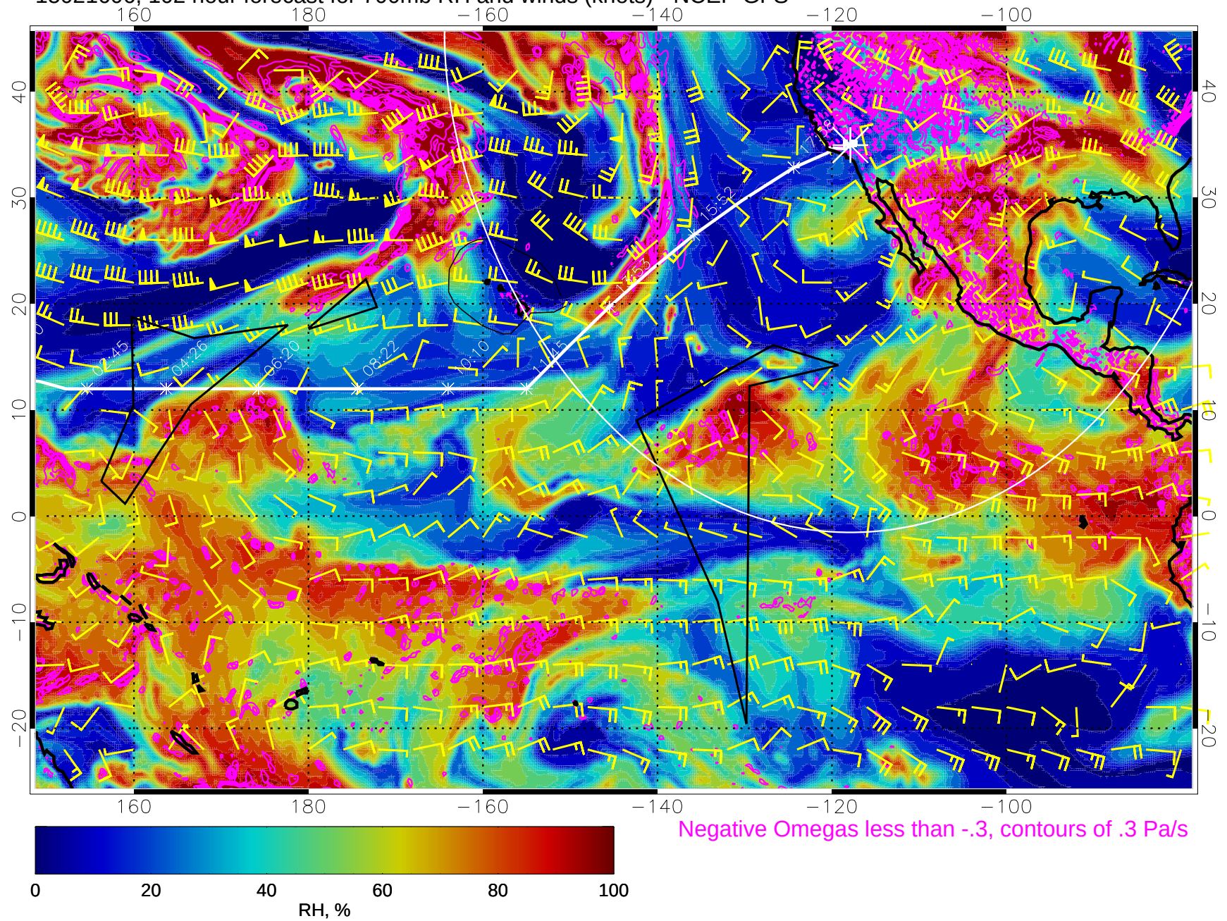
15021606, 102 hour forecast for 700mb RH and winds (knots) - NCEP GFS
