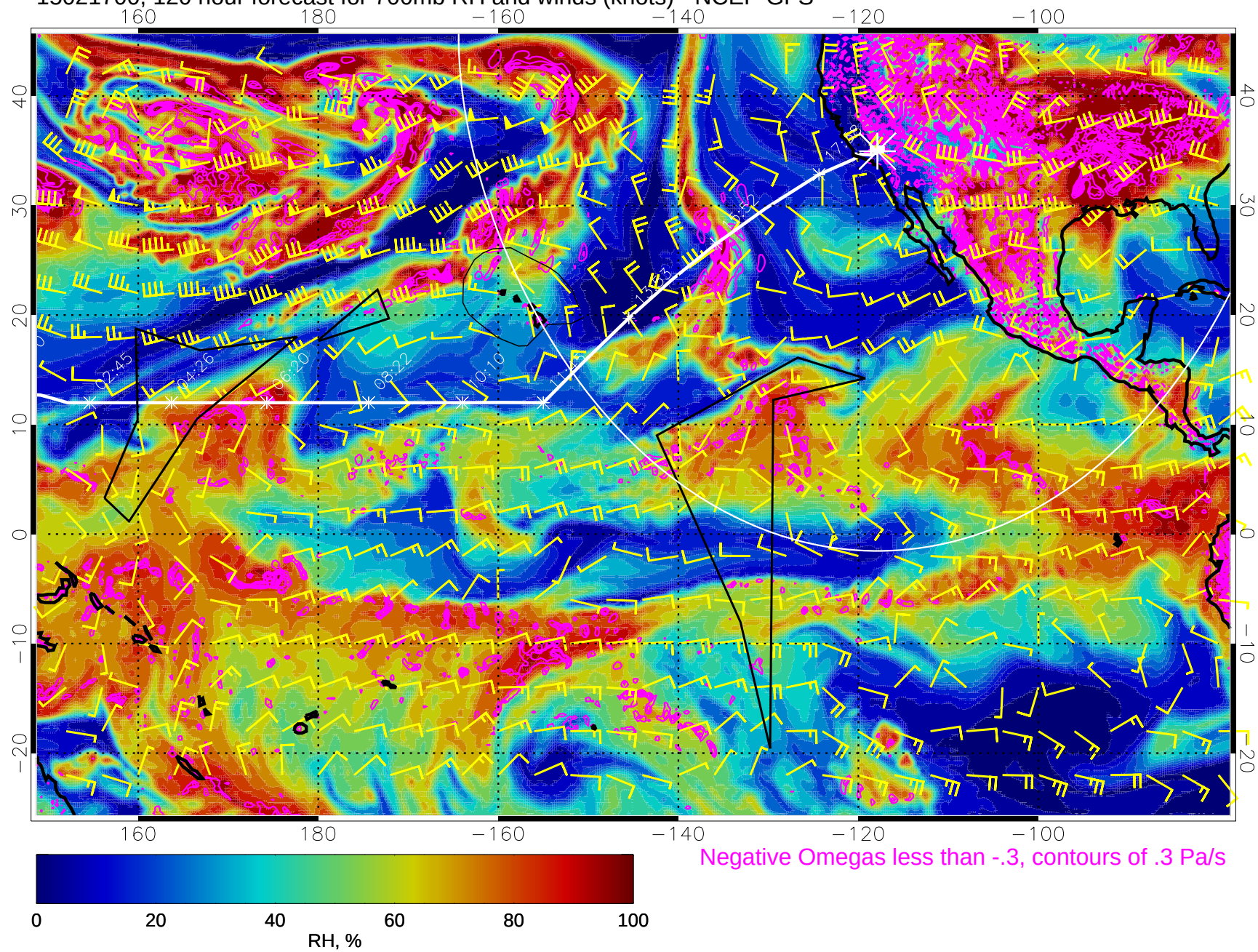
15021700, 120 hour forecast for 700mb RH and winds (knots) - NCEP GFS
