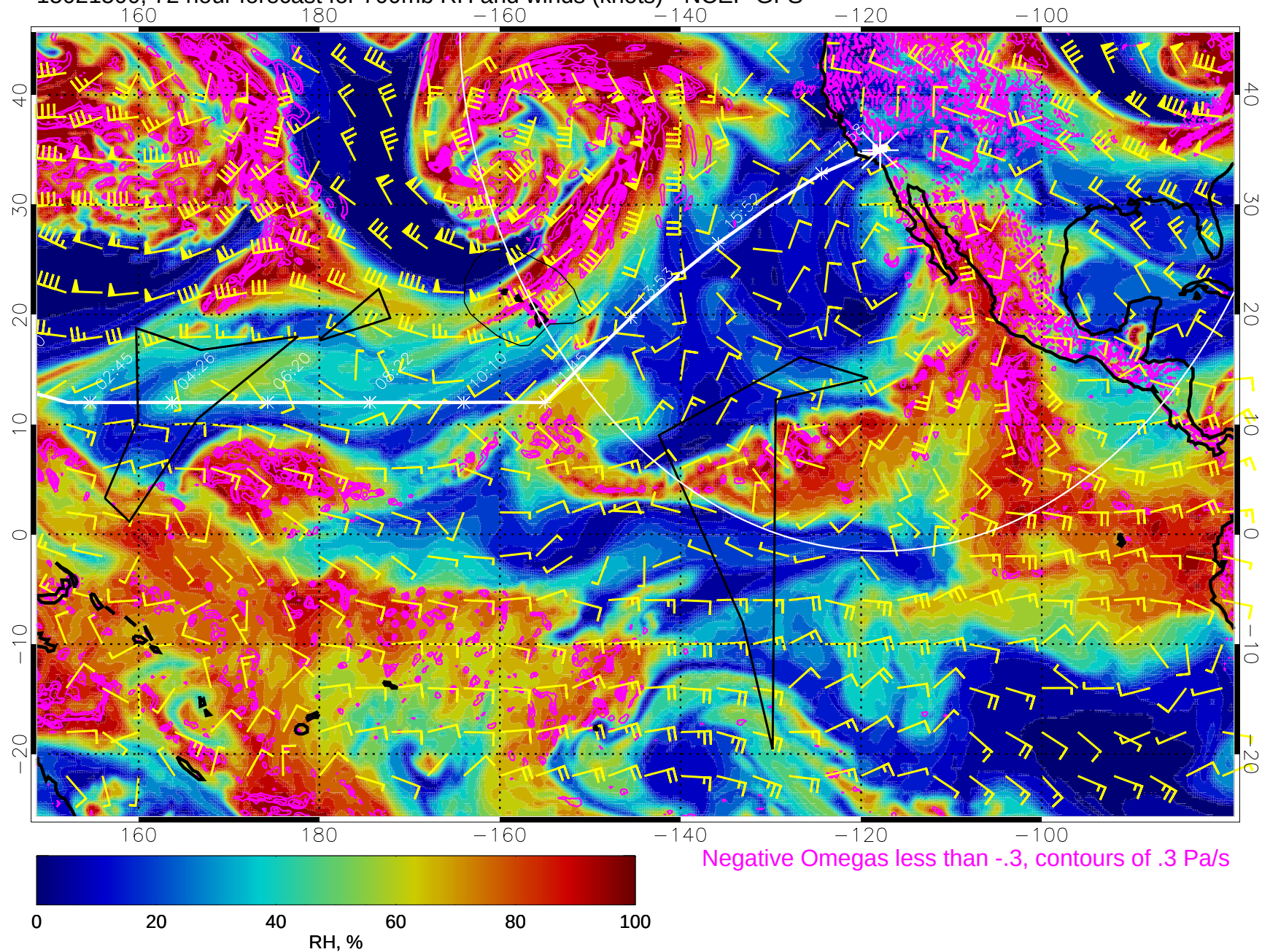
15021500, 72 hour forecast for 700mb RH and winds (knots) - NCEP GFS
