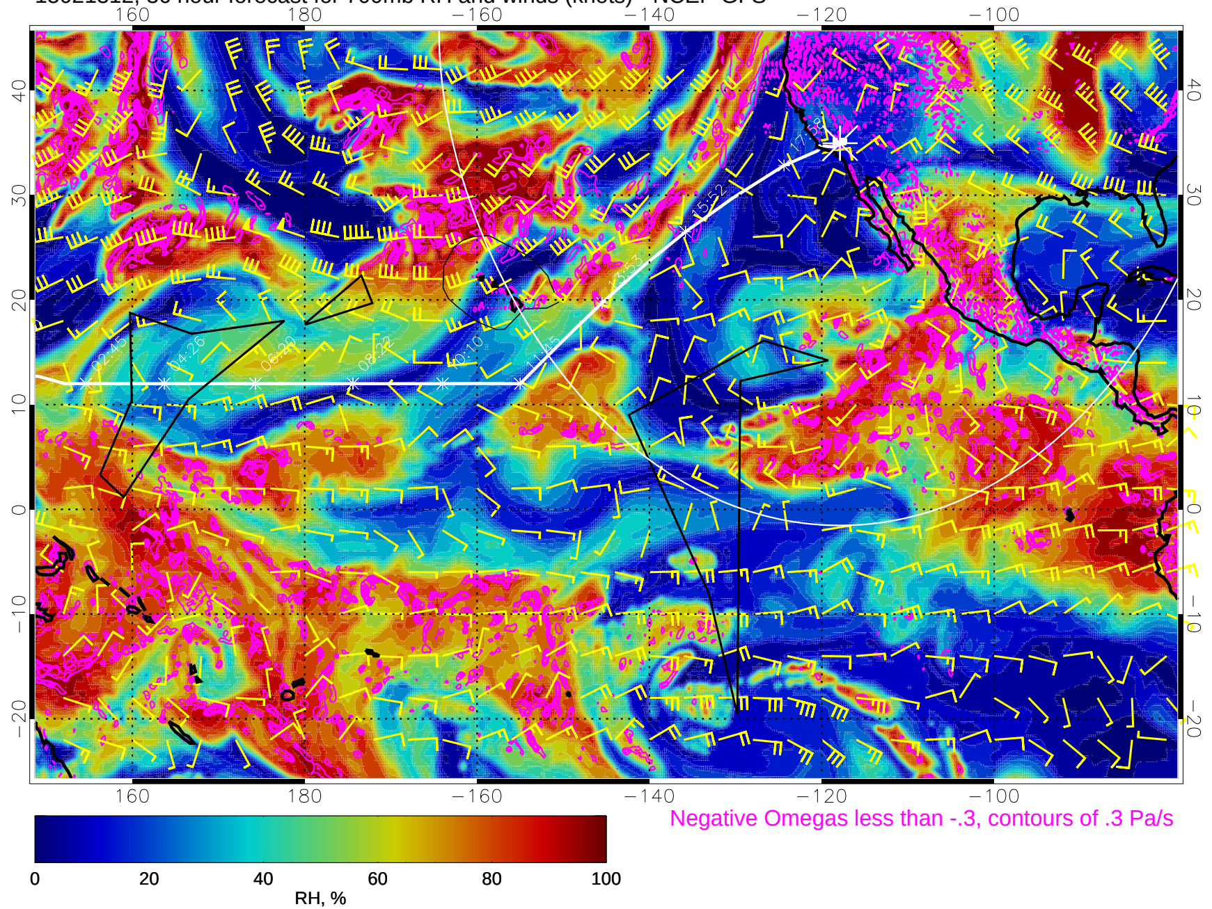
15021312, 36 hour forecast for 700mb RH and winds (knots) - NCEP GFS
