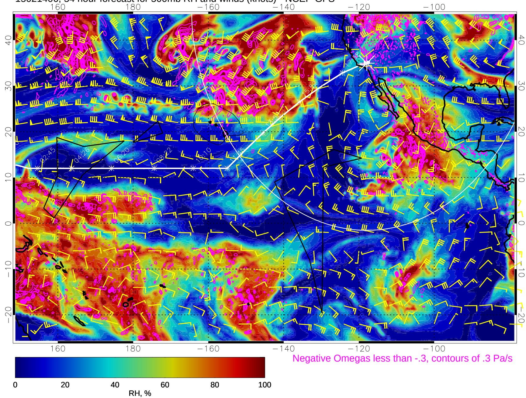
15021406, 54 hour forecast for 500mb RH and winds (knots) - NCEP GFS
