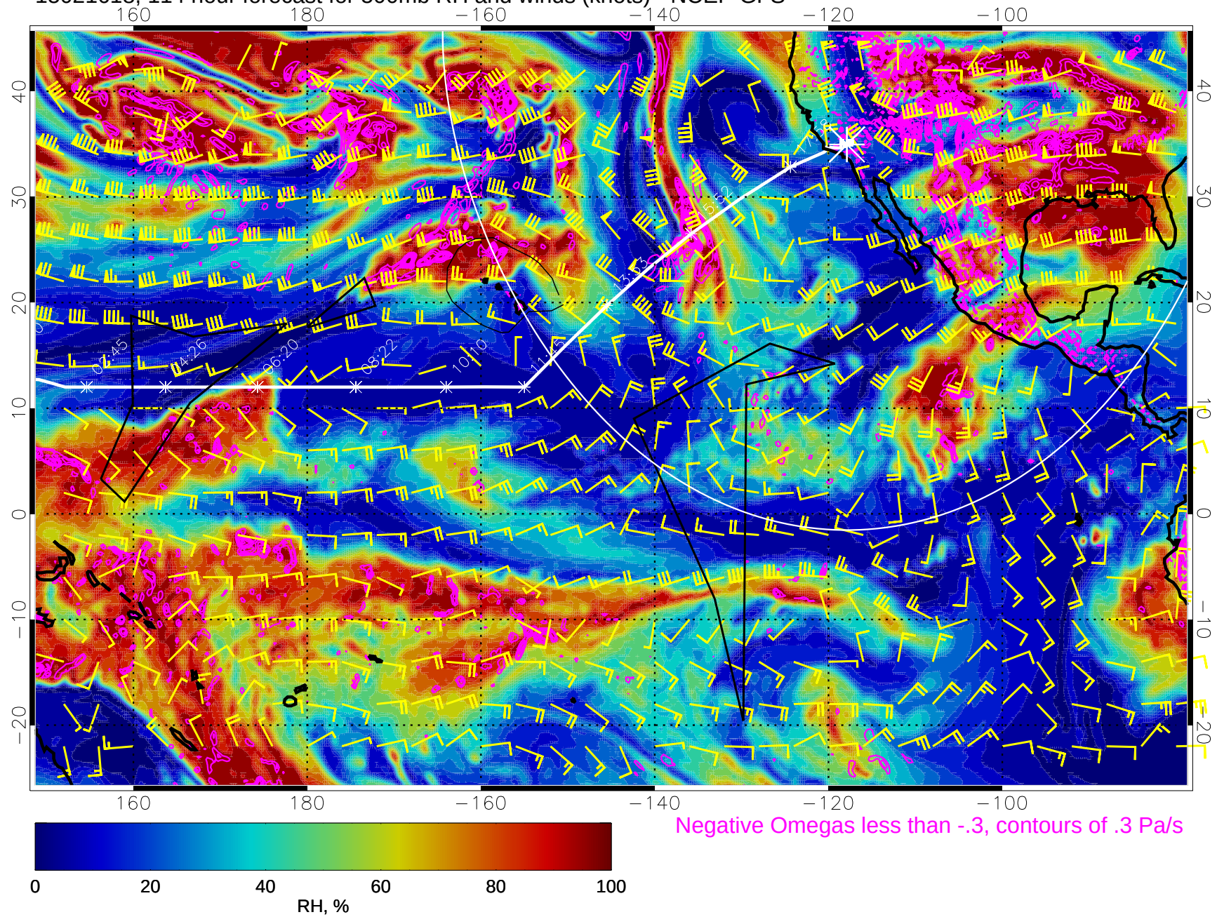
15021618, 114 hour forecast for 500mb RH and winds (knots) - NCEP GFS
