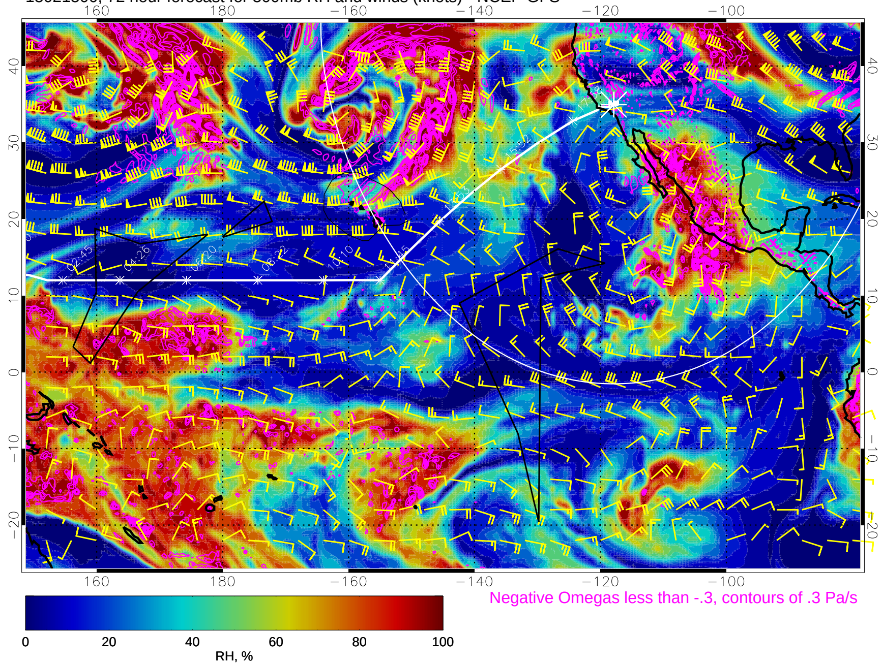
15021500, 72 hour forecast for 500mb RH and winds (knots) - NCEP GFS
