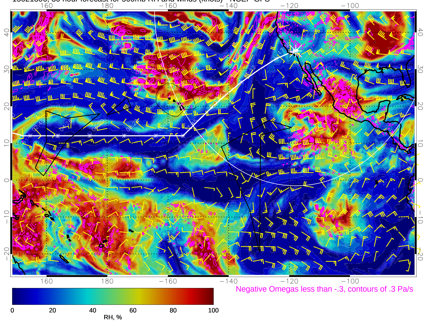
15021306, 30 hour forecast for 500mb RH and winds (knots) - NCEP GFS
