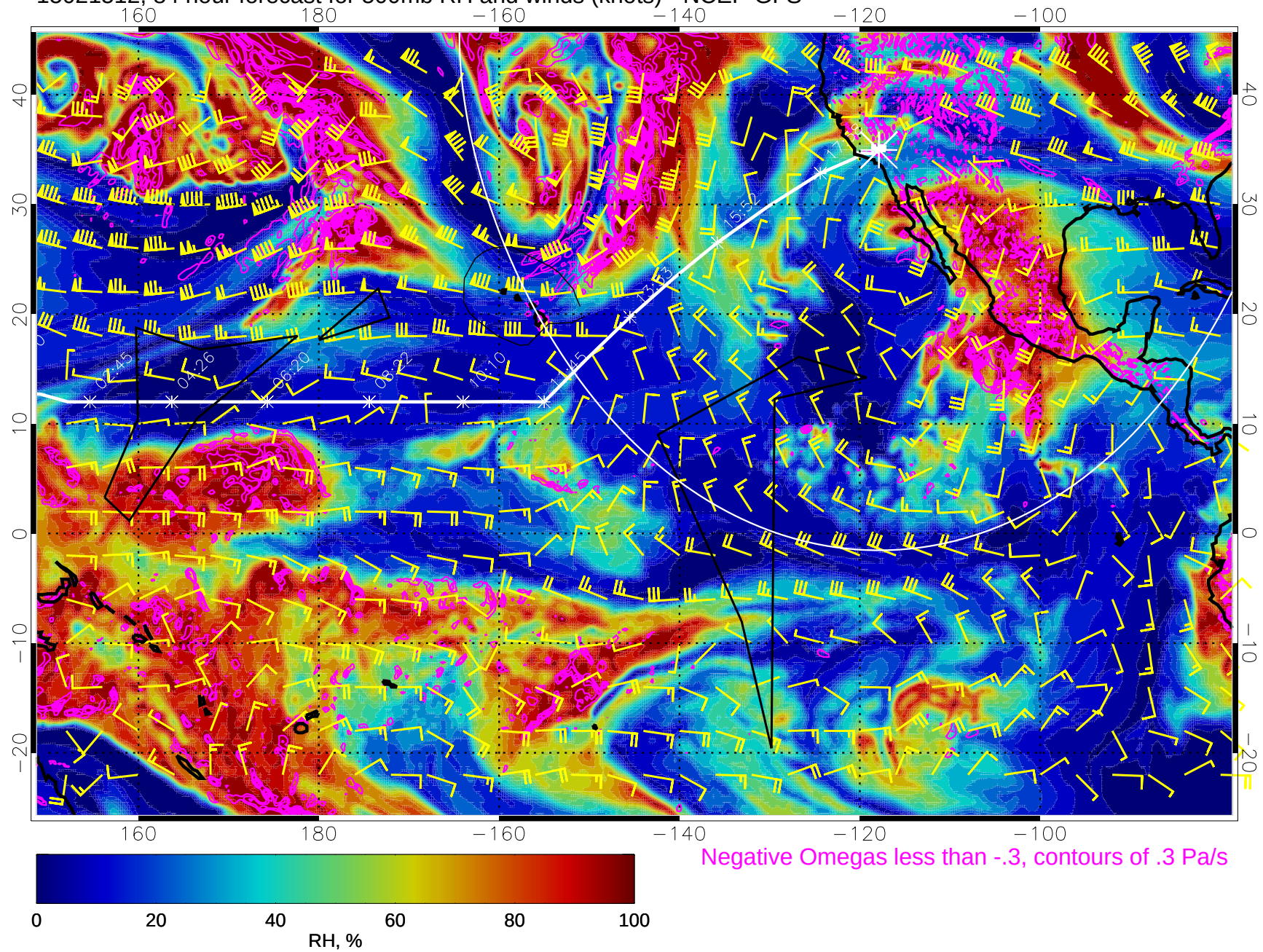
15021512, 84 hour forecast for 500mb RH and winds (knots) - NCEP GFS
