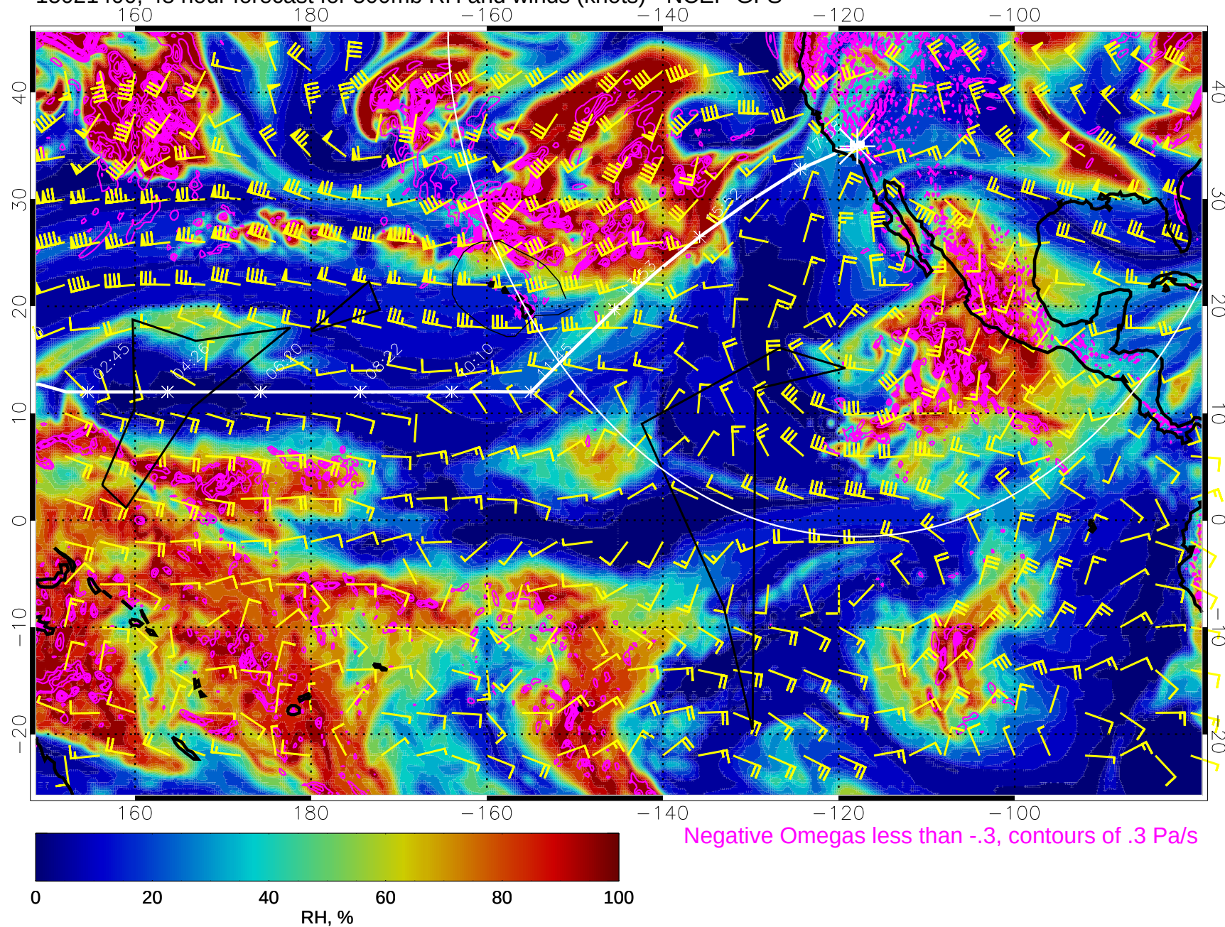
15021400, 48 hour forecast for 500mb RH and winds (knots) - NCEP GFS
