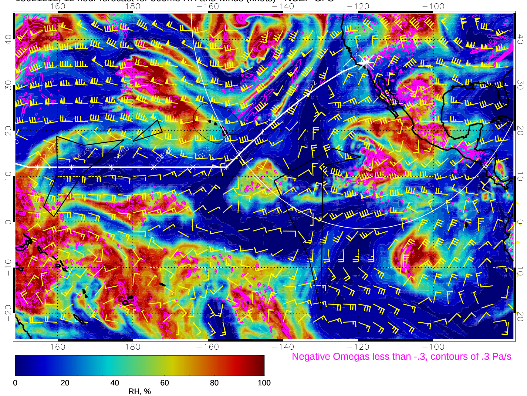
15021212, 12 hour forecast for 500mb RH and winds (knots) - NCEP GFS
