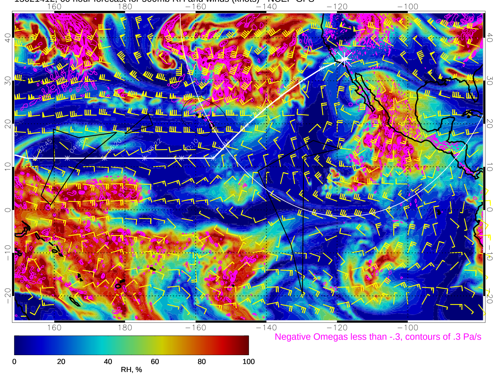
15021412, 60 hour forecast for 500mb RH and winds (knots) - NCEP GFS
