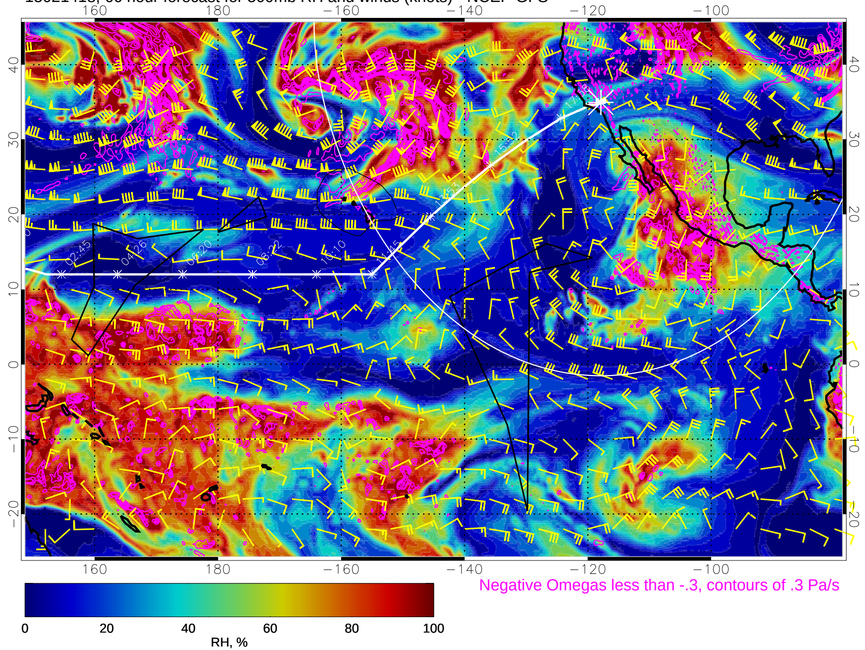
15021418, 66 hour forecast for 500mb RH and winds (knots) - NCEP GFS
