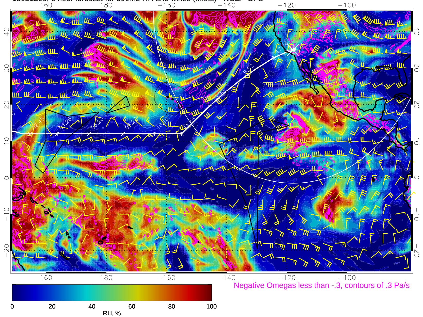
15021206, 6 hour forecast for 500mb RH and winds (knots) - NCEP GFS
