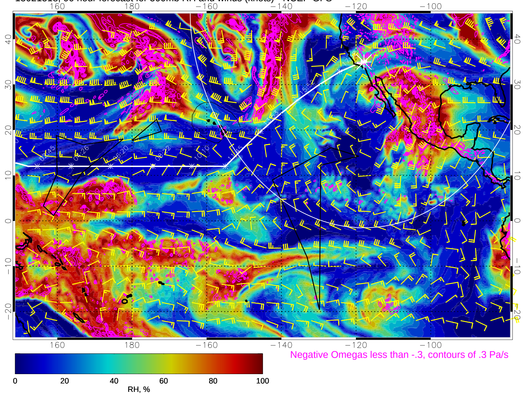
15021518, 90 hour forecast for 500mb RH and winds (knots) - NCEP GFS
