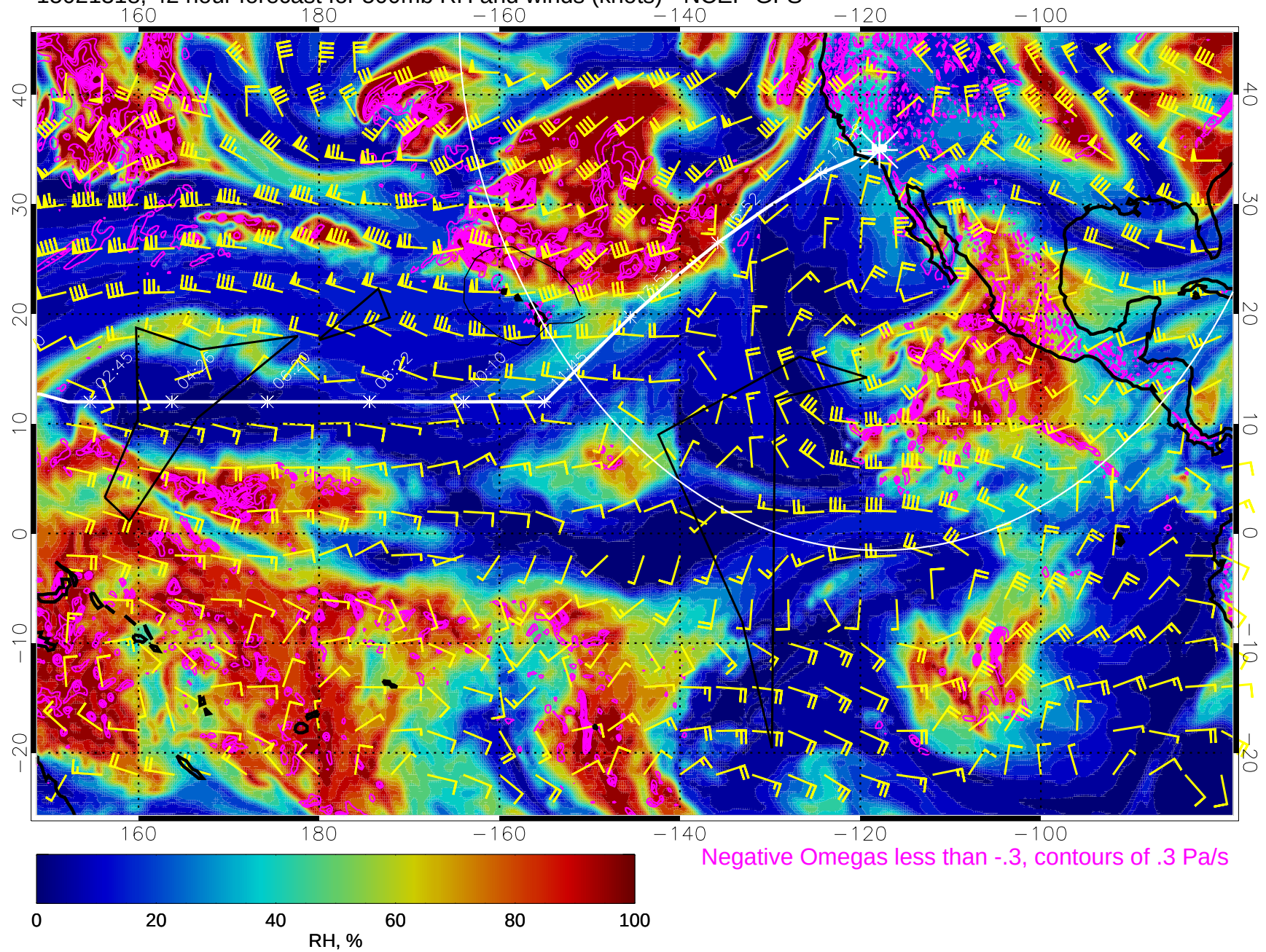
15021318, 42 hour forecast for 500mb RH and winds (knots) - NCEP GFS
