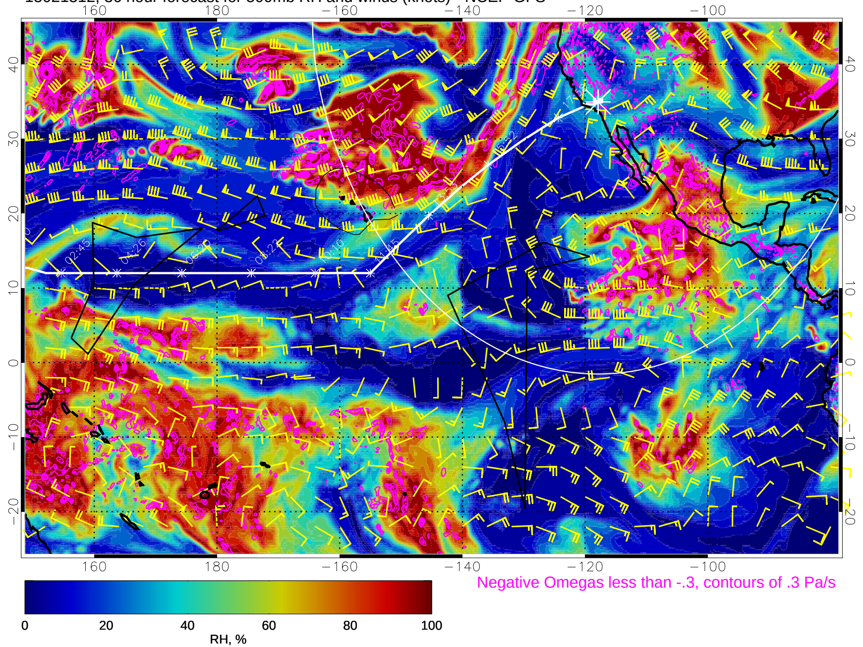
15021312, 36 hour forecast for 500mb RH and winds (knots) - NCEP GFS
