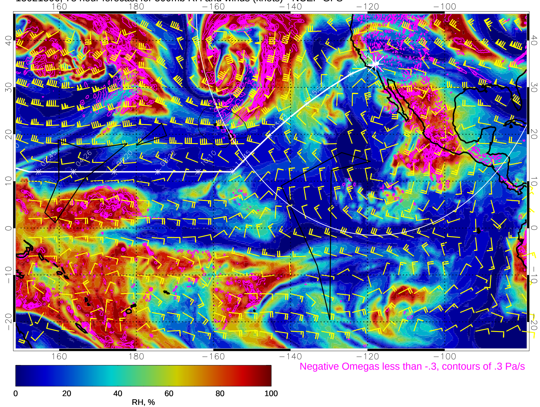
15021506, 78 hour forecast for 500mb RH and winds (knots) - NCEP GFS
