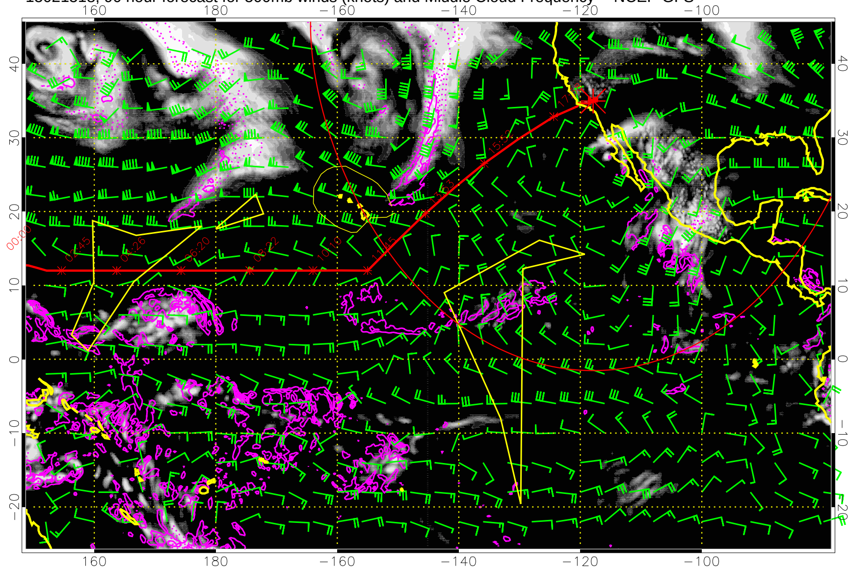
15021518, 90 hour forecast for 500mb winds (knots) and Middle Cloud Frequency -- NCEP GFS
