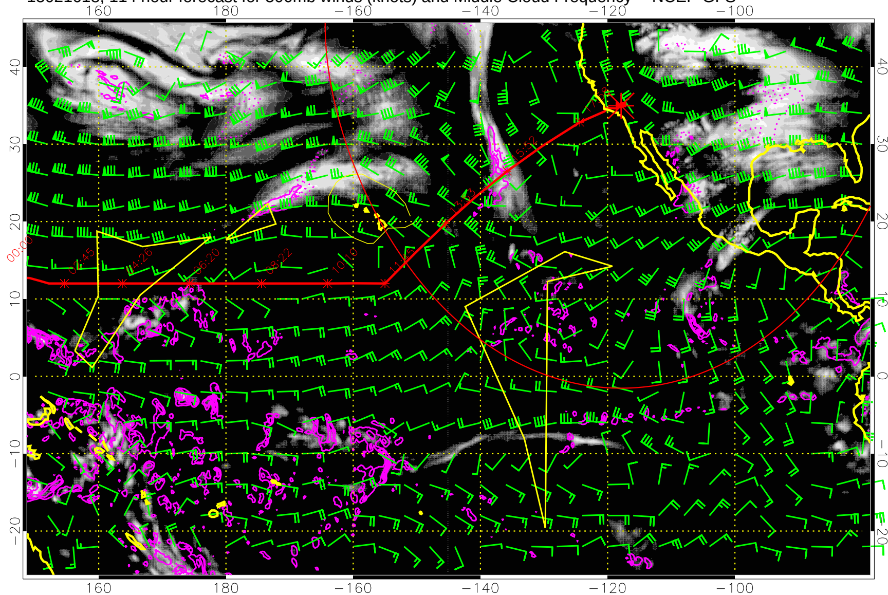
15021618, 114 hour forecast for 500mb winds (knots) and Middle Cloud Frequency -- NCEP GFS
