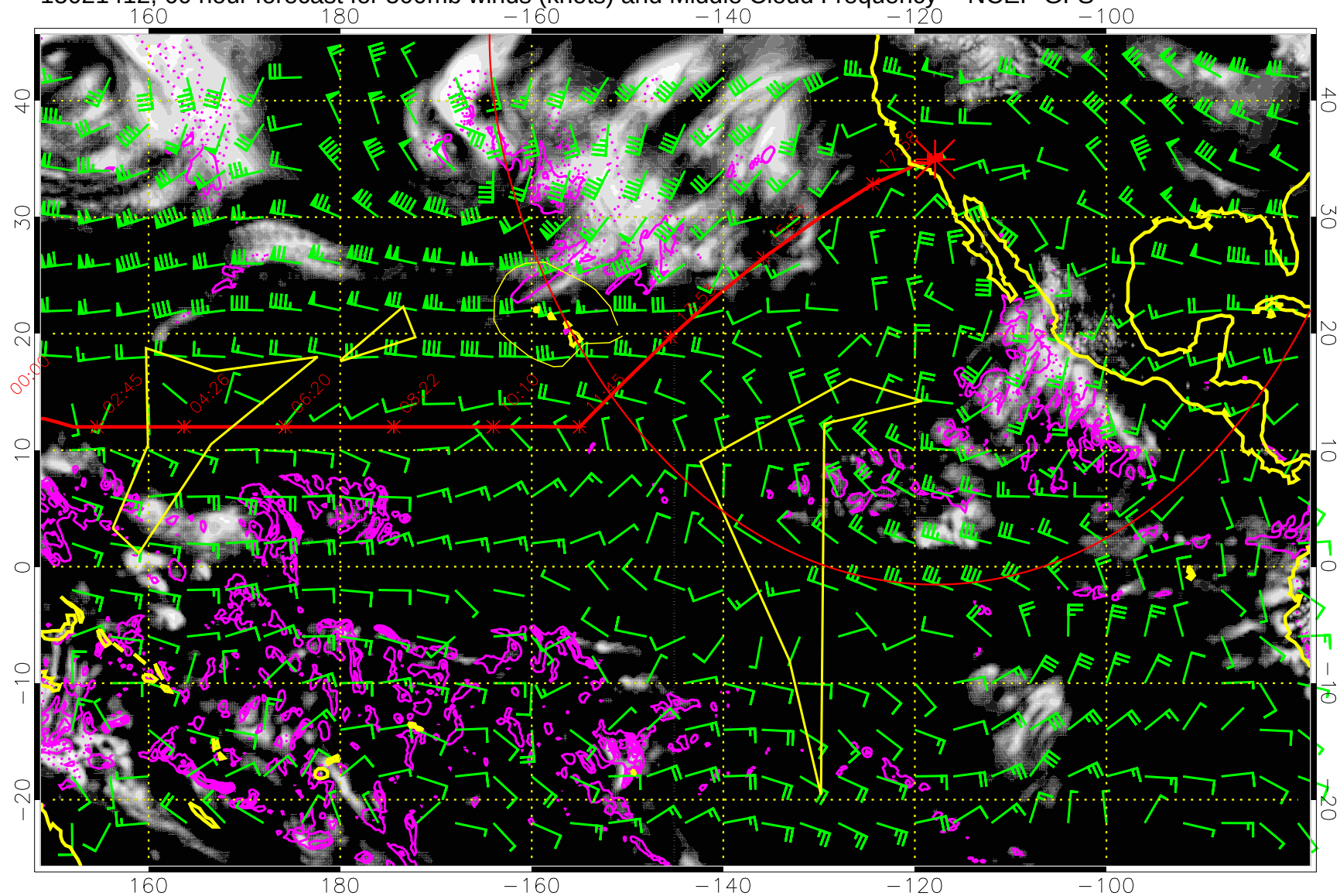
15021412, 60 hour forecast for 500mb winds (knots) and Middle Cloud Frequency -- NCEP GFS
