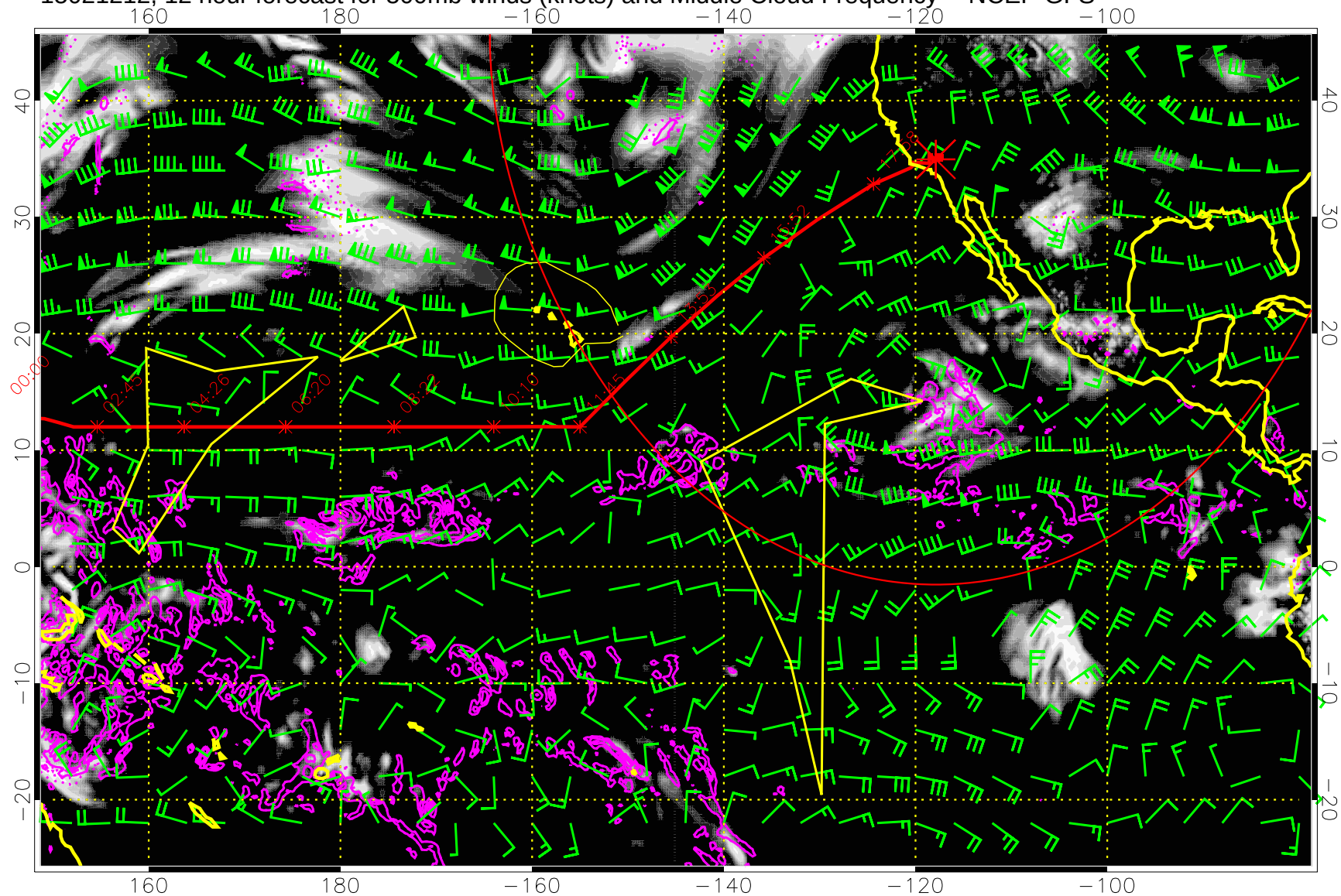
15021212, 12 hour forecast for 500mb winds (knots) and Middle Cloud Frequency -- NCEP GFS
