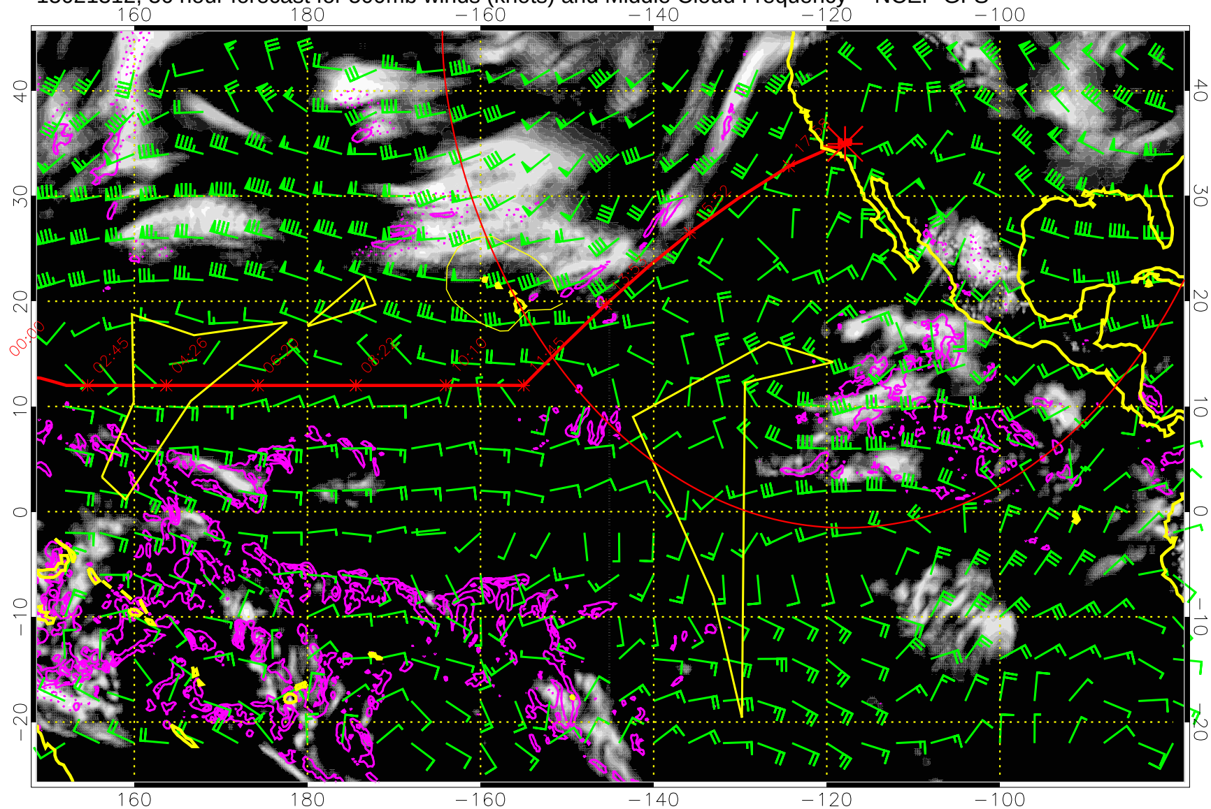
15021312, 36 hour forecast for 500mb winds (knots) and Middle Cloud Frequency -- NCEP GFS
