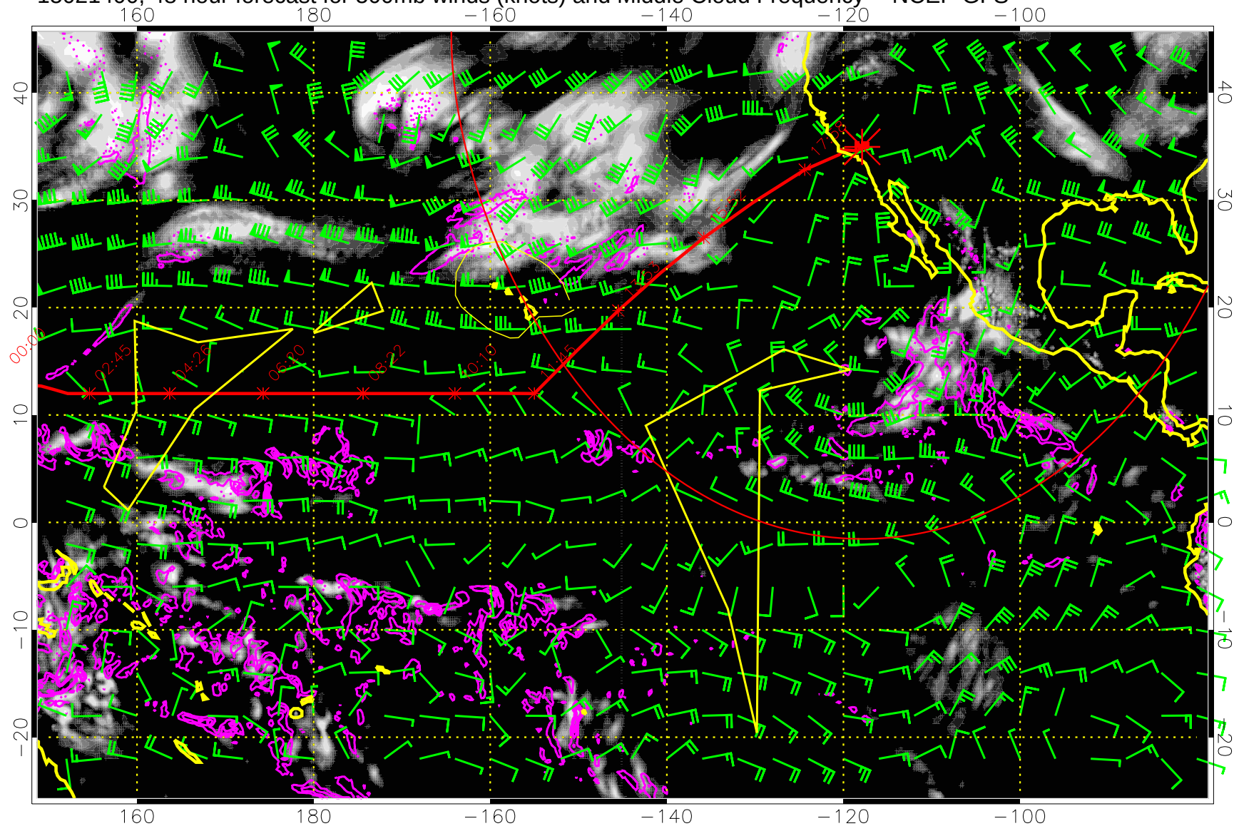
15021400, 48 hour forecast for 500mb winds (knots) and Middle Cloud Frequency -- NCEP GFS
