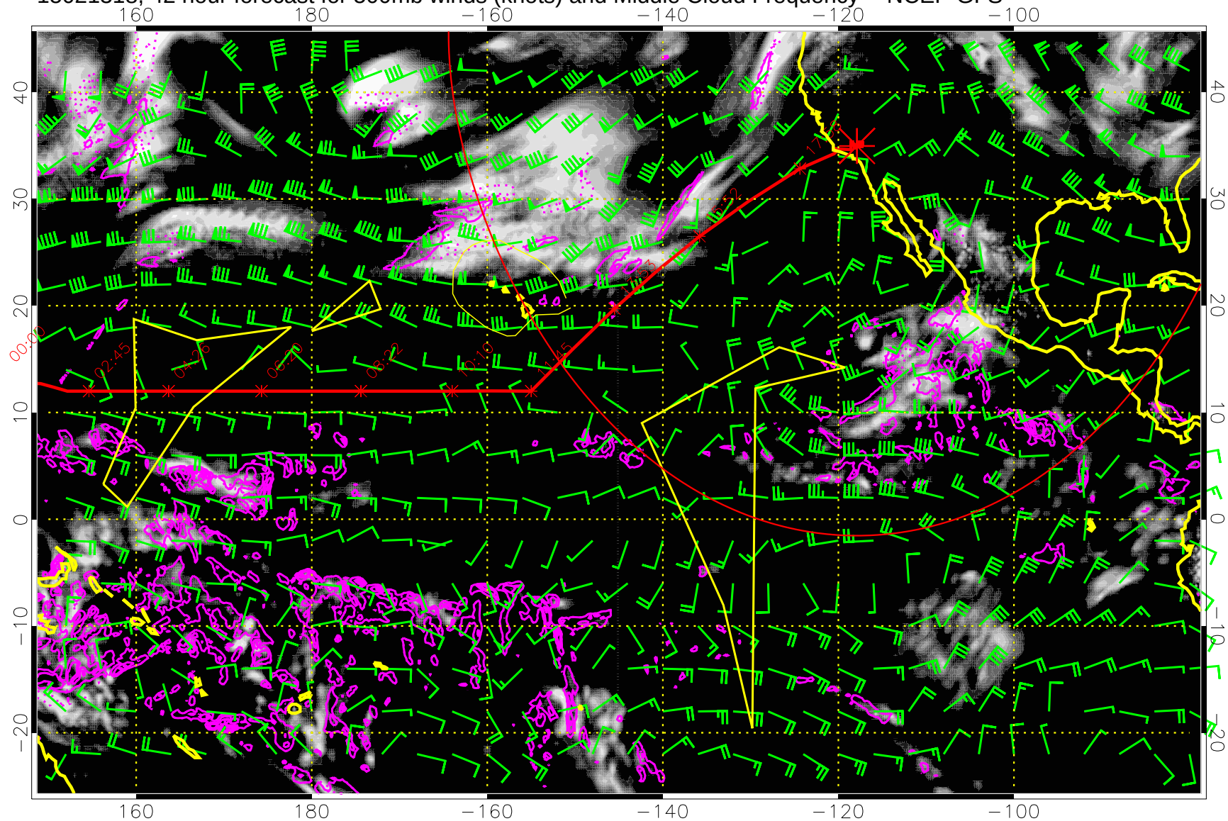
15021318, 42 hour forecast for 500mb winds (knots) and Middle Cloud Frequency -- NCEP GFS
