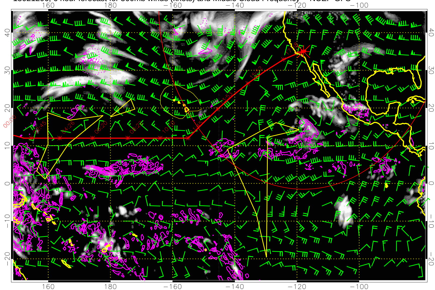
15021206, 6 hour forecast for 500mb winds (knots) and Middle Cloud Frequency -- NCEP GFS
