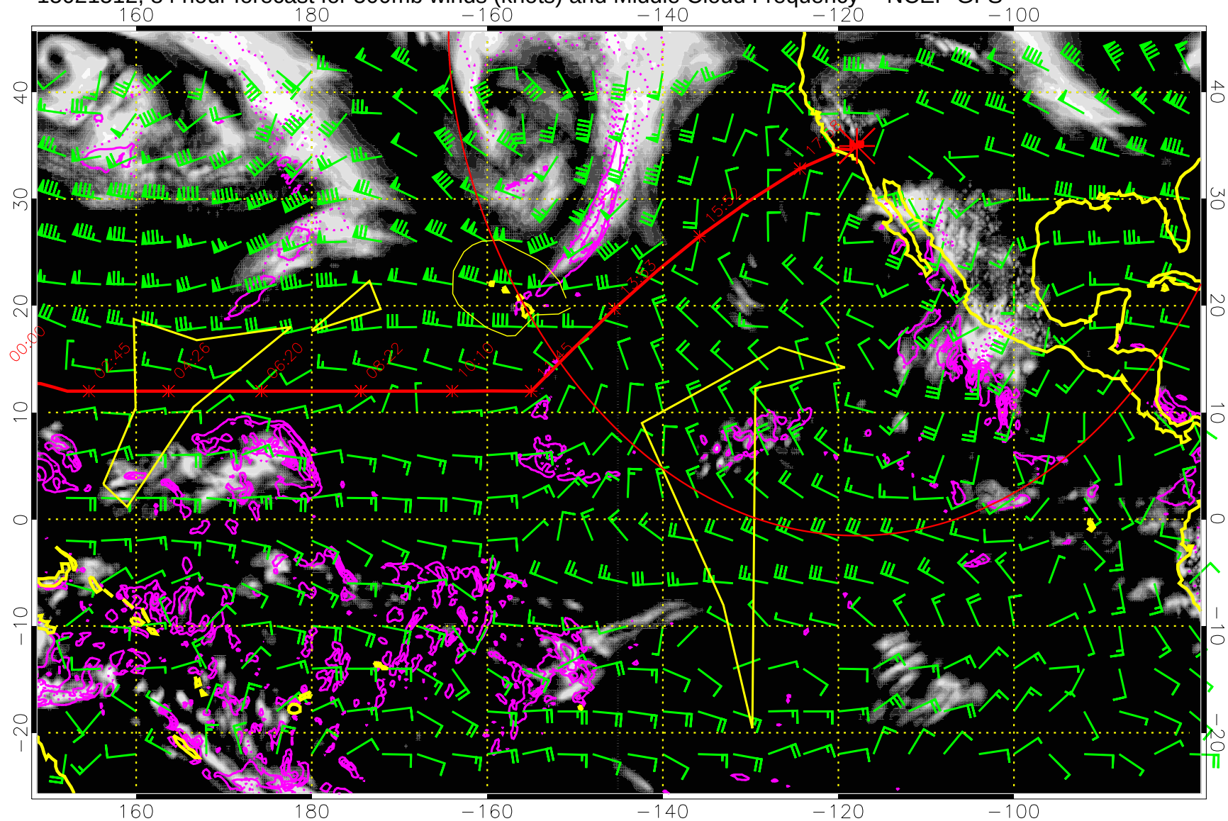
15021512, 84 hour forecast for 500mb winds (knots) and Middle Cloud Frequency -- NCEP GFS
