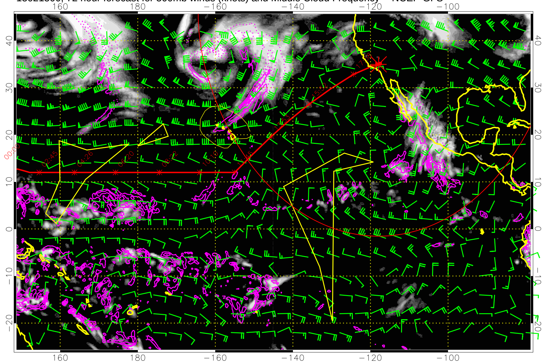
15021500, 72 hour forecast for 500mb winds (knots) and Middle Cloud Frequency -- NCEP GFS
