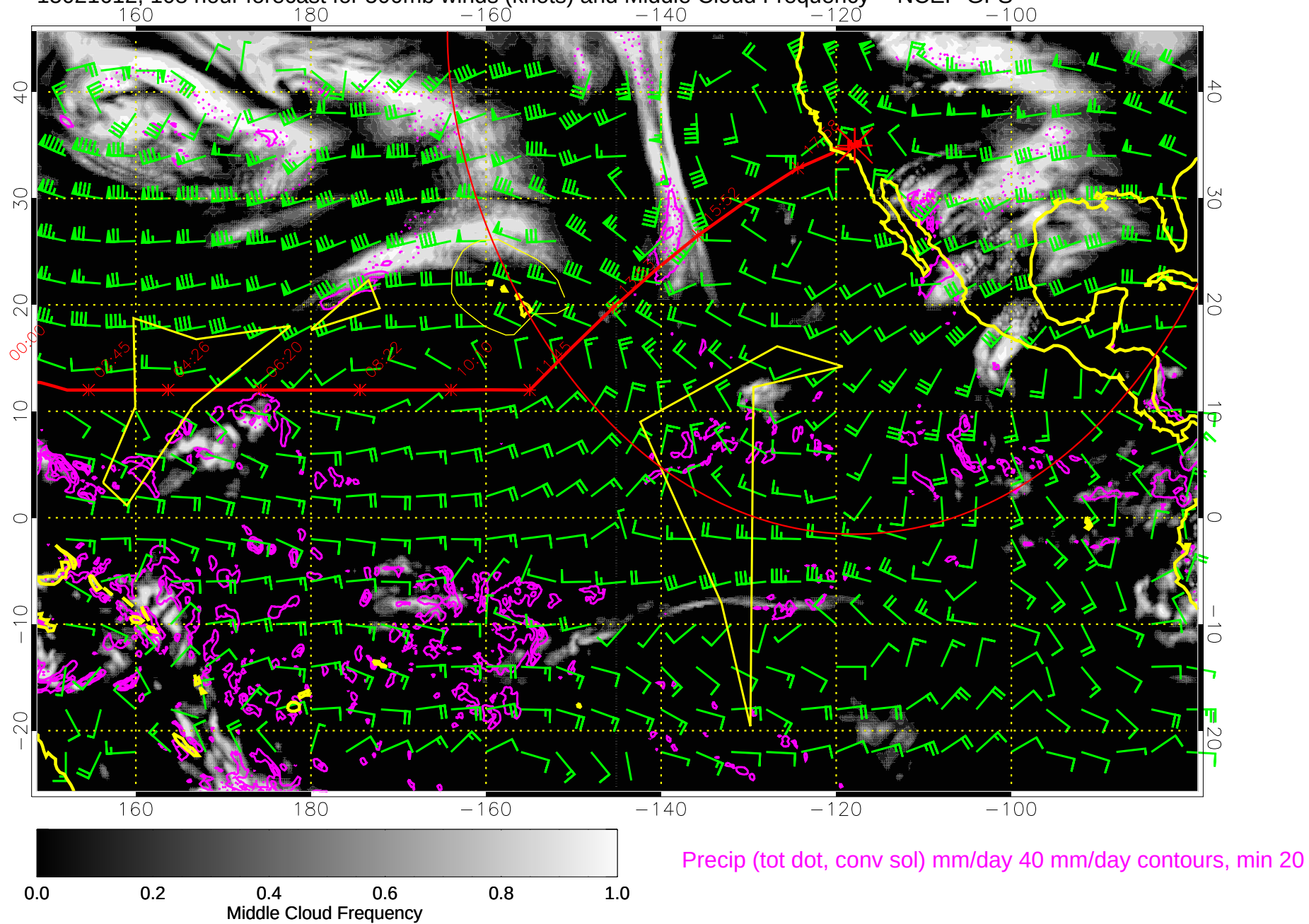
15021612, 108 hour forecast for 500mb winds (knots) and Middle Cloud Frequency -- NCEP GFS
