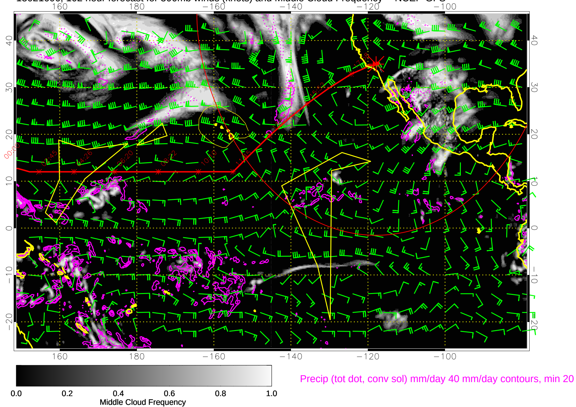
15021606, 102 hour forecast for 500mb winds (knots) and Middle Cloud Frequency -- NCEP GFS
