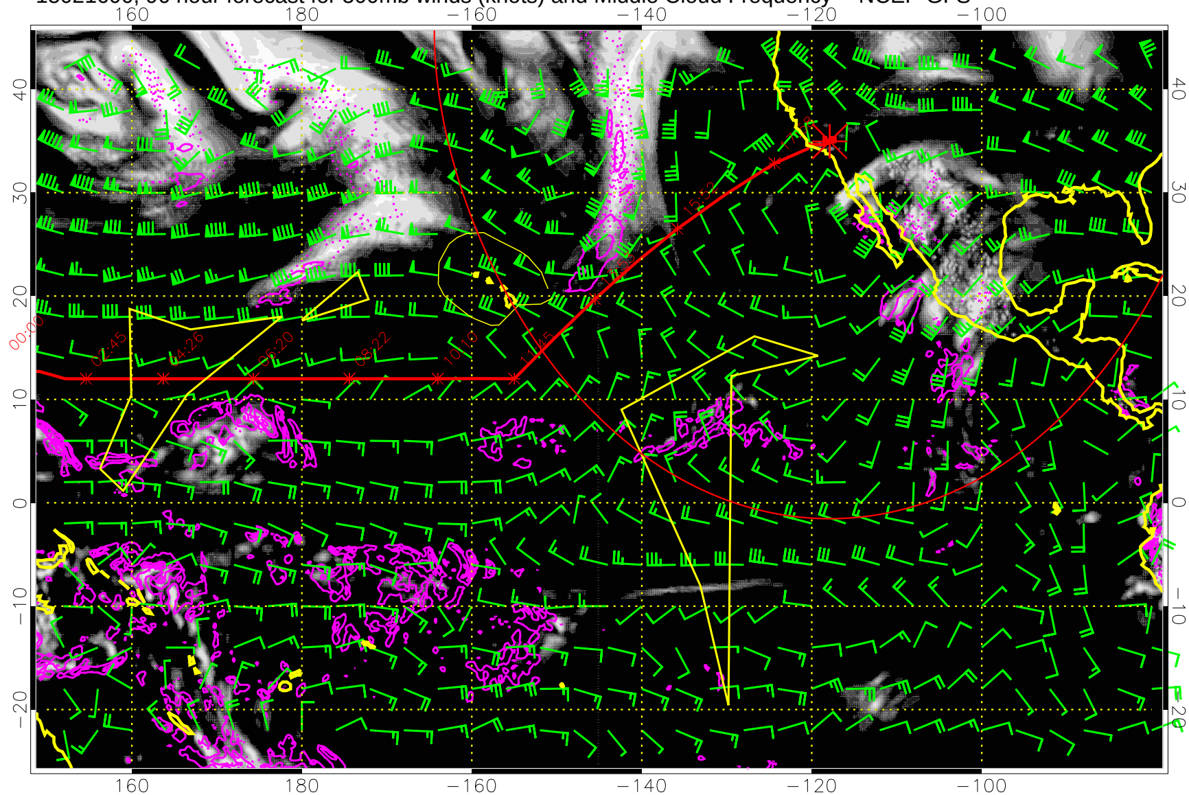
15021600, 96 hour forecast for 500mb winds (knots) and Middle Cloud Frequency -- NCEP GFS
