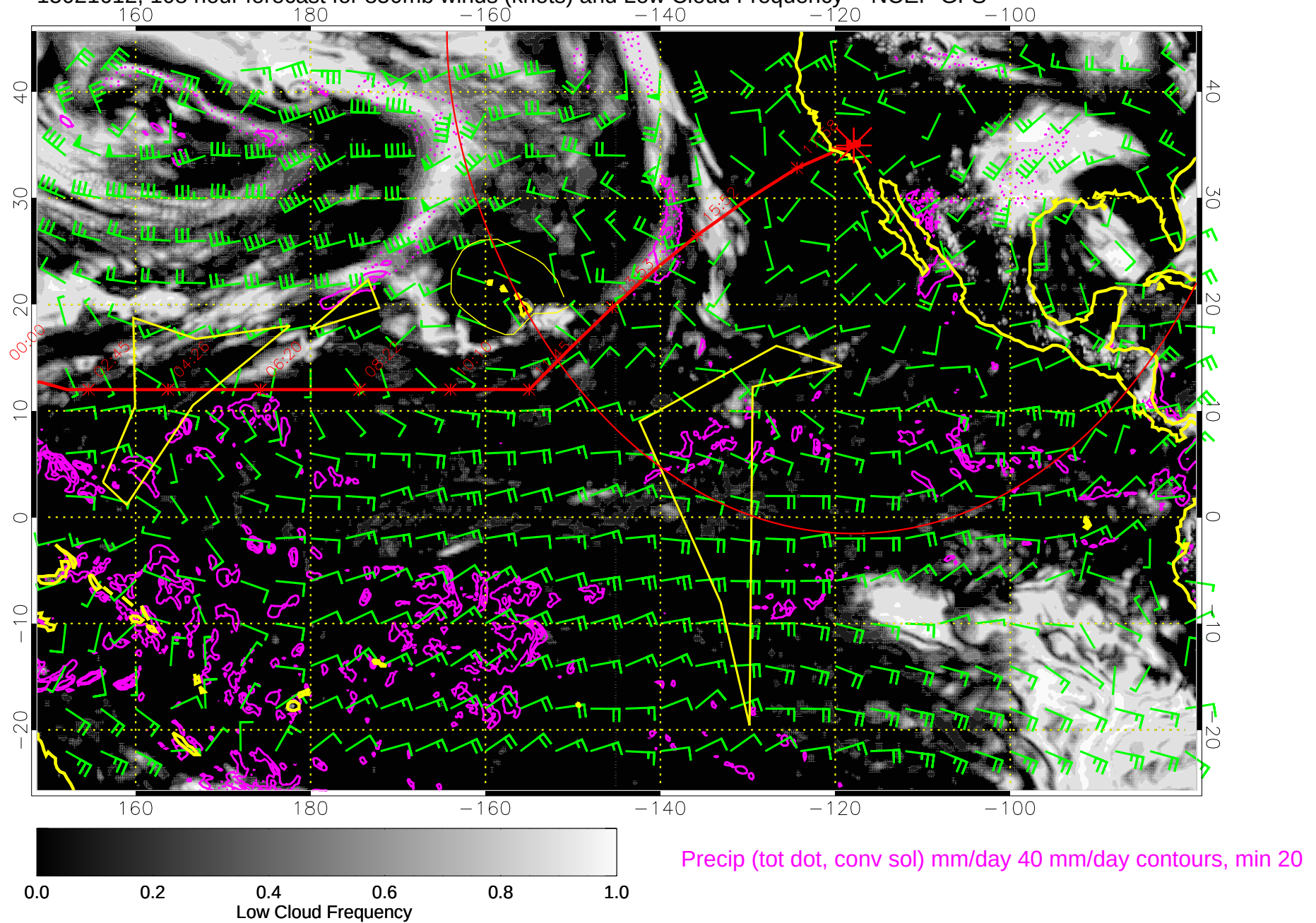
15021612, 108 hour forecast for 850mb winds (knots) and Low Cloud Frequency -- NCEP GFS
