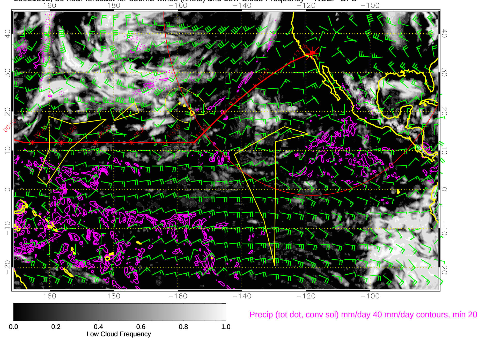
15021312, 36 hour forecast for 850mb winds (knots) and Low Cloud Frequency -- NCEP GFS
