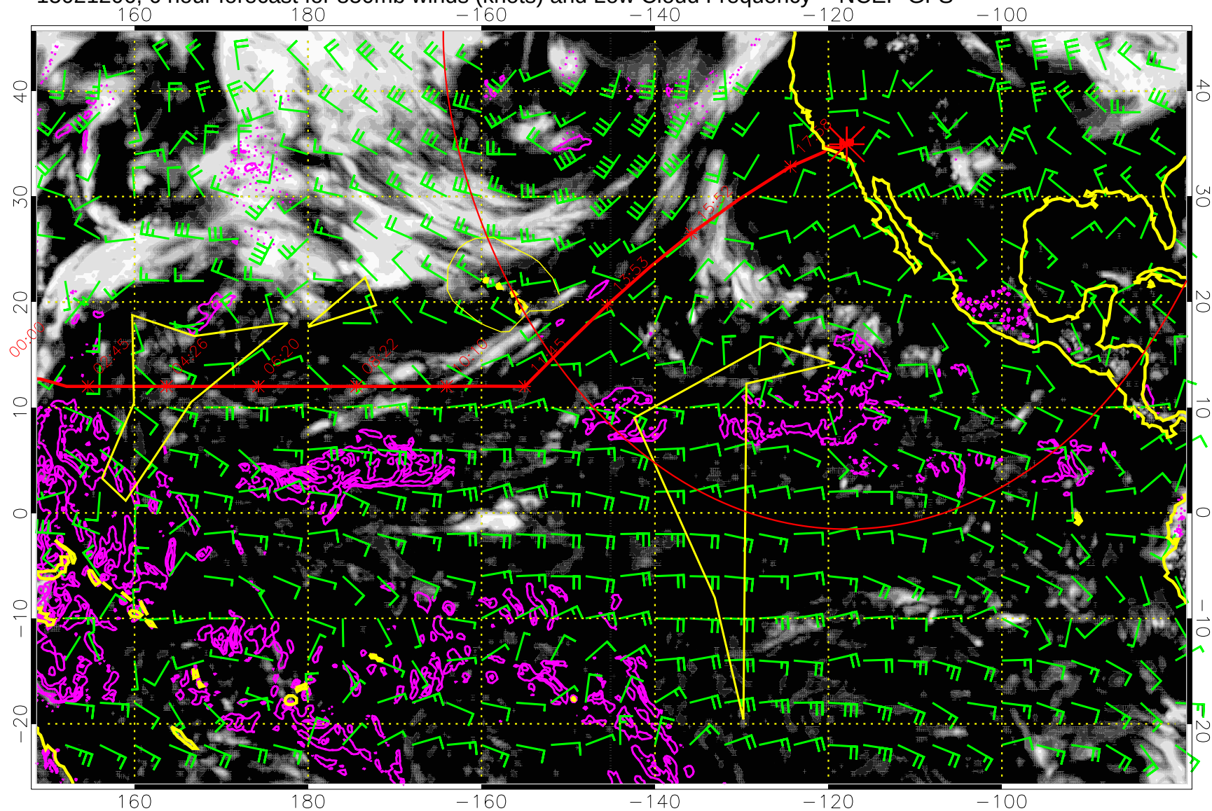
15021206, 6 hour forecast for 850mb winds (knots) and Low Cloud Frequency -- NCEP GFS
