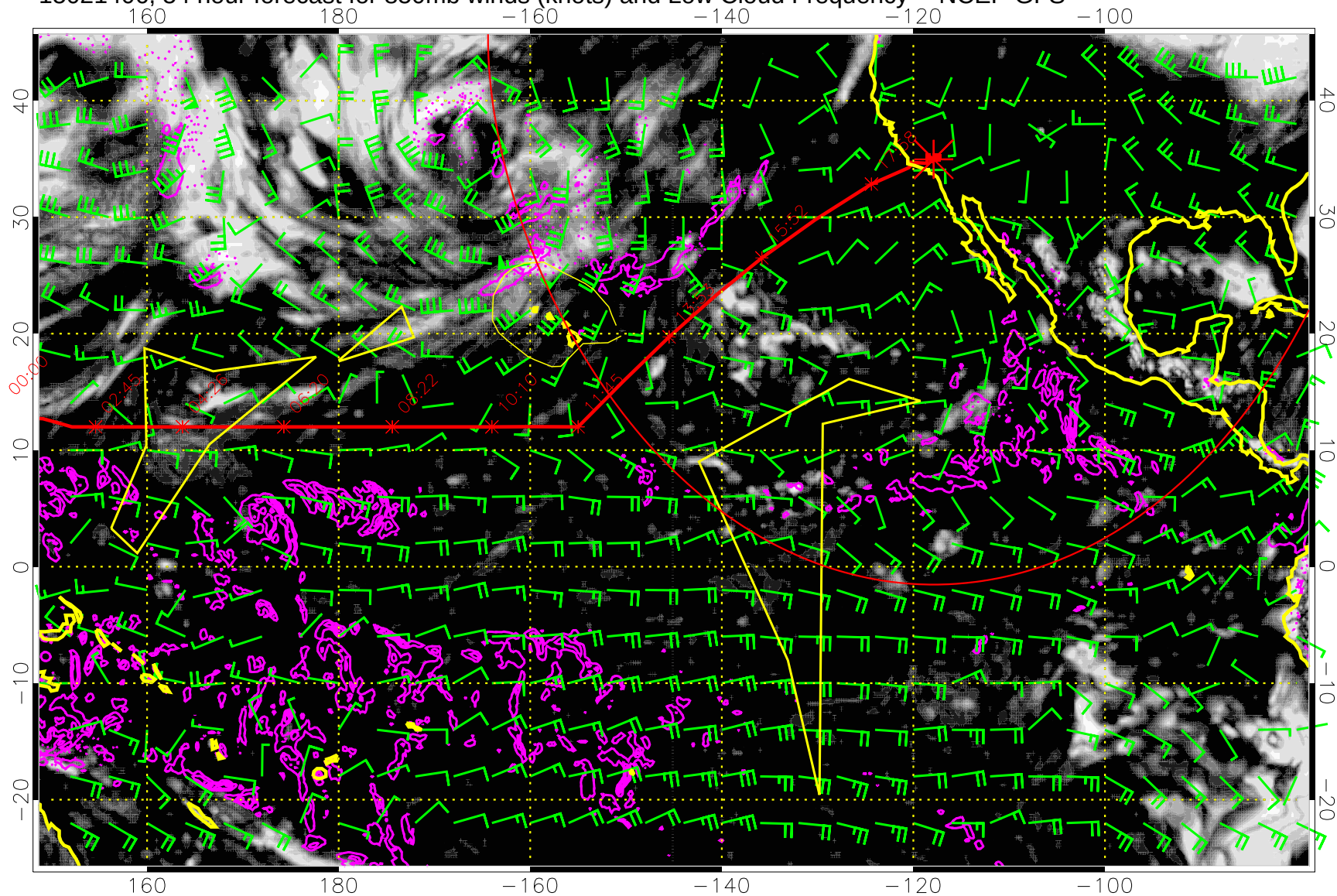
15021406, 54 hour forecast for 850mb winds (knots) and Low Cloud Frequency -- NCEP GFS
