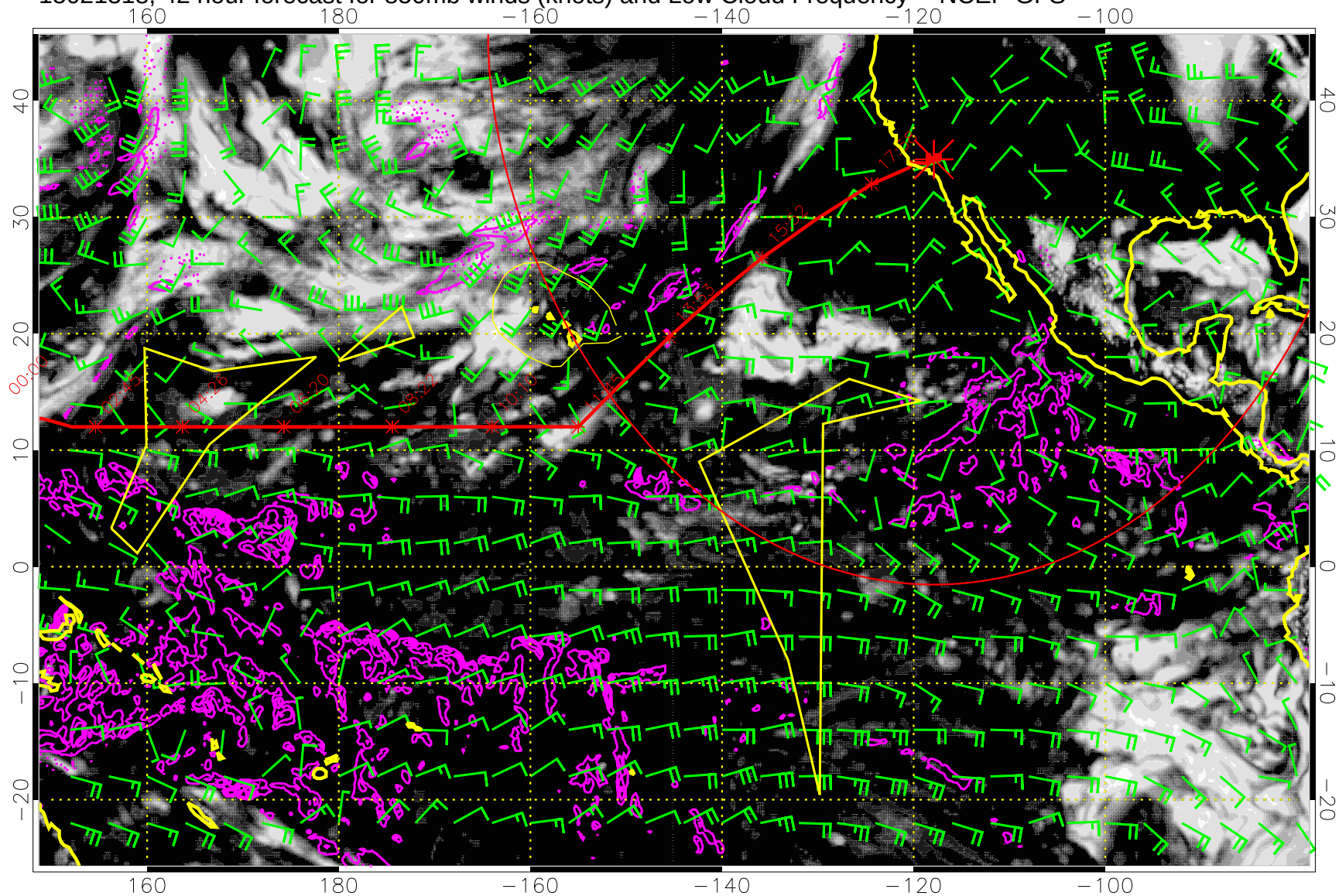
15021318, 42 hour forecast for 850mb winds (knots) and Low Cloud Frequency -- NCEP GFS
