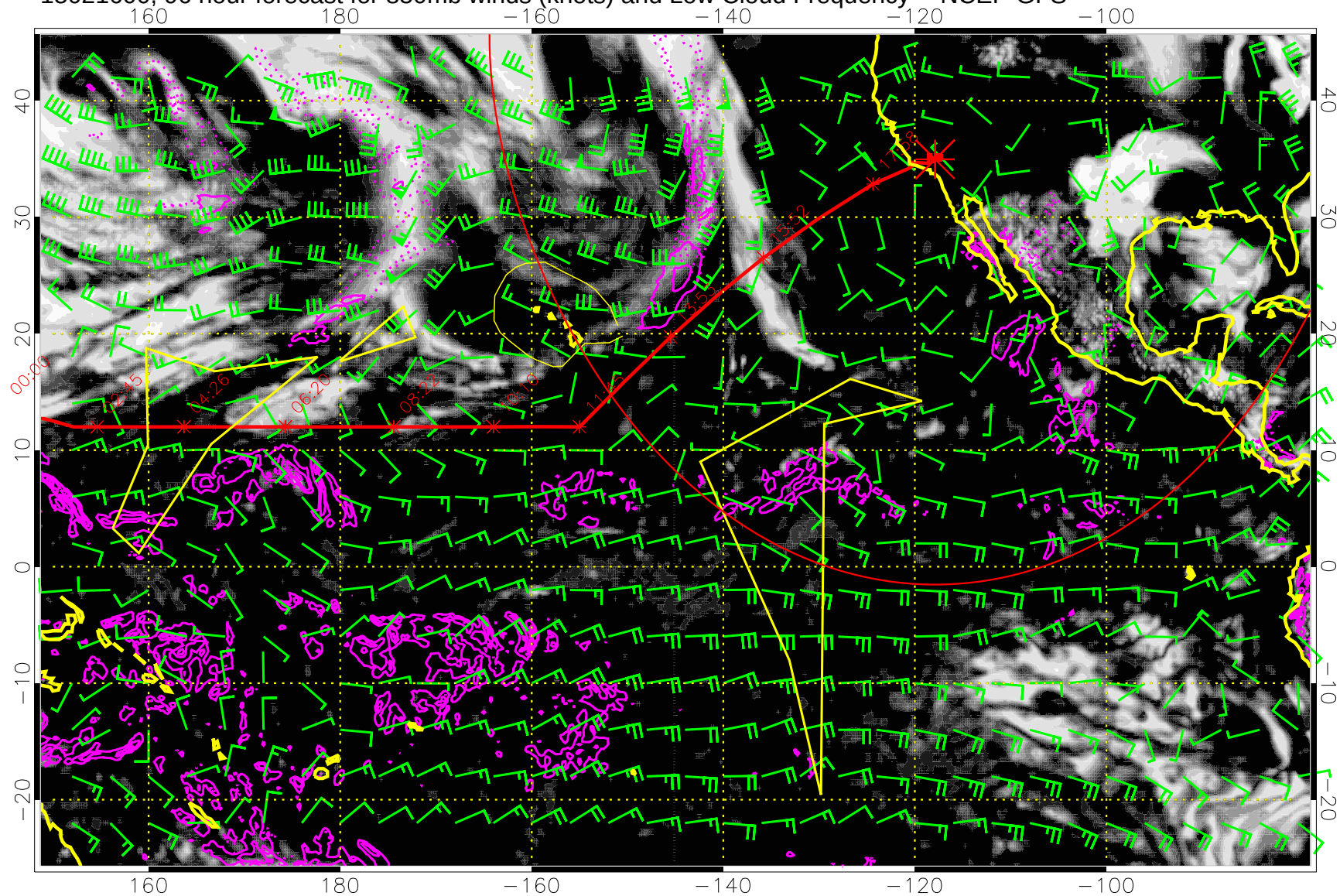
15021600, 96 hour forecast for 850mb winds (knots) and Low Cloud Frequency -- NCEP GFS
