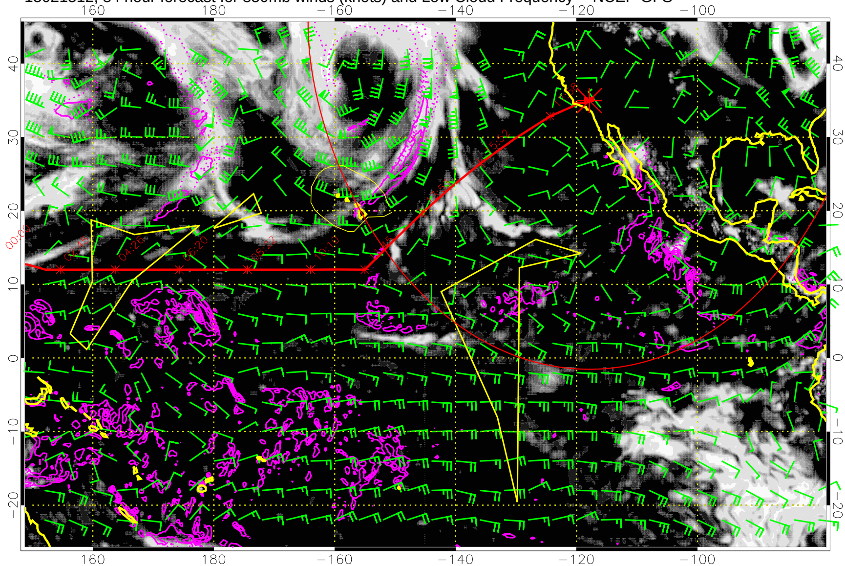
15021512, 84 hour forecast for 850mb winds (knots) and Low Cloud Frequency -- NCEP GFS
