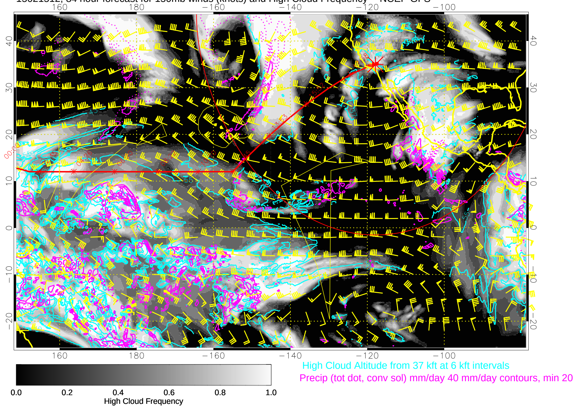
15021512, 84 hour forecast for 150mb winds (knots) and High Cloud Frequency -- NCEP GFS
