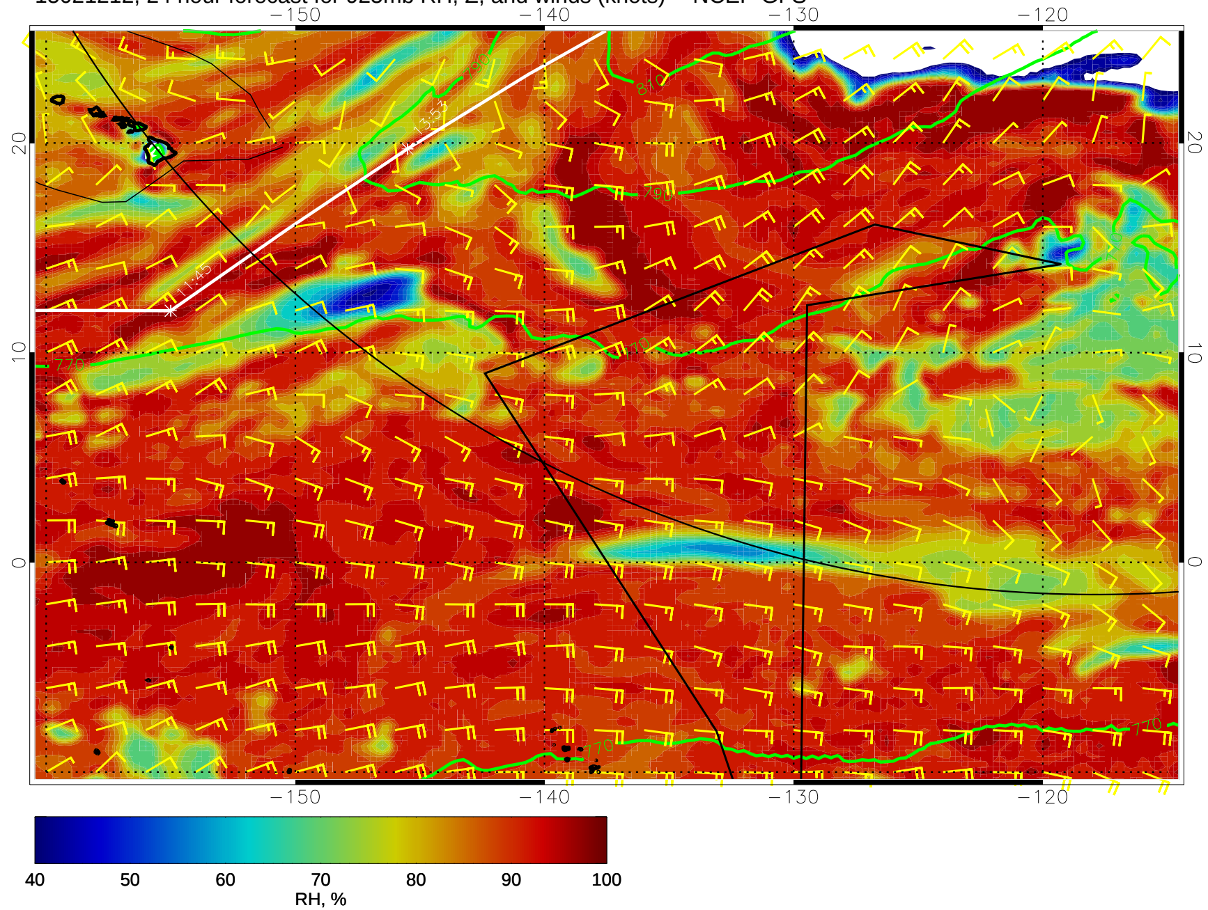
15021212, 24 hour forecast for 925mb RH, Z, and winds (knots) -- NCEP GFS
