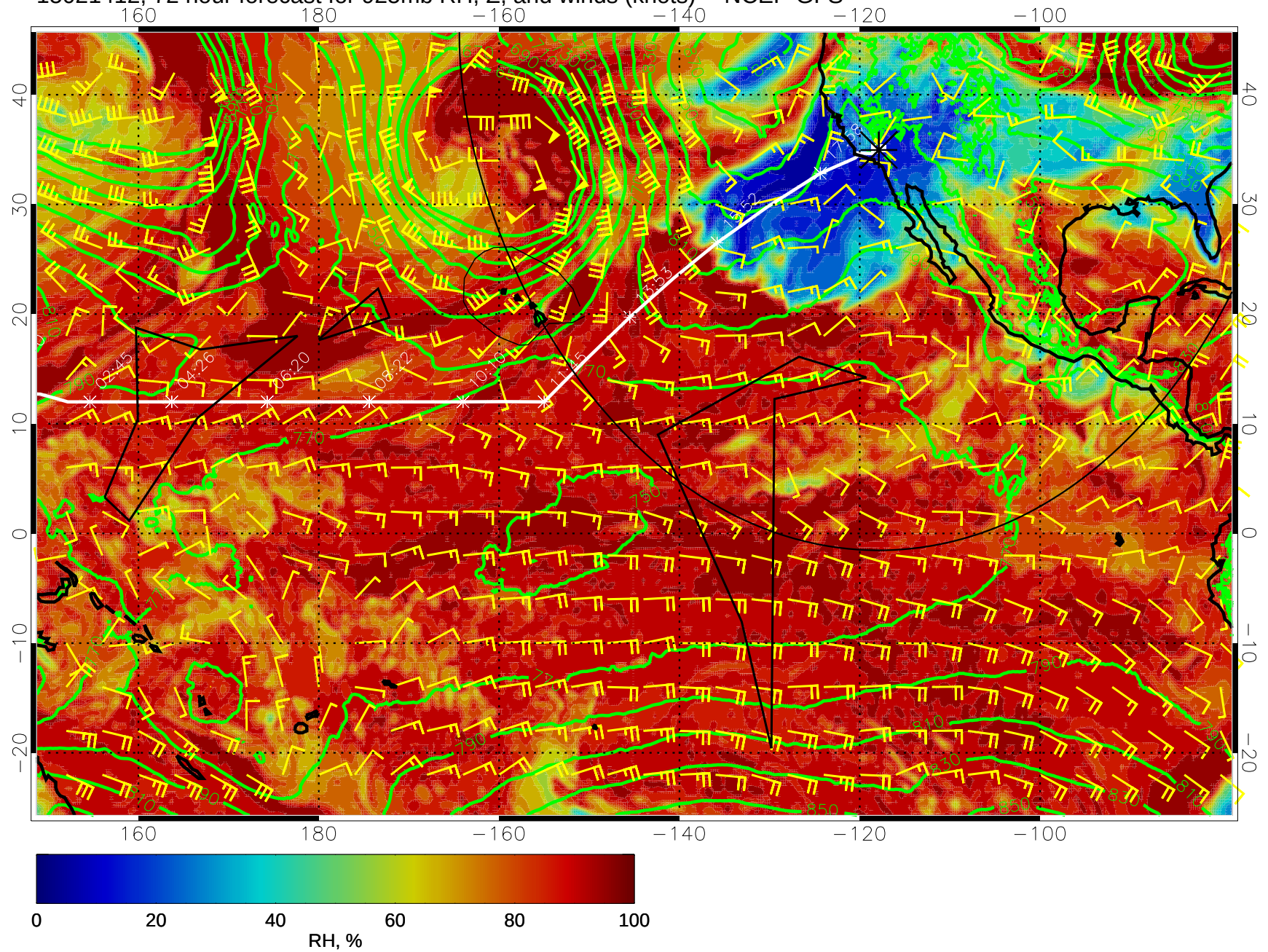
15021412, 72 hour forecast for 925mb RH, Z, and winds (knots) -- NCEP GFS
