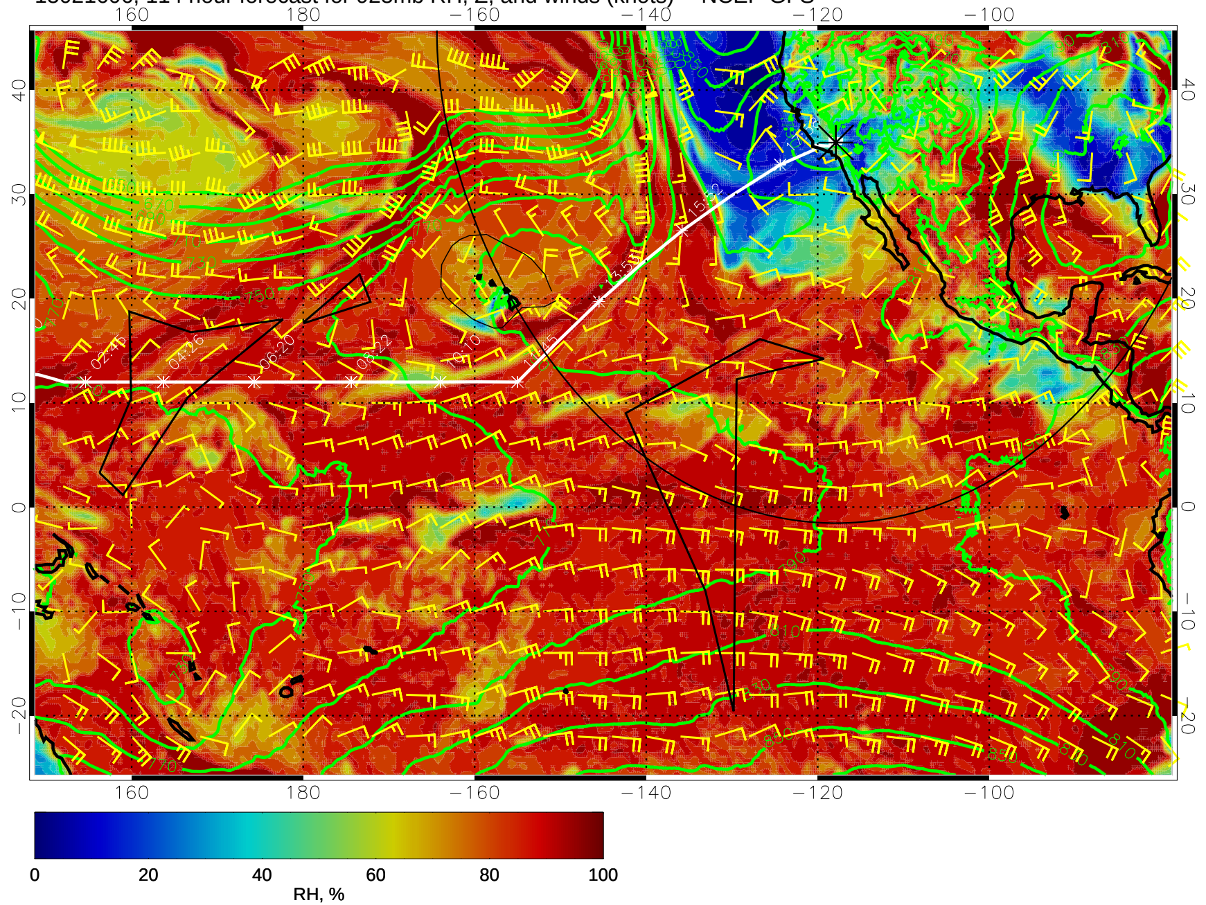
15021606, 114 hour forecast for 925mb RH, Z, and winds (knots) -- NCEP GFS
