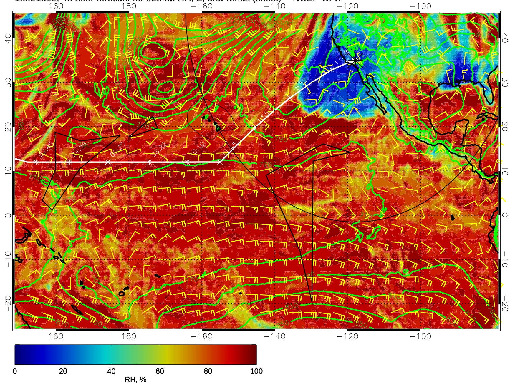
15021312, 48 hour forecast for 925mb RH, Z, and winds (knots) -- NCEP GFS
