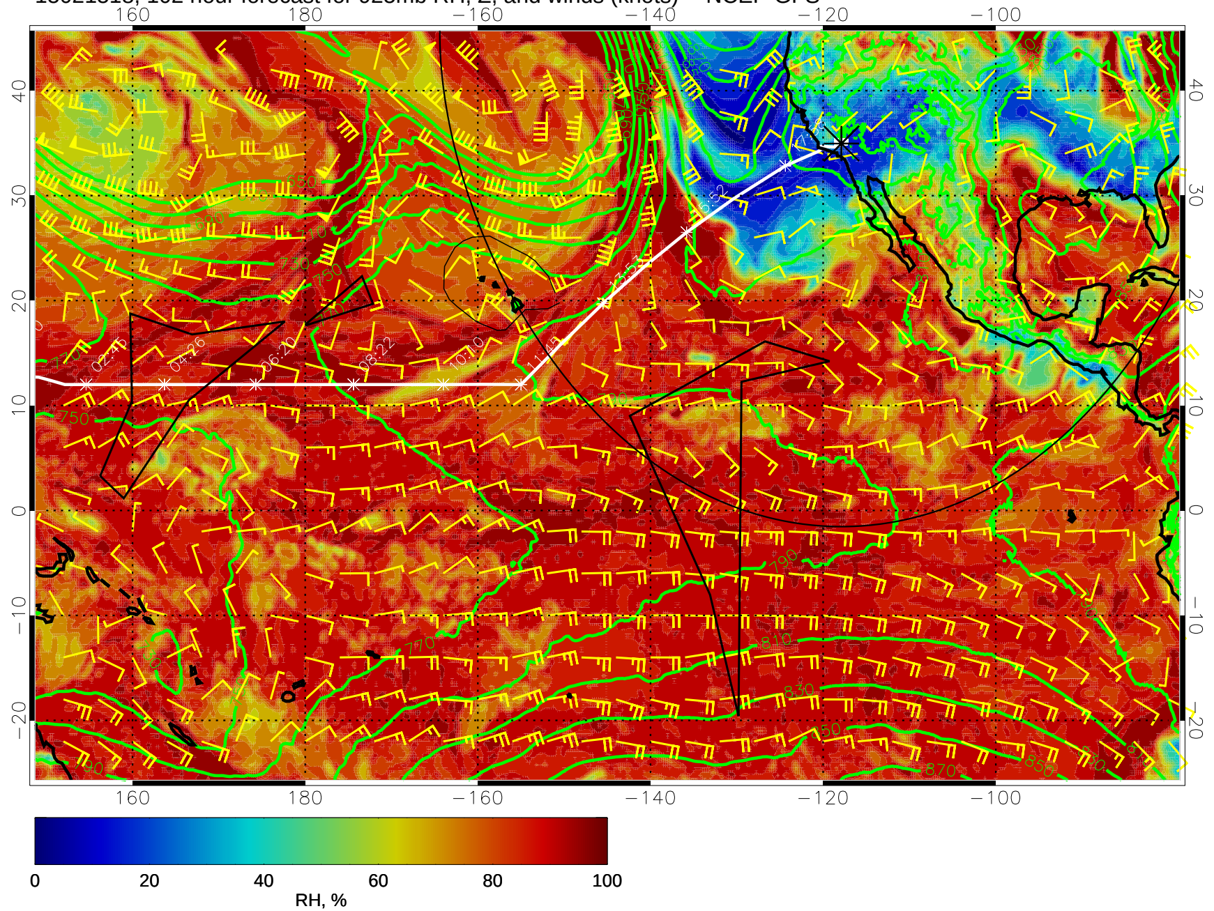
15021518, 102 hour forecast for 925mb RH, Z, and winds (knots) -- NCEP GFS
