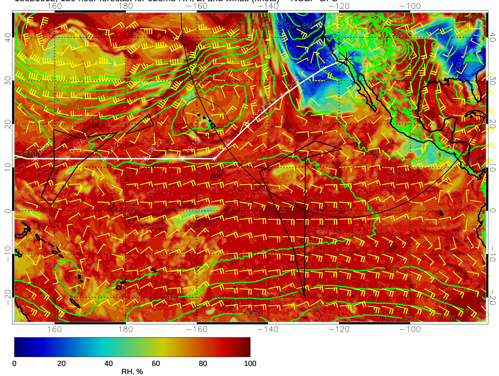
15021612, 120 hour forecast for 925mb RH, Z, and winds (knots) -- NCEP GFS
