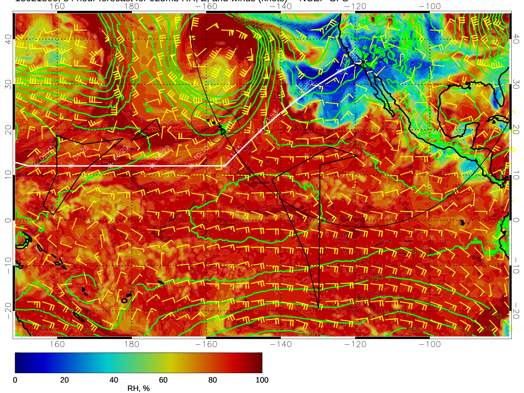
15021500, 84 hour forecast for 925mb RH, Z, and winds (knots) -- NCEP GFS
