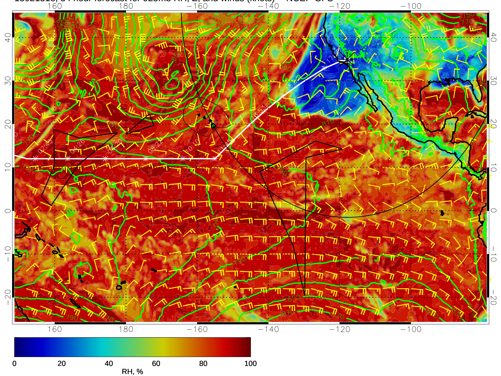
15021318, 54 hour forecast for 925mb RH, Z, and winds (knots) -- NCEP GFS
