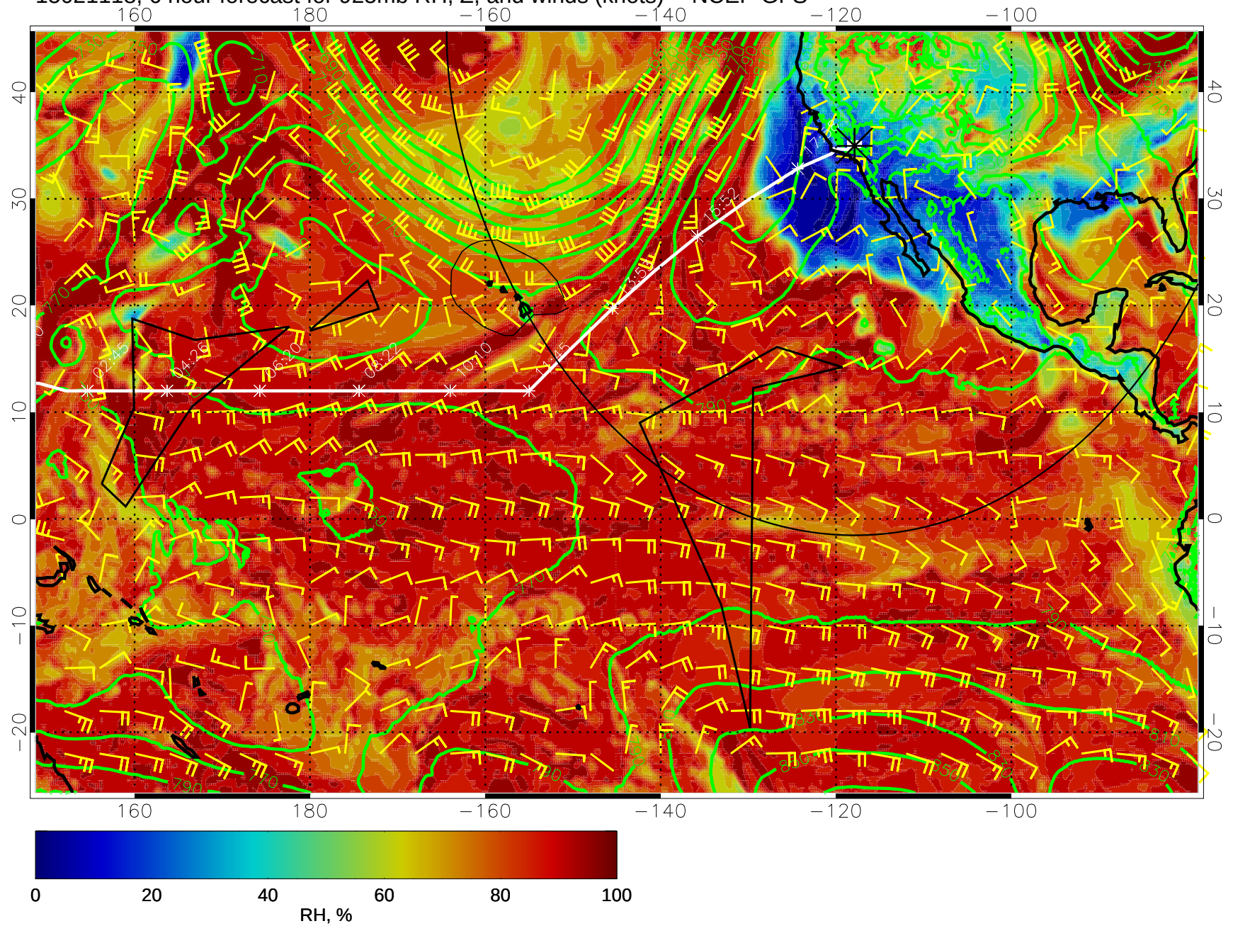
15021118, 6 hour forecast for 925mb RH, Z, and winds (knots) -- NCEP GFS
