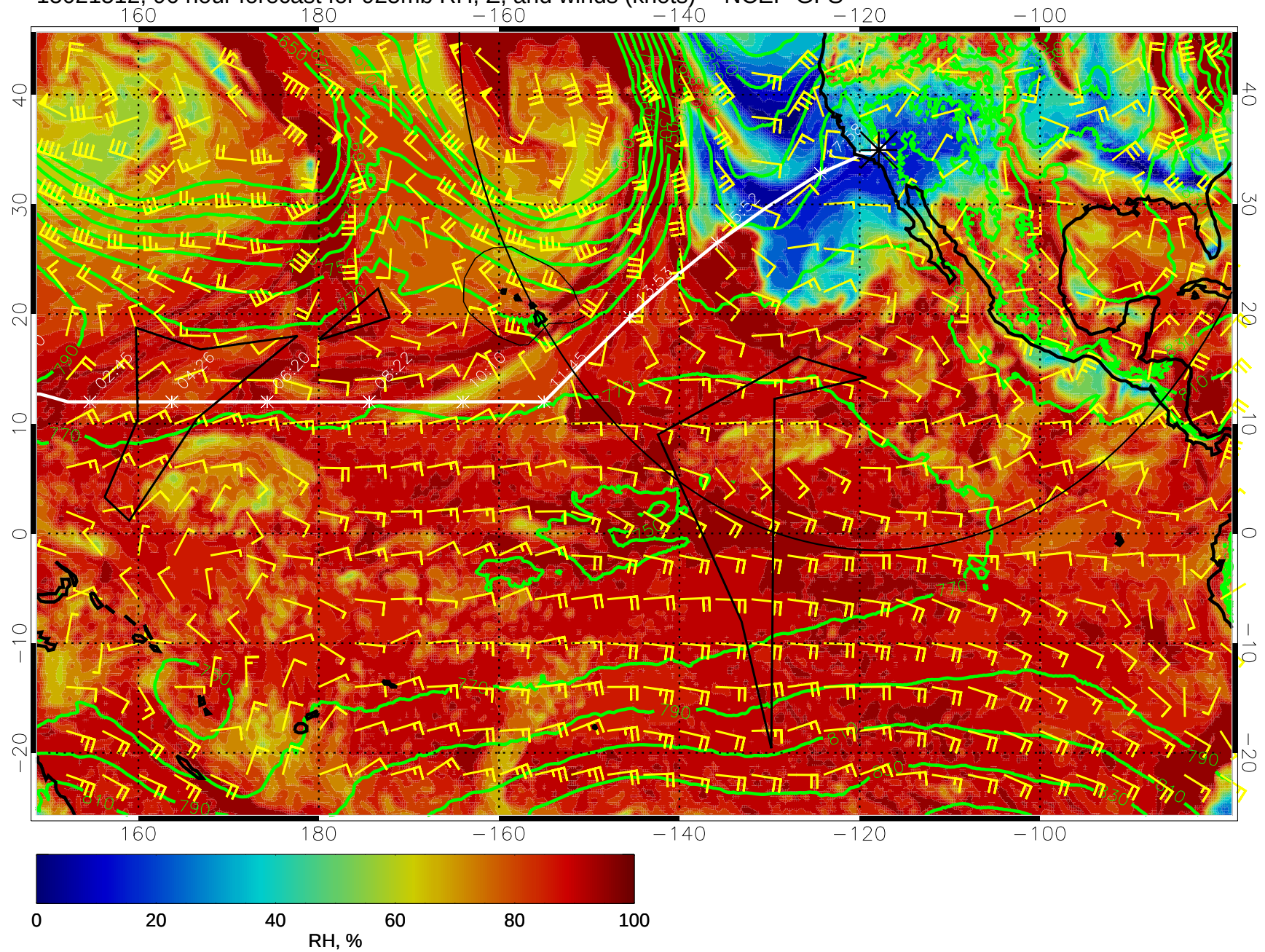
15021512, 96 hour forecast for 925mb RH, Z, and winds (knots) -- NCEP GFS
