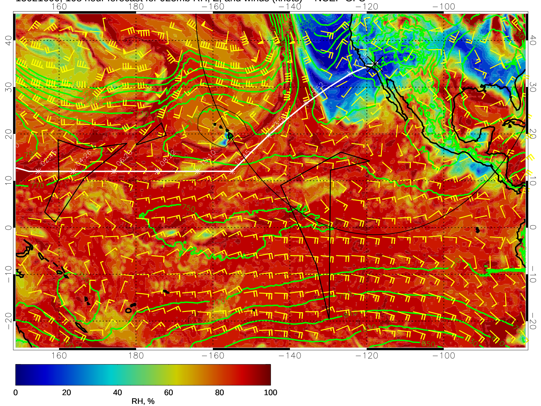
15021600, 108 hour forecast for 925mb RH, Z, and winds (knots) -- NCEP GFS
