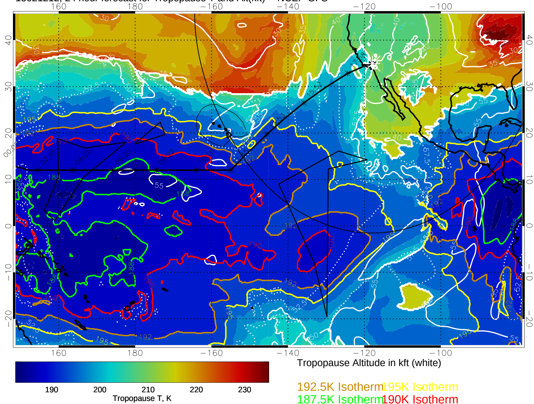
15021212, 24 hour forecast for Tropopause T and Alt(kft) -- NCEP GFS
