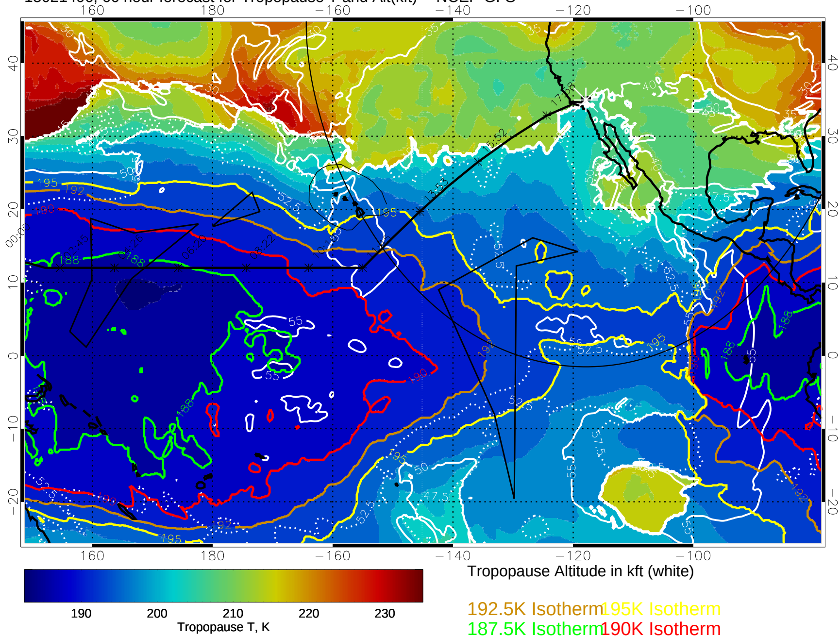
15021406, 66 hour forecast for Tropopause T and Alt(kft) -- NCEP GFS
