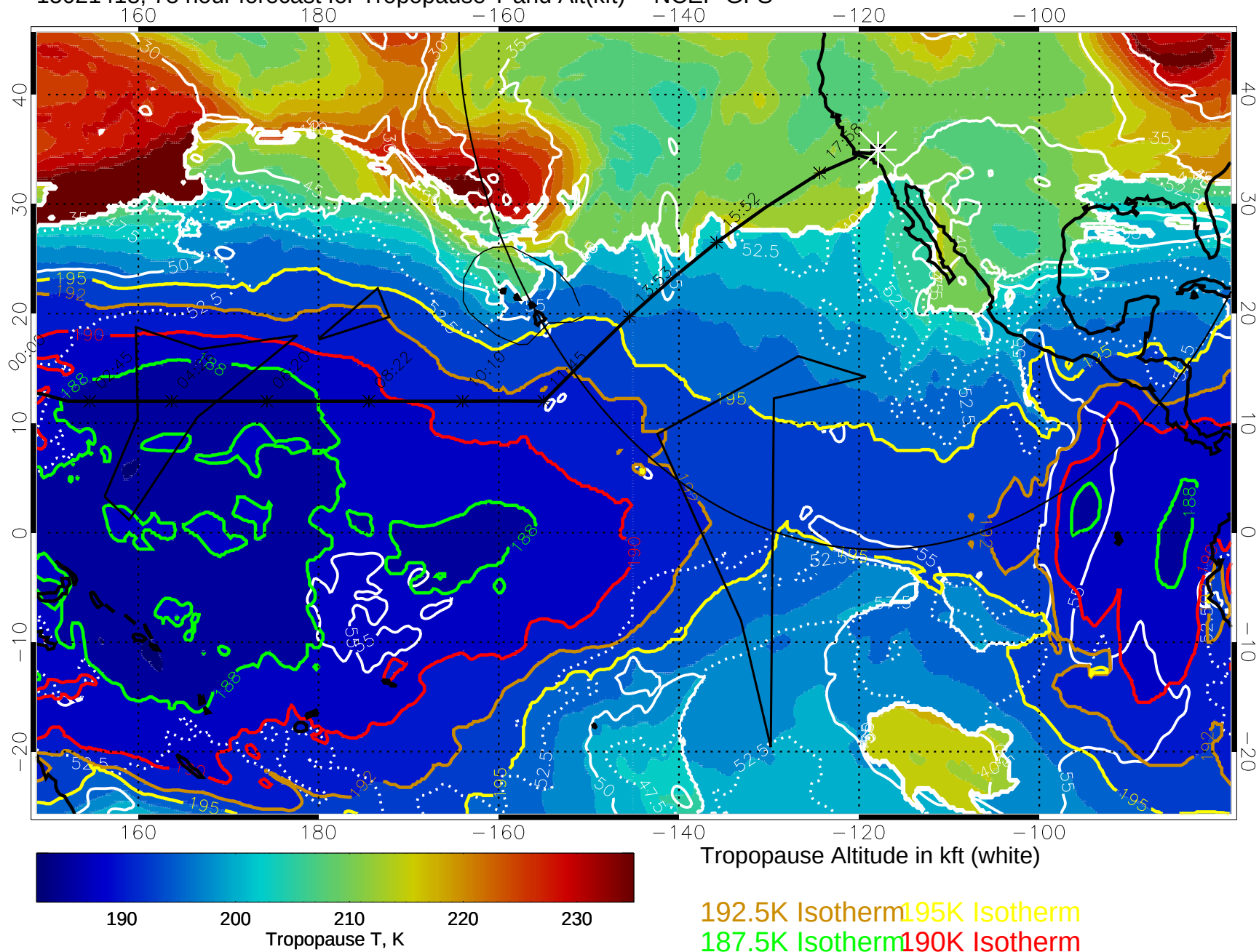
15021418, 78 hour forecast for Tropopause T and Alt(kft) -- NCEP GFS
