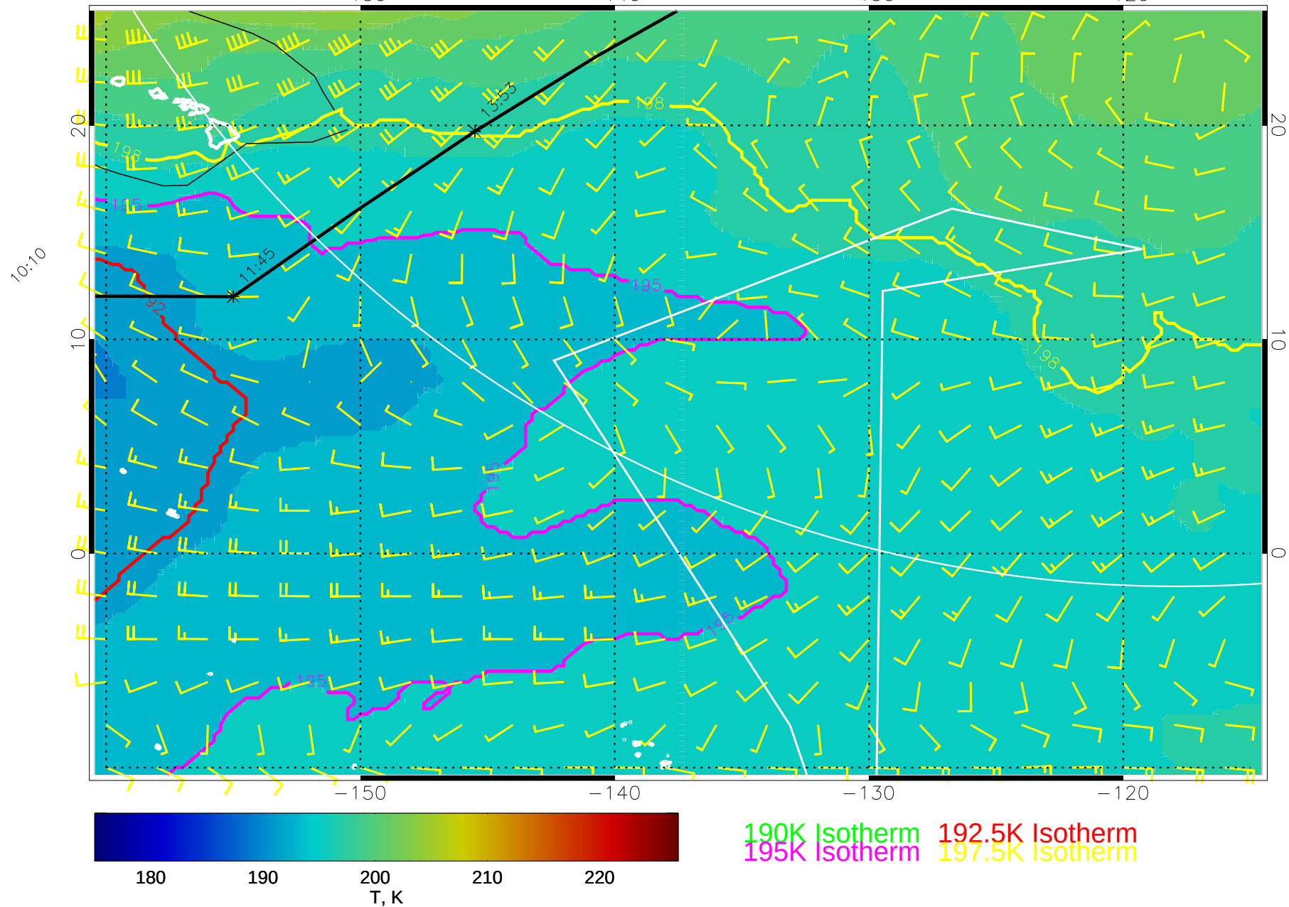
15021118, 6 hour forecast for 70mb T and winds (knots) -- NCEP GFS
