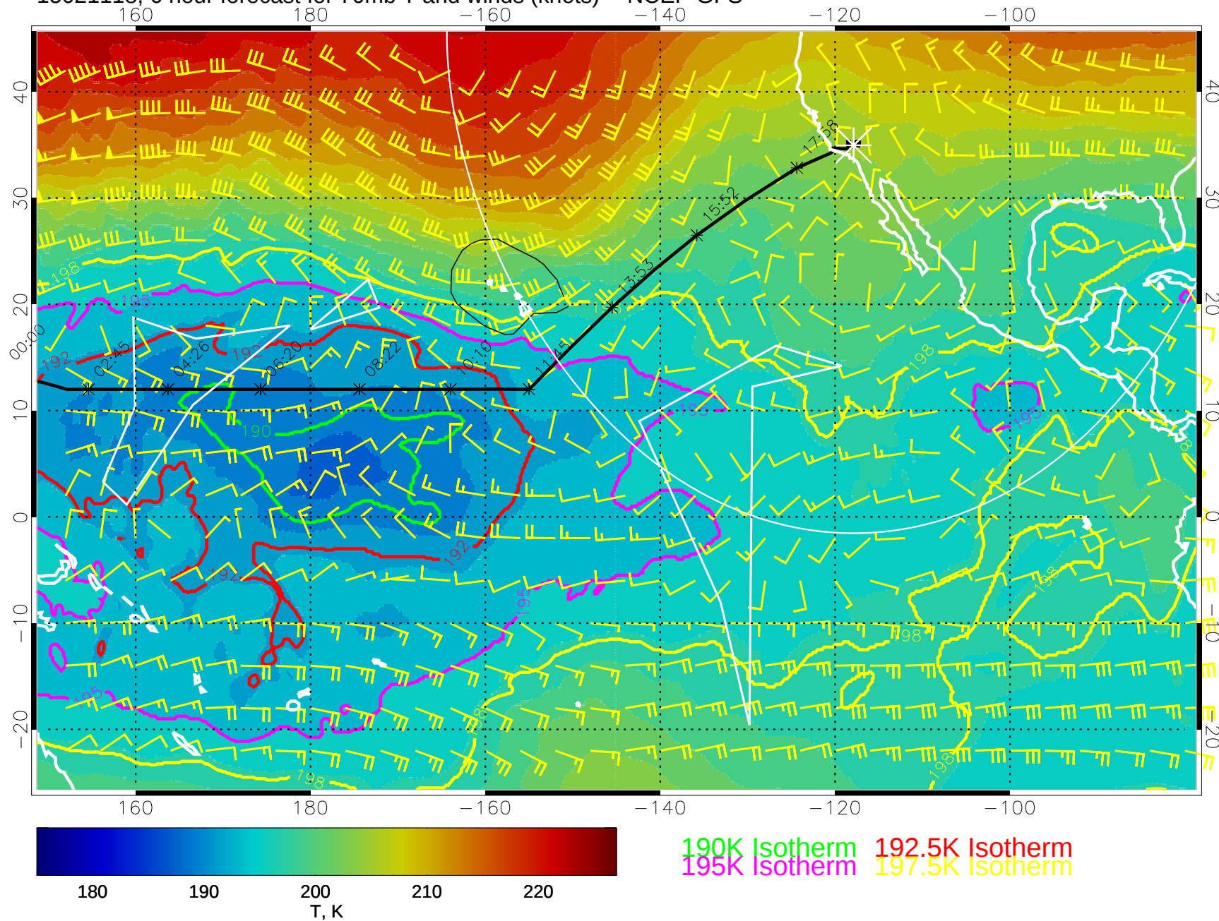
15021118, 6 hour forecast for 70mb T and winds (knots) -- NCEP GFS
