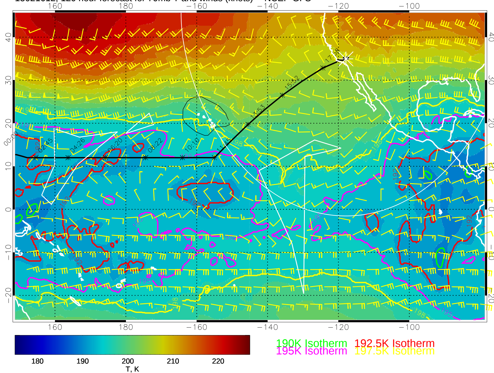
15021612, 120 hour forecast for 70mb T and winds (knots) -- NCEP GFS
