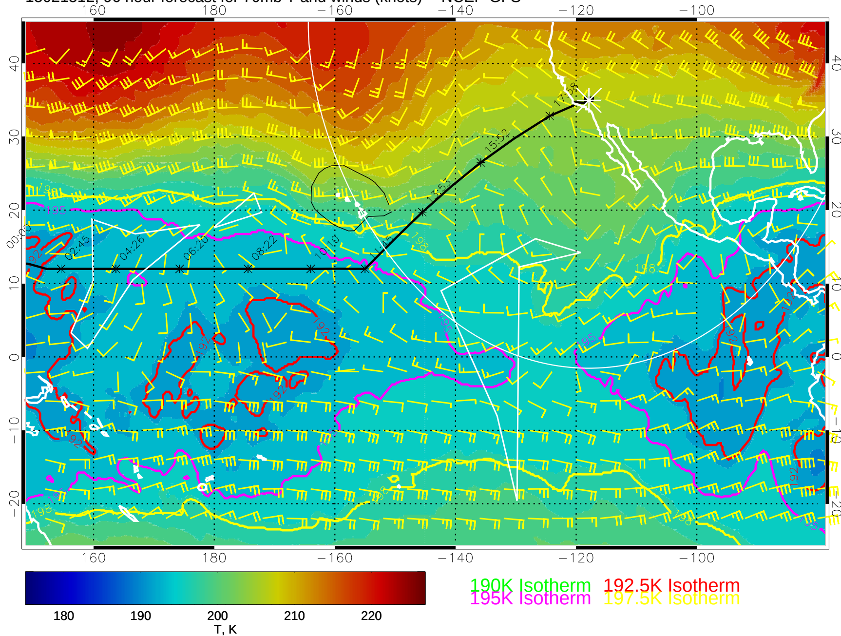
15021512, 96 hour forecast for 70mb T and winds (knots) -- NCEP GFS
