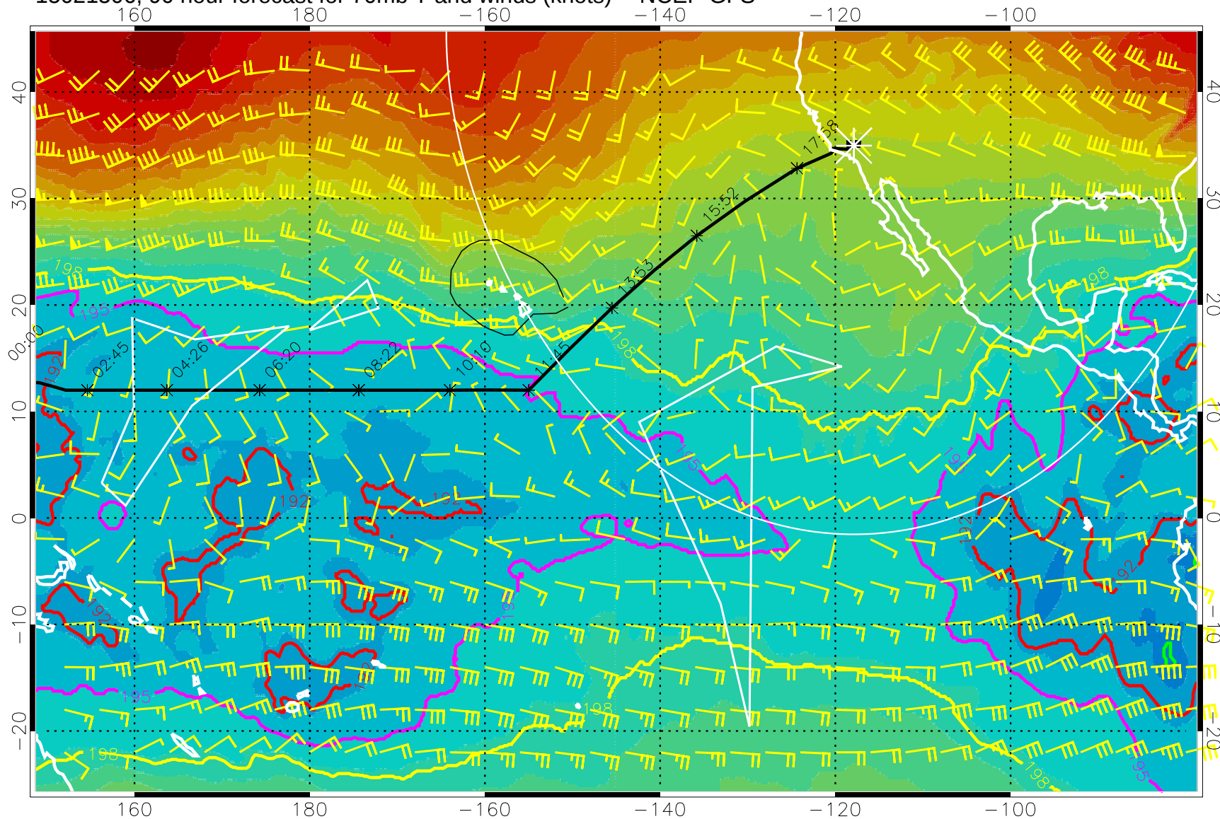
15021506, 90 hour forecast for 70mb T and winds (knots) -- NCEP GFS
