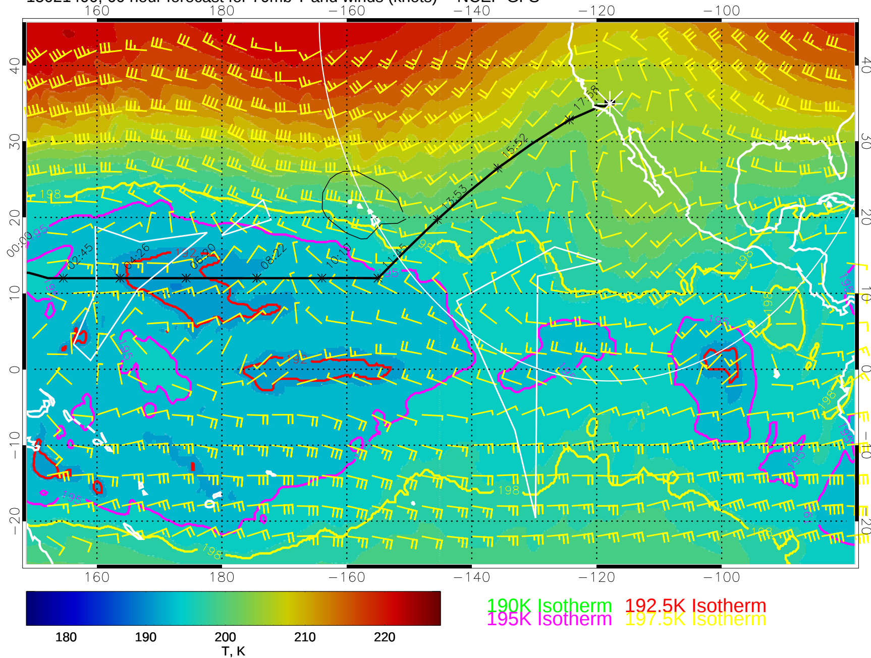
15021400, 60 hour forecast for 70mb T and winds (knots) -- NCEP GFS
