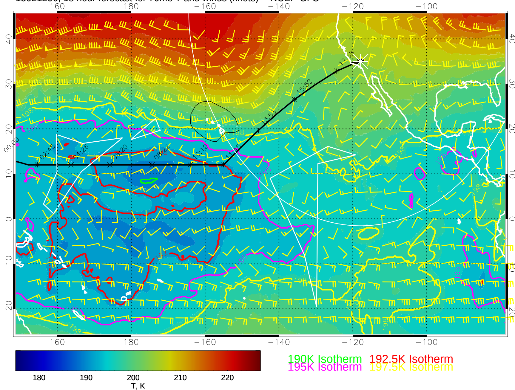
15021206, 18 hour forecast for 70mb T and winds (knots) -- NCEP GFS
