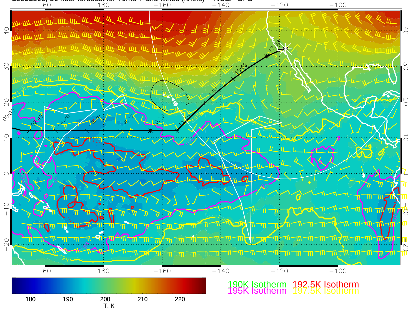
15021300, 36 hour forecast for 70mb T and winds (knots) -- NCEP GFS
