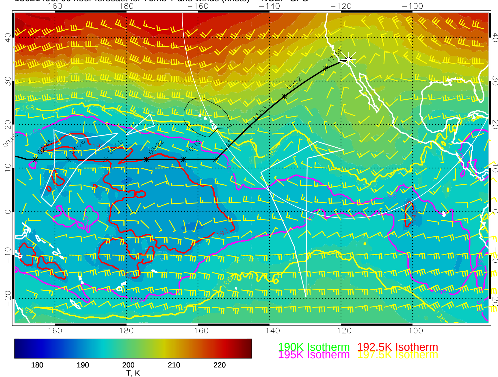
15021406, 66 hour forecast for 70mb T and winds (knots) -- NCEP GFS
