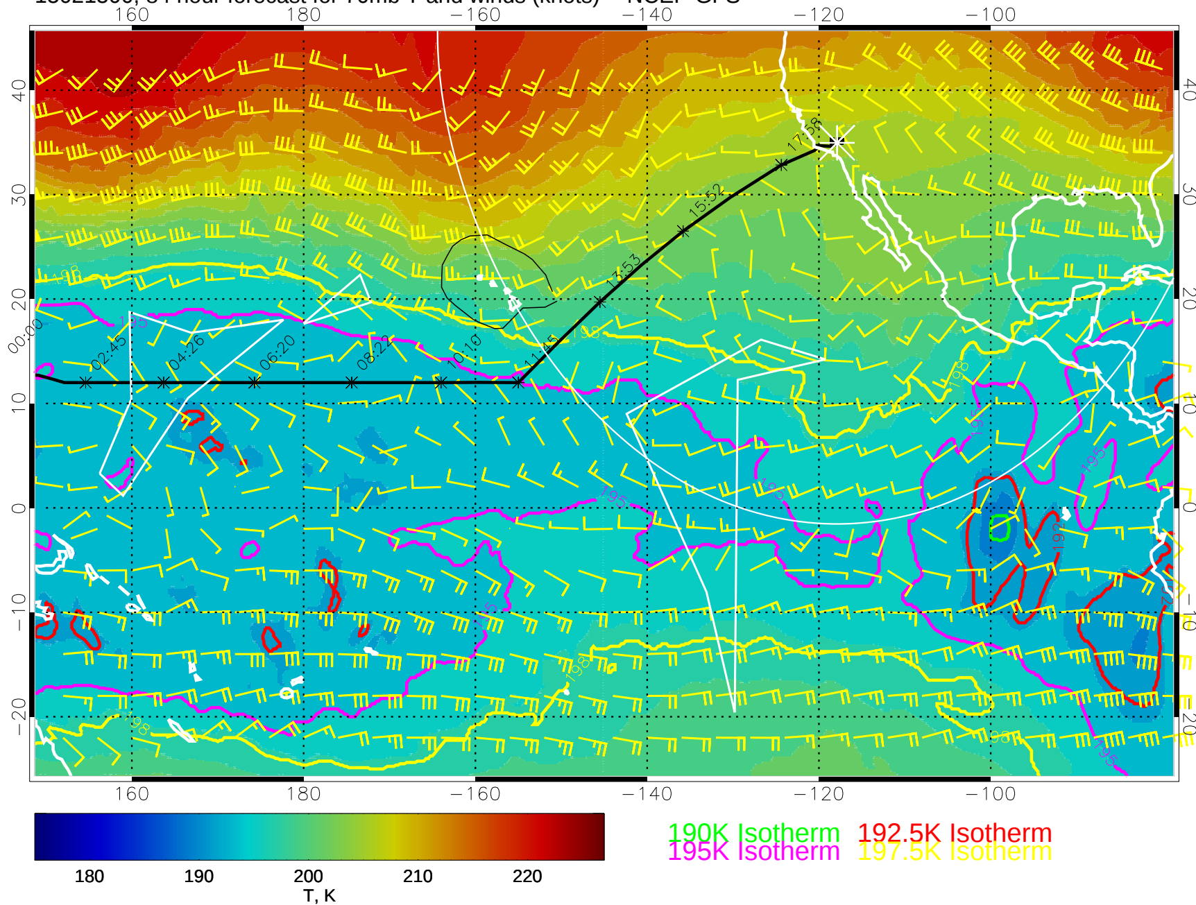
15021500, 84 hour forecast for 70mb T and winds (knots) -- NCEP GFS
