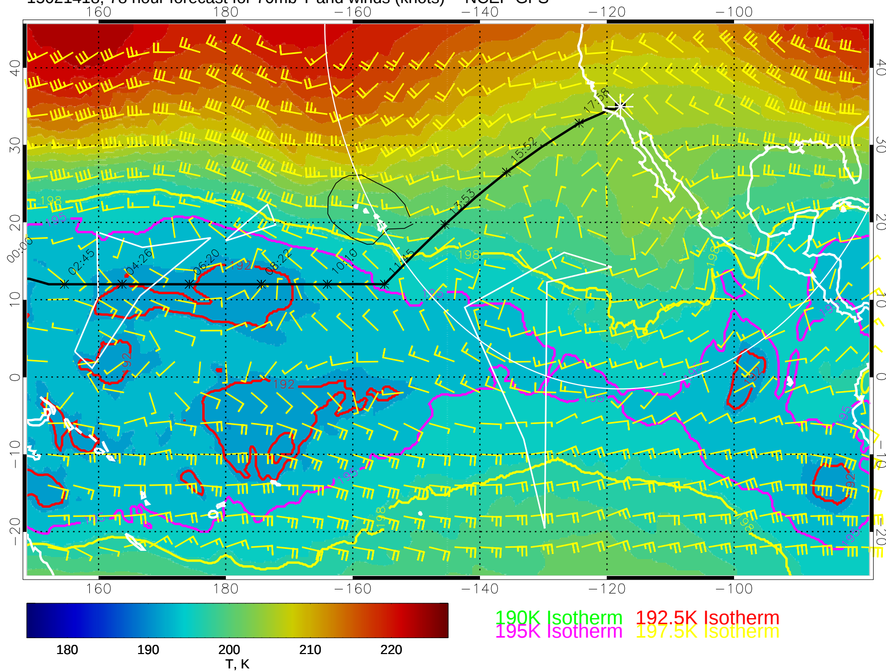
15021418, 78 hour forecast for 70mb T and winds (knots) -- NCEP GFS
