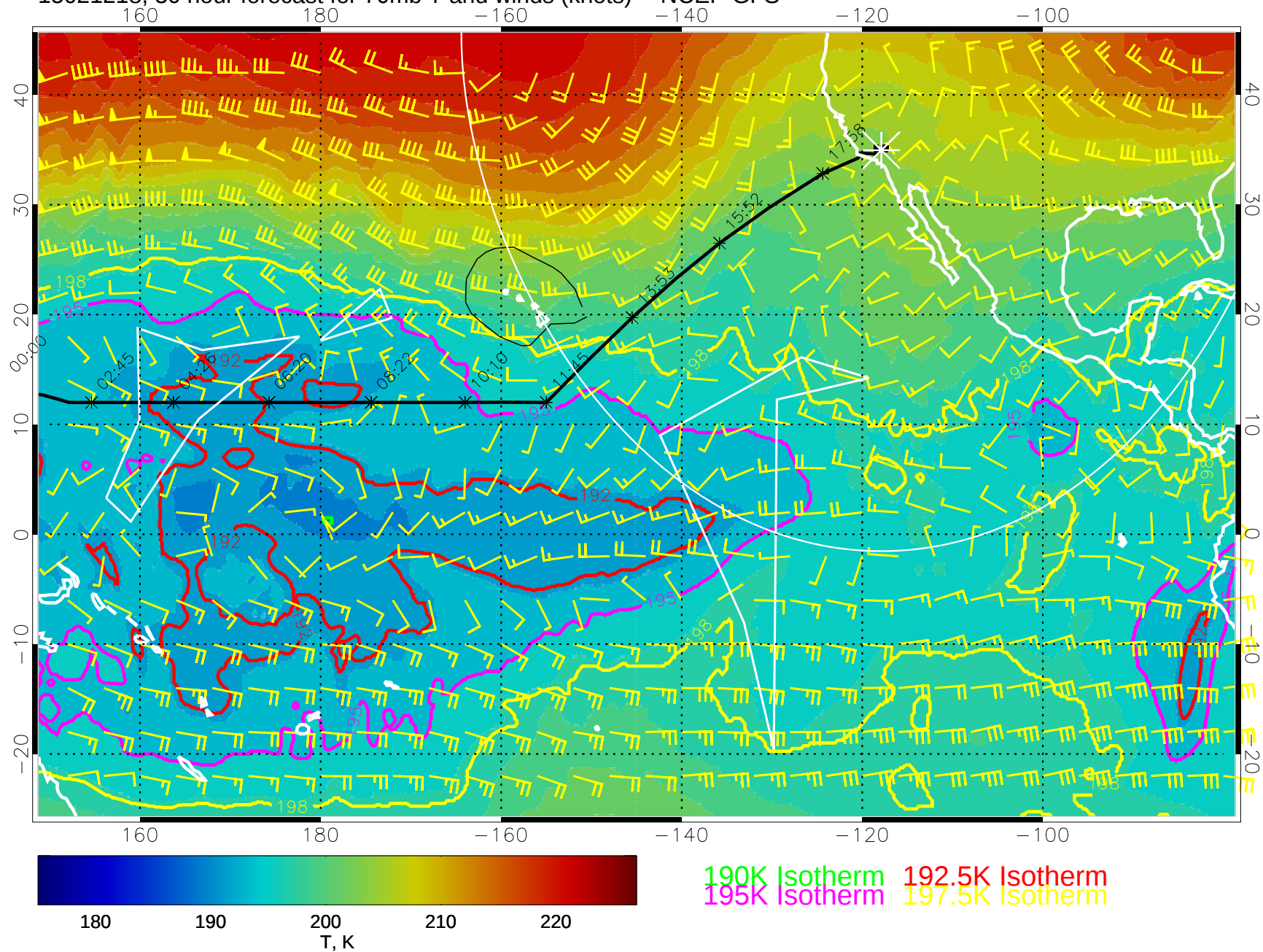
15021218, 30 hour forecast for 70mb T and winds (knots) -- NCEP GFS
