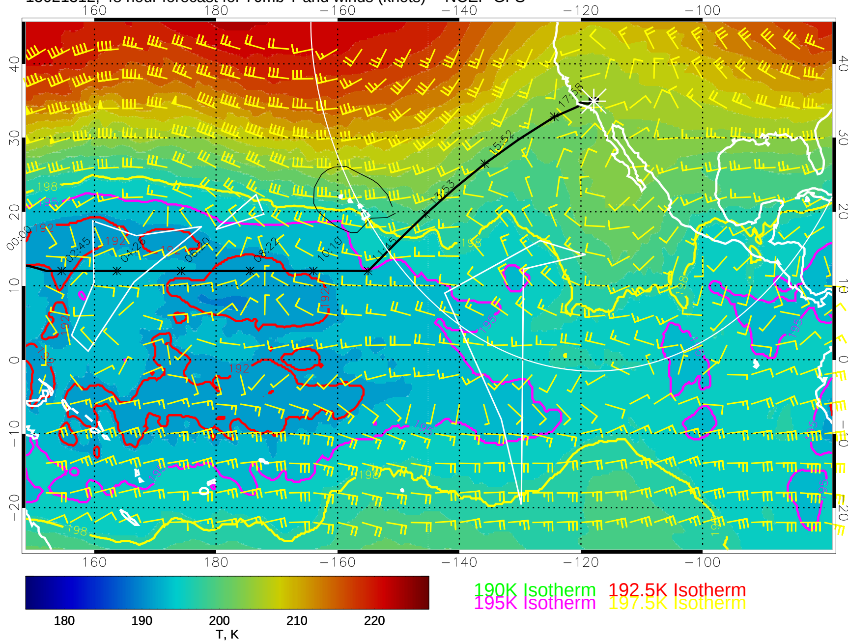
15021312, 48 hour forecast for 70mb T and winds (knots) -- NCEP GFS
