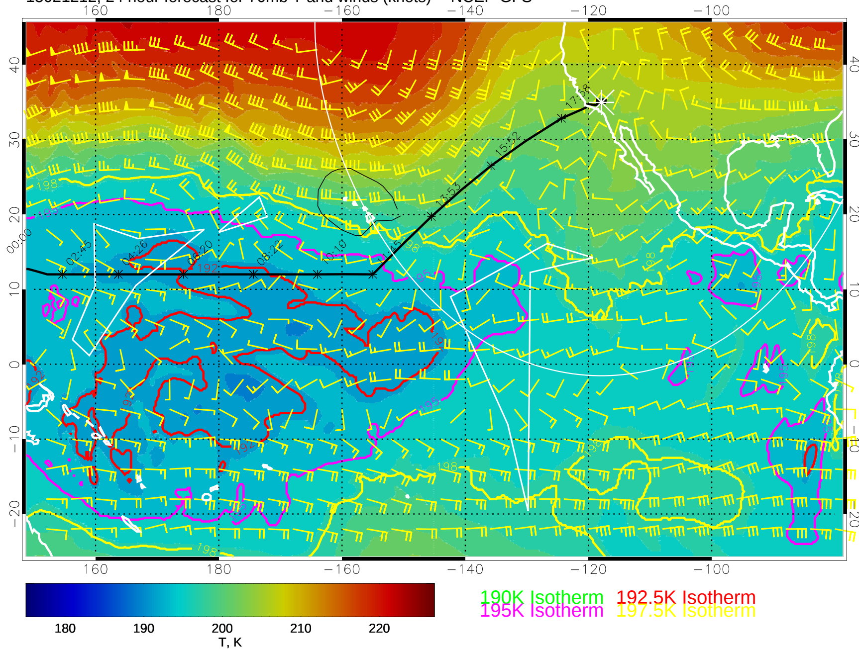
15021212, 24 hour forecast for 70mb T and winds (knots) -- NCEP GFS
