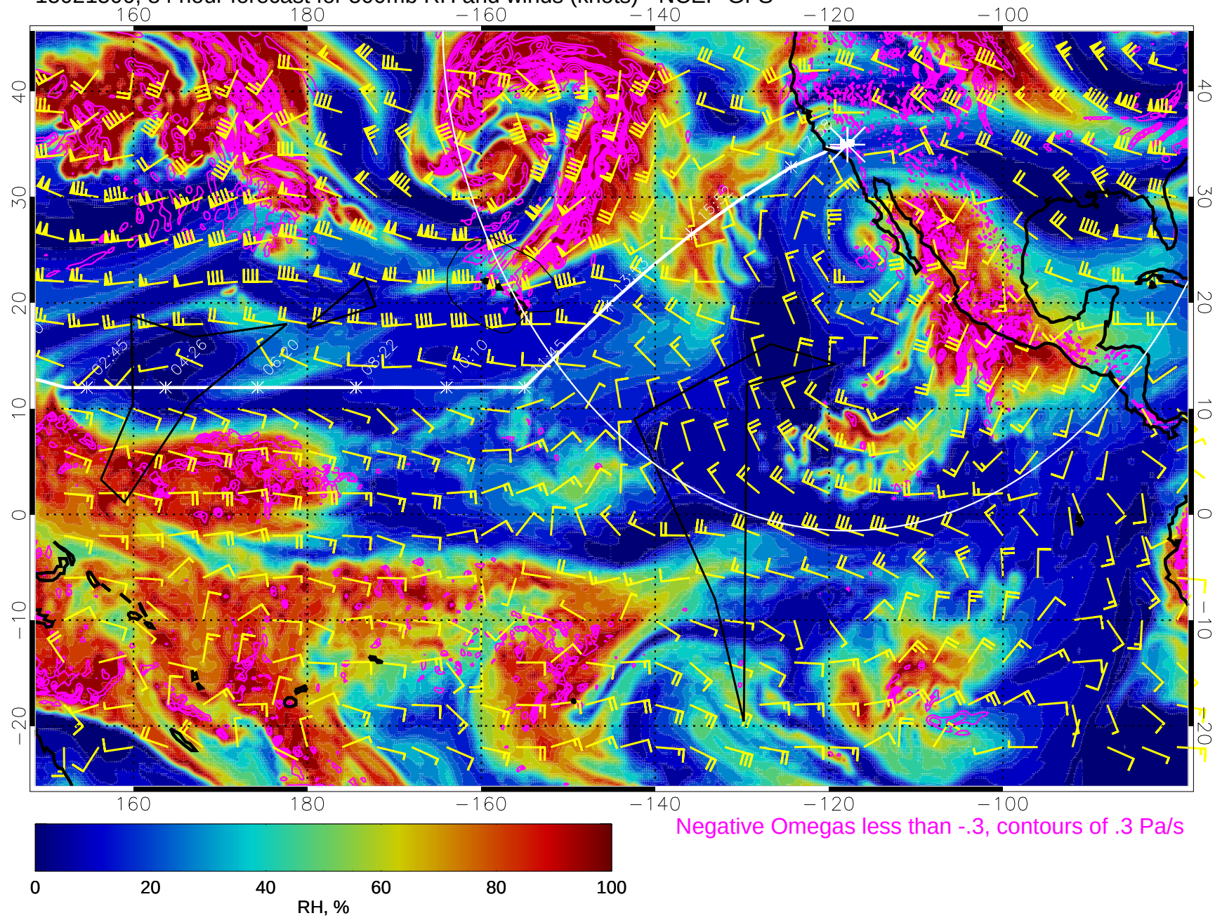
15021500, 84 hour forecast for 500mb RH and winds (knots) - NCEP GFS
