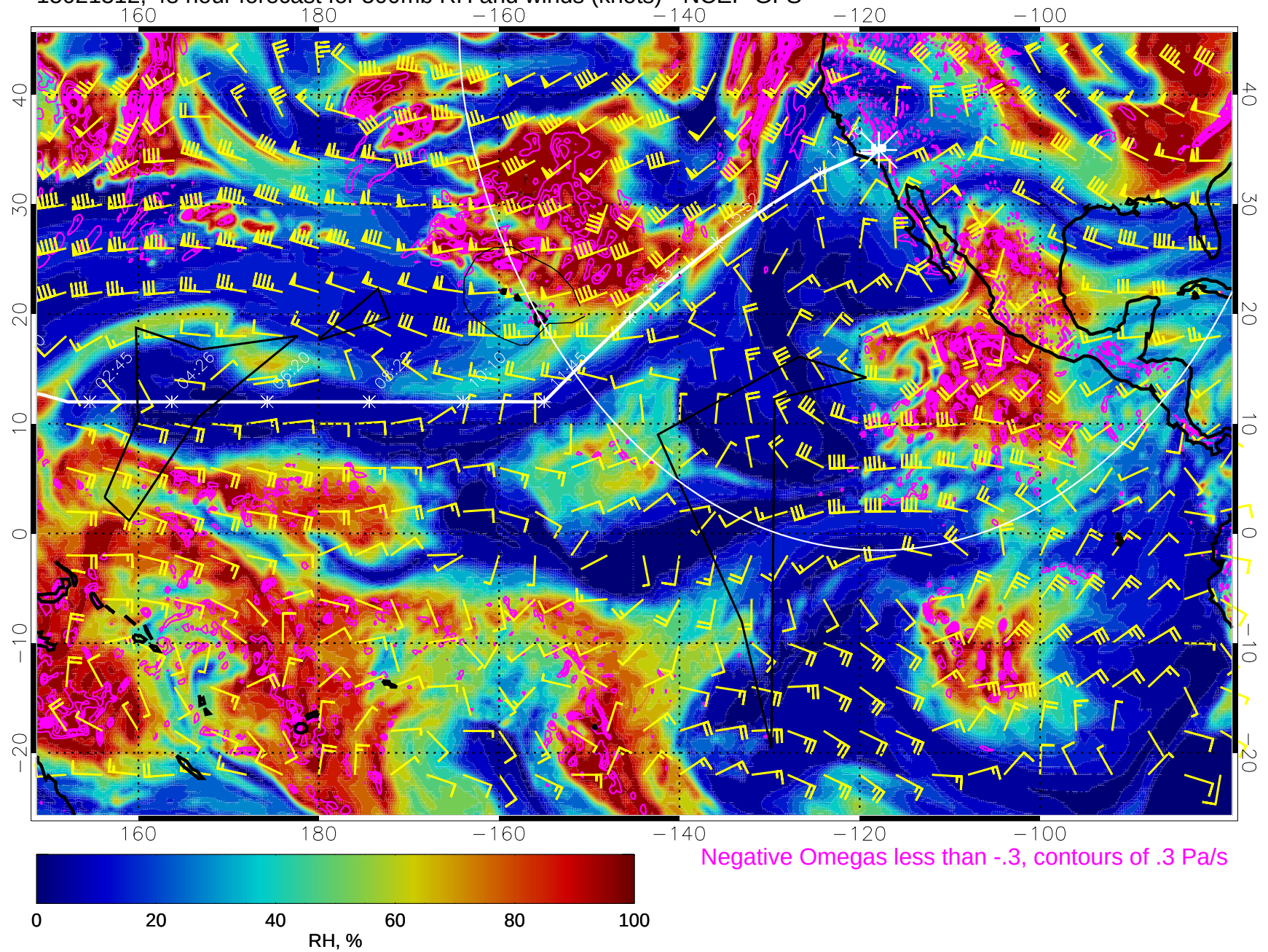
15021312, 48 hour forecast for 500mb RH and winds (knots) - NCEP GFS
