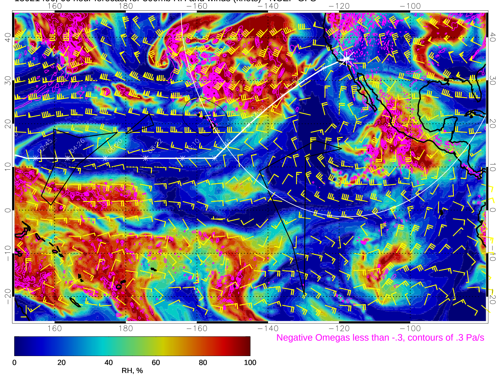
15021406, 66 hour forecast for 500mb RH and winds (knots) - NCEP GFS
