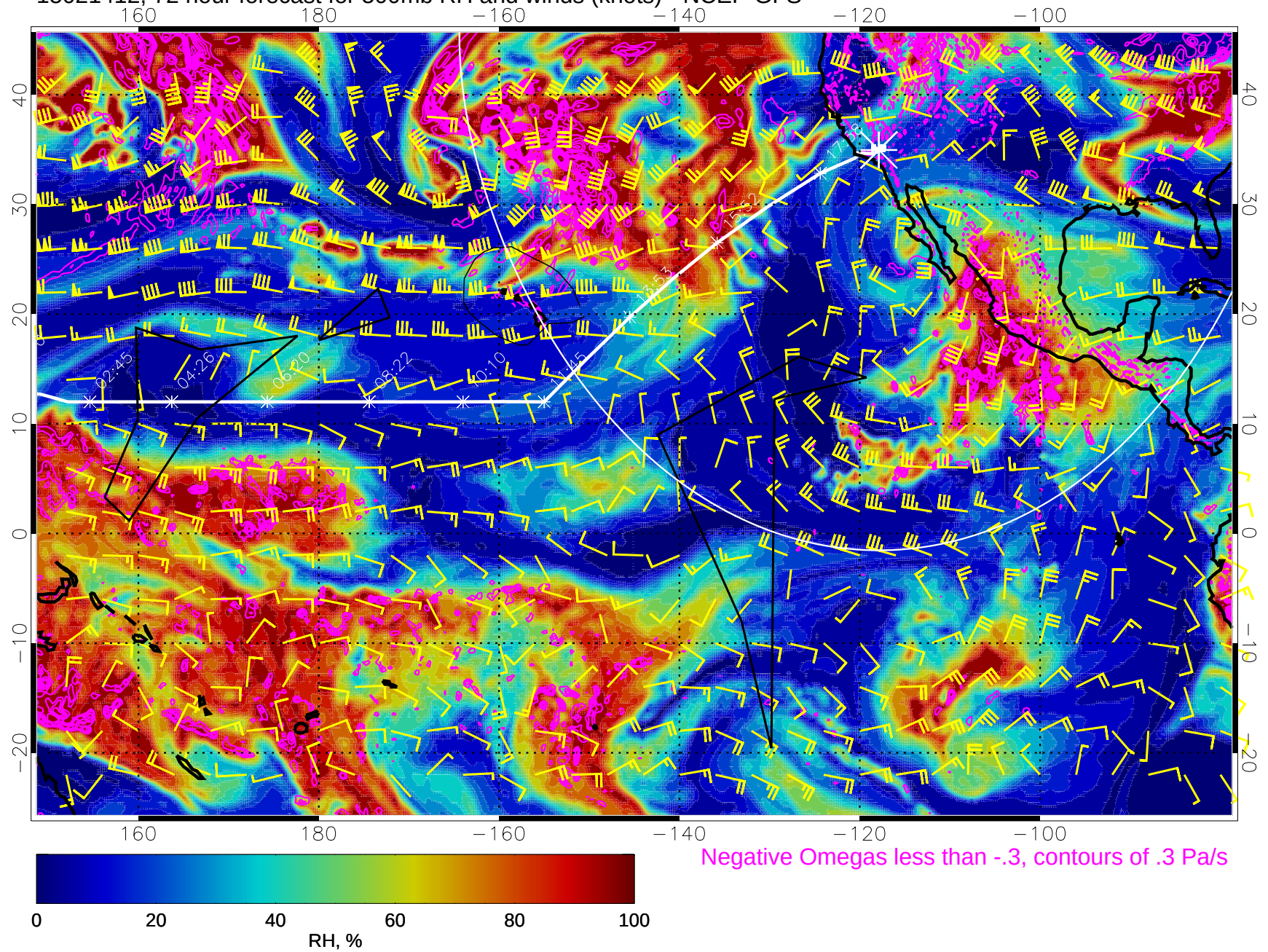
15021412, 72 hour forecast for 500mb RH and winds (knots) - NCEP GFS
