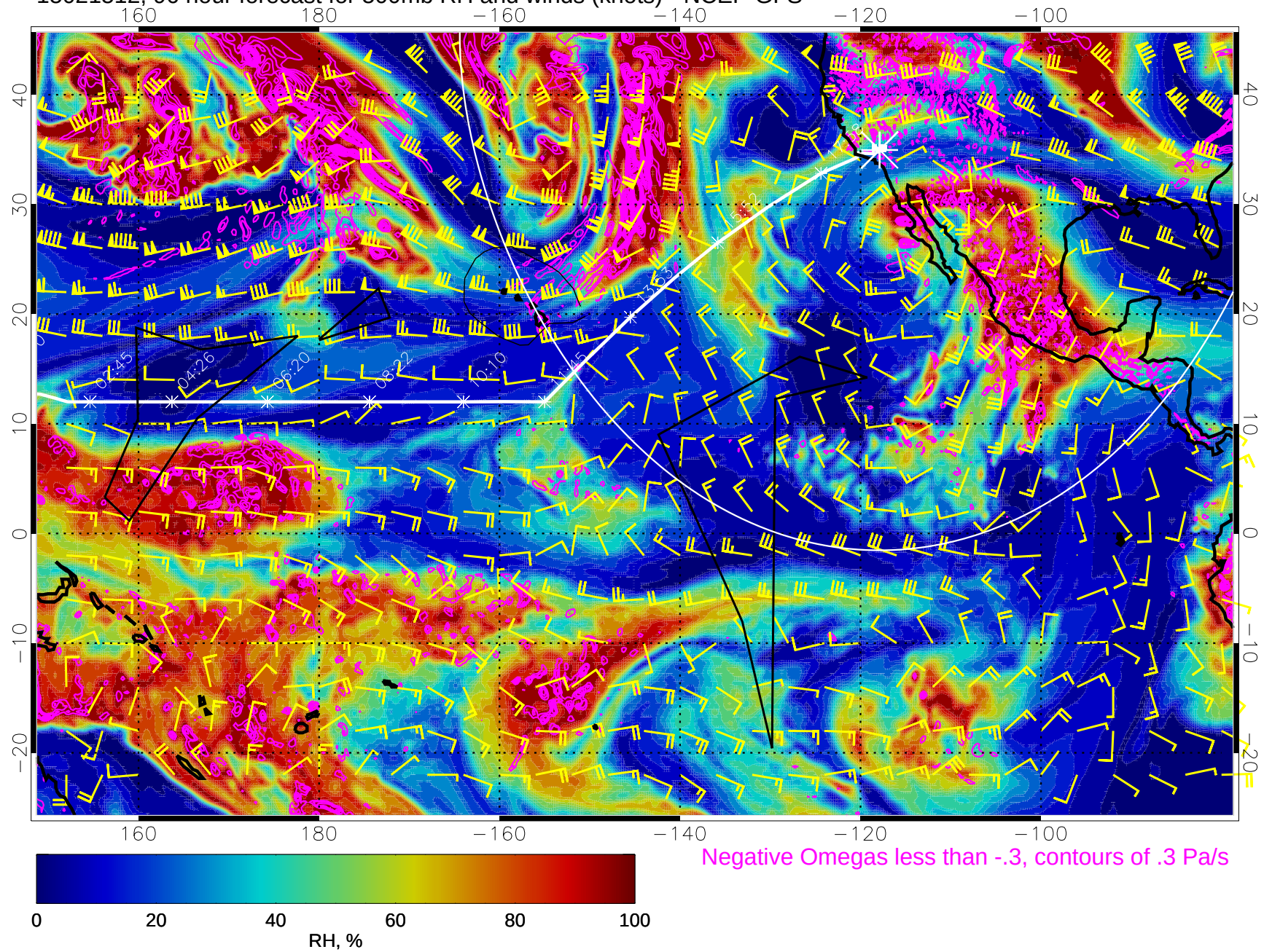
15021512, 96 hour forecast for 500mb RH and winds (knots) - NCEP GFS
