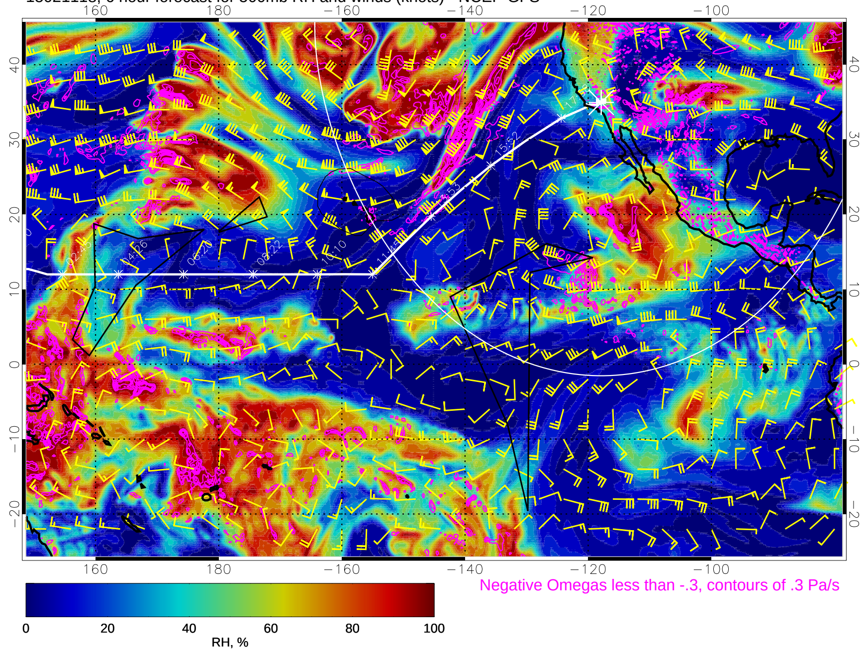
15021118, 6 hour forecast for 500mb RH and winds (knots) - NCEP GFS
