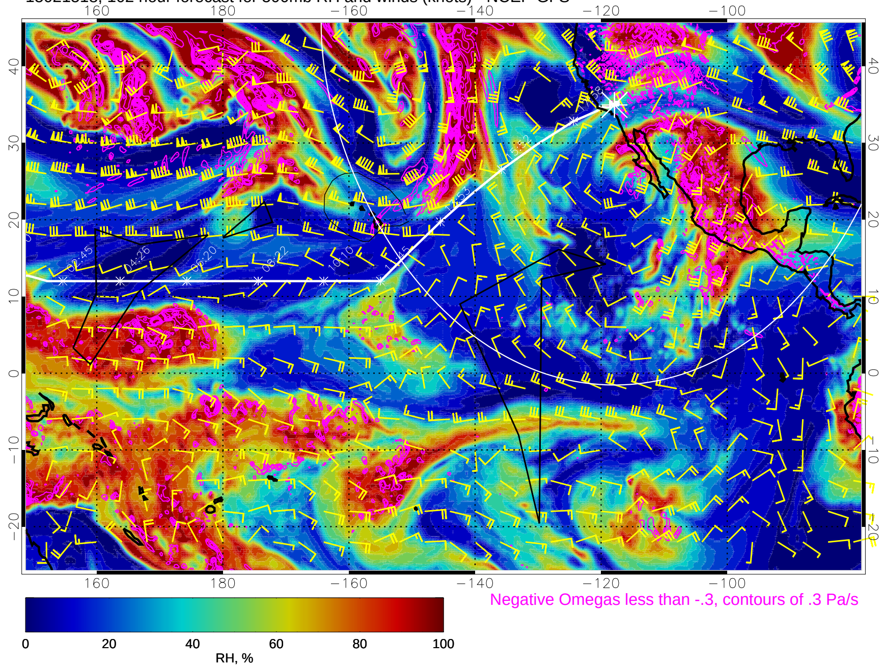
15021518, 102 hour forecast for 500mb RH and winds (knots) - NCEP GFS
