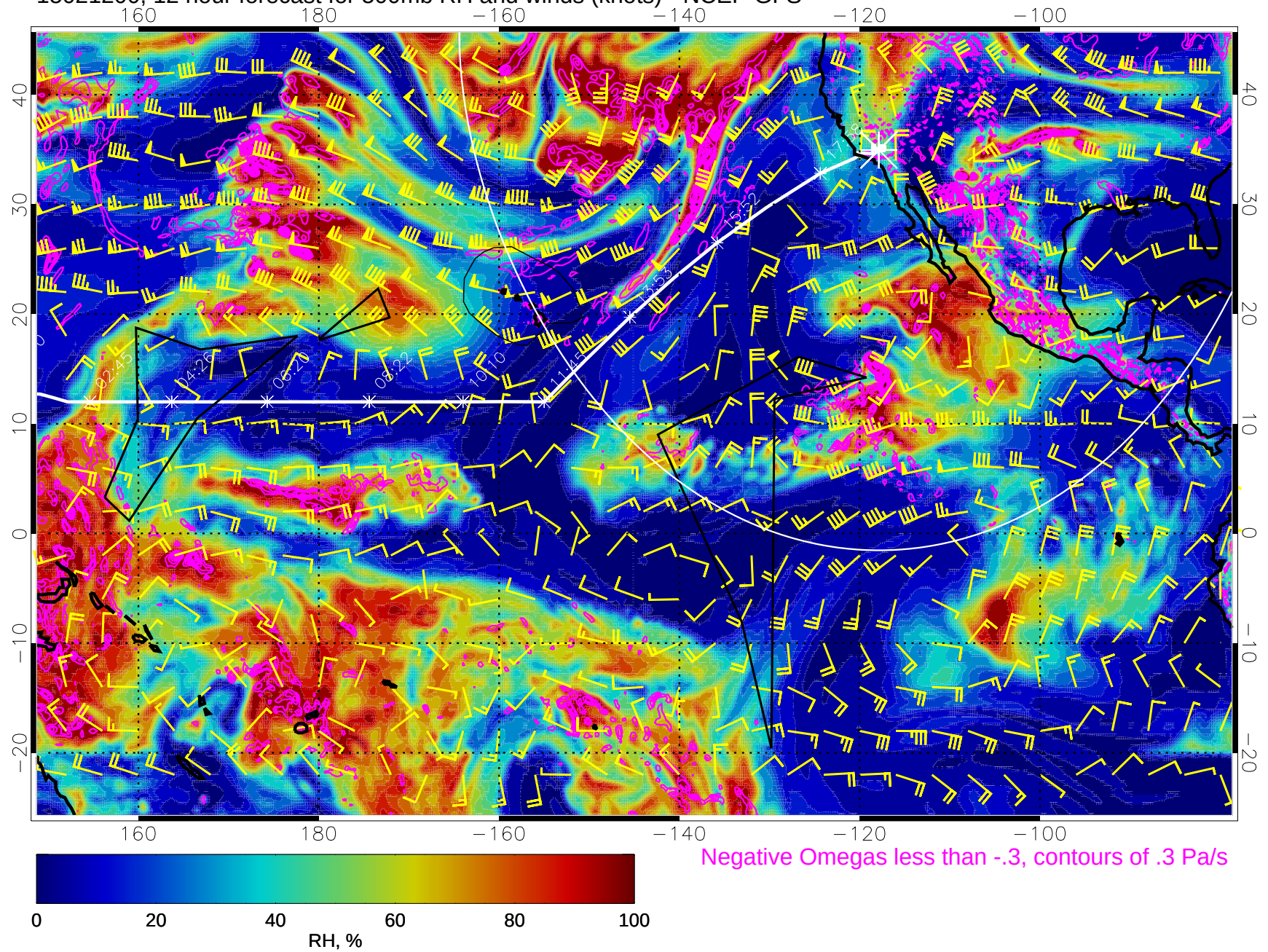
15021200, 12 hour forecast for 500mb RH and winds (knots) - NCEP GFS
