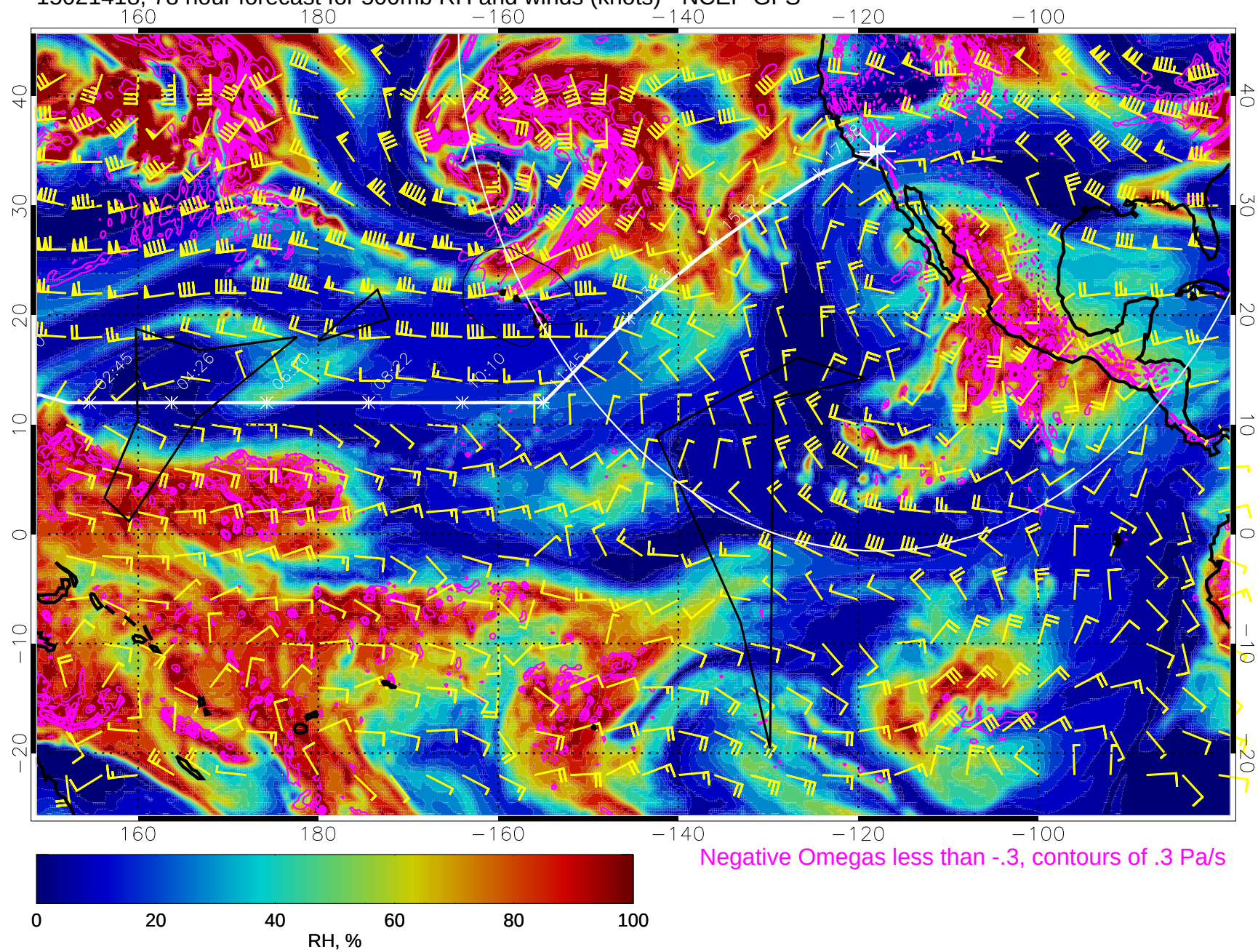
15021418, 78 hour forecast for 500mb RH and winds (knots) - NCEP GFS
