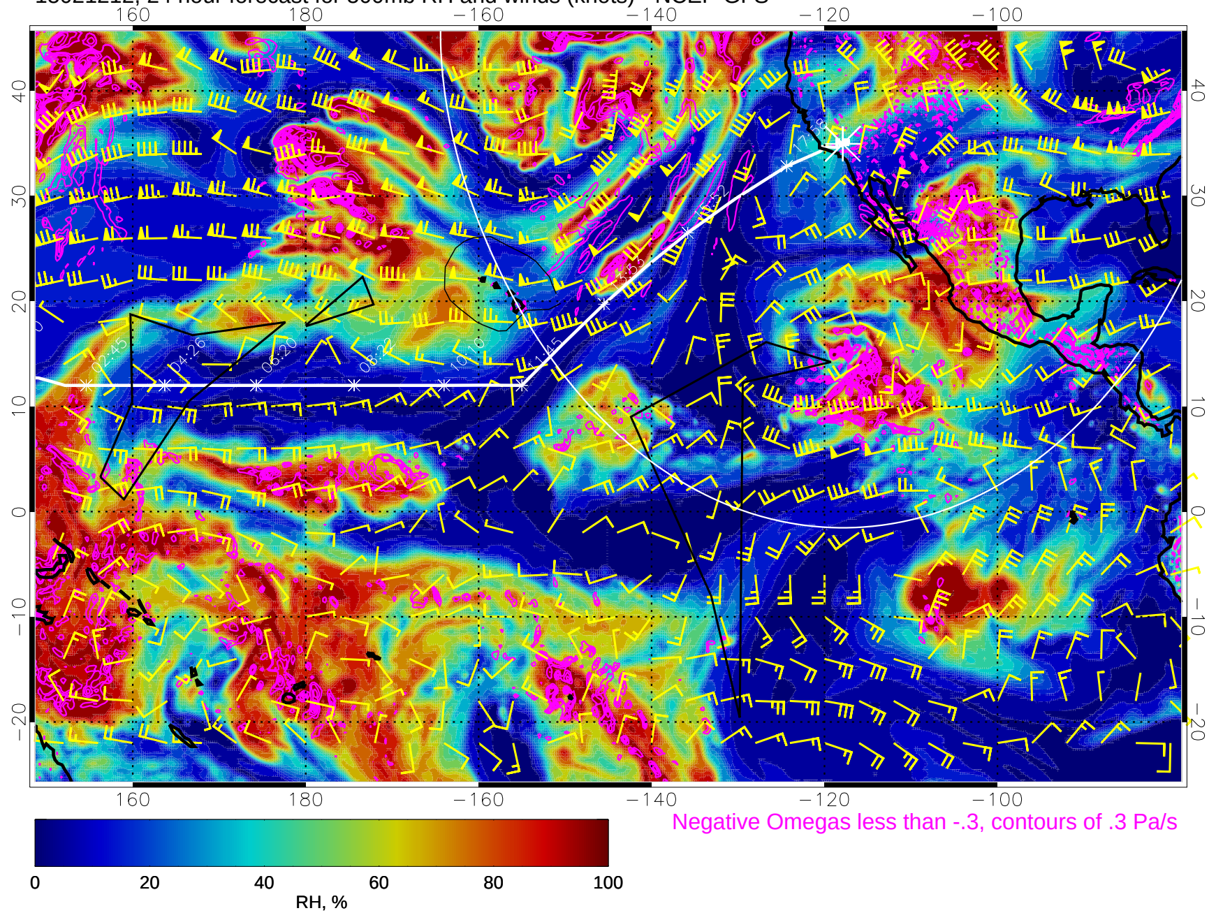
15021212, 24 hour forecast for 500mb RH and winds (knots) - NCEP GFS
