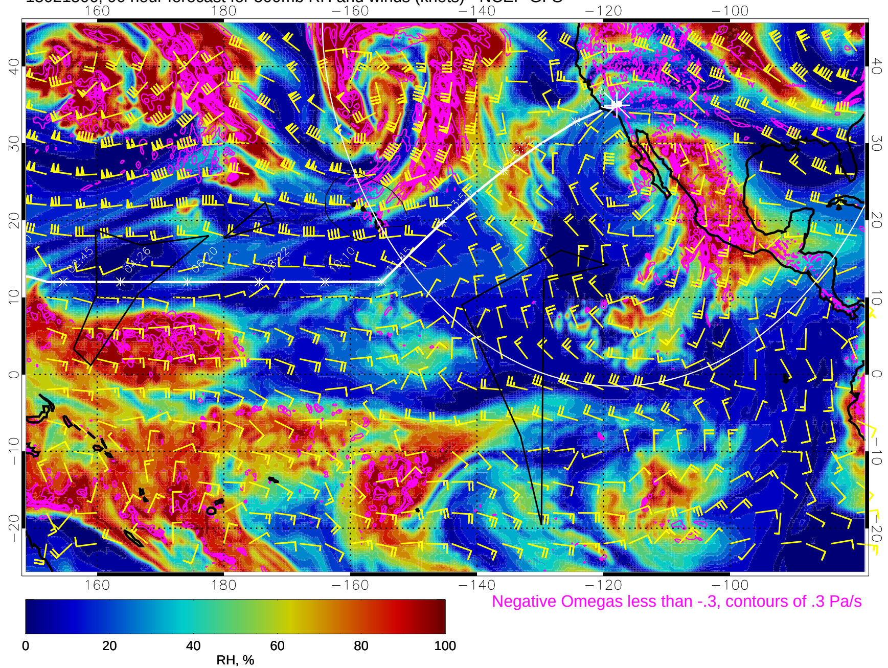
15021506, 90 hour forecast for 500mb RH and winds (knots) - NCEP GFS
