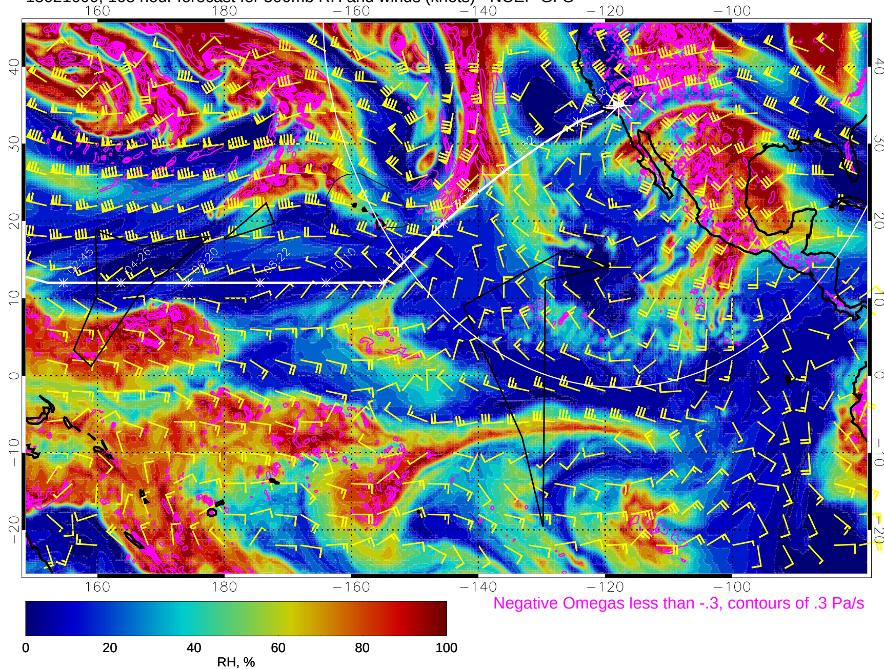
15021600, 108 hour forecast for 500mb RH and winds (knots) - NCEP GFS
