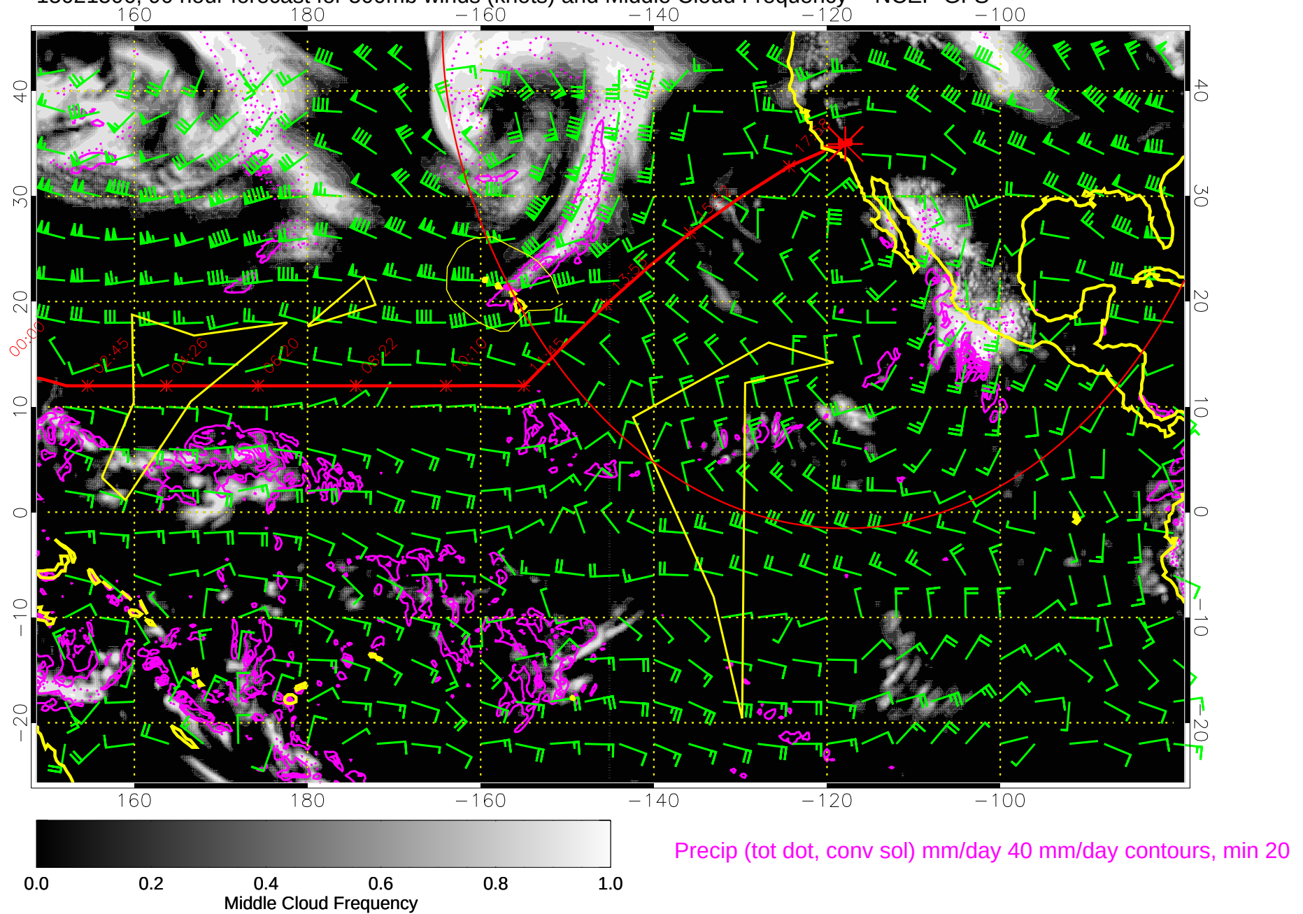
15021506, 90 hour forecast for 500mb winds (knots) and Middle Cloud Frequency -- NCEP GFS
