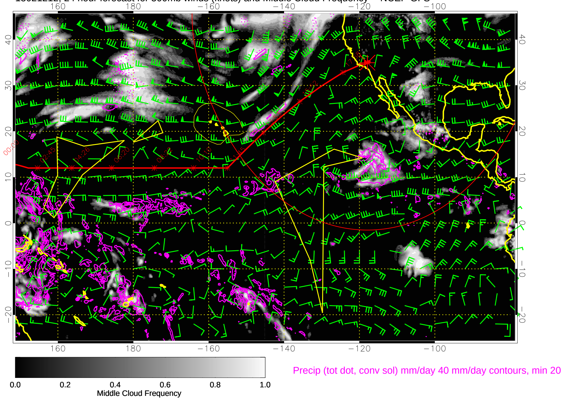
15021212, 24 hour forecast for 500mb winds (knots) and Middle Cloud Frequency -- NCEP GFS
