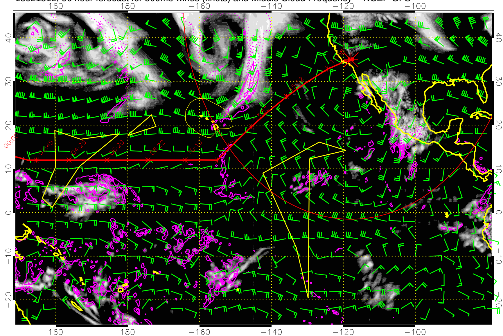
15021512, 96 hour forecast for 500mb winds (knots) and Middle Cloud Frequency -- NCEP GFS
