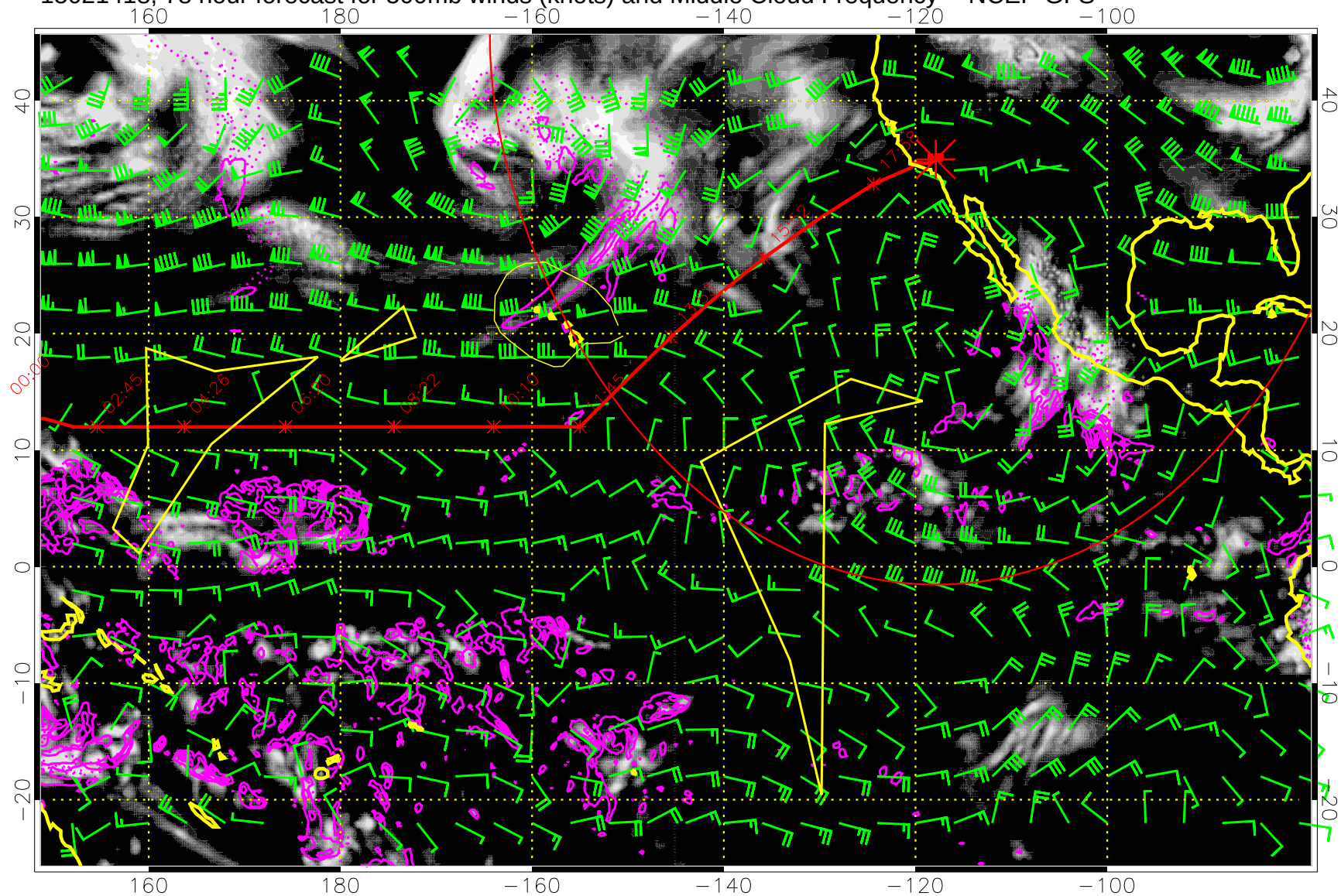
15021418, 78 hour forecast for 500mb winds (knots) and Middle Cloud Frequency -- NCEP GFS
