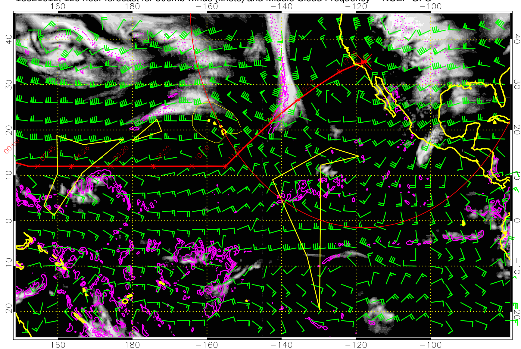
15021612, 120 hour forecast for 500mb winds (knots) and Middle Cloud Frequency -- NCEP GFS
