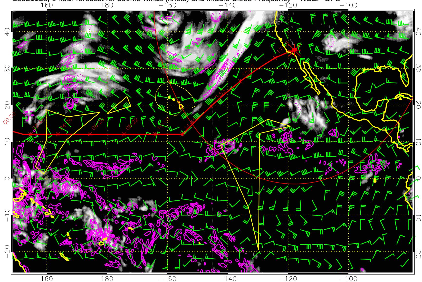
15021118, 6 hour forecast for 500mb winds (knots) and Middle Cloud Frequency -- NCEP GFS
