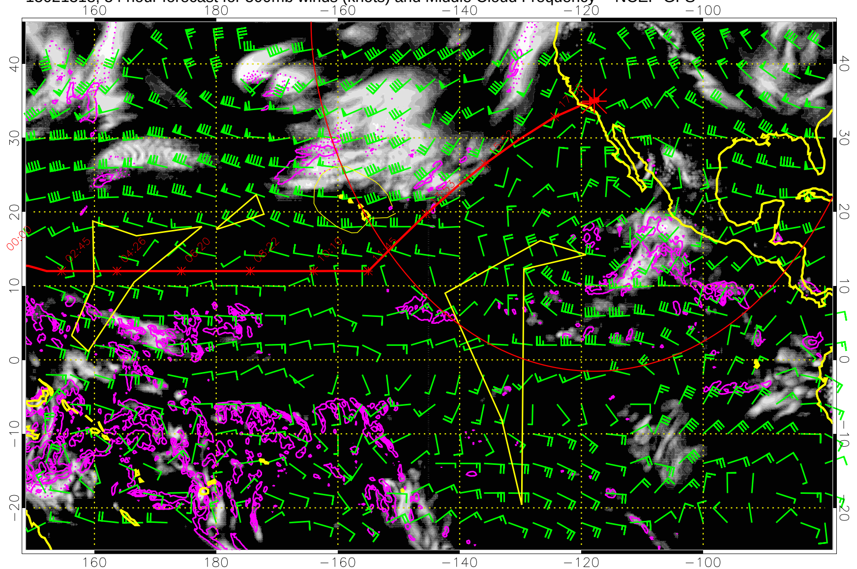
15021318, 54 hour forecast for 500mb winds (knots) and Middle Cloud Frequency -- NCEP GFS
