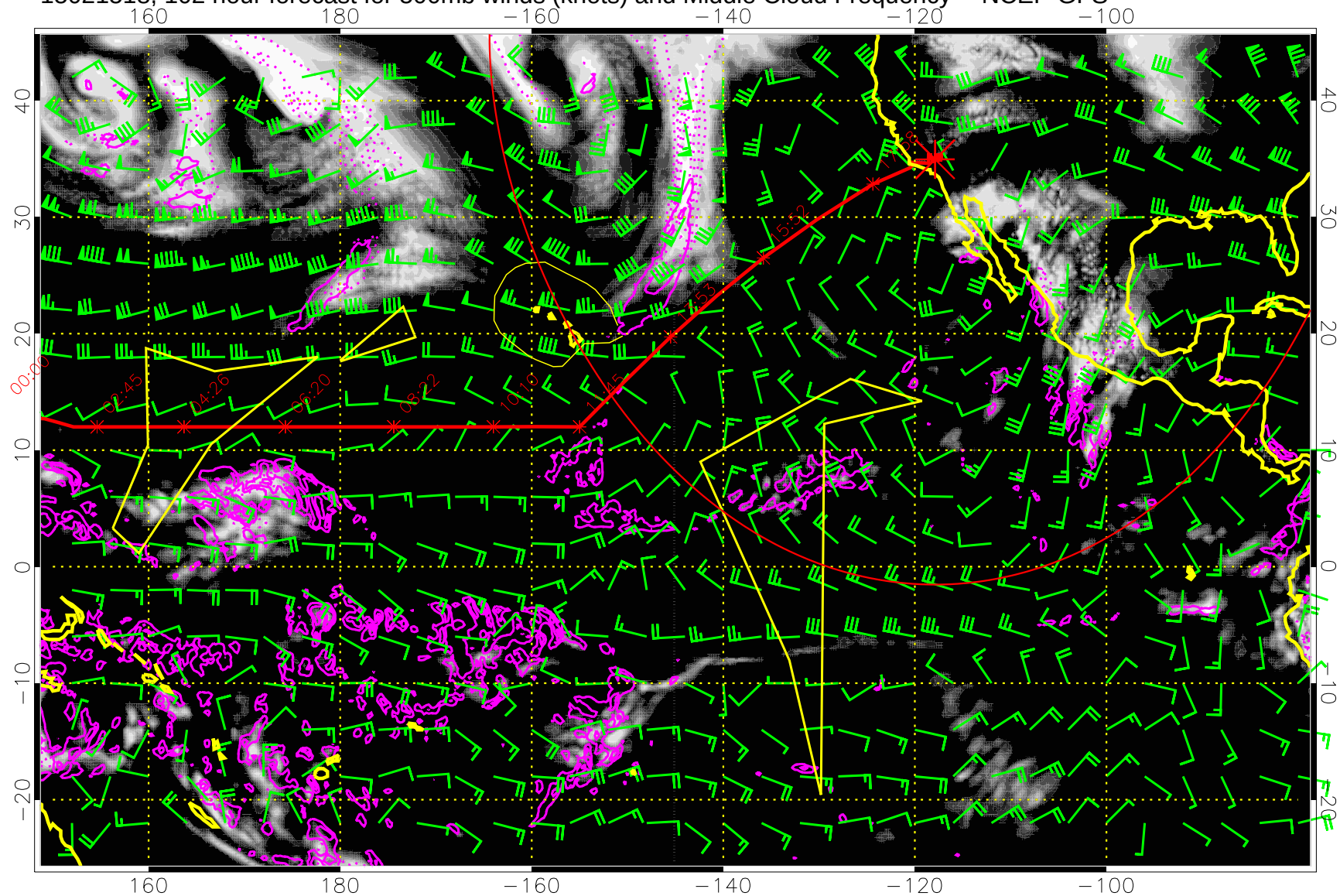
15021518, 102 hour forecast for 500mb winds (knots) and Middle Cloud Frequency -- NCEP GFS
