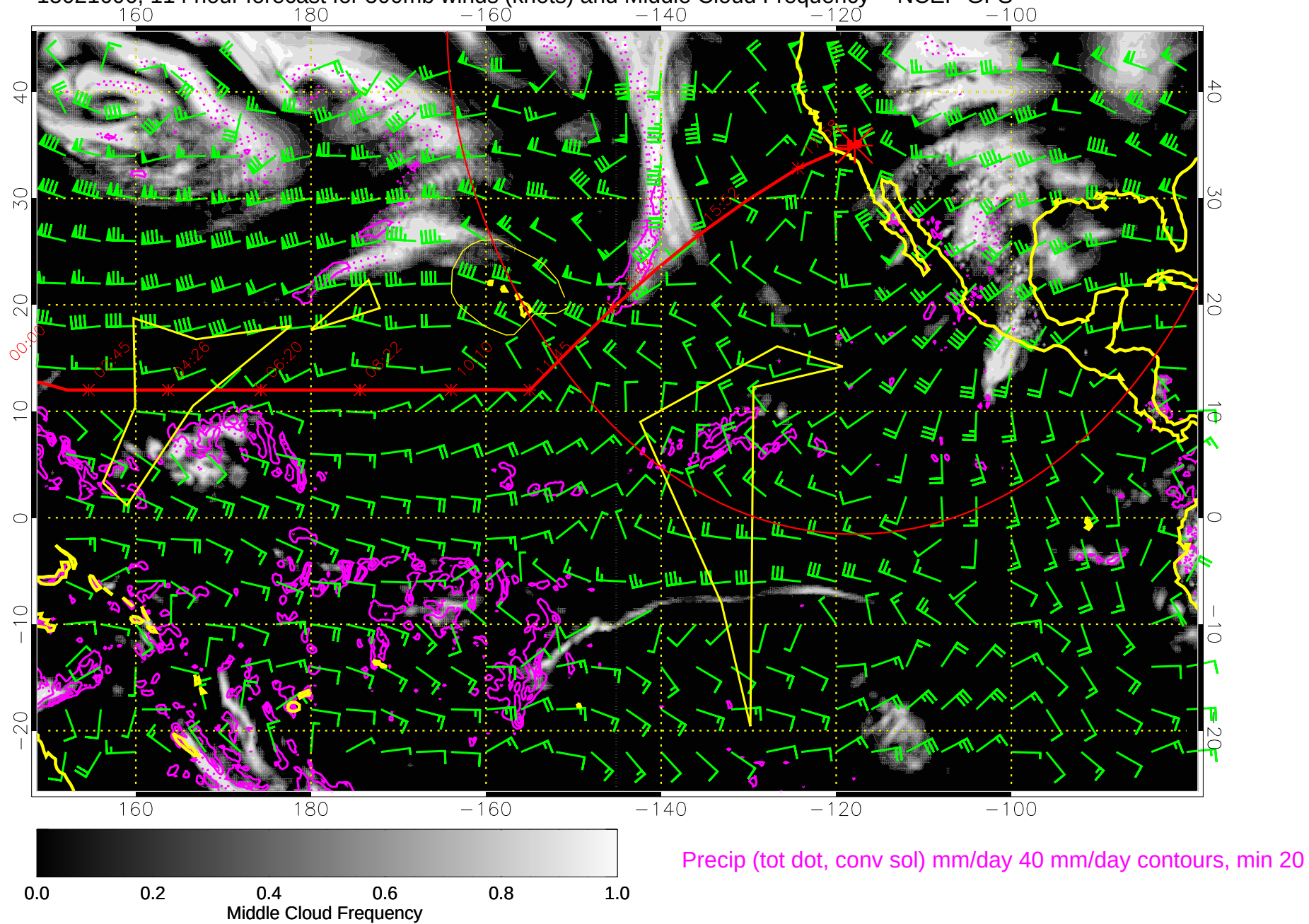
15021606, 114 hour forecast for 500mb winds (knots) and Middle Cloud Frequency -- NCEP GFS
