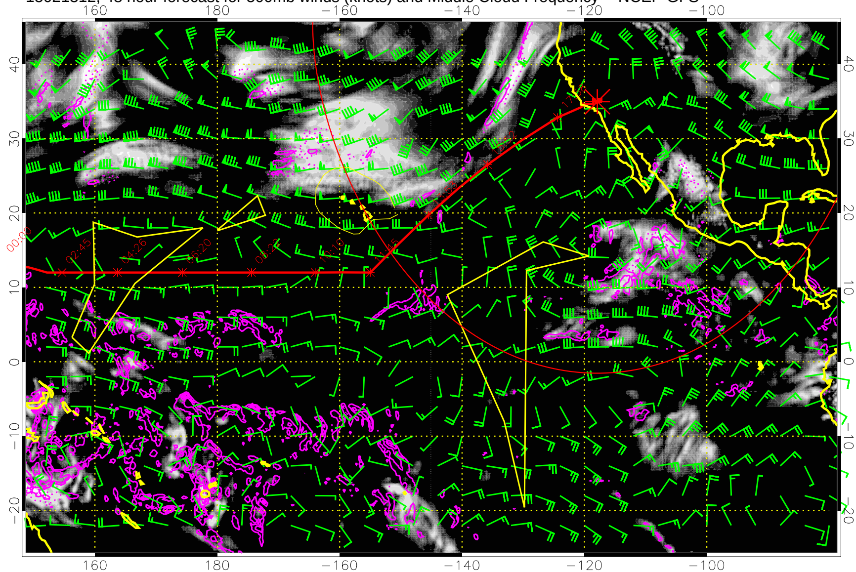
15021312, 48 hour forecast for 500mb winds (knots) and Middle Cloud Frequency -- NCEP GFS
