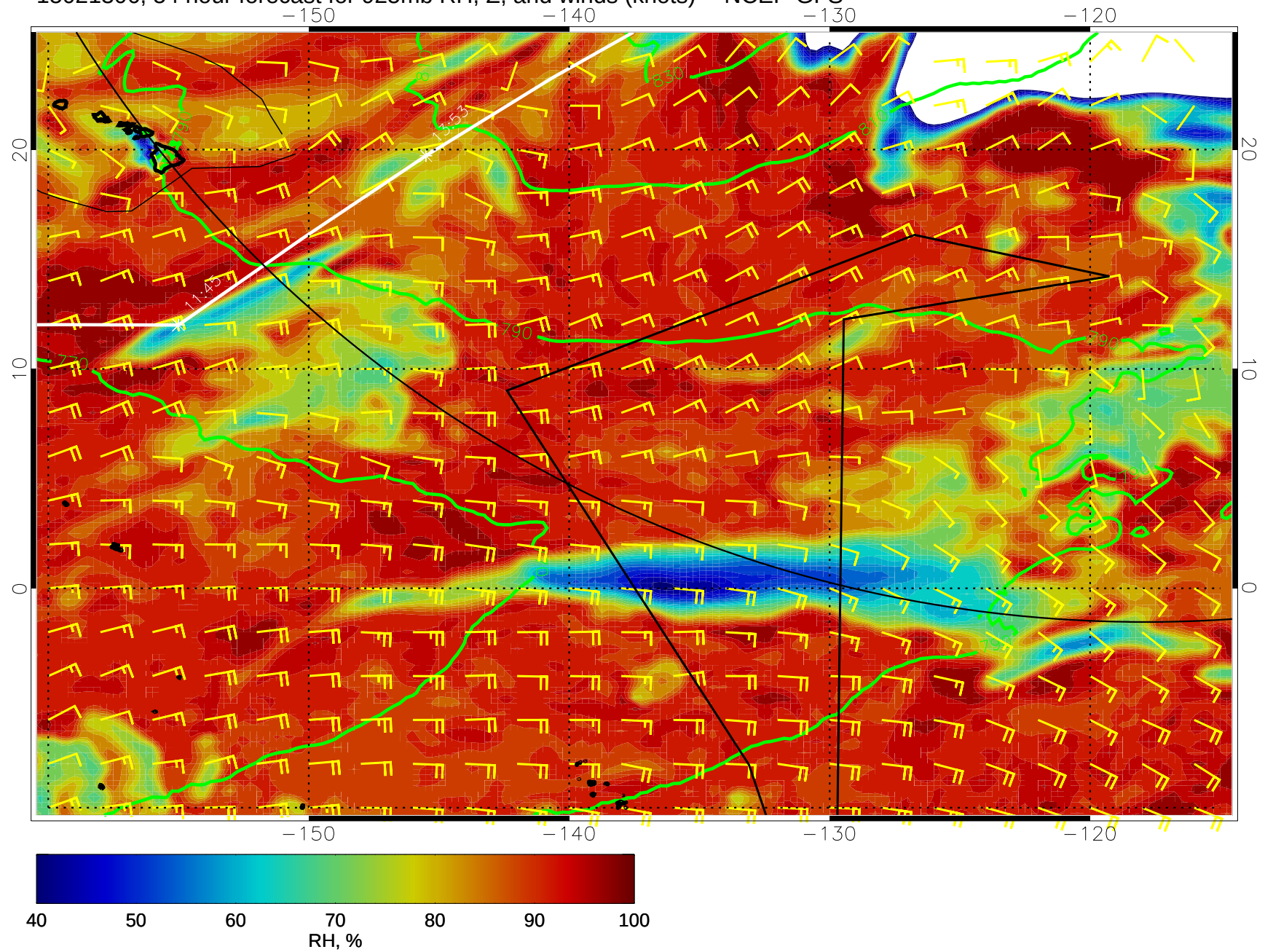
15021306, 54 hour forecast for 925mb RH, Z, and winds (knots) -- NCEP GFS
