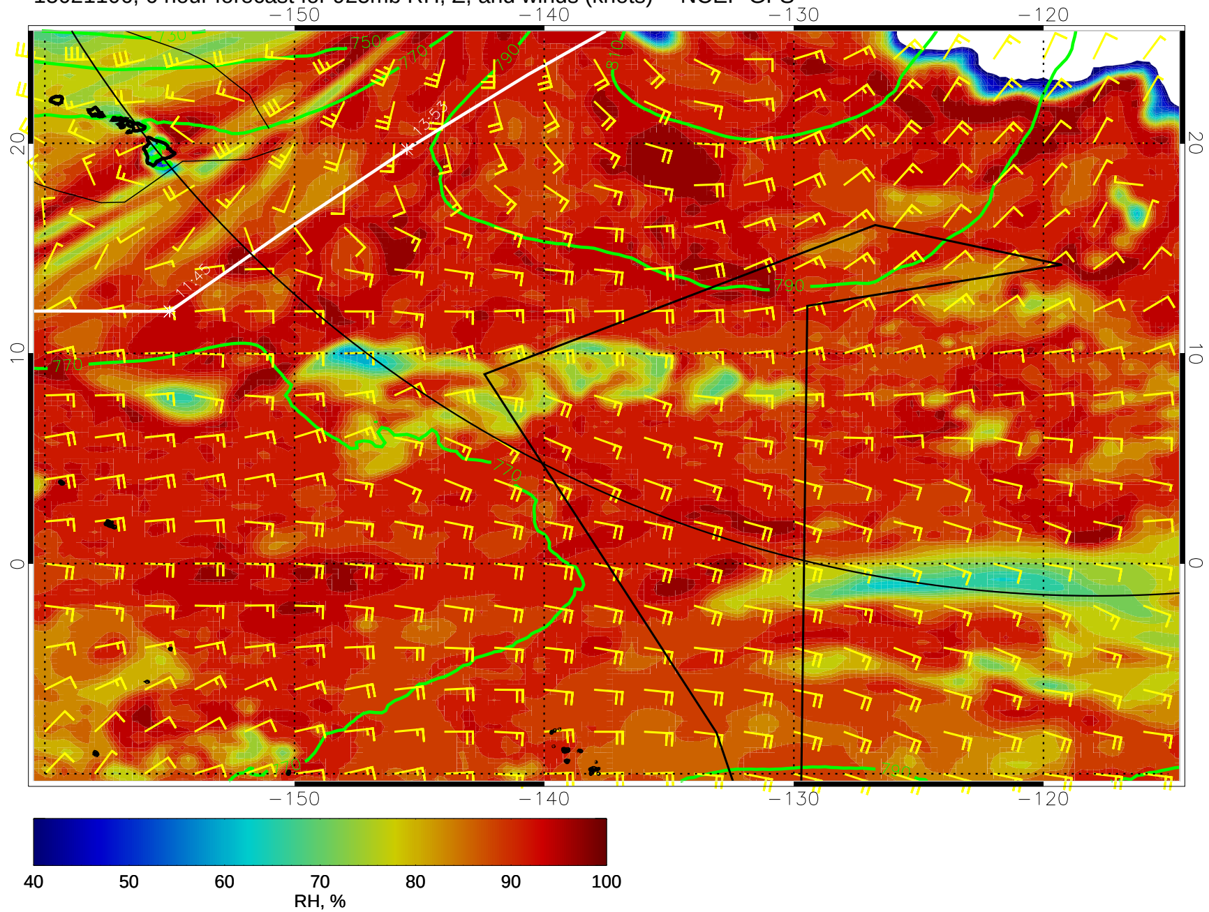
15021106, 6 hour forecast for 925mb RH, Z, and winds (knots) -- NCEP GFS
