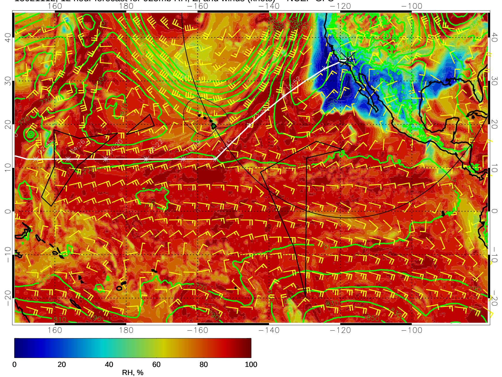
15021112, 12 hour forecast for 925mb RH, Z, and winds (knots) -- NCEP GFS
