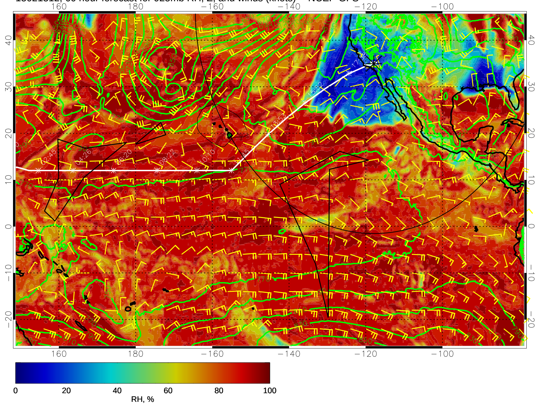
15021312, 60 hour forecast for 925mb RH, Z, and winds (knots) -- NCEP GFS
