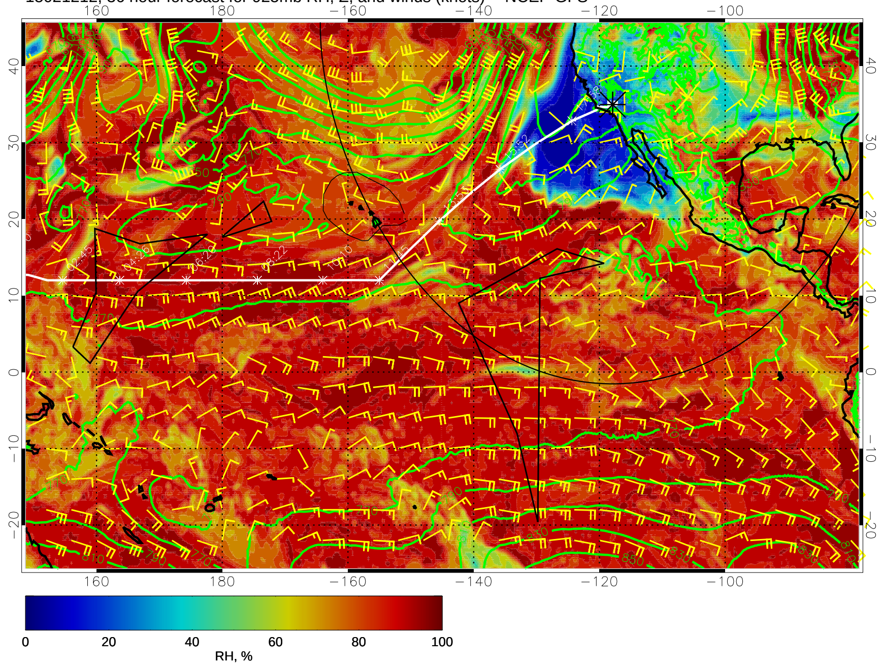
15021212, 36 hour forecast for 925mb RH, Z, and winds (knots) -- NCEP GFS
