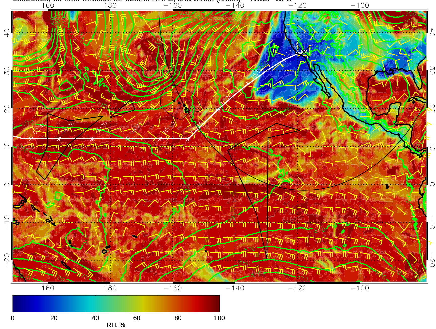
15021318, 66 hour forecast for 925mb RH, Z, and winds (knots) -- NCEP GFS
