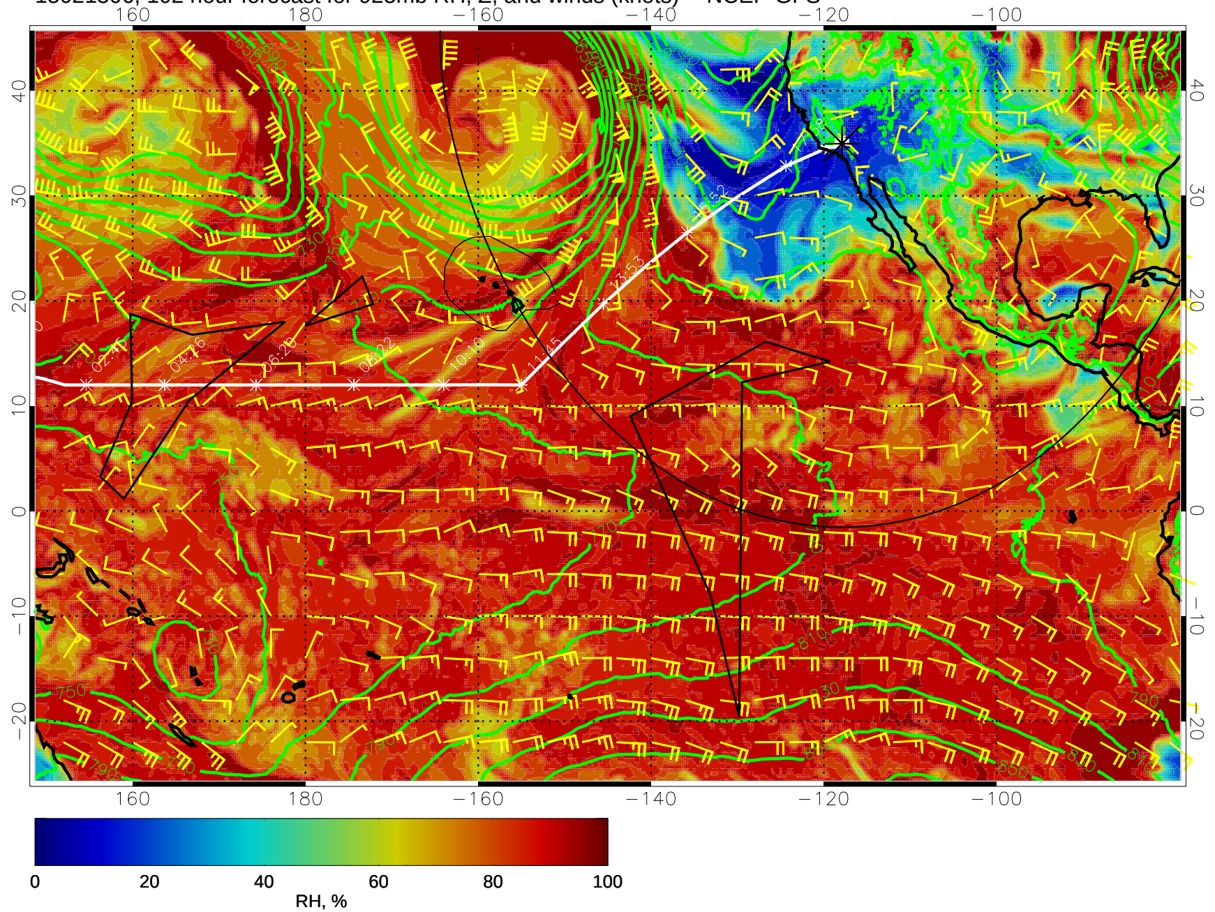
15021506, 102 hour forecast for 925mb RH, Z, and winds (knots) -- NCEP GFS
