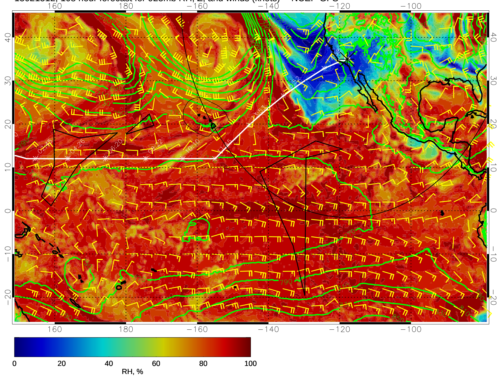
15021512, 108 hour forecast for 925mb RH, Z, and winds (knots) -- NCEP GFS
