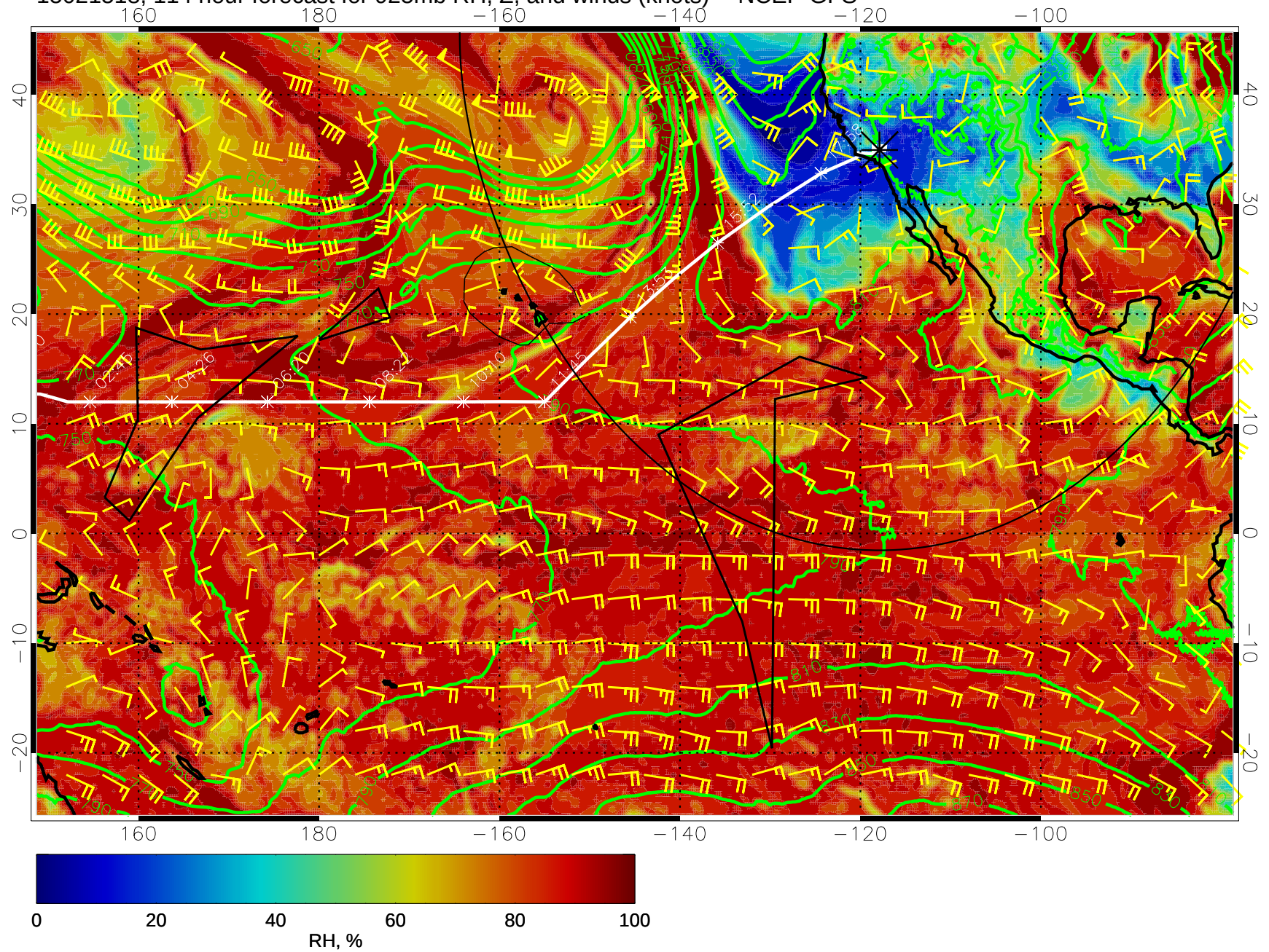
15021518, 114 hour forecast for 925mb RH, Z, and winds (knots) -- NCEP GFS
