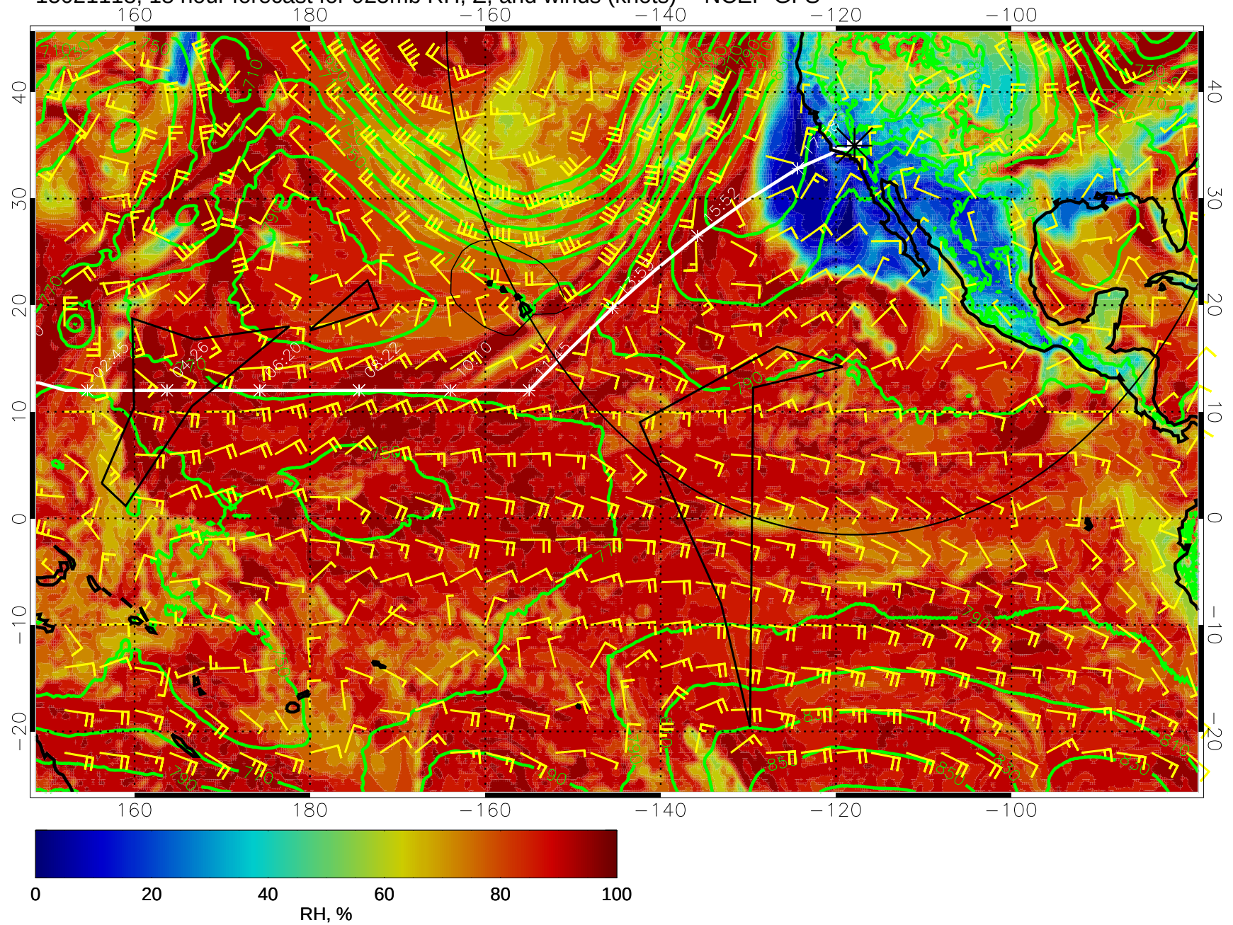
15021118, 18 hour forecast for 925mb RH, Z, and winds (knots) -- NCEP GFS
