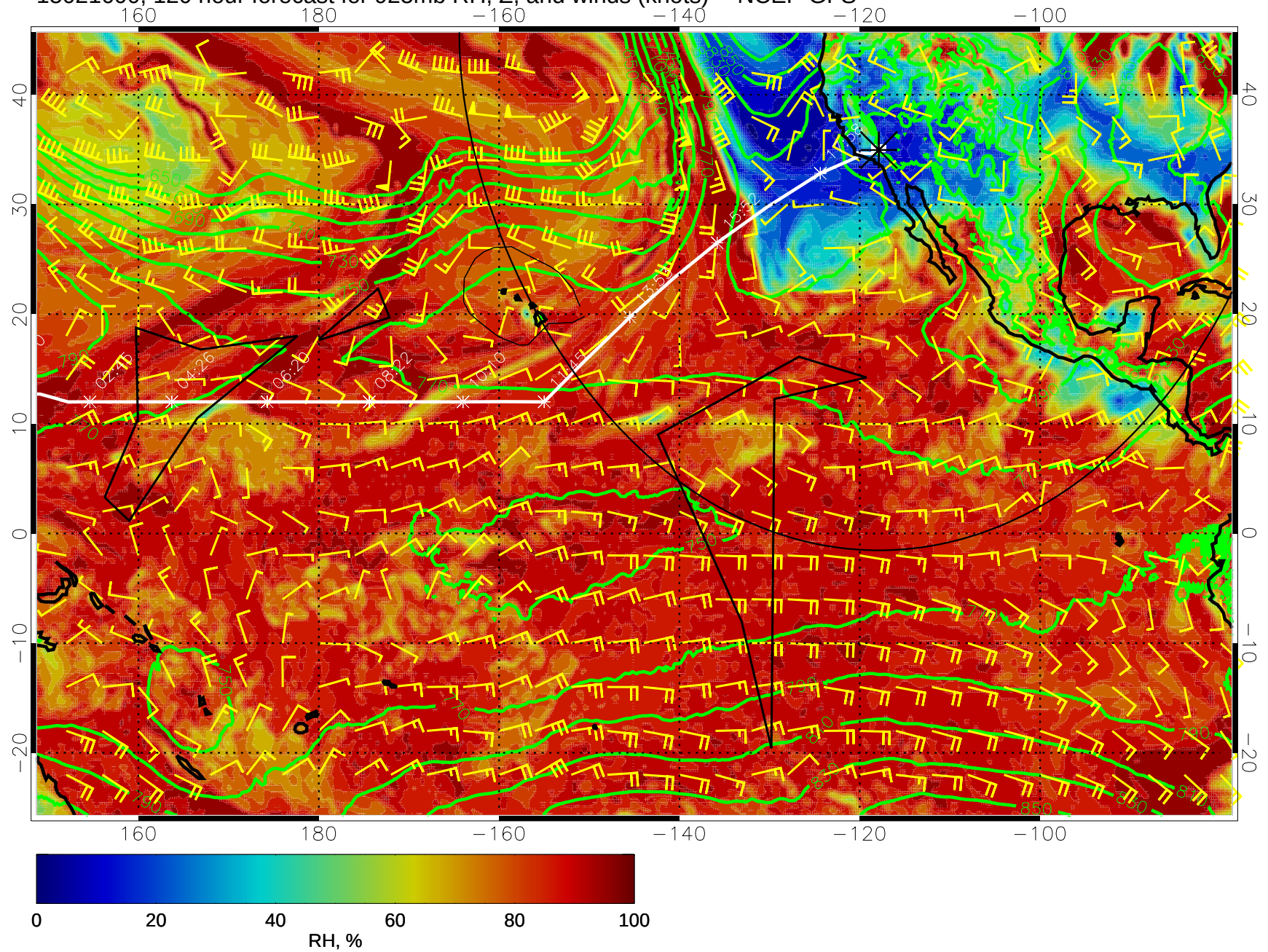
15021600, 120 hour forecast for 925mb RH, Z, and winds (knots) -- NCEP GFS
