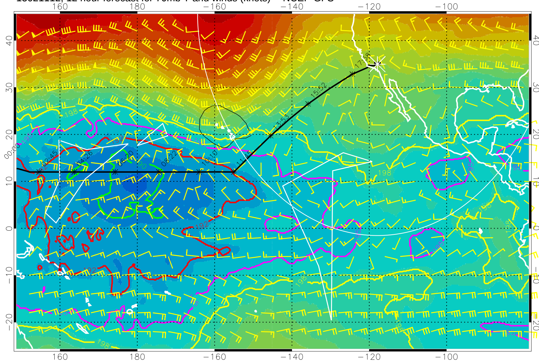
15021112, 12 hour forecast for 70mb T and winds (knots) -- NCEP GFS
