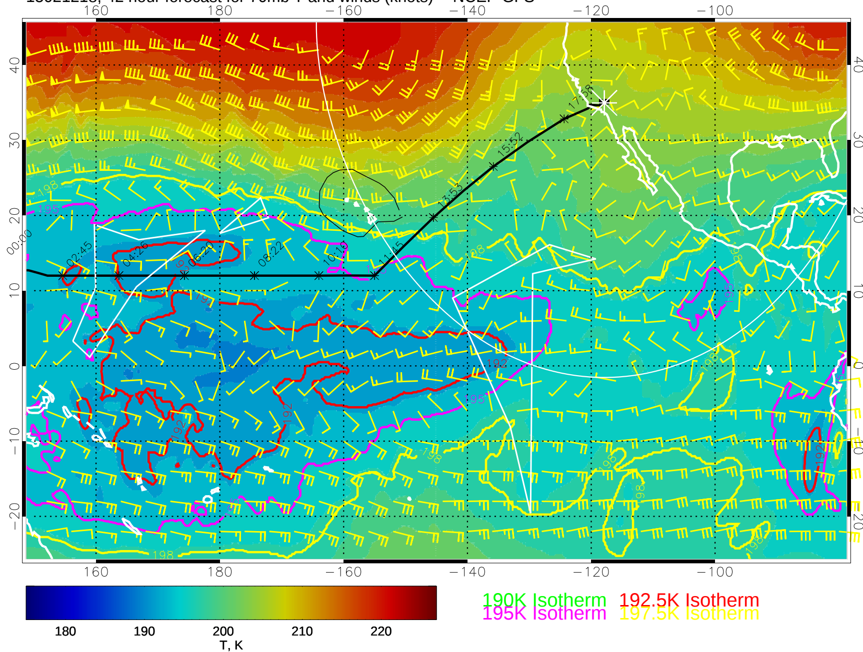
15021218, 42 hour forecast for 70mb T and winds (knots) -- NCEP GFS
