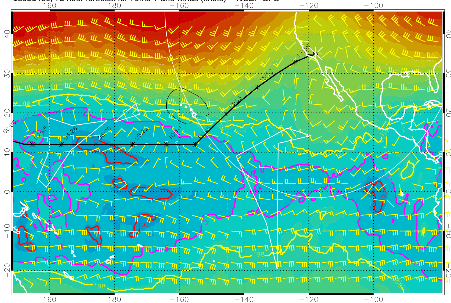
15021400, 72 hour forecast for 70mb T and winds (knots) -- NCEP GFS
