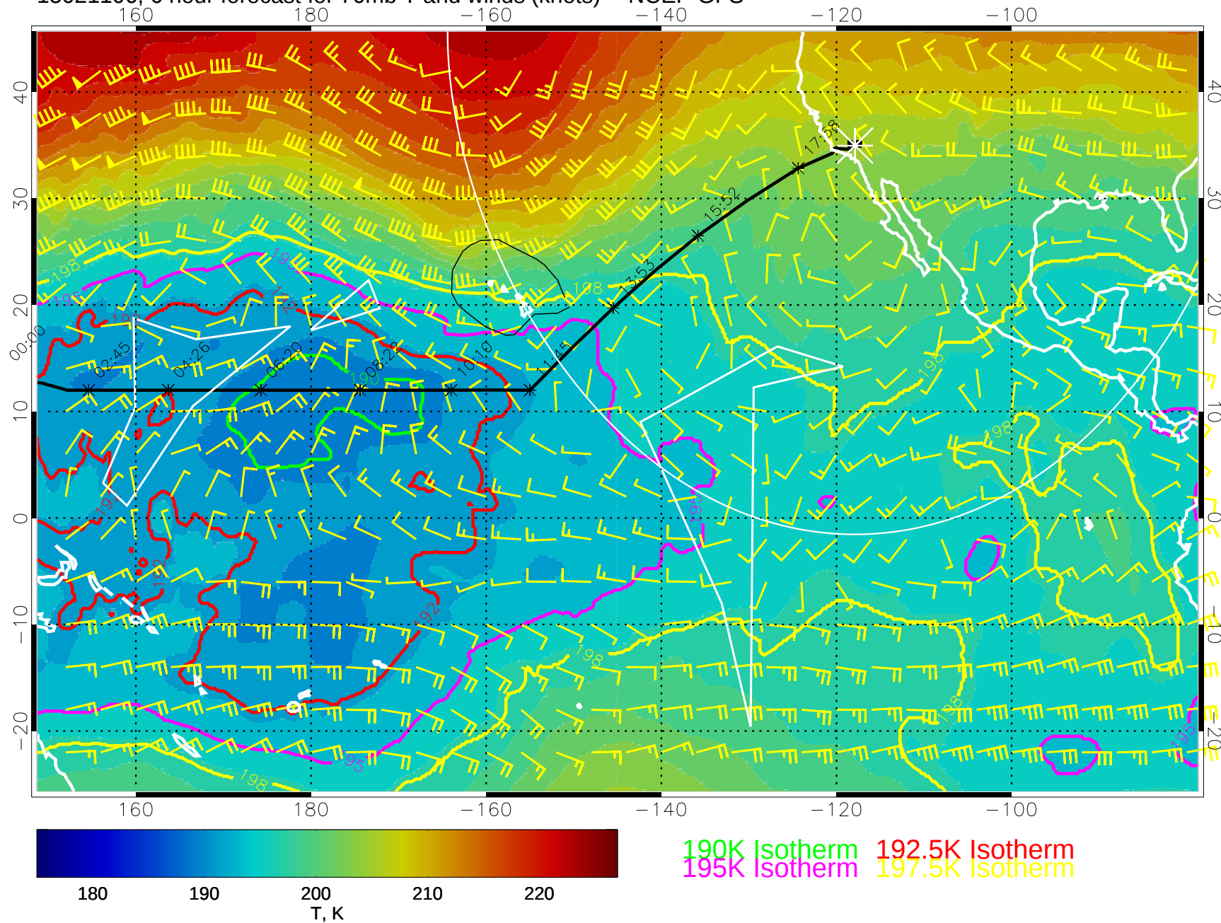
15021106, 6 hour forecast for 70mb T and winds (knots) -- NCEP GFS
