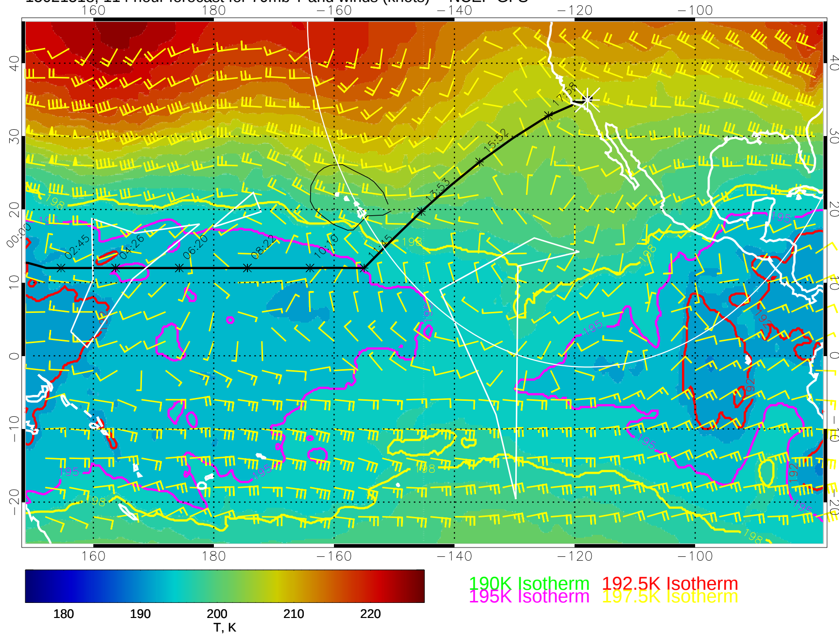
15021518, 114 hour forecast for 70mb T and winds (knots) -- NCEP GFS
