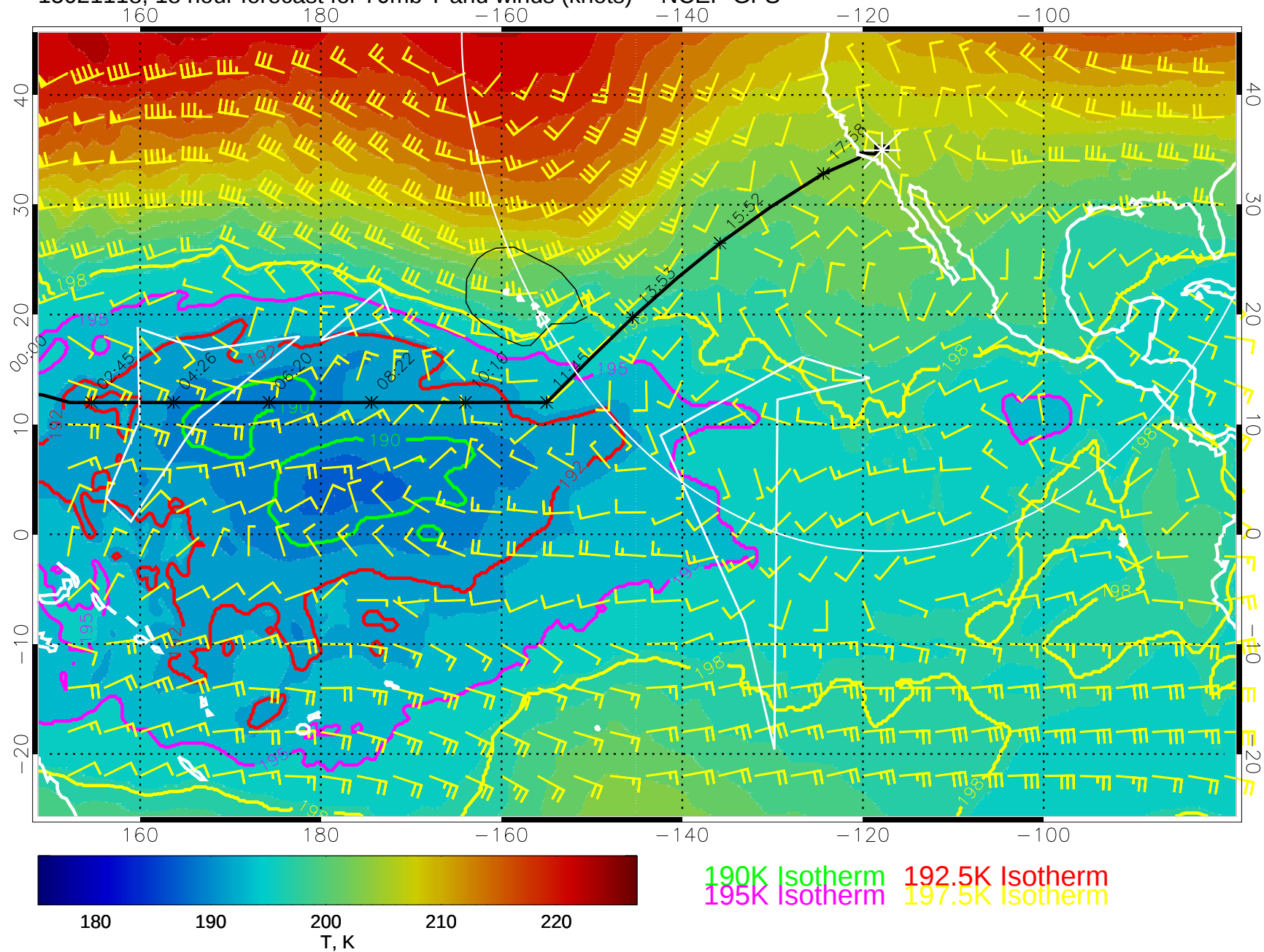
15021118, 18 hour forecast for 70mb T and winds (knots) -- NCEP GFS
