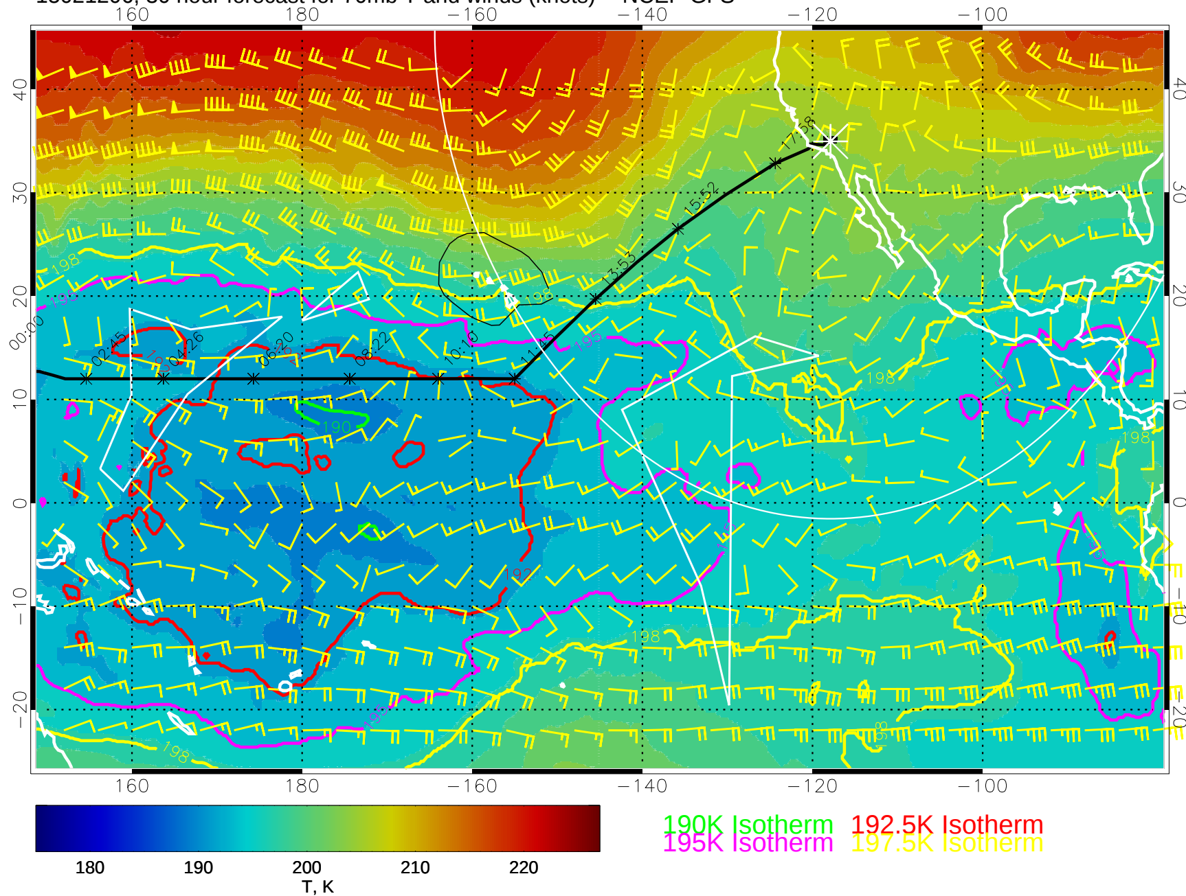
15021206, 30 hour forecast for 70mb T and winds (knots) -- NCEP GFS
