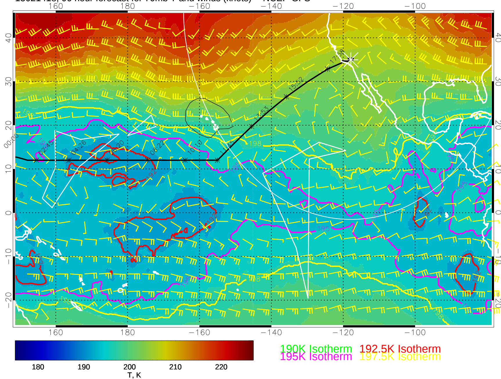
15021418, 90 hour forecast for 70mb T and winds (knots) -- NCEP GFS
