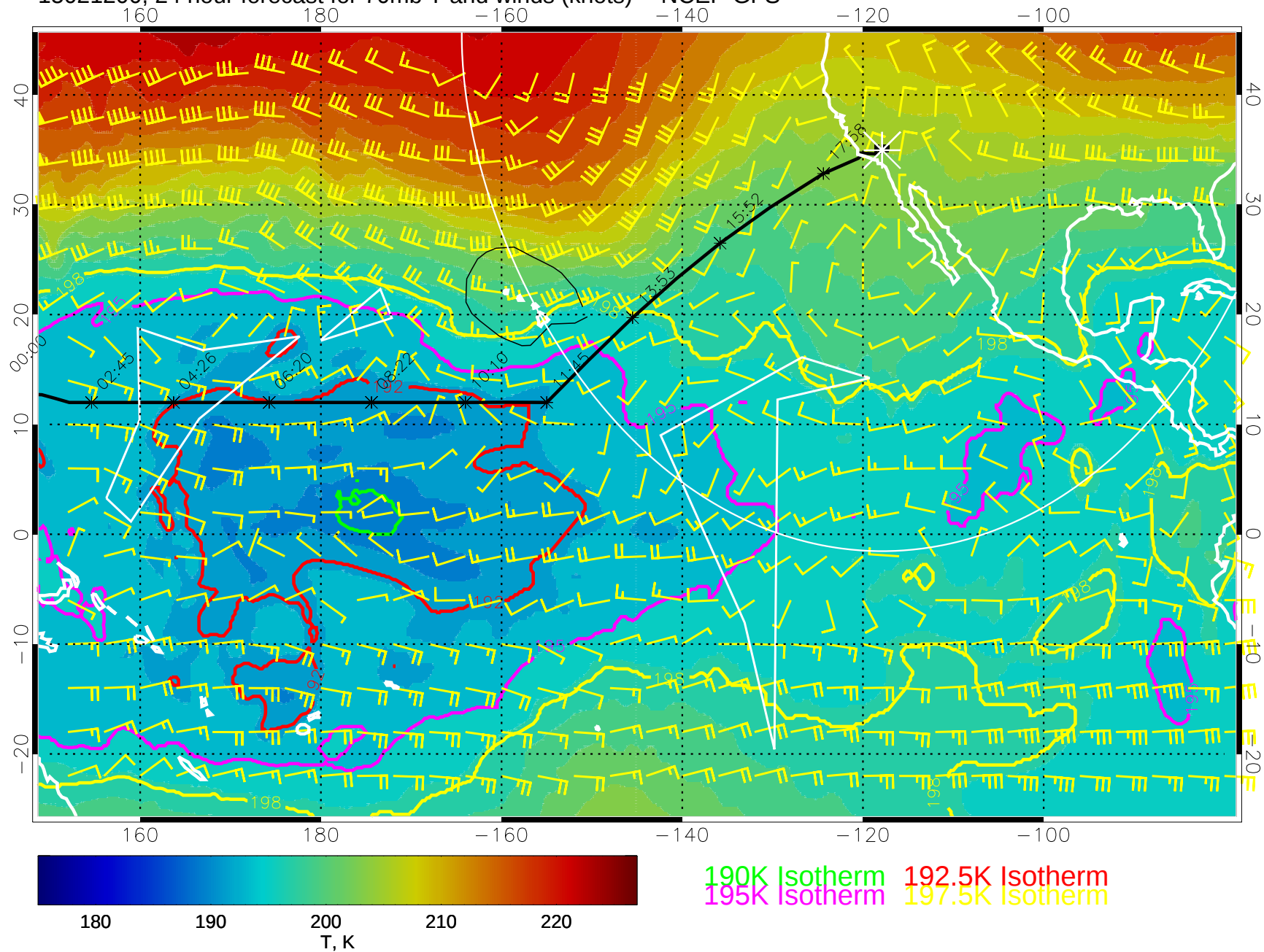
15021200, 24 hour forecast for 70mb T and winds (knots) -- NCEP GFS
