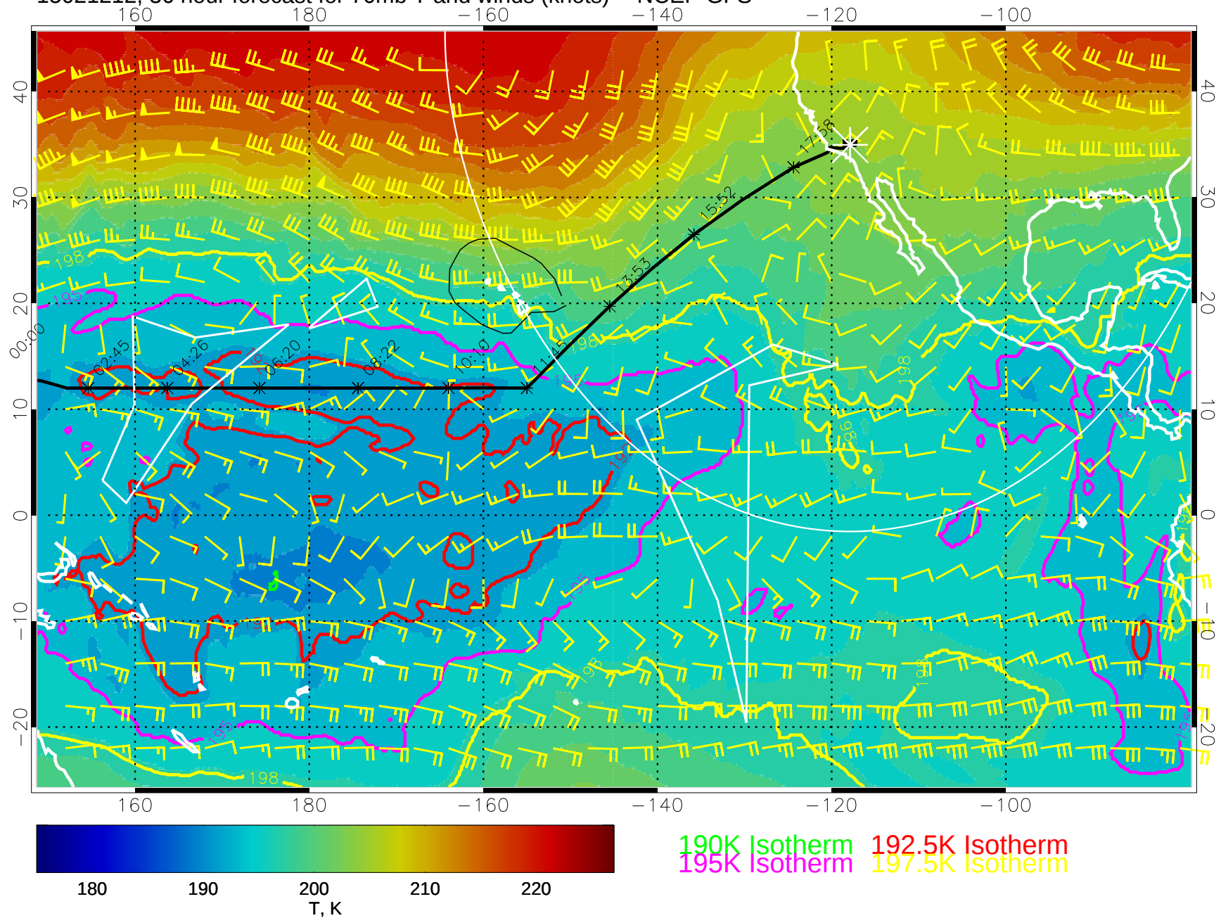
15021212, 36 hour forecast for 70mb T and winds (knots) -- NCEP GFS
