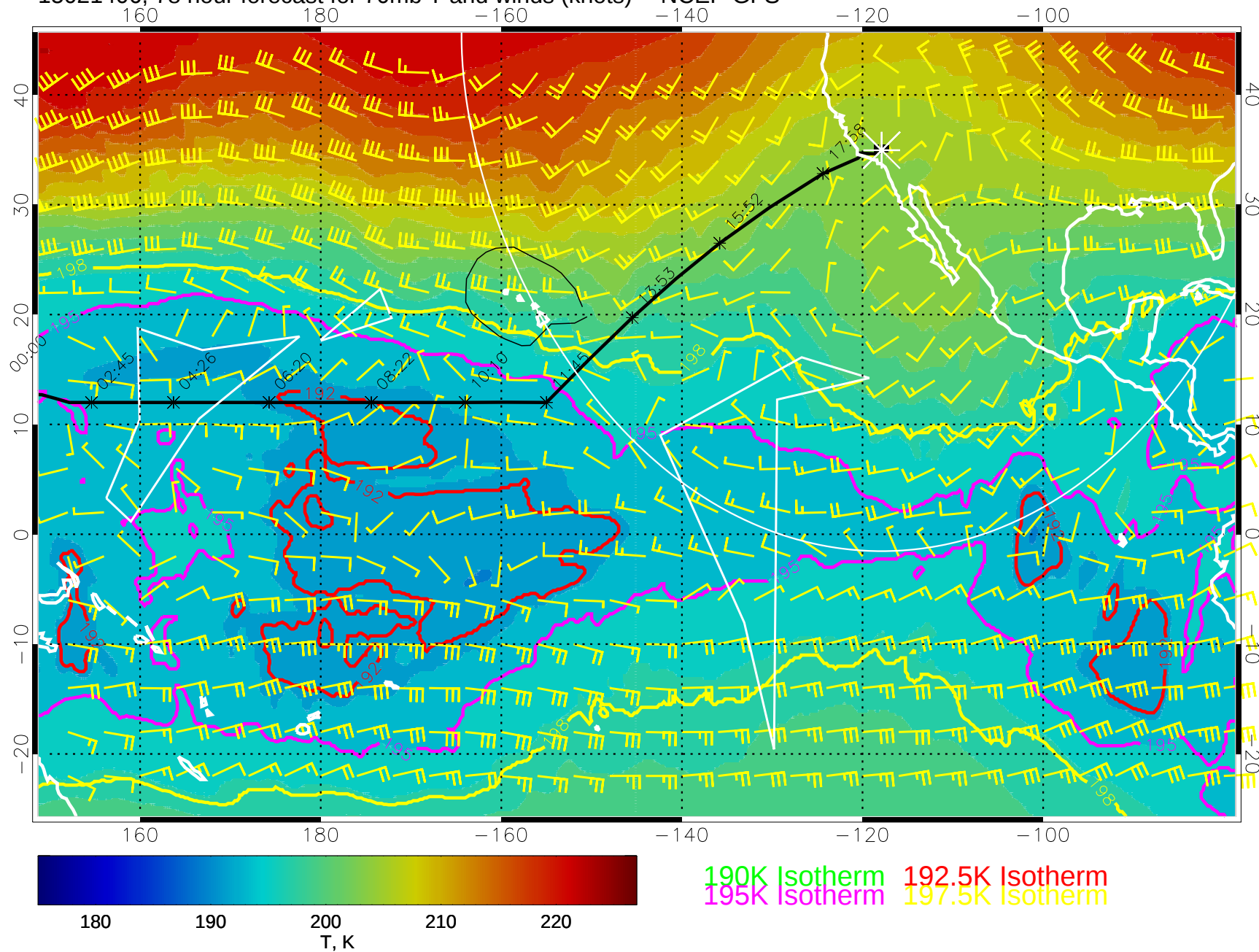
15021406, 78 hour forecast for 70mb T and winds (knots) -- NCEP GFS
