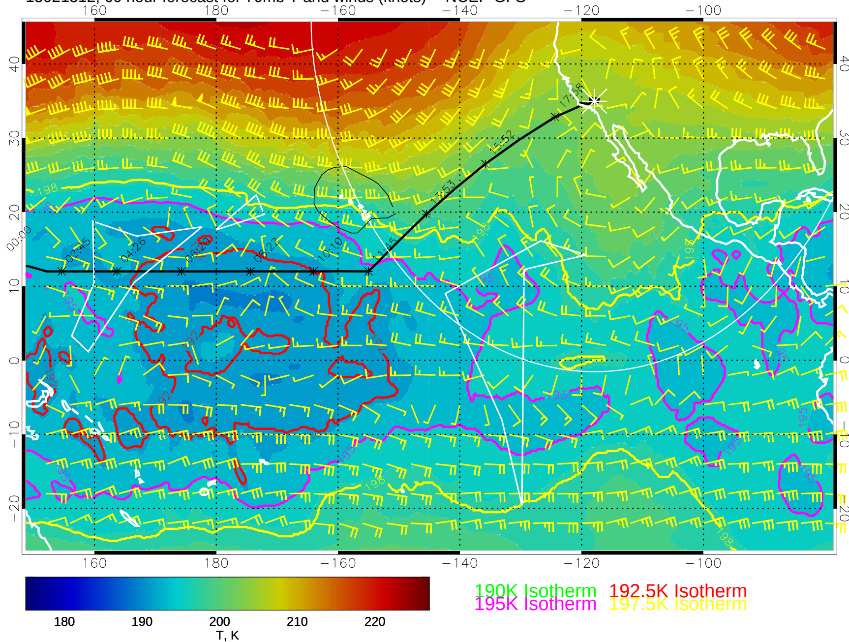
15021312, 60 hour forecast for 70mb T and winds (knots) -- NCEP GFS
