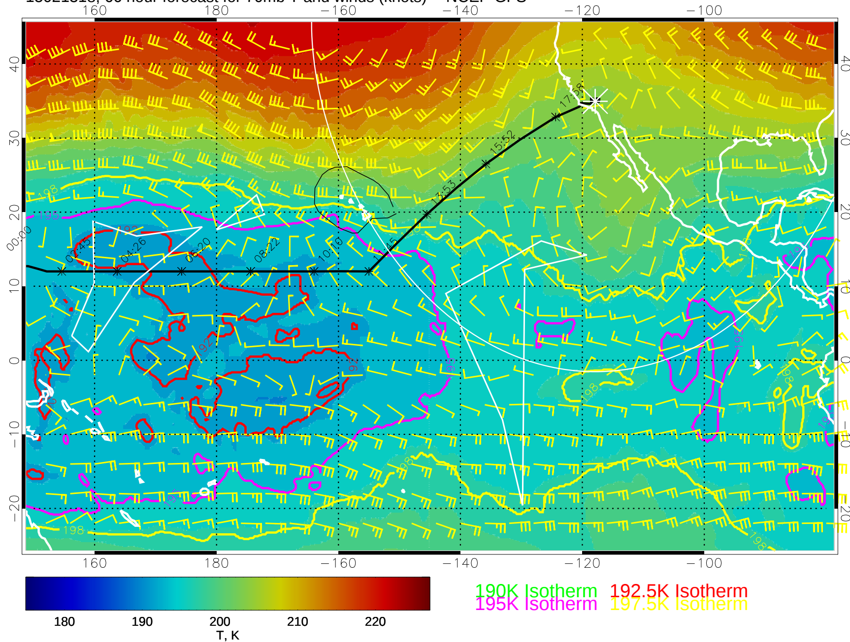
15021318, 66 hour forecast for 70mb T and winds (knots) -- NCEP GFS
