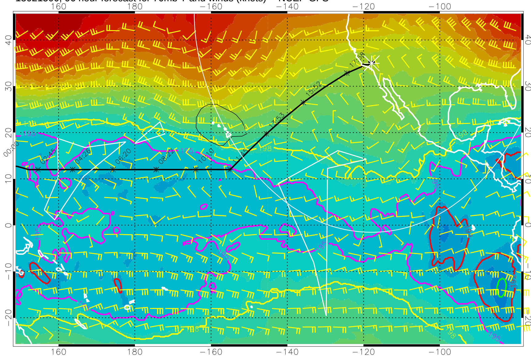
15021500, 96 hour forecast for 70mb T and winds (knots) -- NCEP GFS
