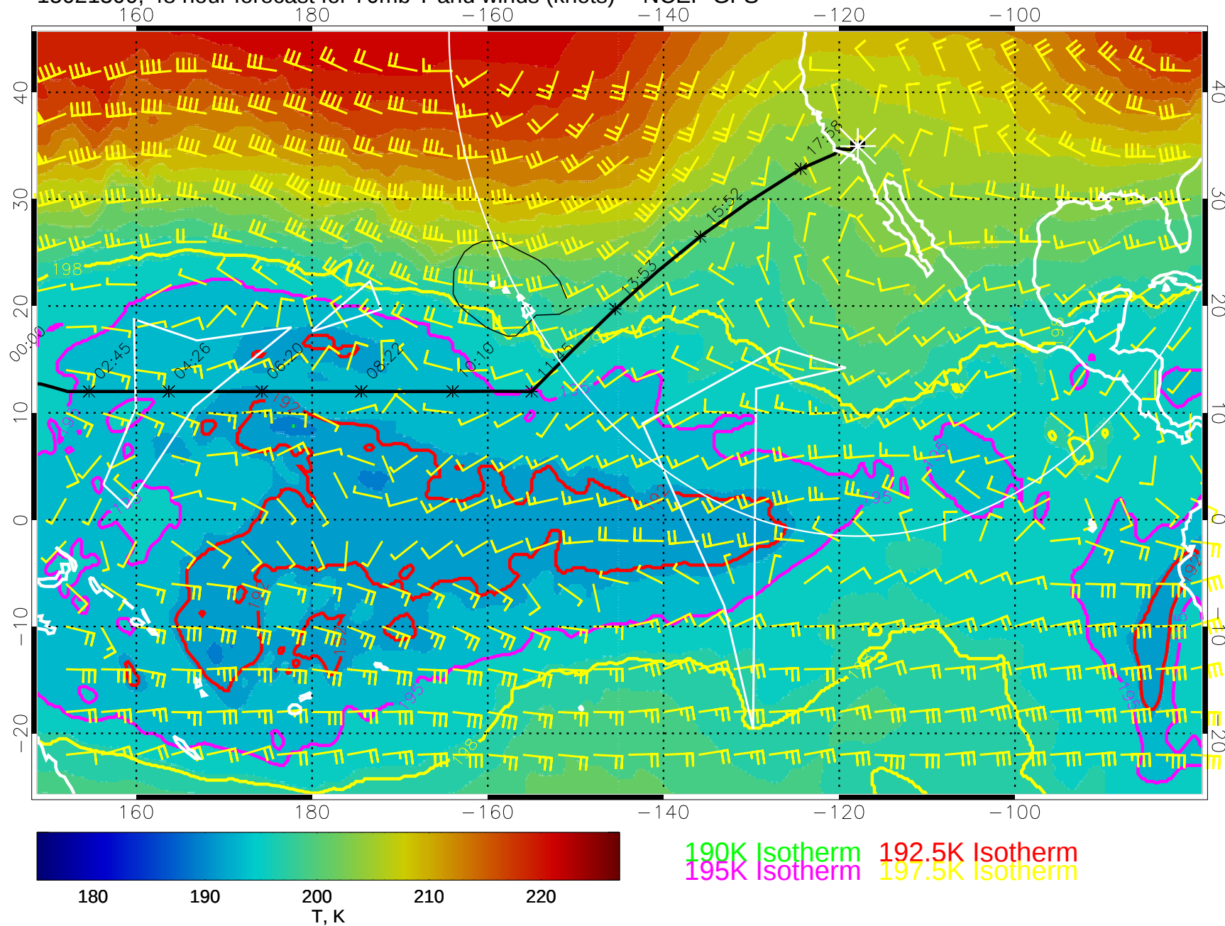
15021300, 48 hour forecast for 70mb T and winds (knots) -- NCEP GFS
