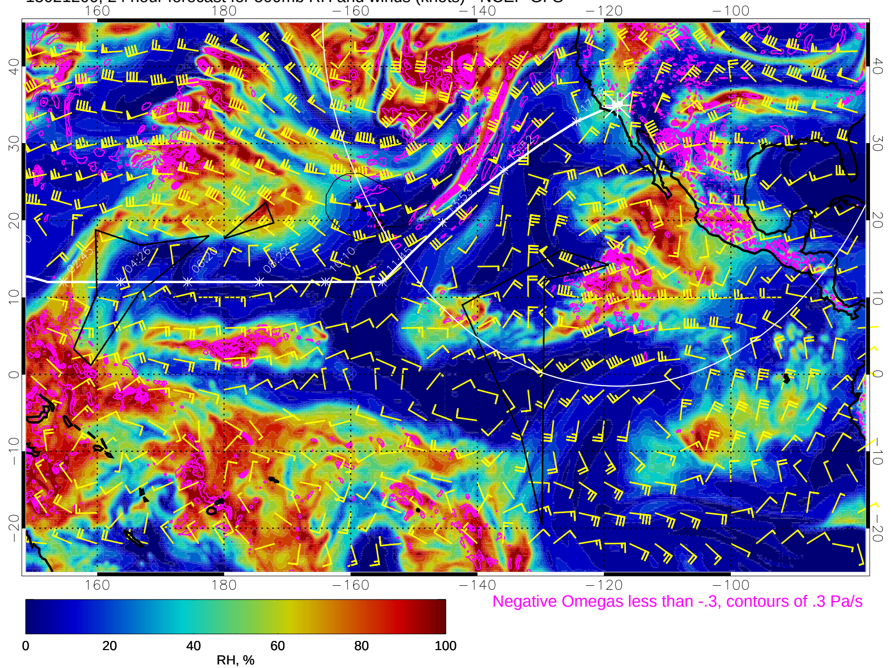
15021200, 24 hour forecast for 500mb RH and winds (knots) - NCEP GFS
