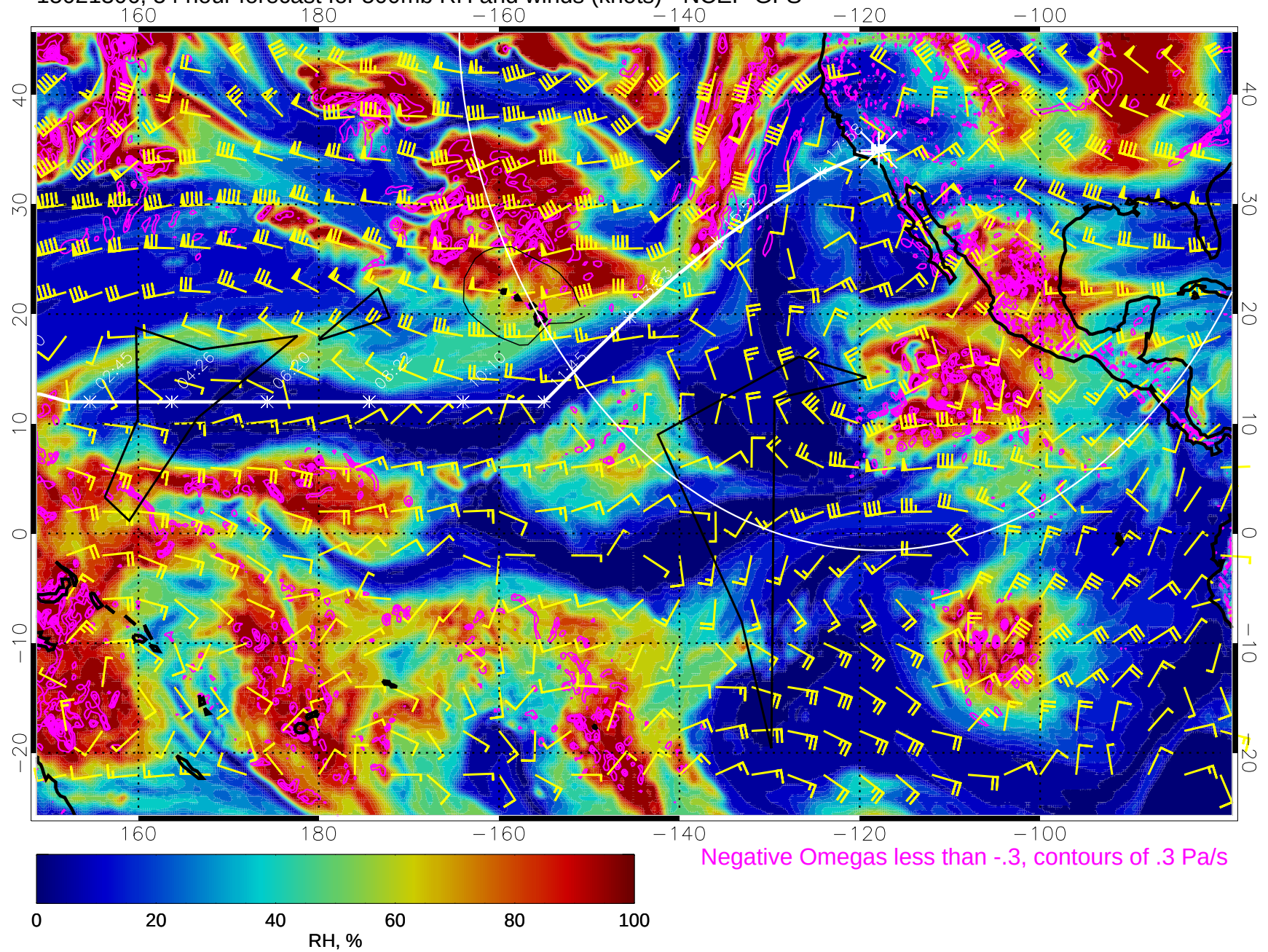
15021306, 54 hour forecast for 500mb RH and winds (knots) - NCEP GFS
