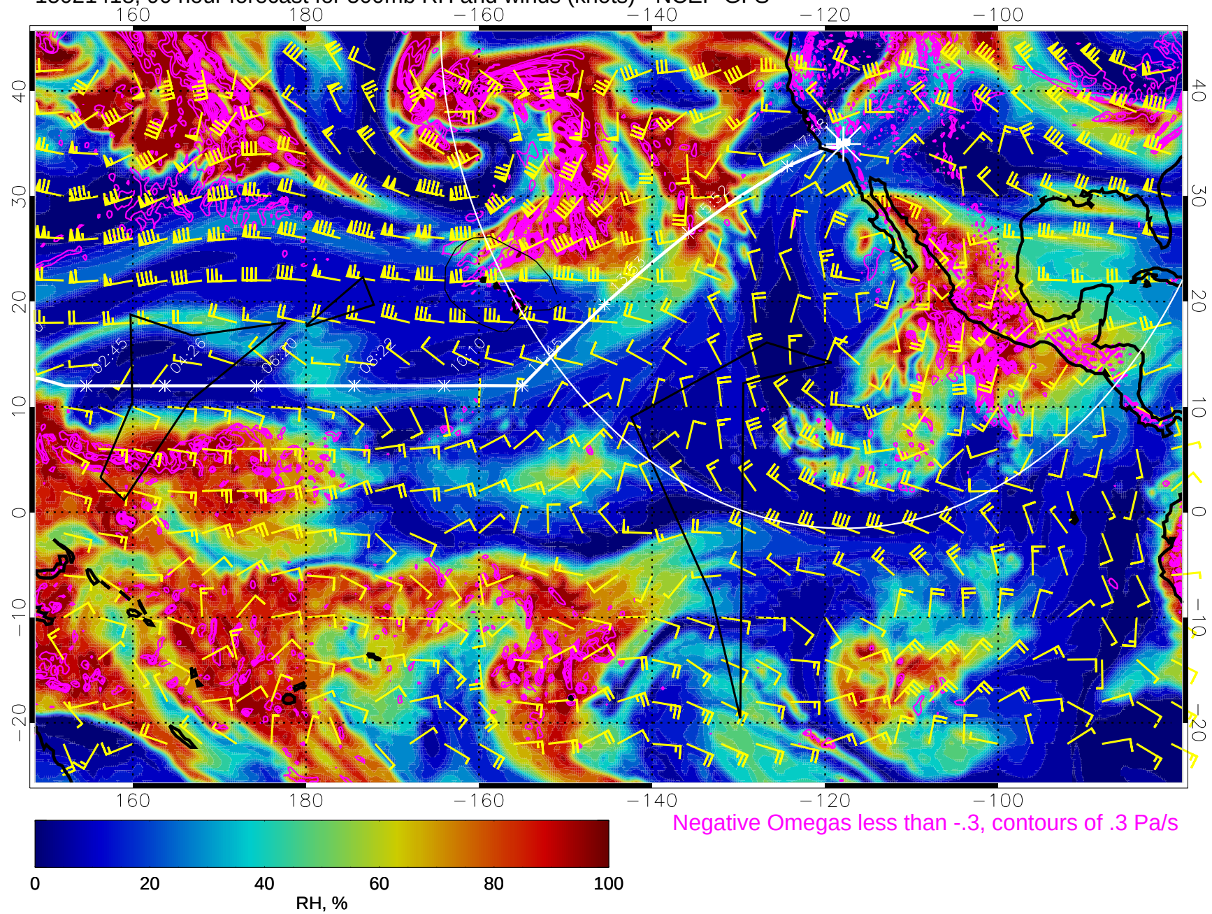
15021418, 90 hour forecast for 500mb RH and winds (knots) - NCEP GFS
