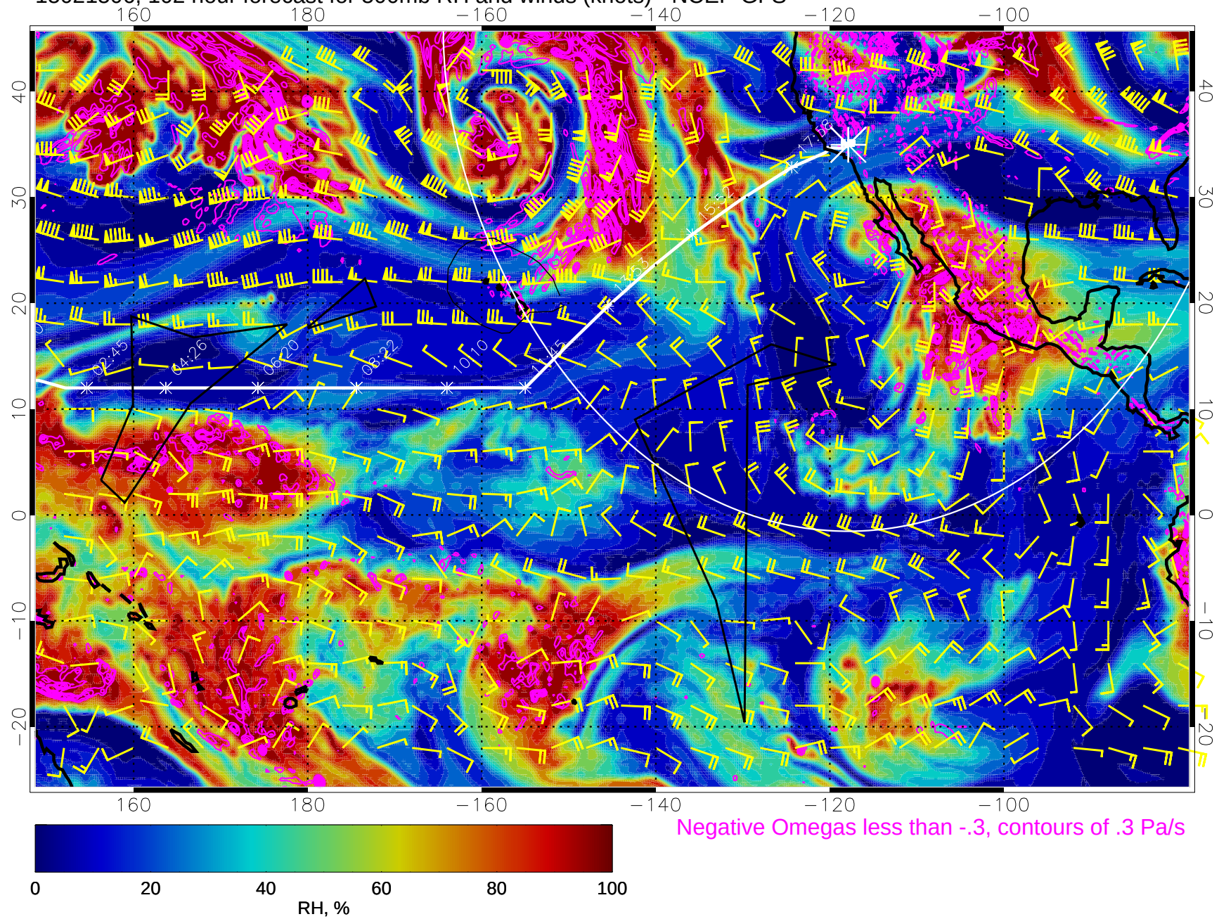
15021506, 102 hour forecast for 500mb RH and winds (knots) - NCEP GFS
