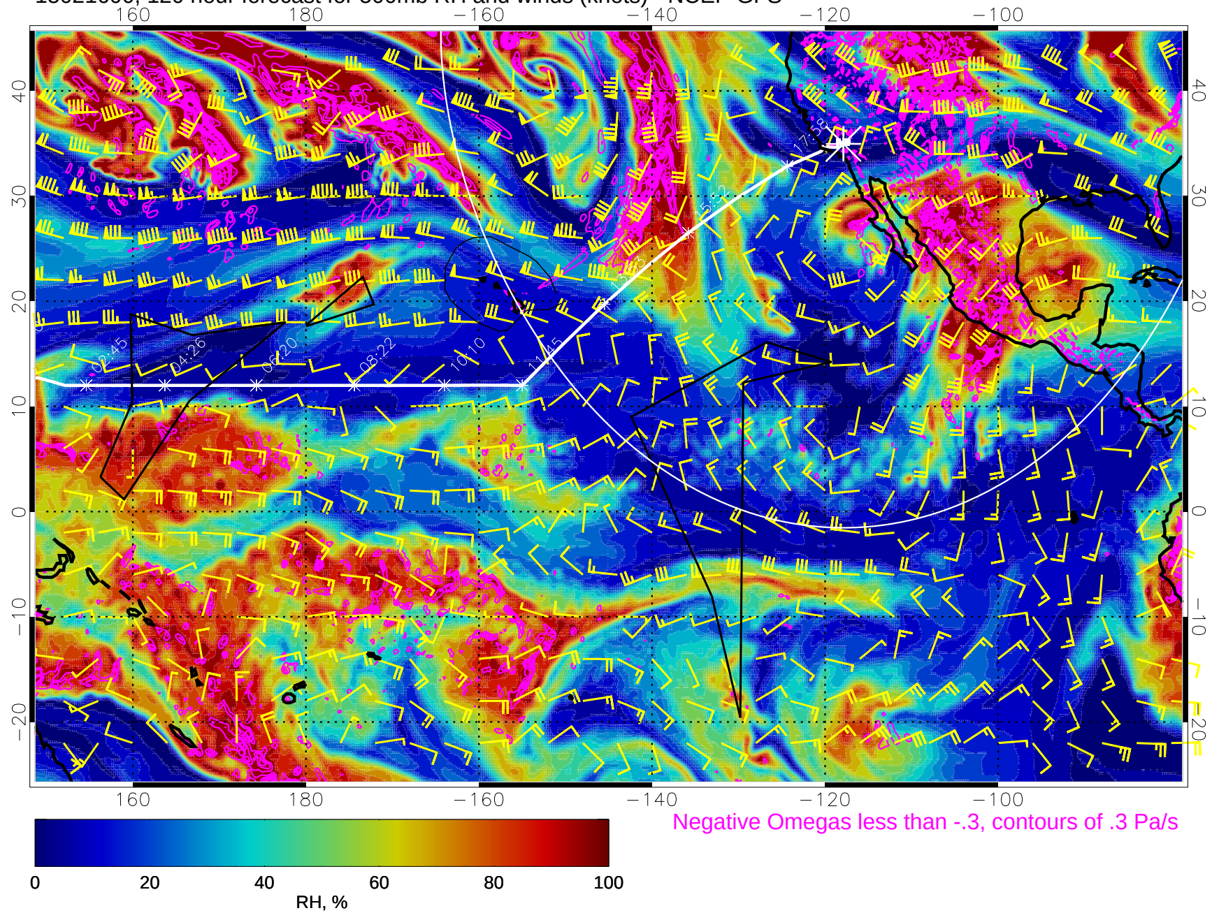
15021600, 120 hour forecast for 500mb RH and winds (knots) - NCEP GFS
