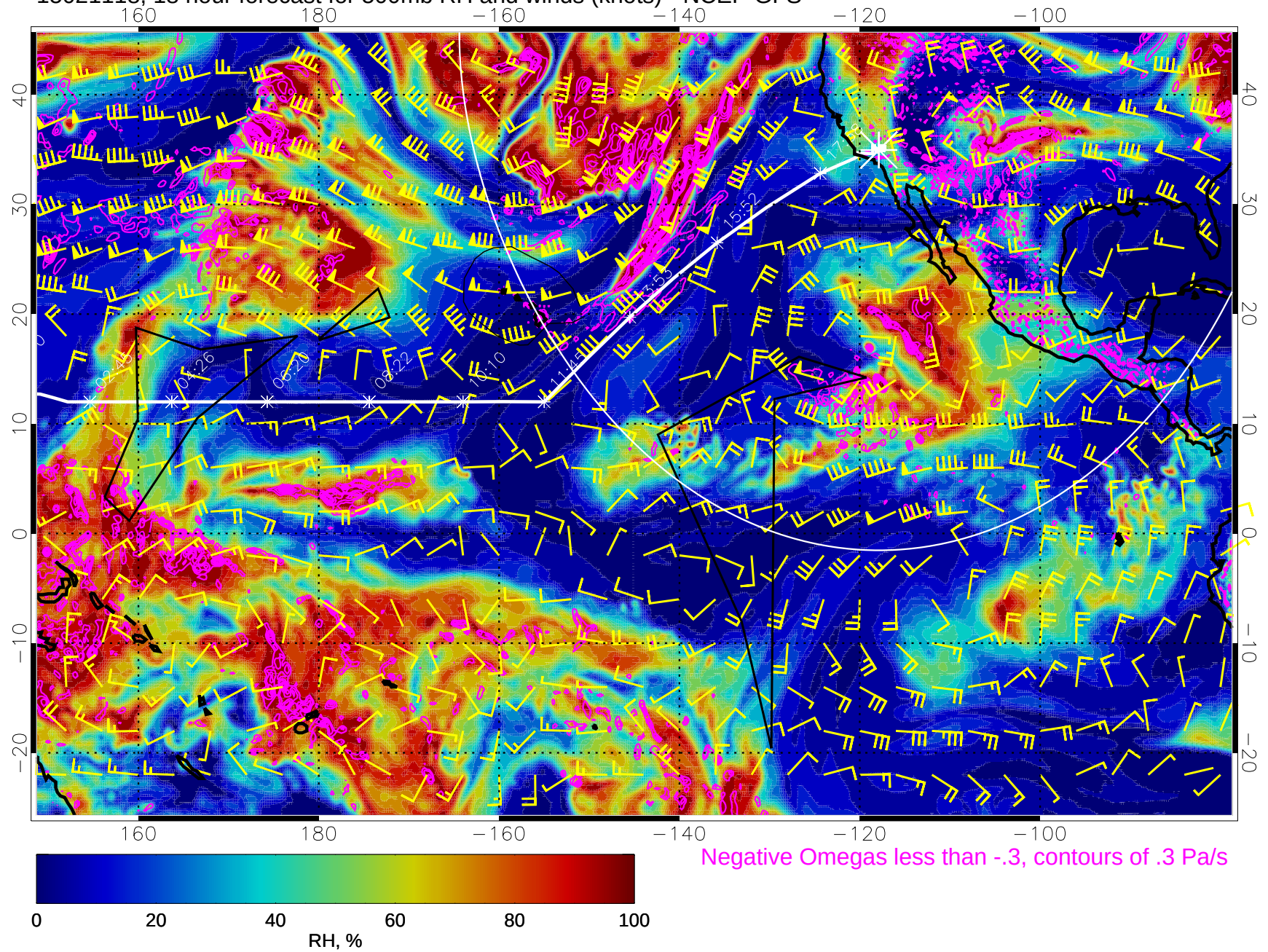
15021118, 18 hour forecast for 500mb RH and winds (knots) - NCEP GFS
