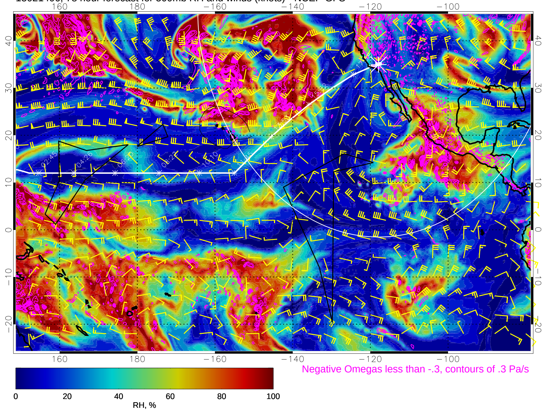
15021406, 78 hour forecast for 500mb RH and winds (knots) - NCEP GFS
