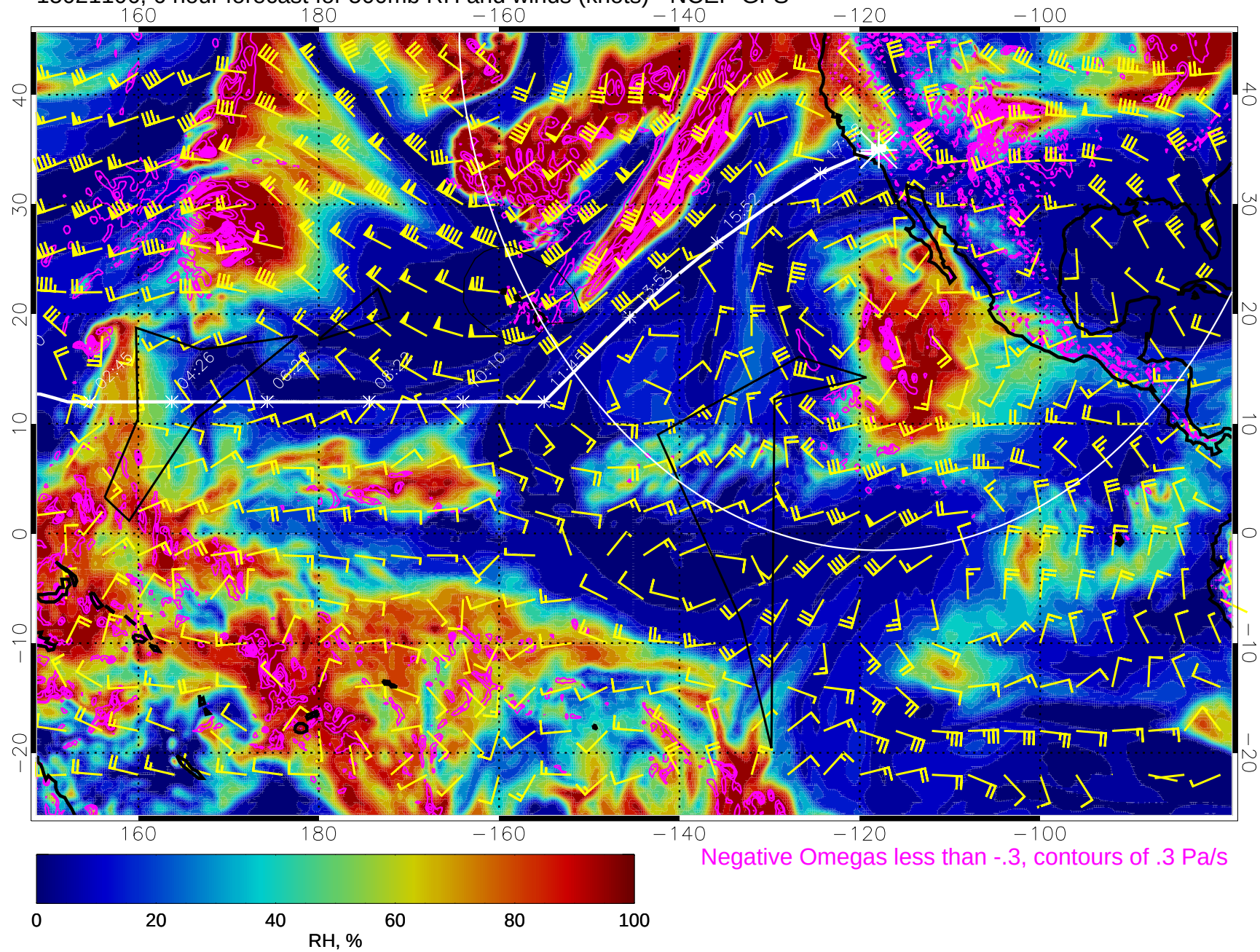
15021106, 6 hour forecast for 500mb RH and winds (knots) - NCEP GFS
