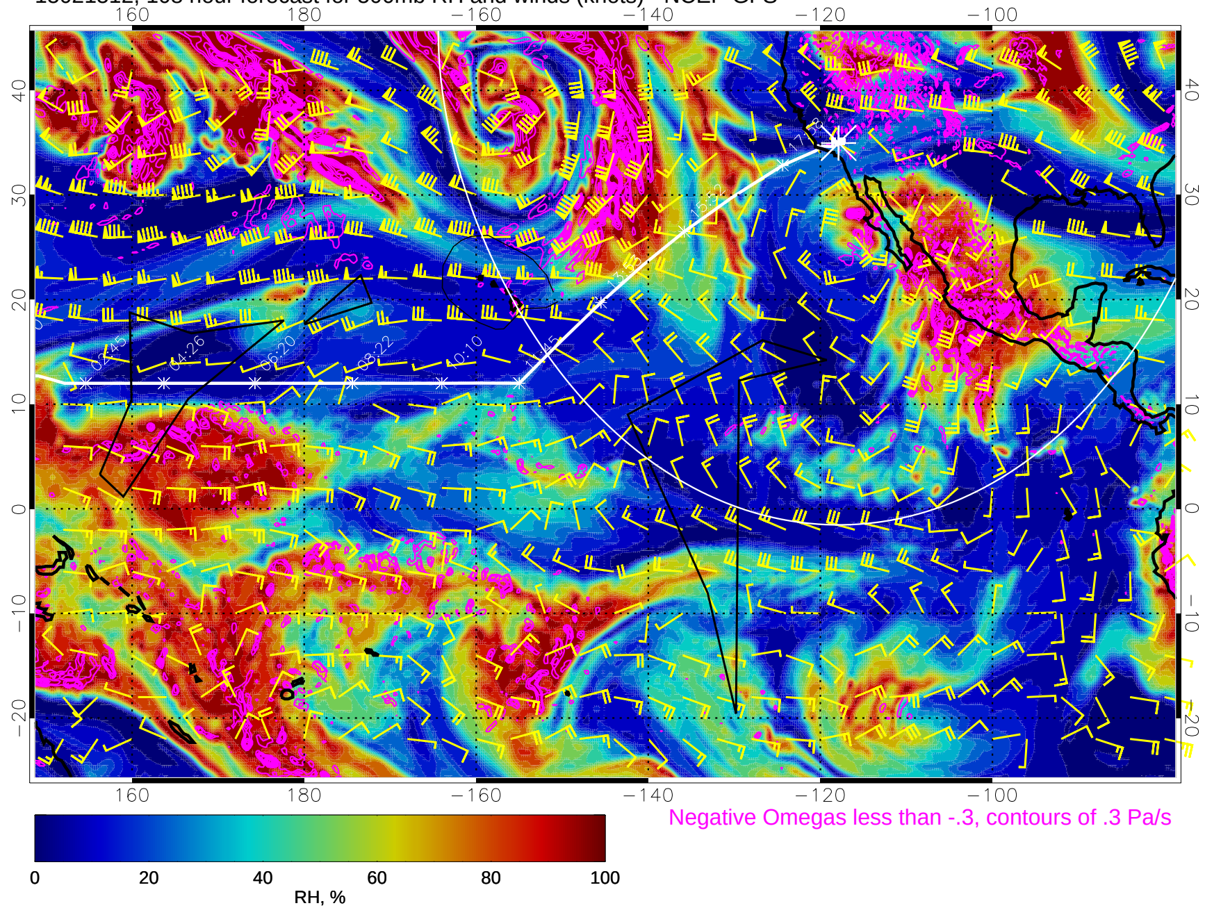
15021512, 108 hour forecast for 500mb RH and winds (knots) - NCEP GFS
