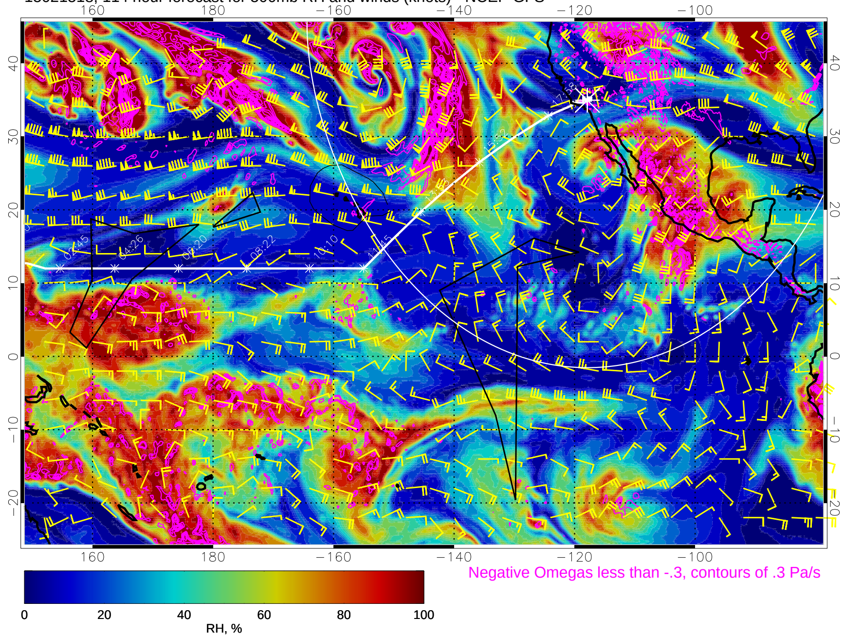
15021518, 114 hour forecast for 500mb RH and winds (knots) - NCEP GFS
