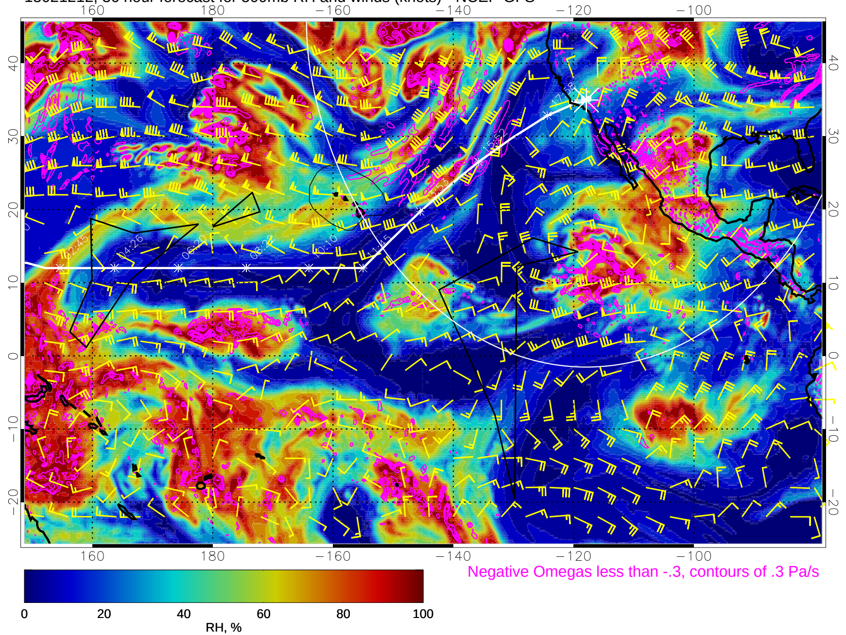
15021212, 36 hour forecast for 500mb RH and winds (knots) - NCEP GFS
