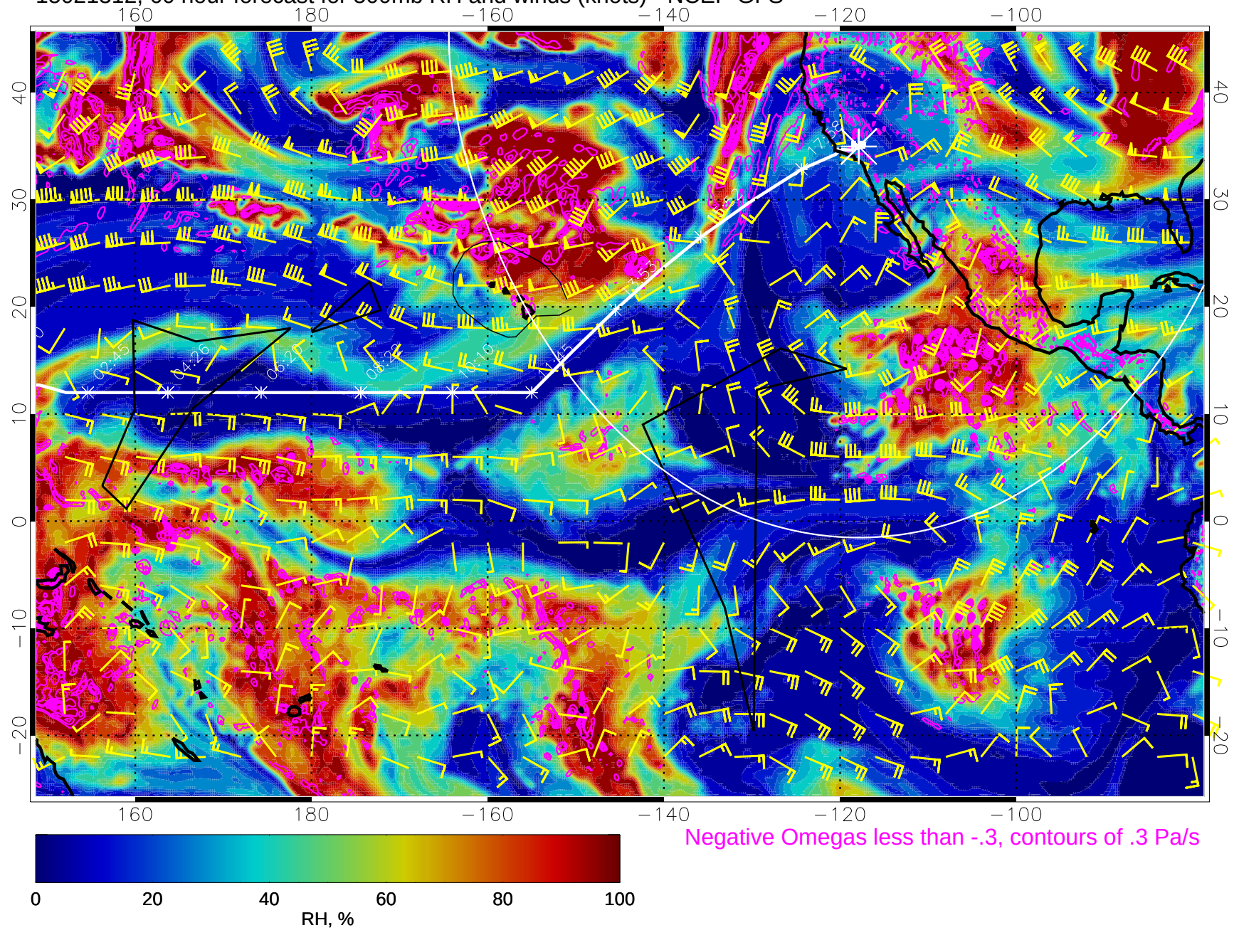
15021312, 60 hour forecast for 500mb RH and winds (knots) - NCEP GFS
