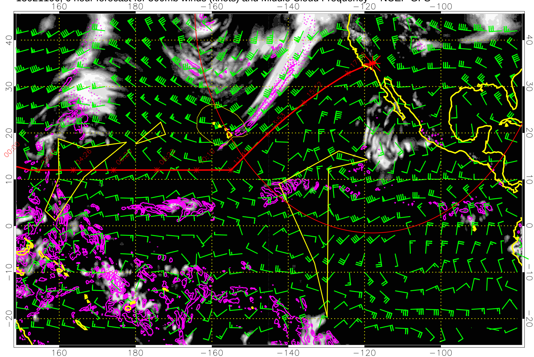
15021106, 6 hour forecast for 500mb winds (knots) and Middle Cloud Frequency -- NCEP GFS
