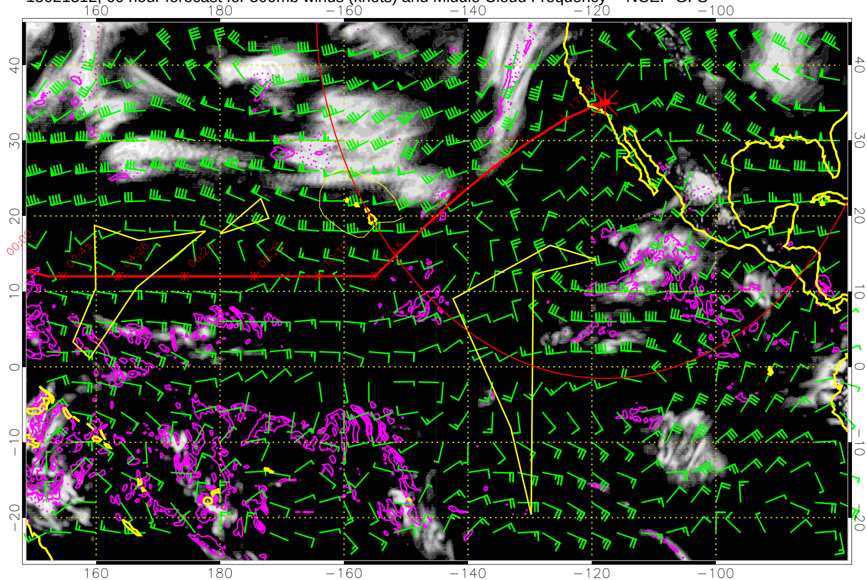
15021312, 60 hour forecast for 500mb winds (knots) and Middle Cloud Frequency -- NCEP GFS
