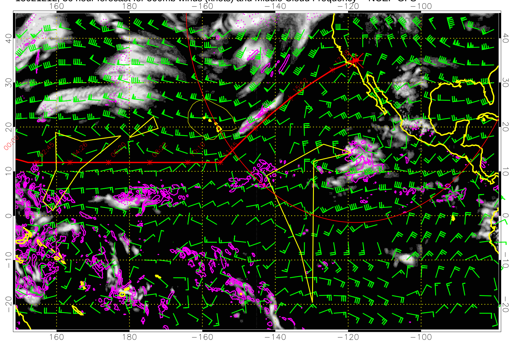
15021212, 36 hour forecast for 500mb winds (knots) and Middle Cloud Frequency -- NCEP GFS
