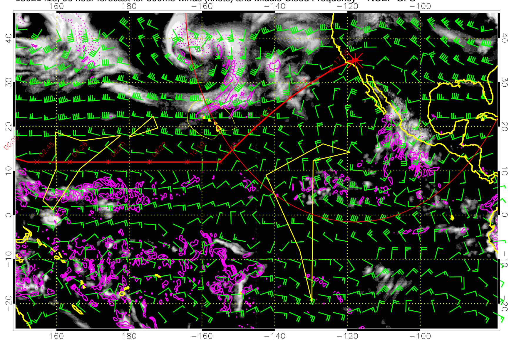
15021418, 90 hour forecast for 500mb winds (knots) and Middle Cloud Frequency -- NCEP GFS
