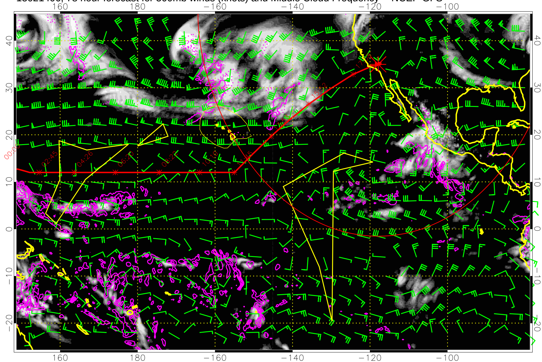
15021406, 78 hour forecast for 500mb winds (knots) and Middle Cloud Frequency -- NCEP GFS
