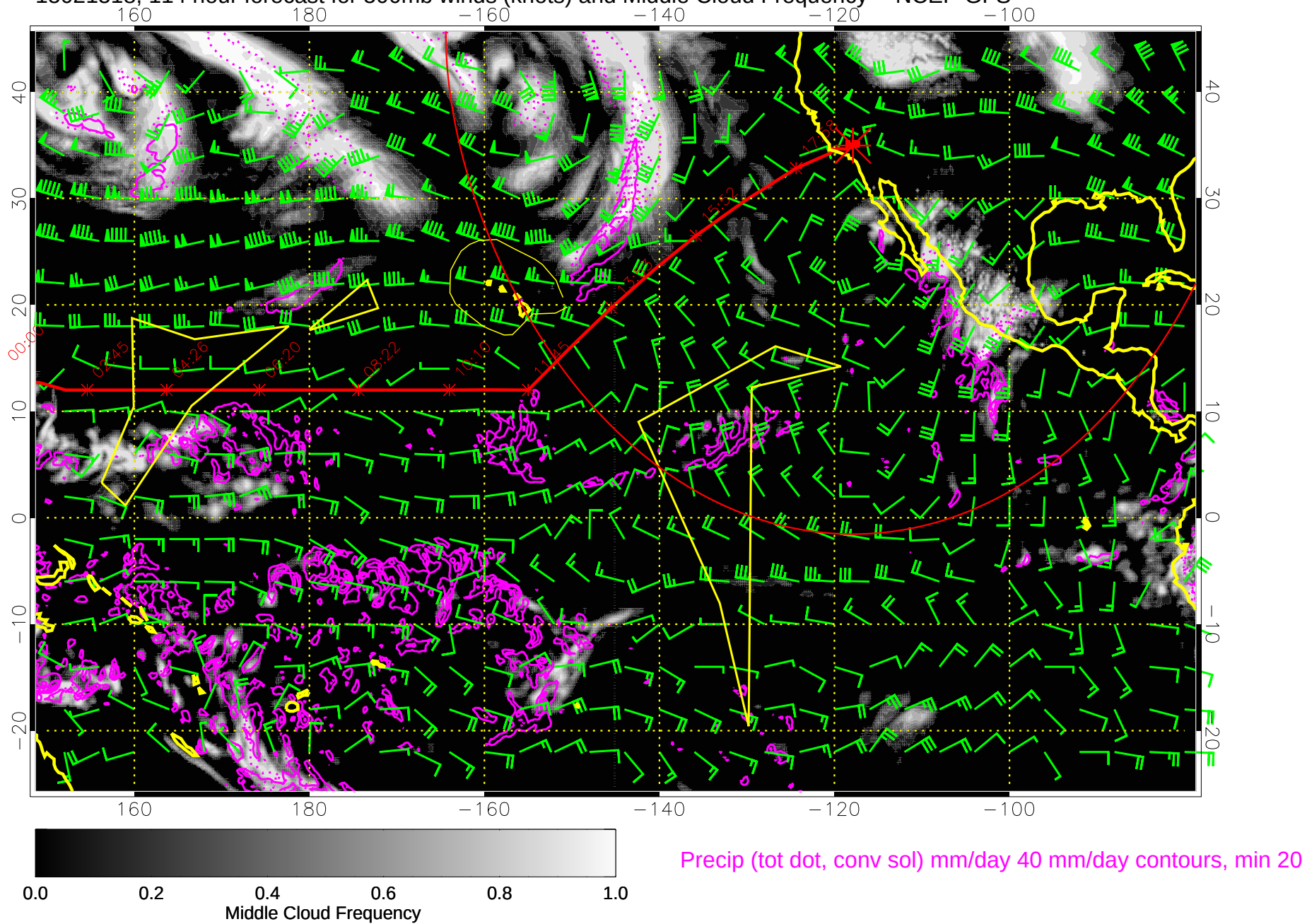
15021518, 114 hour forecast for 500mb winds (knots) and Middle Cloud Frequency -- NCEP GFS
