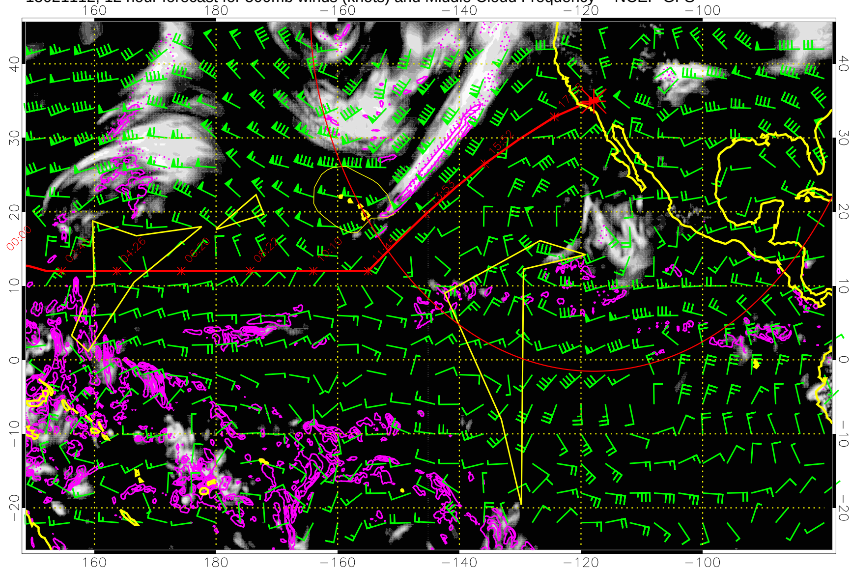
15021112, 12 hour forecast for 500mb winds (knots) and Middle Cloud Frequency -- NCEP GFS
