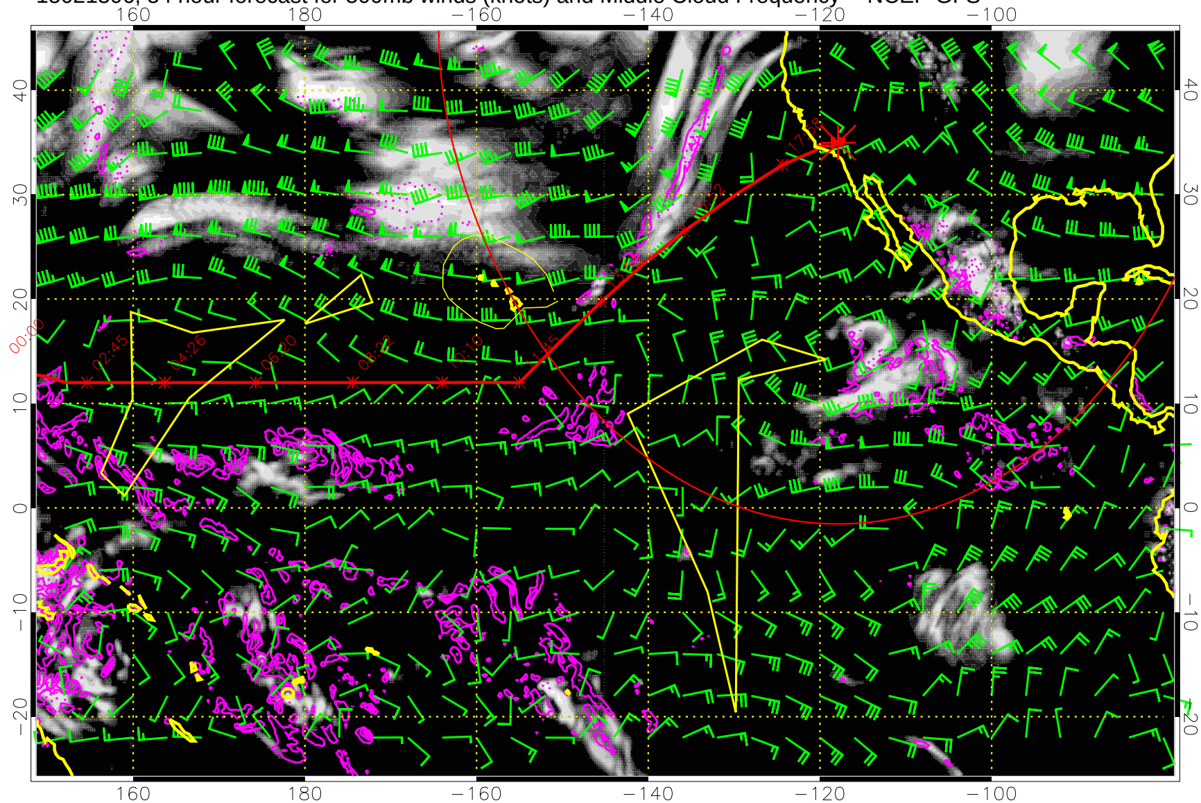
15021306, 54 hour forecast for 500mb winds (knots) and Middle Cloud Frequency -- NCEP GFS
