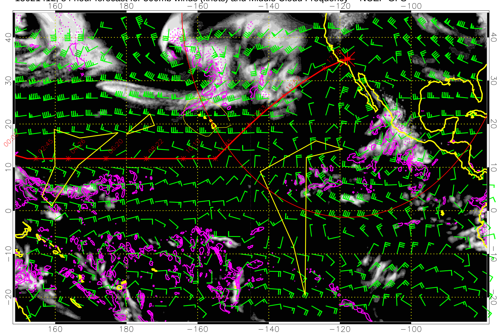
15021412, 84 hour forecast for 500mb winds (knots) and Middle Cloud Frequency -- NCEP GFS
