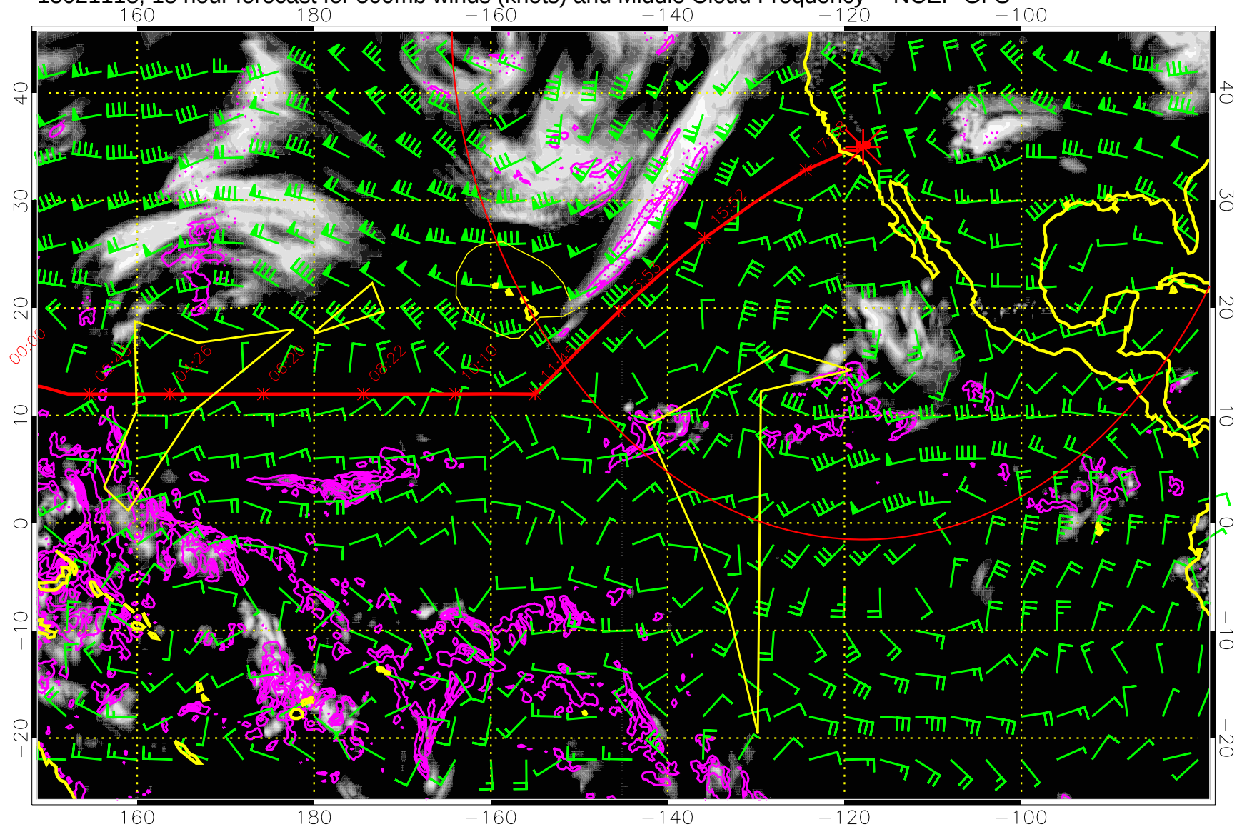
15021118, 18 hour forecast for 500mb winds (knots) and Middle Cloud Frequency -- NCEP GFS
