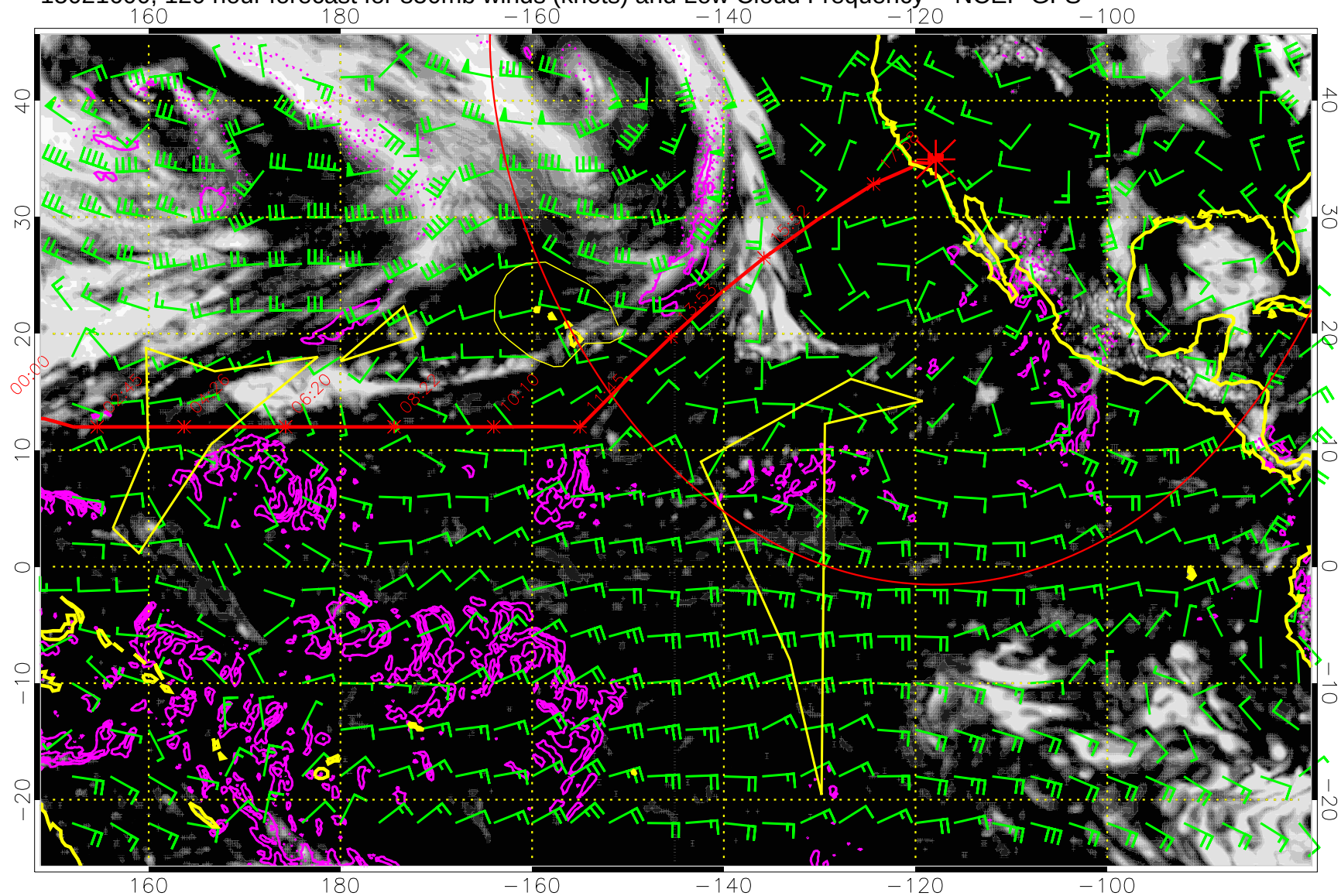
15021600, 120 hour forecast for 850mb winds (knots) and Low Cloud Frequency -- NCEP GFS
