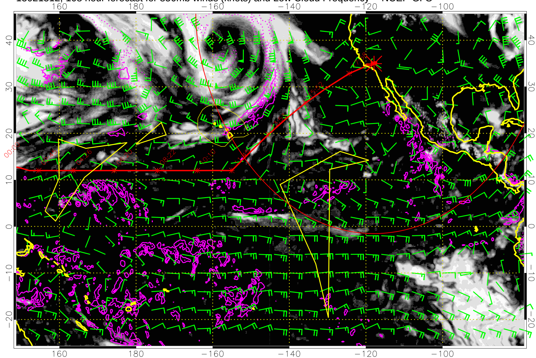
15021512, 108 hour forecast for 850mb winds (knots) and Low Cloud Frequency -- NCEP GFS
