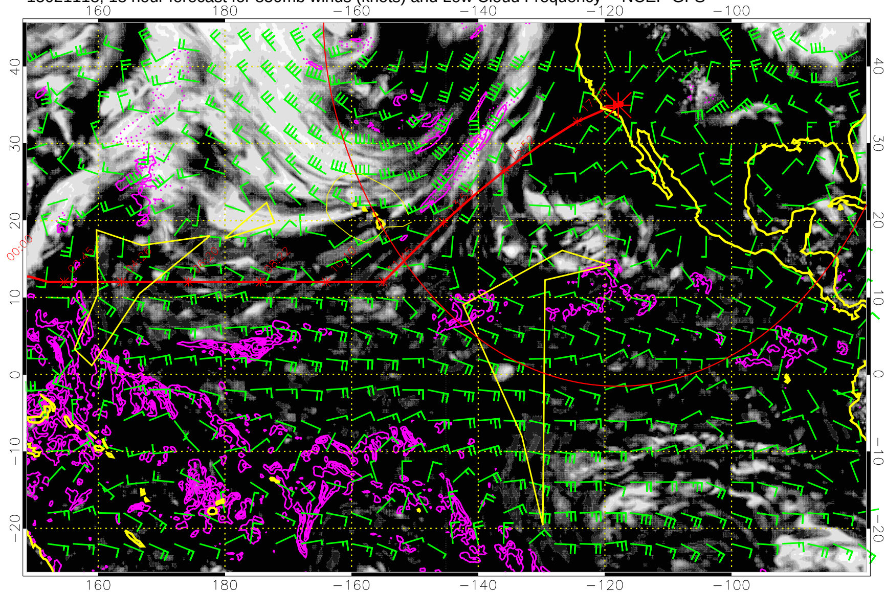
15021118, 18 hour forecast for 850mb winds (knots) and Low Cloud Frequency -- NCEP GFS
