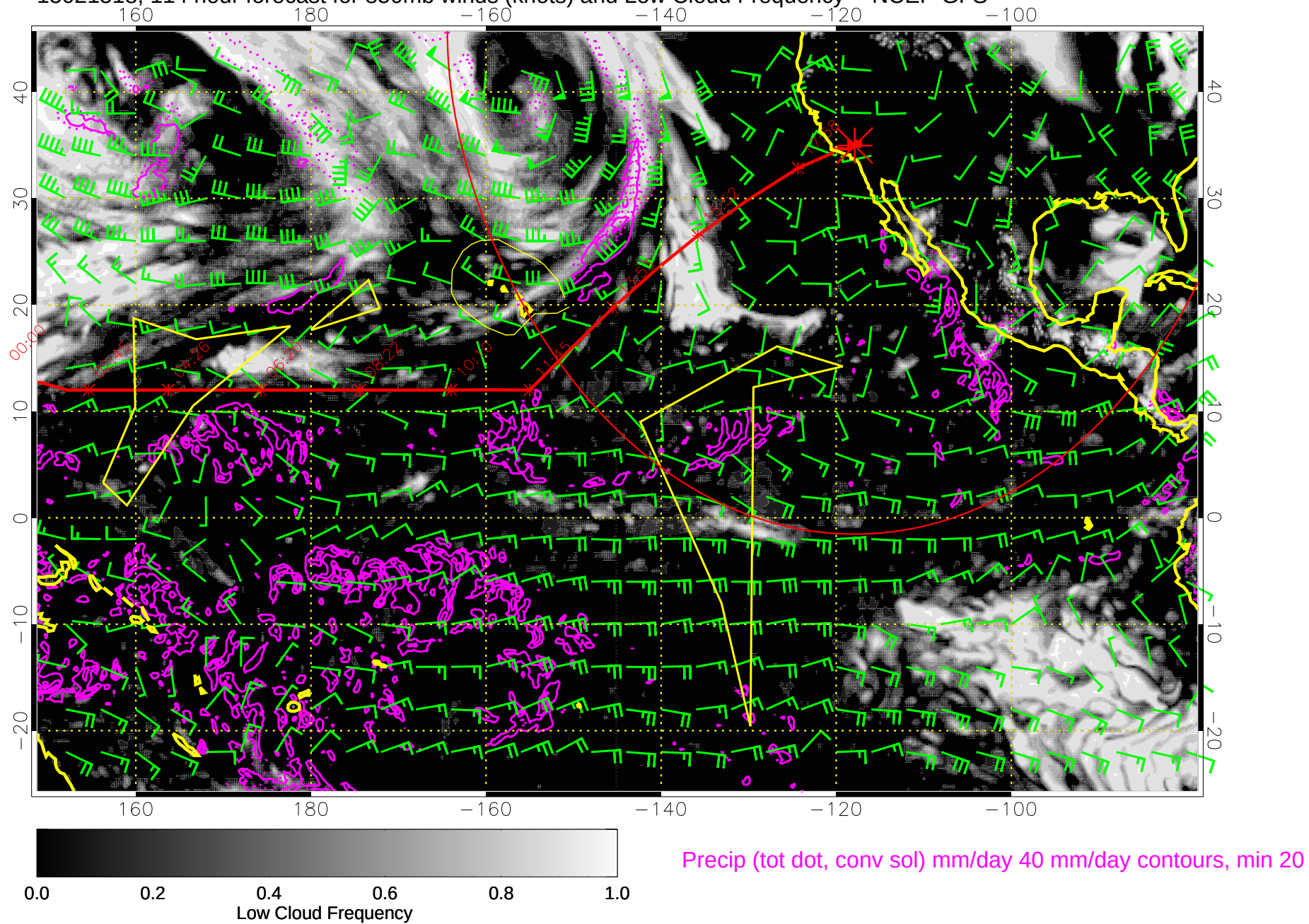
15021518, 114 hour forecast for 850mb winds (knots) and Low Cloud Frequency -- NCEP GFS
