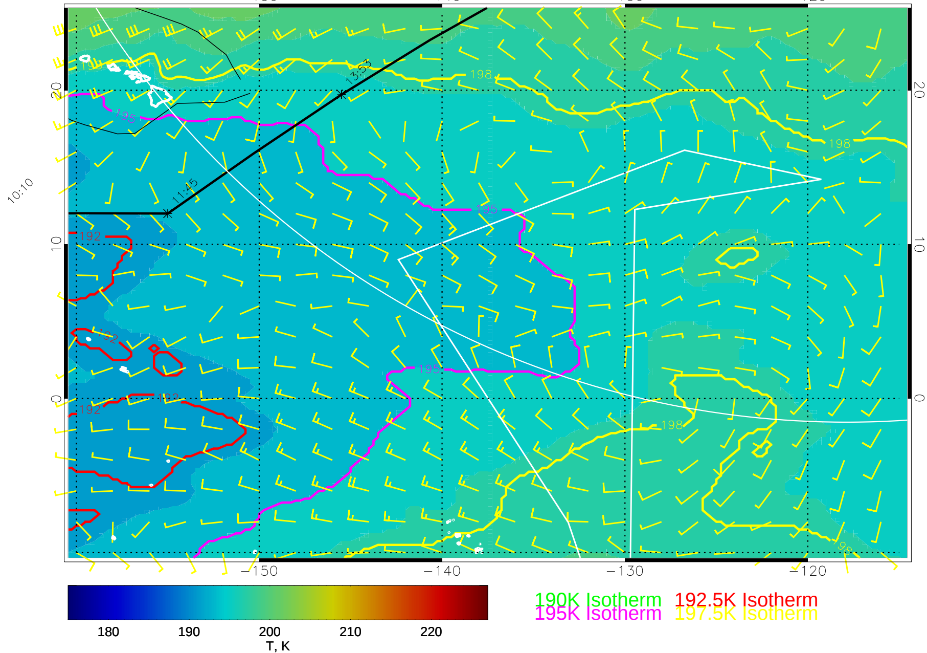
15021006, 6 hour forecast for 70mb T and winds (knots) -- NCEP GFS
