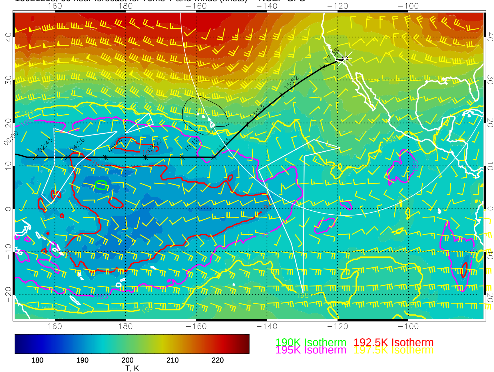
15021218, 66 hour forecast for 70mb T and winds (knots) -- NCEP GFS
