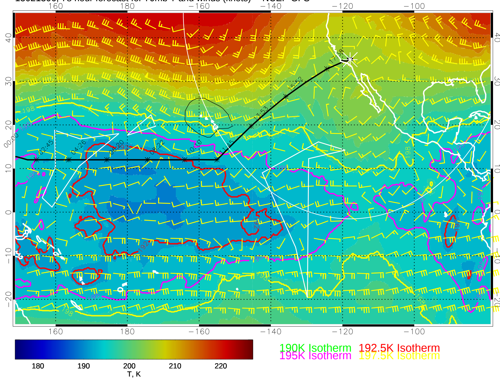
15021306, 78 hour forecast for 70mb T and winds (knots) -- NCEP GFS
