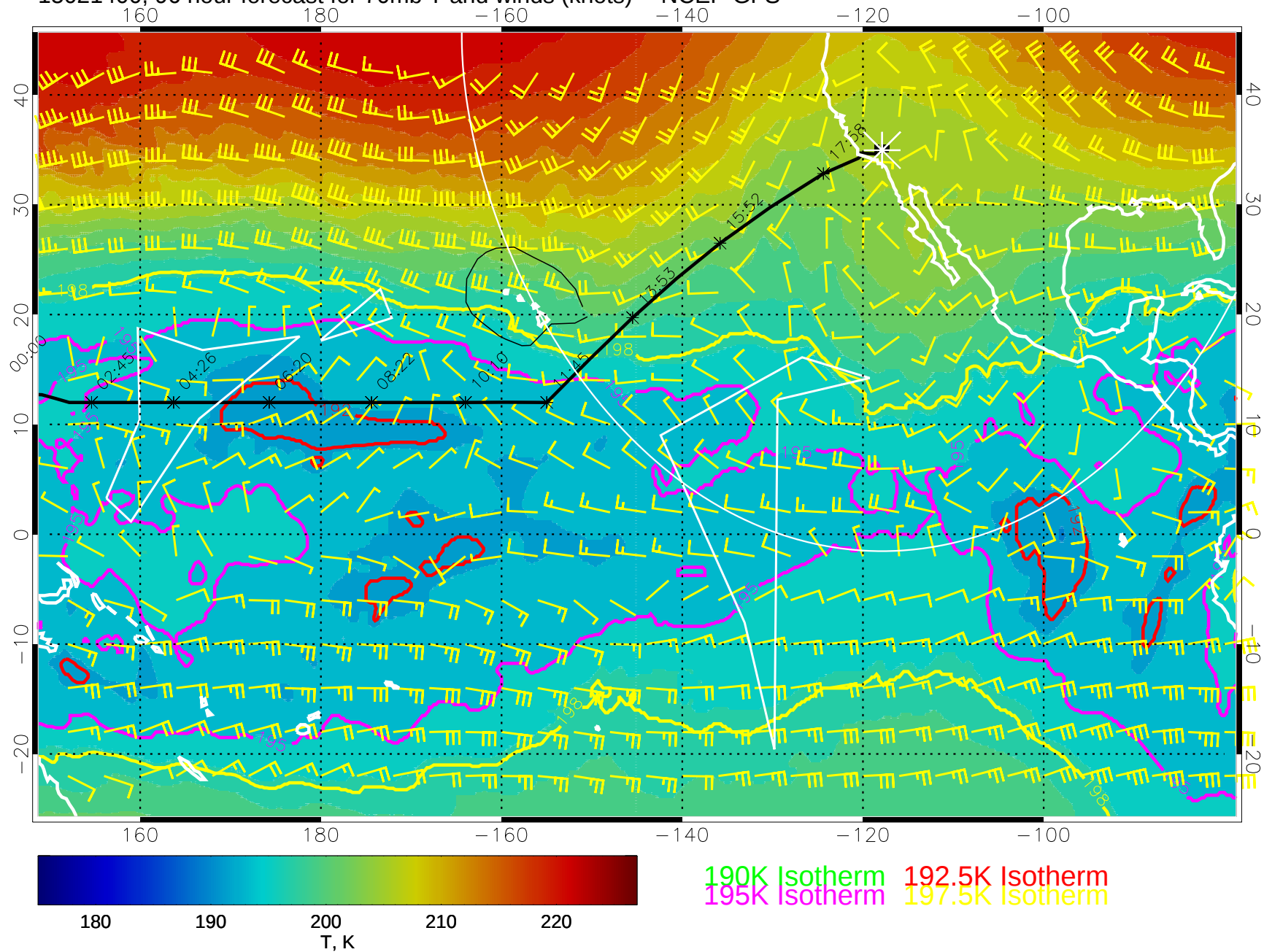
15021400, 96 hour forecast for 70mb T and winds (knots) -- NCEP GFS
