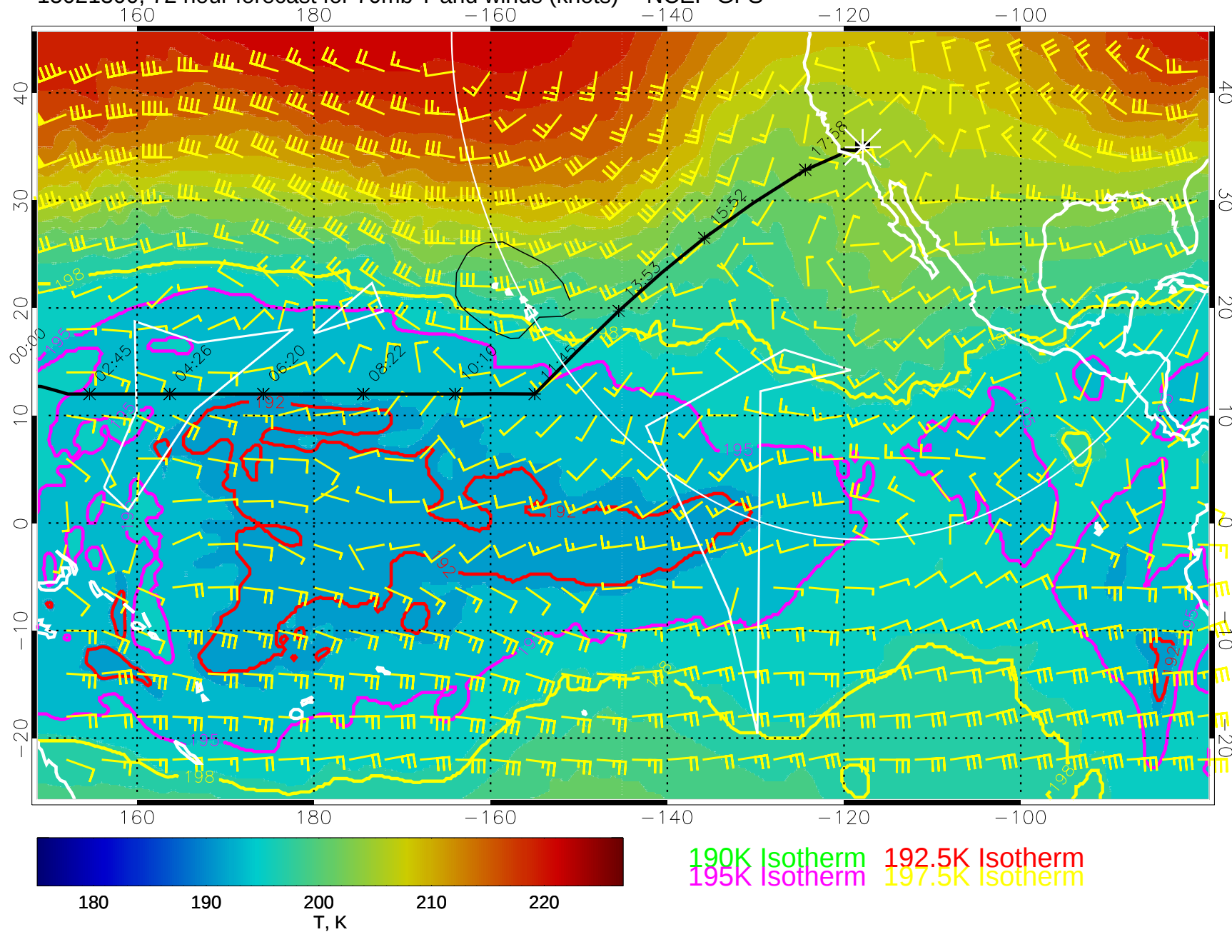
15021300, 72 hour forecast for 70mb T and winds (knots) -- NCEP GFS
