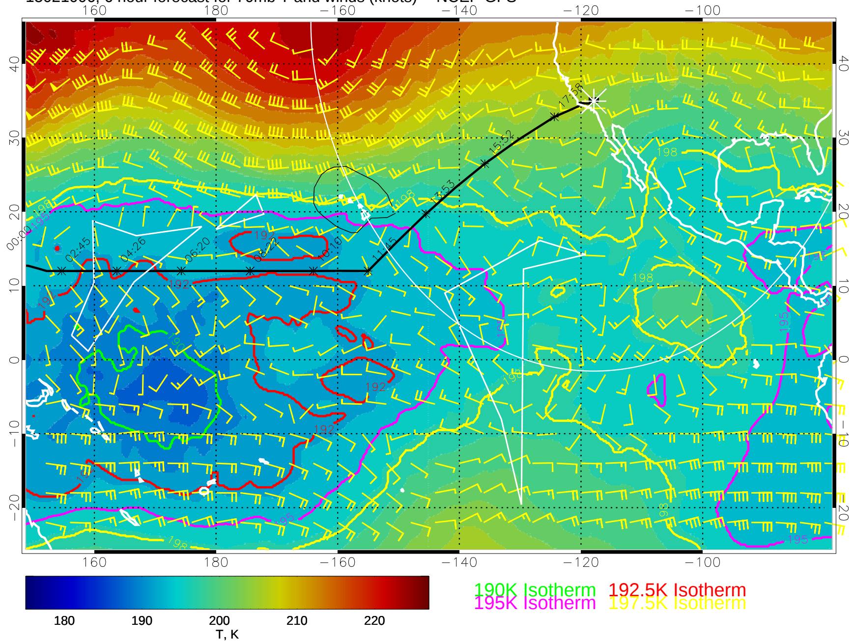
15021006, 6 hour forecast for 70mb T and winds (knots) -- NCEP GFS
