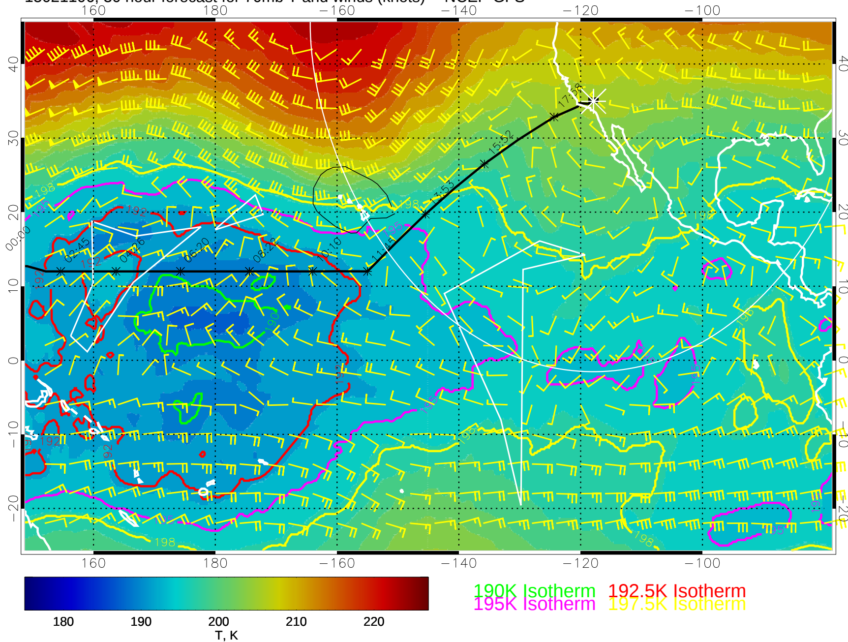
15021106, 30 hour forecast for 70mb T and winds (knots) -- NCEP GFS
