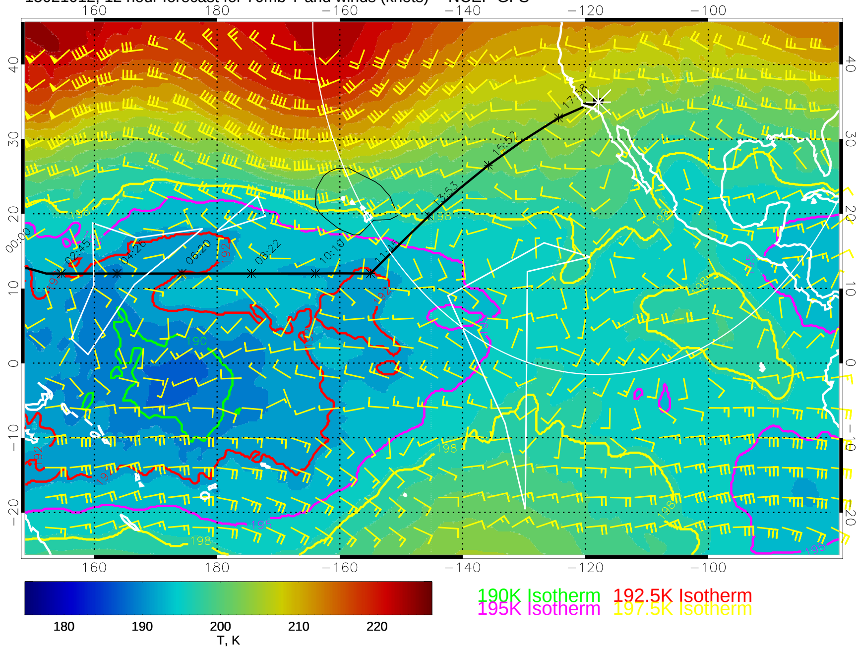
15021012, 12 hour forecast for 70mb T and winds (knots) -- NCEP GFS
