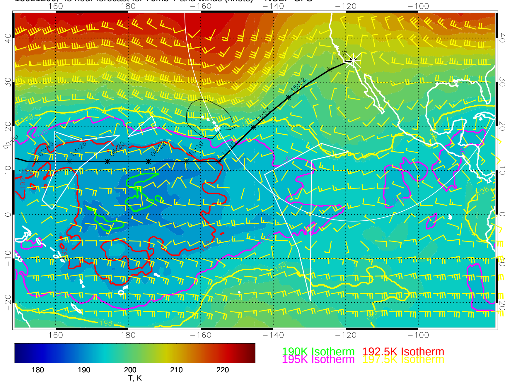
15021200, 48 hour forecast for 70mb T and winds (knots) -- NCEP GFS
