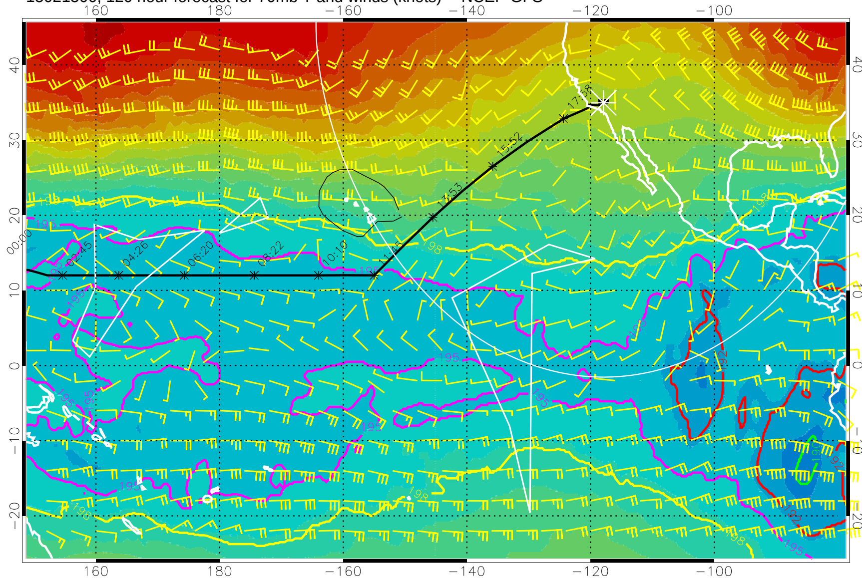
15021500, 120 hour forecast for 70mb T and winds (knots) -- NCEP GFS
