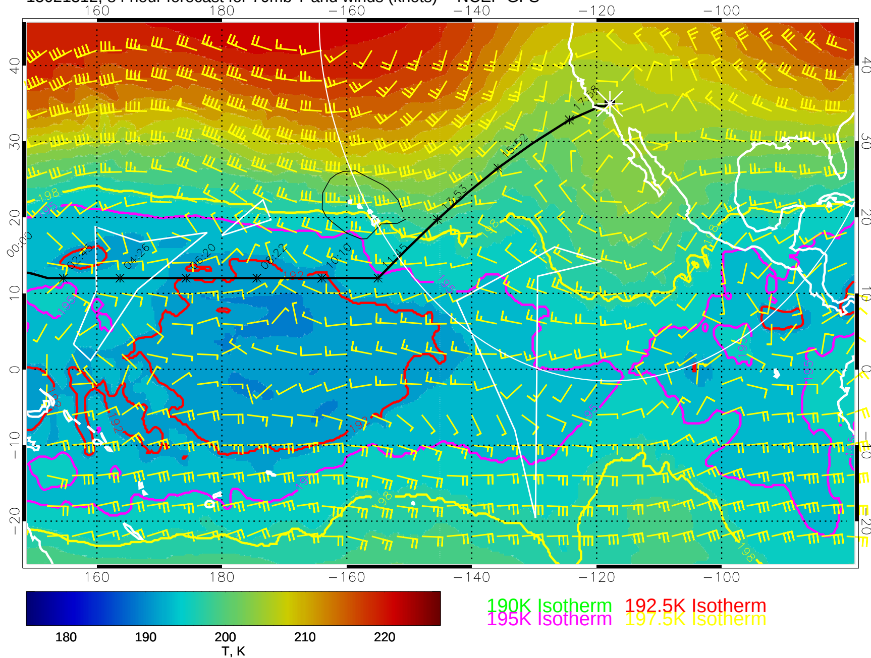
15021312, 84 hour forecast for 70mb T and winds (knots) -- NCEP GFS
