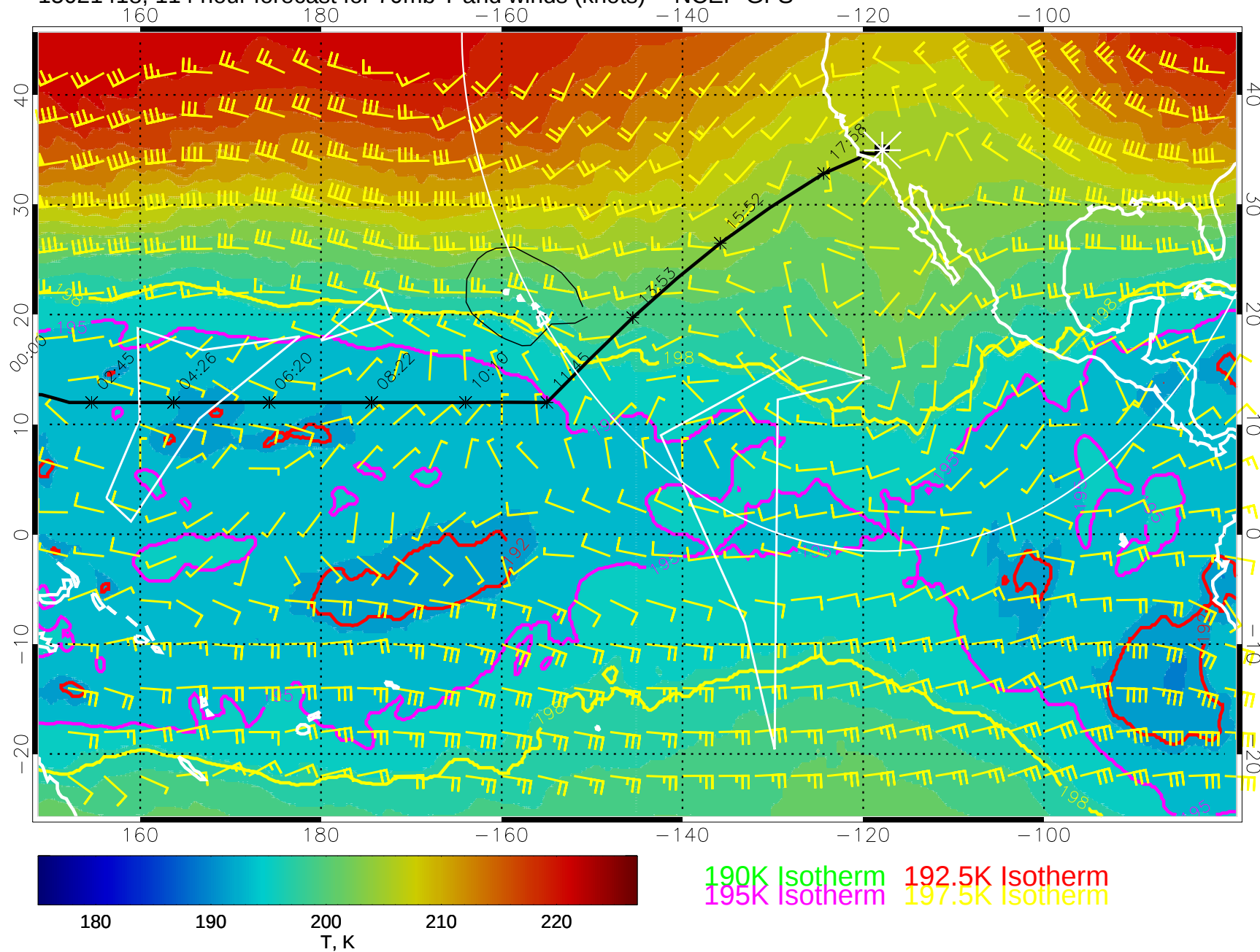
15021418, 114 hour forecast for 70mb T and winds (knots) -- NCEP GFS
