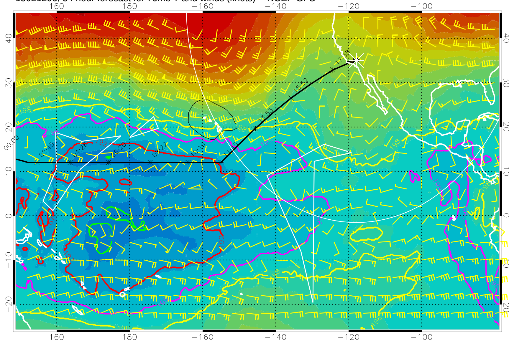
15021206, 54 hour forecast for 70mb T and winds (knots) -- NCEP GFS
