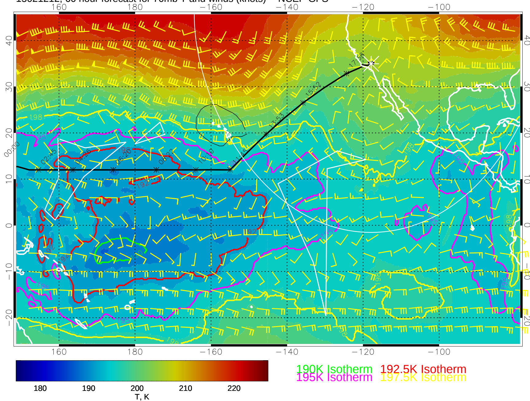
15021212, 60 hour forecast for 70mb T and winds (knots) -- NCEP GFS
