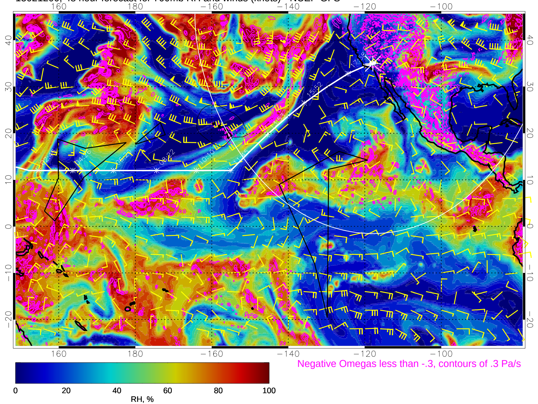
15021200, 48 hour forecast for 700mb RH and winds (knots) - NCEP GFS
