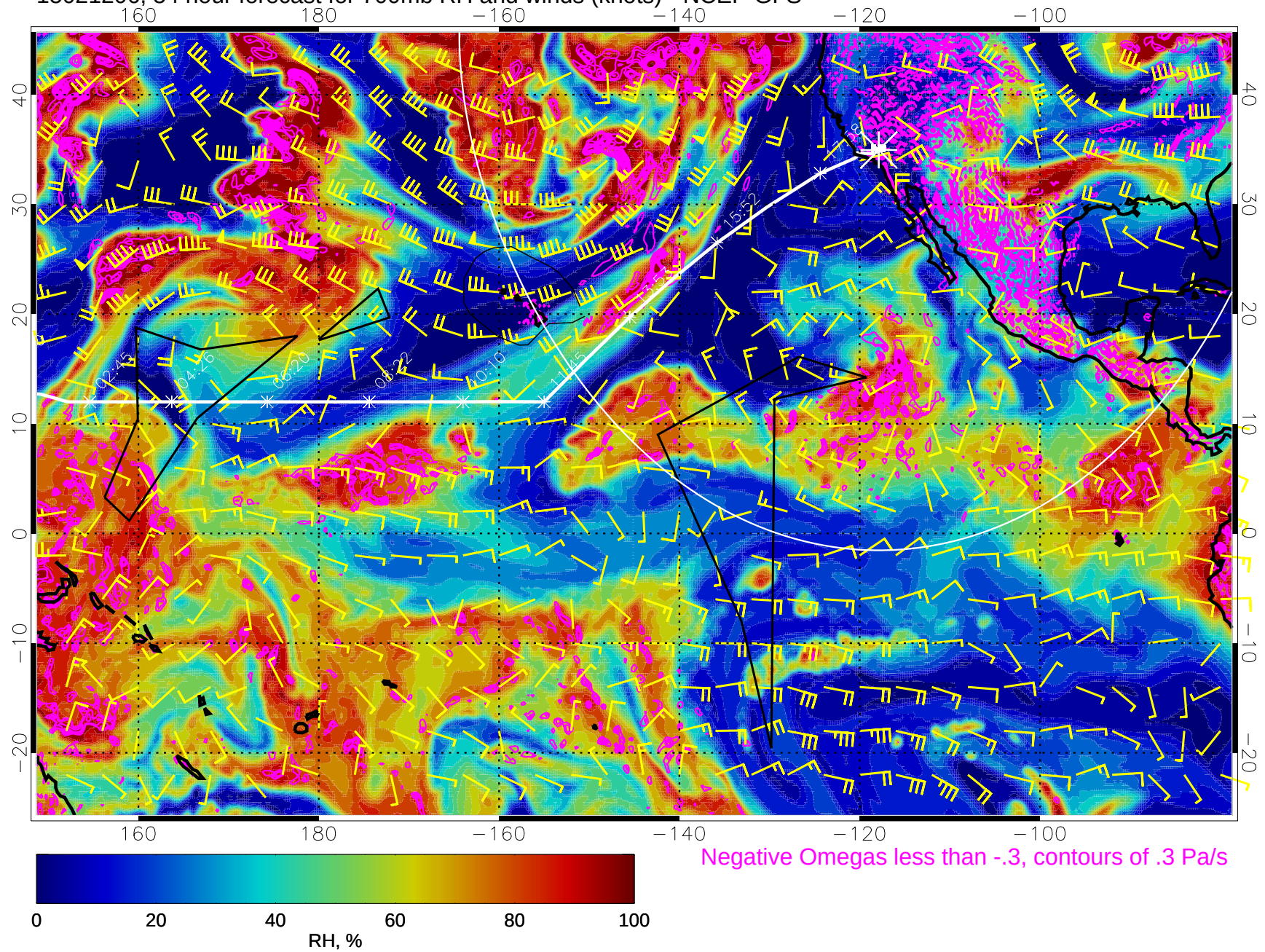
15021206, 54 hour forecast for 700mb RH and winds (knots) - NCEP GFS
