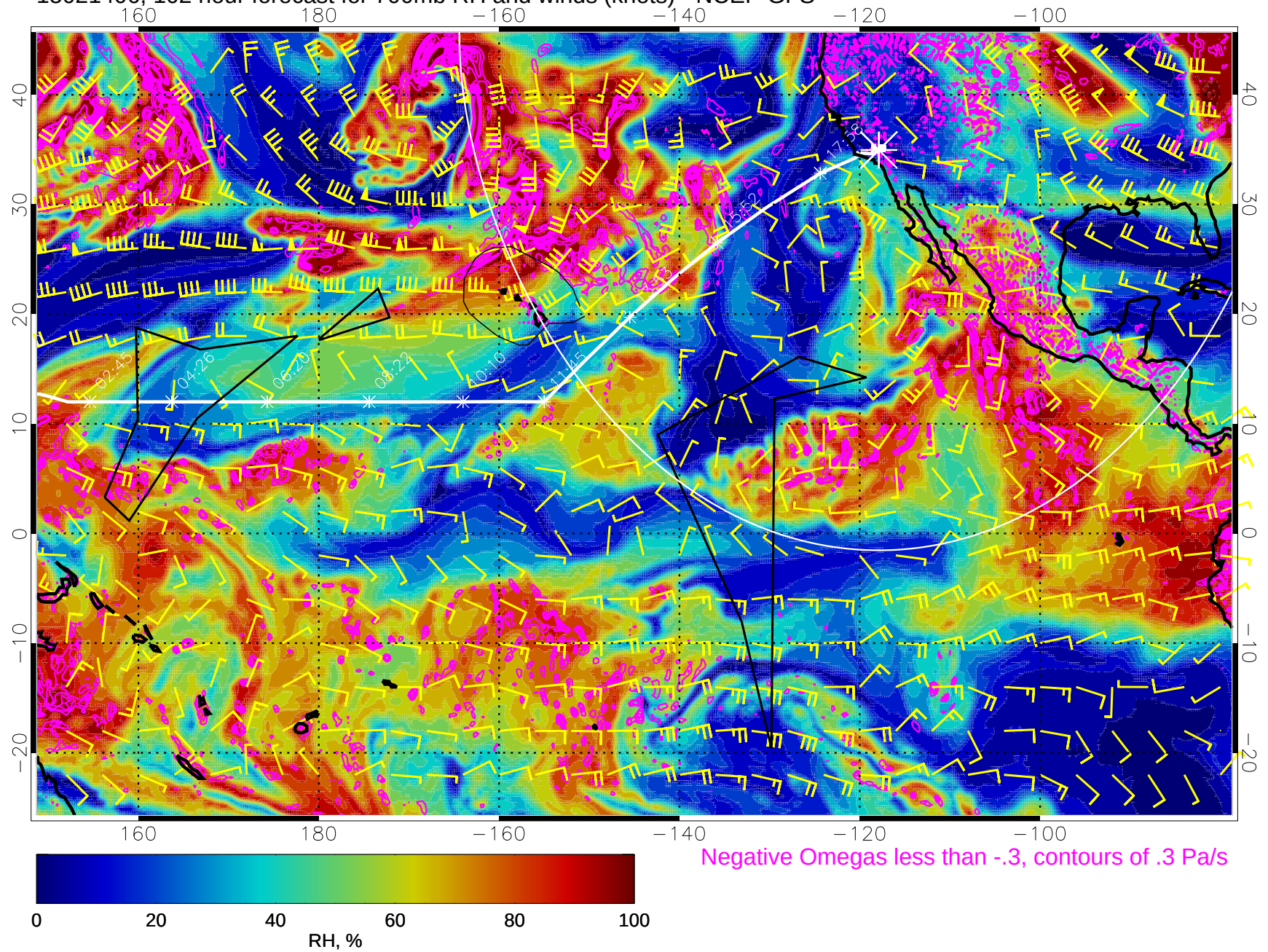
15021406, 102 hour forecast for 700mb RH and winds (knots) - NCEP GFS
