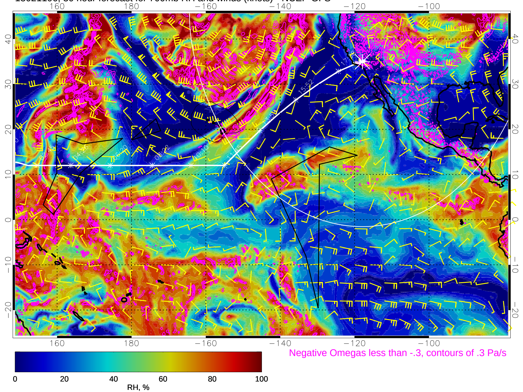
15021106, 30 hour forecast for 700mb RH and winds (knots) - NCEP GFS
