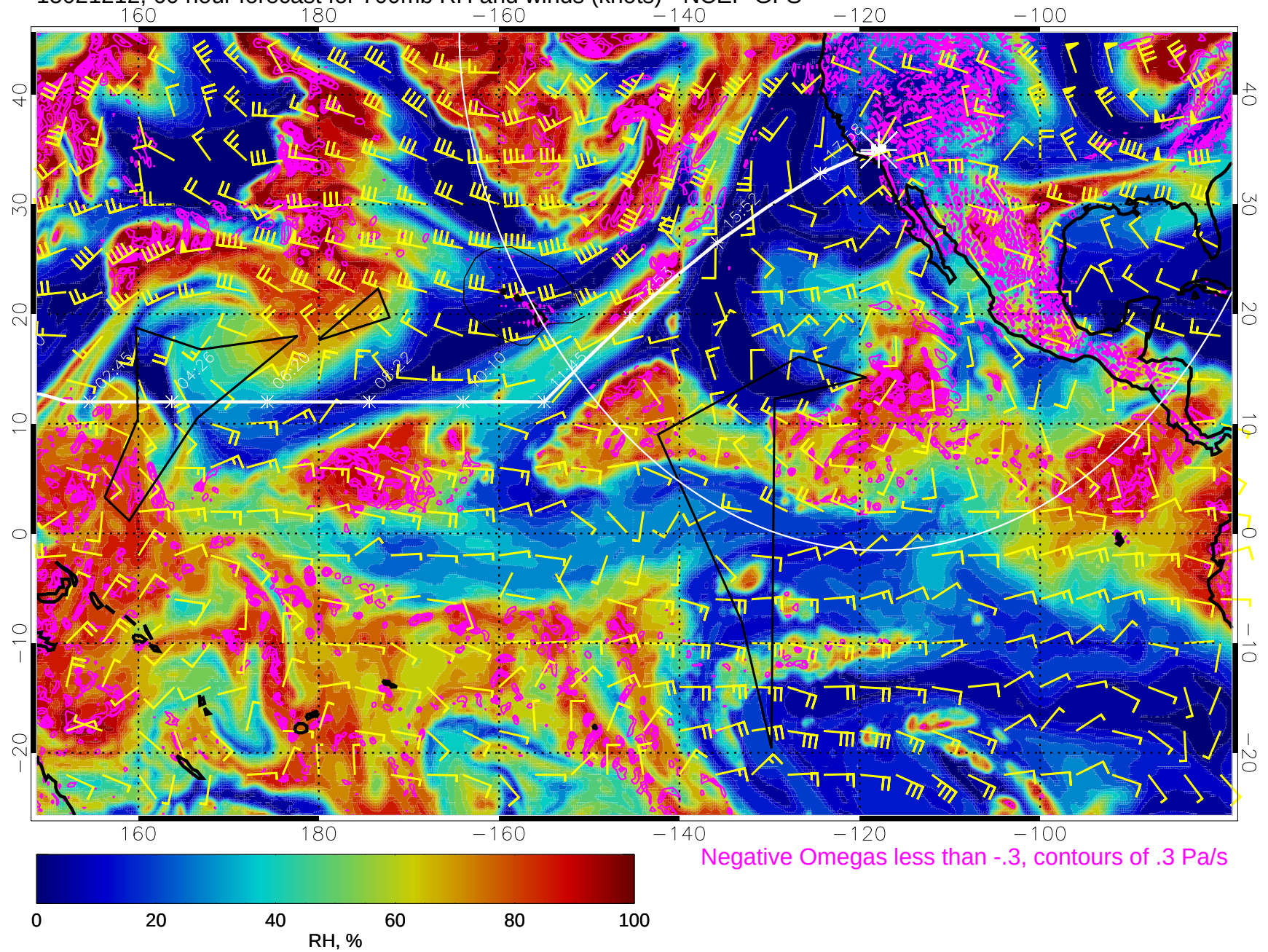
15021212, 60 hour forecast for 700mb RH and winds (knots) - NCEP GFS
