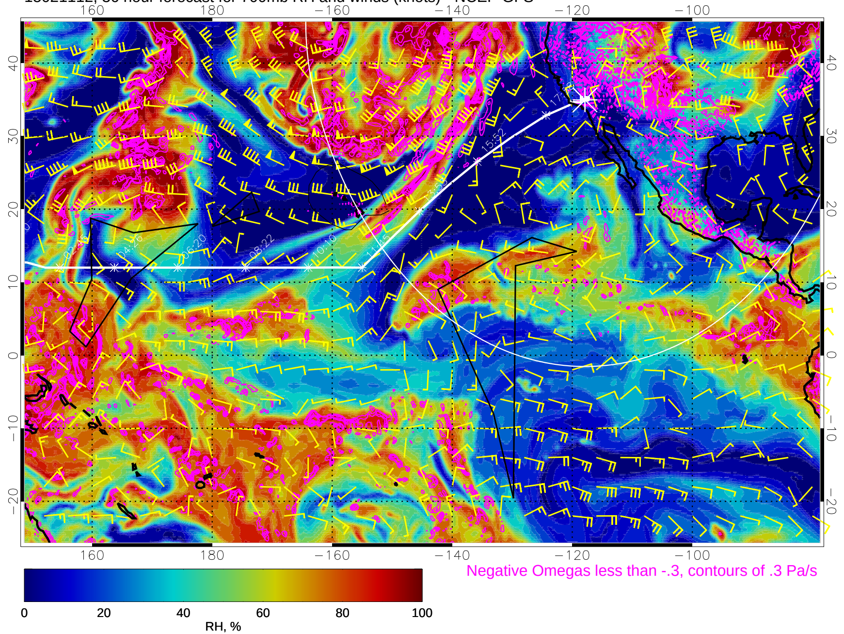
15021112, 36 hour forecast for 700mb RH and winds (knots) - NCEP GFS
