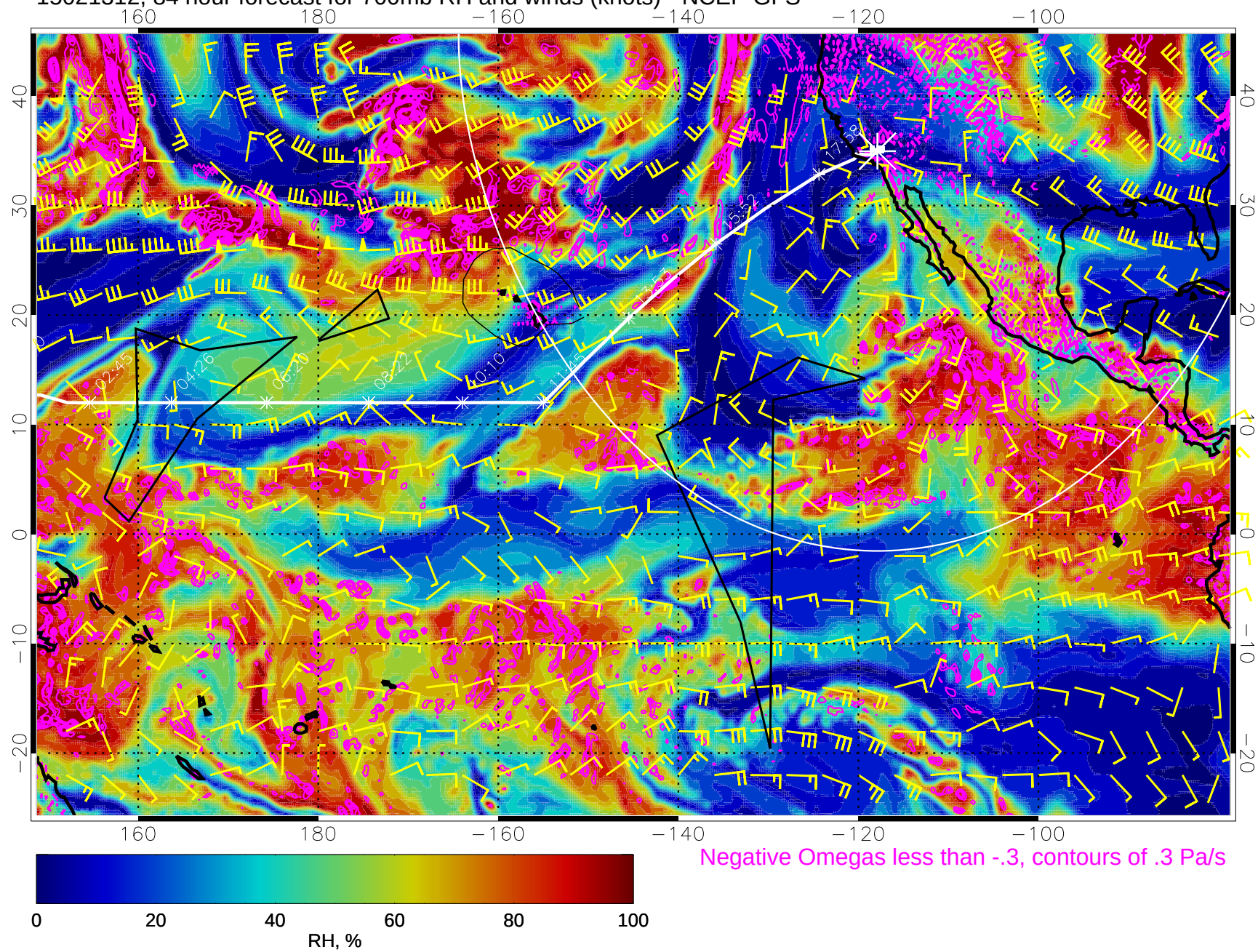
15021312, 84 hour forecast for 700mb RH and winds (knots) - NCEP GFS
