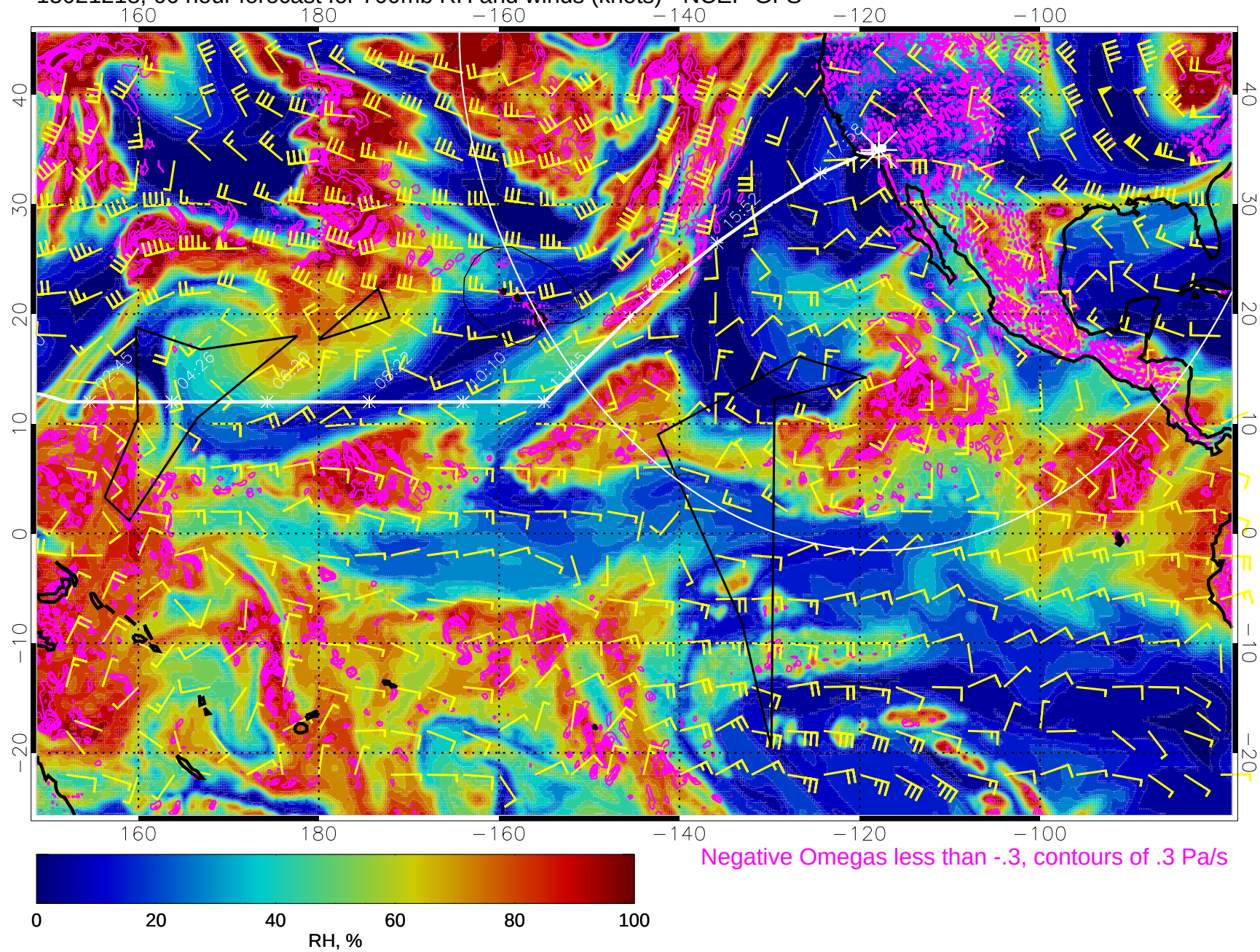
15021218, 66 hour forecast for 700mb RH and winds (knots) - NCEP GFS
