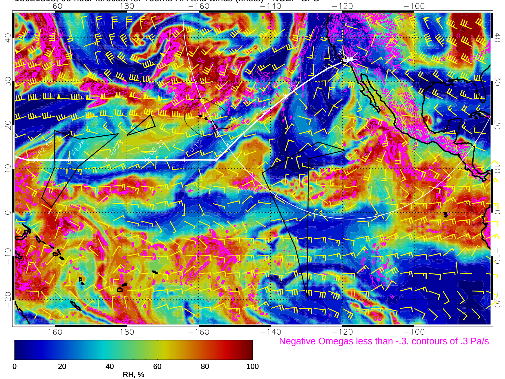
15021318, 90 hour forecast for 700mb RH and winds (knots) - NCEP GFS
