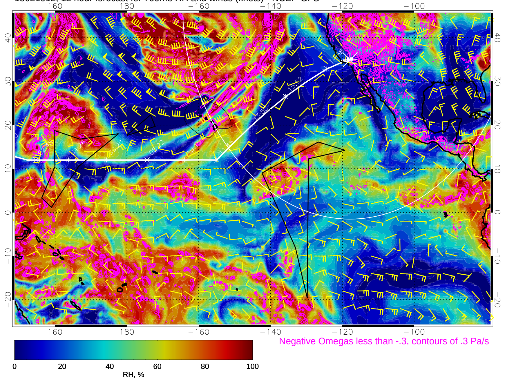
15021012, 12 hour forecast for 700mb RH and winds (knots) - NCEP GFS
