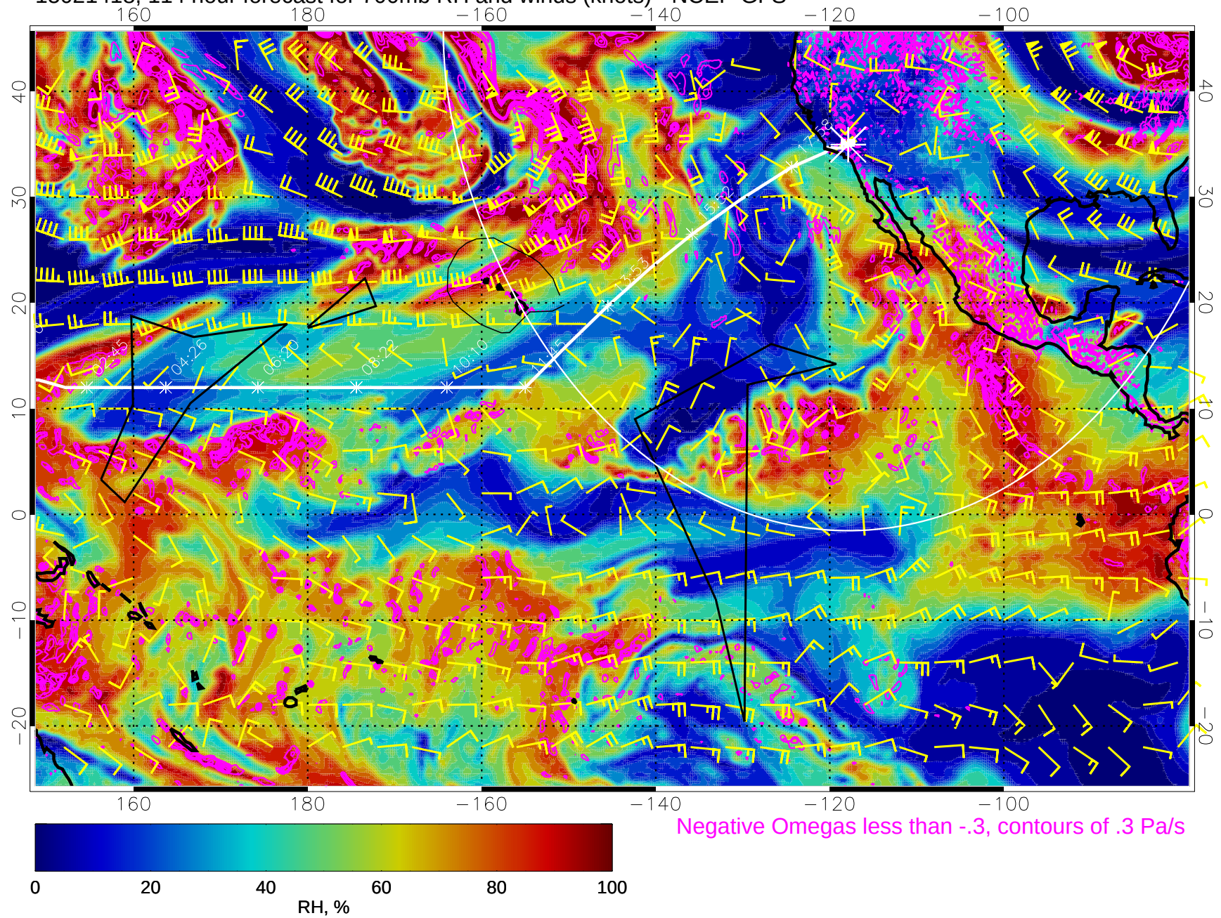
15021418, 114 hour forecast for 700mb RH and winds (knots) - NCEP GFS
