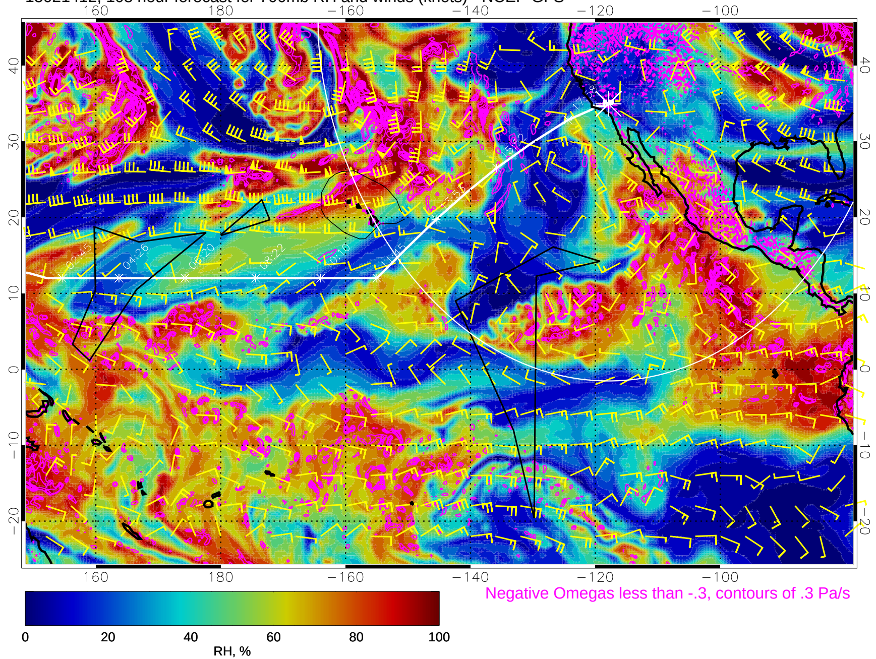
15021412, 108 hour forecast for 700mb RH and winds (knots) - NCEP GFS
