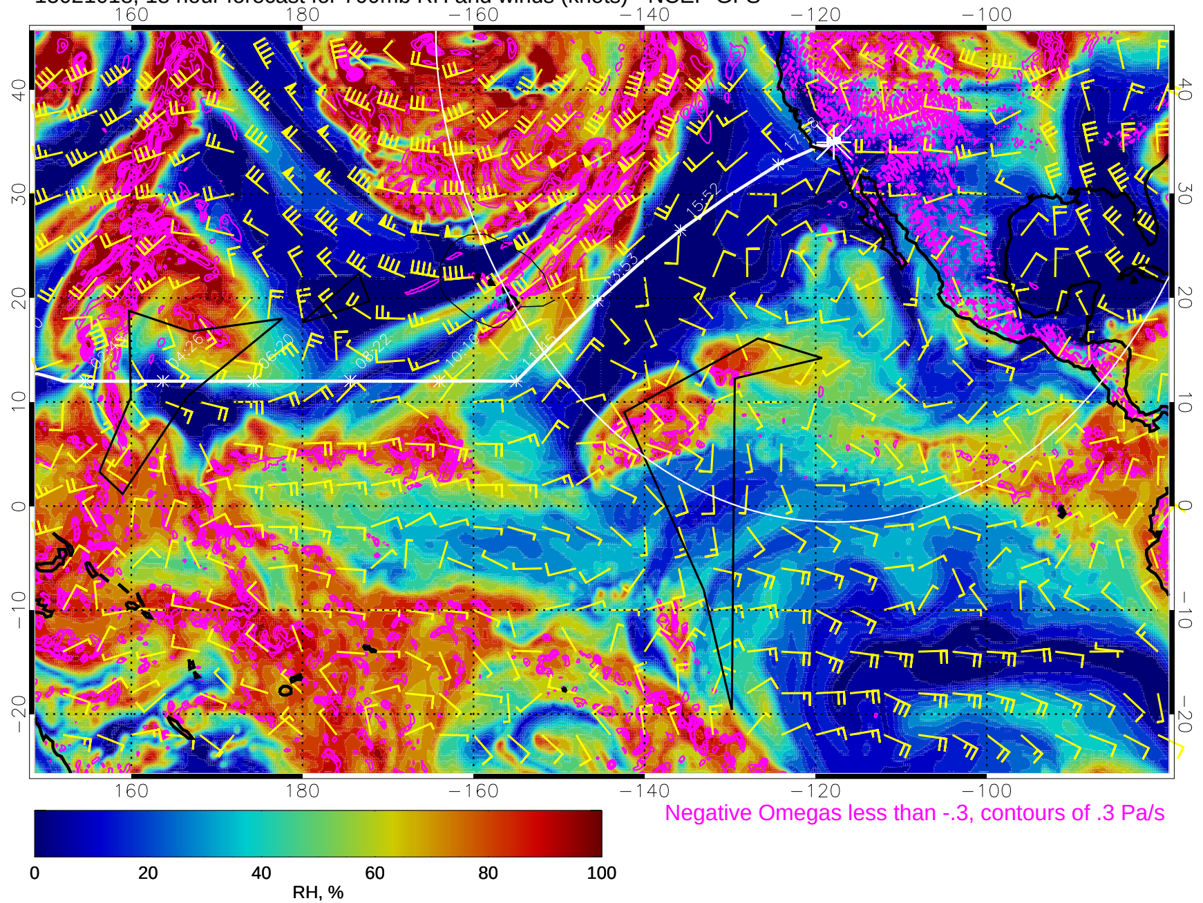
15021018, 18 hour forecast for 700mb RH and winds (knots) - NCEP GFS
