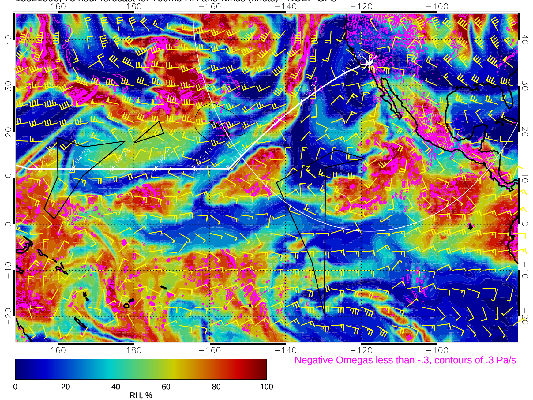
15021306, 78 hour forecast for 700mb RH and winds (knots) - NCEP GFS
