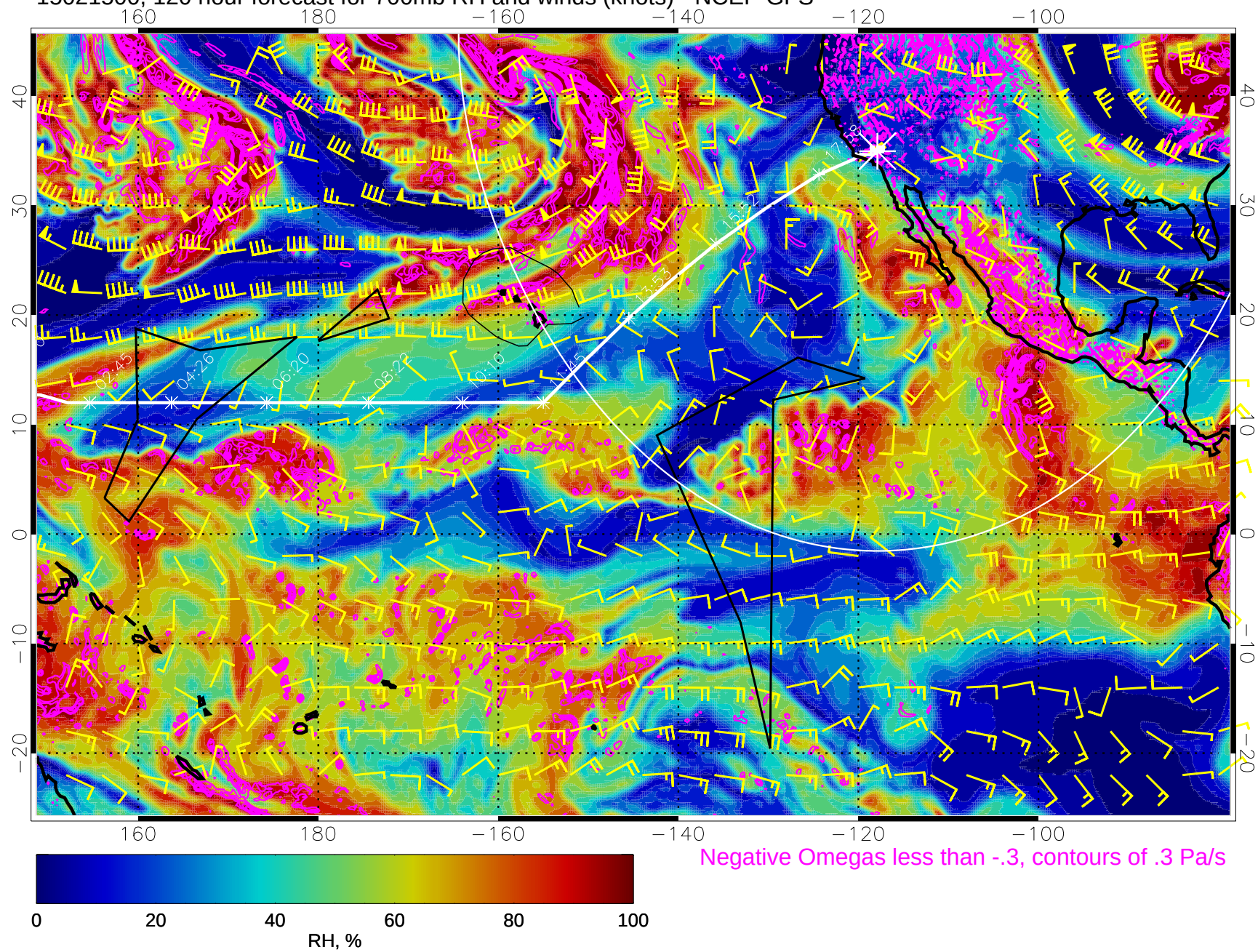
15021500, 120 hour forecast for 700mb RH and winds (knots) - NCEP GFS
