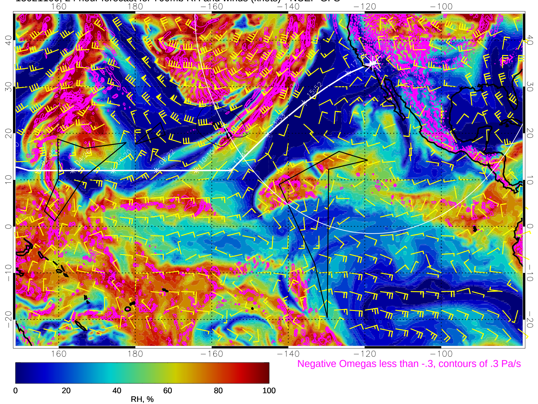
15021100, 24 hour forecast for 700mb RH and winds (knots) - NCEP GFS
