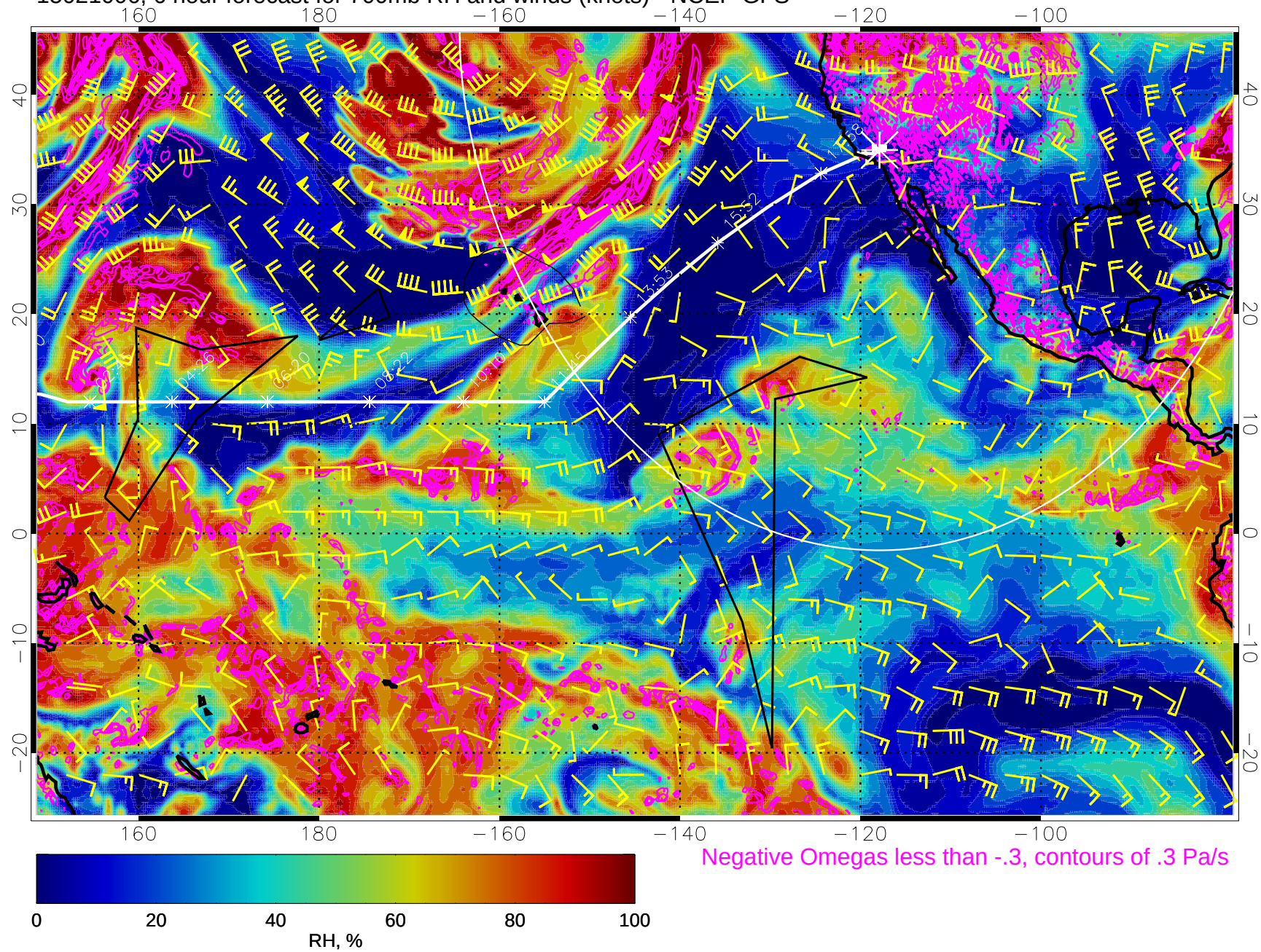
15021006, 6 hour forecast for 700mb RH and winds (knots) - NCEP GFS
