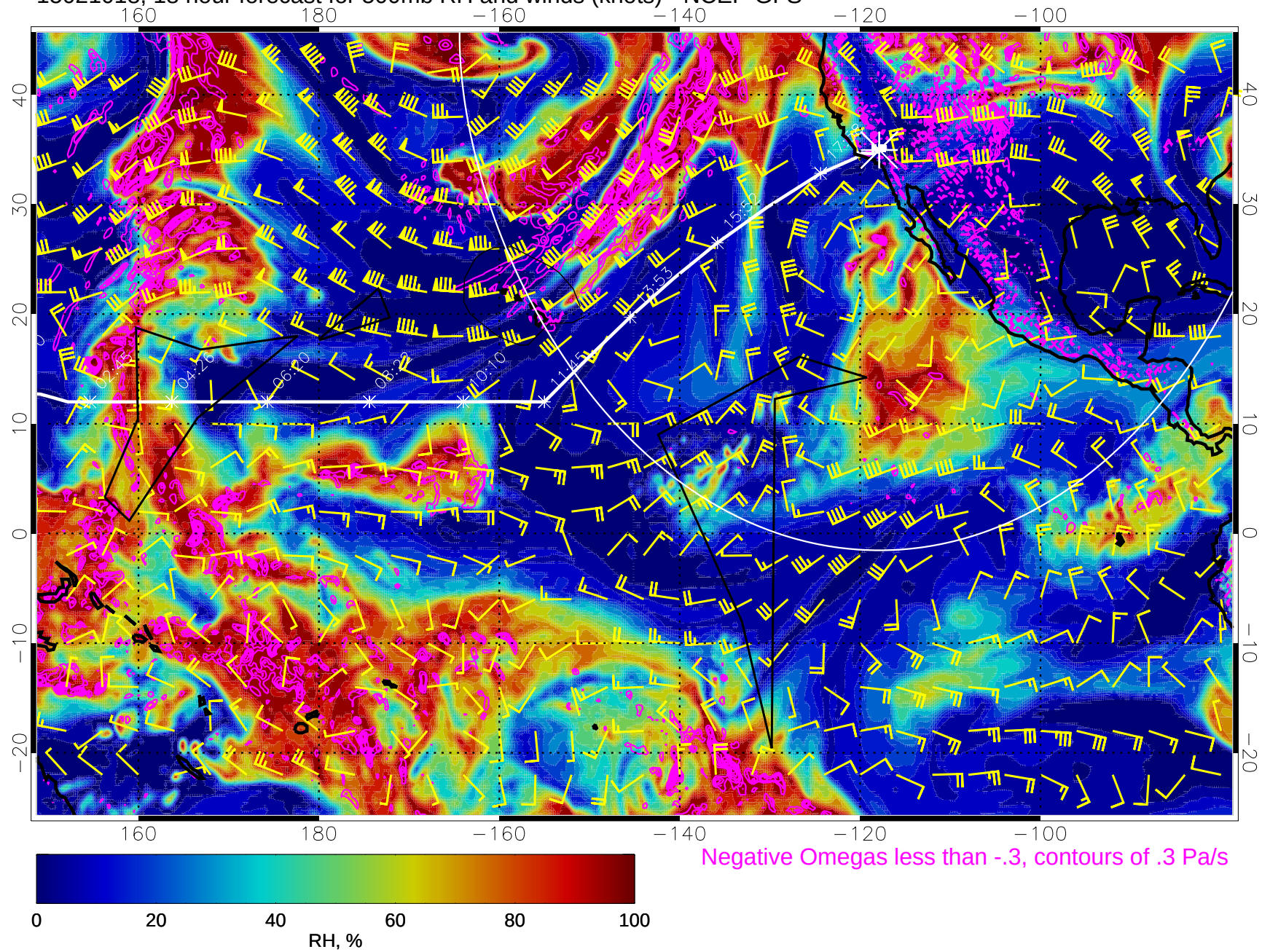
15021018, 18 hour forecast for 500mb RH and winds (knots) - NCEP GFS
