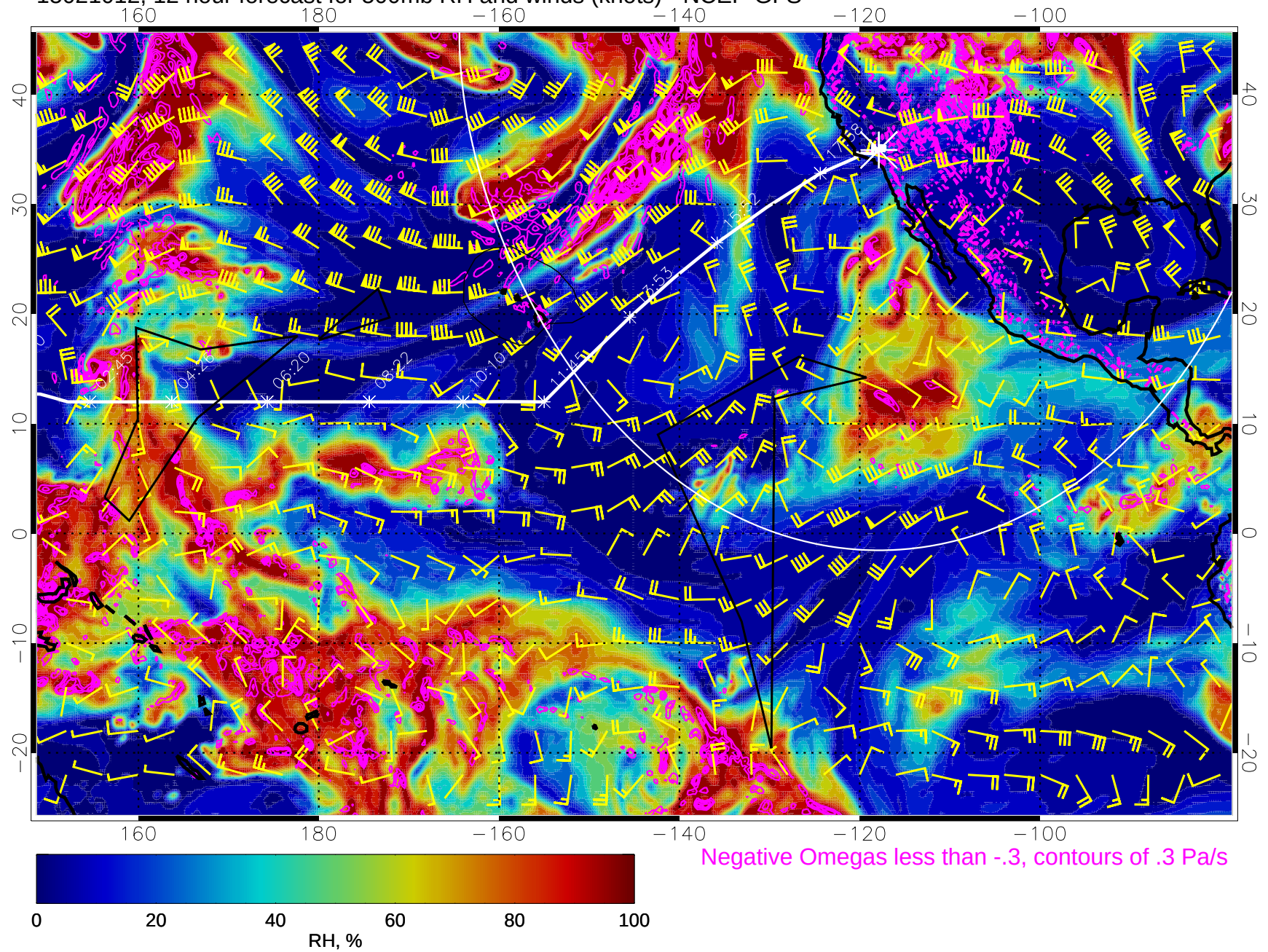
15021012, 12 hour forecast for 500mb RH and winds (knots) - NCEP GFS
