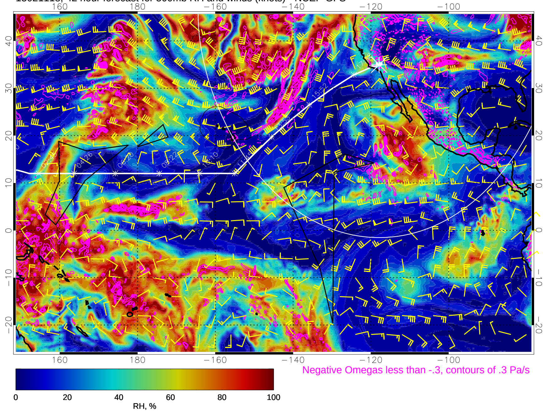
15021118, 42 hour forecast for 500mb RH and winds (knots) - NCEP GFS
