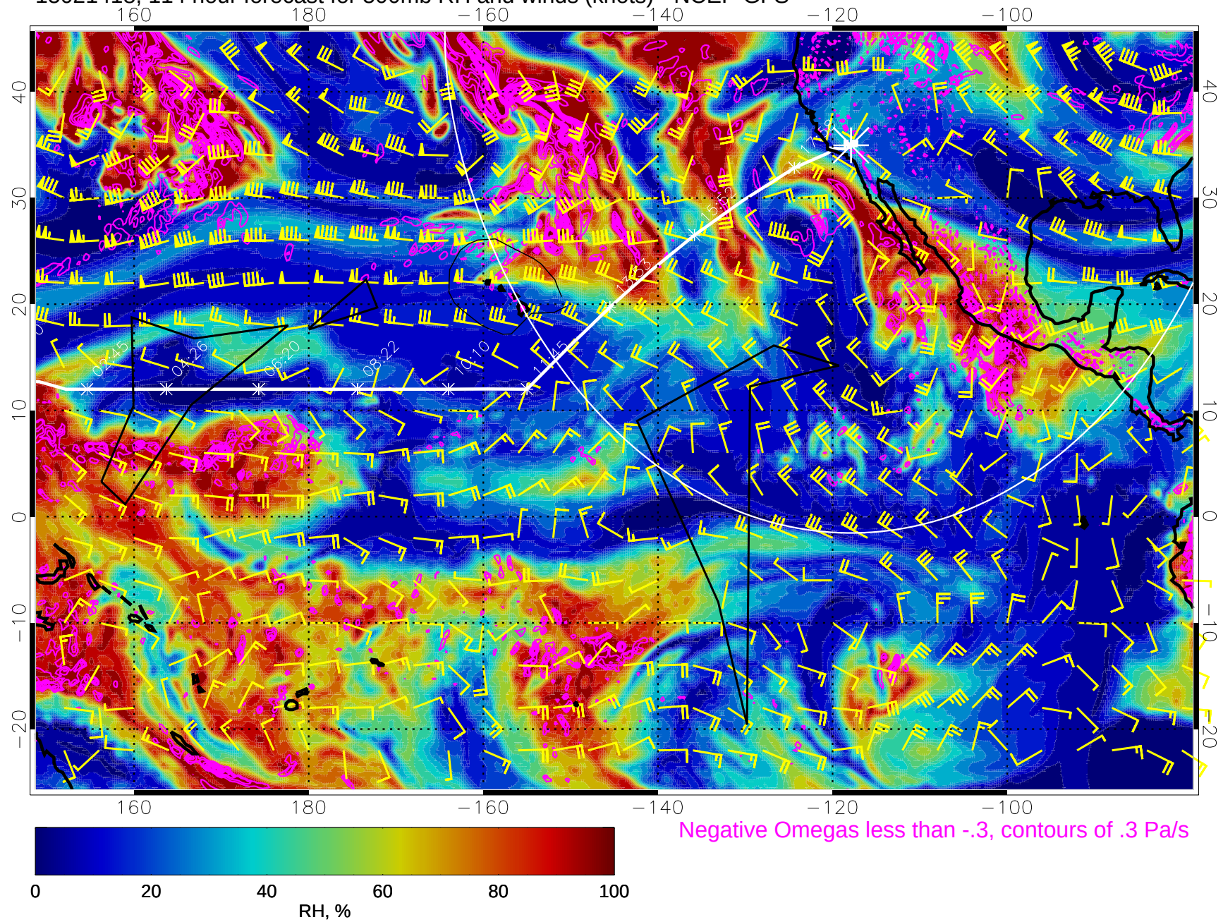
15021418, 114 hour forecast for 500mb RH and winds (knots) - NCEP GFS
