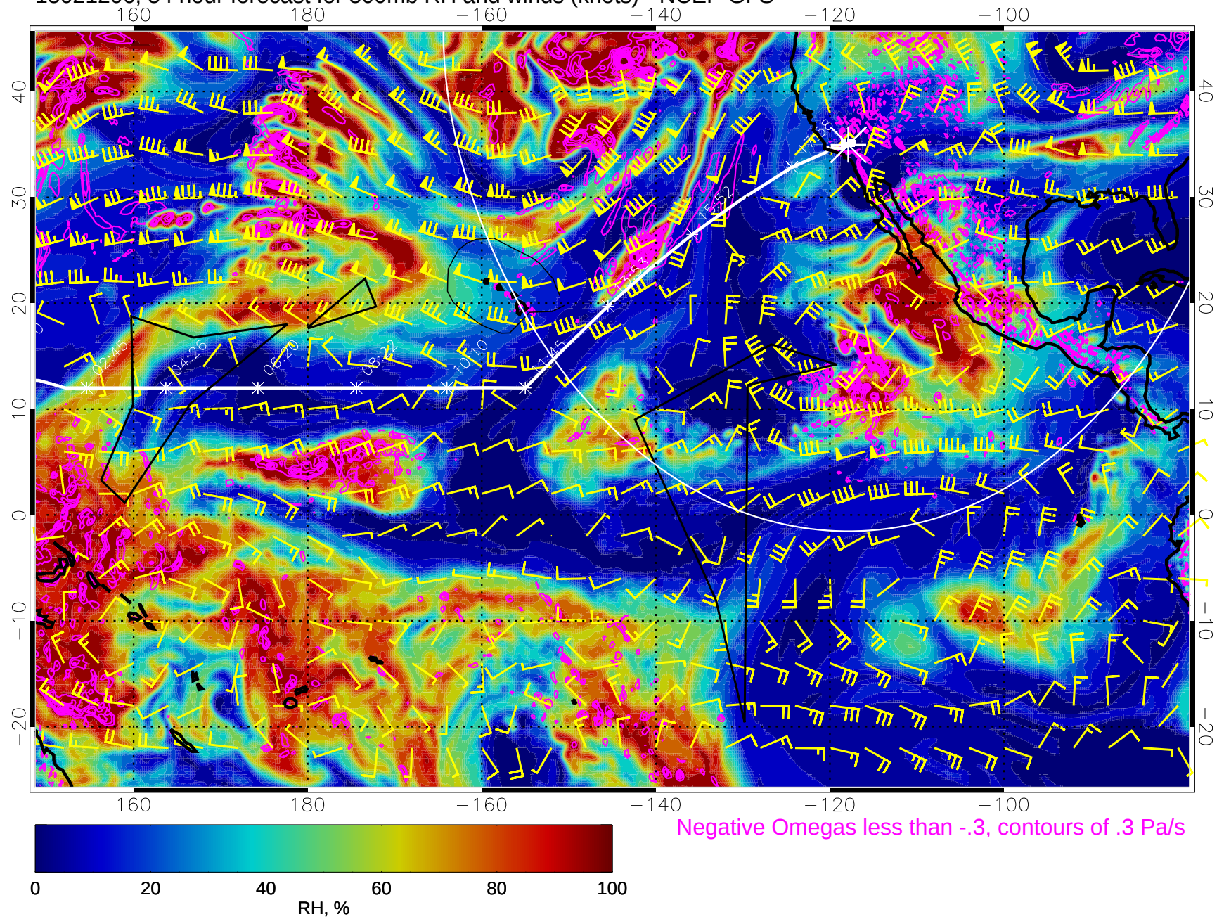
15021206, 54 hour forecast for 500mb RH and winds (knots) - NCEP GFS
