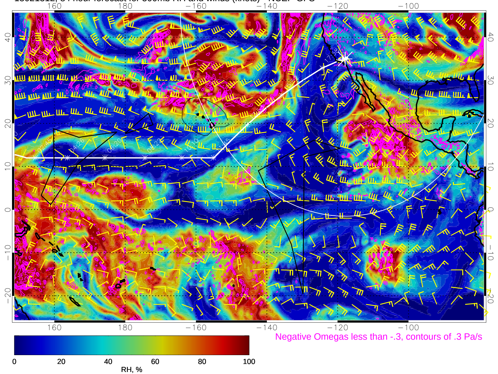
15021312, 84 hour forecast for 500mb RH and winds (knots) - NCEP GFS
