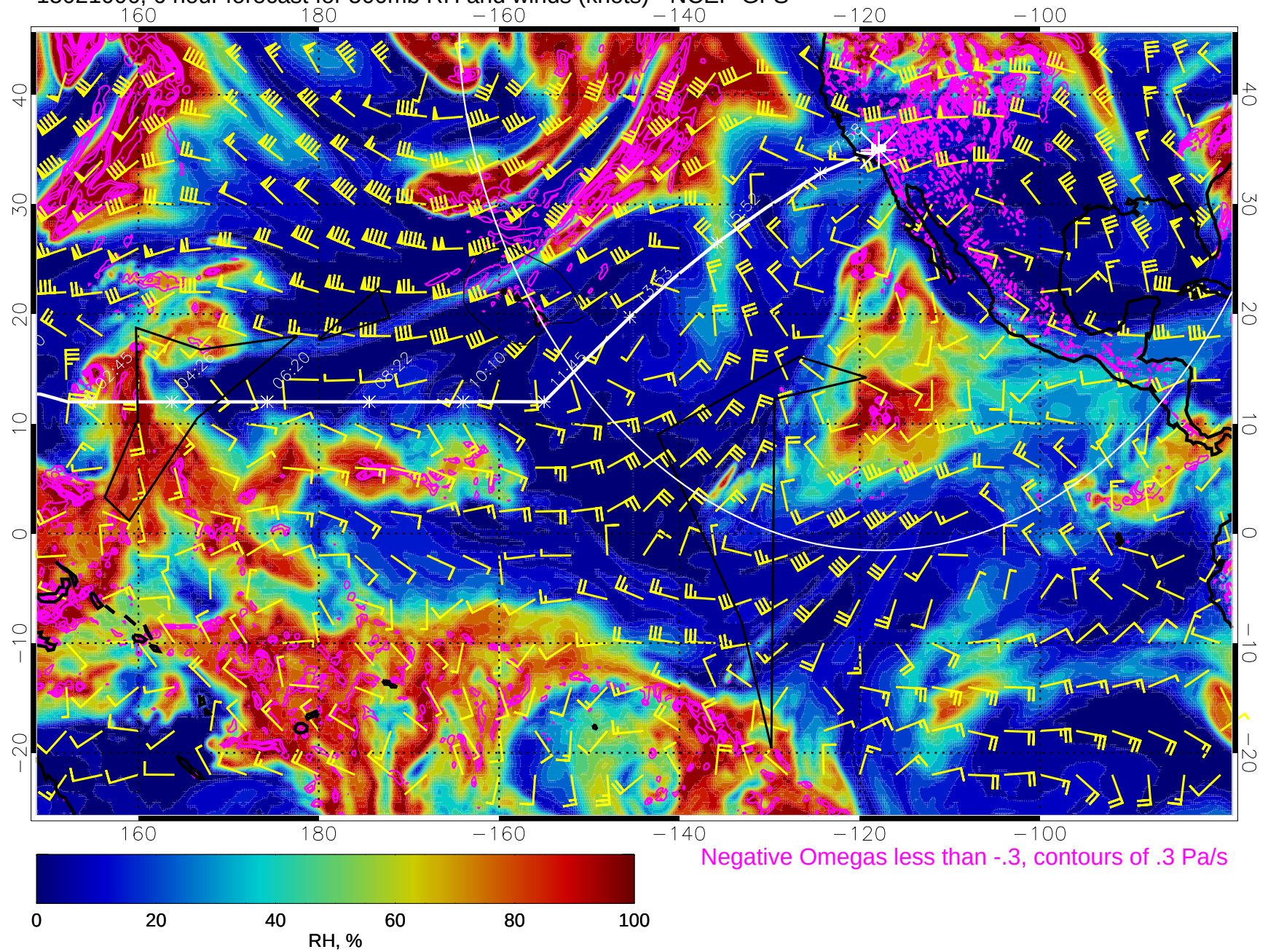
15021006, 6 hour forecast for 500mb RH and winds (knots) - NCEP GFS
