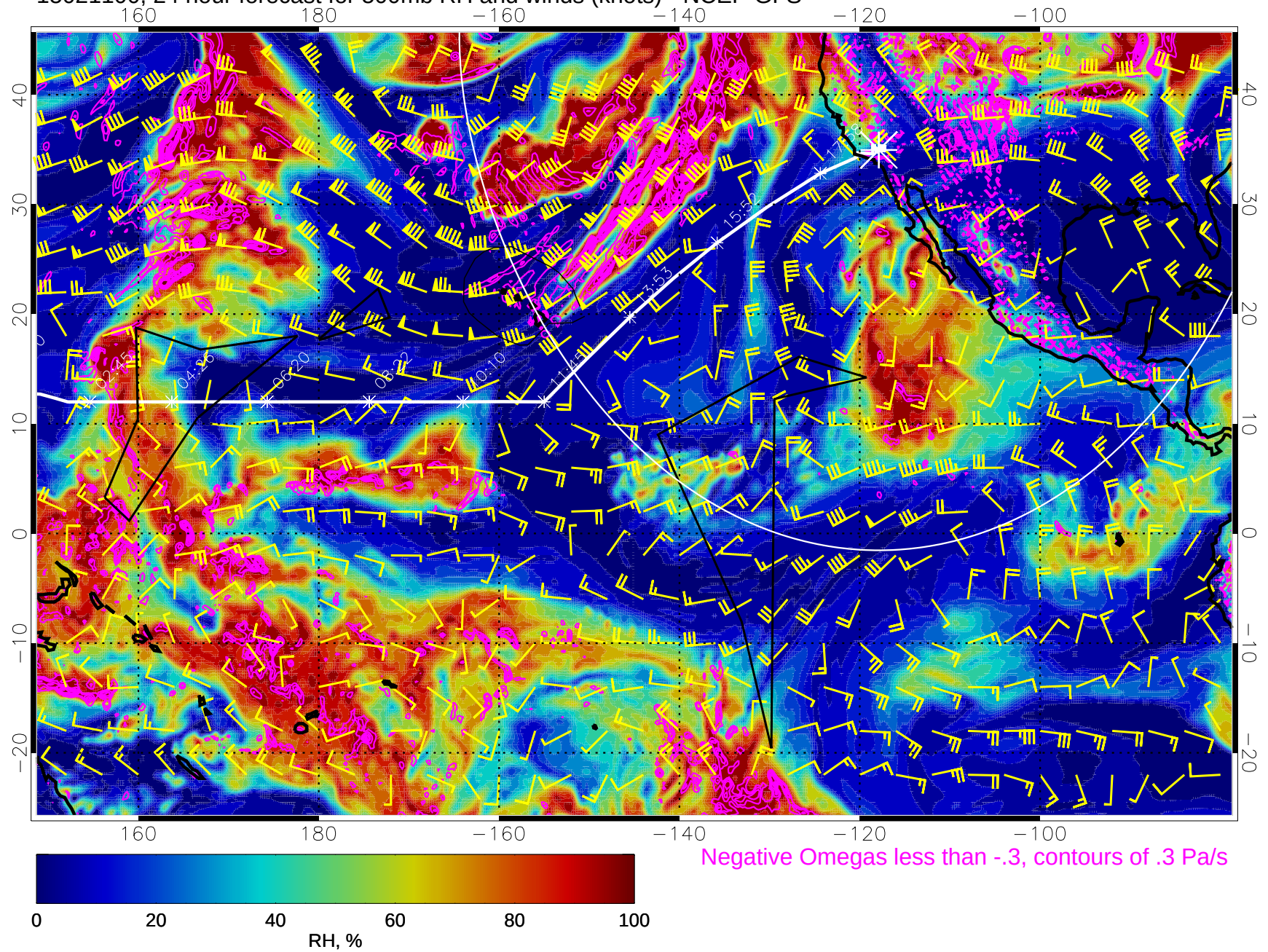
15021100, 24 hour forecast for 500mb RH and winds (knots) - NCEP GFS
