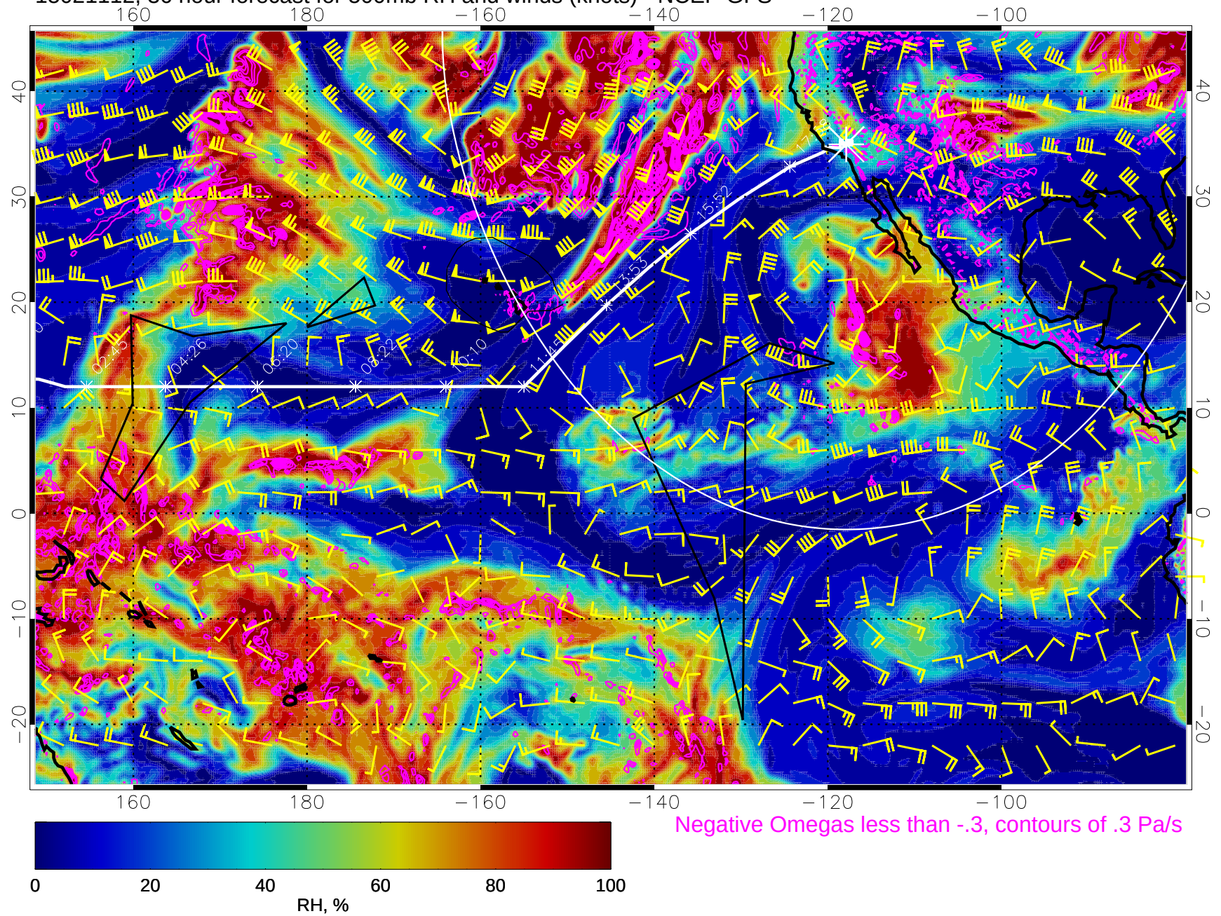
15021112, 36 hour forecast for 500mb RH and winds (knots) - NCEP GFS
