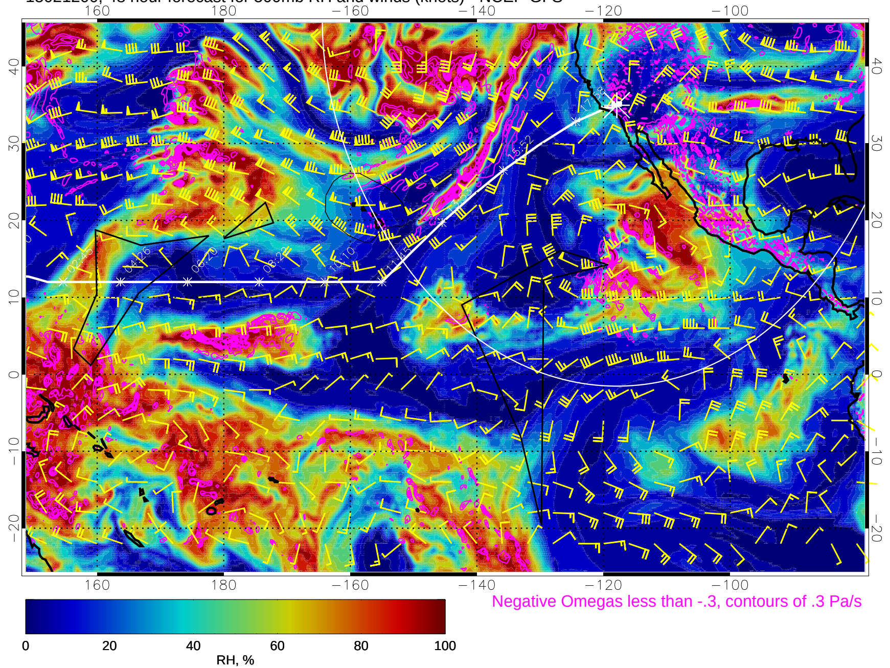
15021200, 48 hour forecast for 500mb RH and winds (knots) - NCEP GFS
