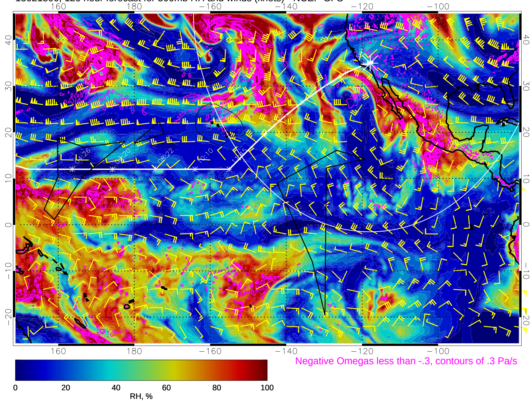
15021500, 120 hour forecast for 500mb RH and winds (knots) - NCEP GFS
