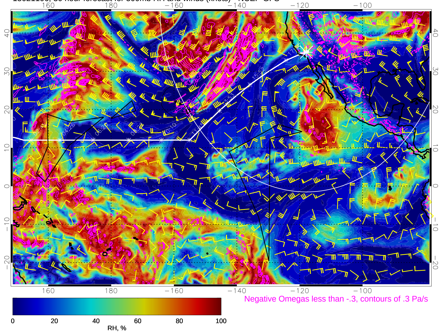
15021106, 30 hour forecast for 500mb RH and winds (knots) - NCEP GFS
