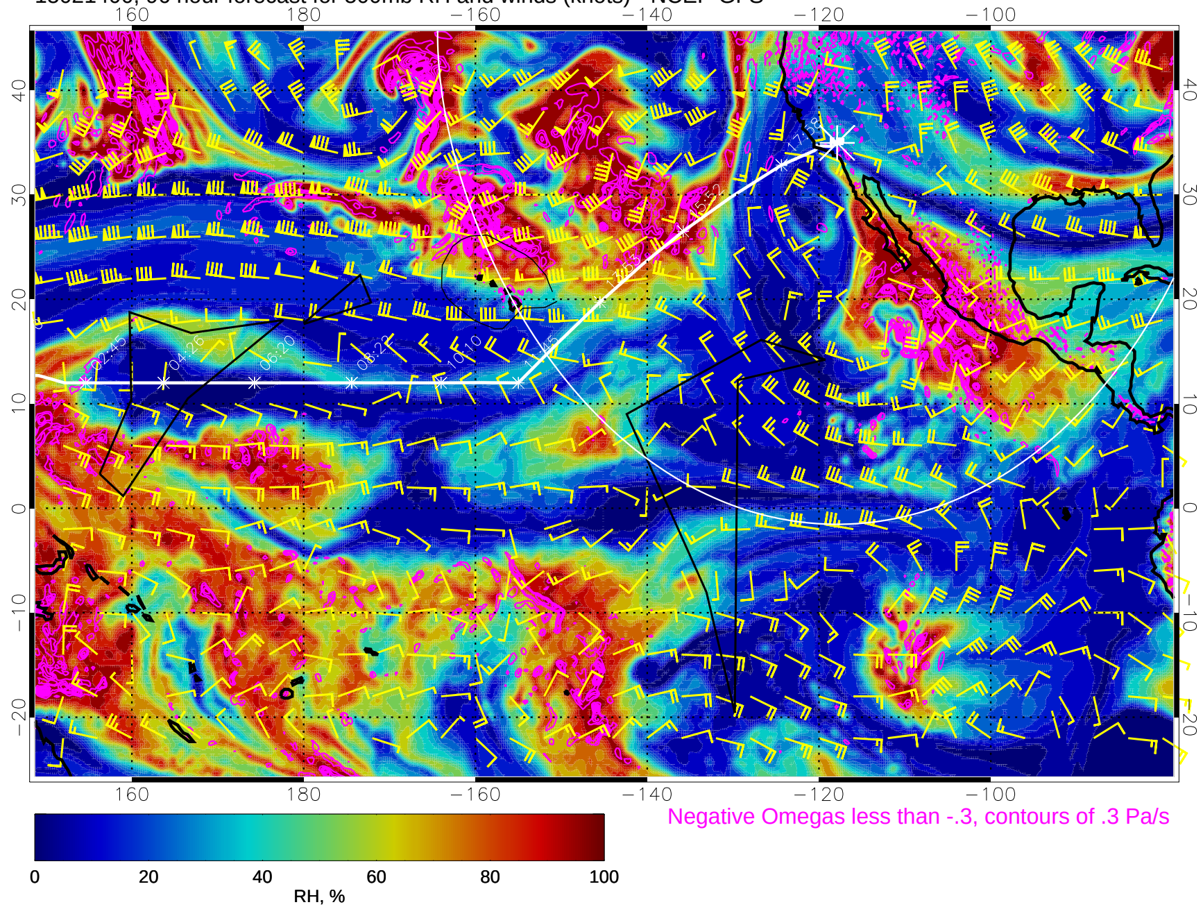
15021400, 96 hour forecast for 500mb RH and winds (knots) - NCEP GFS
