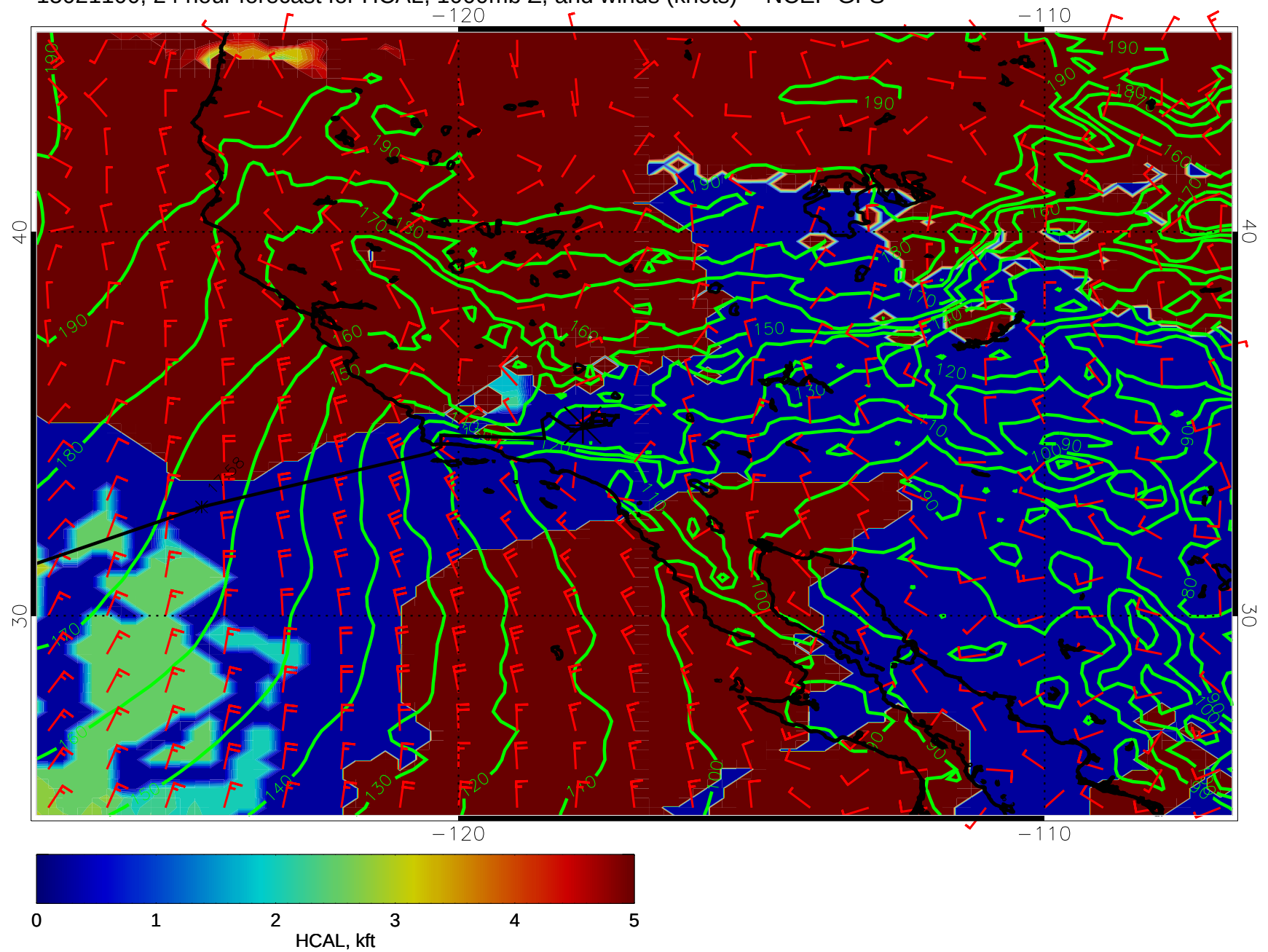
15021100, 24 hour forecast for HCAL, 1000mb Z, and winds (knots) -- NCEP GFS
