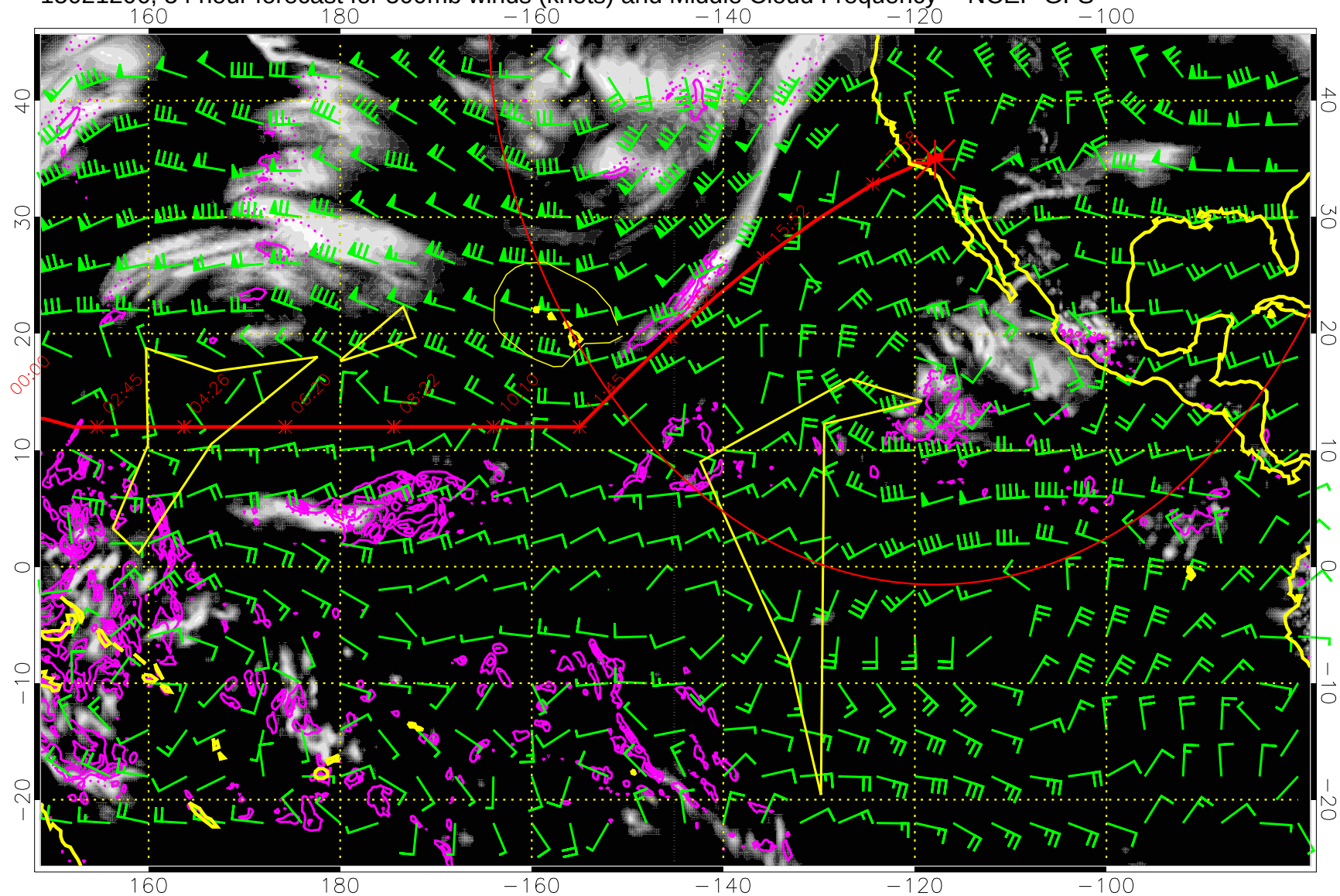
15021206, 54 hour forecast for 500mb winds (knots) and Middle Cloud Frequency -- NCEP GFS
