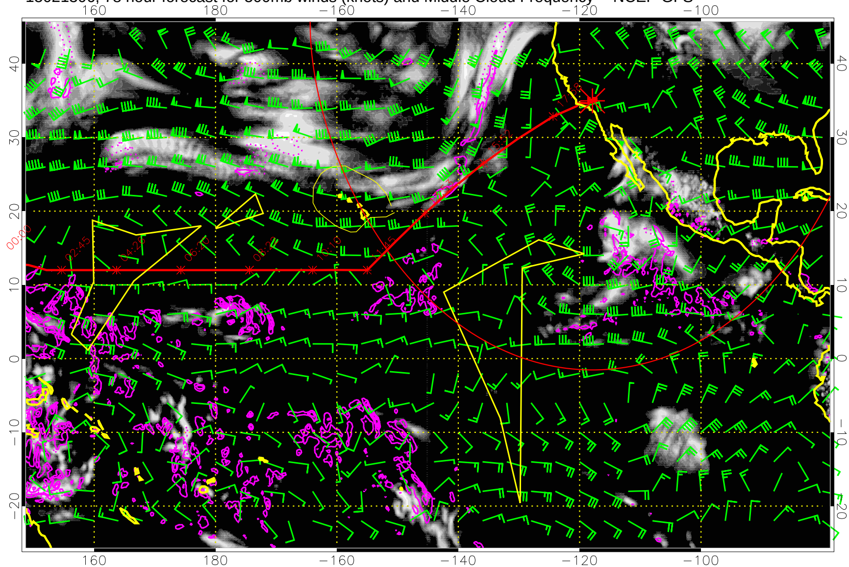
15021306, 78 hour forecast for 500mb winds (knots) and Middle Cloud Frequency -- NCEP GFS
