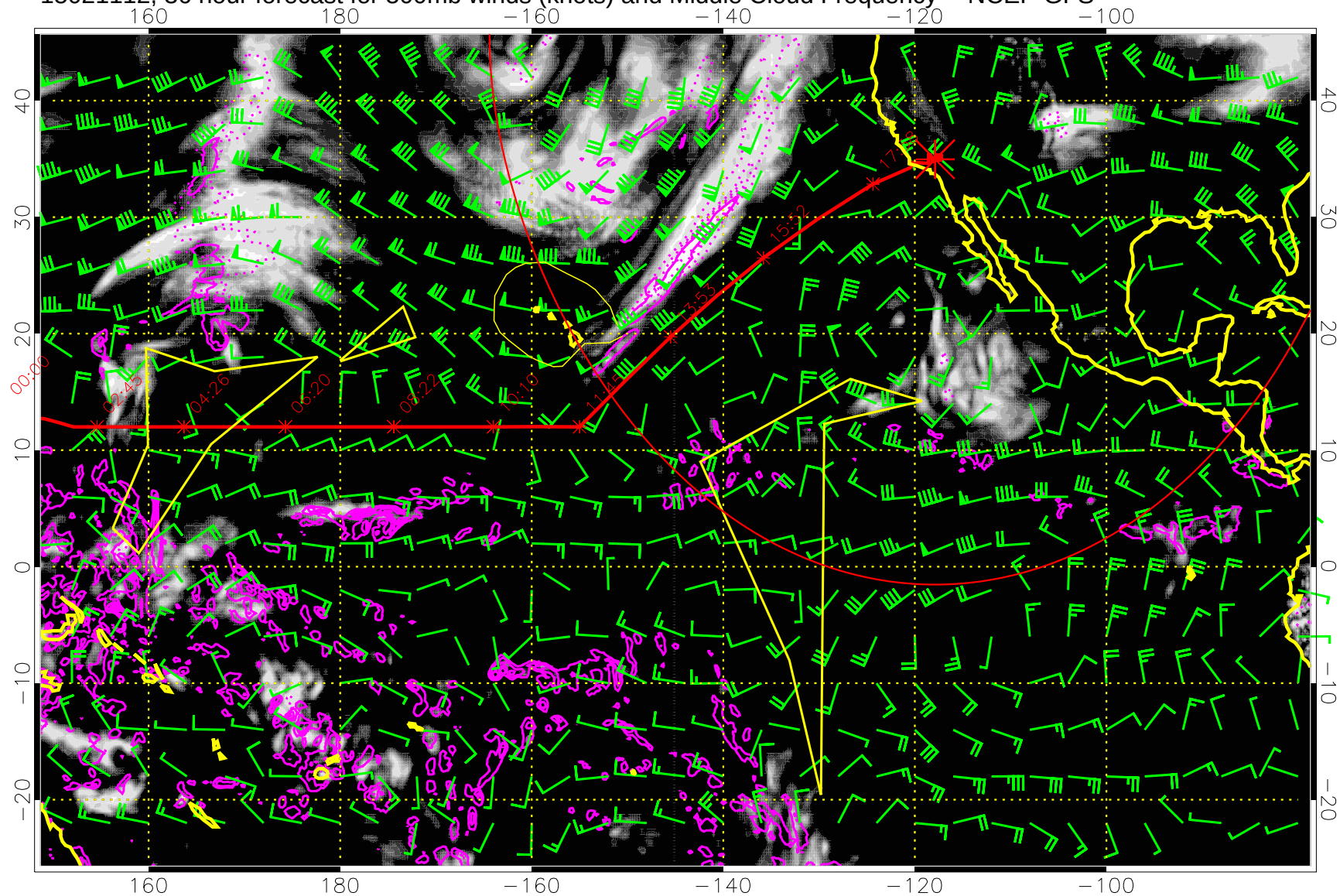
15021112, 36 hour forecast for 500mb winds (knots) and Middle Cloud Frequency -- NCEP GFS
