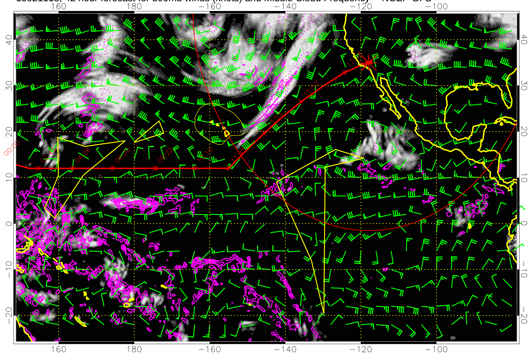
15021118, 42 hour forecast for 500mb winds (knots) and Middle Cloud Frequency -- NCEP GFS
