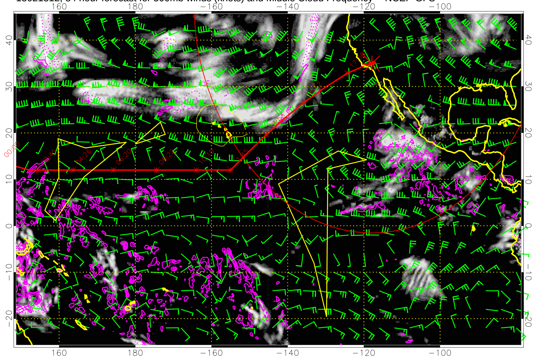
15021312, 84 hour forecast for 500mb winds (knots) and Middle Cloud Frequency -- NCEP GFS
