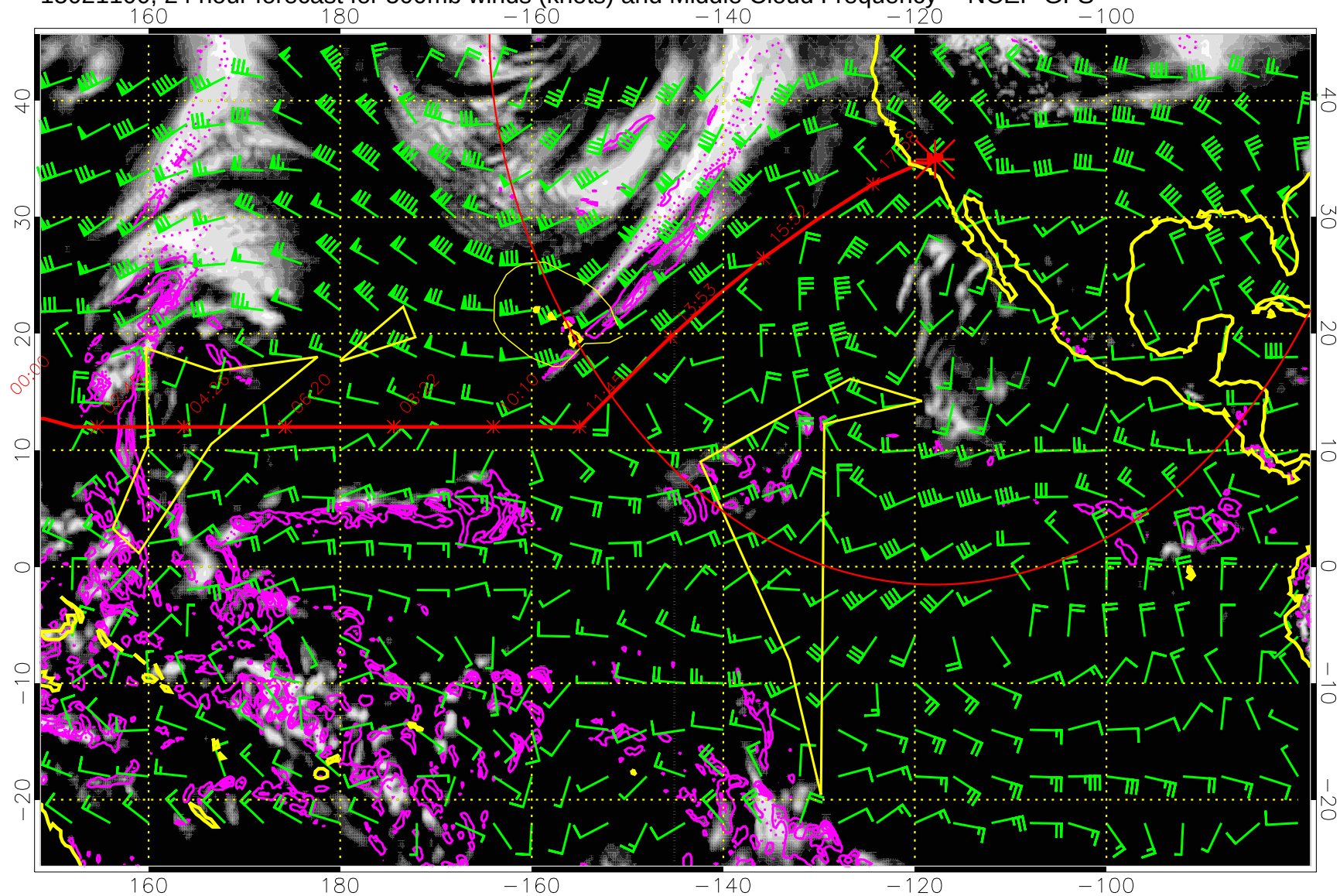
15021100, 24 hour forecast for 500mb winds (knots) and Middle Cloud Frequency -- NCEP GFS
