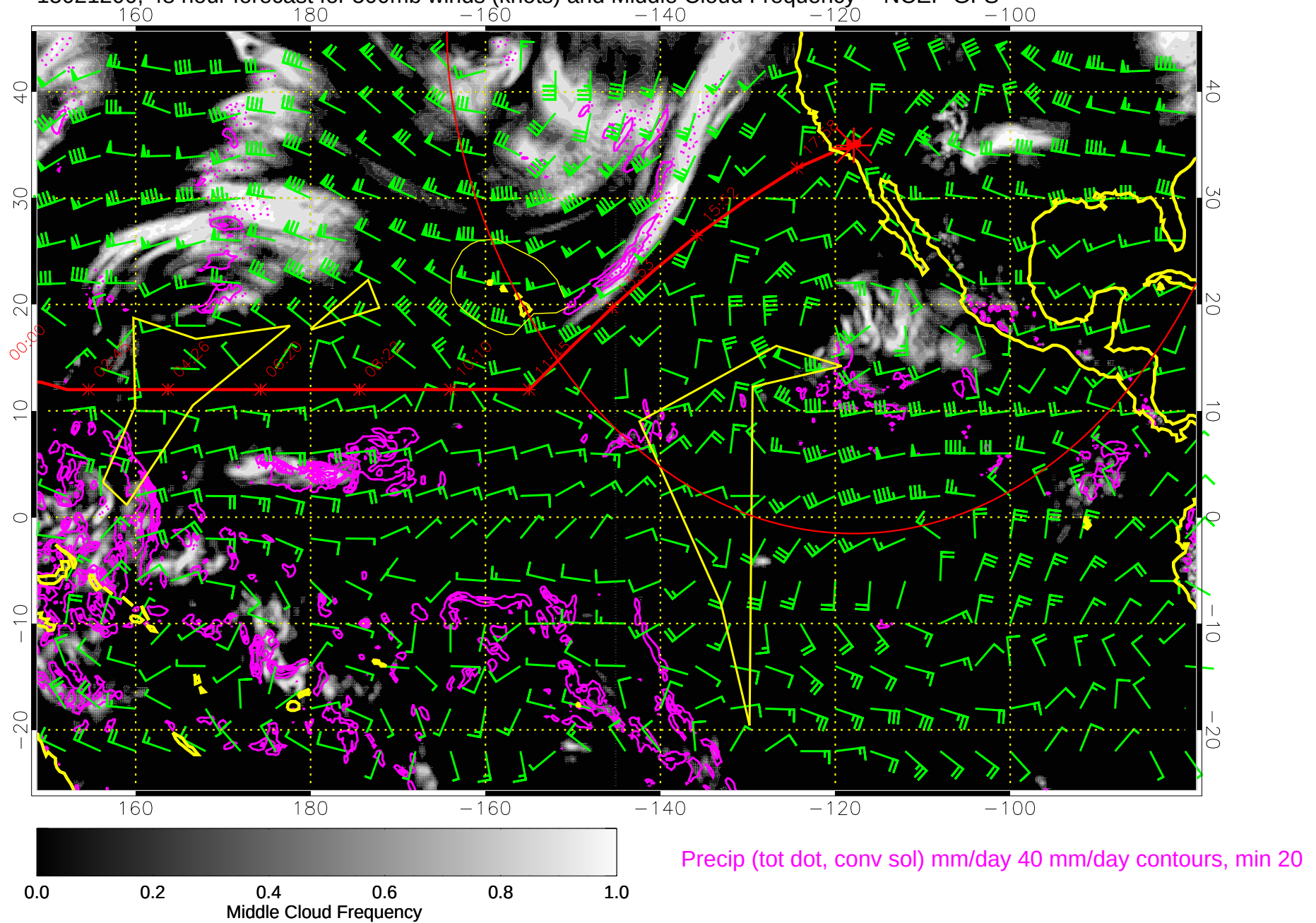
15021200, 48 hour forecast for 500mb winds (knots) and Middle Cloud Frequency -- NCEP GFS
