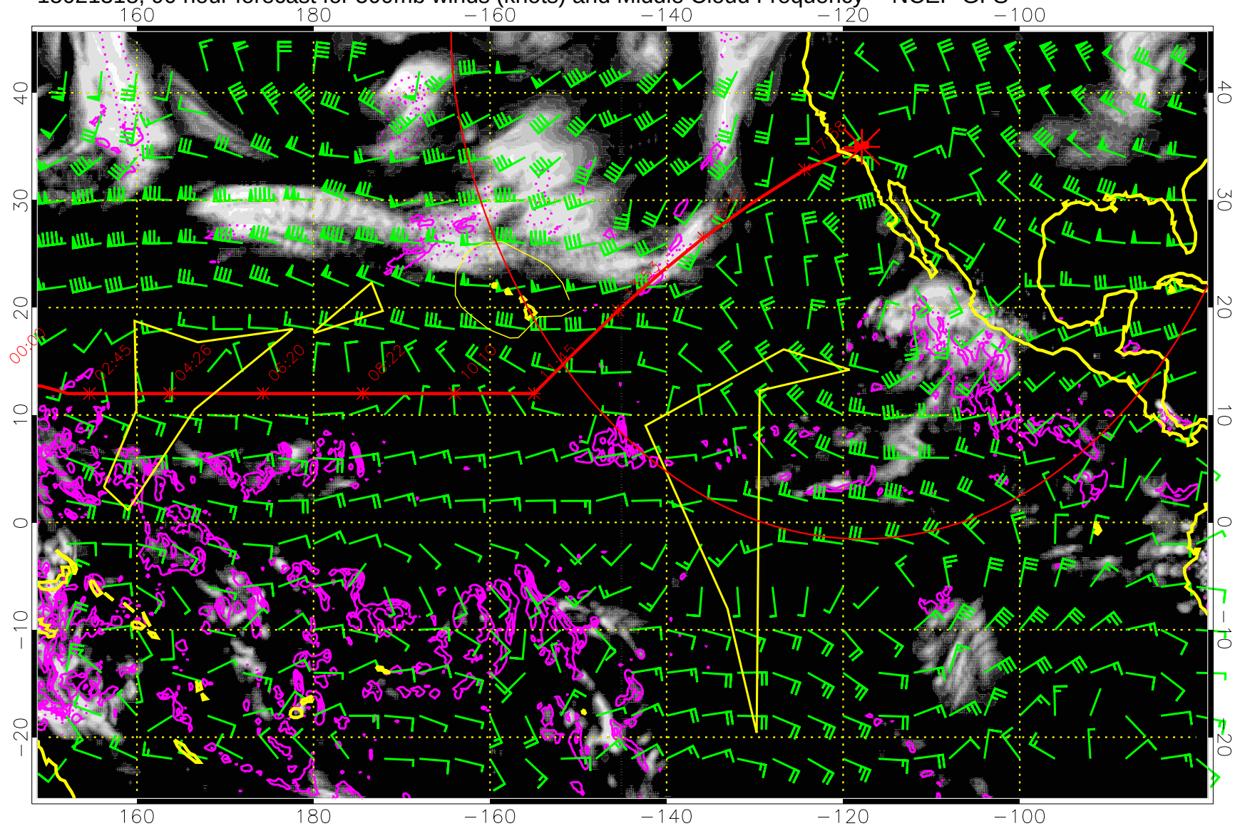
15021318, 90 hour forecast for 500mb winds (knots) and Middle Cloud Frequency -- NCEP GFS
