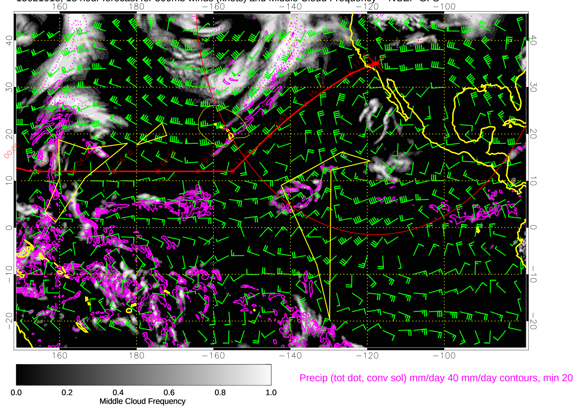
15021018, 18 hour forecast for 500mb winds (knots) and Middle Cloud Frequency -- NCEP GFS
