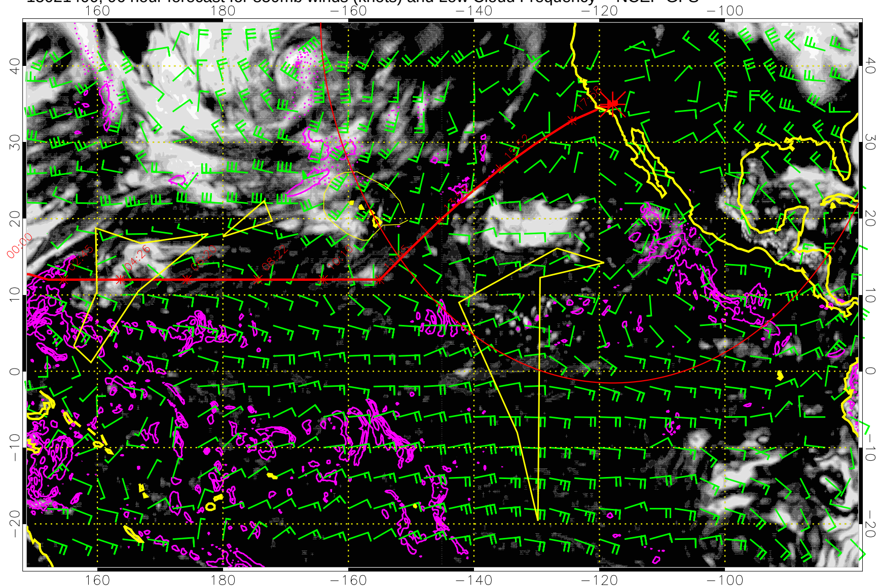
15021400, 96 hour forecast for 850mb winds (knots) and Low Cloud Frequency -- NCEP GFS
