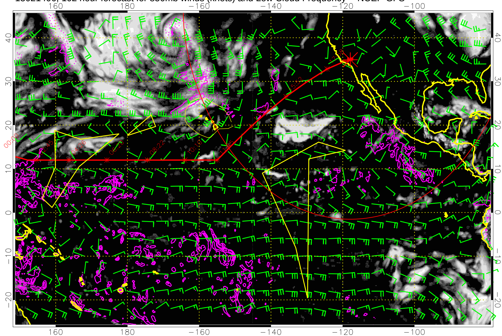
15021406, 102 hour forecast for 850mb winds (knots) and Low Cloud Frequency -- NCEP GFS
