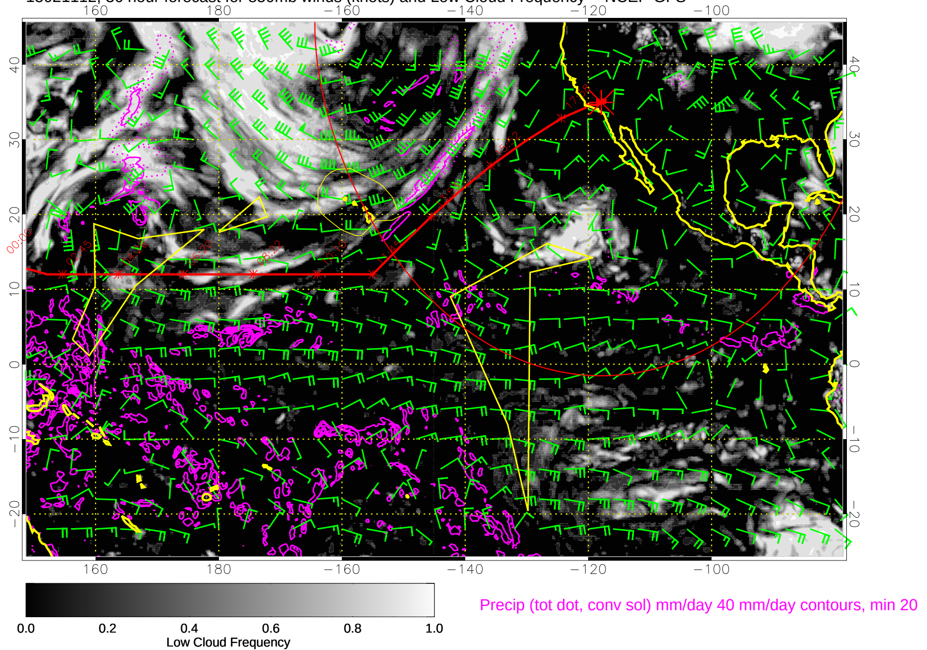
15021112, 36 hour forecast for 850mb winds (knots) and Low Cloud Frequency -- NCEP GFS
