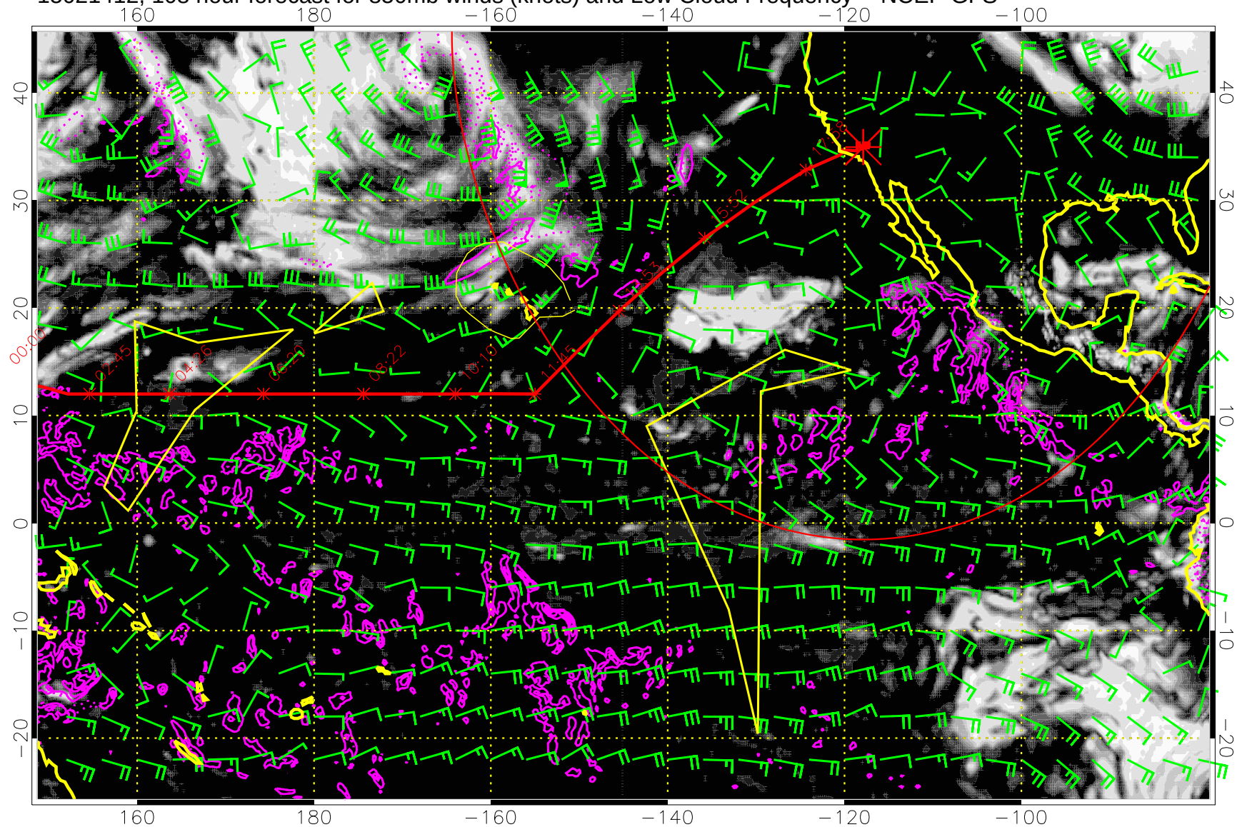
15021412, 108 hour forecast for 850mb winds (knots) and Low Cloud Frequency -- NCEP GFS
