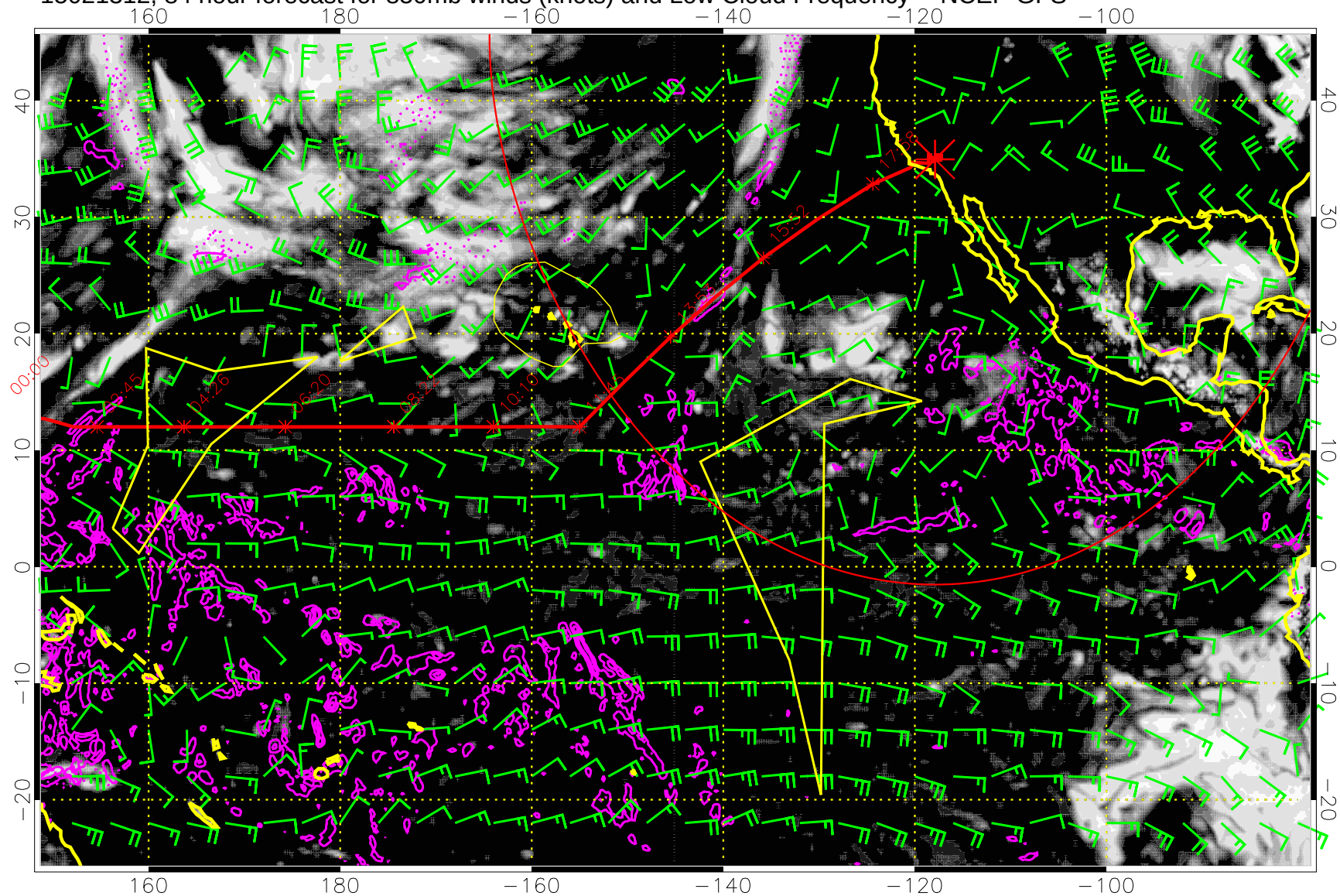
15021312, 84 hour forecast for 850mb winds (knots) and Low Cloud Frequency -- NCEP GFS
