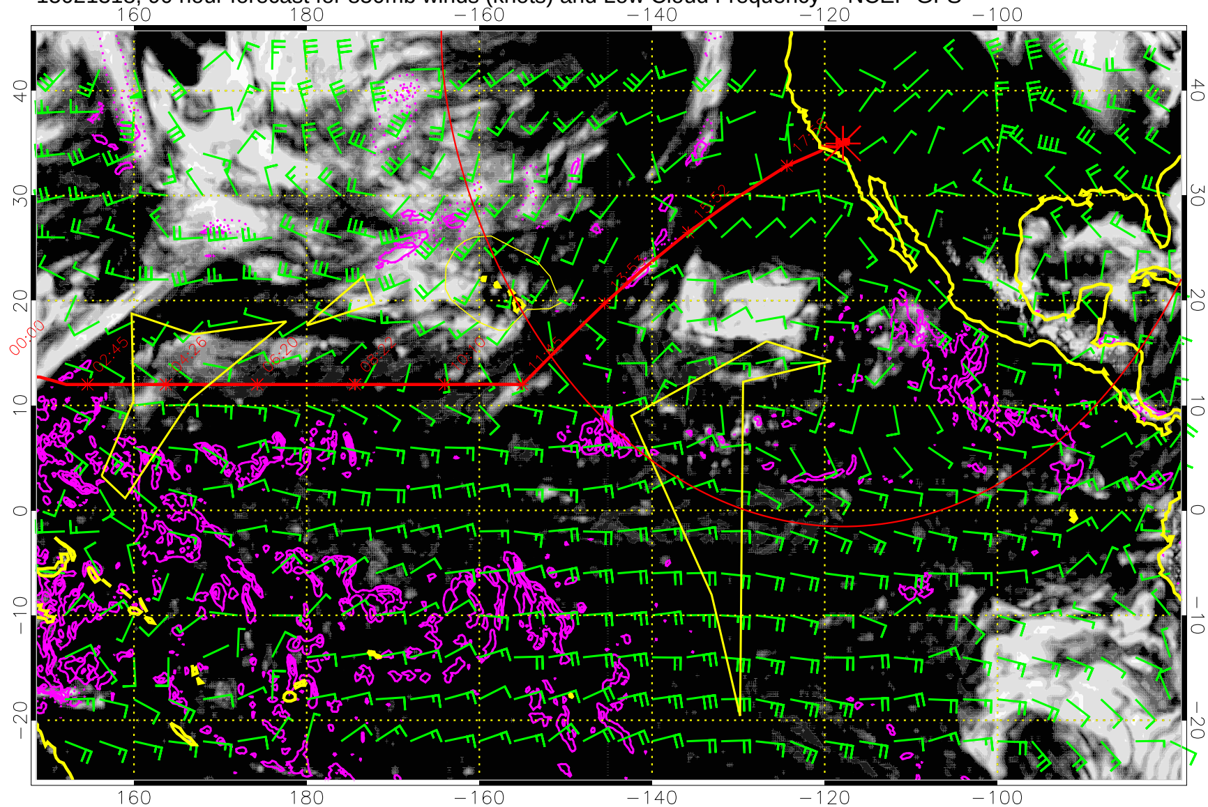
15021318, 90 hour forecast for 850mb winds (knots) and Low Cloud Frequency -- NCEP GFS
