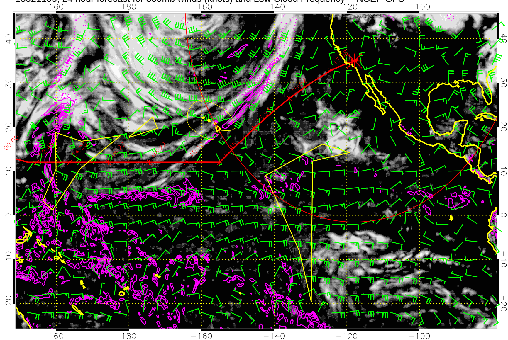
15021100, 24 hour forecast for 850mb winds (knots) and Low Cloud Frequency -- NCEP GFS
