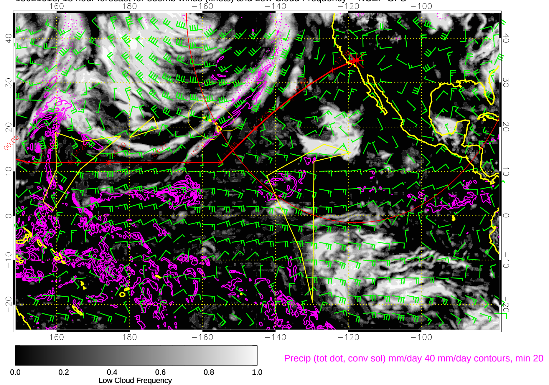
15021018, 18 hour forecast for 850mb winds (knots) and Low Cloud Frequency -- NCEP GFS
