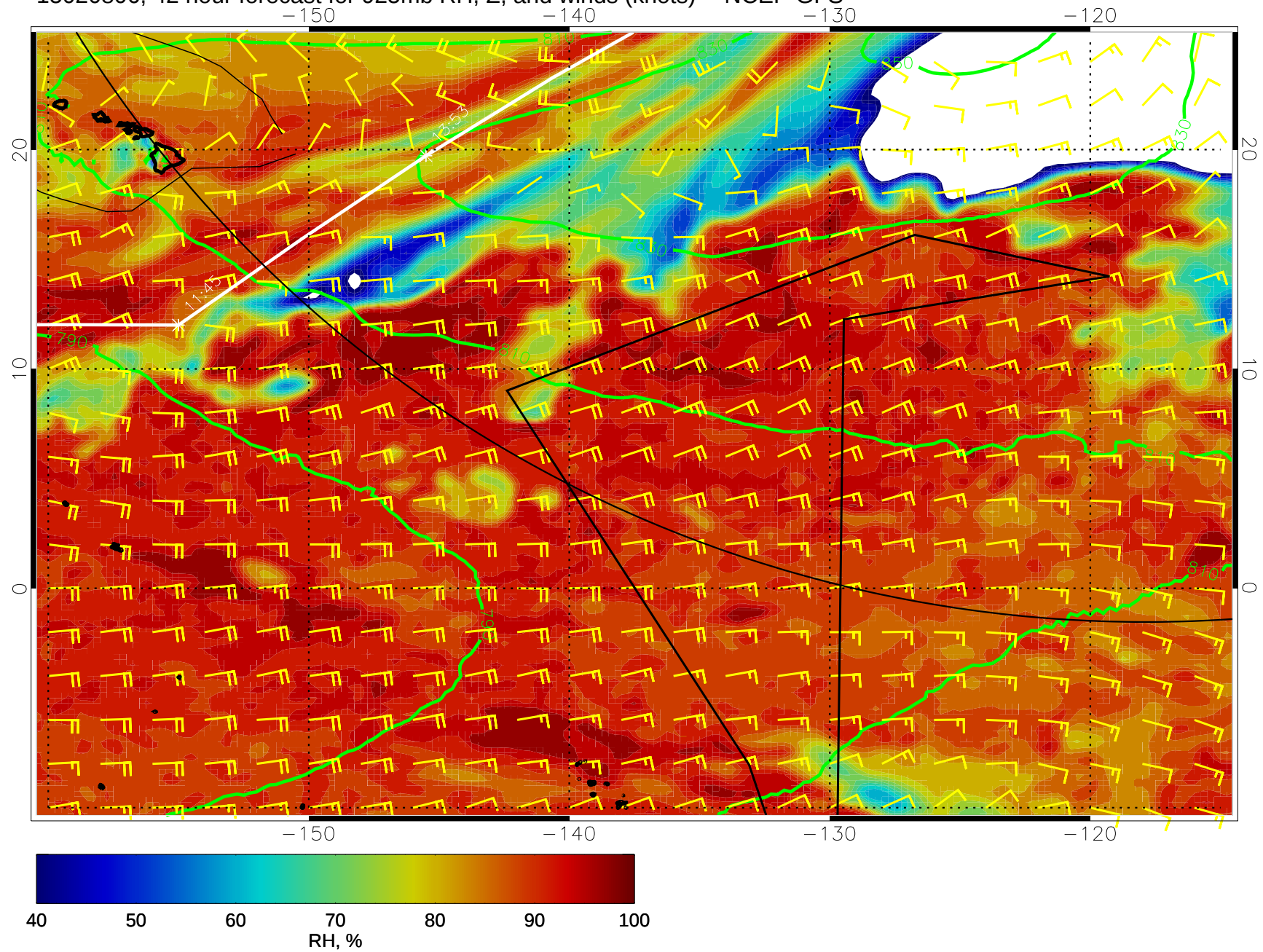
15020806, 42 hour forecast for 925mb RH, Z, and winds (knots) -- NCEP GFS
