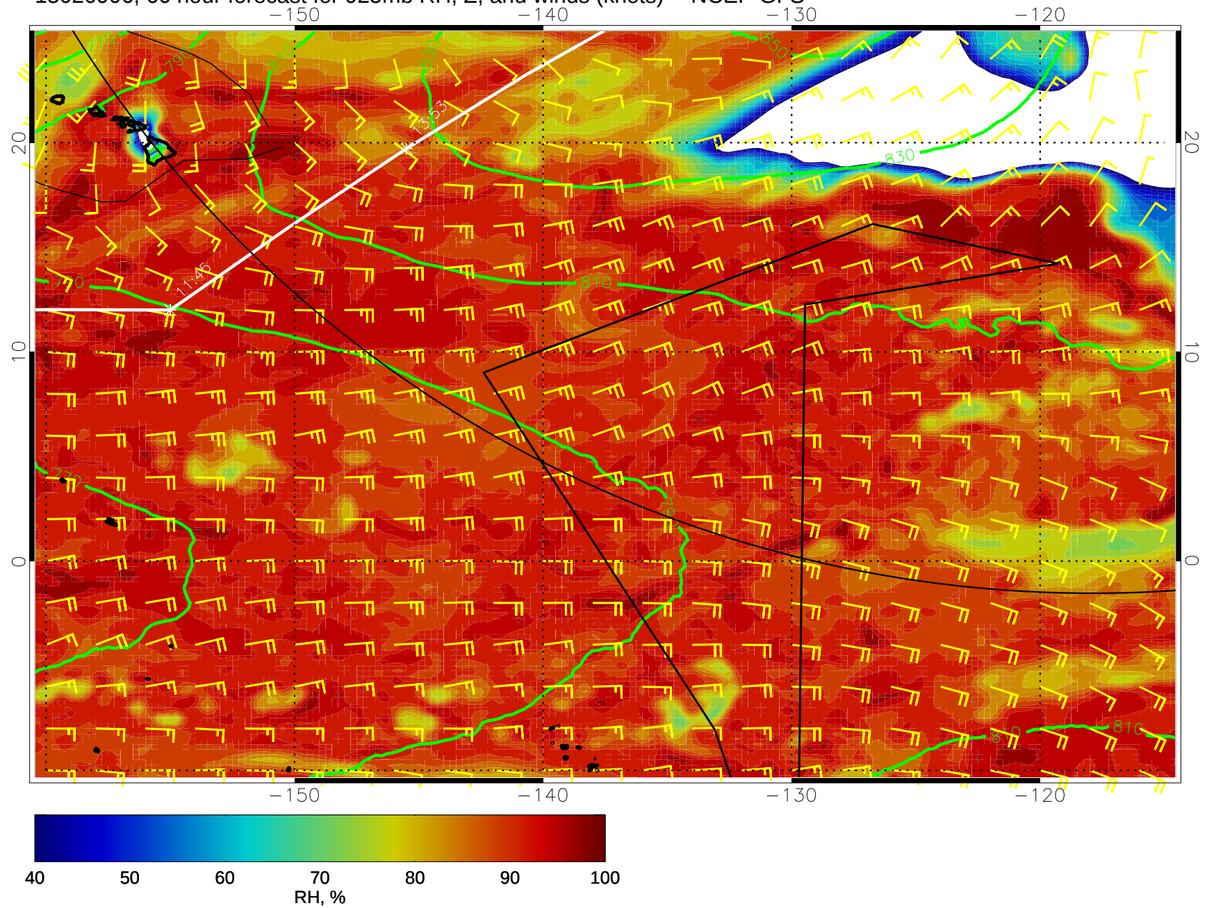
15020906, 66 hour forecast for 925mb RH, Z, and winds (knots) -- NCEP GFS
