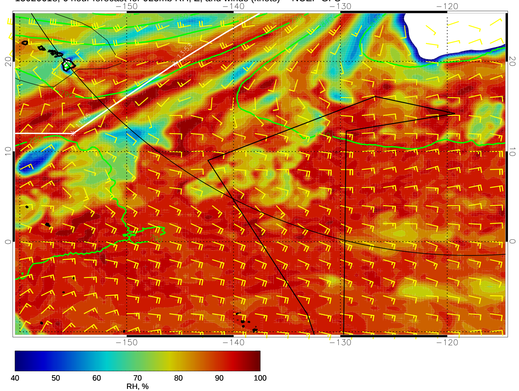
15020618, 6 hour forecast for 925mb RH, Z, and winds (knots) -- NCEP GFS
