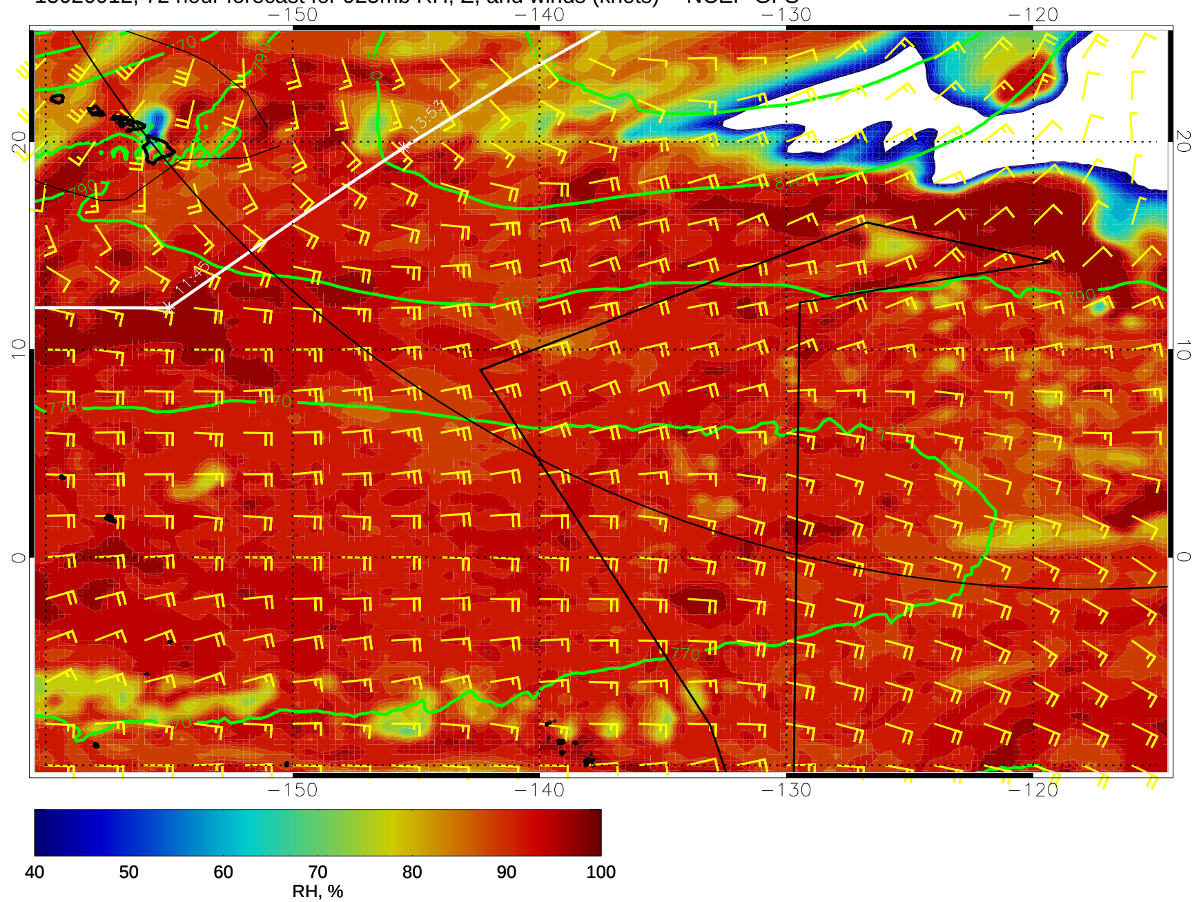
15020912, 72 hour forecast for 925mb RH, Z, and winds (knots) -- NCEP GFS
