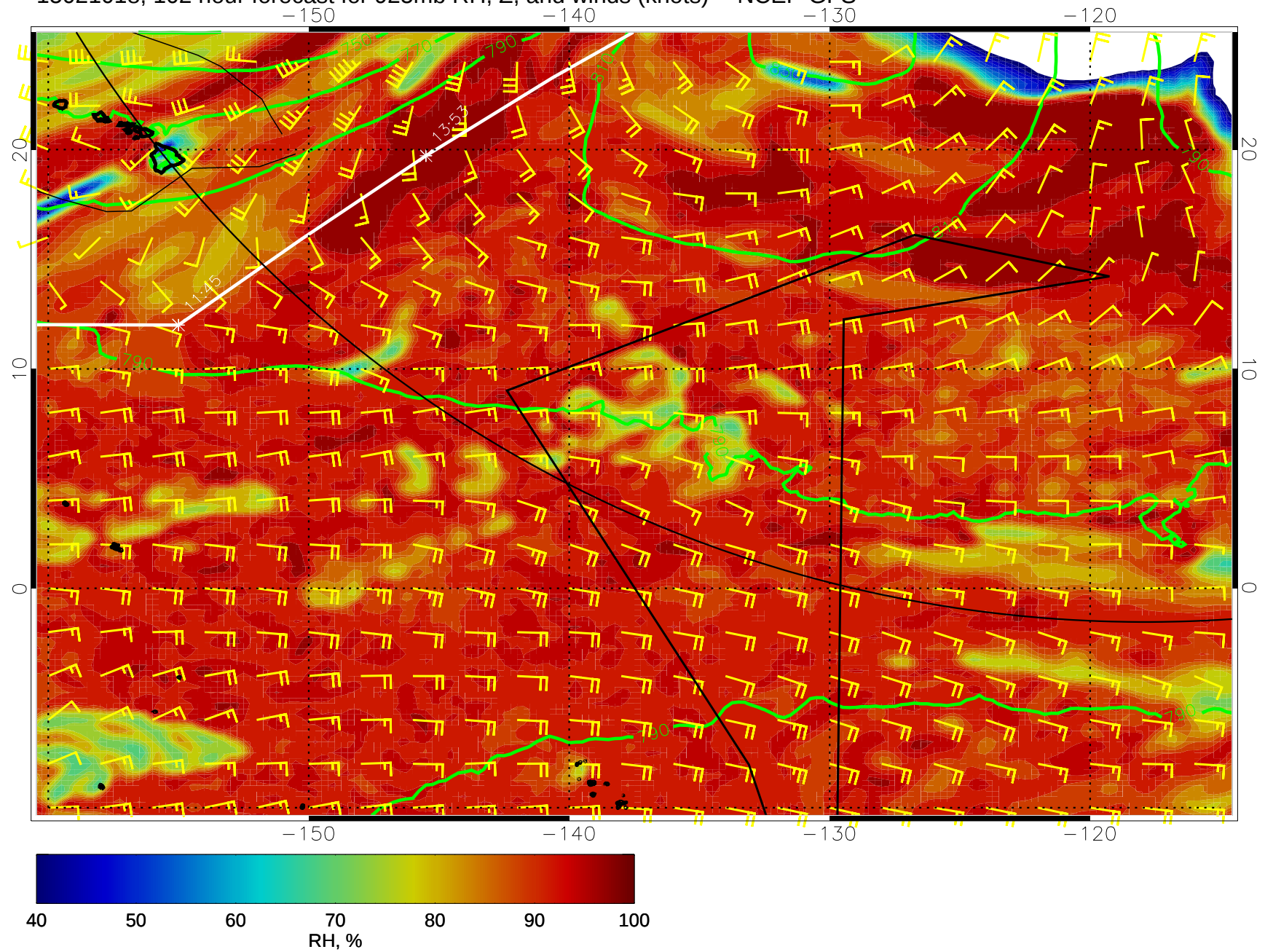
15021018, 102 hour forecast for 925mb RH, Z, and winds (knots) -- NCEP GFS
