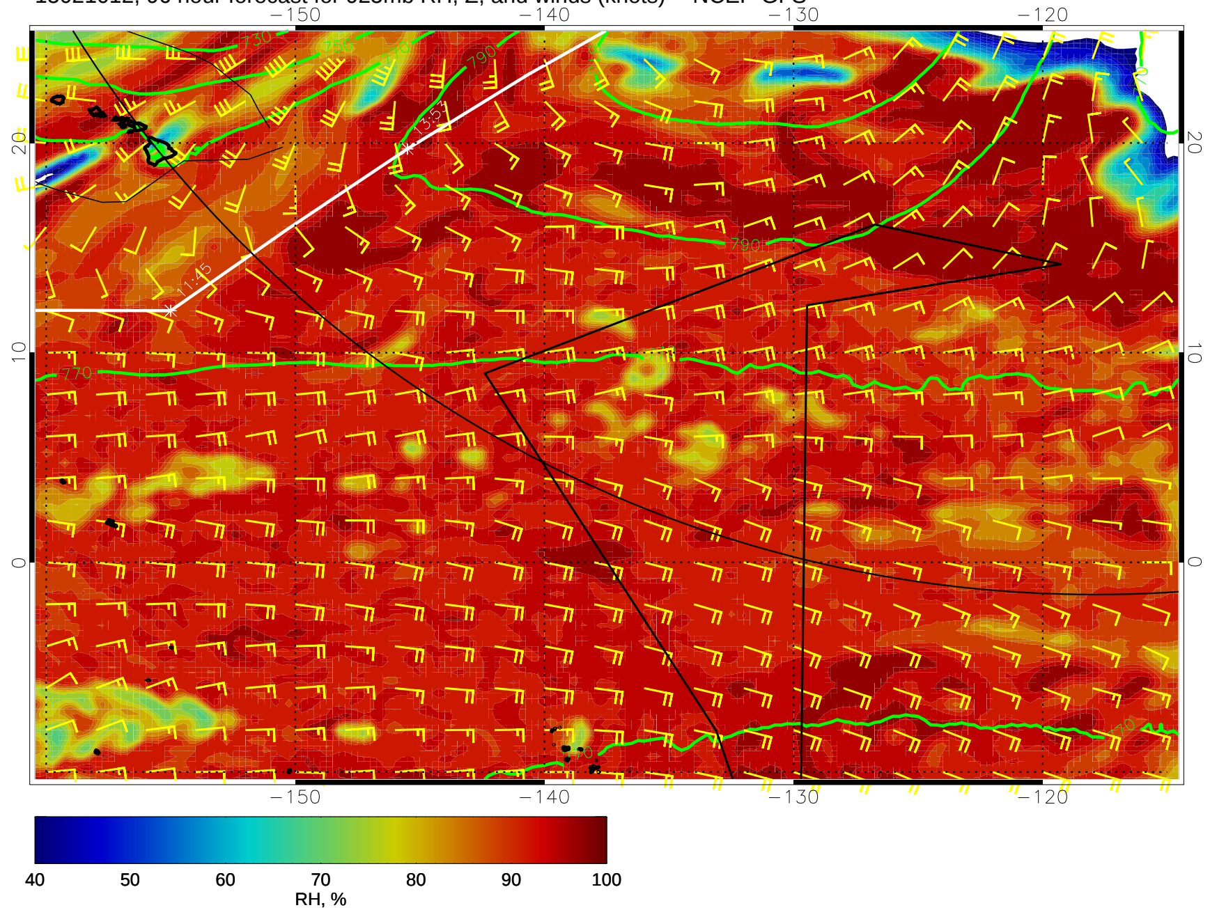
15021012, 96 hour forecast for 925mb RH, Z, and winds (knots) -- NCEP GFS
