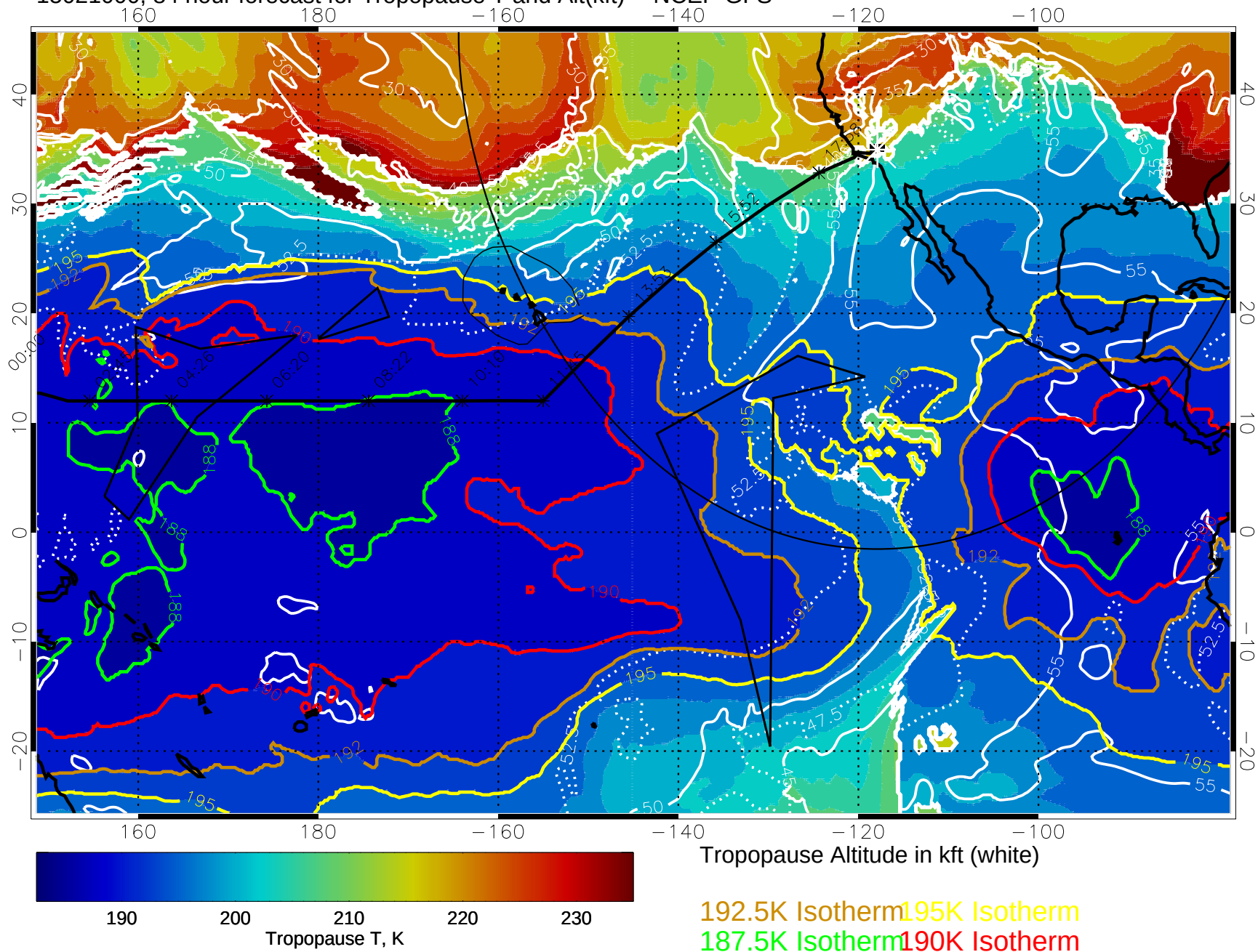
15021000, 84 hour forecast for Tropopause T and Alt(kft) -- NCEP GFS
