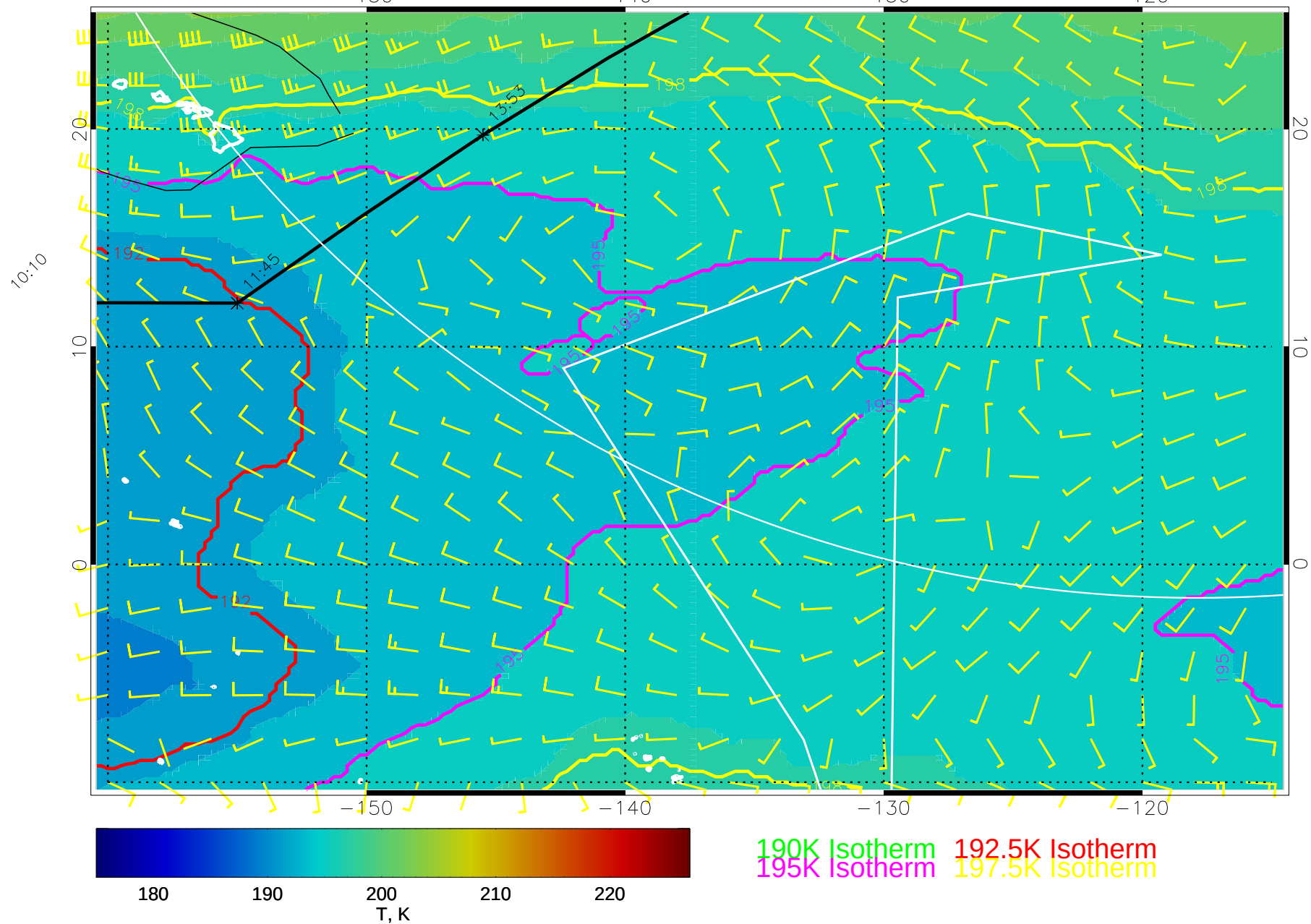
15021018, 102 hour forecast for 70mb T and winds (knots) -- NCEP GFS
