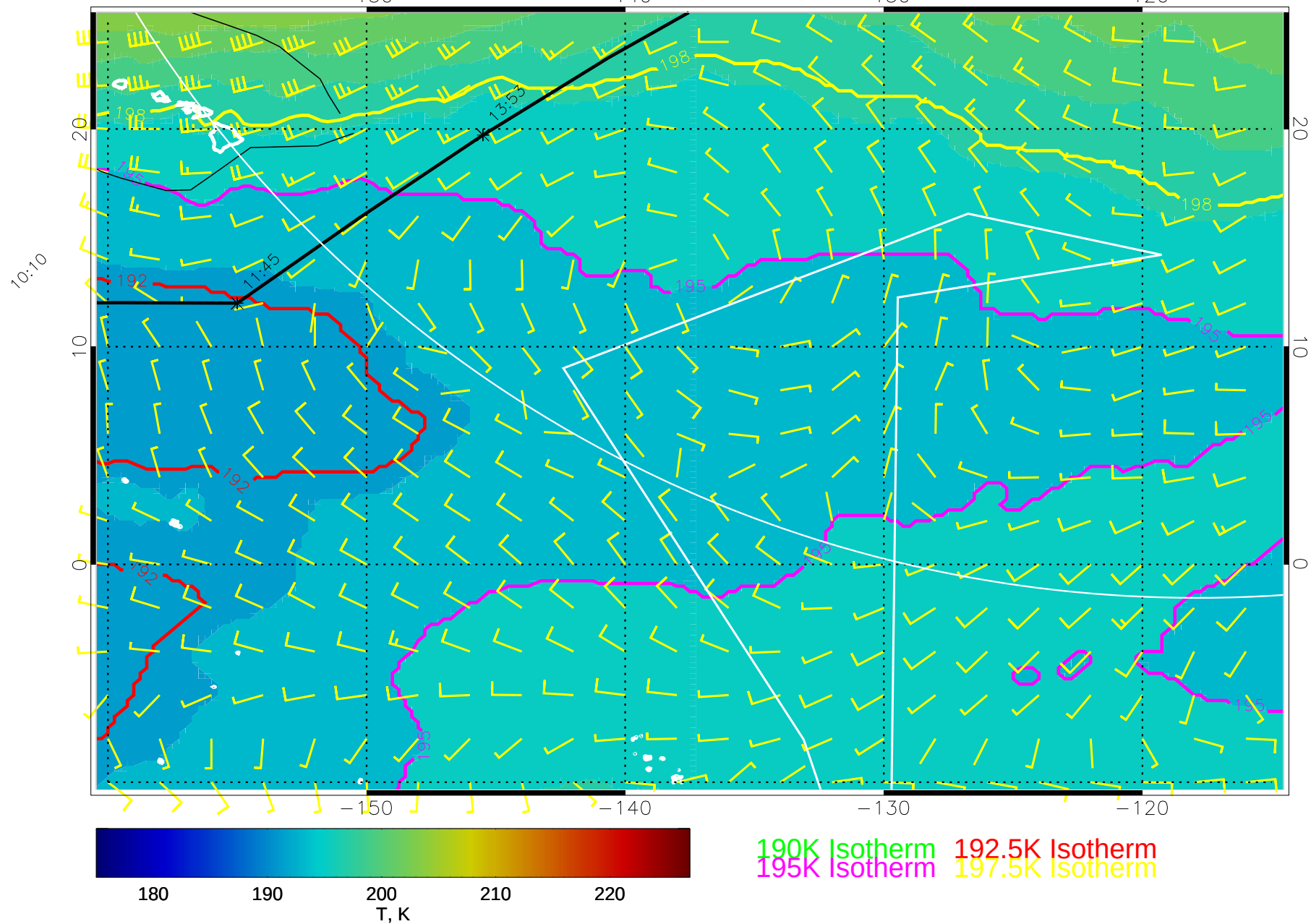
15021100, 108 hour forecast for 70mb T and winds (knots) -- NCEP GFS
