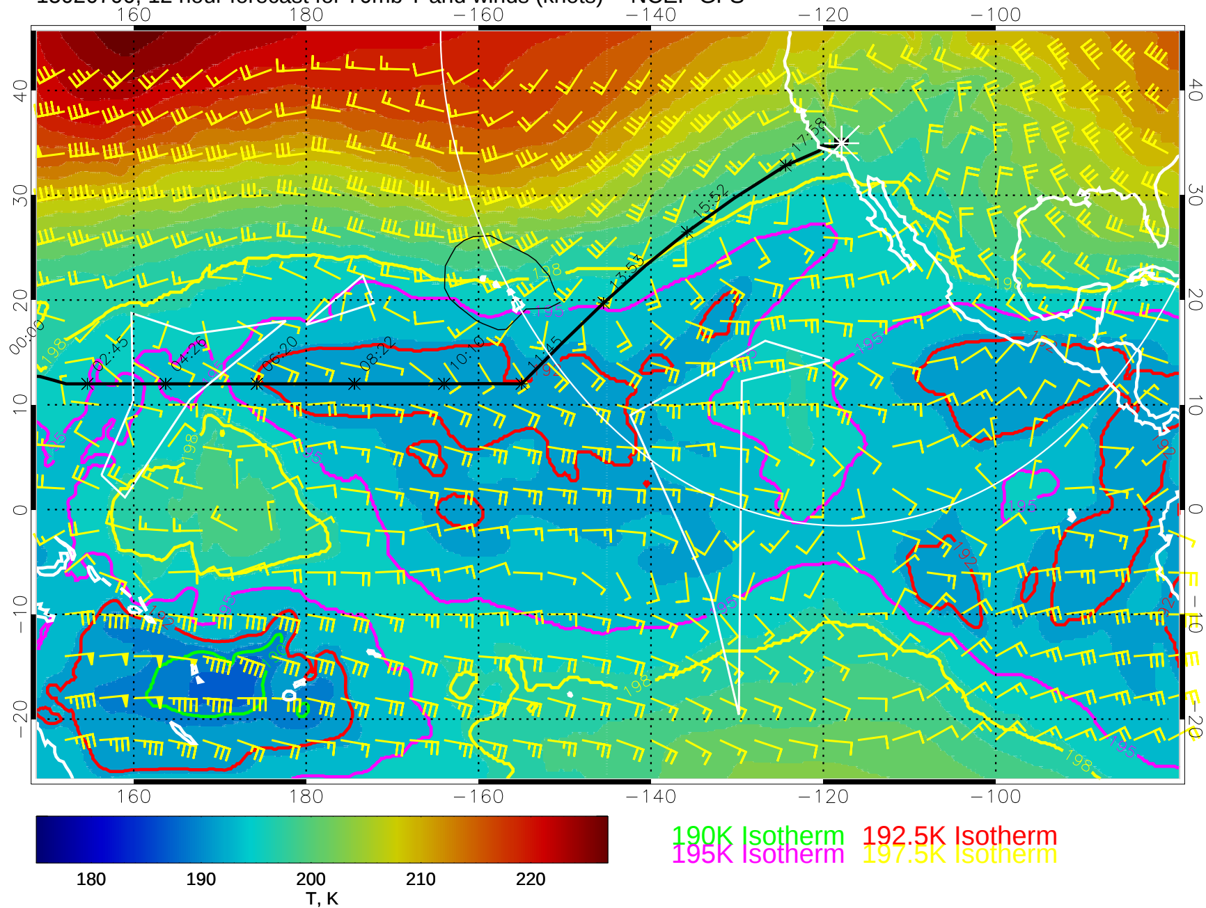
15020700, 12 hour forecast for 70mb T and winds (knots) -- NCEP GFS
