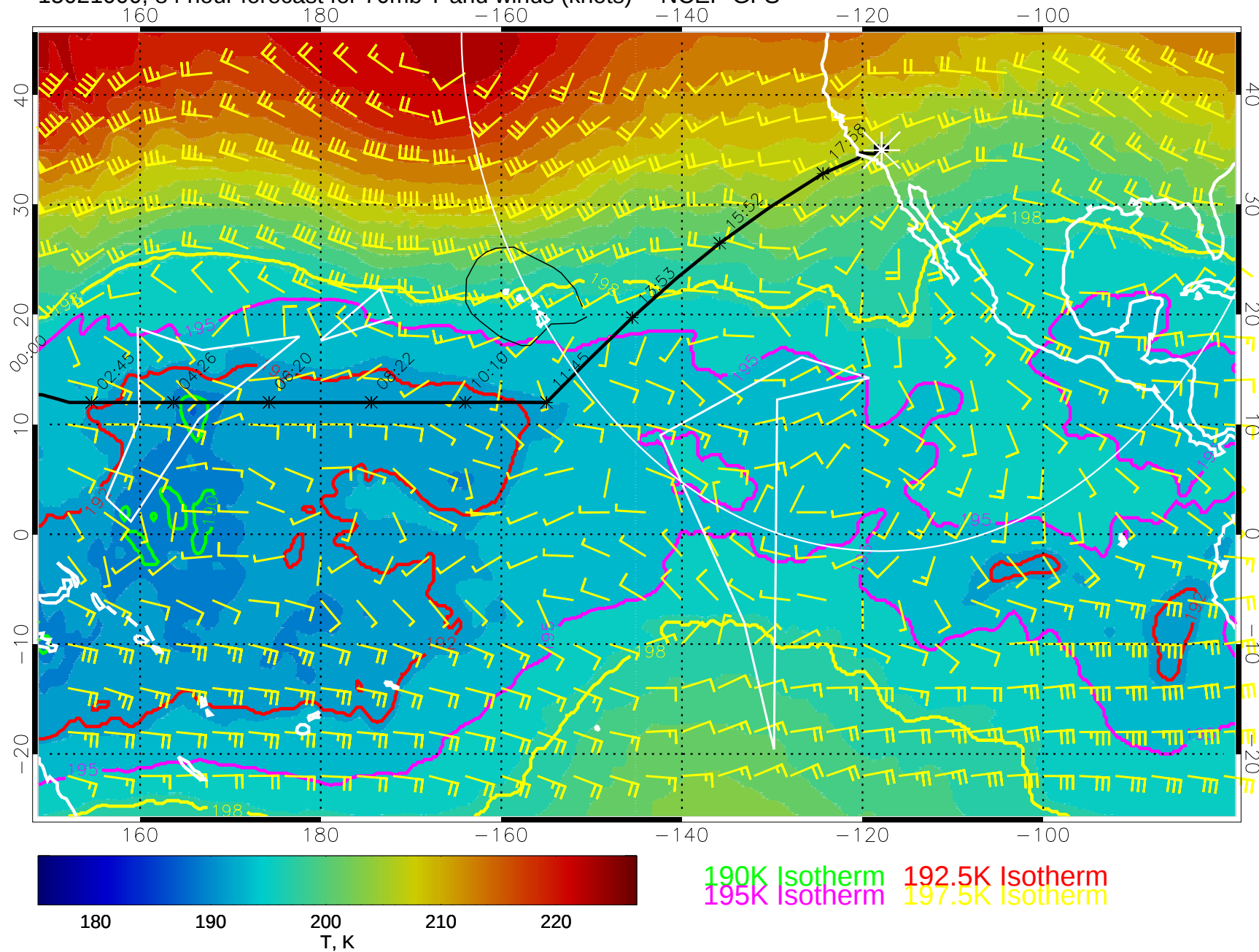
15021000, 84 hour forecast for 70mb T and winds (knots) -- NCEP GFS
