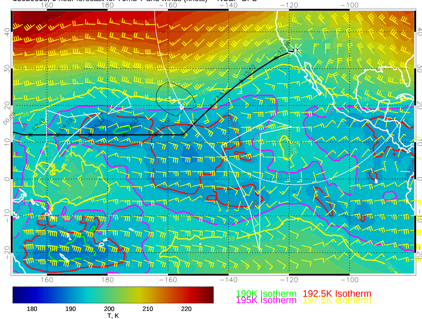
15020618, 6 hour forecast for 70mb T and winds (knots) -- NCEP GFS
