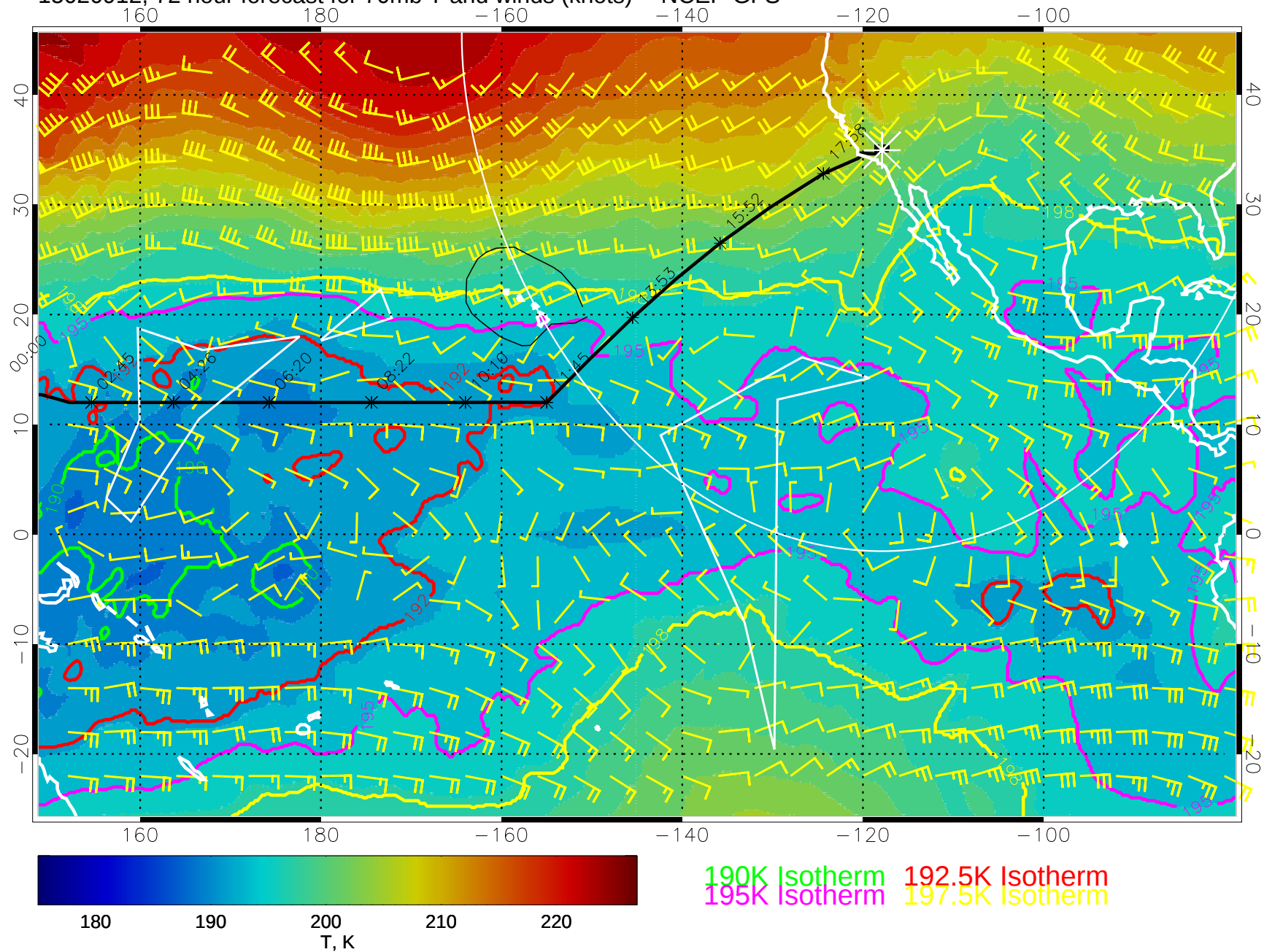
15020912, 72 hour forecast for 70mb T and winds (knots) -- NCEP GFS
