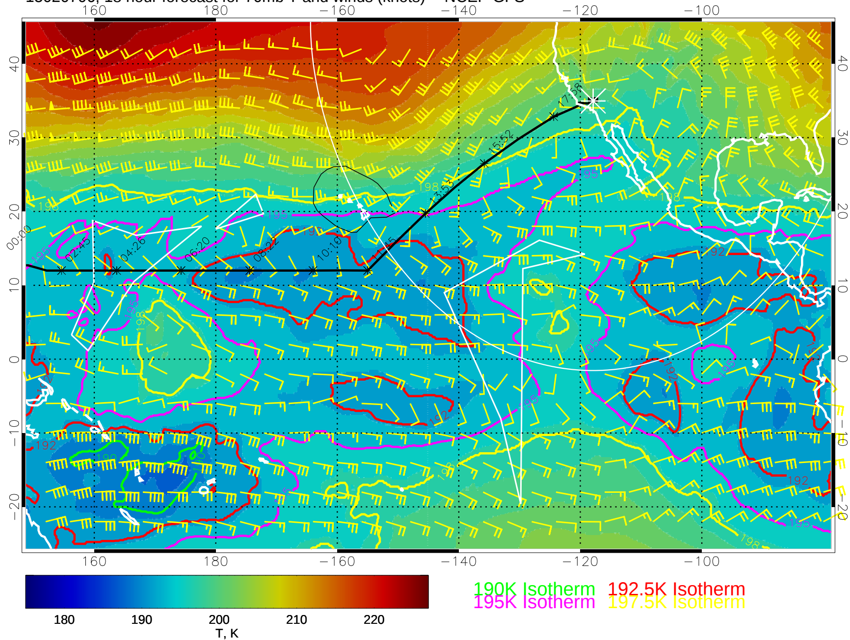
15020706, 18 hour forecast for 70mb T and winds (knots) -- NCEP GFS
