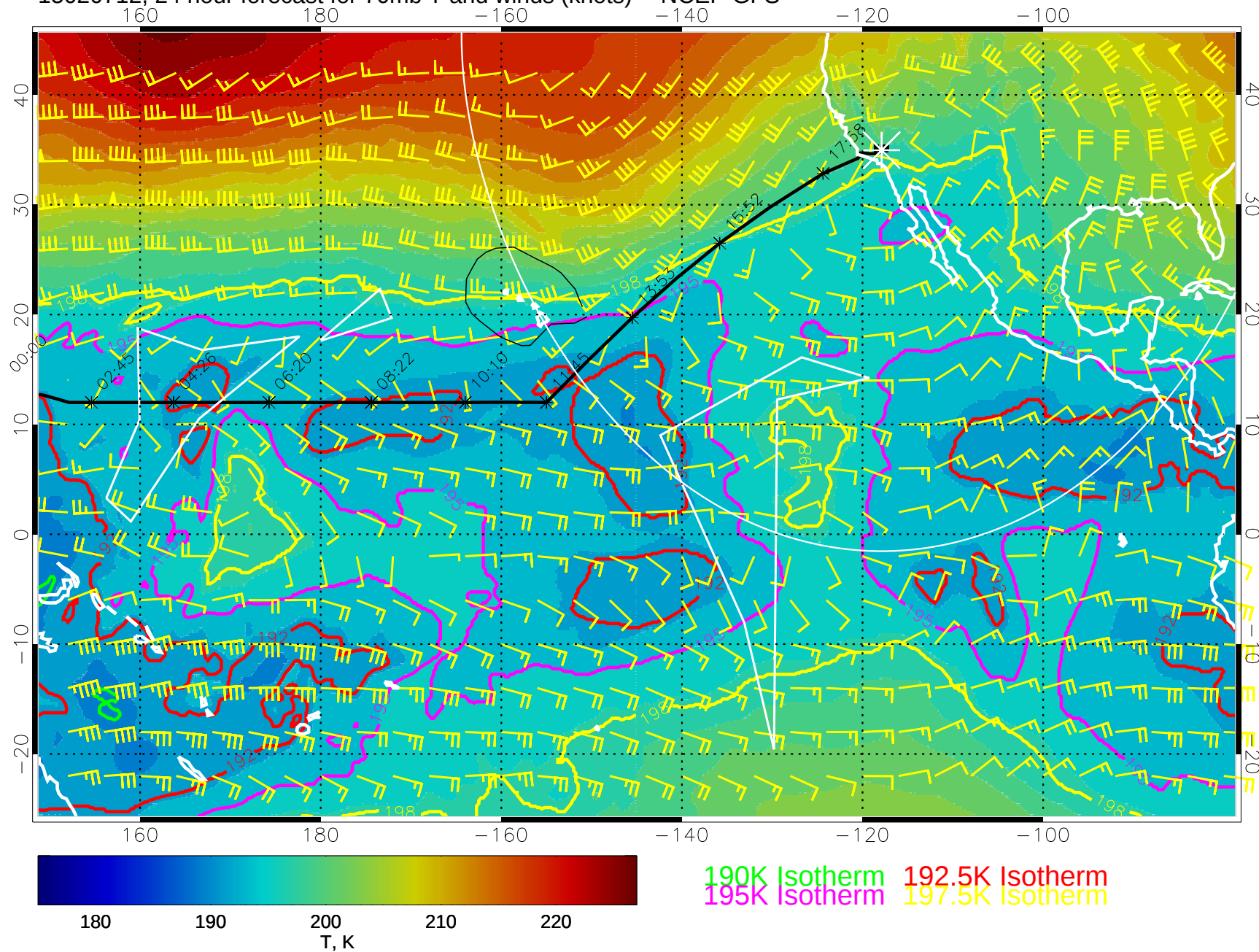
15020712, 24 hour forecast for 70mb T and winds (knots) -- NCEP GFS
