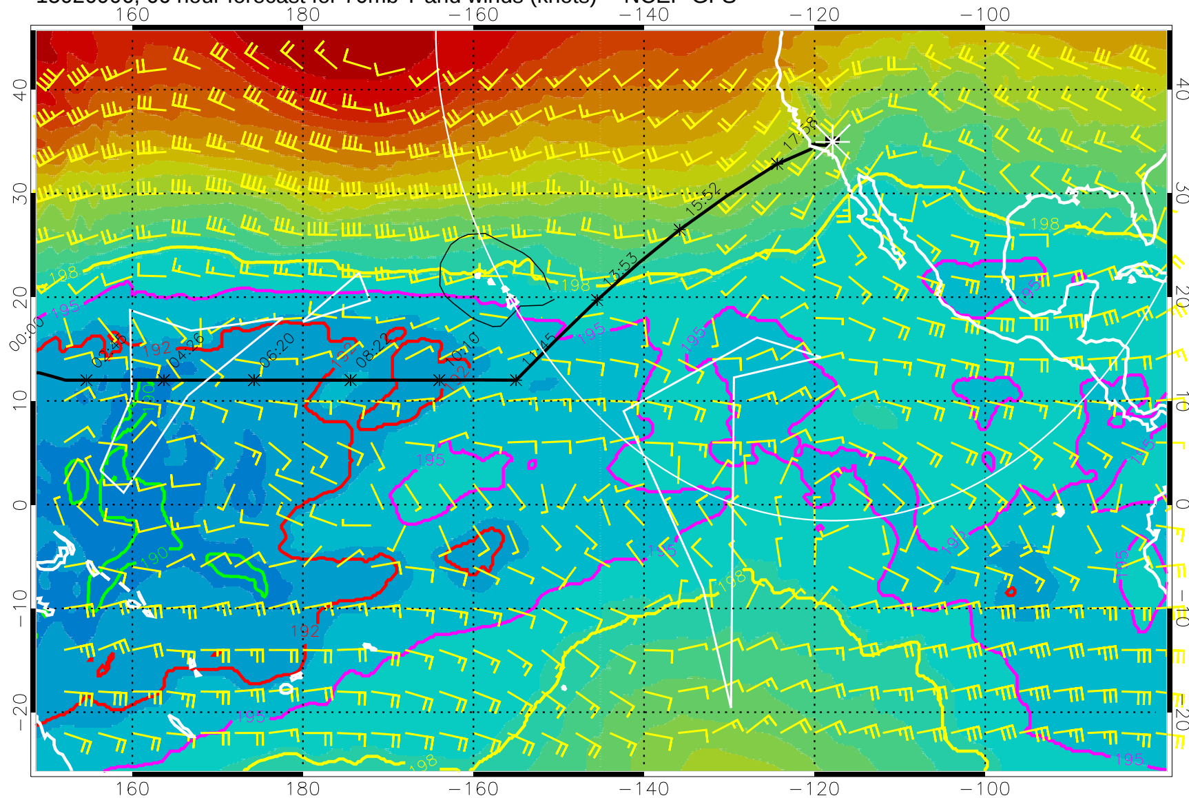
15020906, 66 hour forecast for 70mb T and winds (knots) -- NCEP GFS
