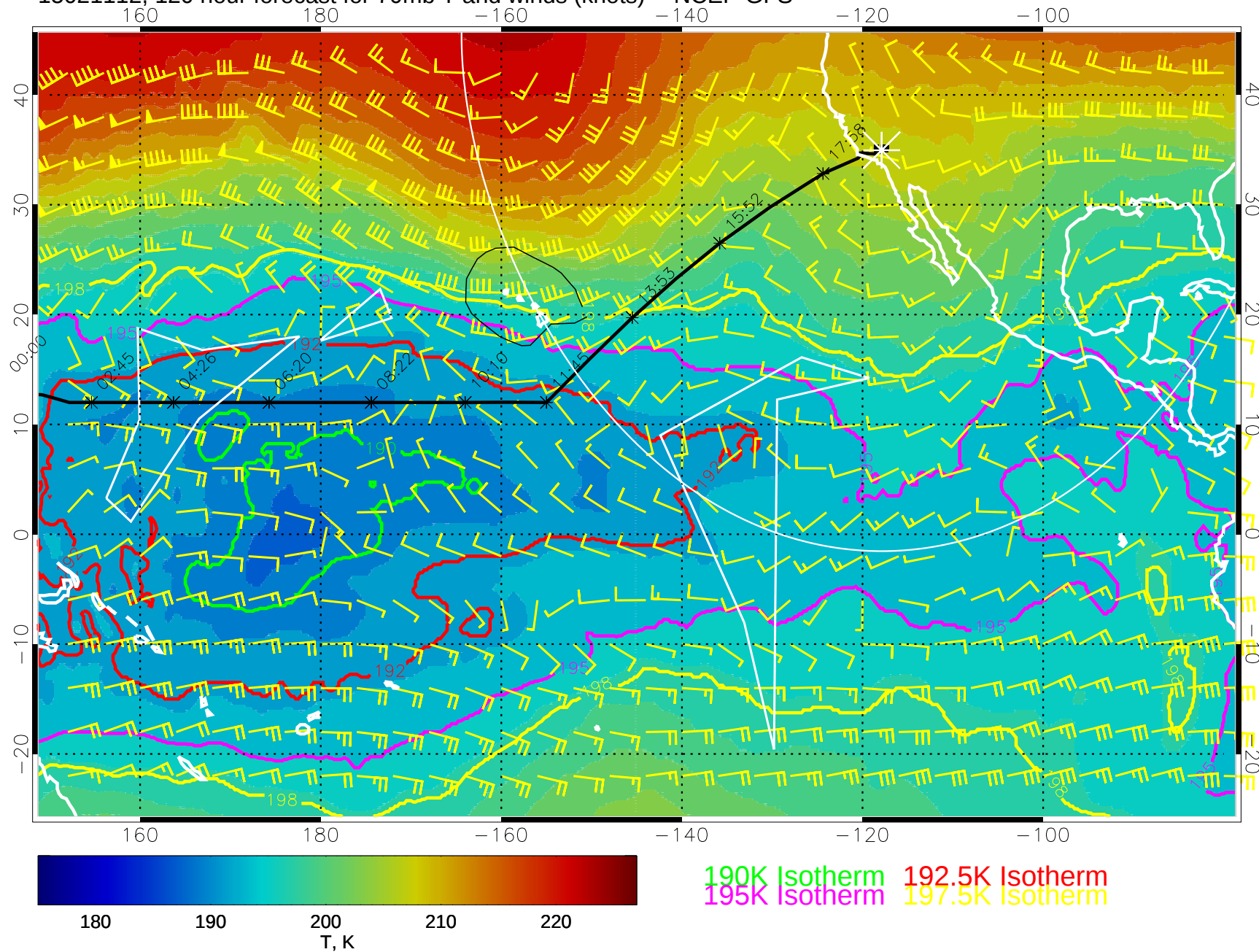
15021112, 120 hour forecast for 70mb T and winds (knots) -- NCEP GFS
