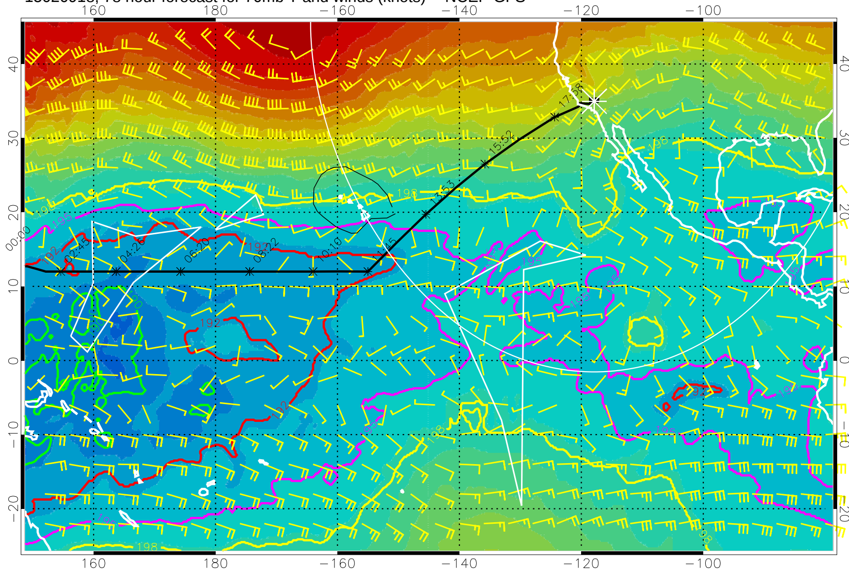
15020918, 78 hour forecast for 70mb T and winds (knots) -- NCEP GFS
