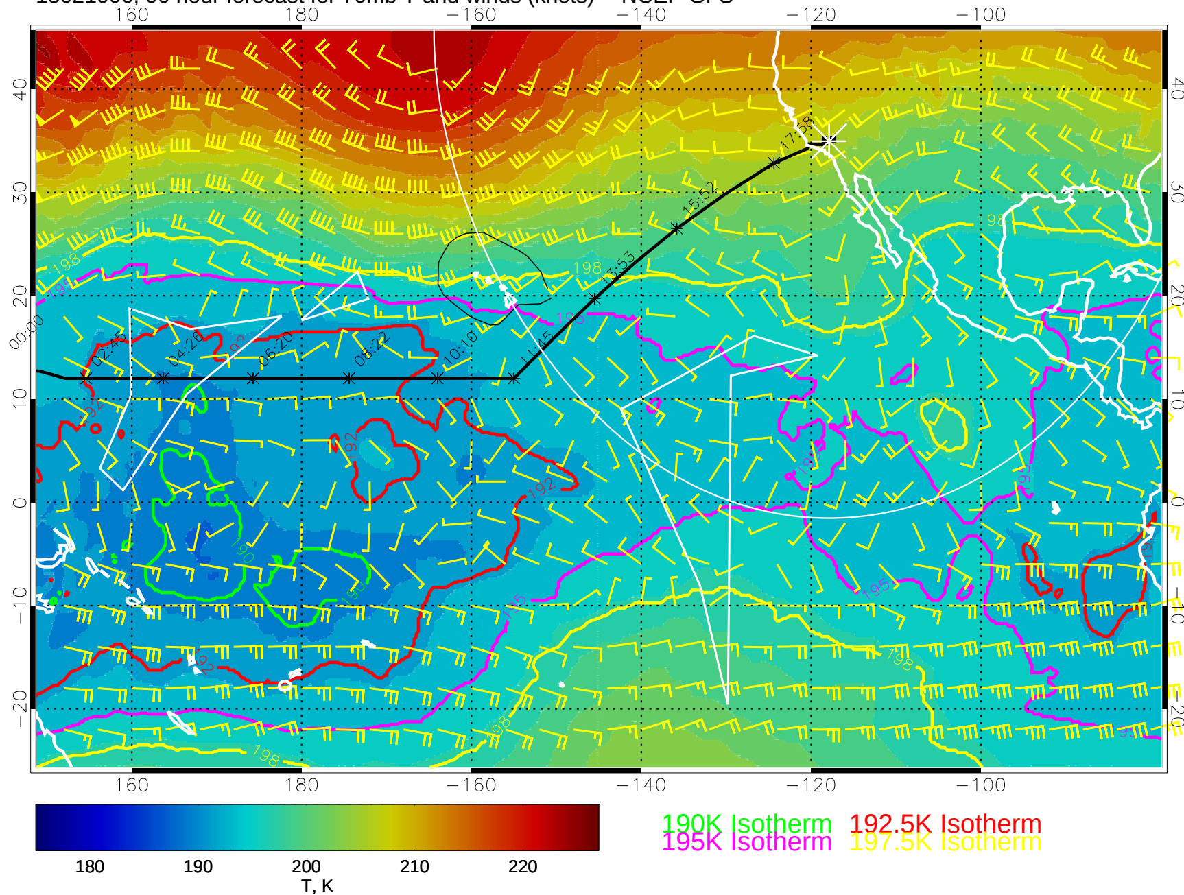
15021006, 90 hour forecast for 70mb T and winds (knots) -- NCEP GFS
