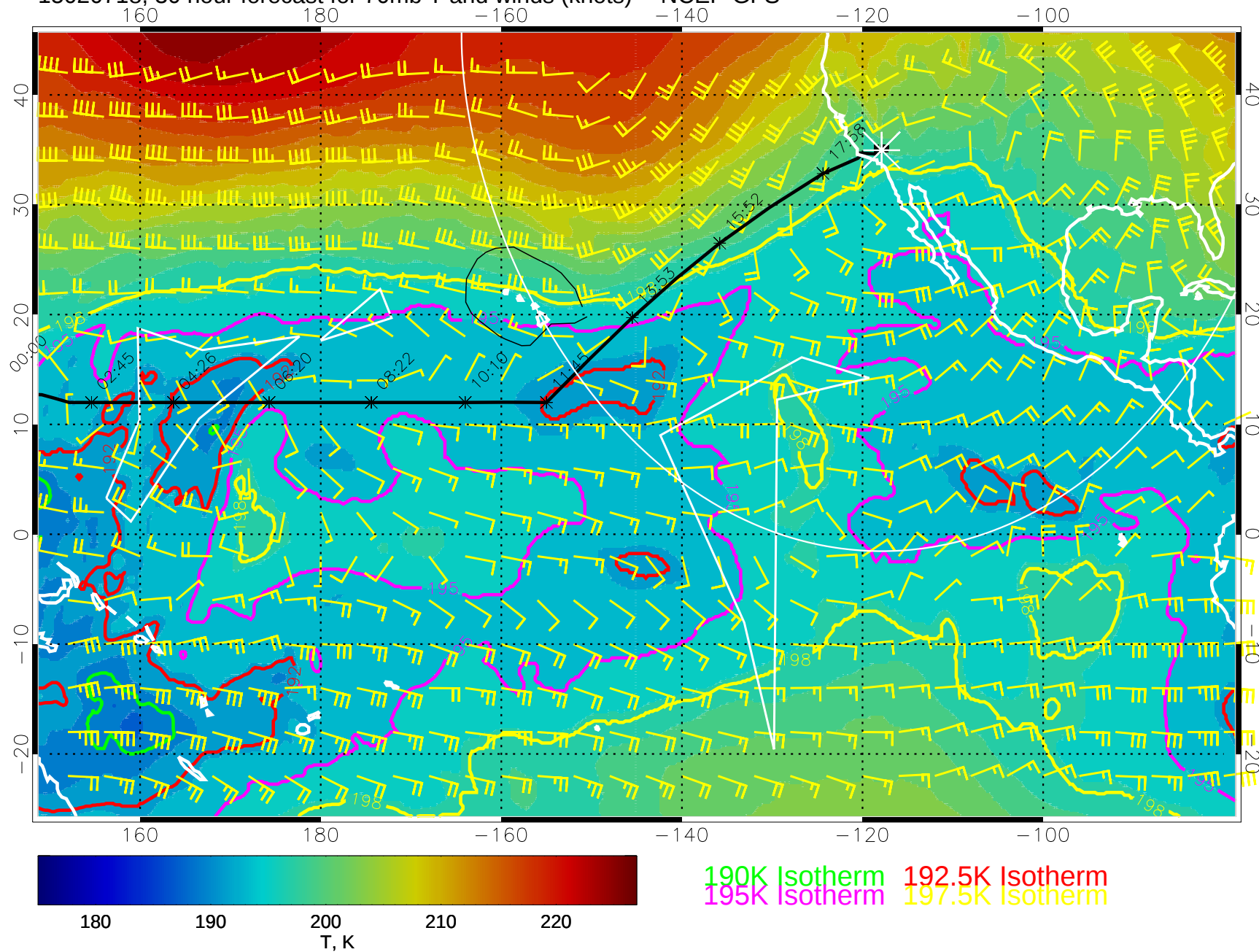
15020718, 30 hour forecast for 70mb T and winds (knots) -- NCEP GFS
