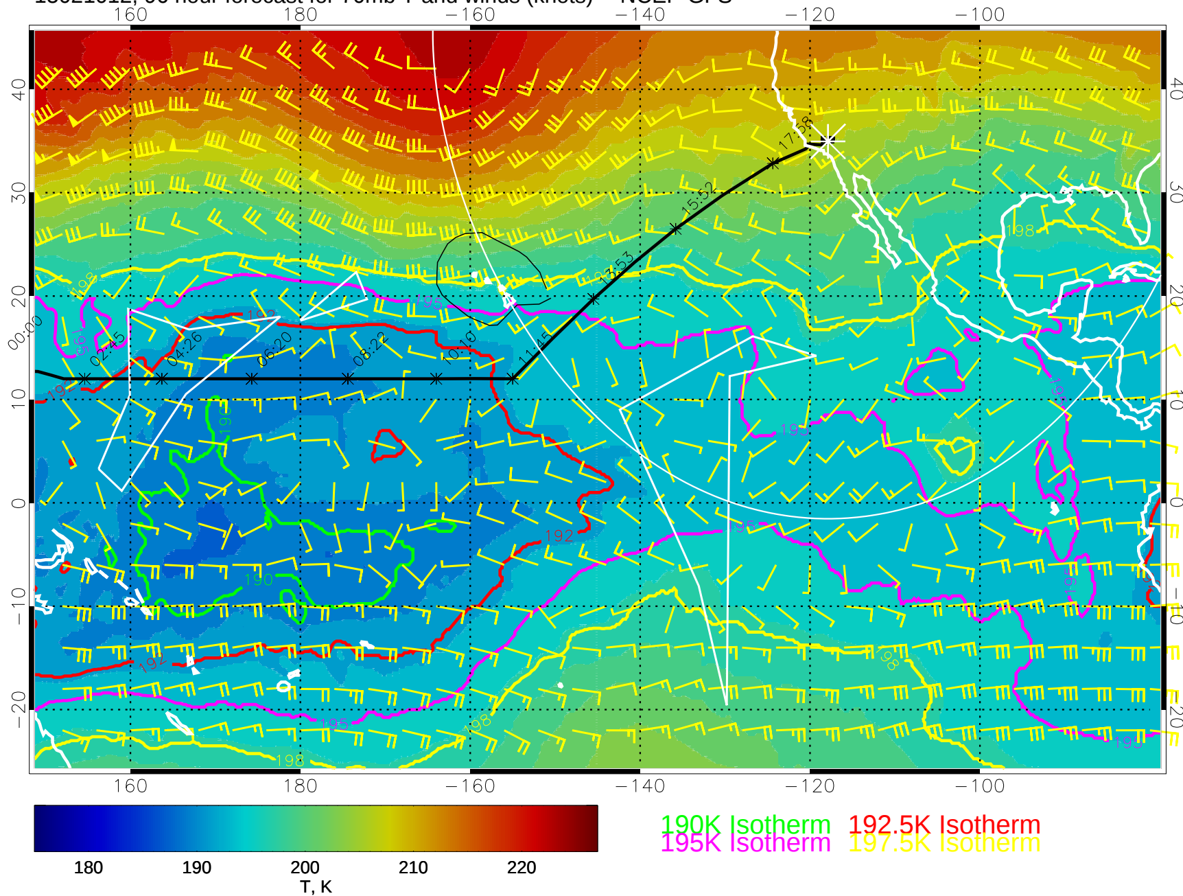
15021012, 96 hour forecast for 70mb T and winds (knots) -- NCEP GFS
