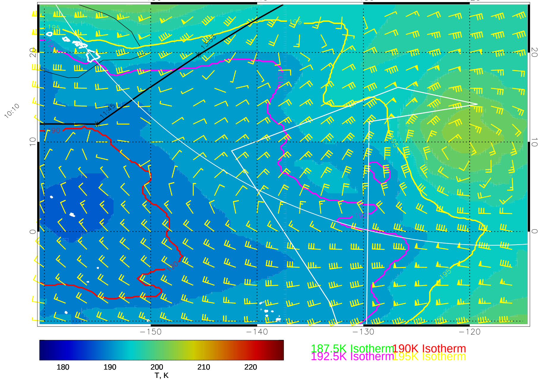
15020700, 12 hour forecast for 100mb T and winds (knots) -- NCEP GFS
