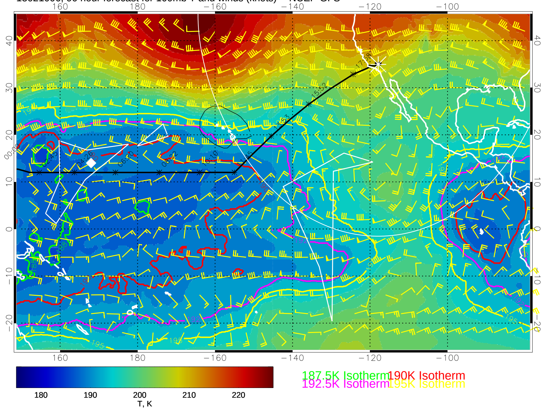
15021006, 90 hour forecast for 100mb T and winds (knots) -- NCEP GFS
