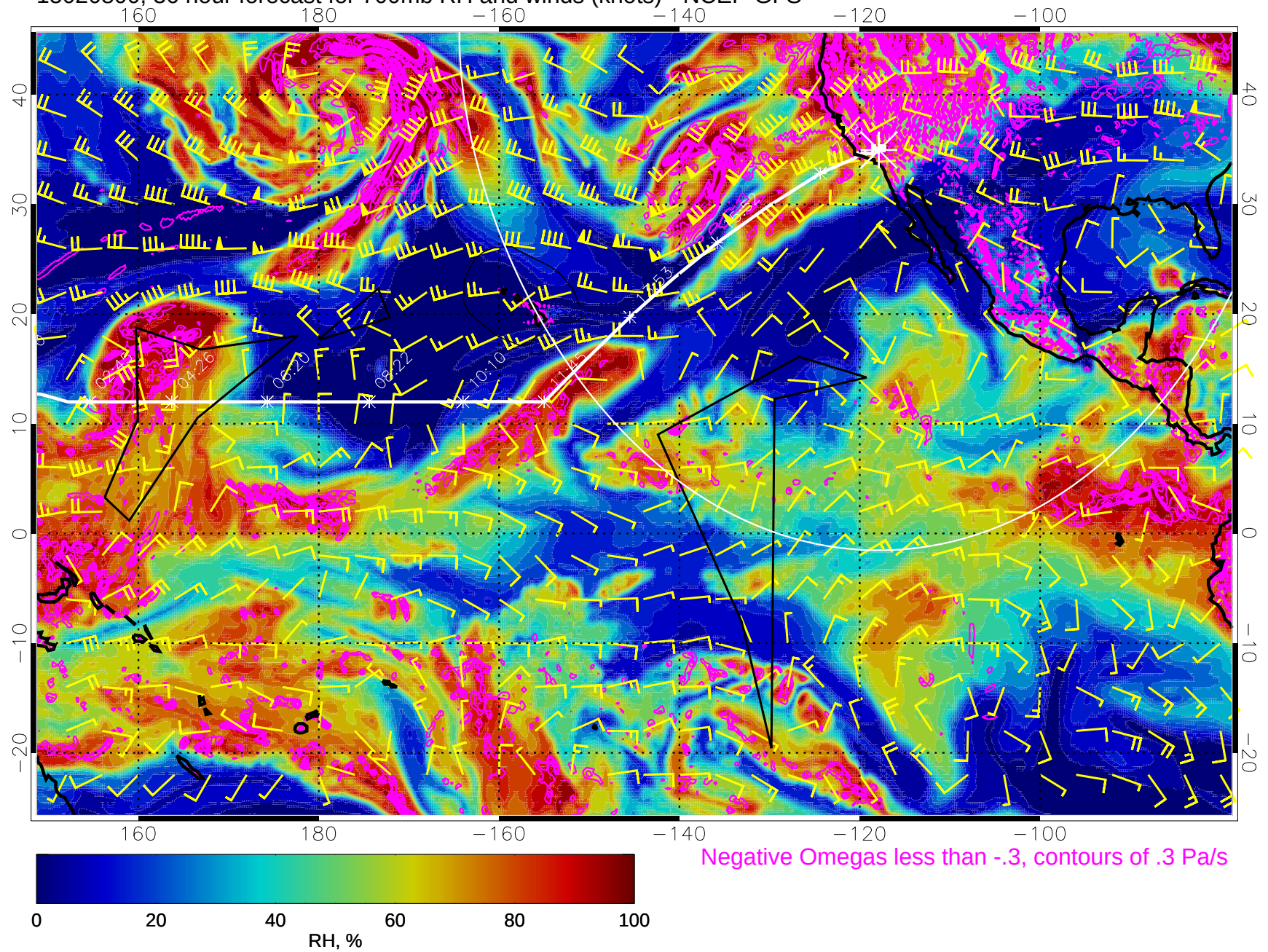
15020800, 36 hour forecast for 700mb RH and winds (knots) - NCEP GFS
