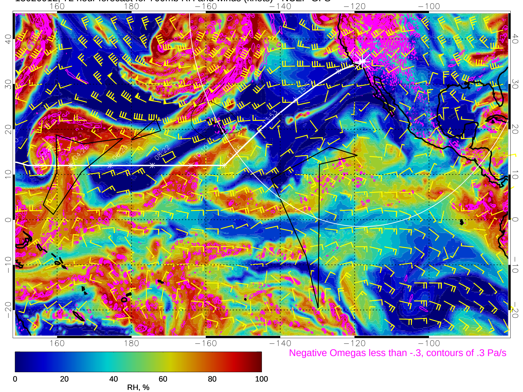
15020912, 72 hour forecast for 700mb RH and winds (knots) - NCEP GFS
