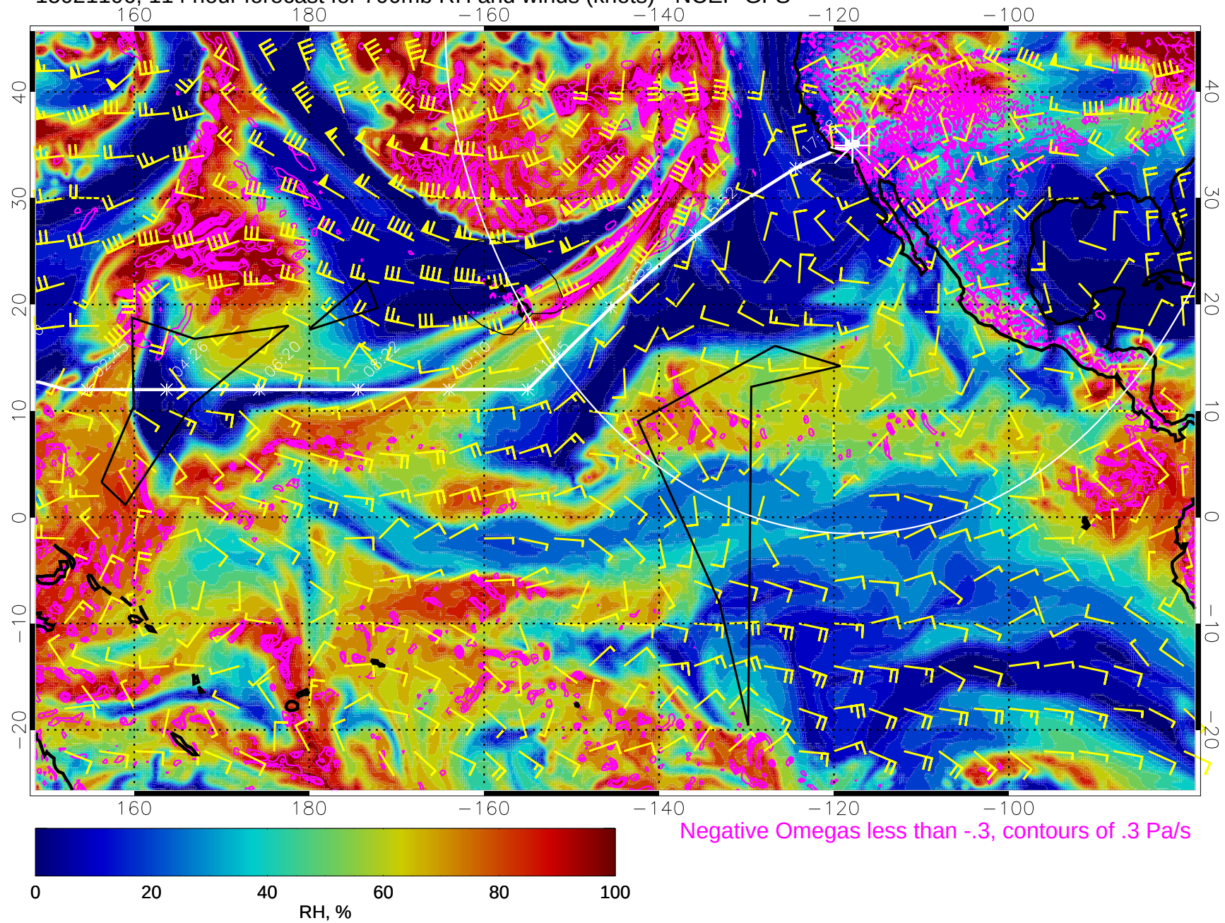
15021106, 114 hour forecast for 700mb RH and winds (knots) - NCEP GFS
