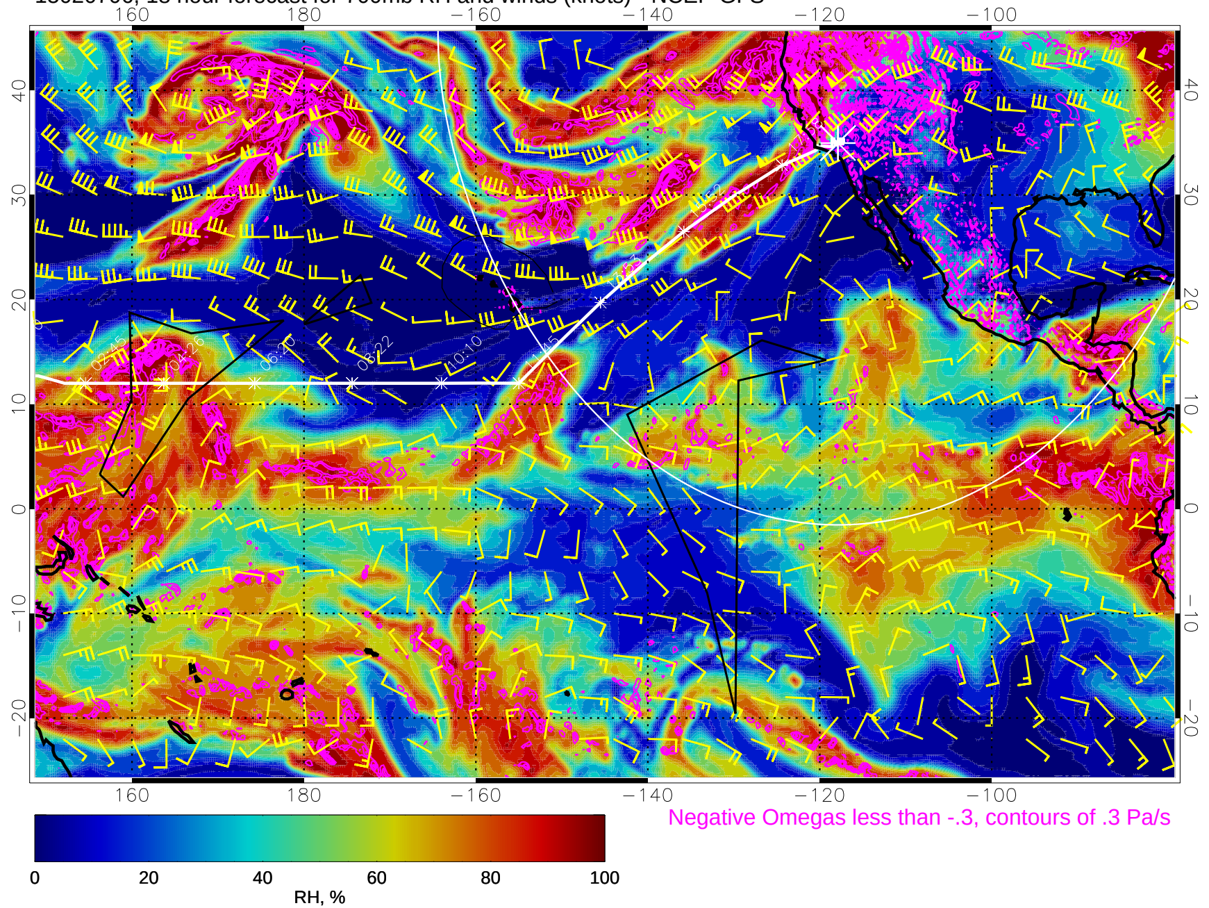
15020706, 18 hour forecast for 700mb RH and winds (knots) - NCEP GFS
