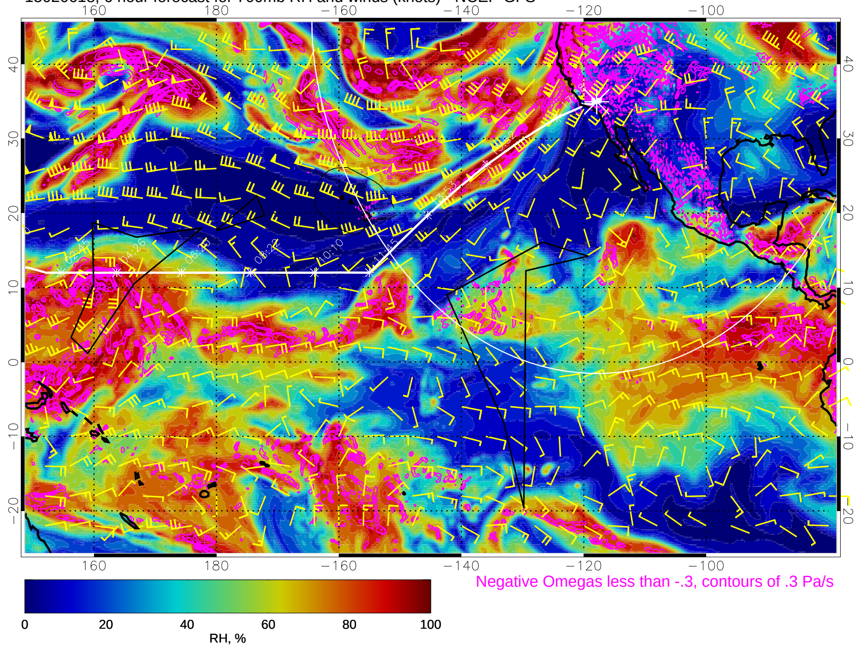
15020618, 6 hour forecast for 700mb RH and winds (knots) - NCEP GFS
