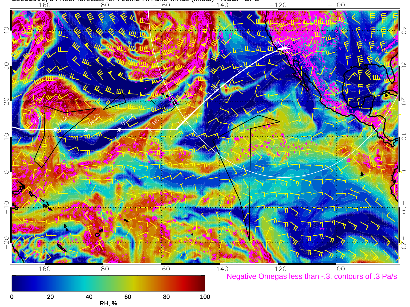
15021000, 84 hour forecast for 700mb RH and winds (knots) - NCEP GFS
