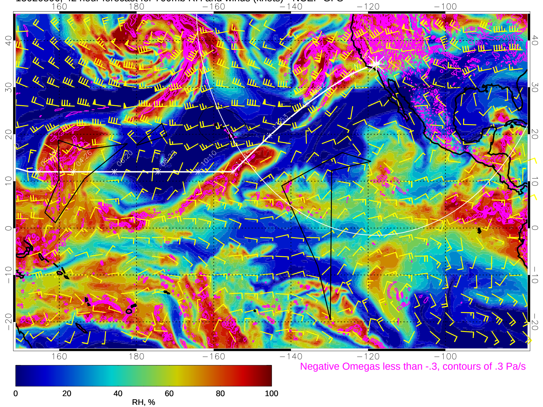
15020806, 42 hour forecast for 700mb RH and winds (knots) - NCEP GFS
