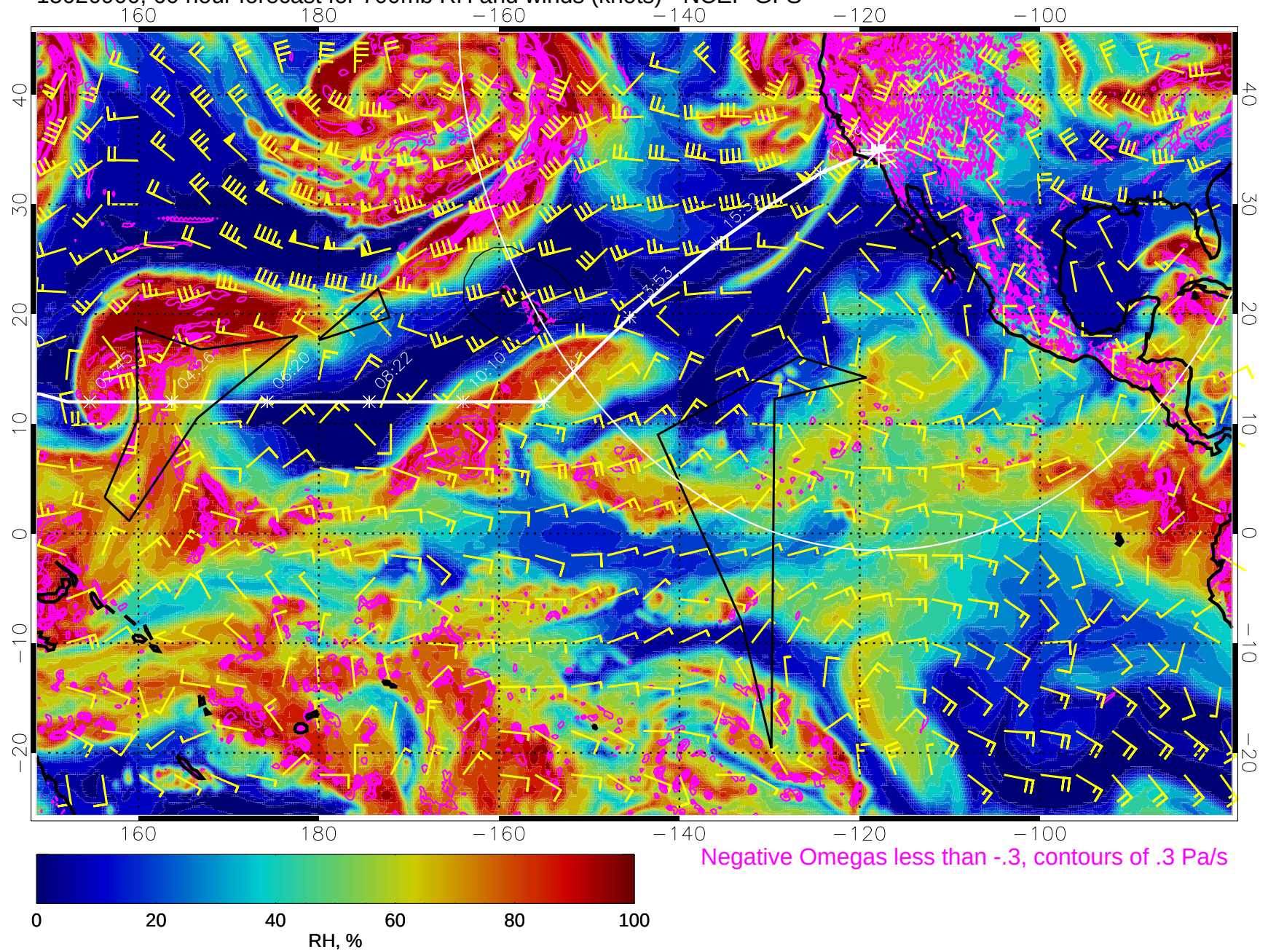
15020900, 60 hour forecast for 700mb RH and winds (knots) - NCEP GFS
