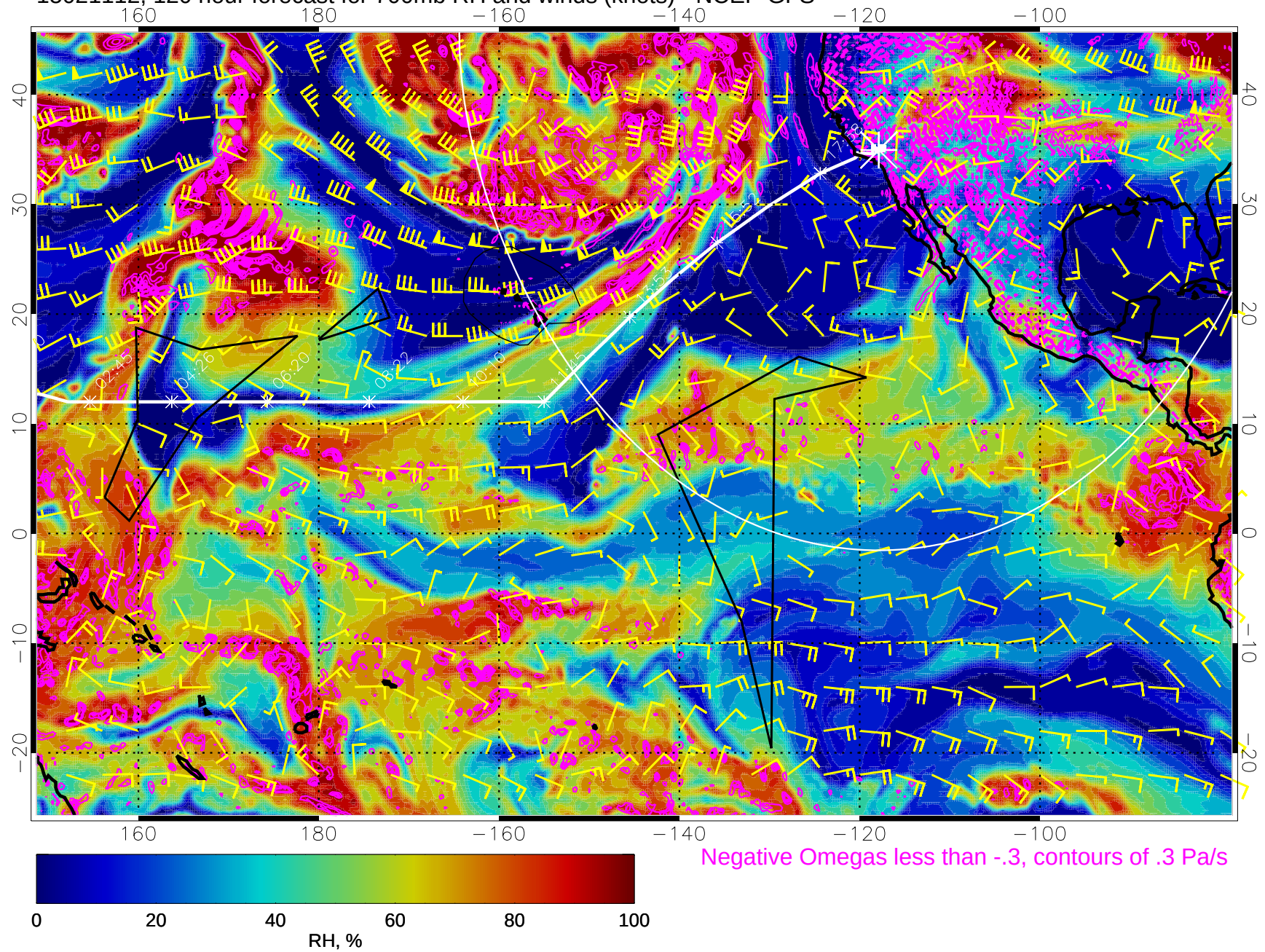
15021112, 120 hour forecast for 700mb RH and winds (knots) - NCEP GFS
