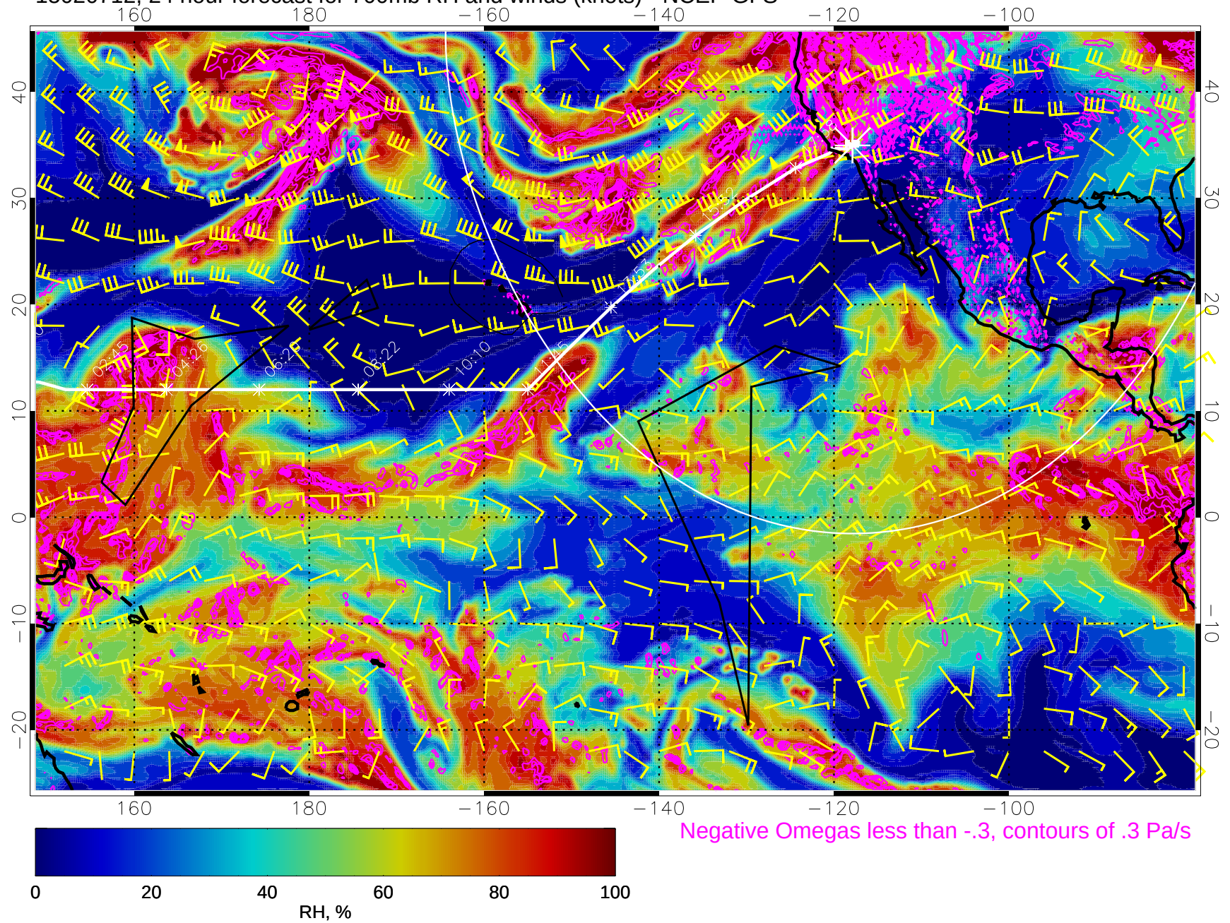
15020712, 24 hour forecast for 700mb RH and winds (knots) - NCEP GFS
