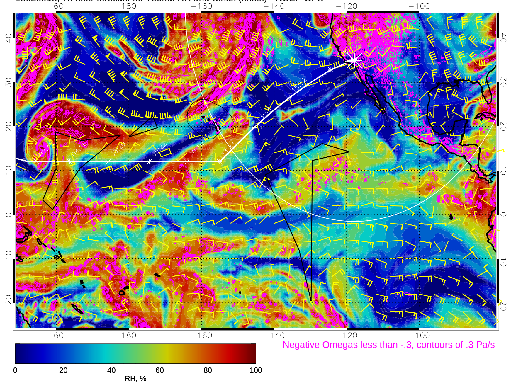
15020918, 78 hour forecast for 700mb RH and winds (knots) - NCEP GFS
