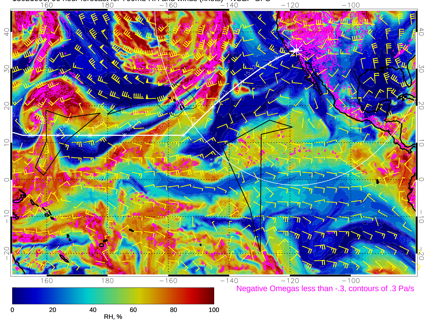
15021006, 90 hour forecast for 700mb RH and winds (knots) - NCEP GFS
