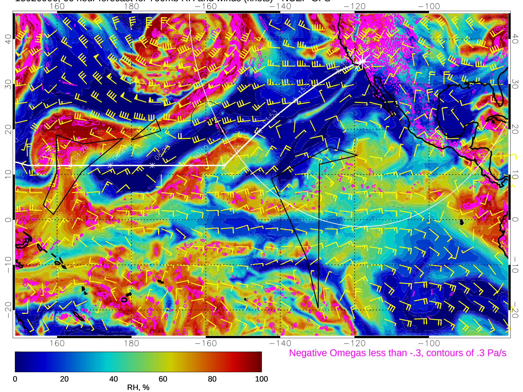
15020906, 66 hour forecast for 700mb RH and winds (knots) - NCEP GFS
