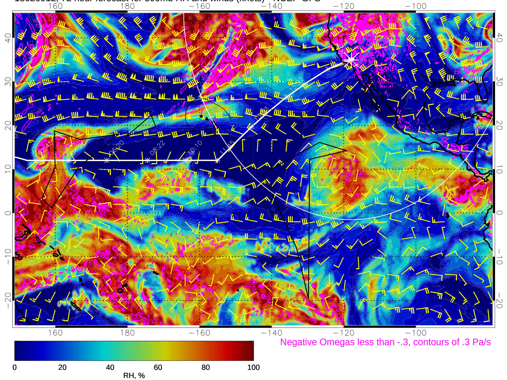
15020912, 72 hour forecast for 500mb RH and winds (knots) - NCEP GFS
