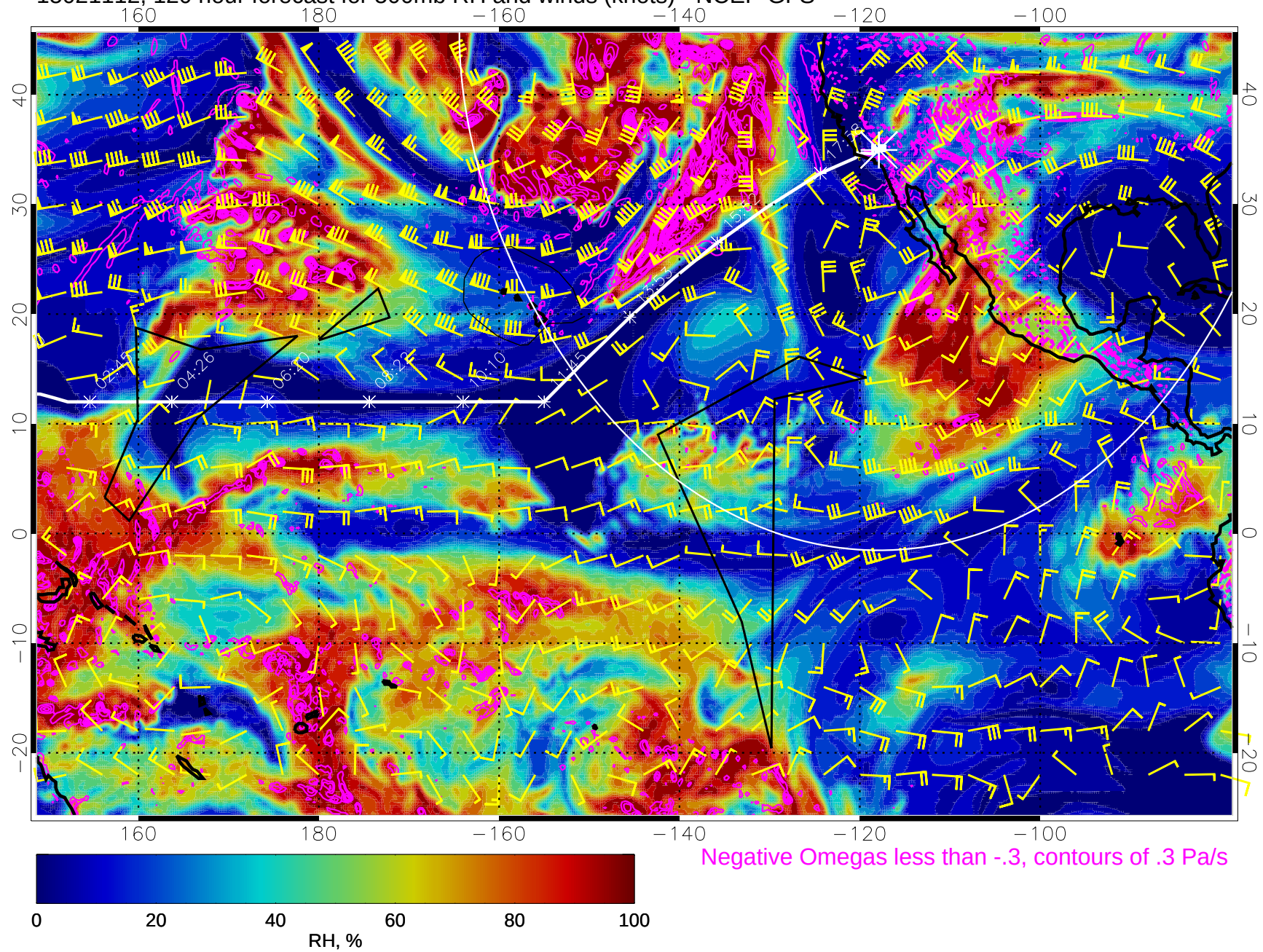
15021112, 120 hour forecast for 500mb RH and winds (knots) - NCEP GFS
