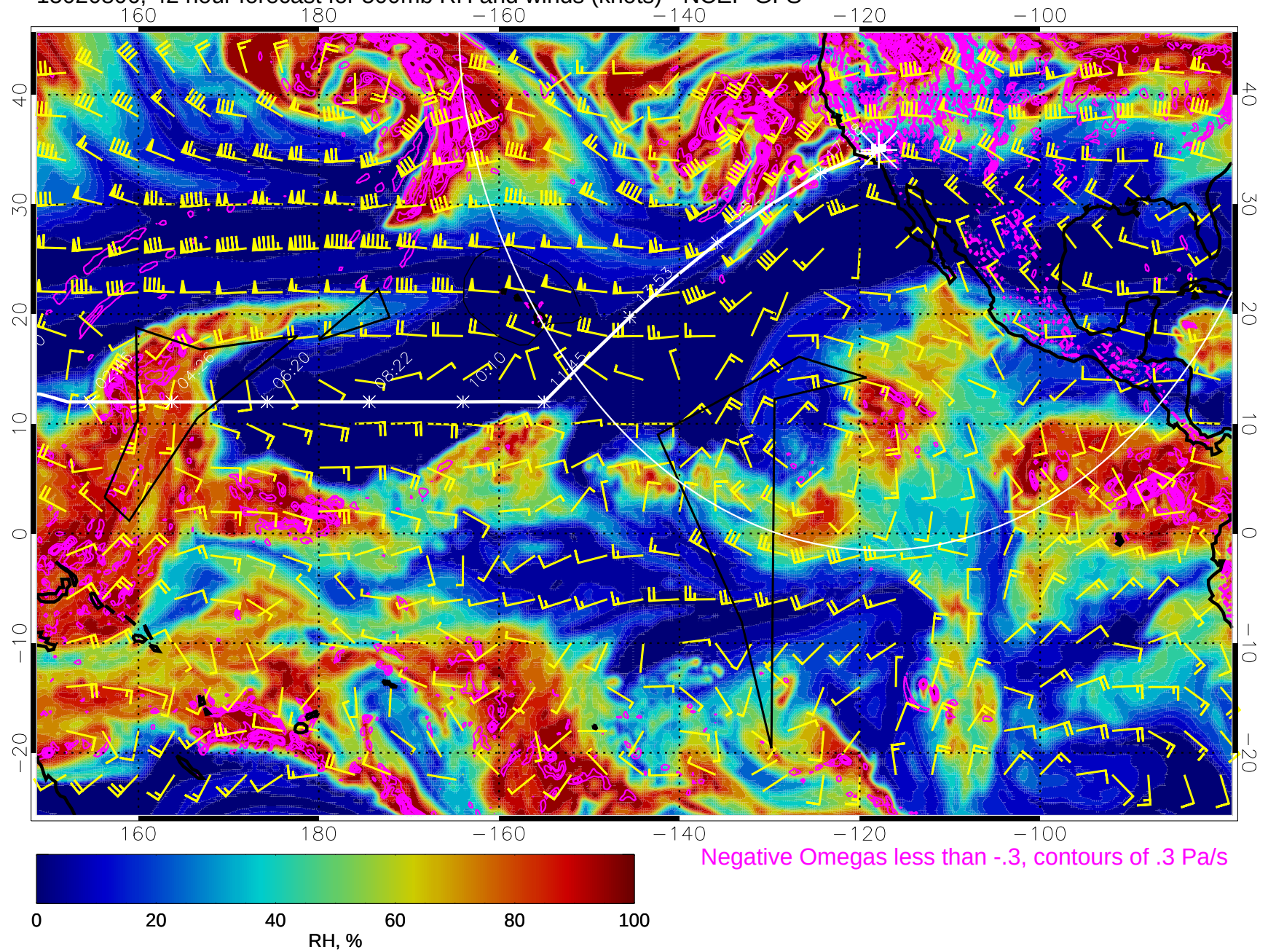
15020806, 42 hour forecast for 500mb RH and winds (knots) - NCEP GFS
