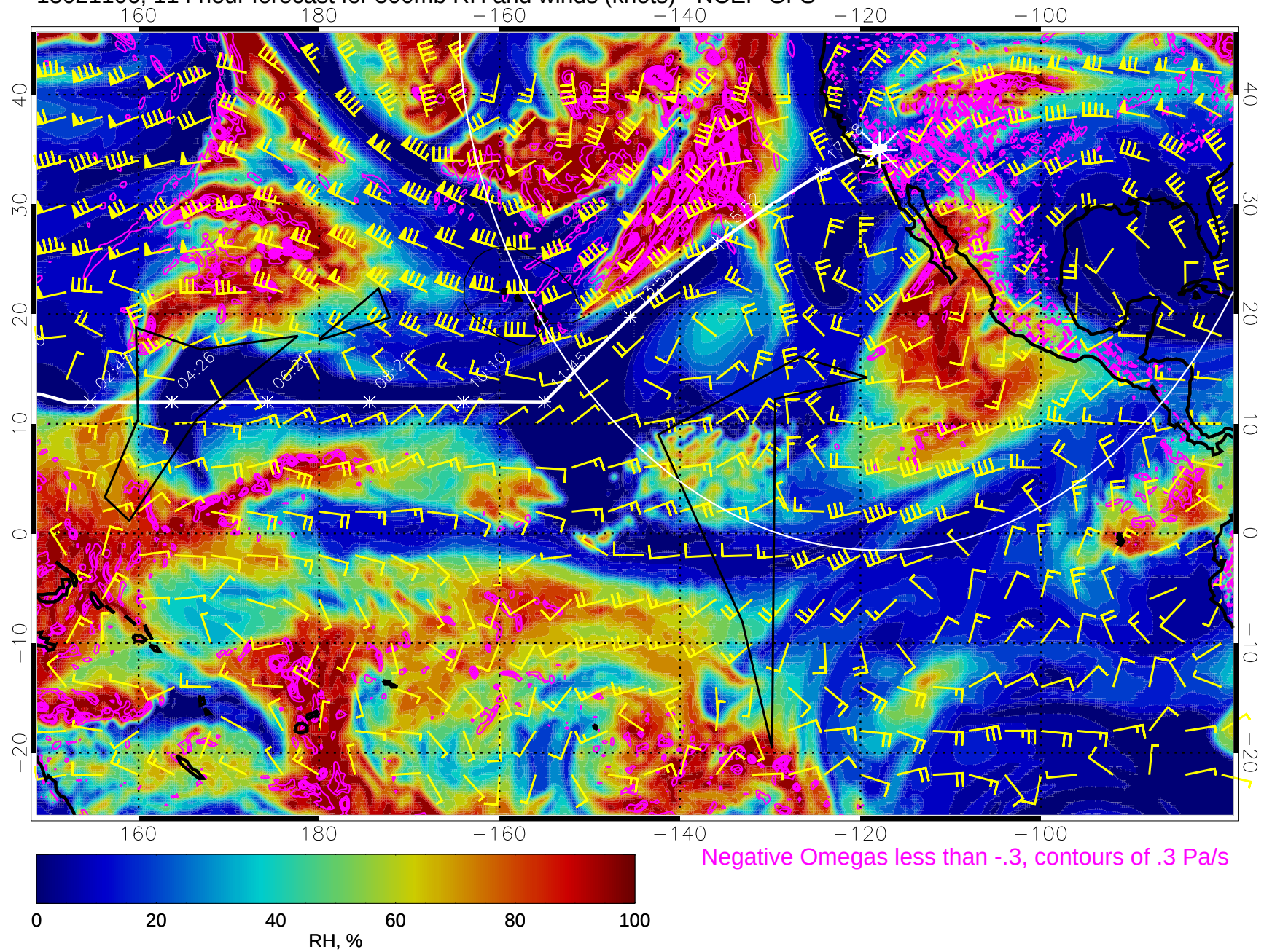
15021106, 114 hour forecast for 500mb RH and winds (knots) - NCEP GFS
