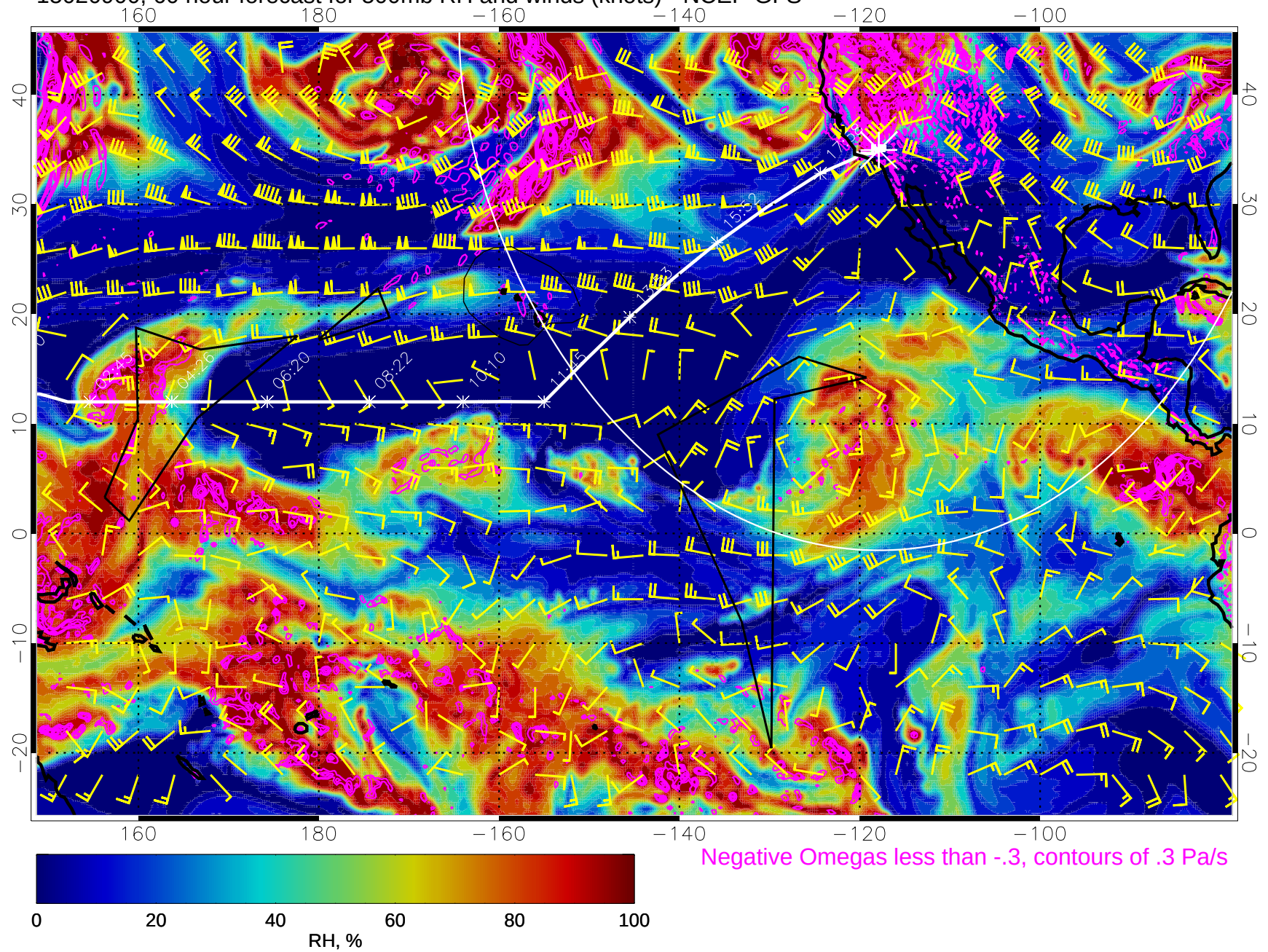
15020900, 60 hour forecast for 500mb RH and winds (knots) - NCEP GFS
