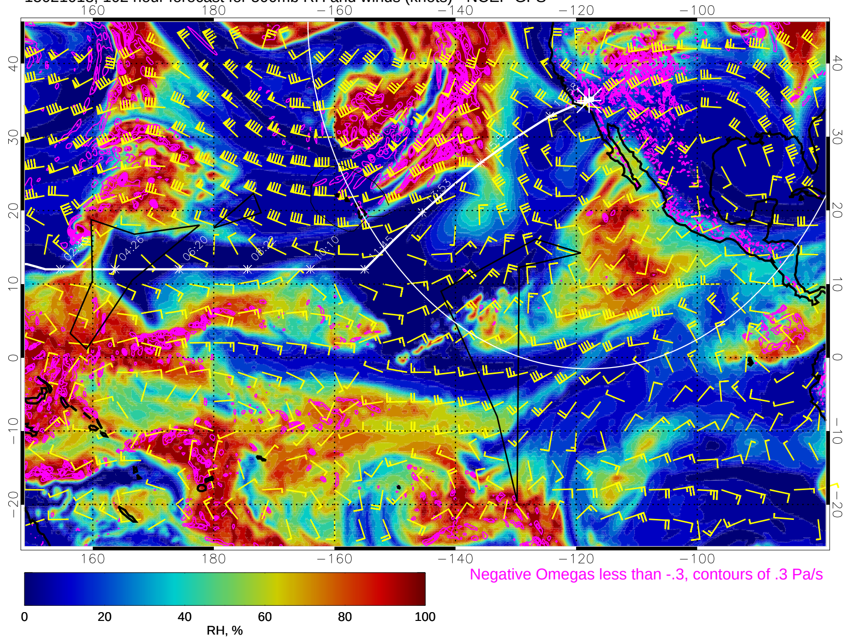
15021018, 102 hour forecast for 500mb RH and winds (knots) - NCEP GFS
