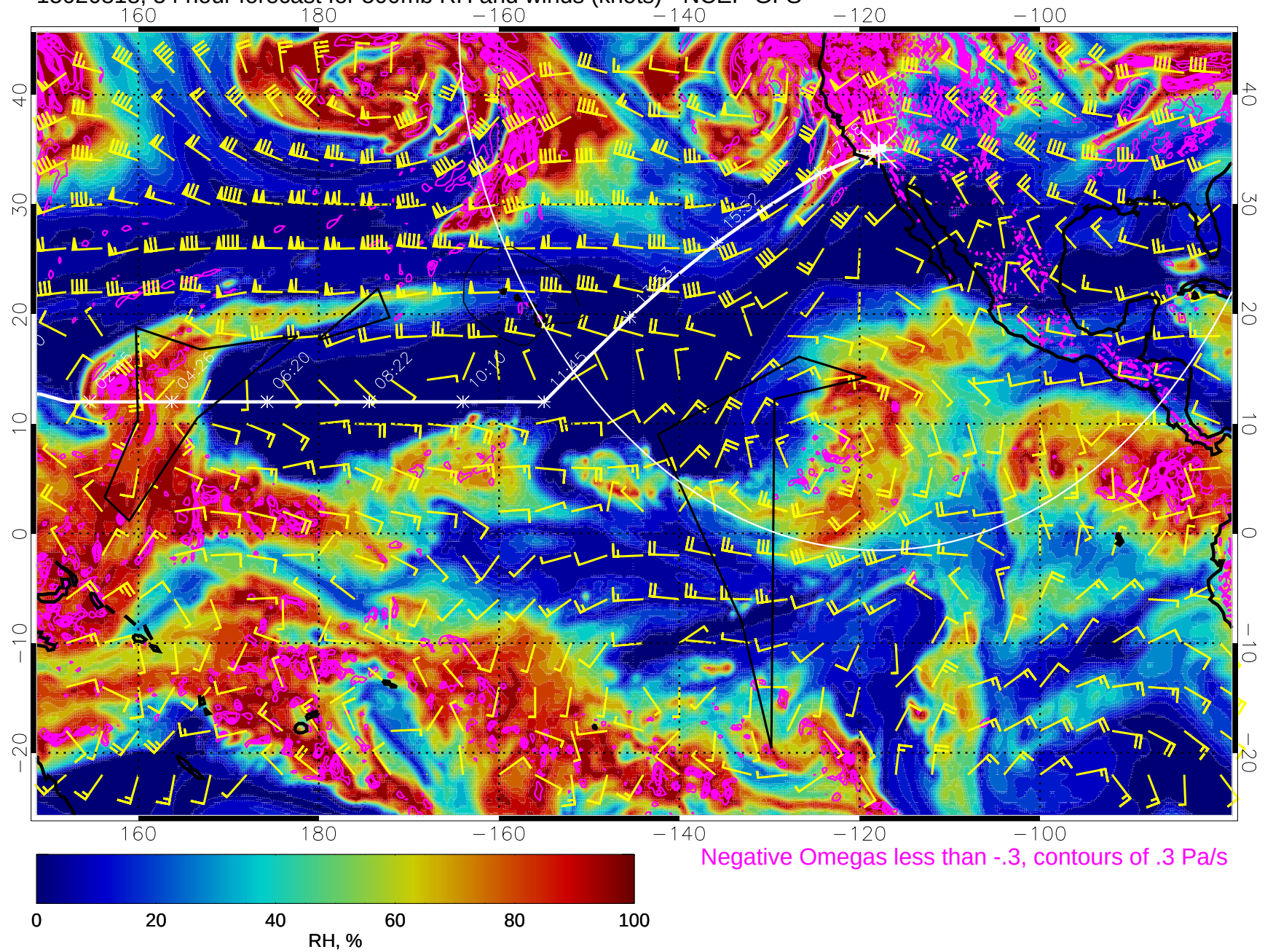
15020818, 54 hour forecast for 500mb RH and winds (knots) - NCEP GFS
