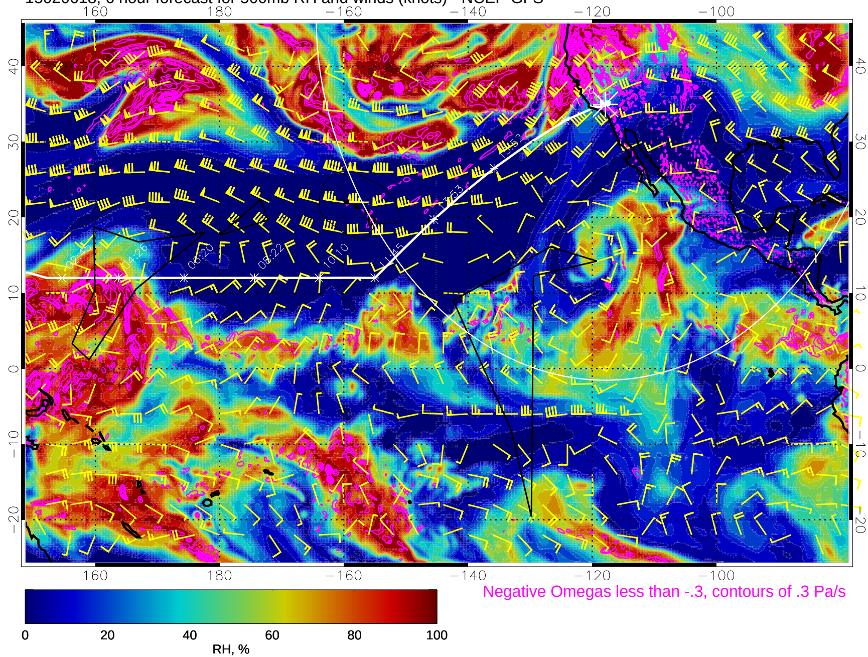
15020618, 6 hour forecast for 500mb RH and winds (knots) - NCEP GFS
