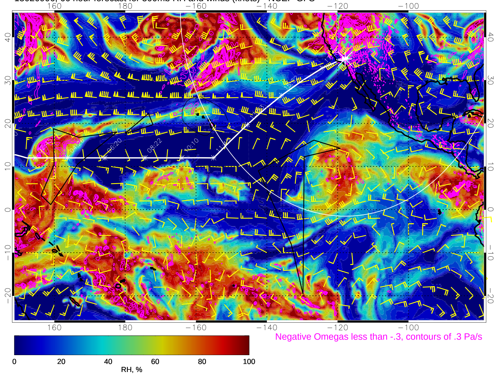
15020906, 66 hour forecast for 500mb RH and winds (knots) - NCEP GFS
