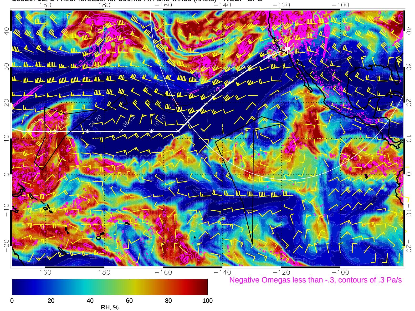
15020712, 24 hour forecast for 500mb RH and winds (knots) - NCEP GFS
