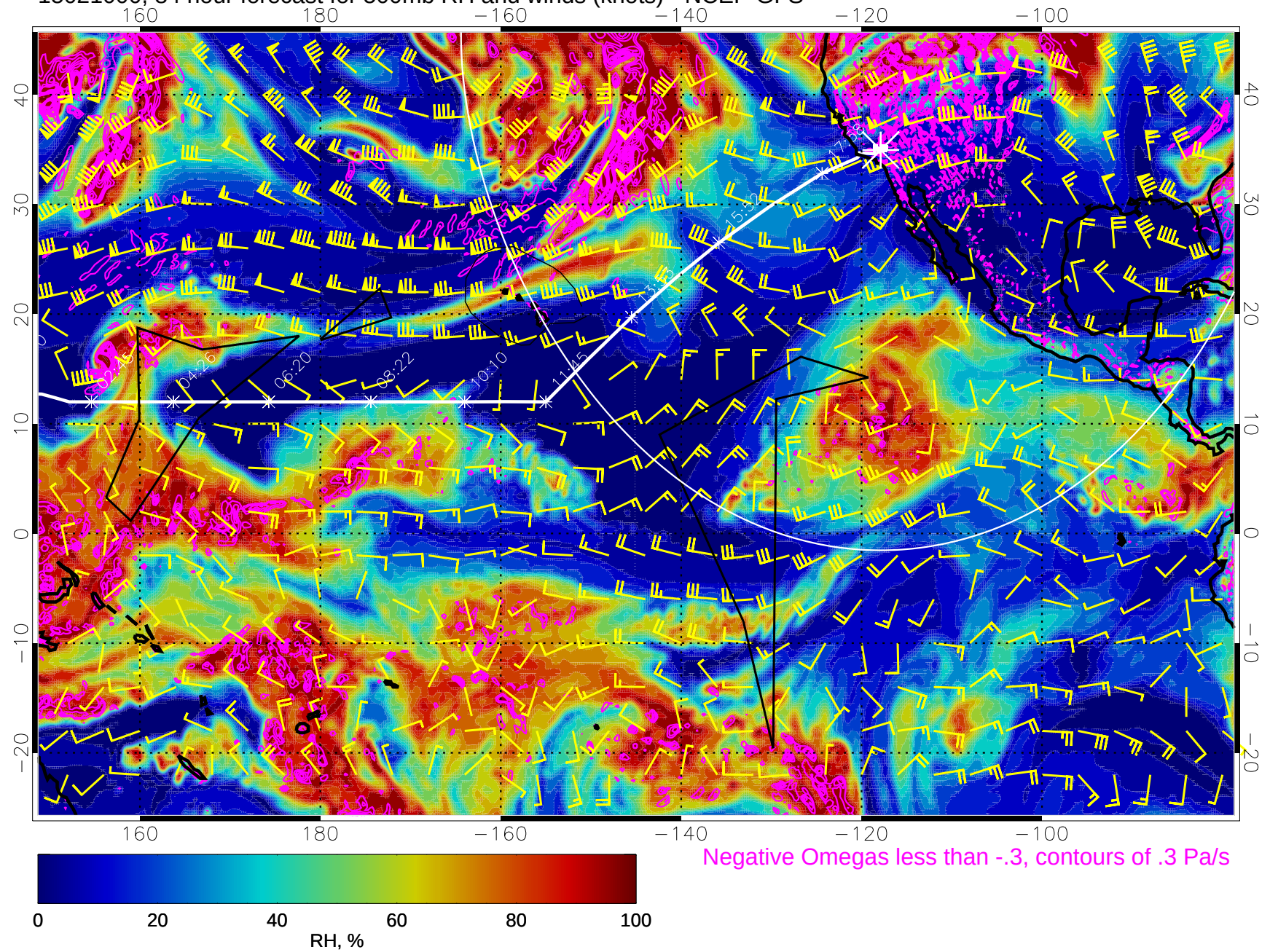
15021000, 84 hour forecast for 500mb RH and winds (knots) - NCEP GFS
