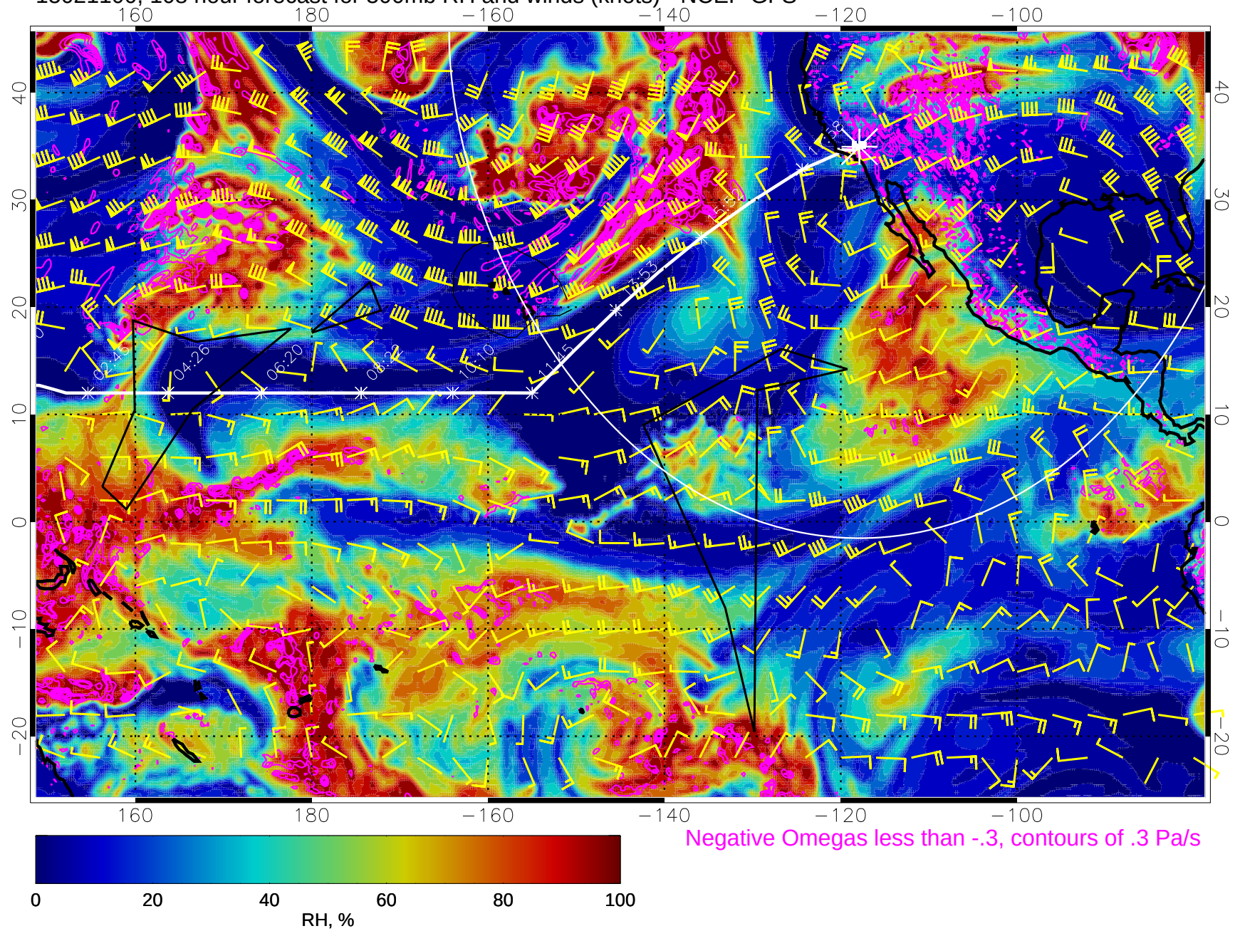
15021100, 108 hour forecast for 500mb RH and winds (knots) - NCEP GFS
