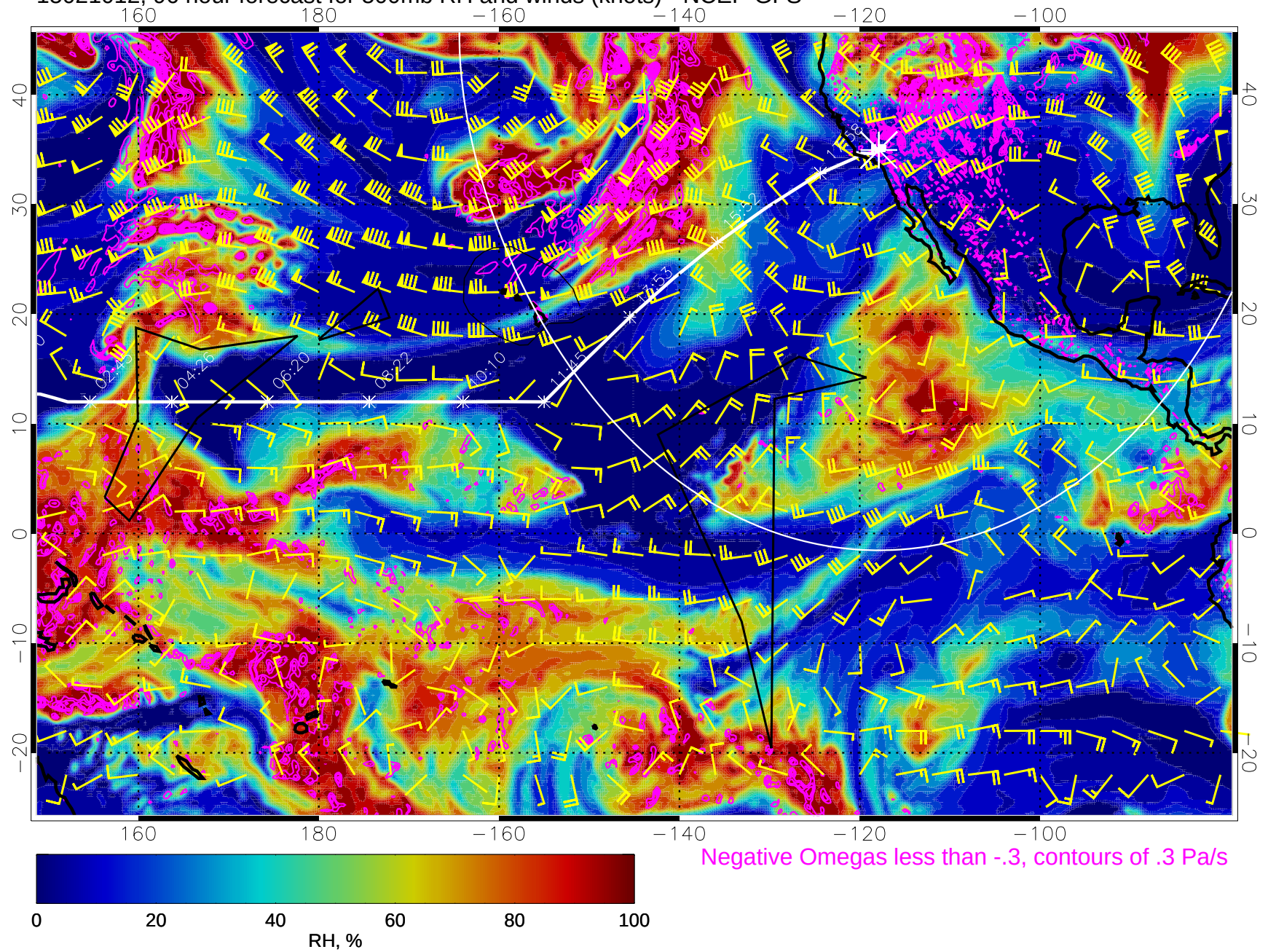
15021012, 96 hour forecast for 500mb RH and winds (knots) - NCEP GFS
