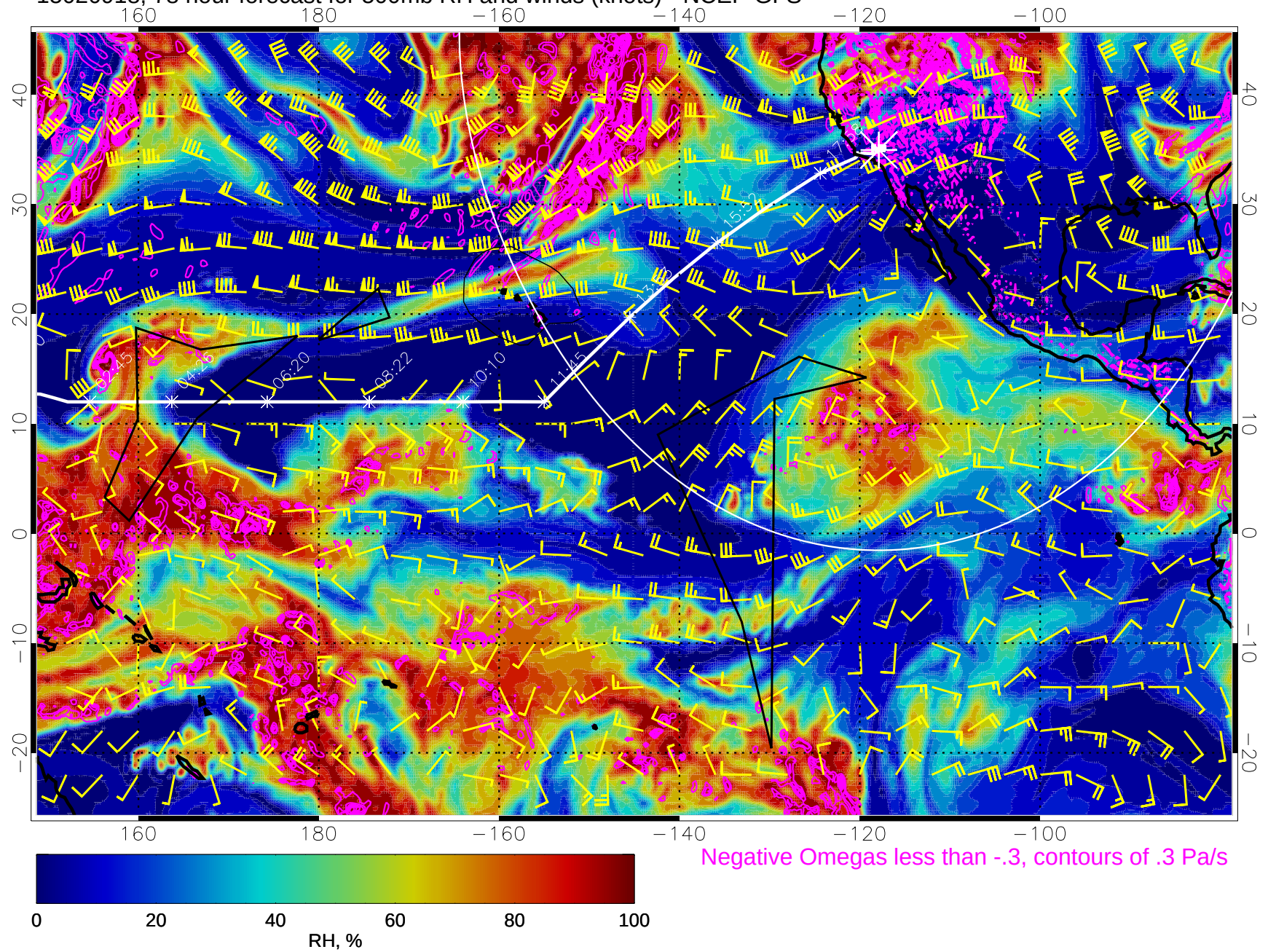
15020918, 78 hour forecast for 500mb RH and winds (knots) - NCEP GFS
